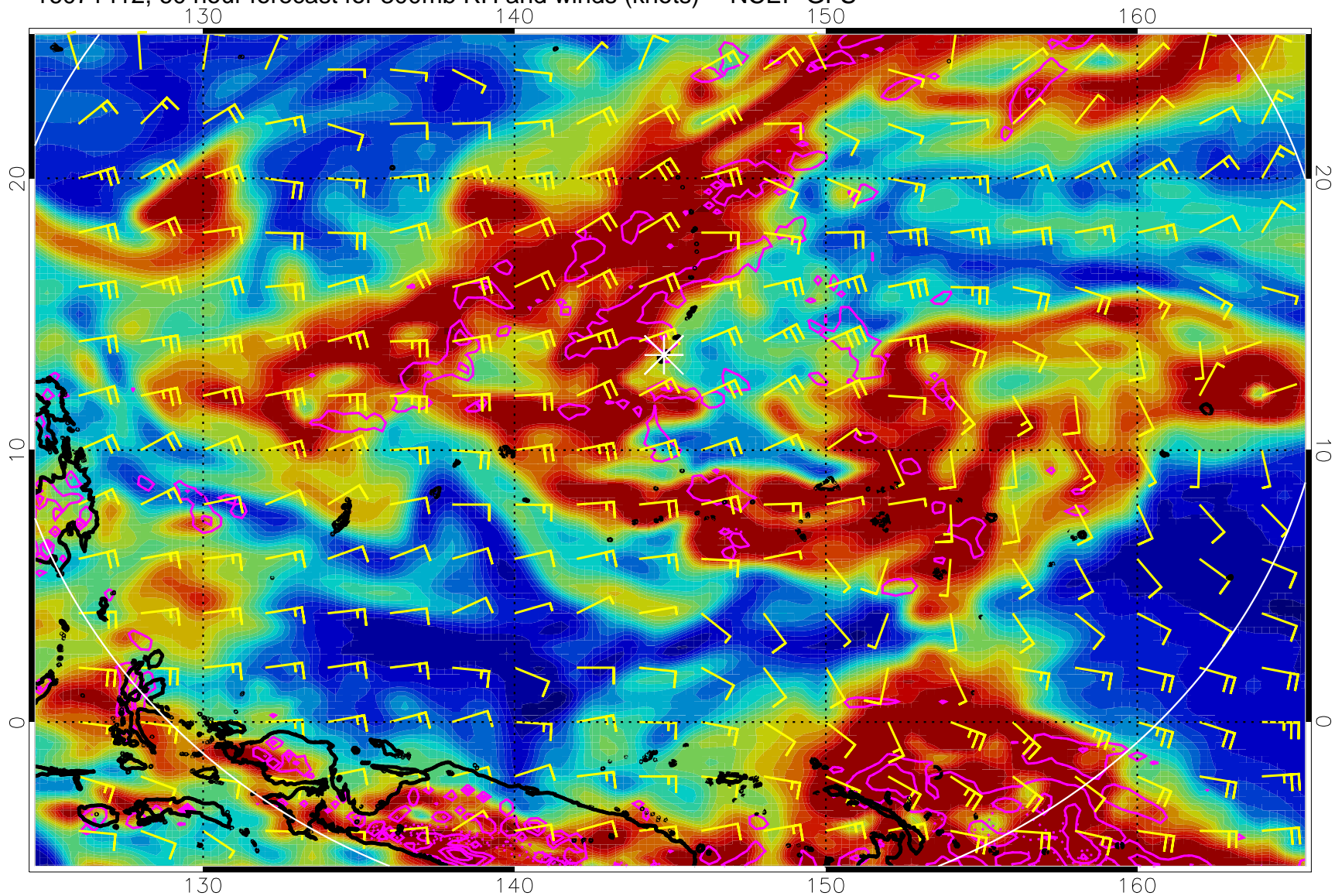
16071412, 60 hour forecast for 300mb RH and winds (knots) -- NCEP GFS
