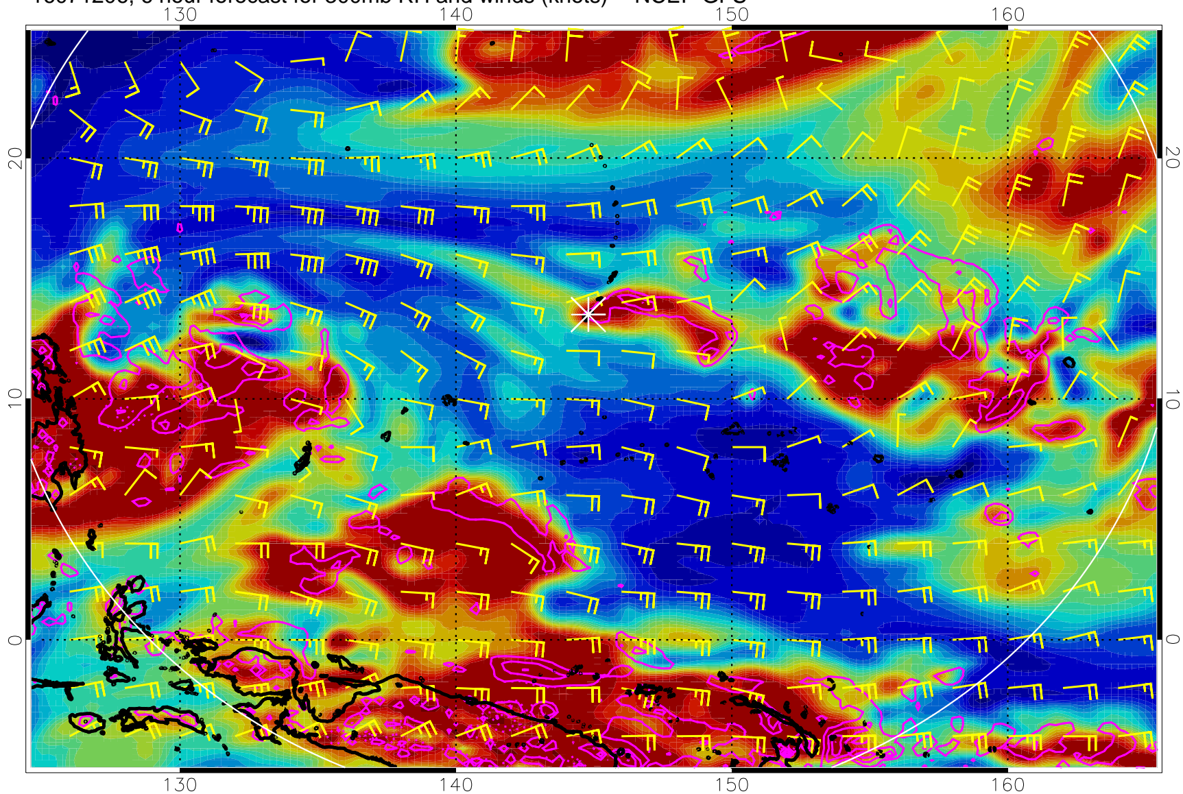
16071206, 6 hour forecast for 300mb RH and winds (knots) -- NCEP GFS
