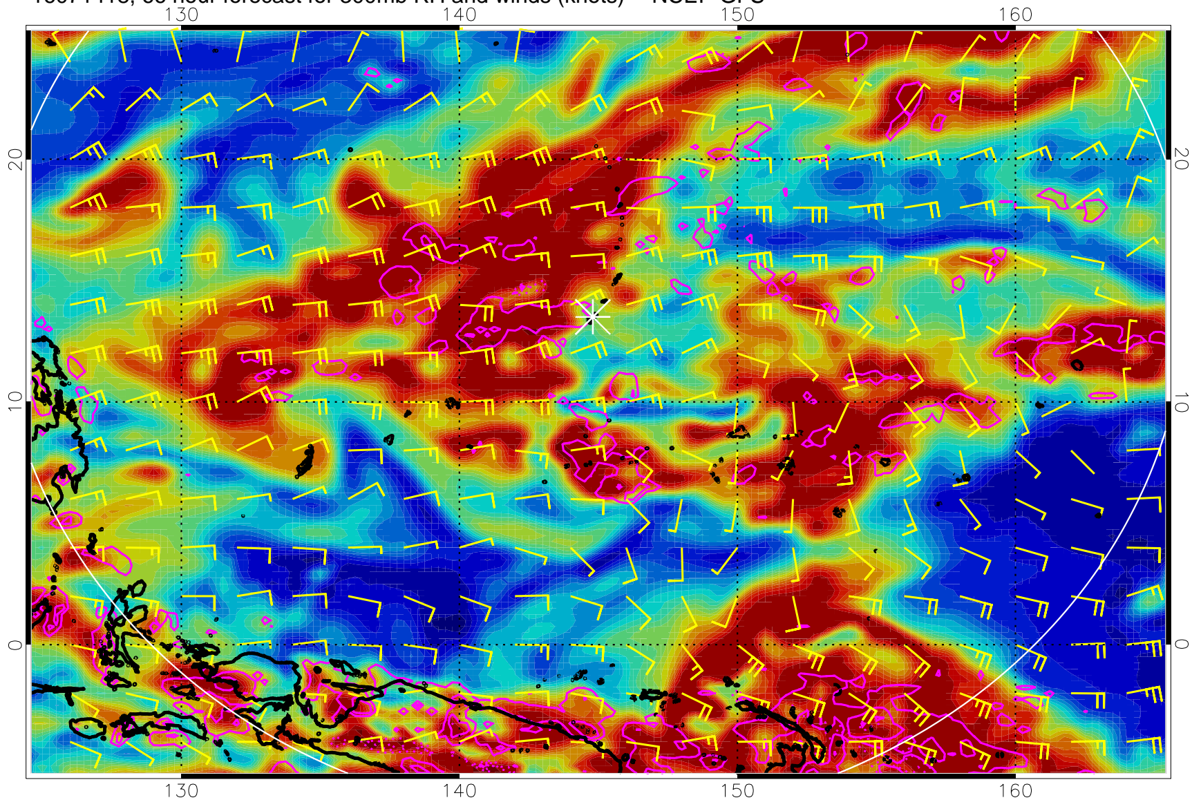
16071418, 66 hour forecast for 300mb RH and winds (knots) -- NCEP GFS
