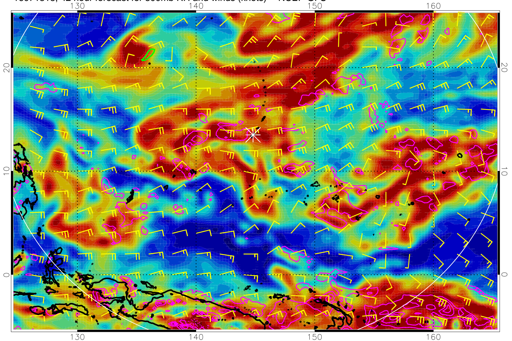
16071318, 42 hour forecast for 300mb RH and winds (knots) -- NCEP GFS
