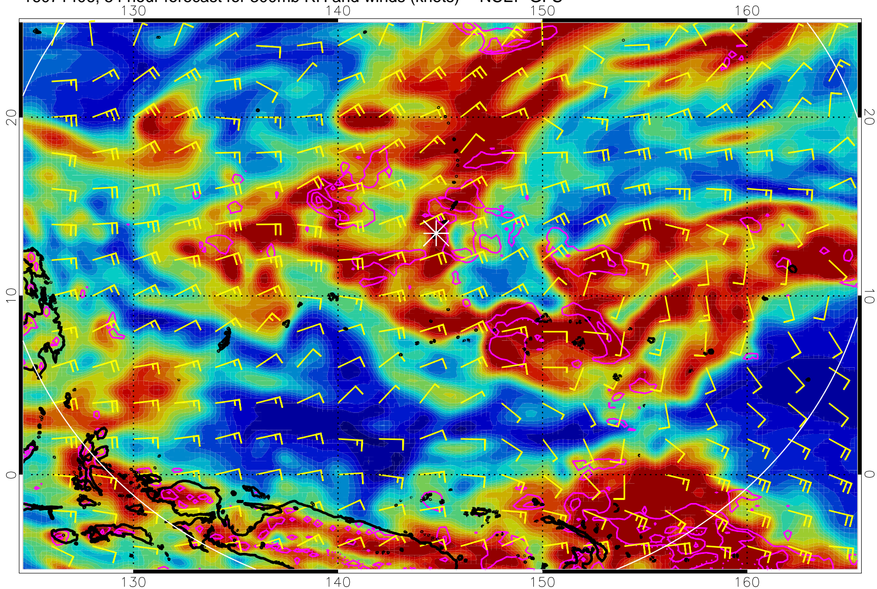
16071406, 54 hour forecast for 300mb RH and winds (knots) -- NCEP GFS
