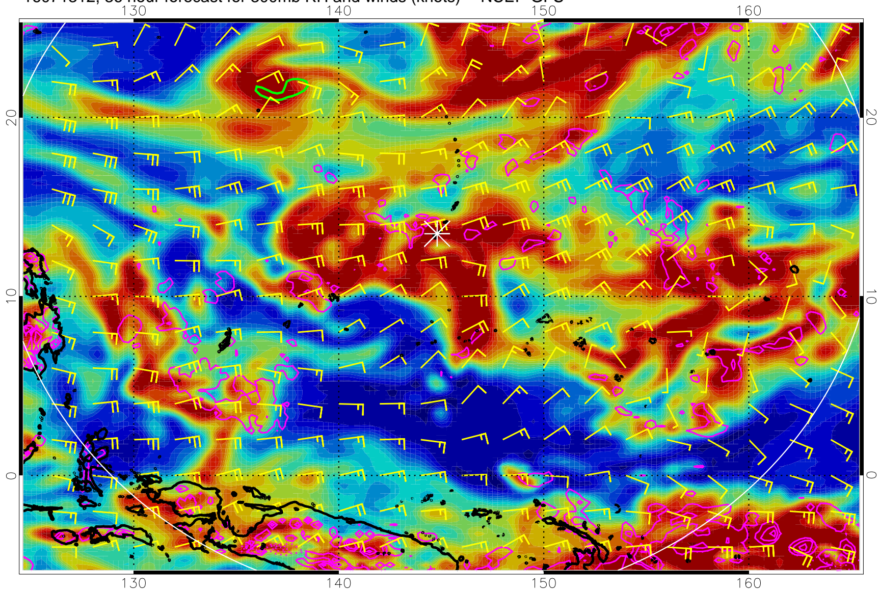
16071312, 36 hour forecast for 300mb RH and winds (knots) -- NCEP GFS
