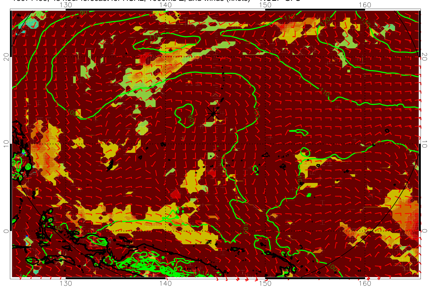
16071400, 48 hour forecast for HCAL, 1000mb Z, and winds (knots) -- NCEP GFS
