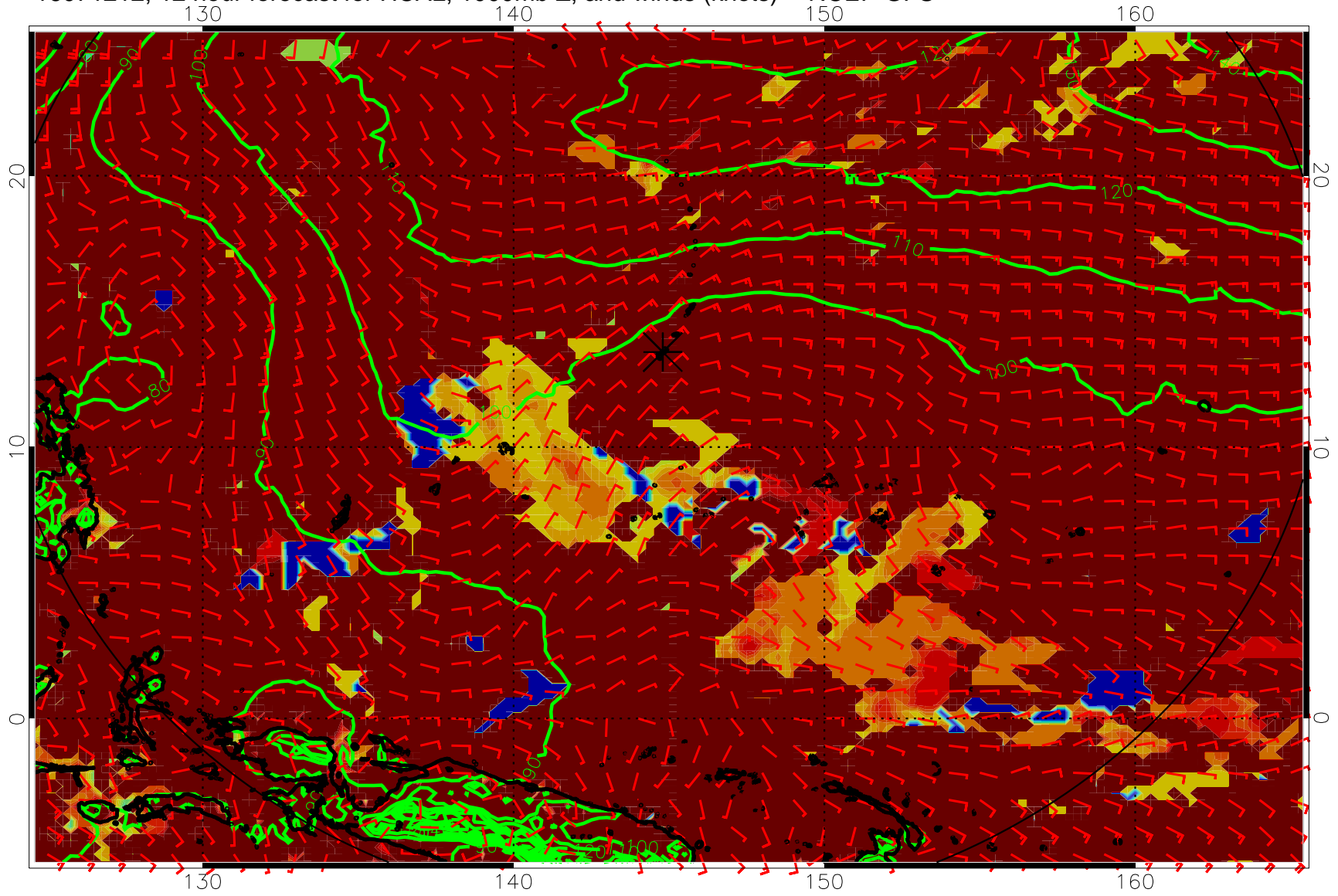
16071212, 12 hour forecast for HCAL, 1000mb Z, and winds (knots) -- NCEP GFS
