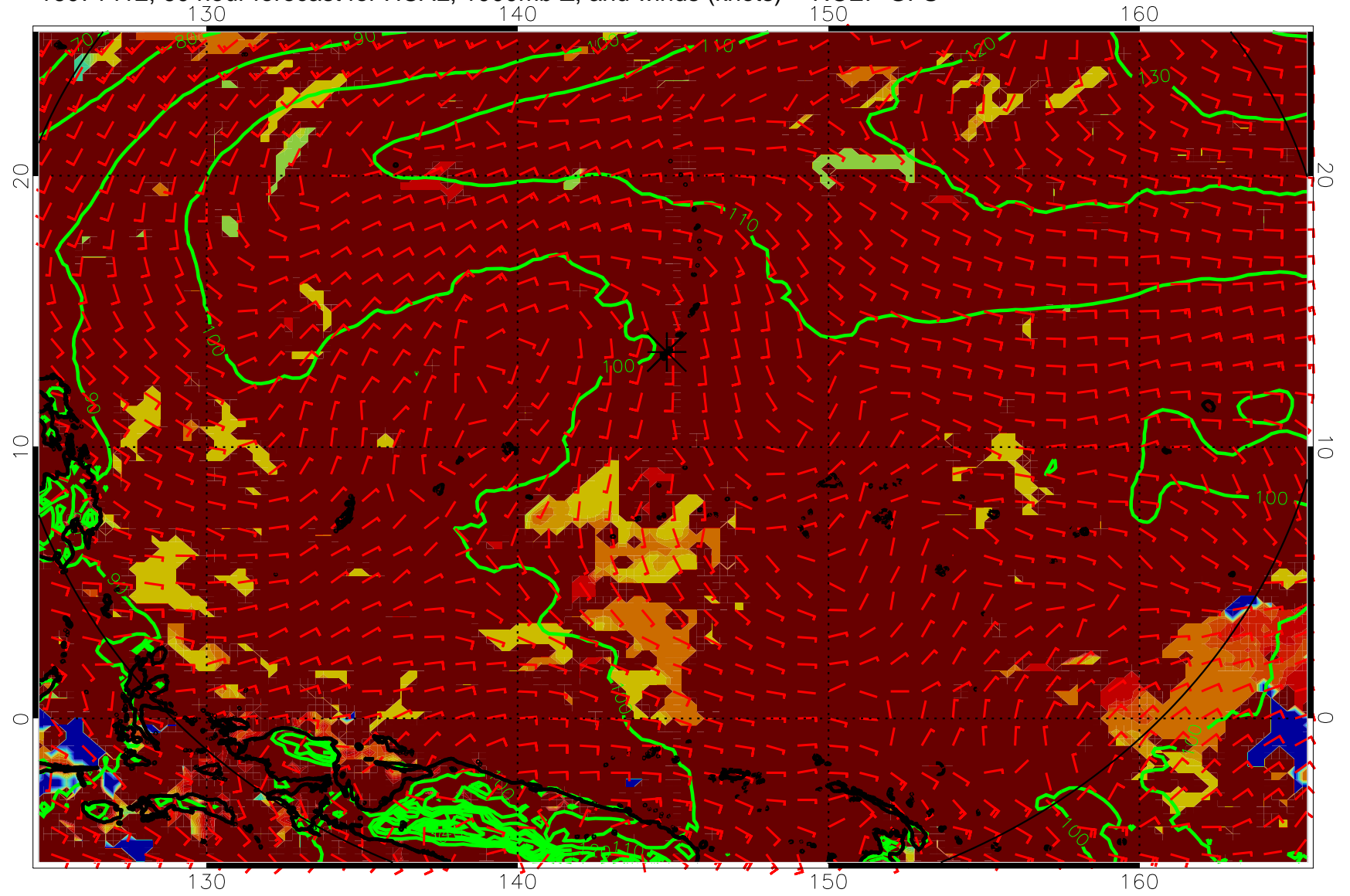
16071412, 60 hour forecast for HCAL, 1000mb Z, and winds (knots) -- NCEP GFS
