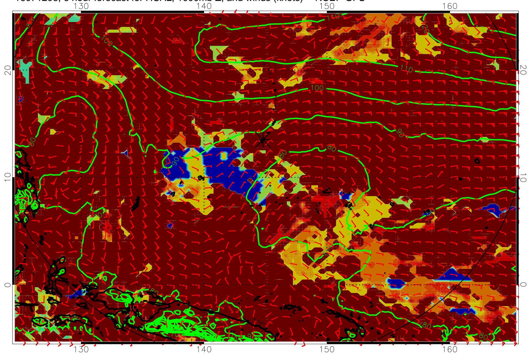
16071206, 6 hour forecast for HCAL, 1000mb Z, and winds (knots) -- NCEP GFS
