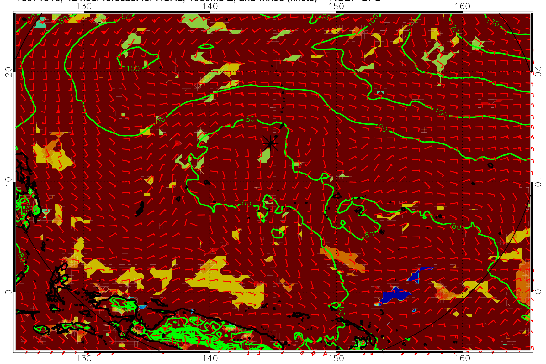
16071318, 42 hour forecast for HCAL, 1000mb Z, and winds (knots) -- NCEP GFS
