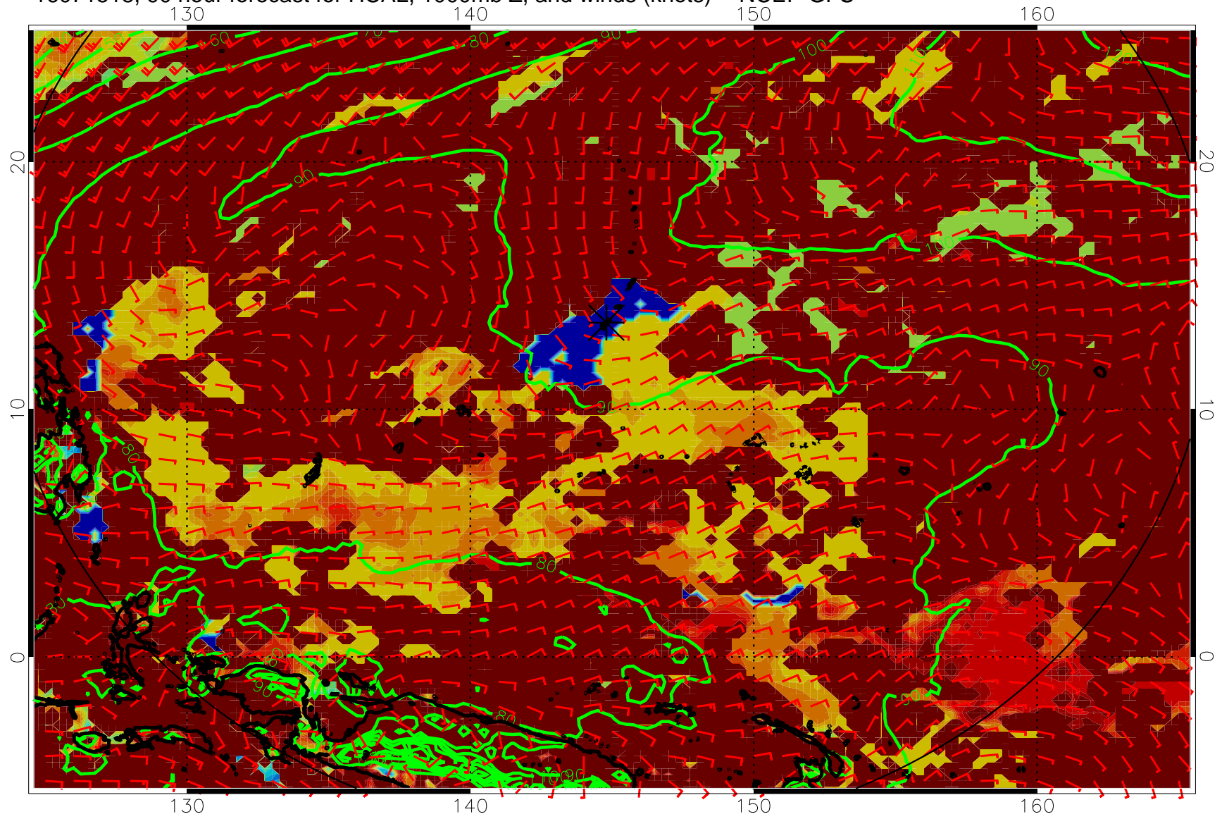
16071518, 90 hour forecast for HCAL, 1000mb Z, and winds (knots) -- NCEP GFS
