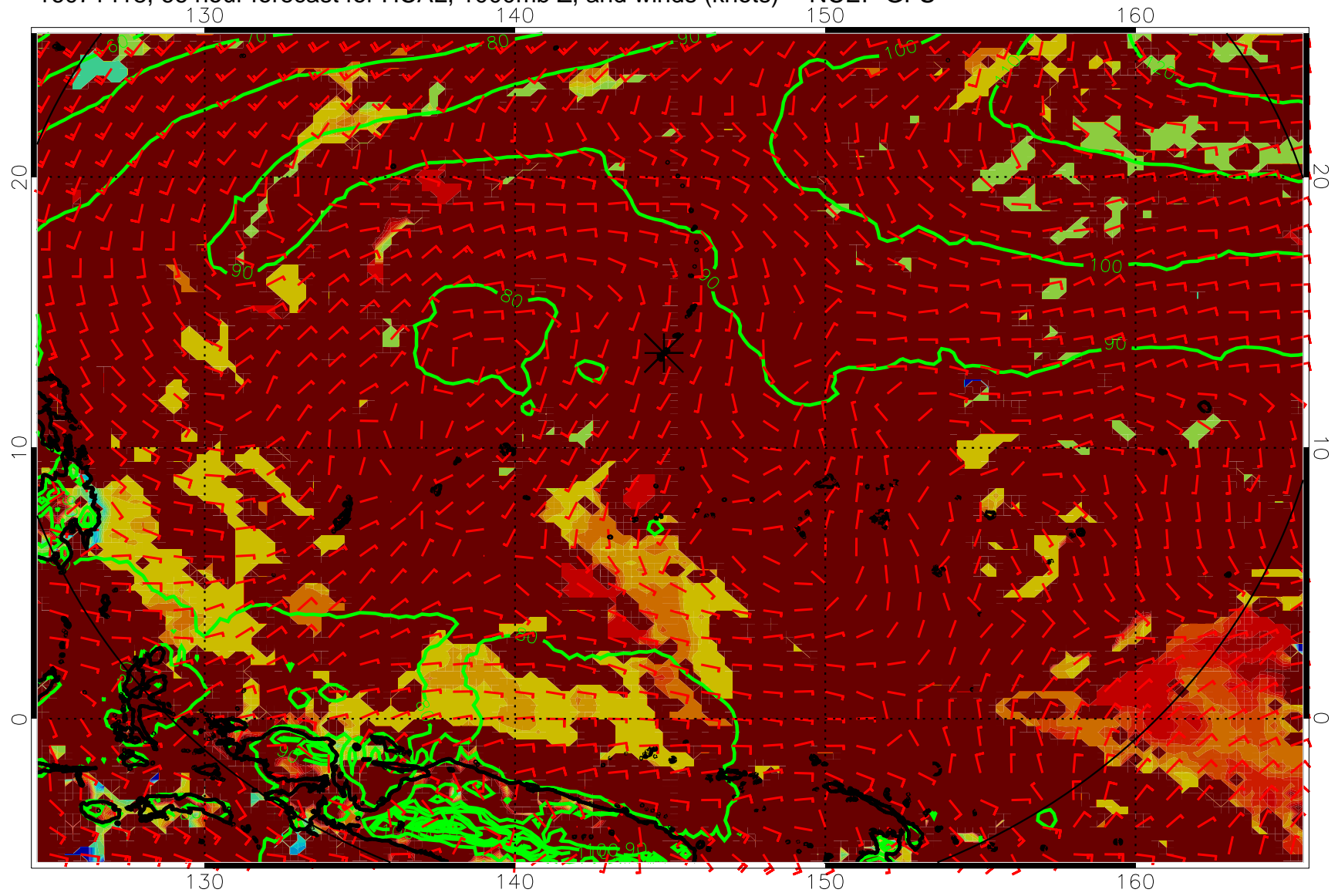
16071418, 66 hour forecast for HCAL, 1000mb Z, and winds (knots) -- NCEP GFS
