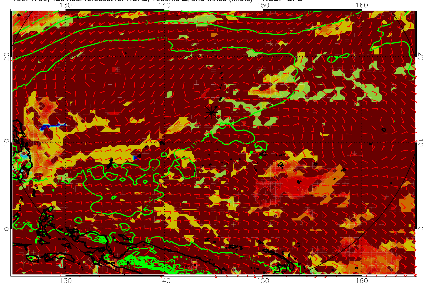
16071700, 120 hour forecast for HCAL, 1000mb Z, and winds (knots) -- NCEP GFS
