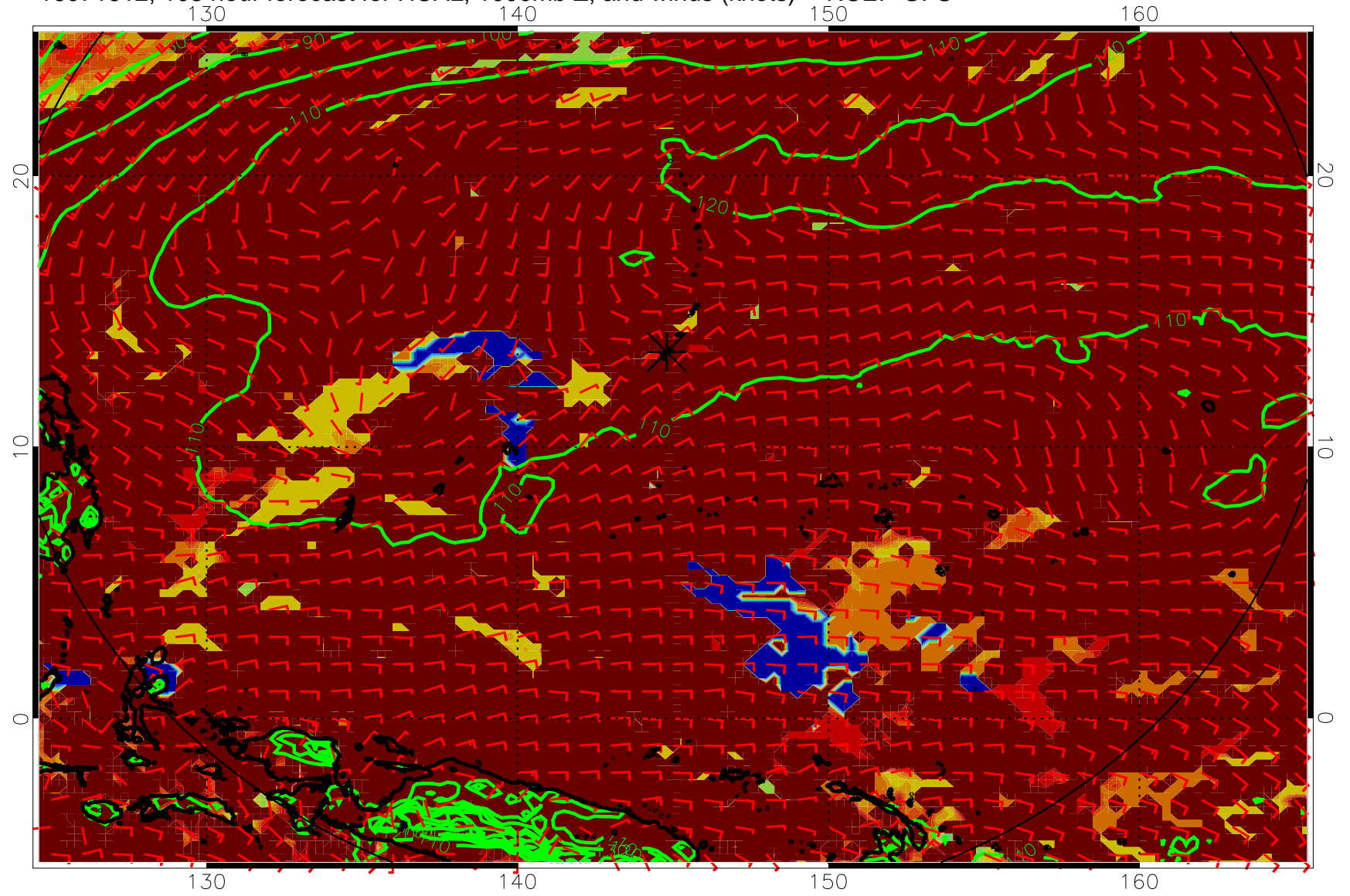
16071612, 108 hour forecast for HCAL, 1000mb Z, and winds (knots) -- NCEP GFS
