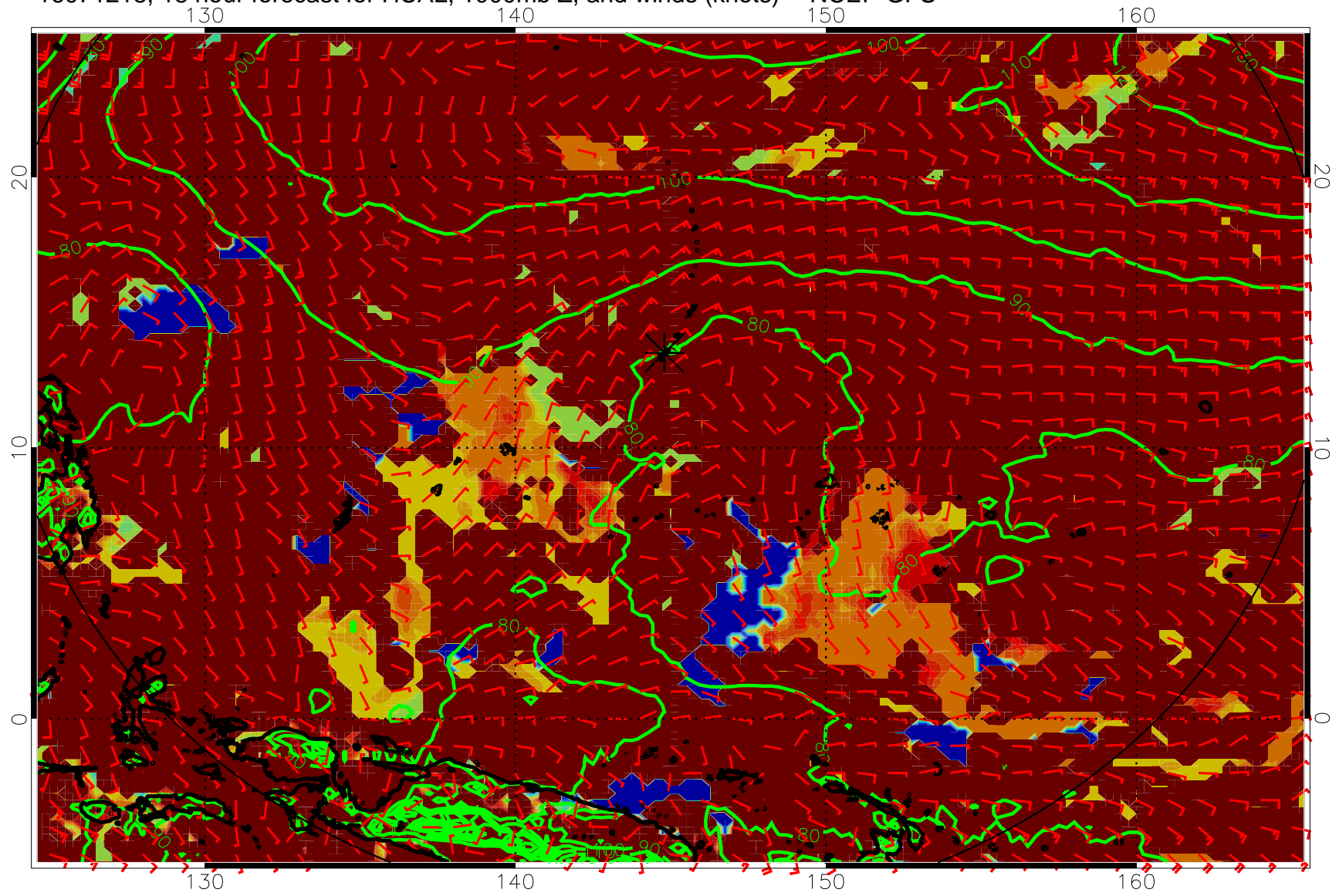
16071218, 18 hour forecast for HCAL, 1000mb Z, and winds (knots) -- NCEP GFS
