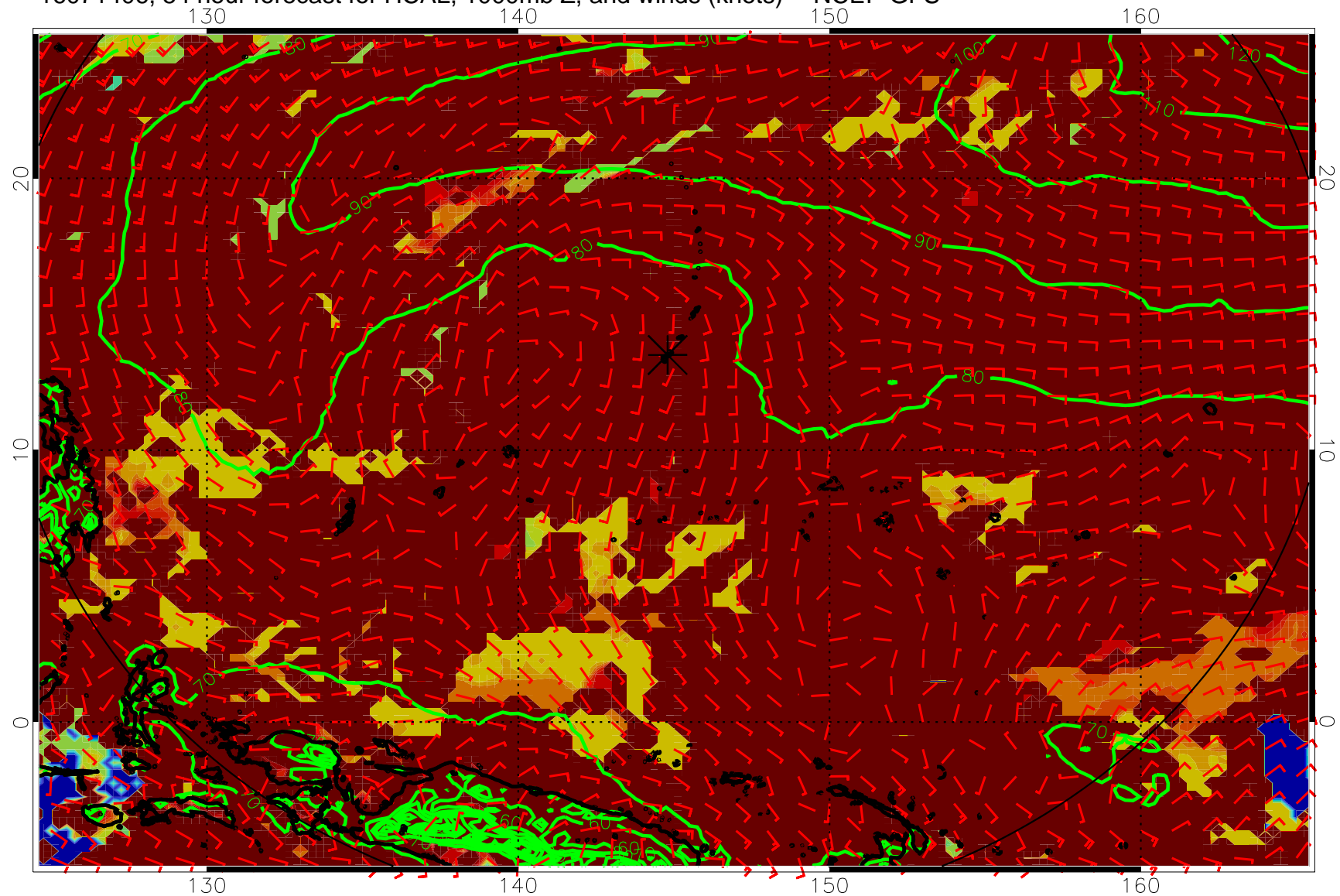
16071406, 54 hour forecast for HCAL, 1000mb Z, and winds (knots) -- NCEP GFS
