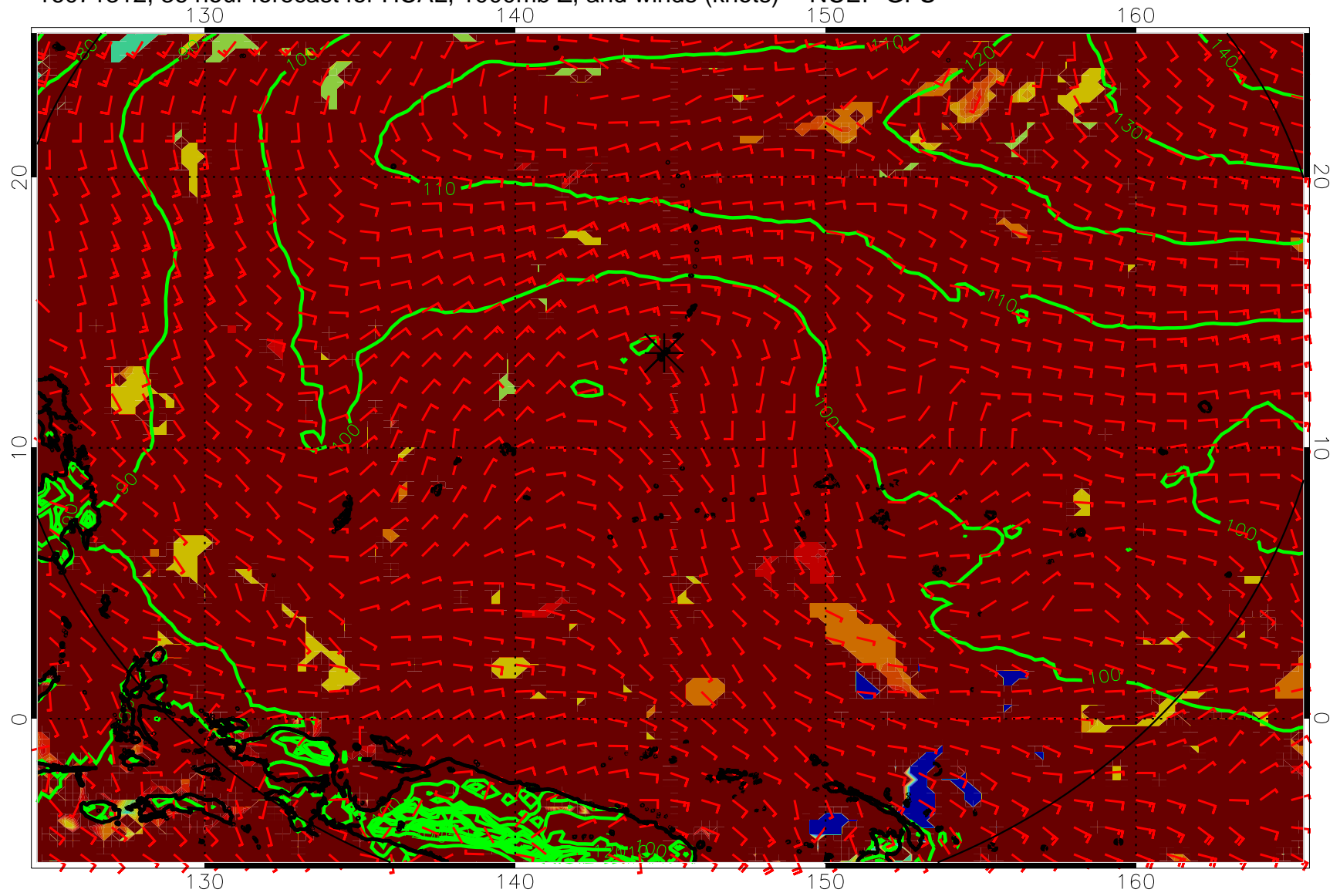
16071312, 36 hour forecast for HCAL, 1000mb Z, and winds (knots) -- NCEP GFS
