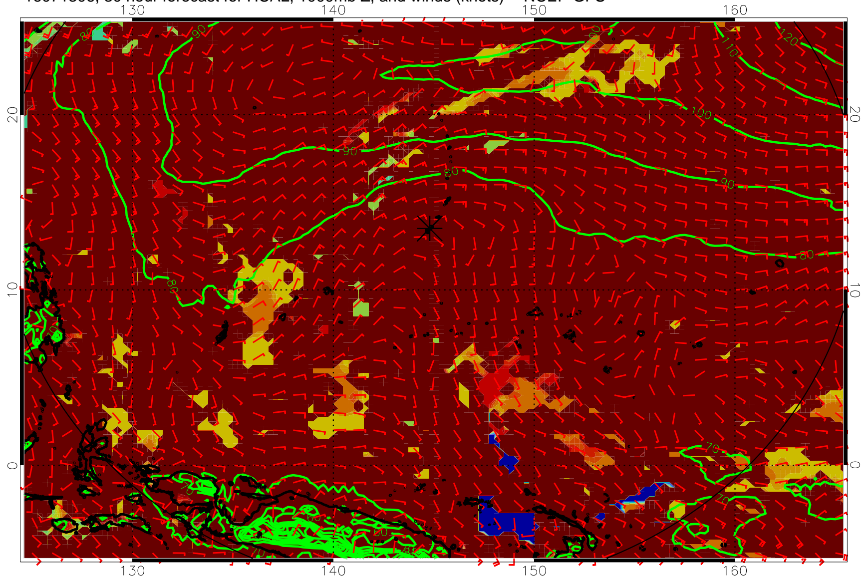
16071306, 30 hour forecast for HCAL, 1000mb Z, and winds (knots) -- NCEP GFS
