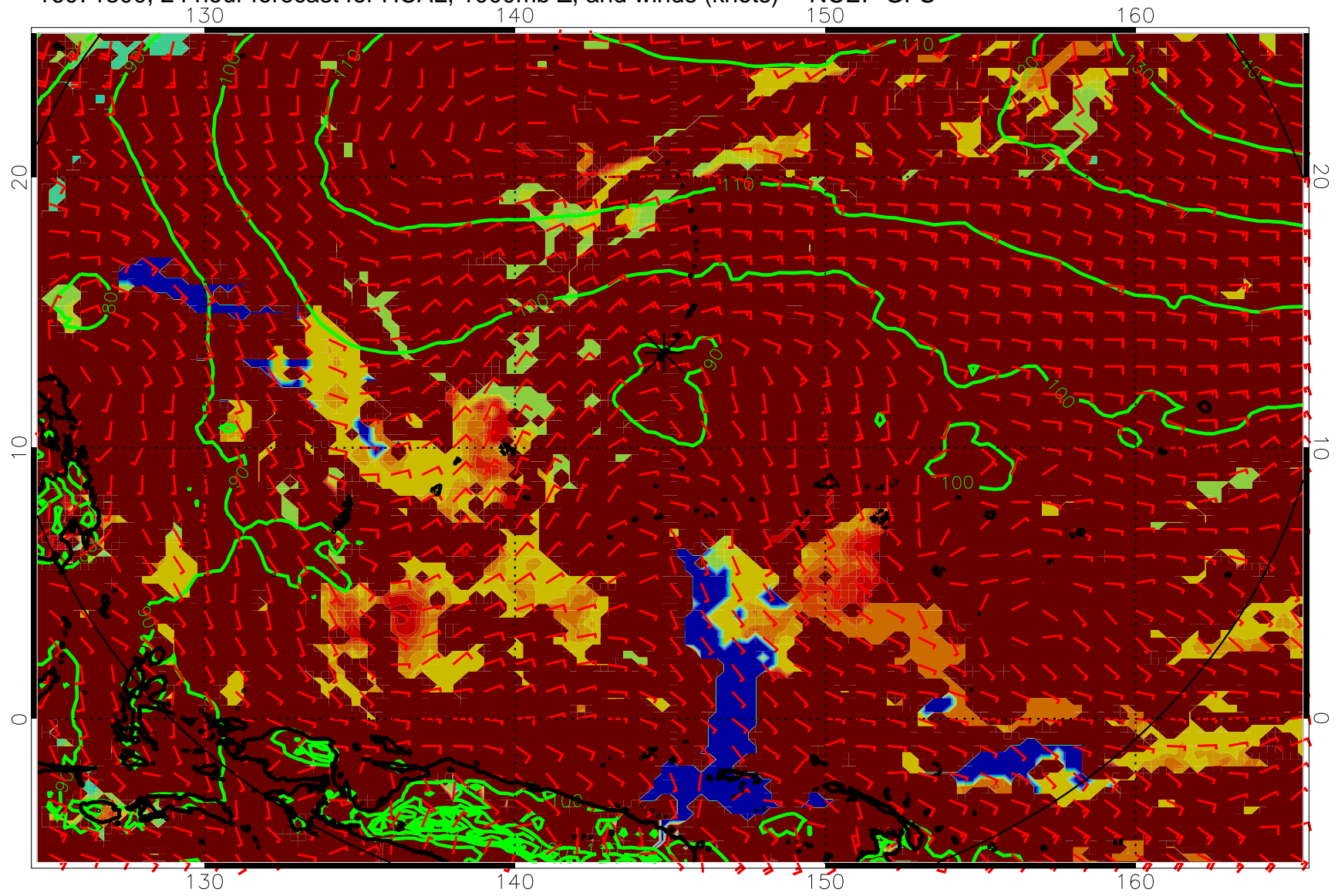
16071300, 24 hour forecast for HCAL, 1000mb Z, and winds (knots) -- NCEP GFS
