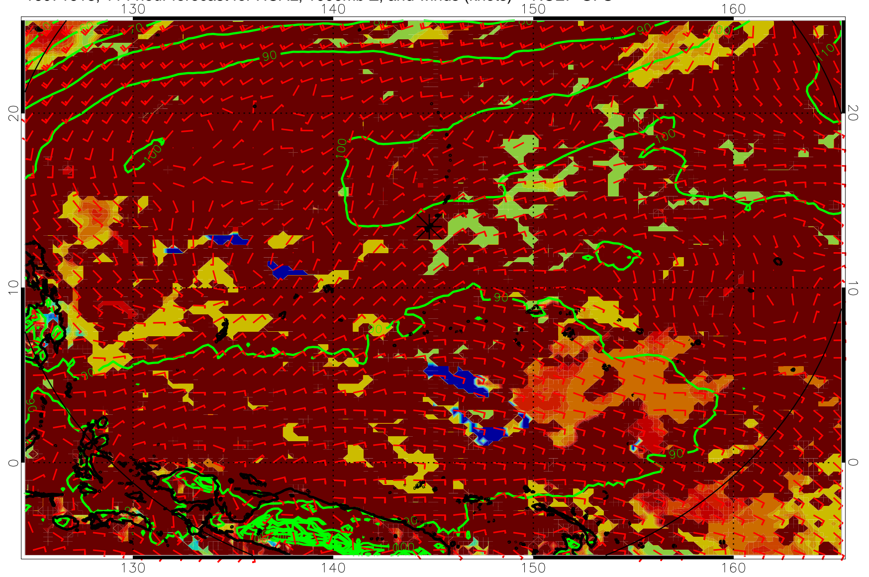
16071618, 114 hour forecast for HCAL, 1000mb Z, and winds (knots) -- NCEP GFS
