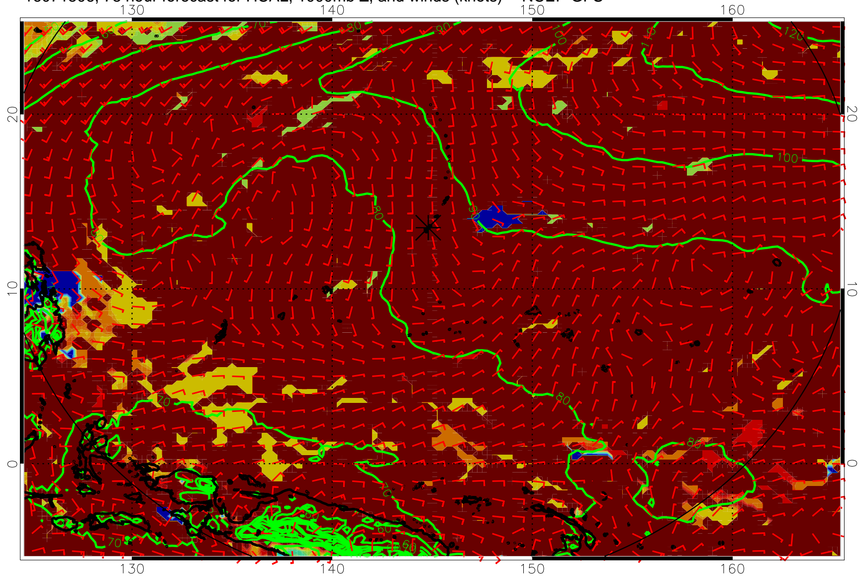
16071506, 78 hour forecast for HCAL, 1000mb Z, and winds (knots) -- NCEP GFS
