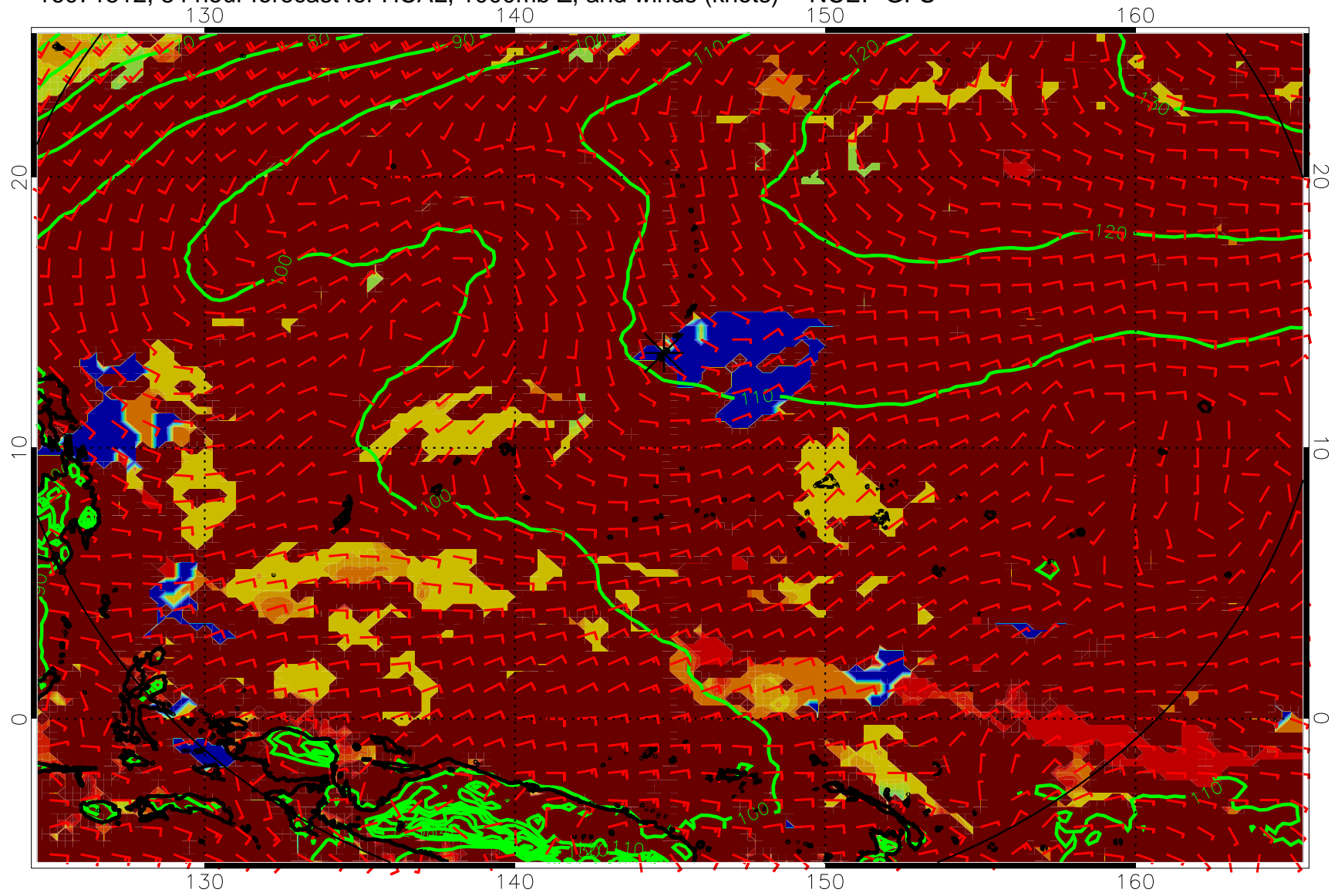
16071512, 84 hour forecast for HCAL, 1000mb Z, and winds (knots) -- NCEP GFS
