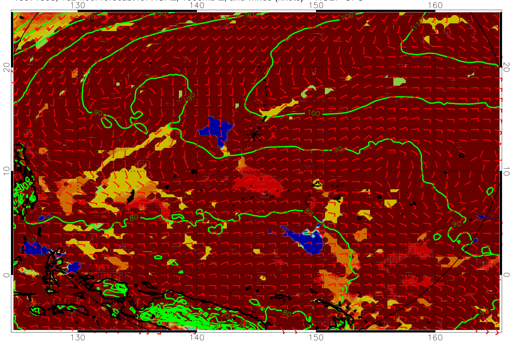
16071606, 102 hour forecast for HCAL, 1000mb Z, and winds (knots) -- NCEP GFS
