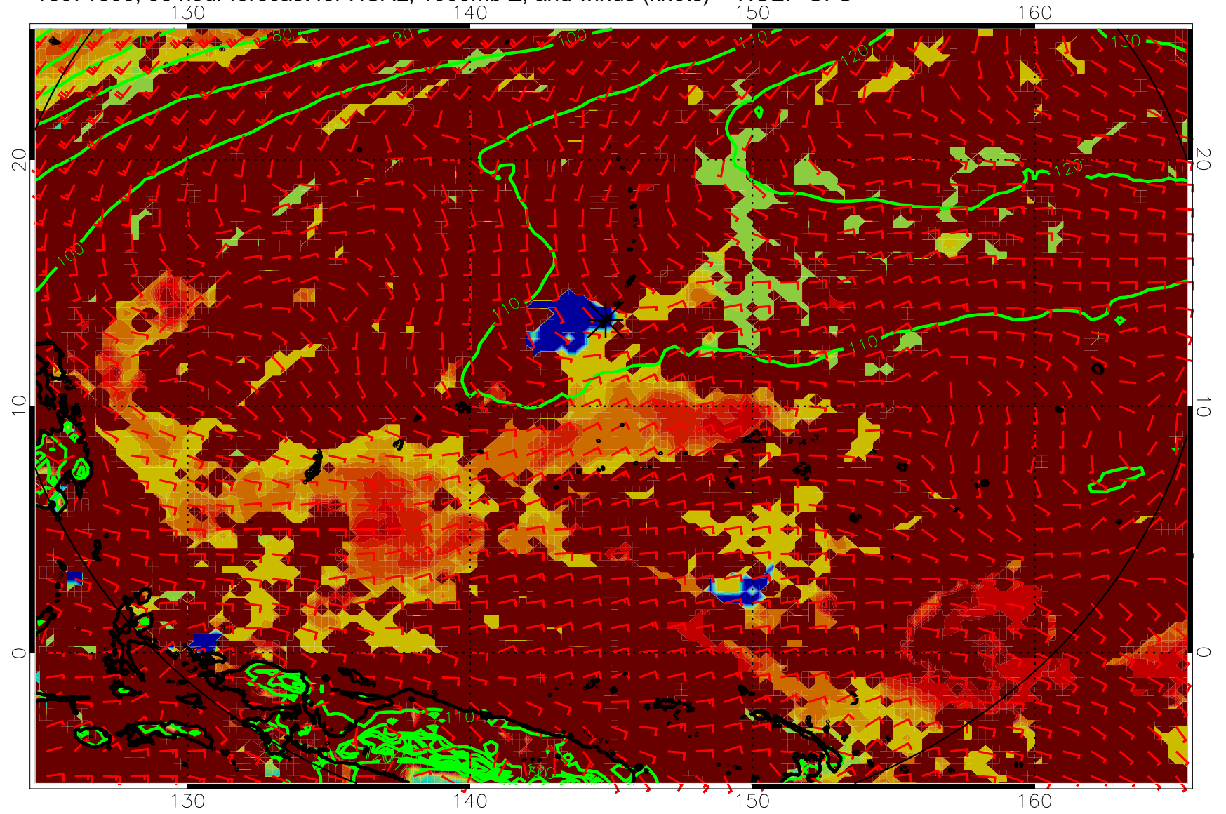
16071600, 96 hour forecast for HCAL, 1000mb Z, and winds (knots) -- NCEP GFS
