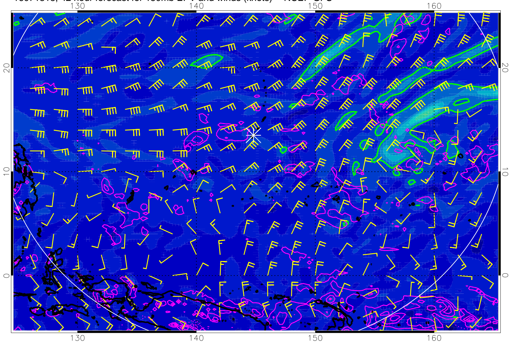
16071318, 42 hour forecast for 150mb EPV and winds (knots) -- NCEP GFS
