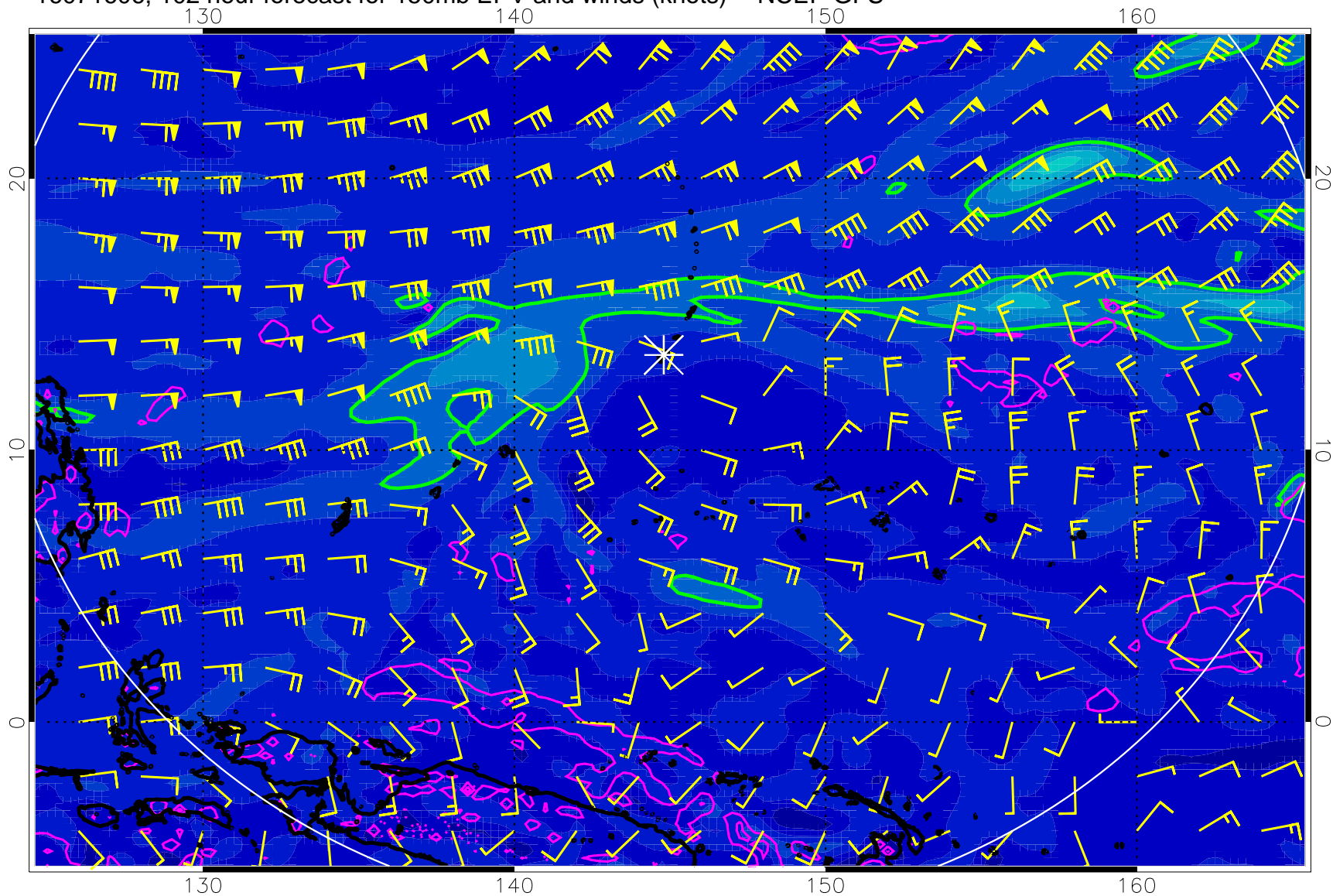
16071606, 102 hour forecast for 150mb EPV and winds (knots) -- NCEP GFS
