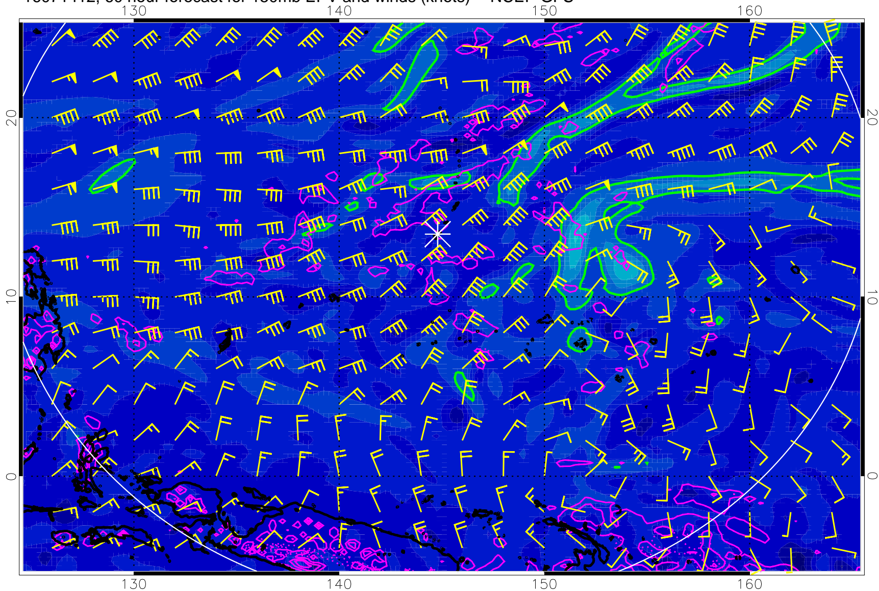
16071412, 60 hour forecast for 150mb EPV and winds (knots) -- NCEP GFS
