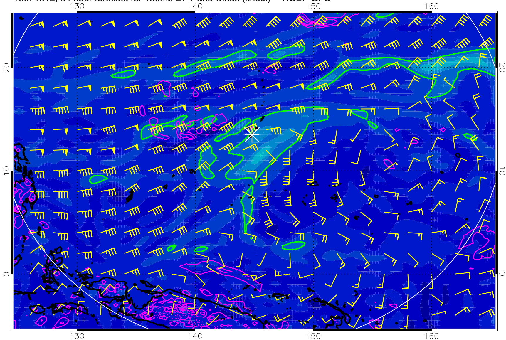
16071512, 84 hour forecast for 150mb EPV and winds (knots) -- NCEP GFS
