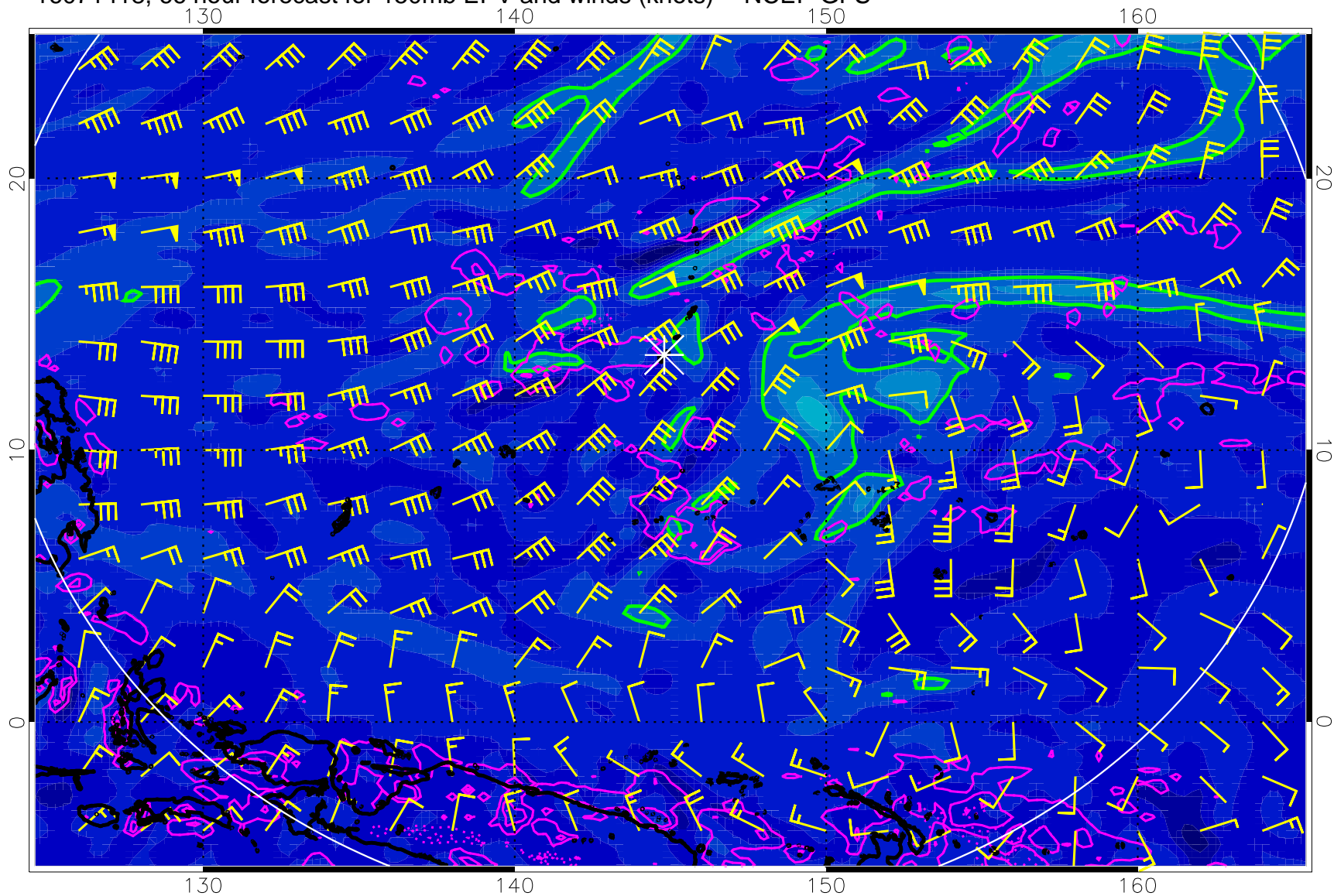
16071418, 66 hour forecast for 150mb EPV and winds (knots) -- NCEP GFS
