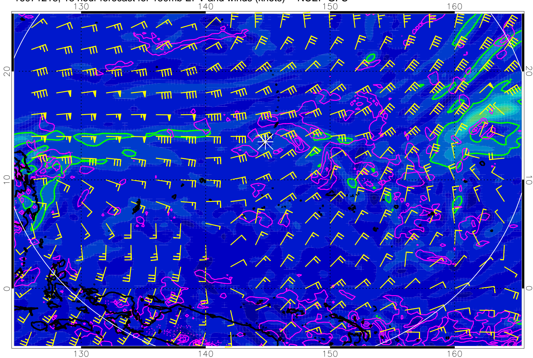
16071218, 18 hour forecast for 150mb EPV and winds (knots) -- NCEP GFS
