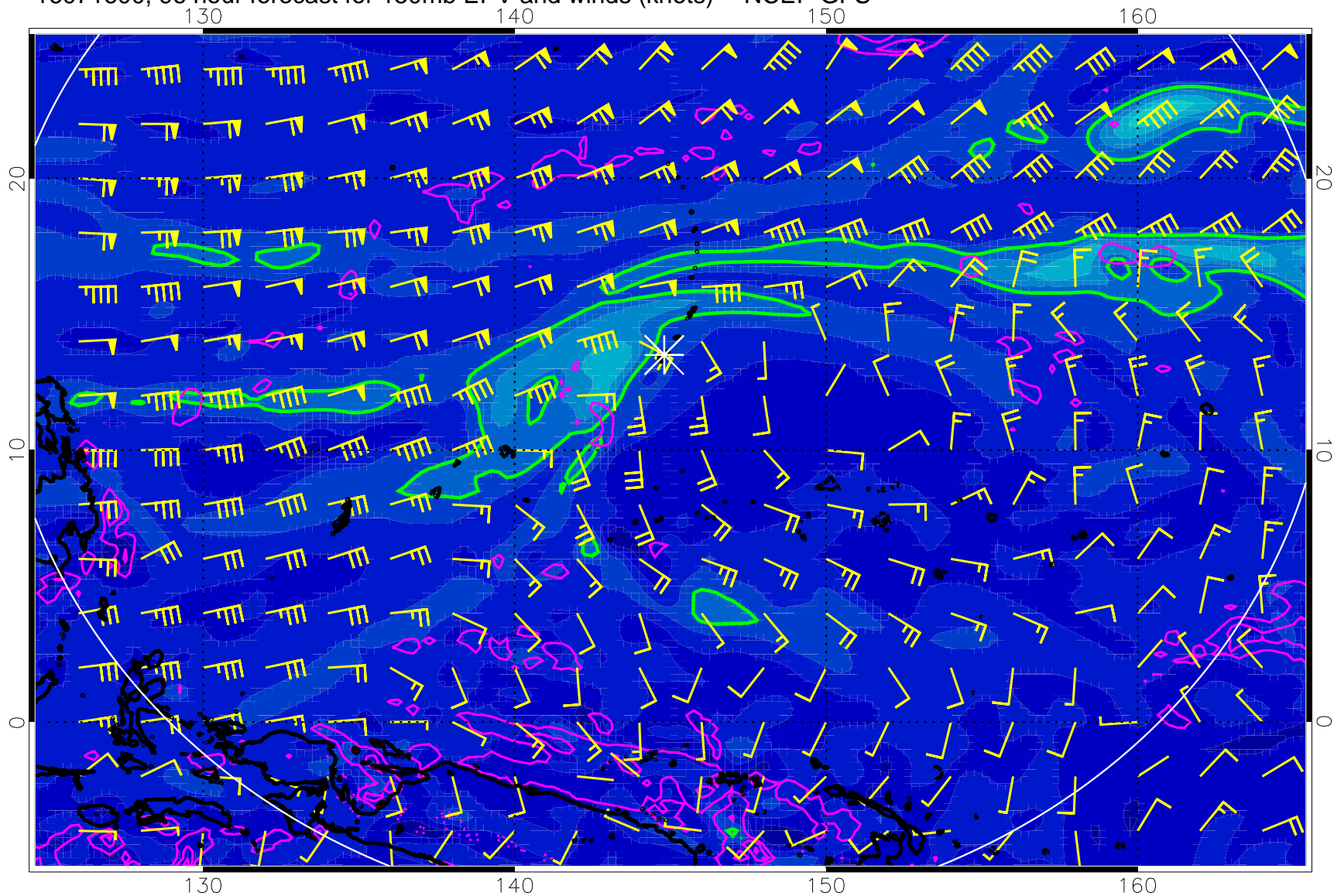
16071600, 96 hour forecast for 150mb EPV and winds (knots) -- NCEP GFS
