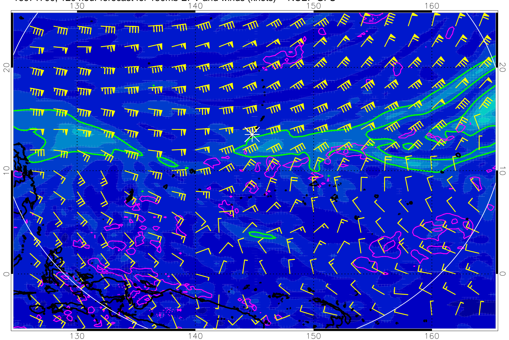
16071700, 120 hour forecast for 150mb EPV and winds (knots) -- NCEP GFS
