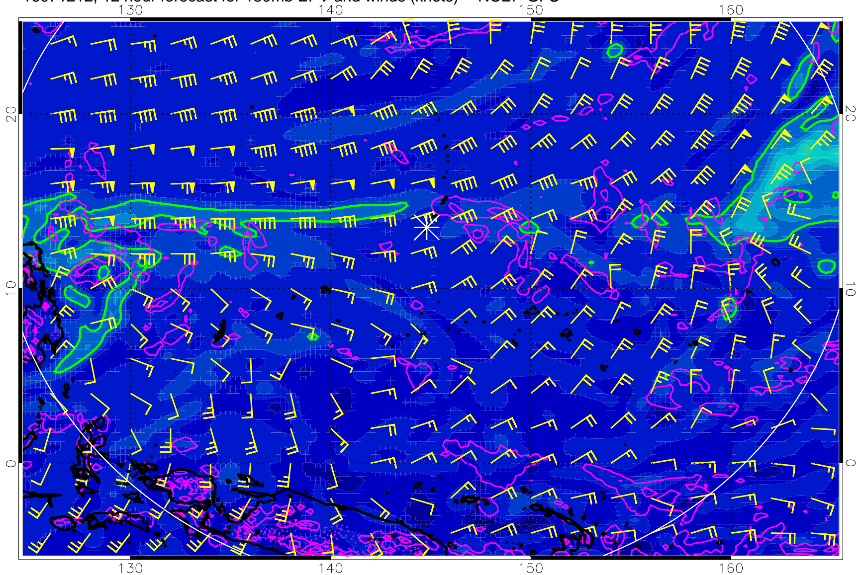
16071212, 12 hour forecast for 150mb EPV and winds (knots) -- NCEP GFS
