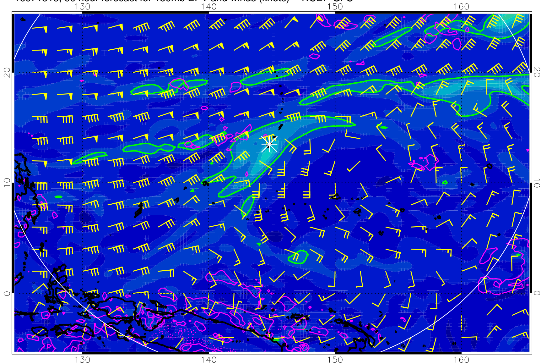
16071518, 90 hour forecast for 150mb EPV and winds (knots) -- NCEP GFS
