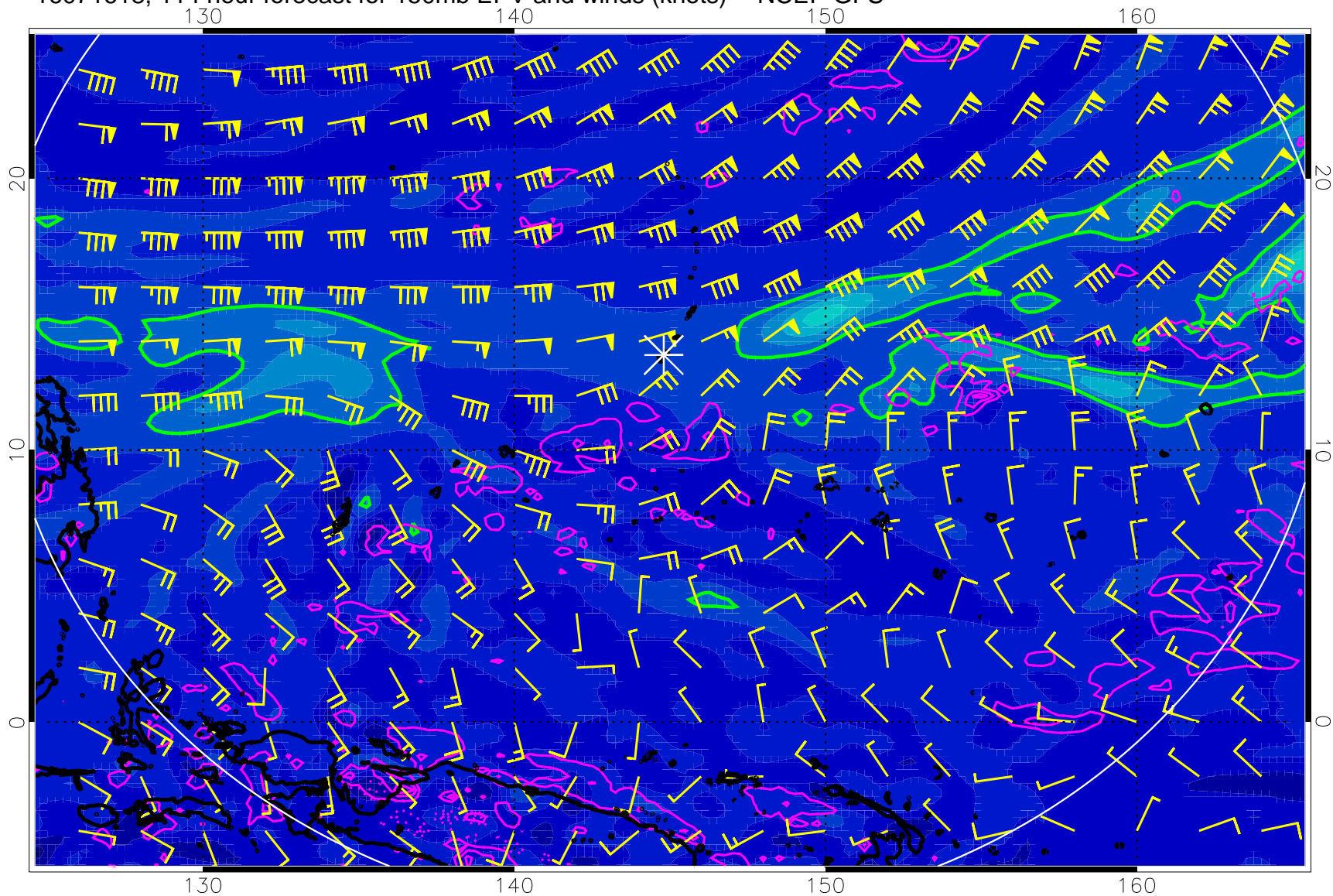
16071618, 114 hour forecast for 150mb EPV and winds (knots) -- NCEP GFS
