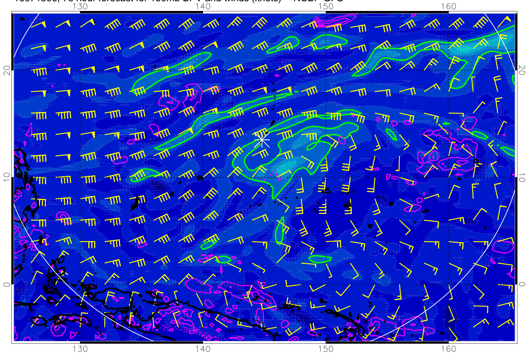
16071506, 78 hour forecast for 150mb EPV and winds (knots) -- NCEP GFS
