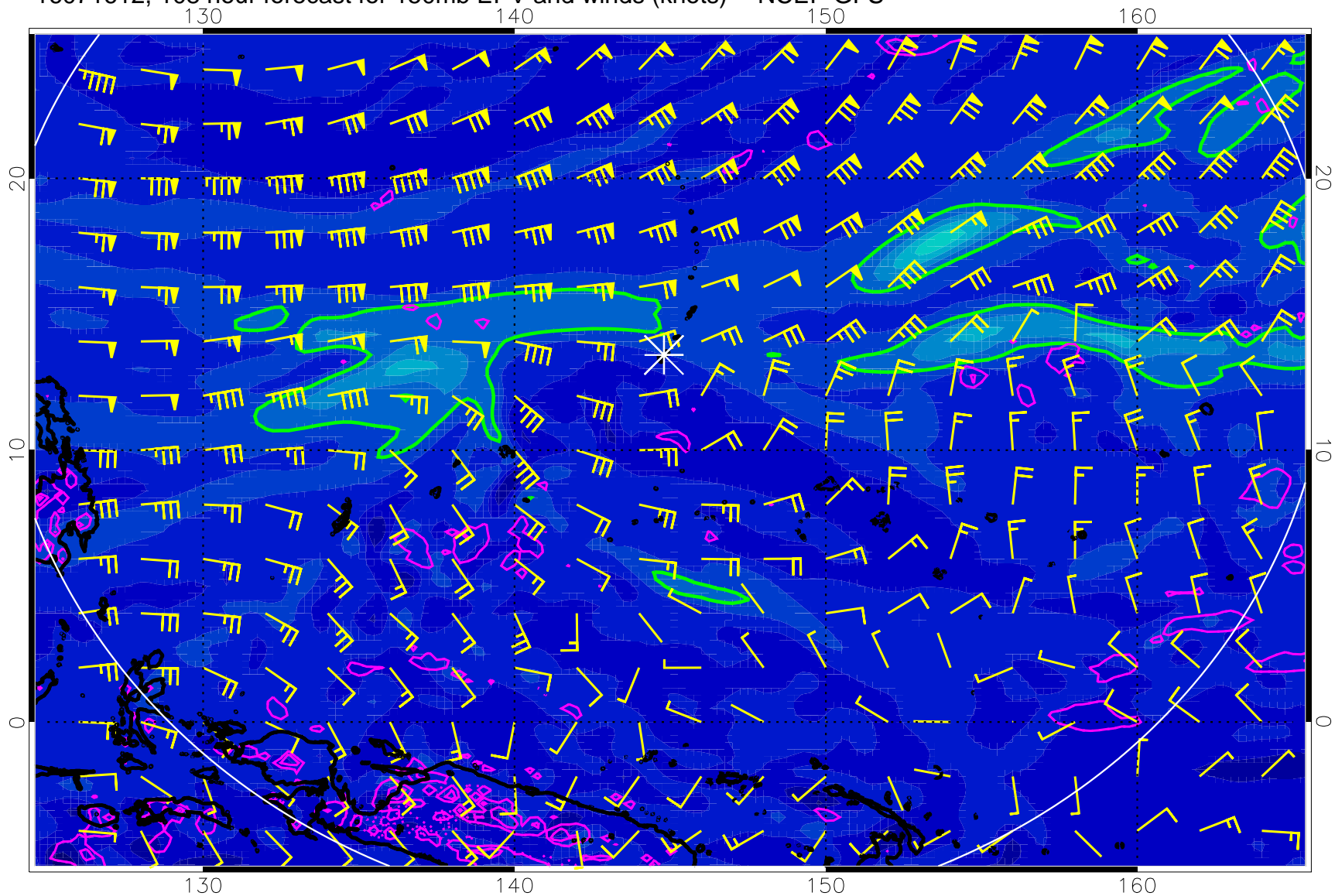
16071612, 108 hour forecast for 150mb EPV and winds (knots) -- NCEP GFS
