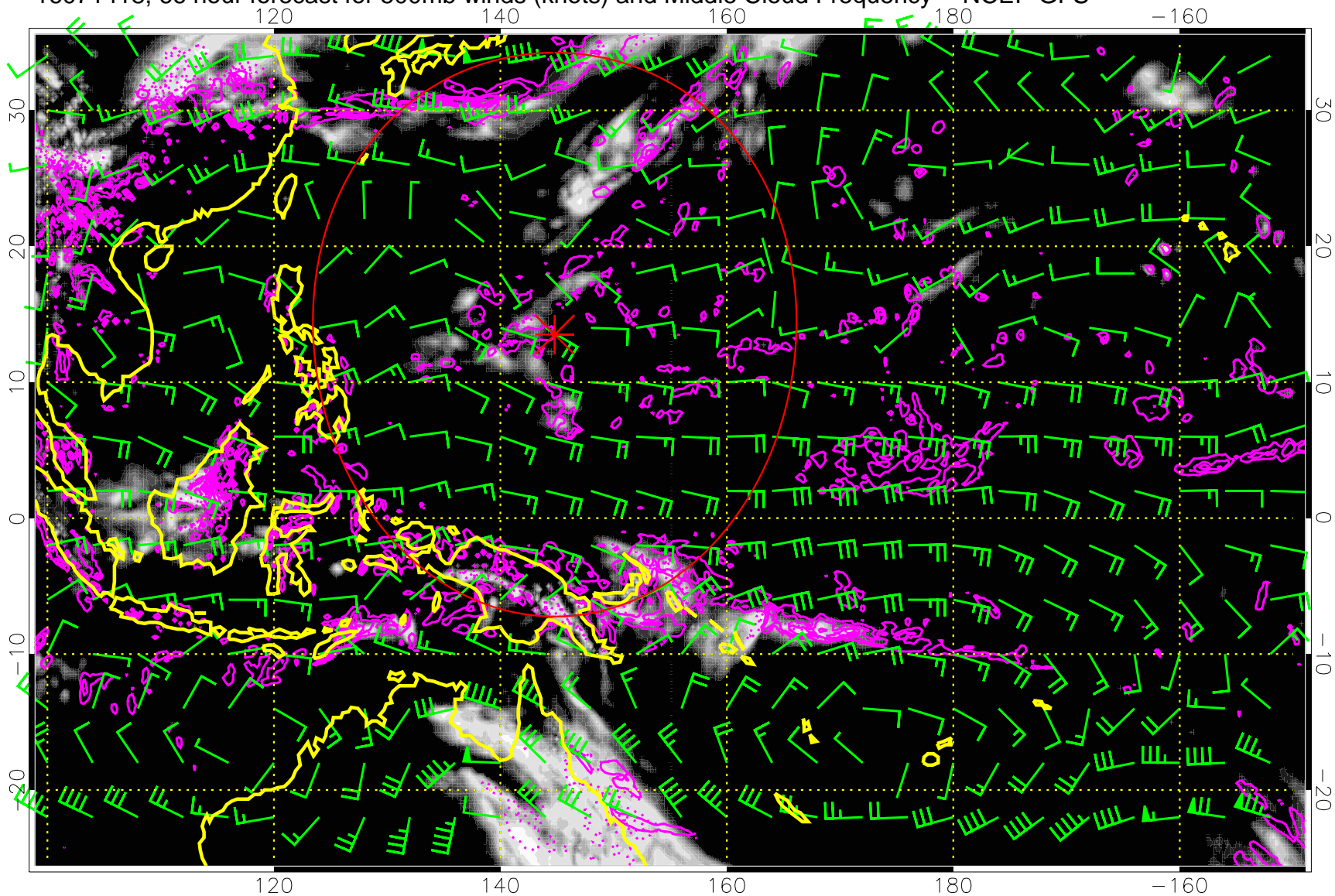
16071418, 66 hour forecast for 500mb winds (knots) and Middle Cloud Frequency -- NCEP GFS
