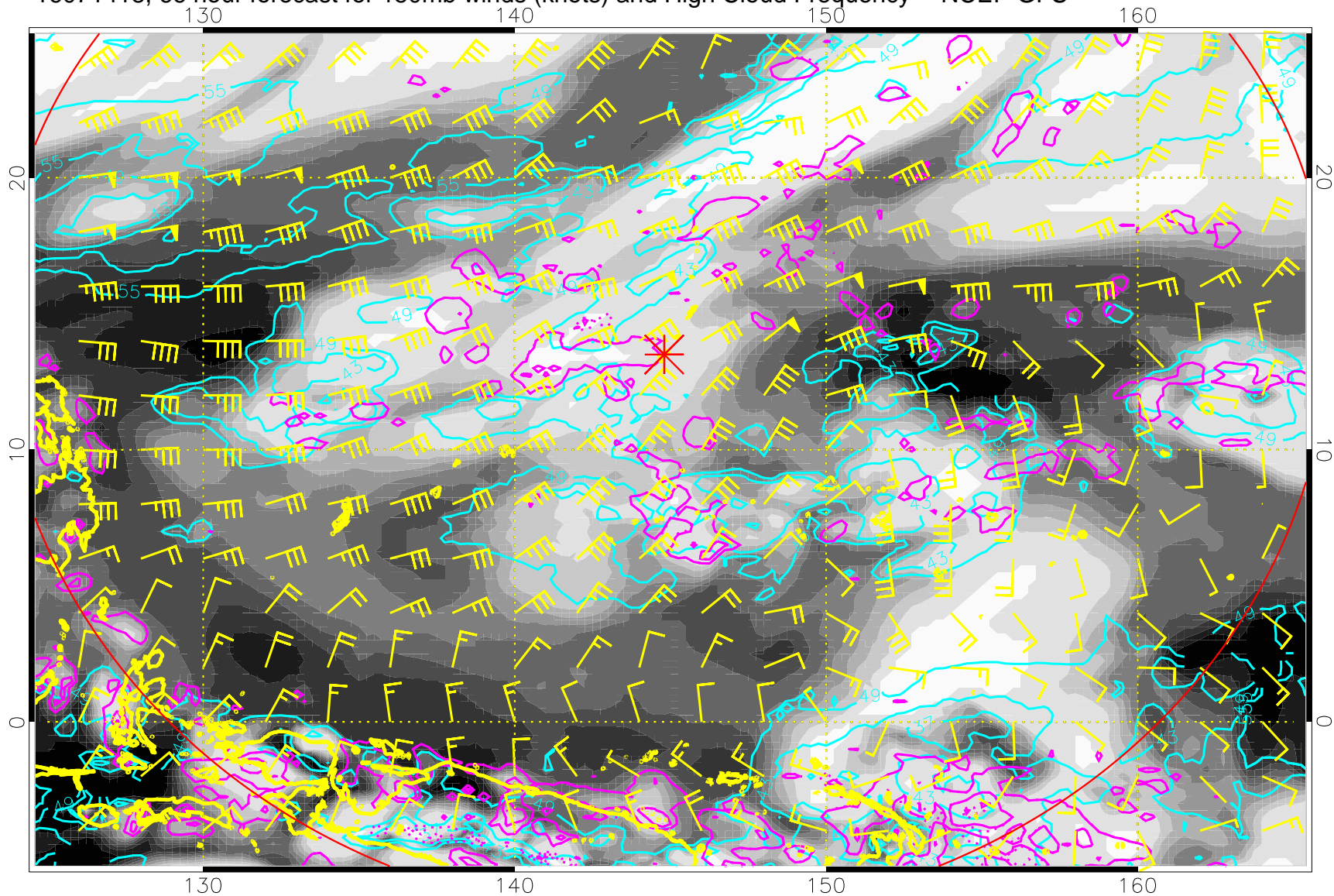
16071418, 66 hour forecast for 150mb winds (knots) and High Cloud Frequency -- NCEP GFS
