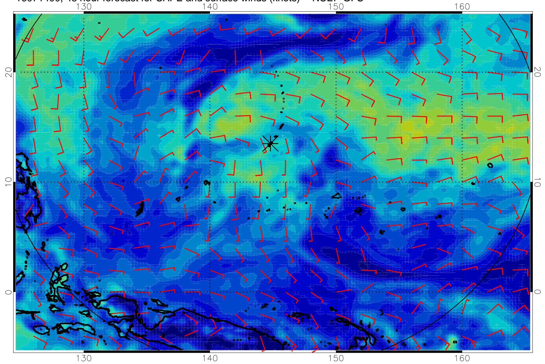
16071400, 48 hour forecast for CAPE and surface winds (knots) -- NCEP GFS
