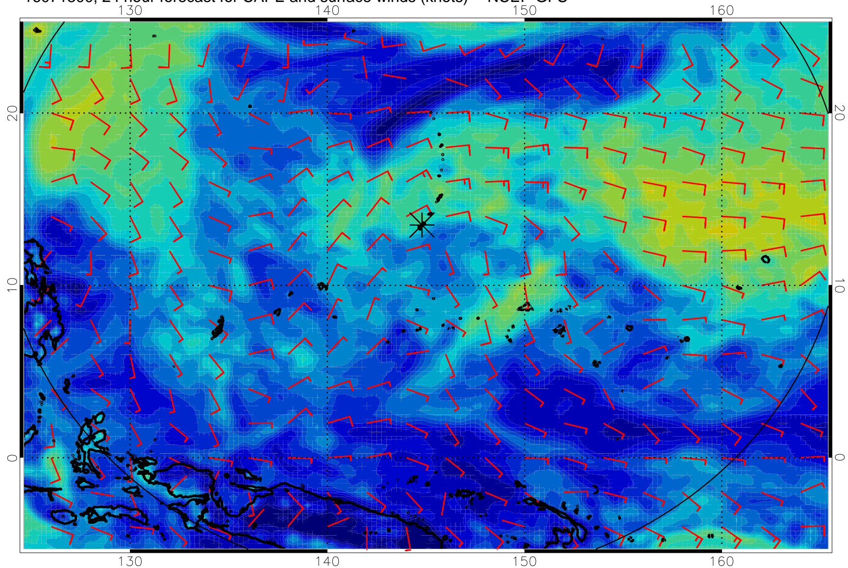
16071300, 24 hour forecast for CAPE and surface winds (knots) -- NCEP GFS
