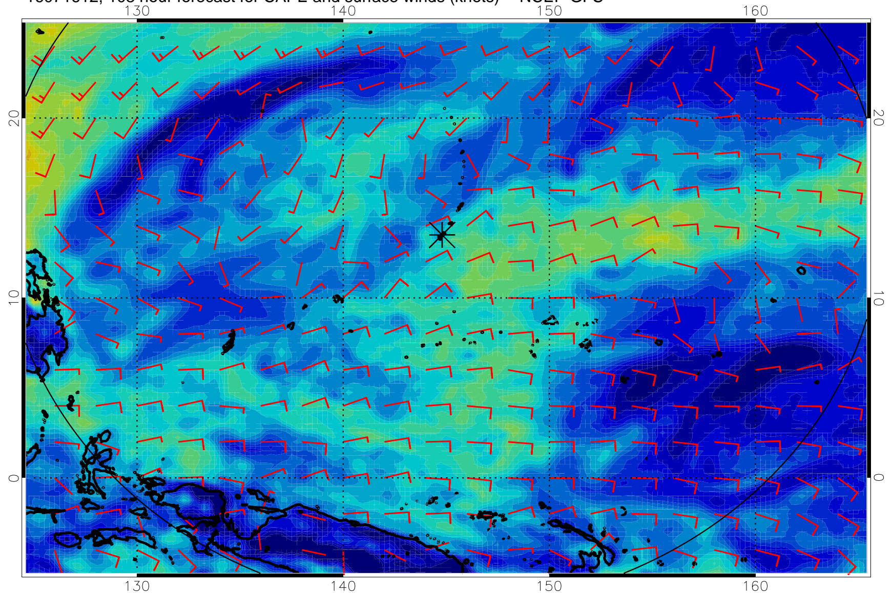
16071612, 108 hour forecast for CAPE and surface winds (knots) -- NCEP GFS
