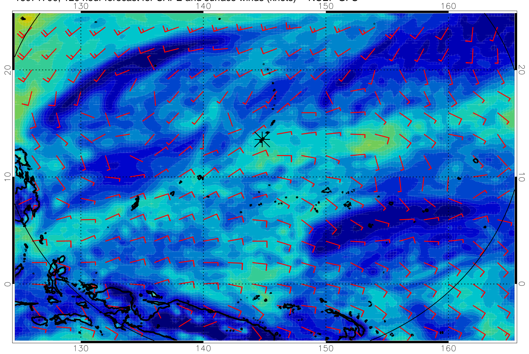
16071700, 120 hour forecast for CAPE and surface winds (knots) -- NCEP GFS
