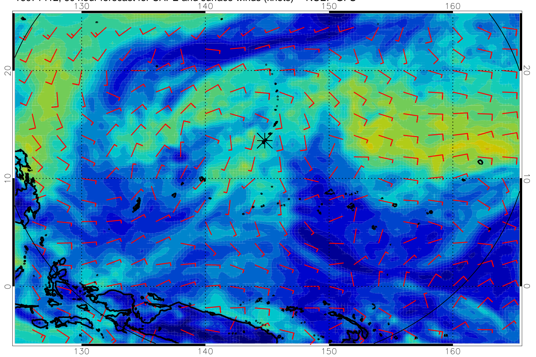
16071412, 60 hour forecast for CAPE and surface winds (knots) -- NCEP GFS
