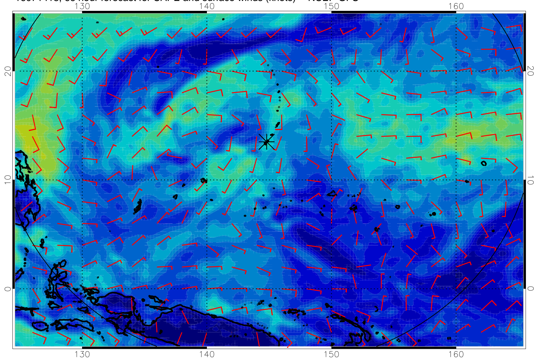
16071418, 66 hour forecast for CAPE and surface winds (knots) -- NCEP GFS
