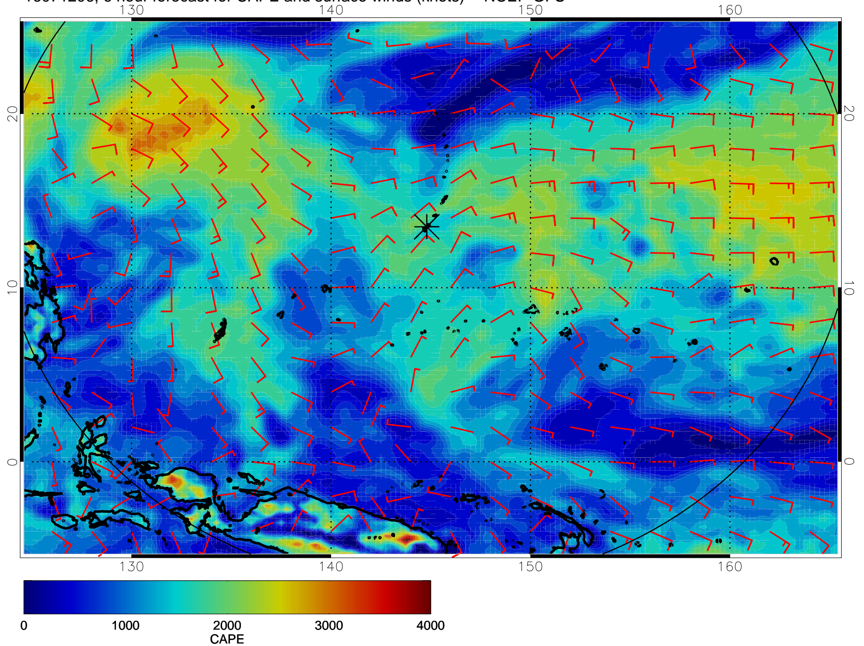
16071206, 6 hour forecast for CAPE and surface winds (knots) -- NCEP GFS
