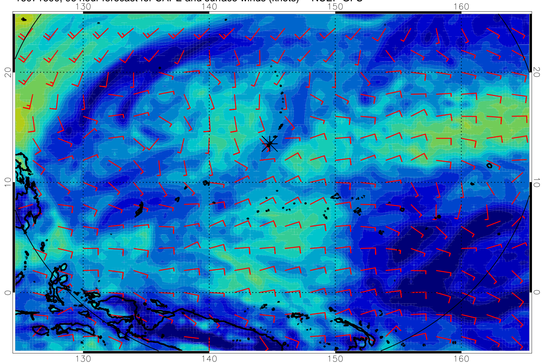
16071600, 96 hour forecast for CAPE and surface winds (knots) -- NCEP GFS
