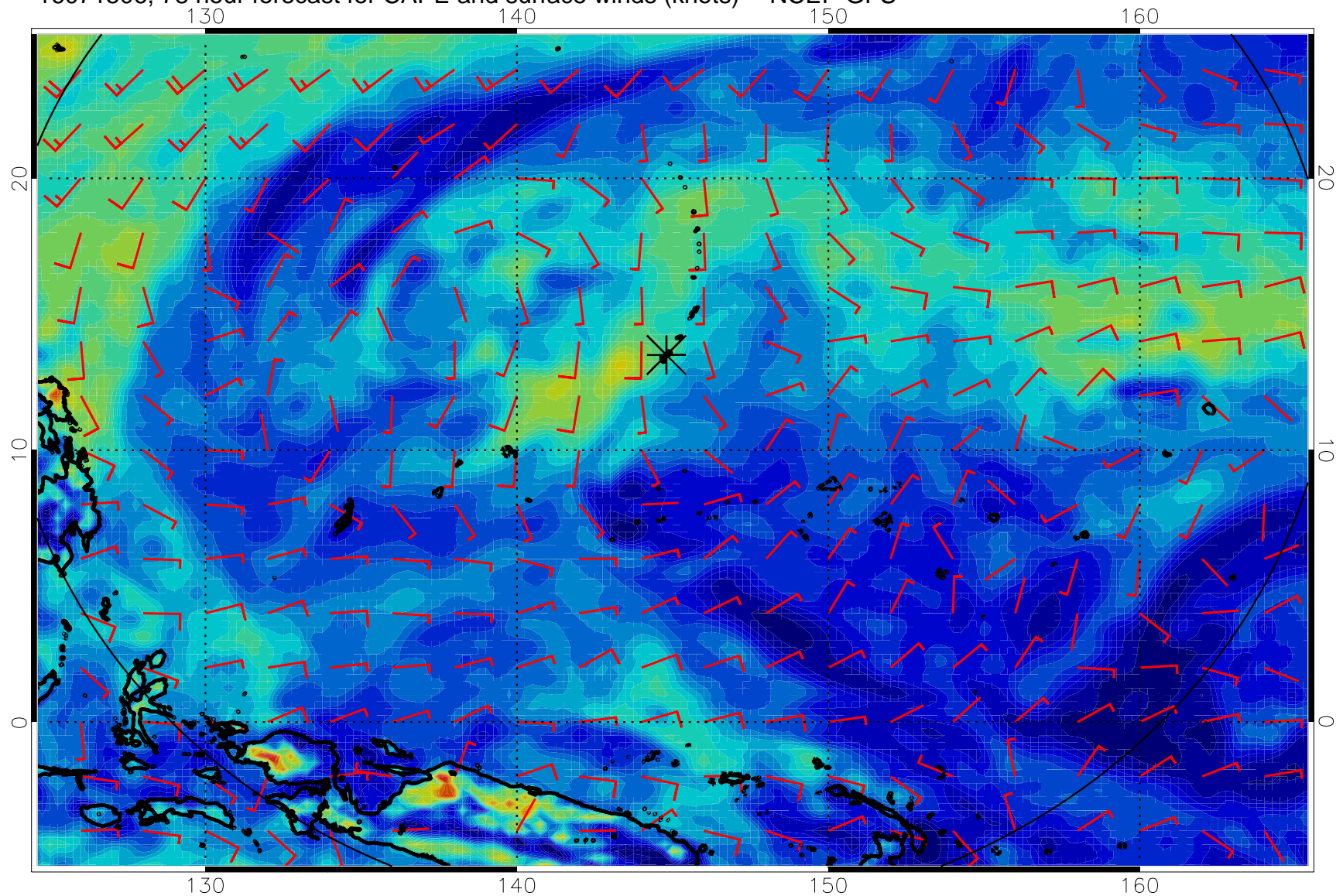
16071506, 78 hour forecast for CAPE and surface winds (knots) -- NCEP GFS
