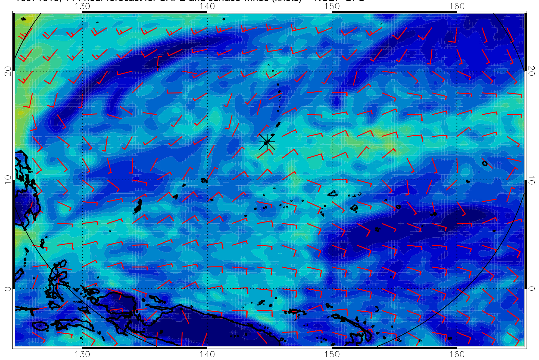
16071618, 114 hour forecast for CAPE and surface winds (knots) -- NCEP GFS
