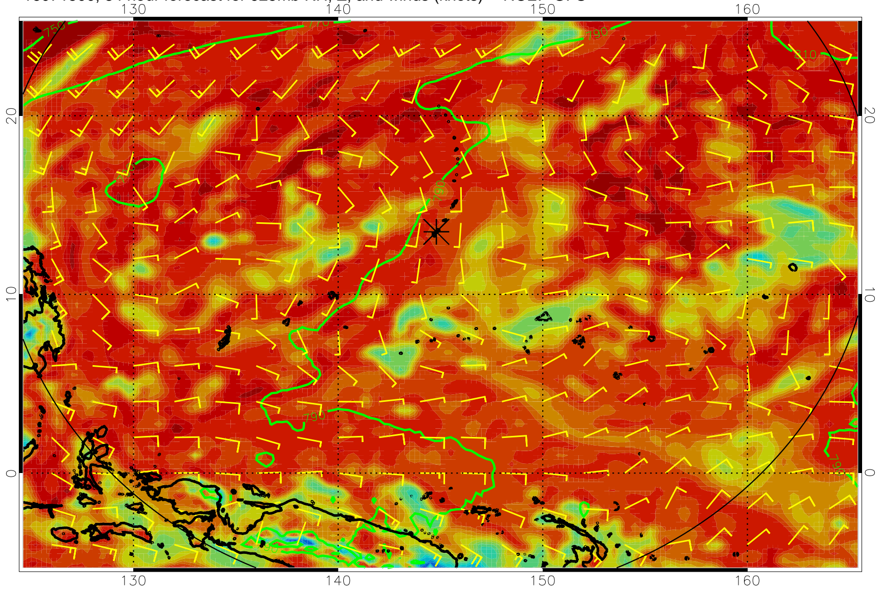
16071500, 84 hour forecast for 925mb RH, Z, and winds (knots) -- NCEP GFS
