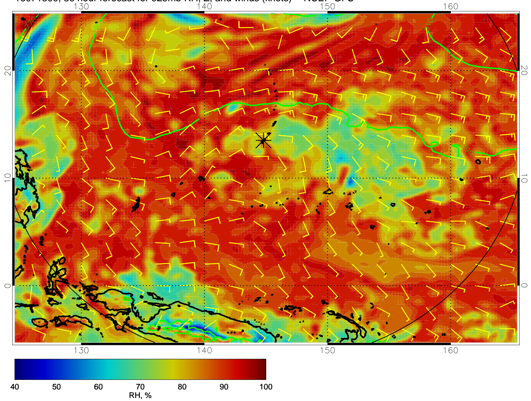
16071300, 36 hour forecast for 925mb RH, Z, and winds (knots) -- NCEP GFS
