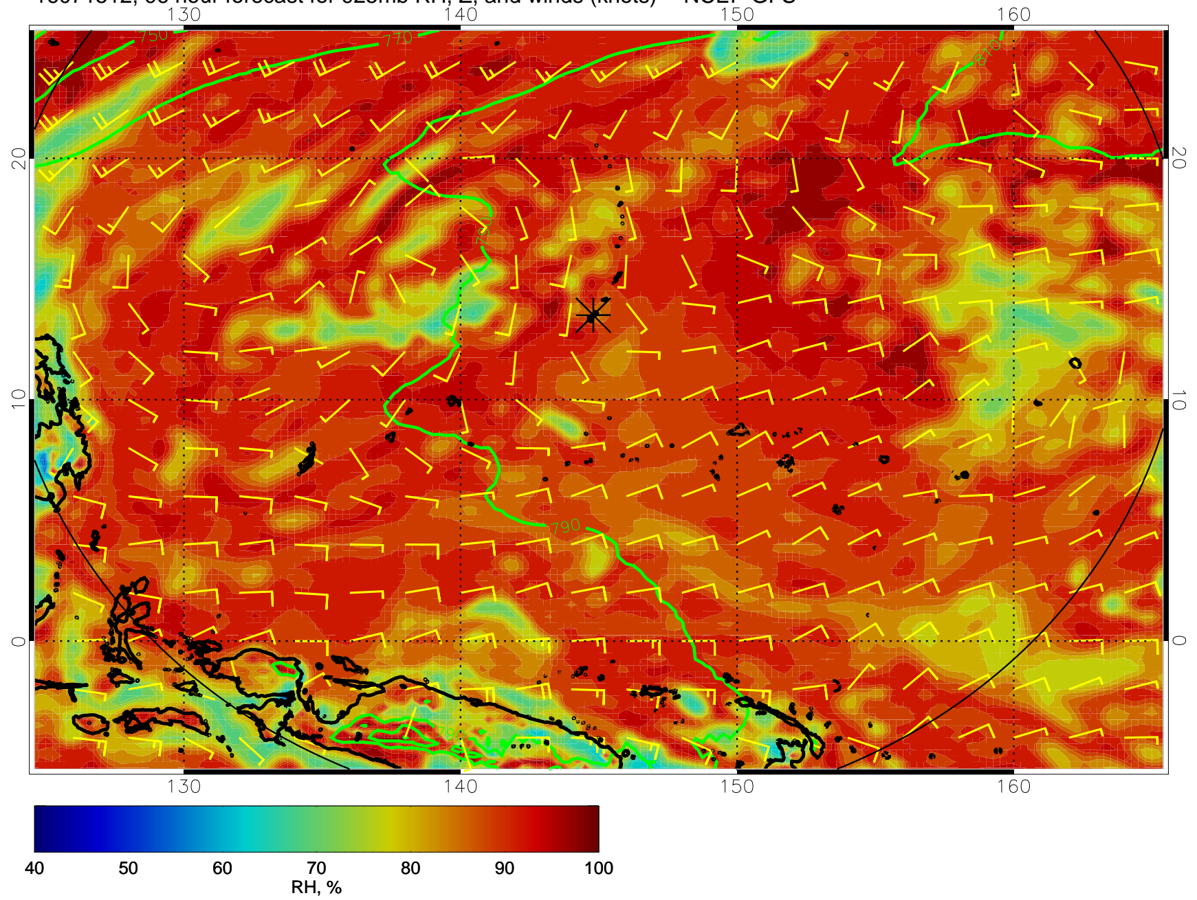
16071512, 96 hour forecast for 925mb RH, Z, and winds (knots) -- NCEP GFS
