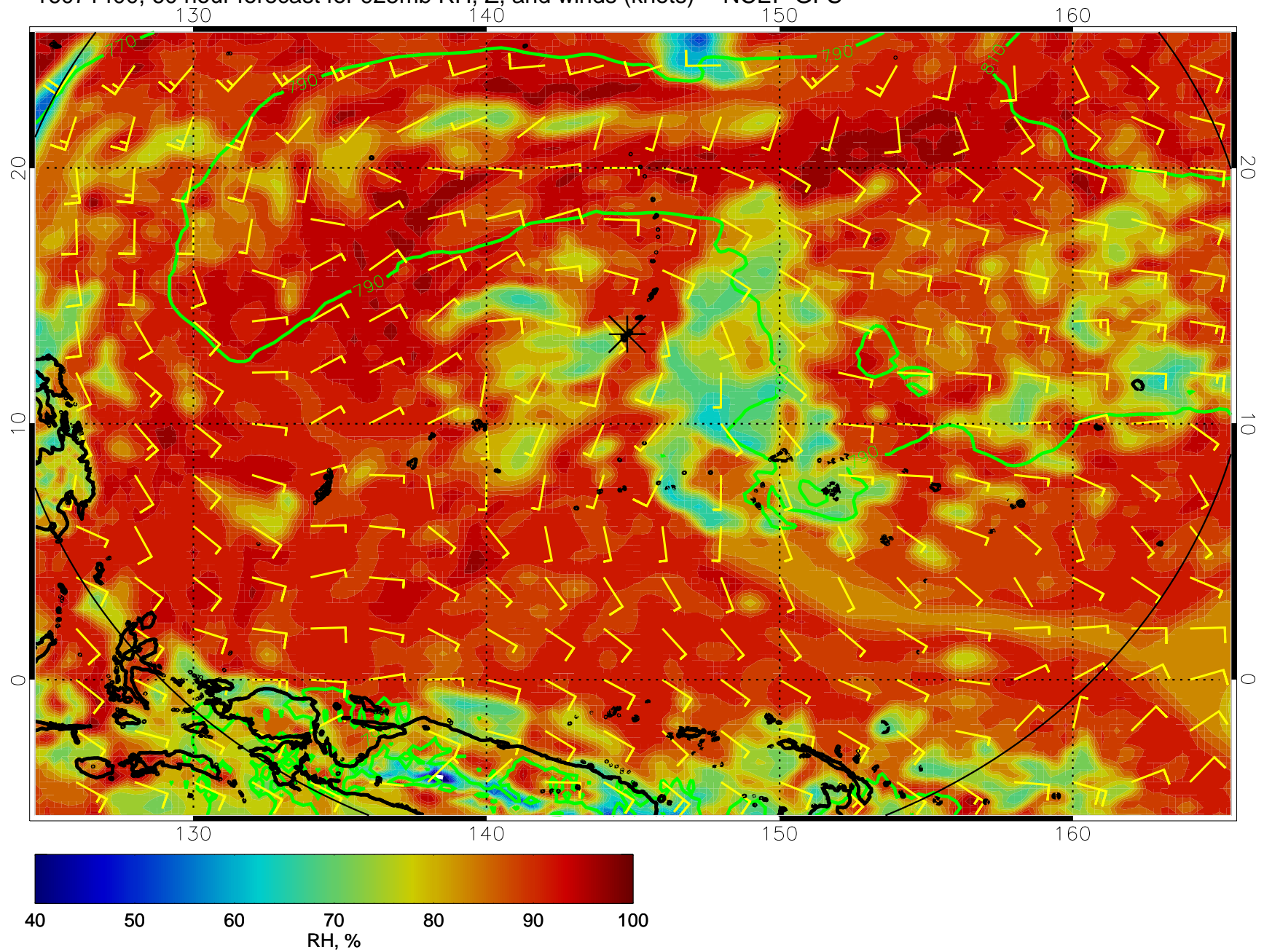
16071400, 60 hour forecast for 925mb RH, Z, and winds (knots) -- NCEP GFS
