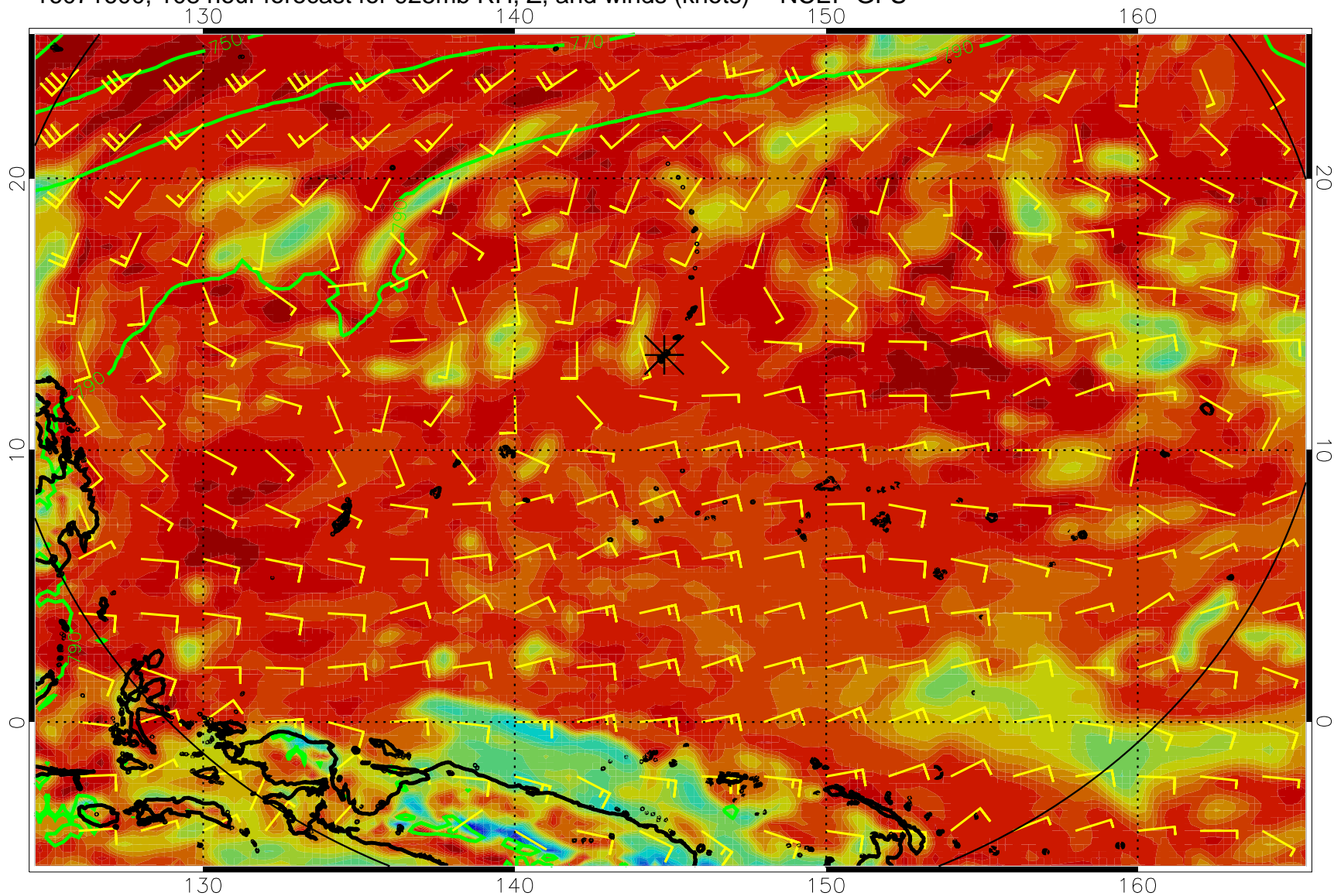
16071600, 108 hour forecast for 925mb RH, Z, and winds (knots) -- NCEP GFS
