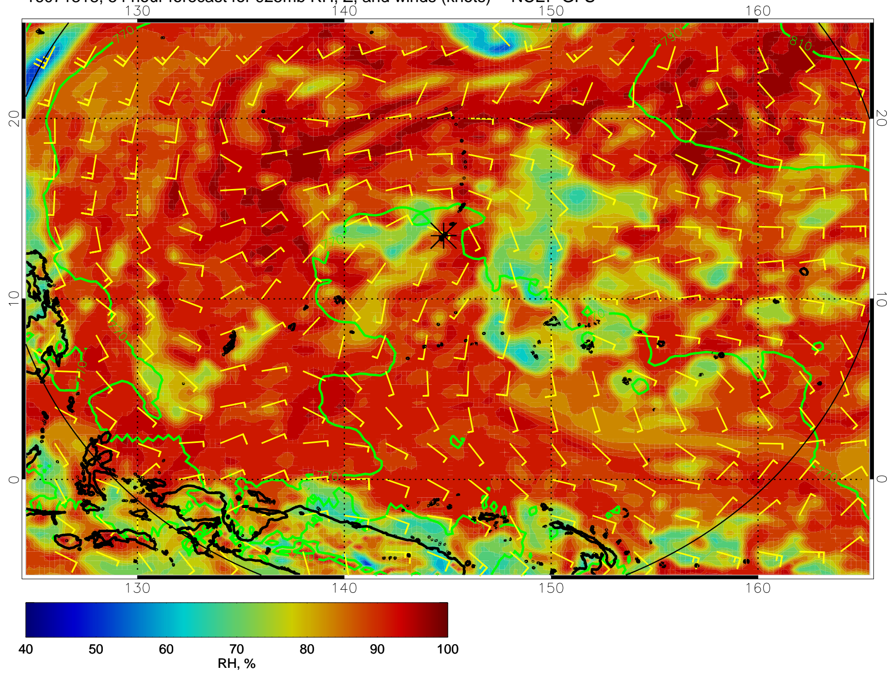
16071318, 54 hour forecast for 925mb RH, Z, and winds (knots) -- NCEP GFS
