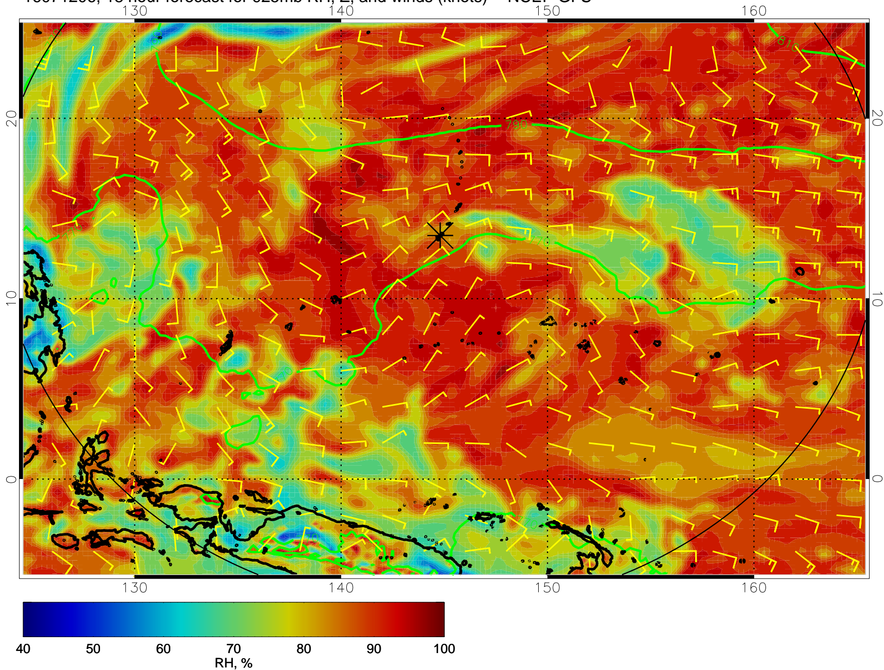
16071206, 18 hour forecast for 925mb RH, Z, and winds (knots) -- NCEP GFS
