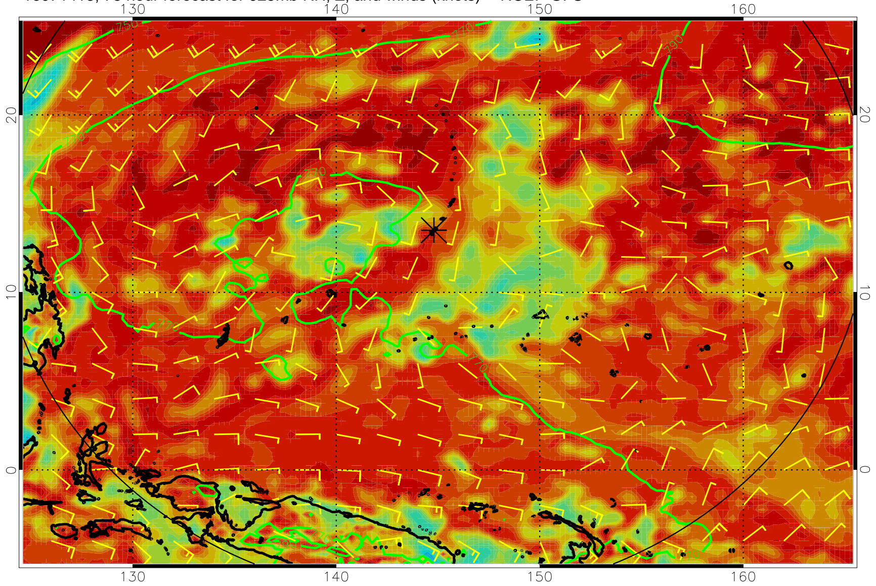
16071418, 78 hour forecast for 925mb RH, Z, and winds (knots) -- NCEP GFS
