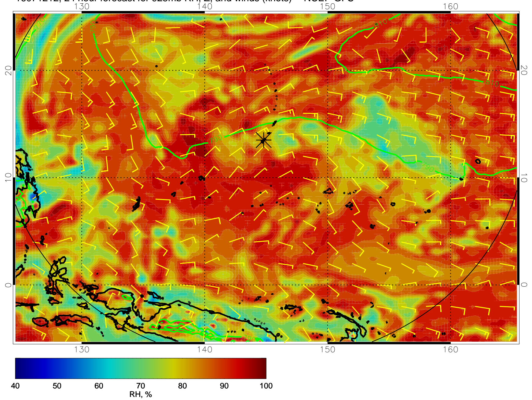
16071212, 24 hour forecast for 925mb RH, Z, and winds (knots) -- NCEP GFS
