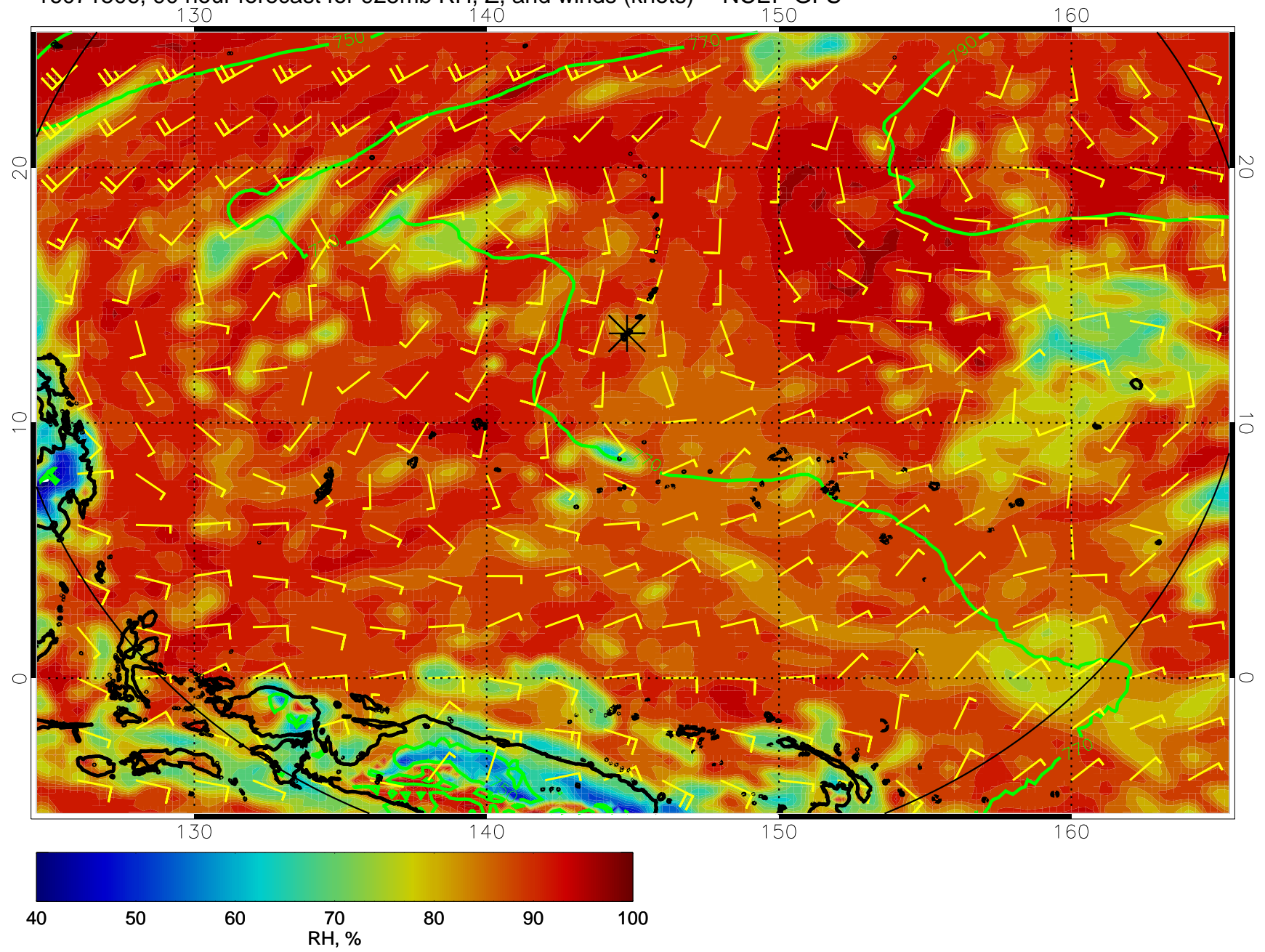
16071506, 90 hour forecast for 925mb RH, Z, and winds (knots) -- NCEP GFS
