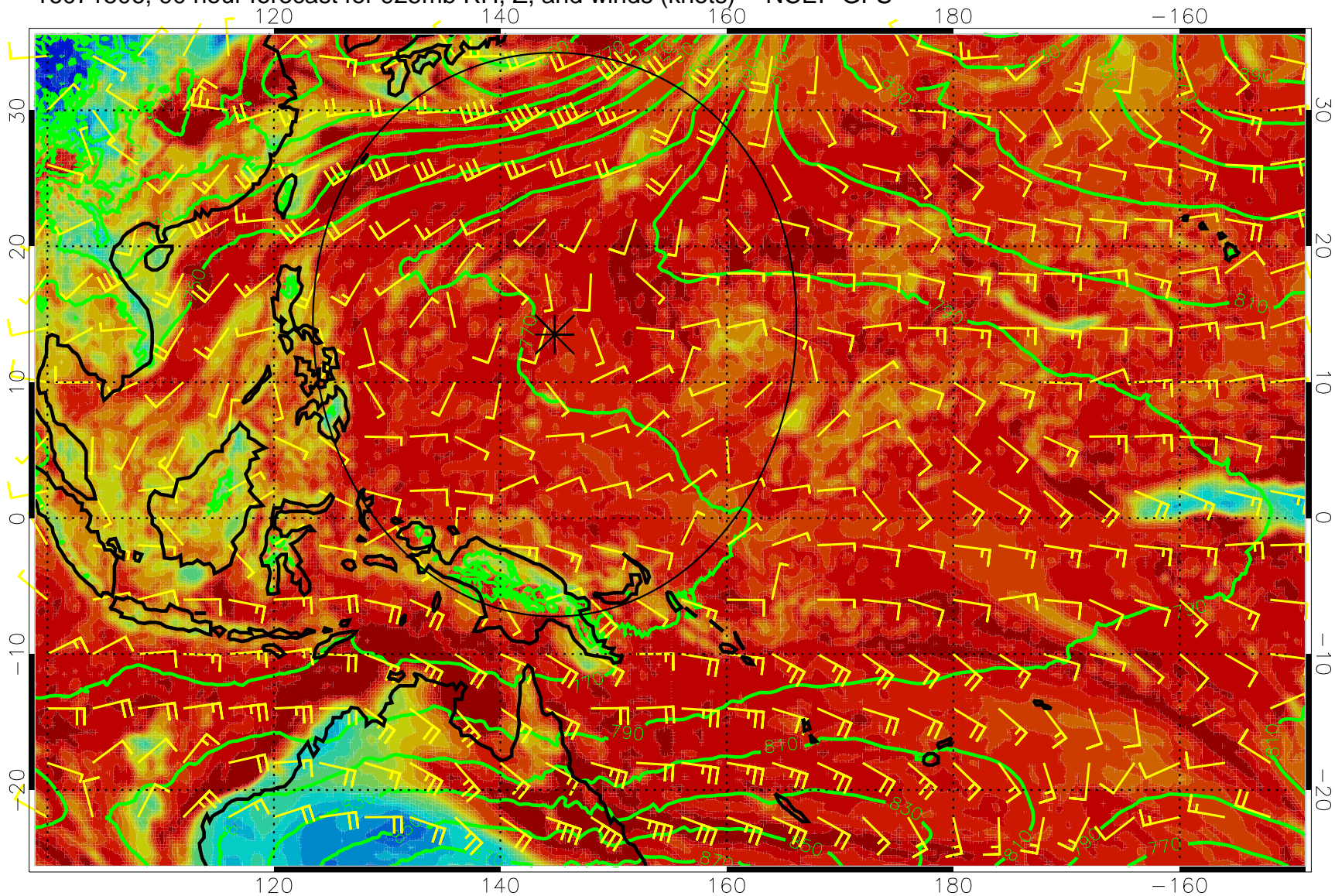
16071506, 90 hour forecast for 925mb RH, Z, and winds (knots) -- NCEP GFS
