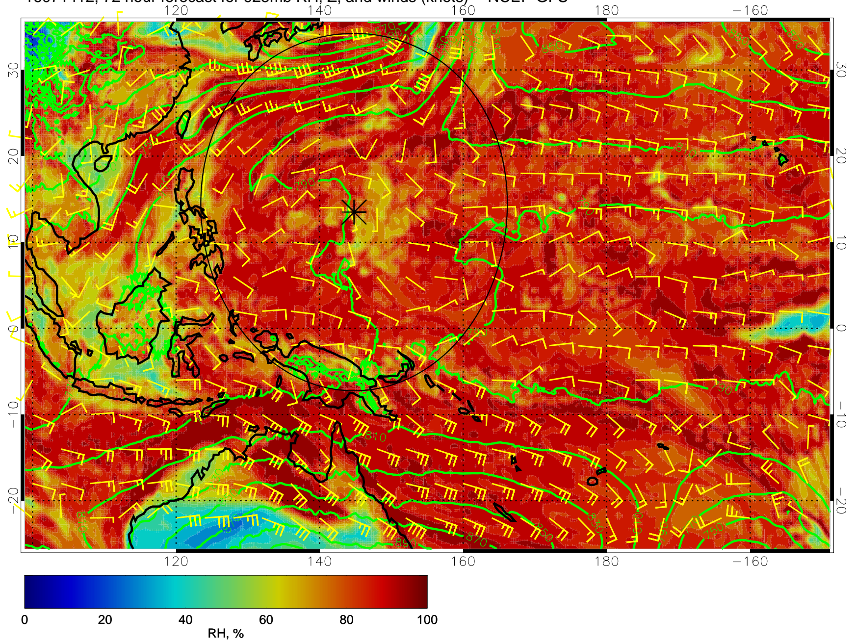
16071412, 72 hour forecast for 925mb RH, Z, and winds (knots) -- NCEP GFS
