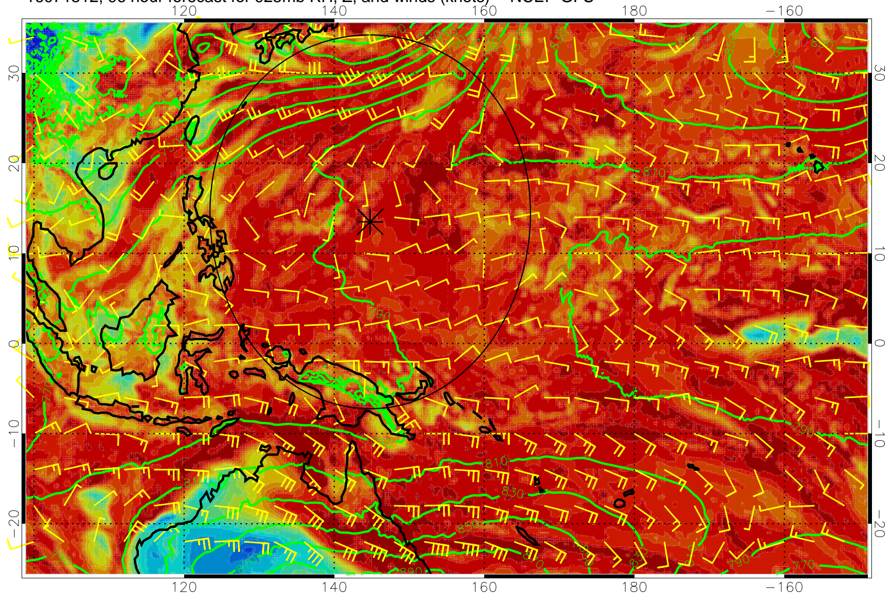
16071512, 96 hour forecast for 925mb RH, Z, and winds (knots) -- NCEP GFS
