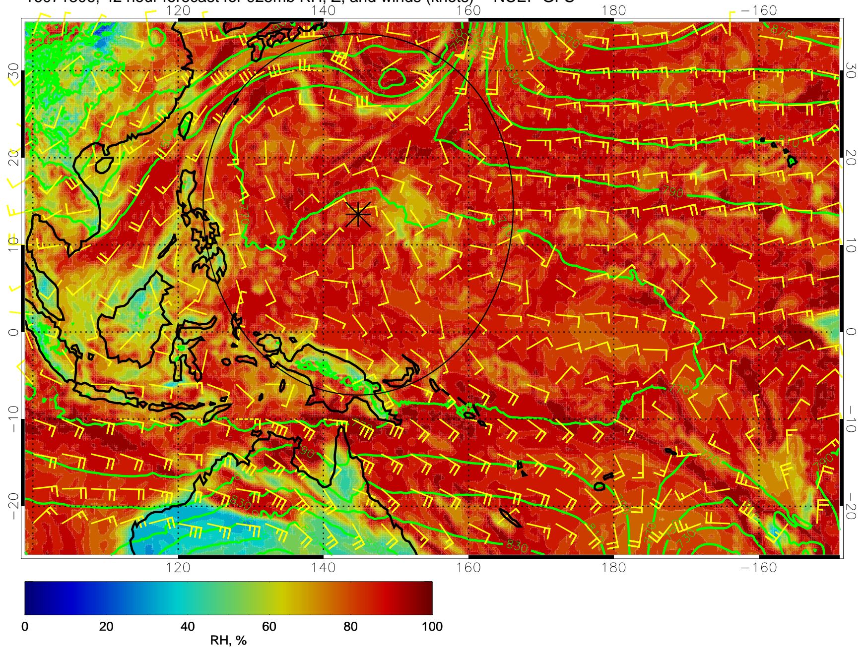
16071306, 42 hour forecast for 925mb RH, Z, and winds (knots) -- NCEP GFS
