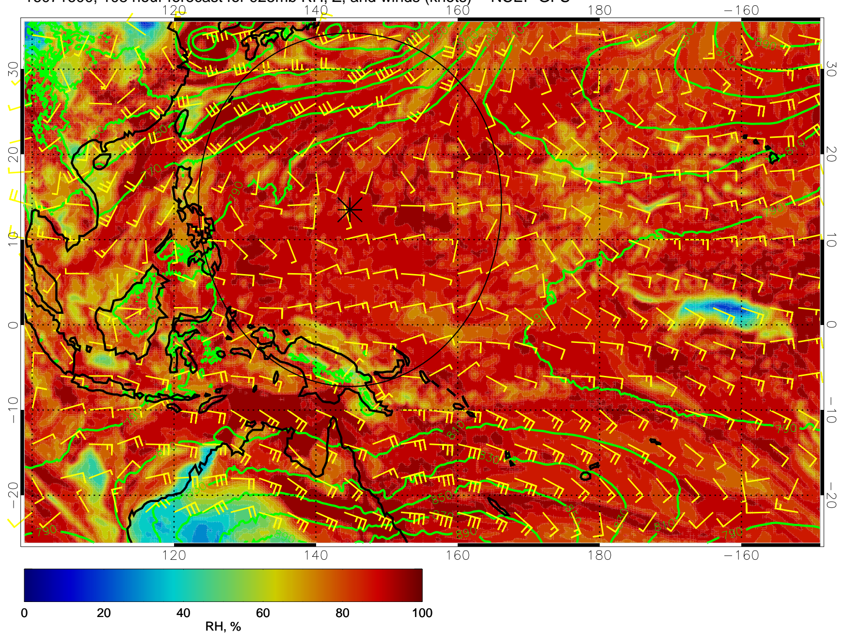
16071600, 108 hour forecast for 925mb RH, Z, and winds (knots) -- NCEP GFS
