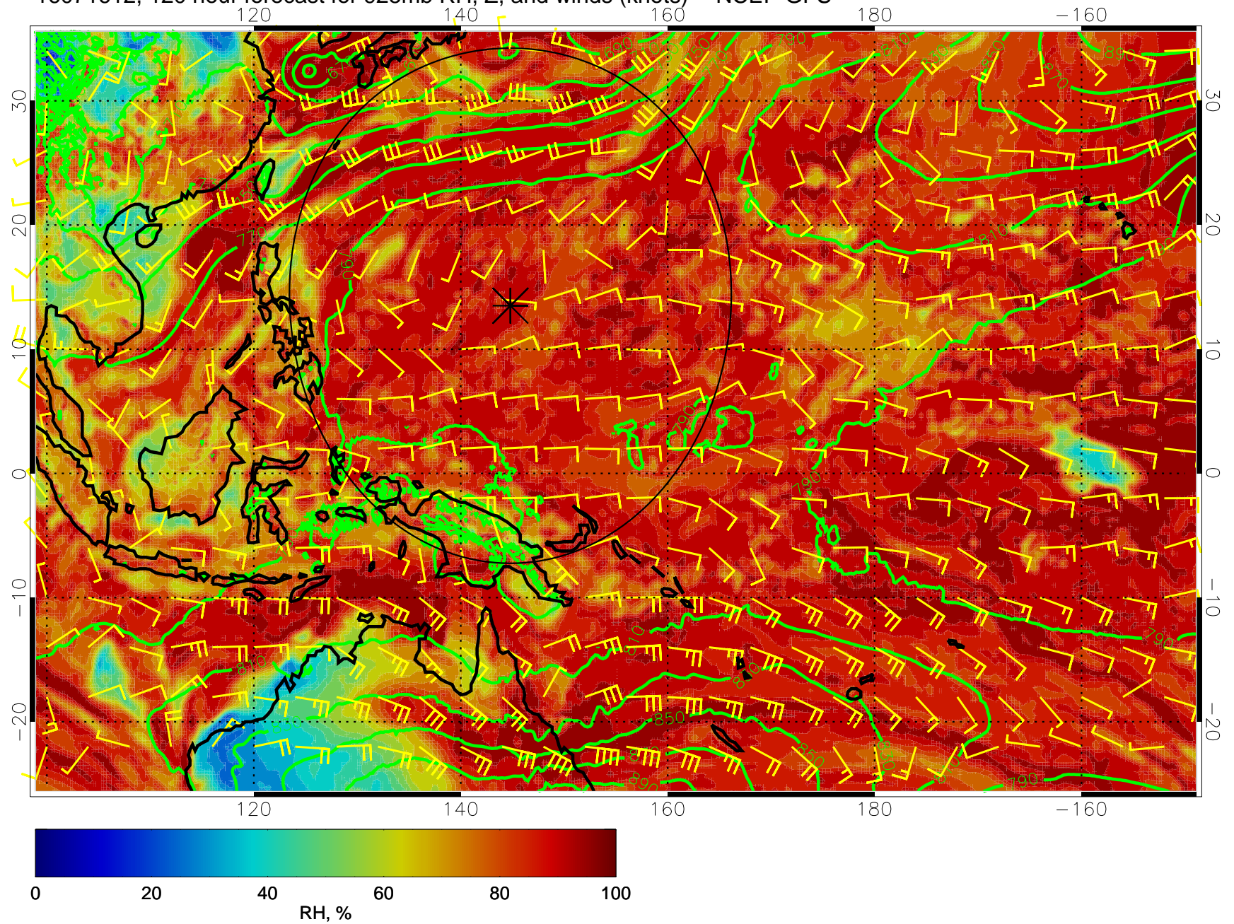
16071612, 120 hour forecast for 925mb RH, Z, and winds (knots) -- NCEP GFS
