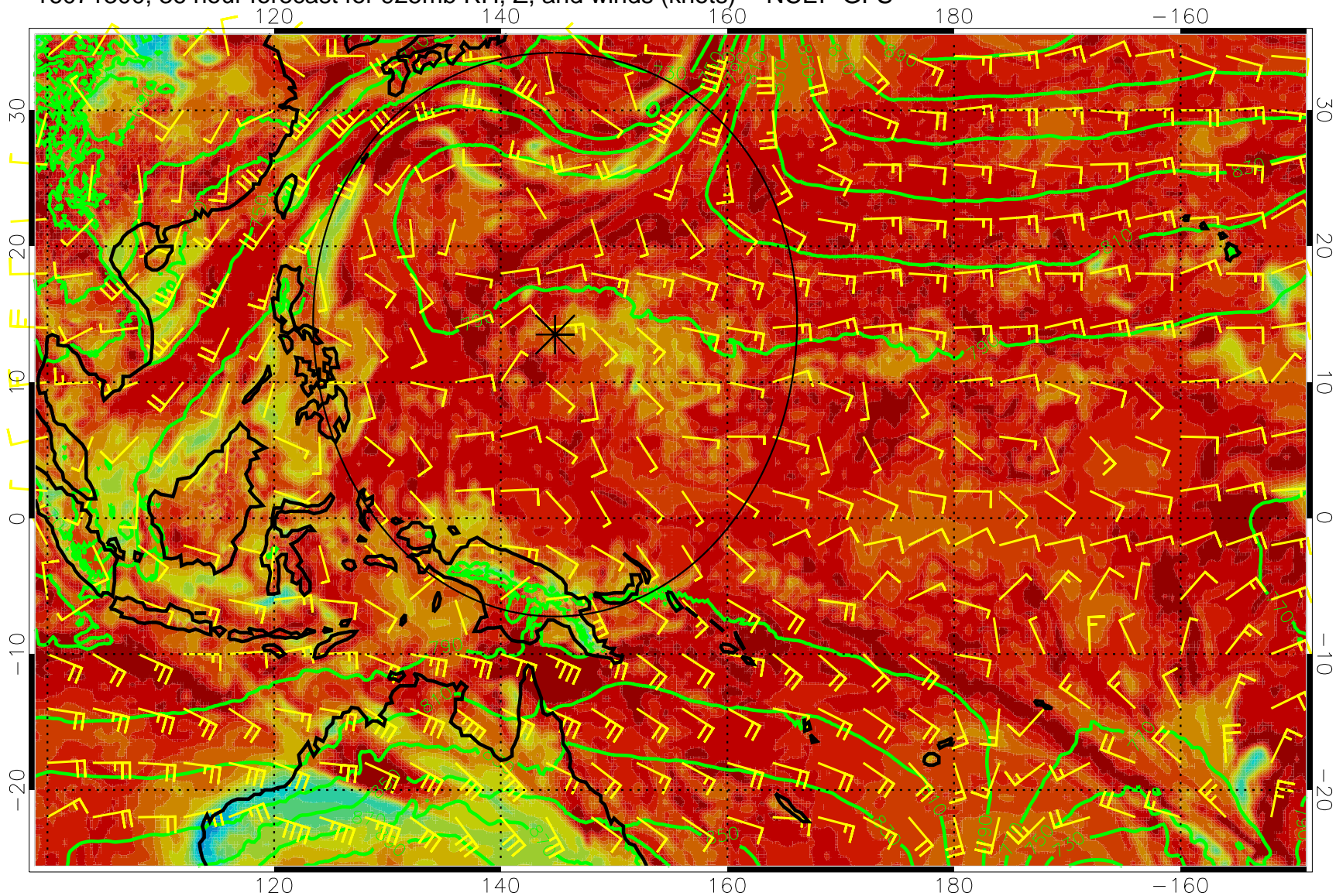
16071300, 36 hour forecast for 925mb RH, Z, and winds (knots) -- NCEP GFS
