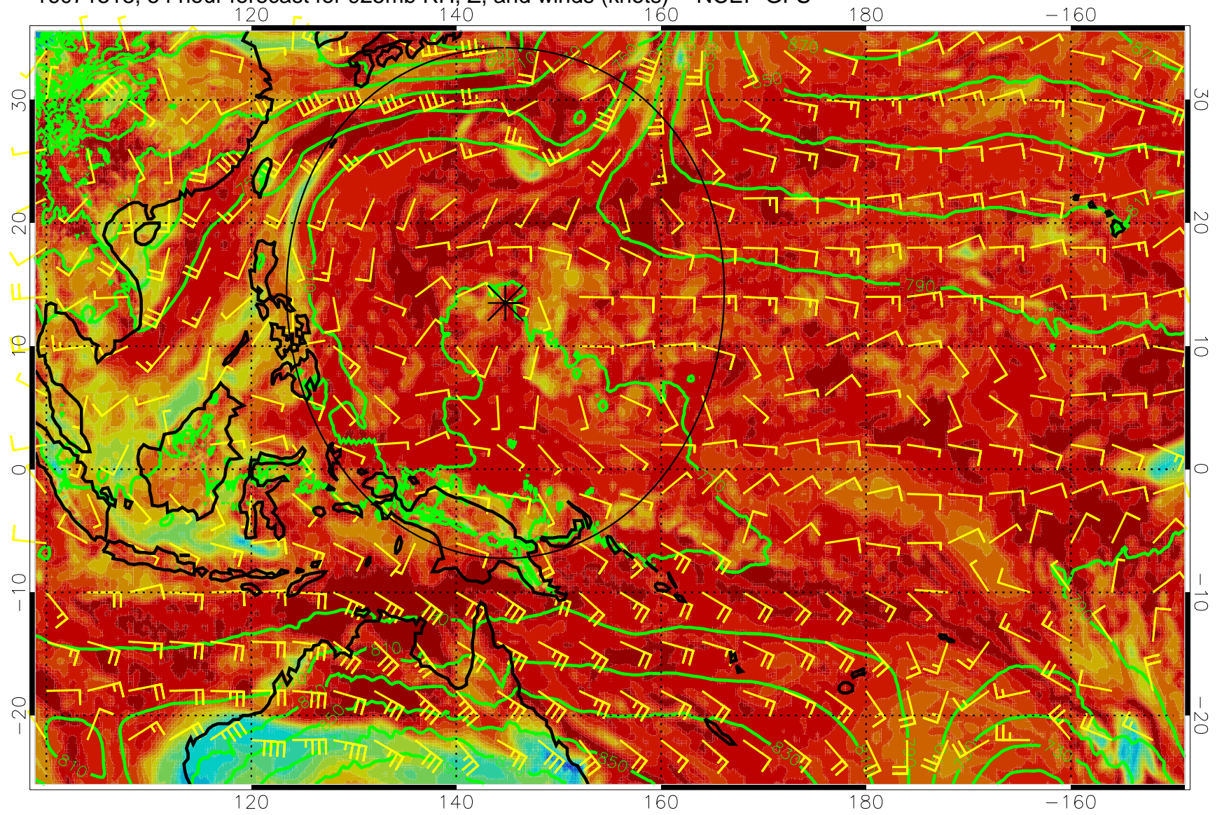
16071318, 54 hour forecast for 925mb RH, Z, and winds (knots) -- NCEP GFS
