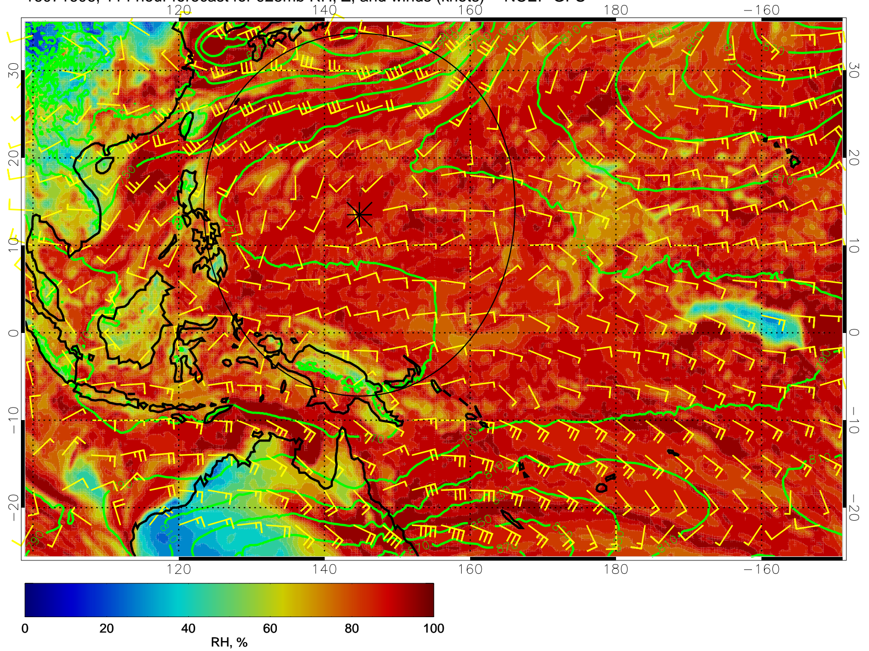
16071606, 114 hour forecast for 925mb RH, Z, and winds (knots) -- NCEP GFS
