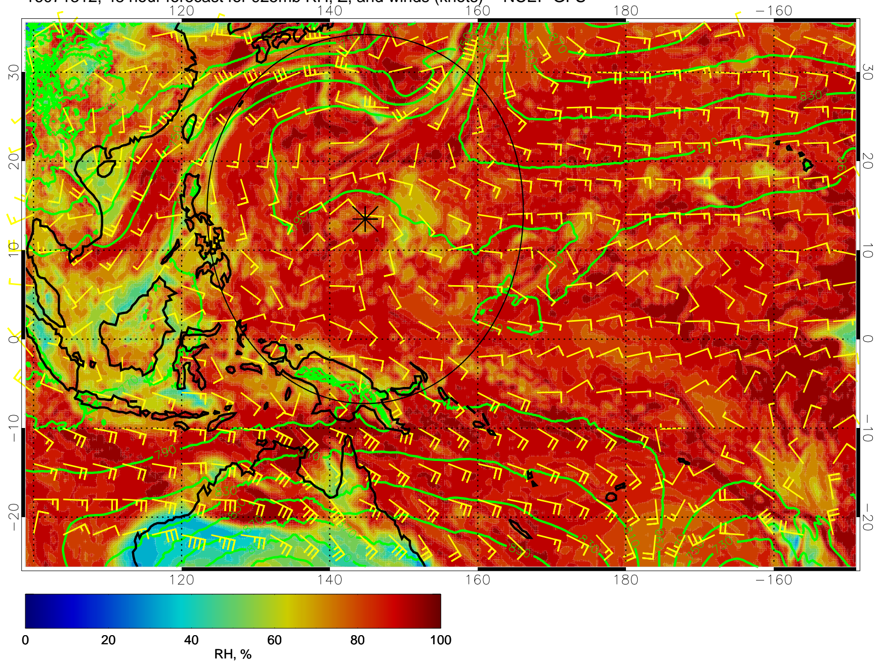
16071312, 48 hour forecast for 925mb RH, Z, and winds (knots) -- NCEP GFS
