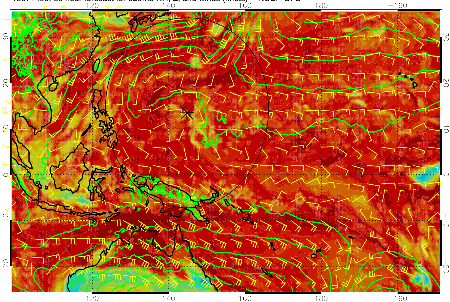
16071400, 60 hour forecast for 925mb RH, Z, and winds (knots) -- NCEP GFS
