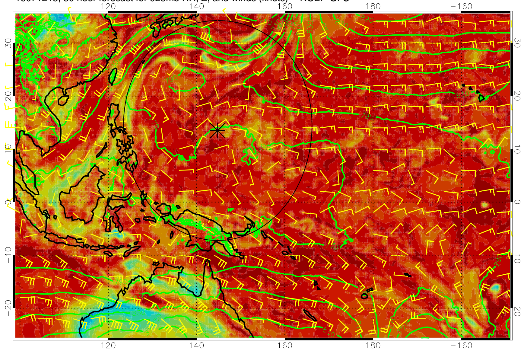
16071218, 30 hour forecast for 925mb RH, Z, and winds (knots) -- NCEP GFS
