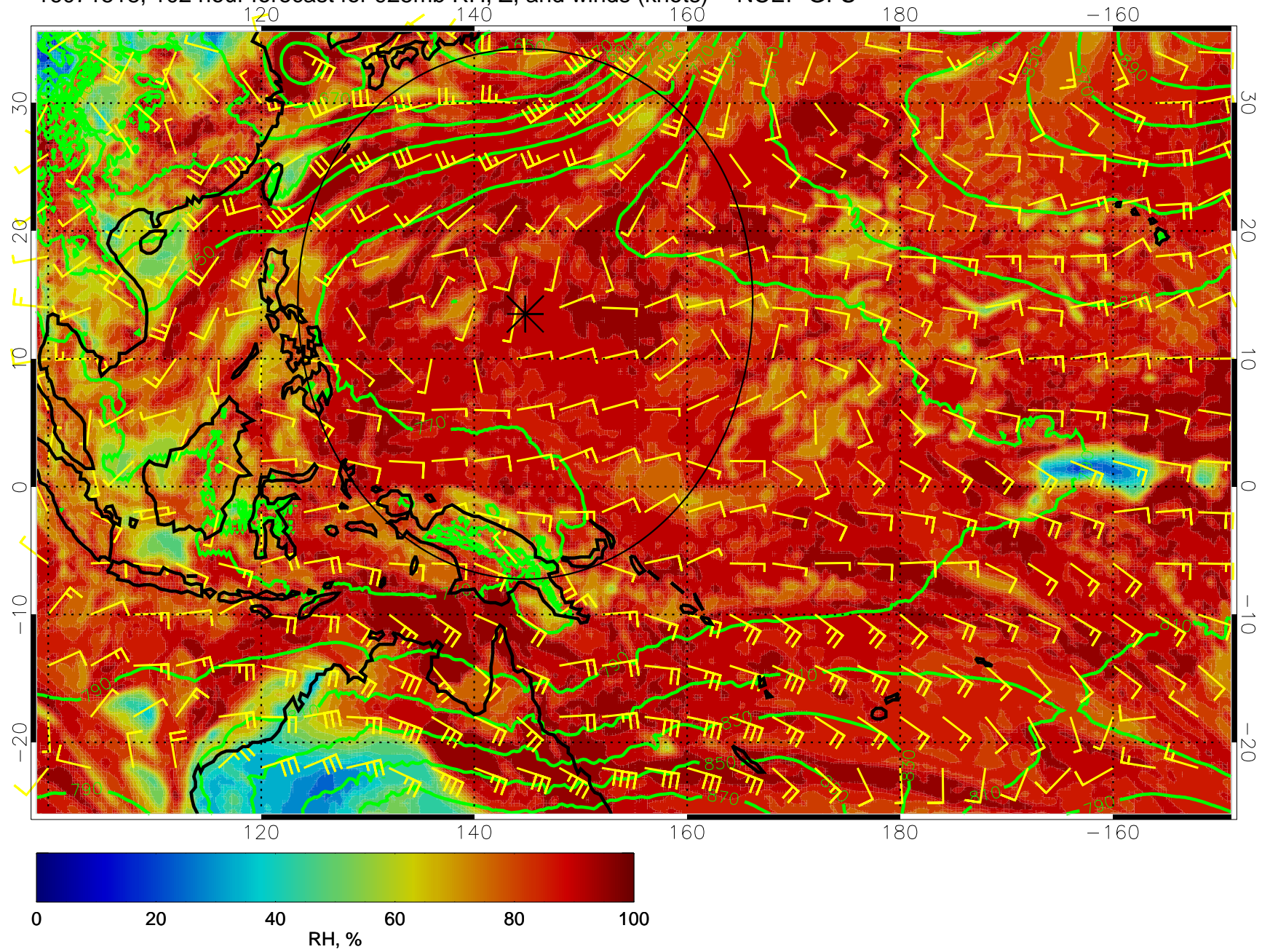
16071518, 102 hour forecast for 925mb RH, Z, and winds (knots) -- NCEP GFS
