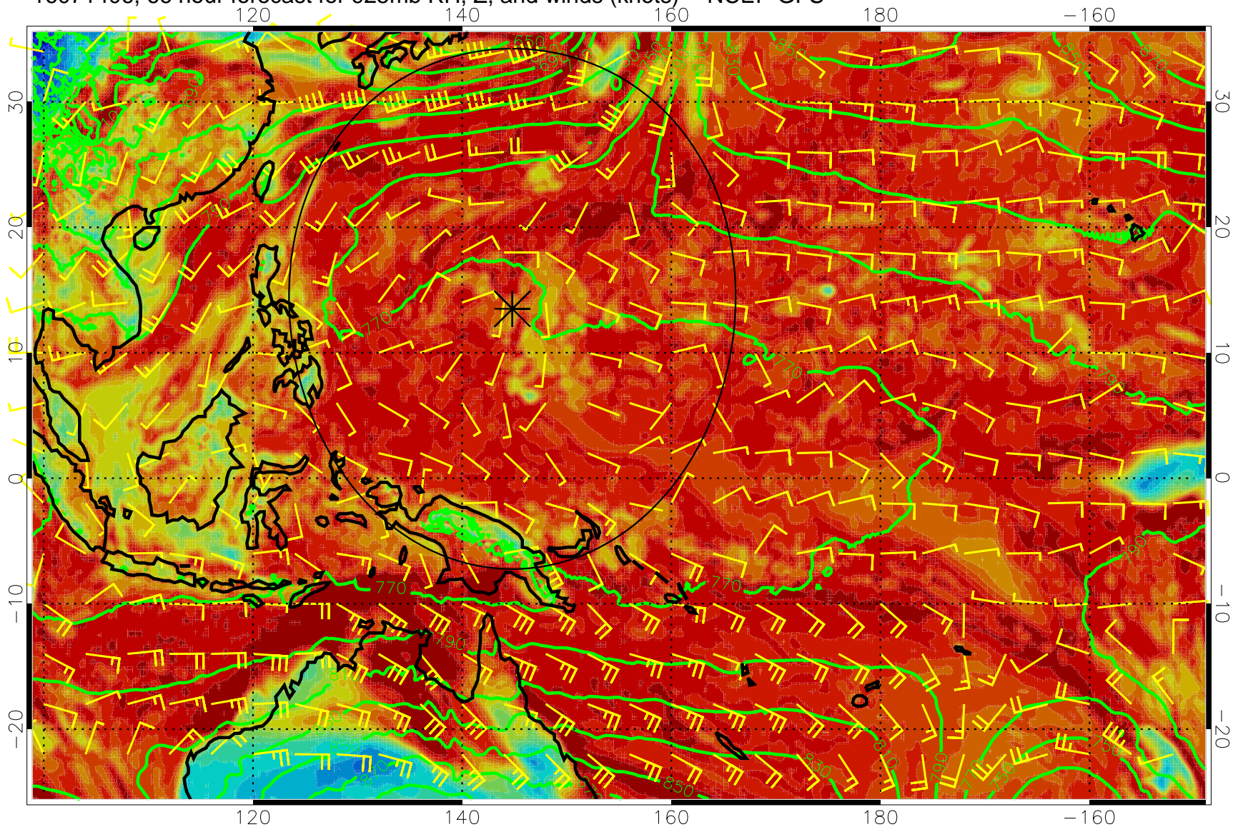
16071406, 66 hour forecast for 925mb RH, Z, and winds (knots) -- NCEP GFS
