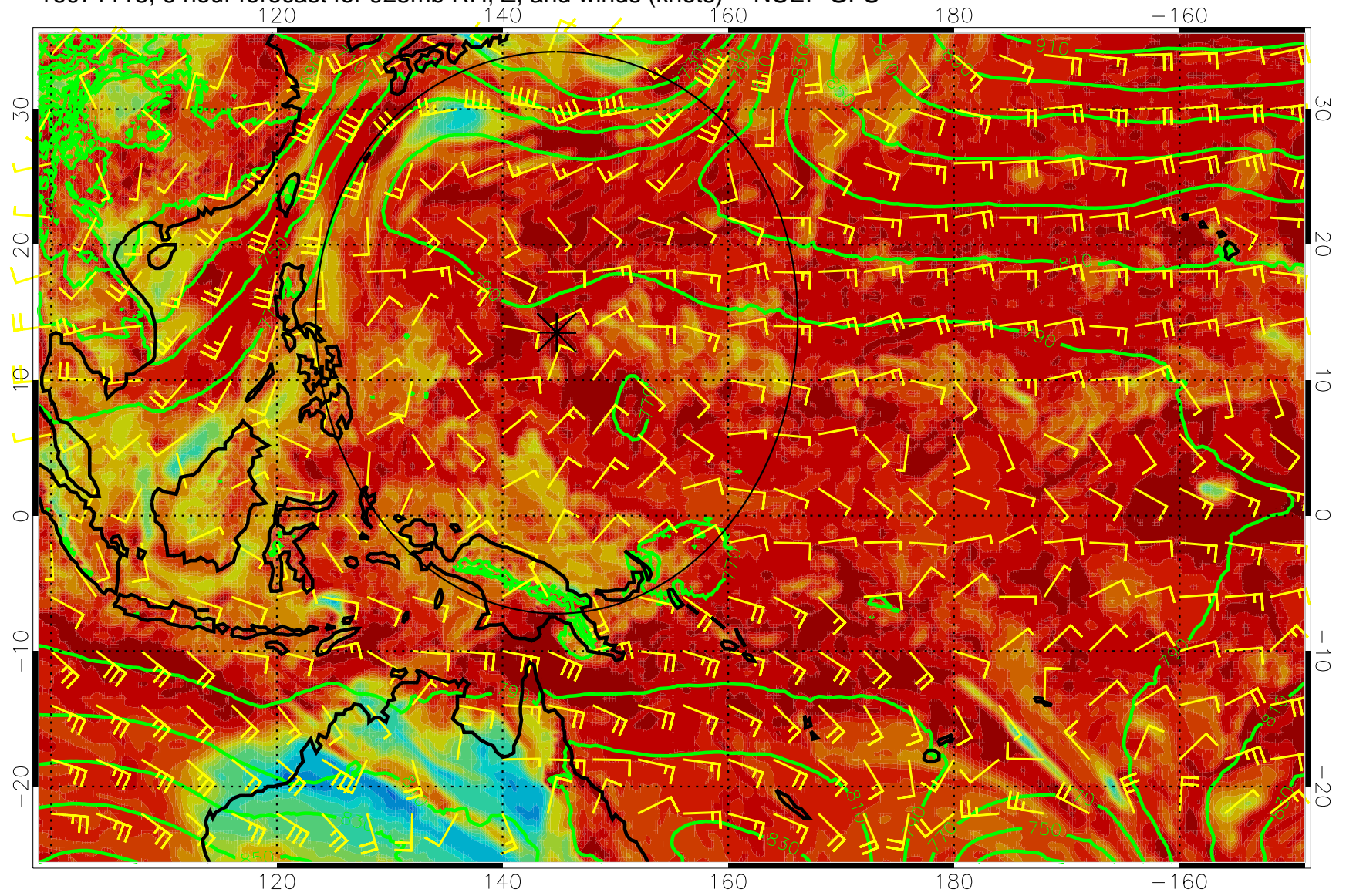
16071118, 6 hour forecast for 925mb RH, Z, and winds (knots) -- NCEP GFS
