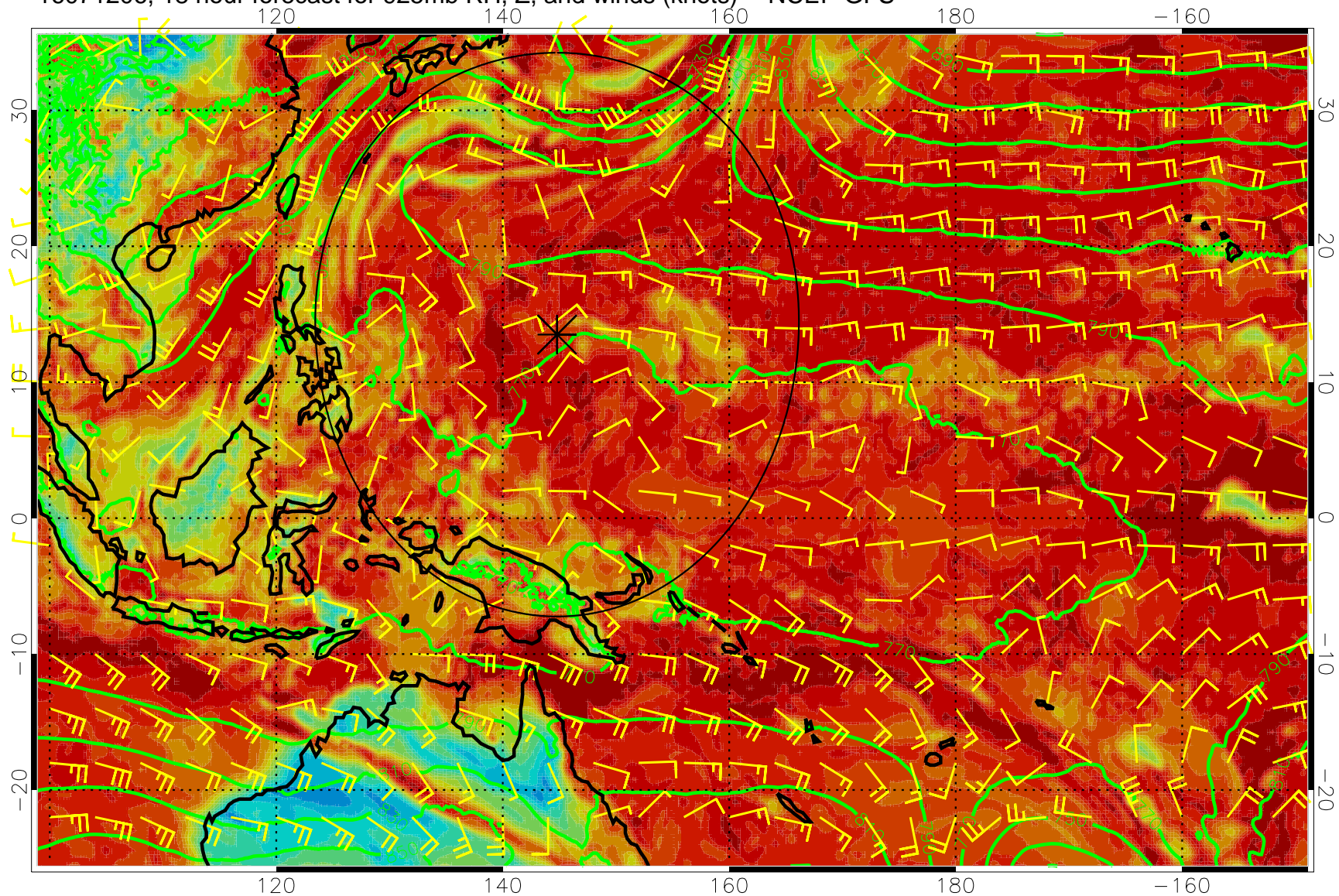
16071206, 18 hour forecast for 925mb RH, Z, and winds (knots) -- NCEP GFS
