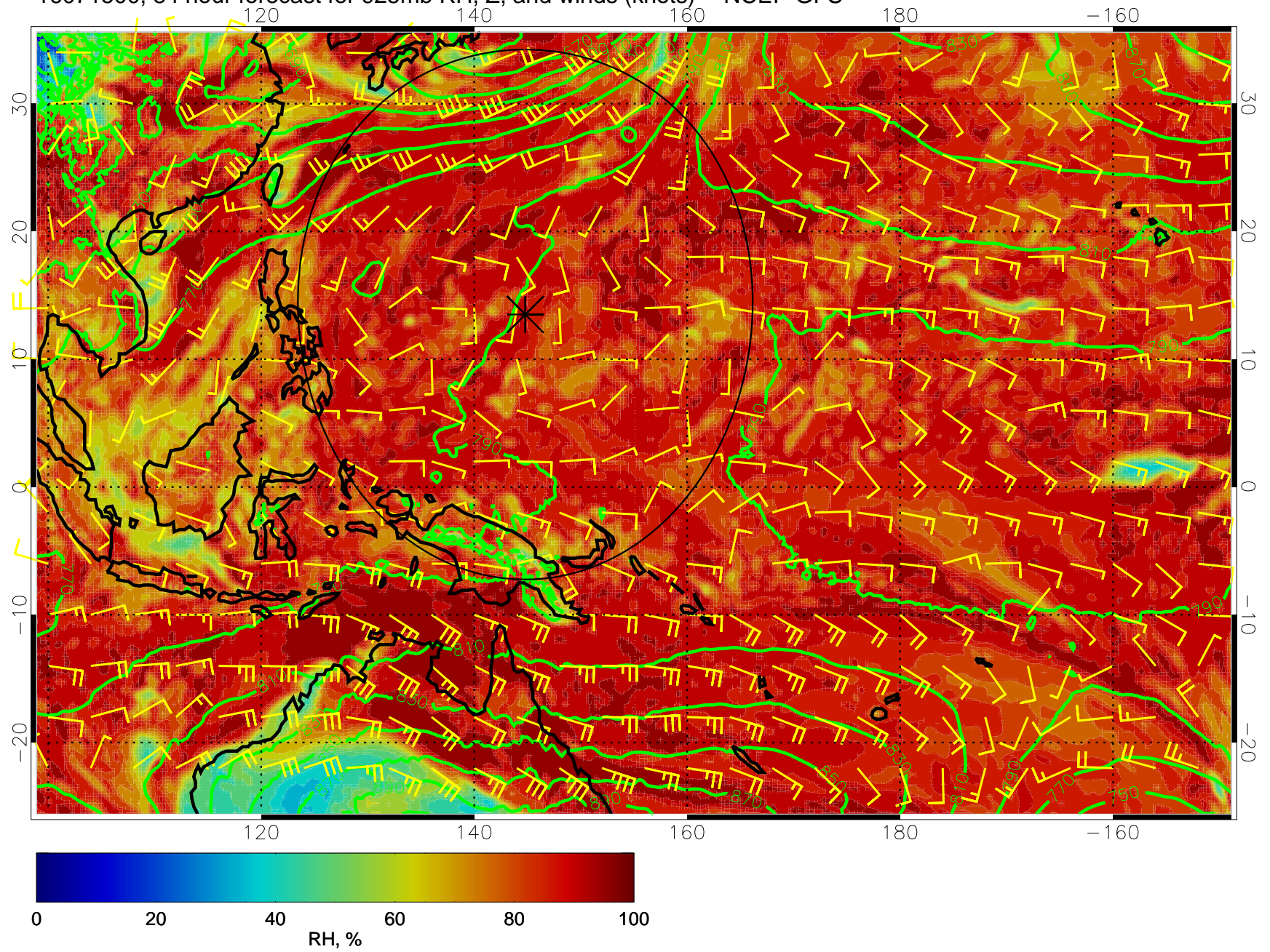
16071500, 84 hour forecast for 925mb RH, Z, and winds (knots) -- NCEP GFS
