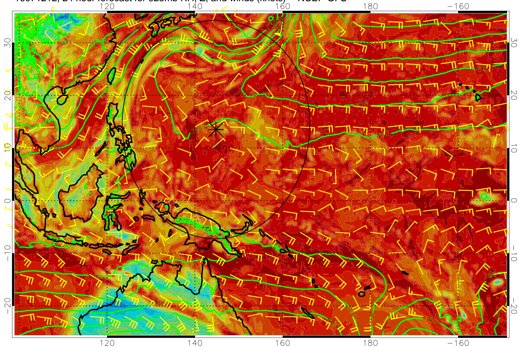
16071212, 24 hour forecast for 925mb RH, Z, and winds (knots) -- NCEP GFS
