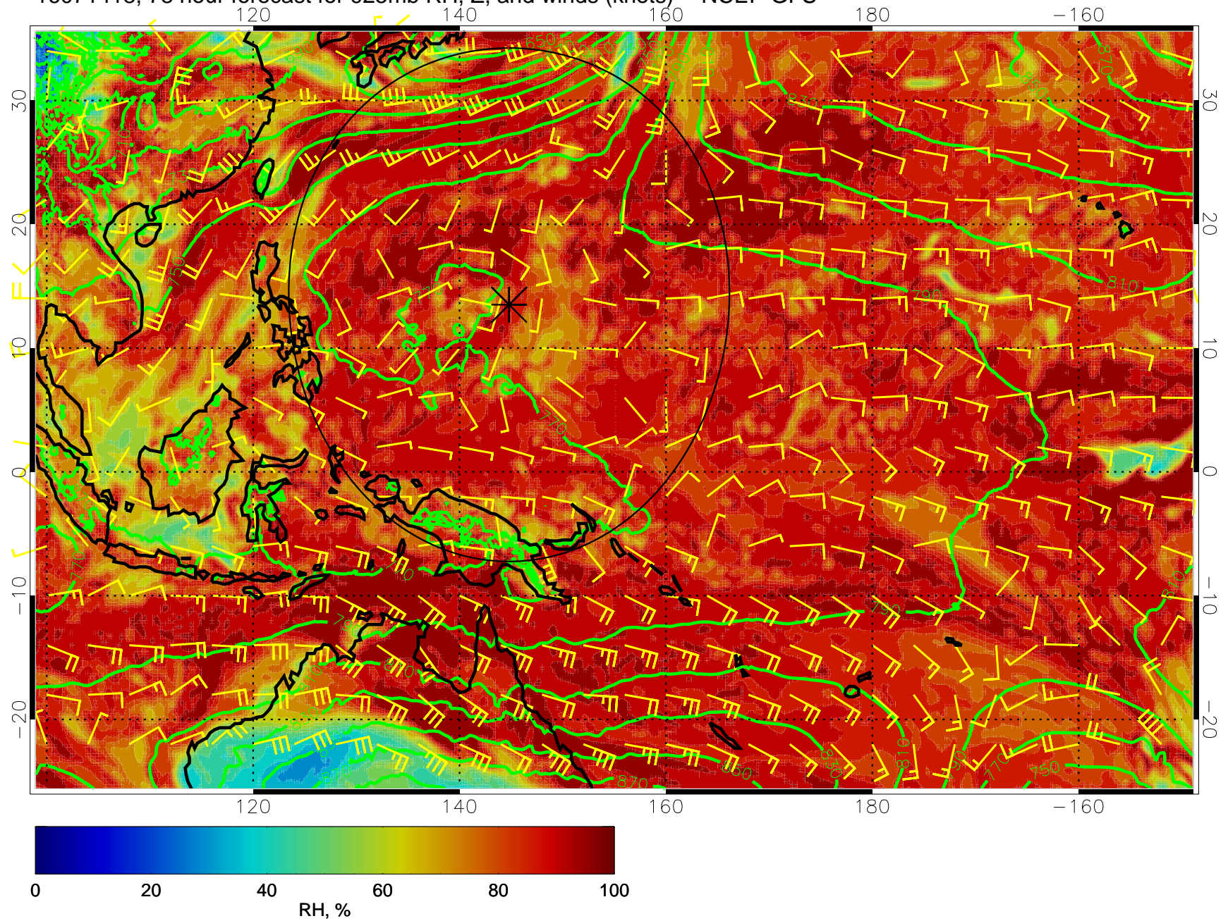
16071418, 78 hour forecast for 925mb RH, Z, and winds (knots) -- NCEP GFS
