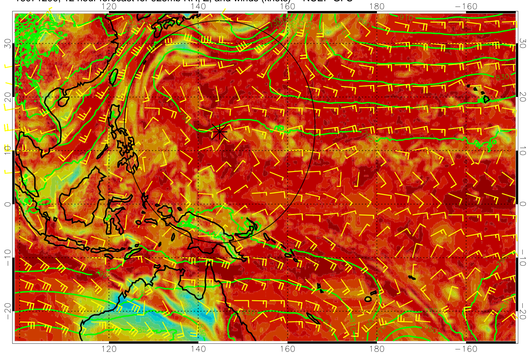
16071200, 12 hour forecast for 925mb RH, Z, and winds (knots) -- NCEP GFS
