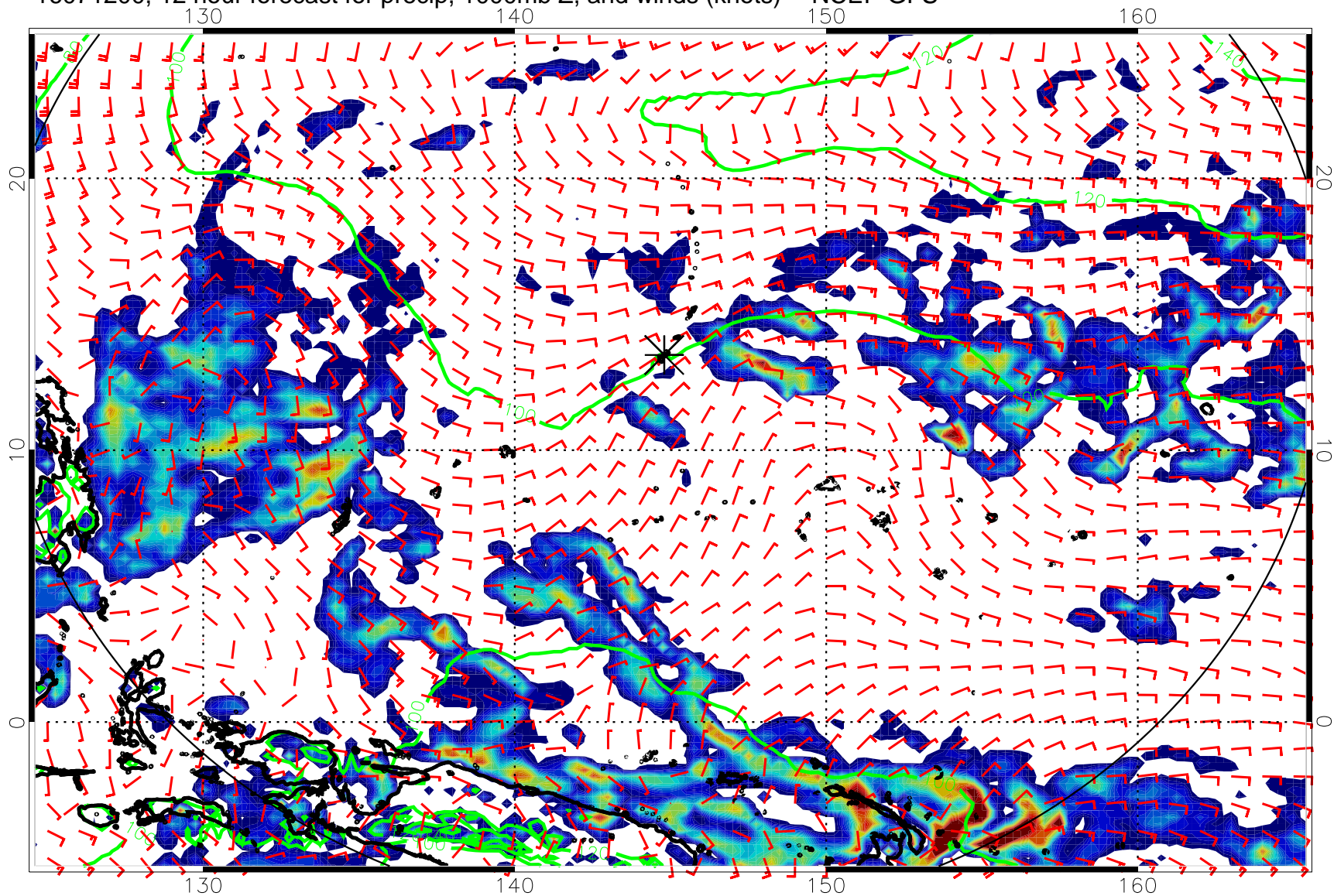
16071200, 12 hour forecast for precip, 1000mb Z, and winds (knots) -- NCEP GFS
