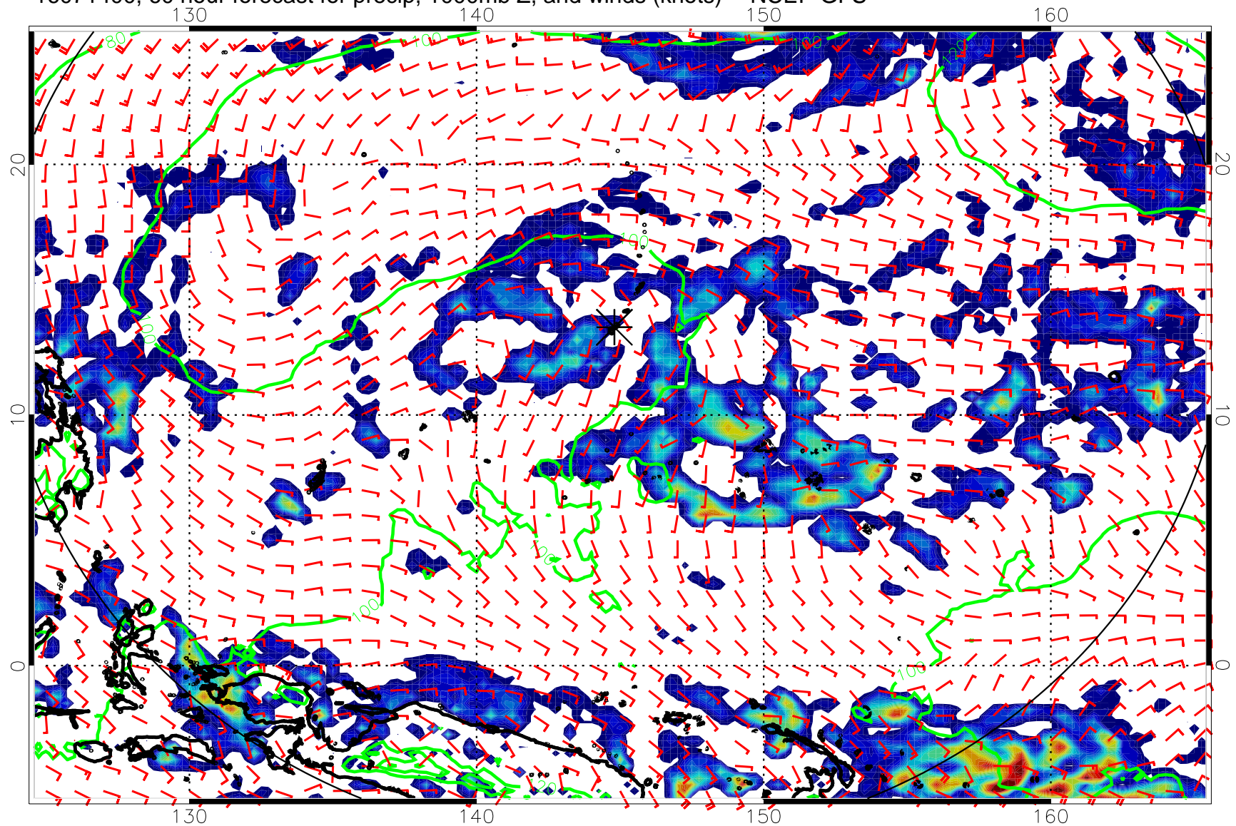
16071400, 60 hour forecast for precip, 1000mb Z, and winds (knots) -- NCEP GFS
