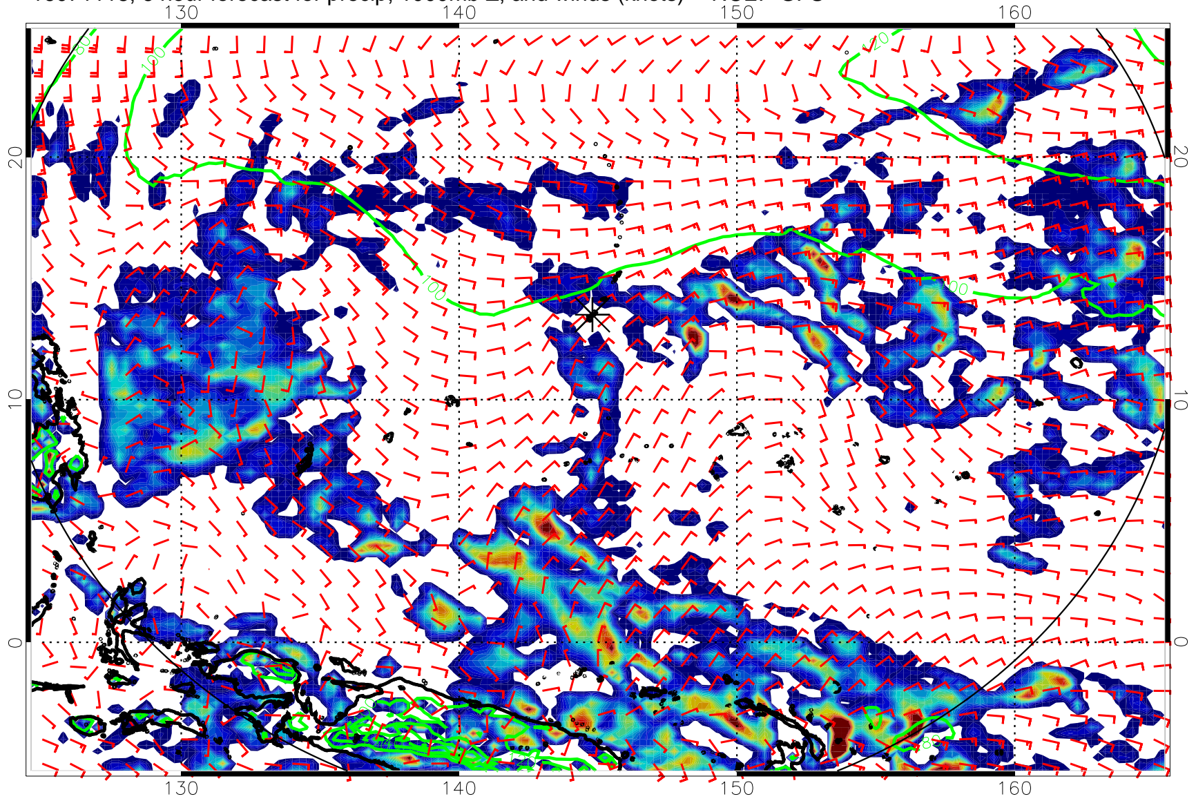
16071118, 6 hour forecast for precip, 1000mb Z, and winds (knots) -- NCEP GFS
