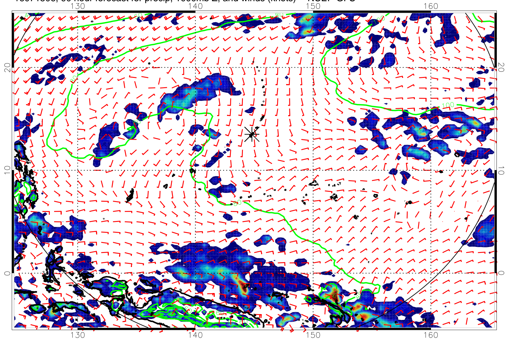
16071506, 90 hour forecast for precip, 1000mb Z, and winds (knots) -- NCEP GFS
