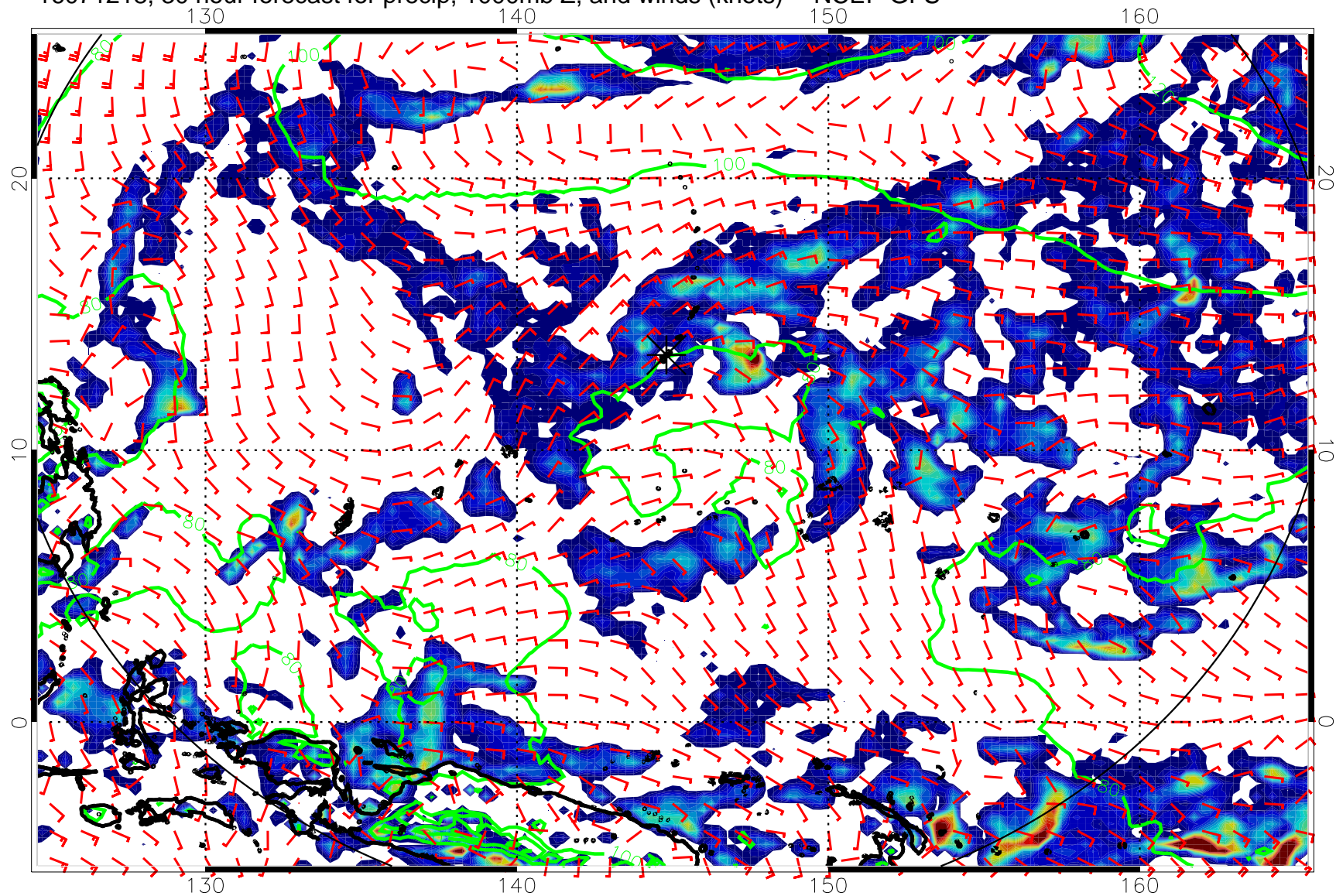
16071218, 30 hour forecast for precip, 1000mb Z, and winds (knots) -- NCEP GFS
