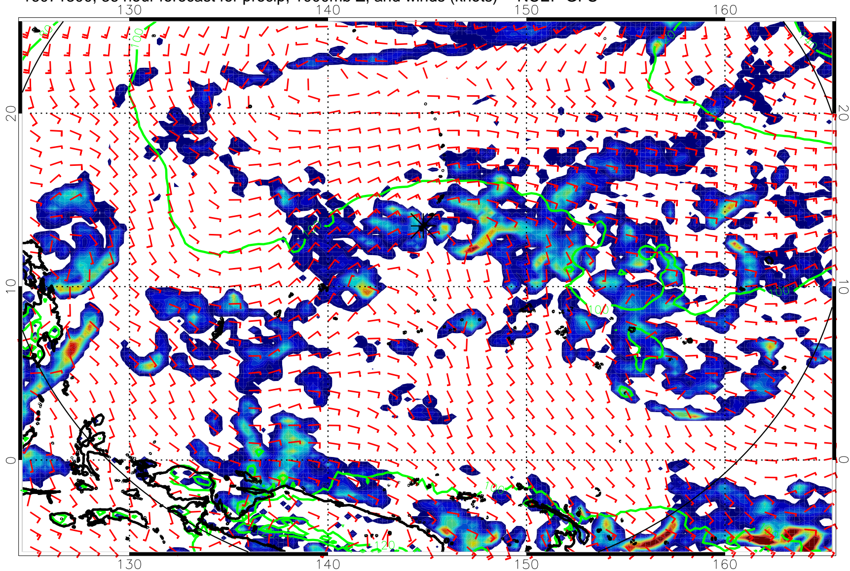
16071300, 36 hour forecast for precip, 1000mb Z, and winds (knots) -- NCEP GFS
