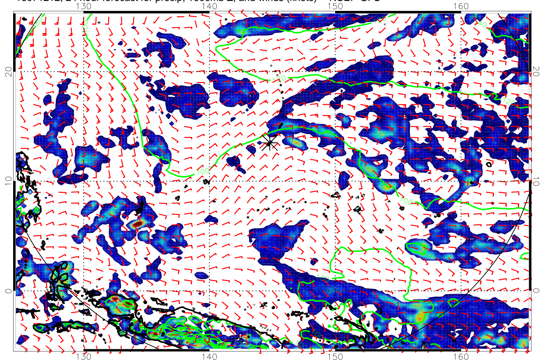
16071212, 24 hour forecast for precip, 1000mb Z, and winds (knots) -- NCEP GFS
