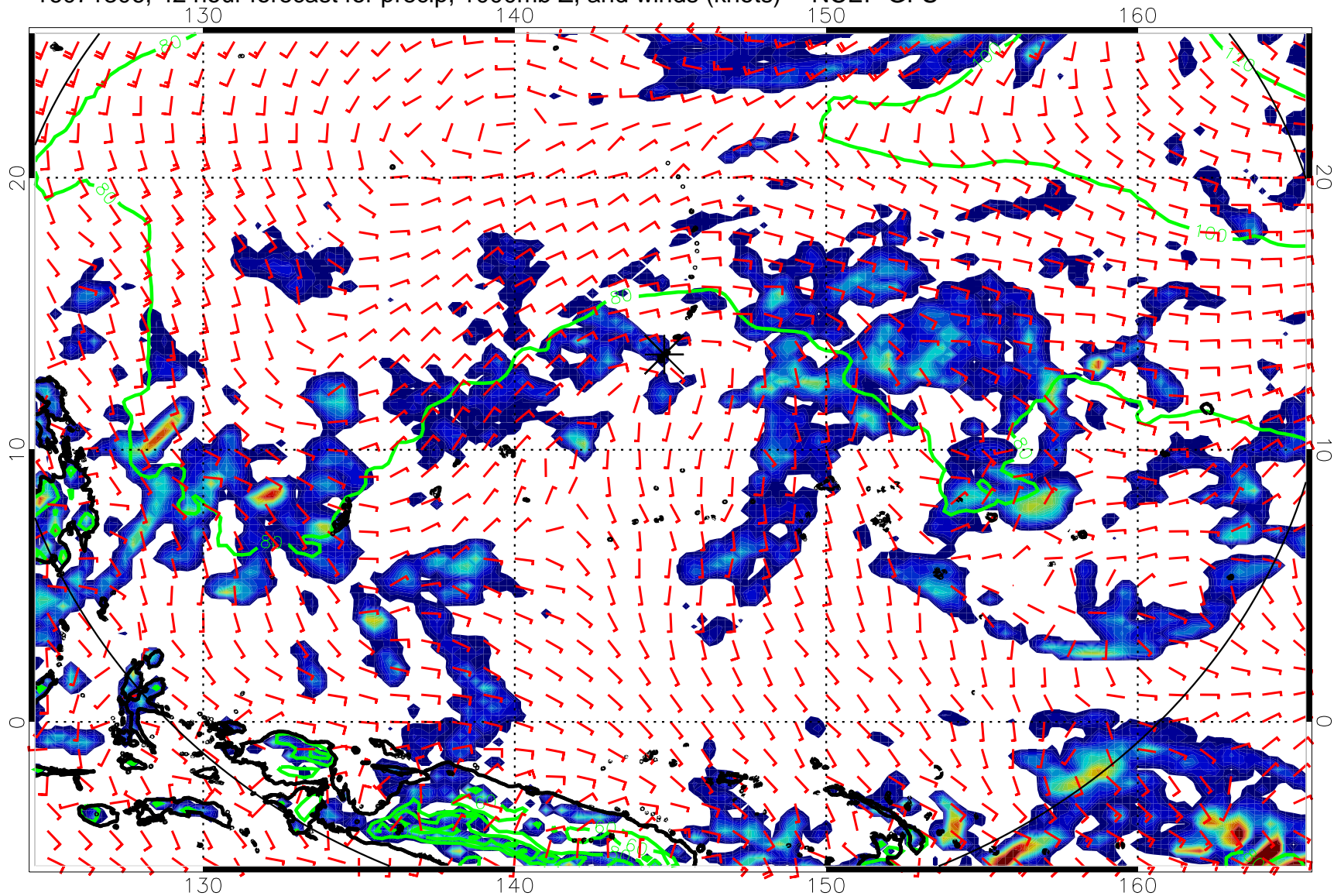
16071306, 42 hour forecast for precip, 1000mb Z, and winds (knots) -- NCEP GFS
