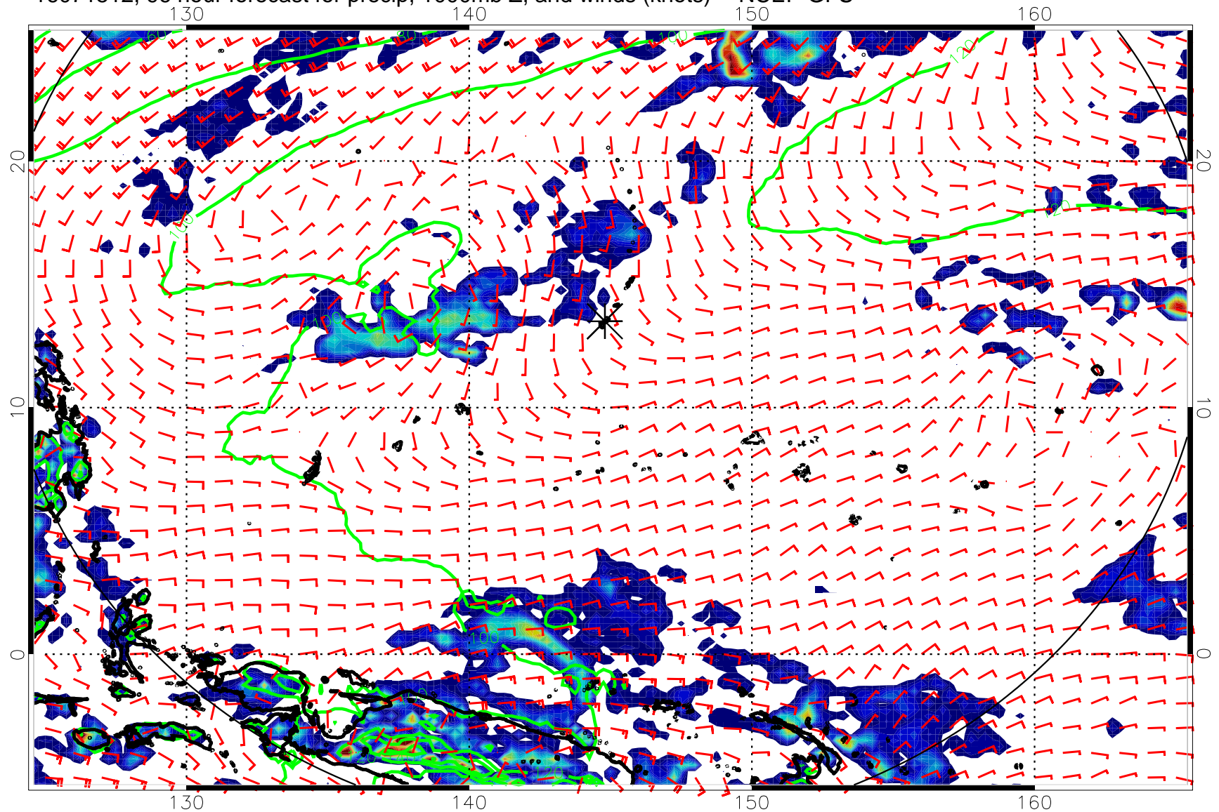
16071512, 96 hour forecast for precip, 1000mb Z, and winds (knots) -- NCEP GFS
