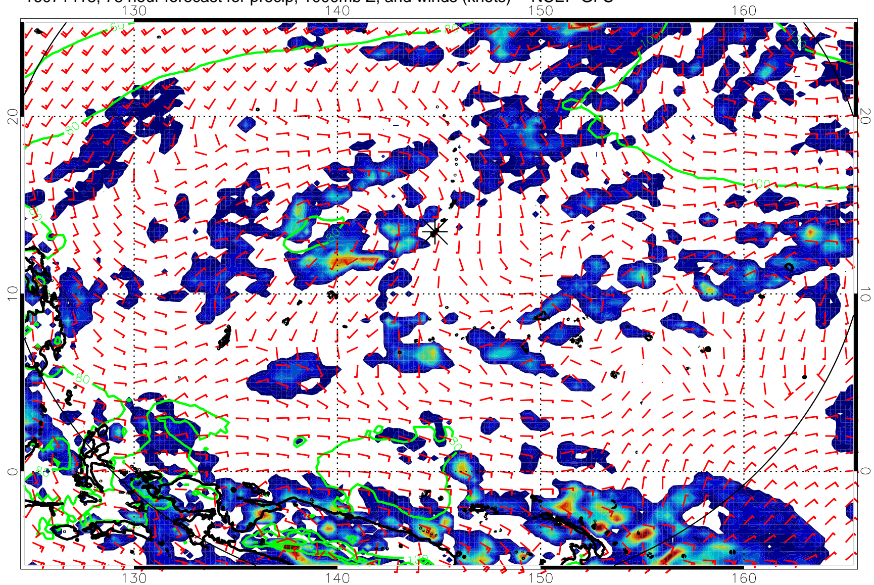
16071418, 78 hour forecast for precip, 1000mb Z, and winds (knots) -- NCEP GFS
