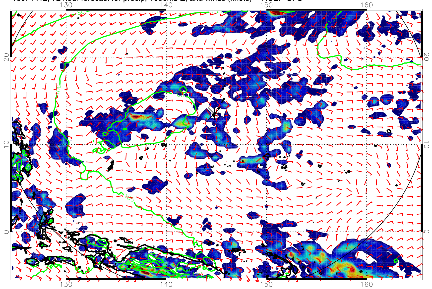
16071412, 72 hour forecast for precip, 1000mb Z, and winds (knots) -- NCEP GFS
