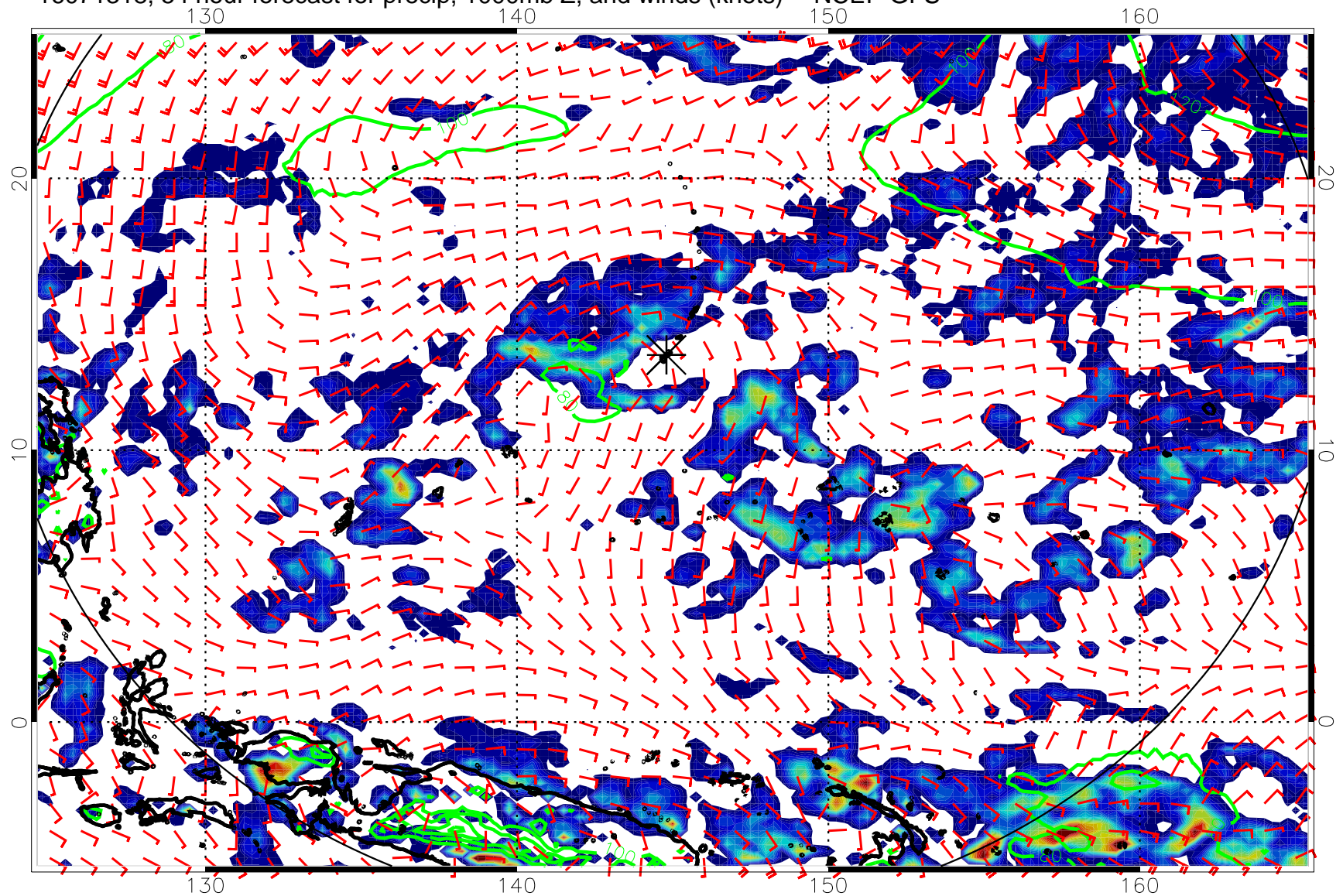
16071318, 54 hour forecast for precip, 1000mb Z, and winds (knots) -- NCEP GFS
