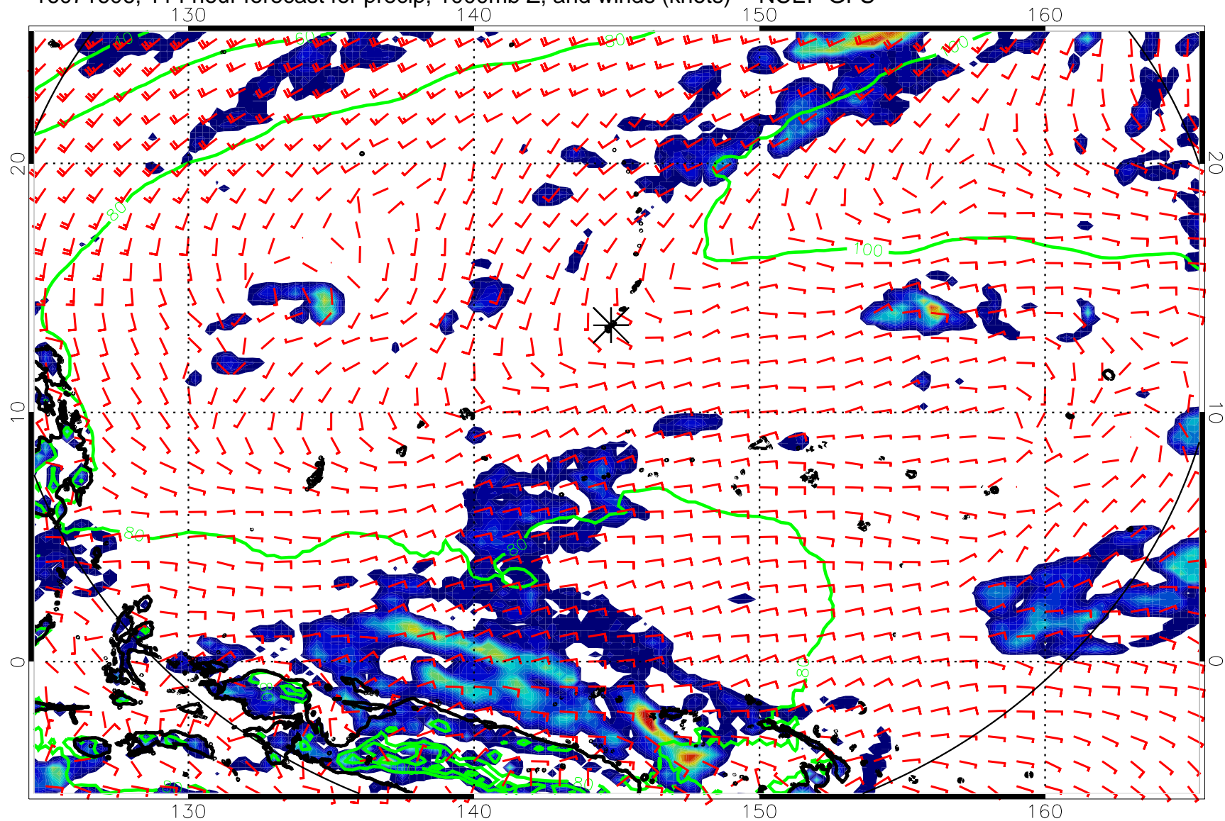
16071606, 114 hour forecast for precip, 1000mb Z, and winds (knots) -- NCEP GFS
