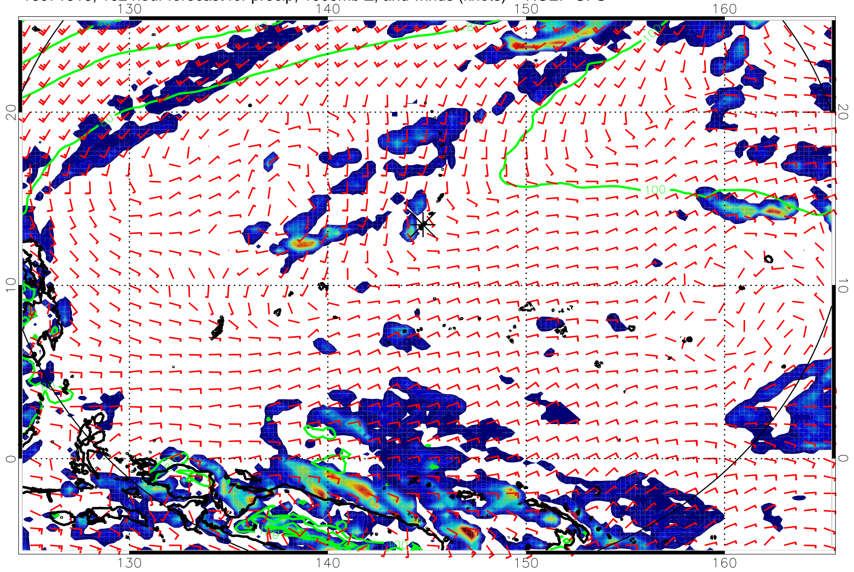
16071518, 102 hour forecast for precip, 1000mb Z, and winds (knots) -- NCEP GFS
