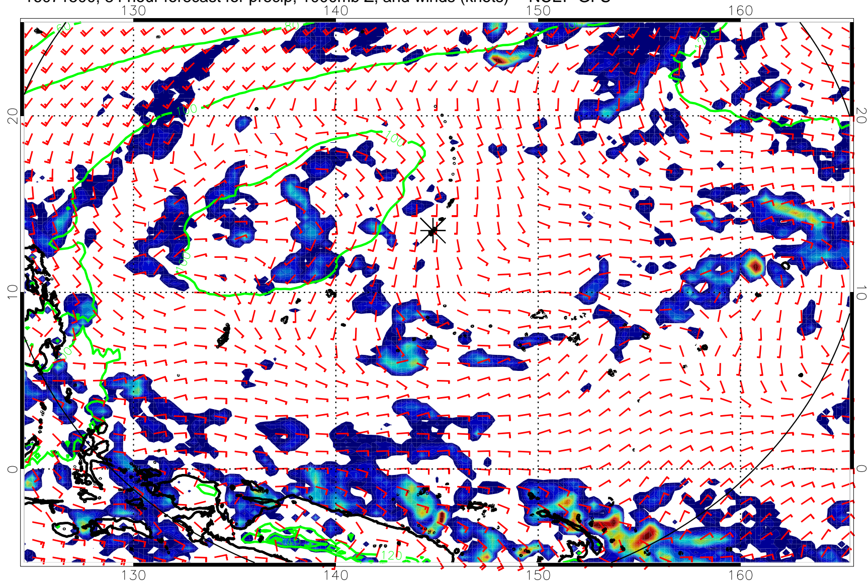
16071500, 84 hour forecast for precip, 1000mb Z, and winds (knots) -- NCEP GFS
