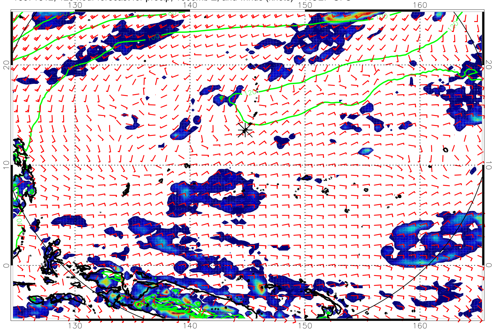
16071612, 120 hour forecast for precip, 1000mb Z, and winds (knots) -- NCEP GFS
