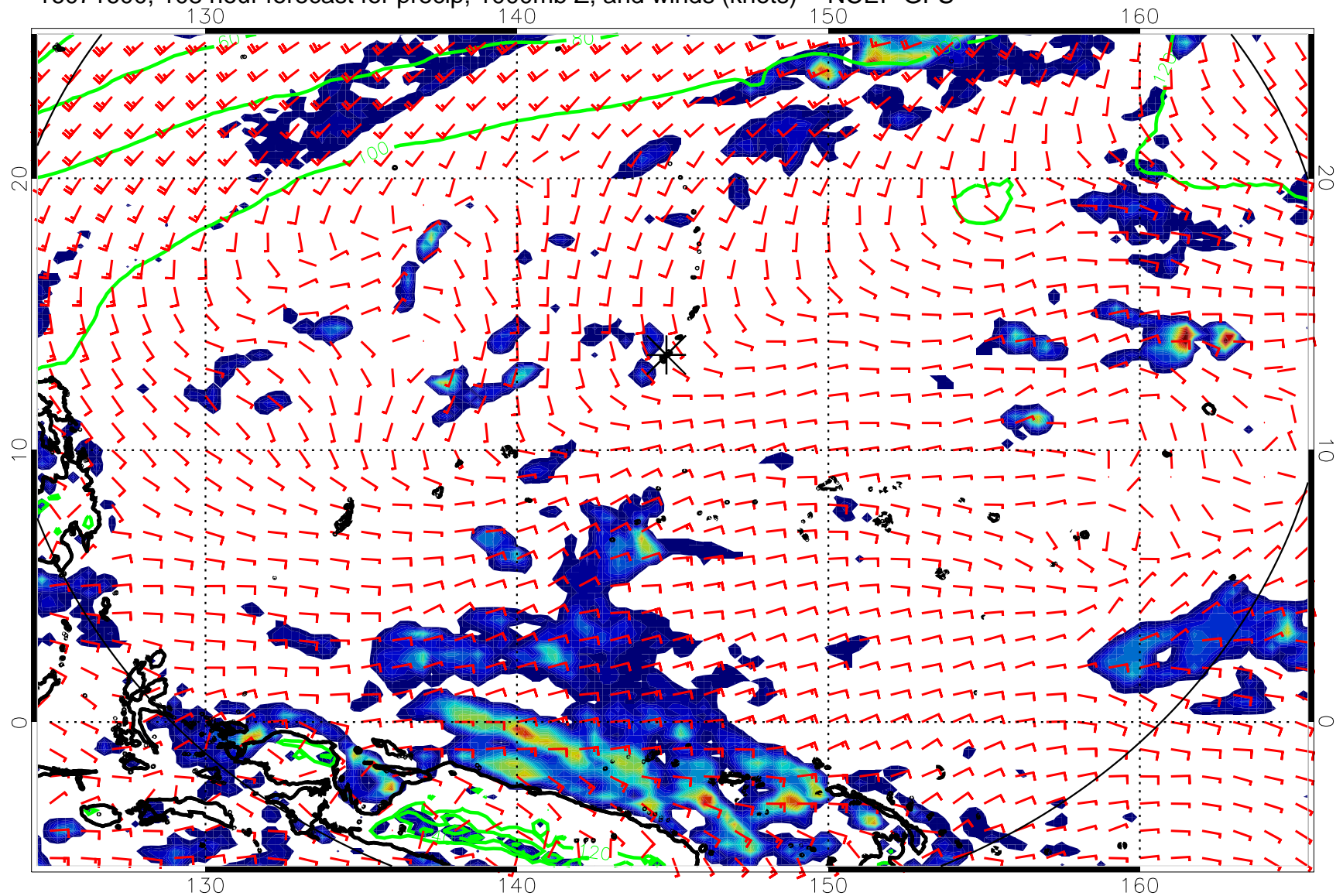
16071600, 108 hour forecast for precip, 1000mb Z, and winds (knots) -- NCEP GFS
