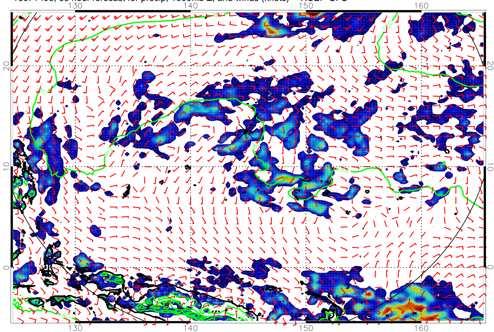
16071406, 66 hour forecast for precip, 1000mb Z, and winds (knots) -- NCEP GFS
