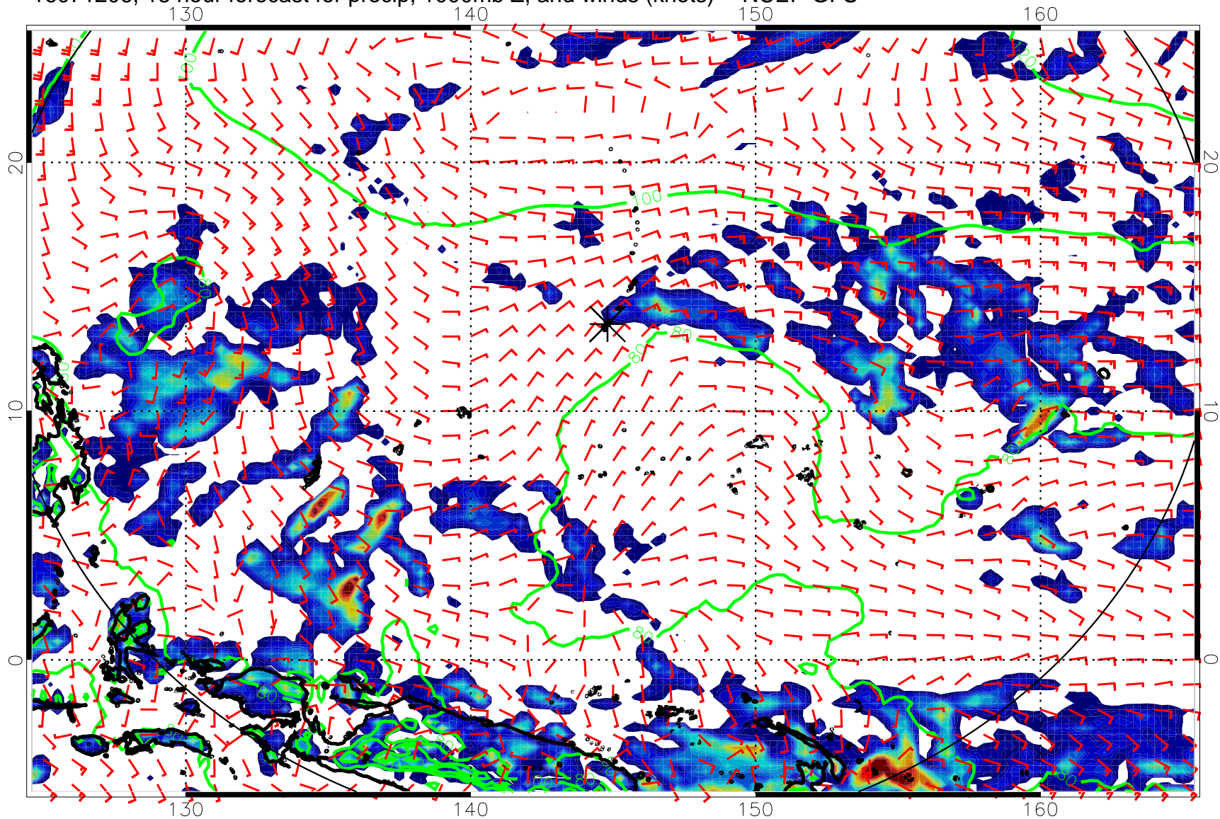
16071206, 18 hour forecast for precip, 1000mb Z, and winds (knots) -- NCEP GFS
