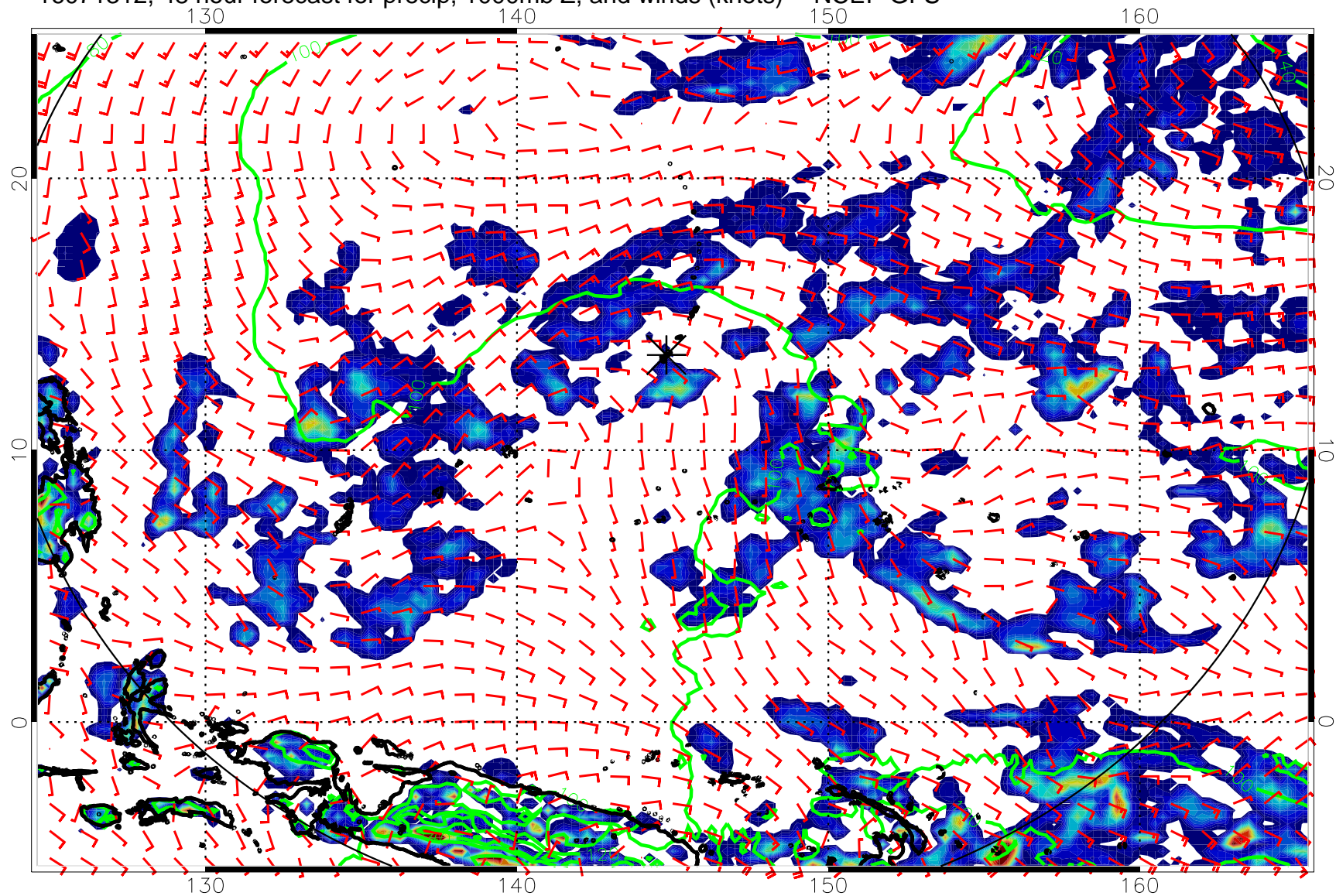
16071312, 48 hour forecast for precip, 1000mb Z, and winds (knots) -- NCEP GFS
