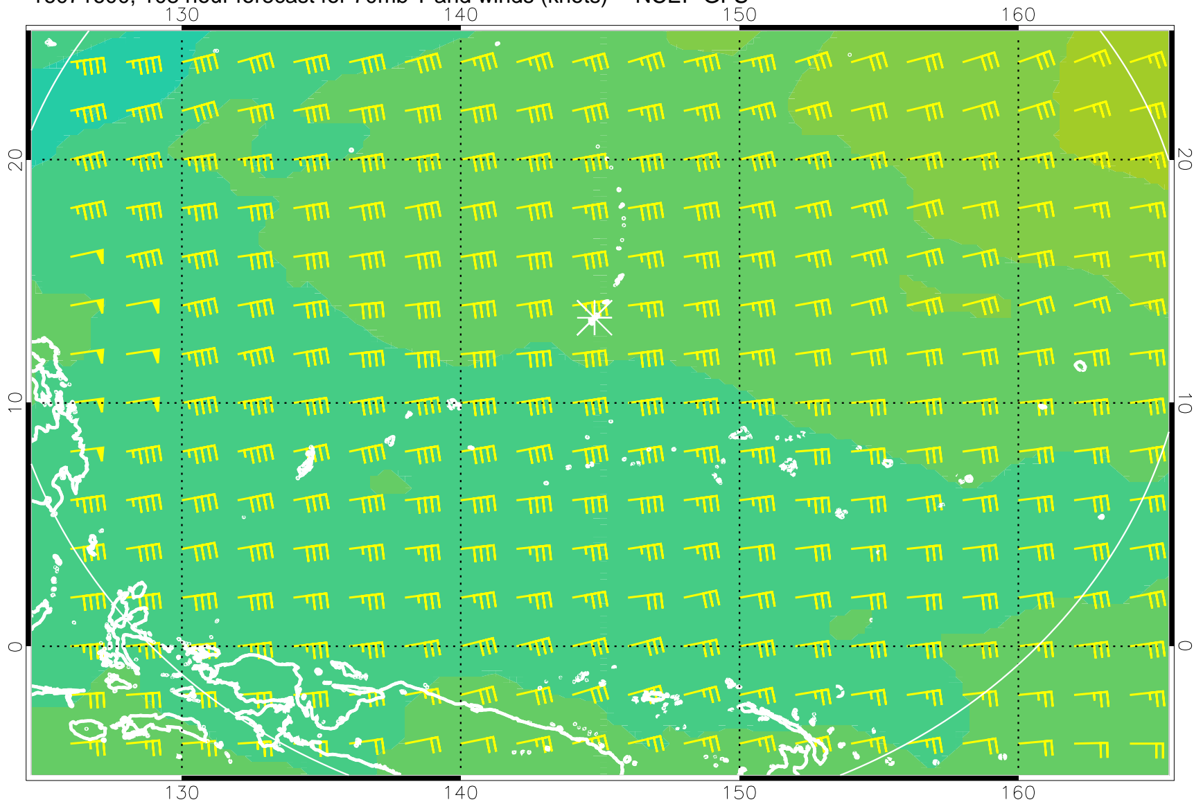
16071600, 108 hour forecast for 70mb T and winds (knots) -- NCEP GFS
