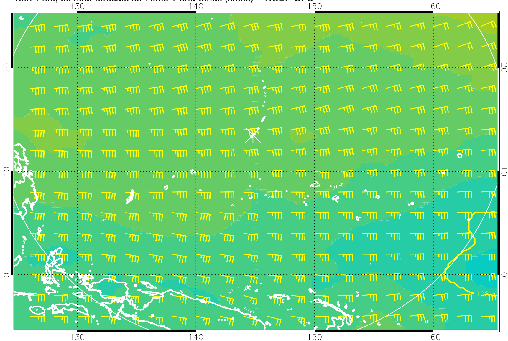
16071406, 66 hour forecast for 70mb T and winds (knots) -- NCEP GFS
