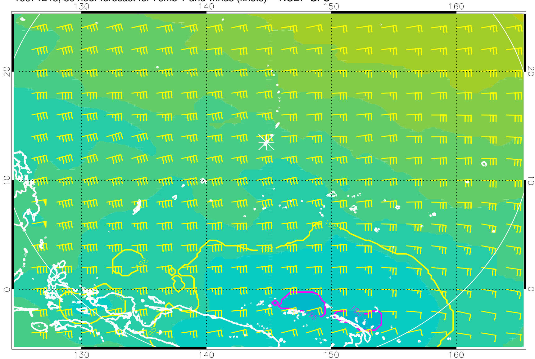
16071218, 30 hour forecast for 70mb T and winds (knots) -- NCEP GFS
