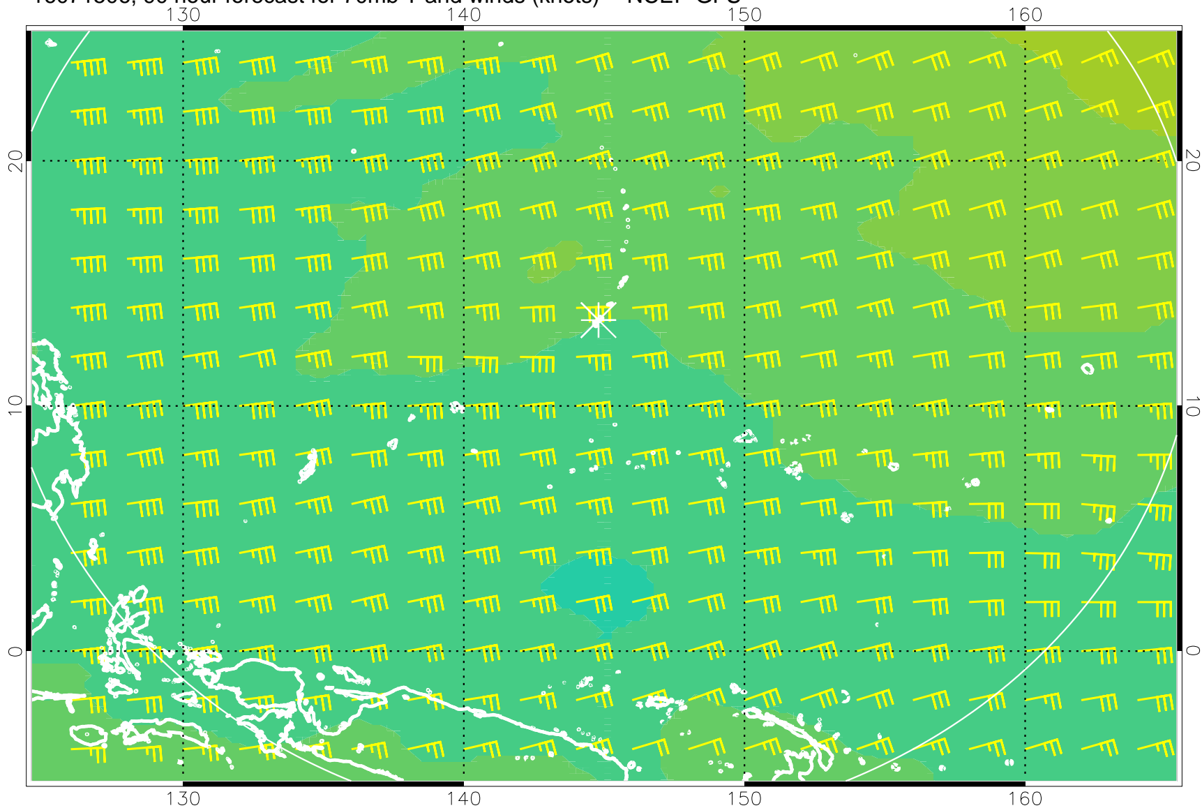
16071506, 90 hour forecast for 70mb T and winds (knots) -- NCEP GFS
