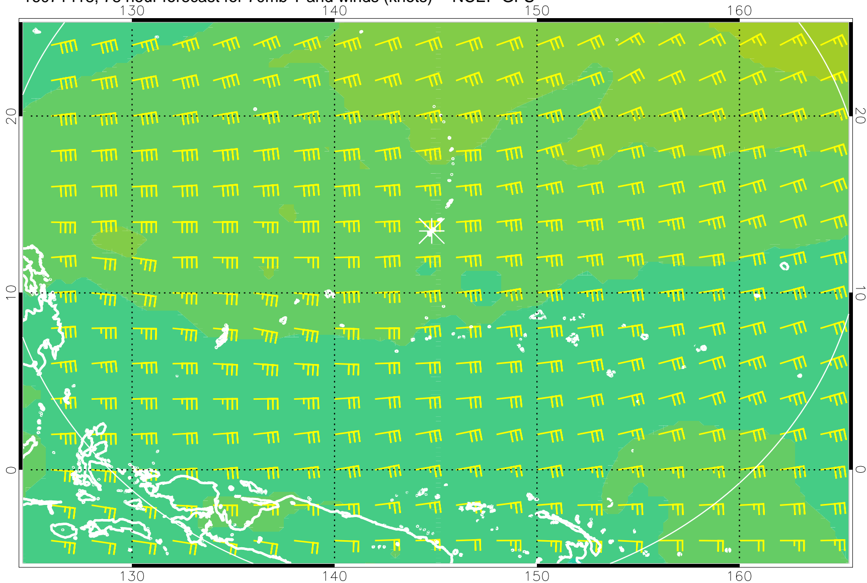
16071418, 78 hour forecast for 70mb T and winds (knots) -- NCEP GFS
