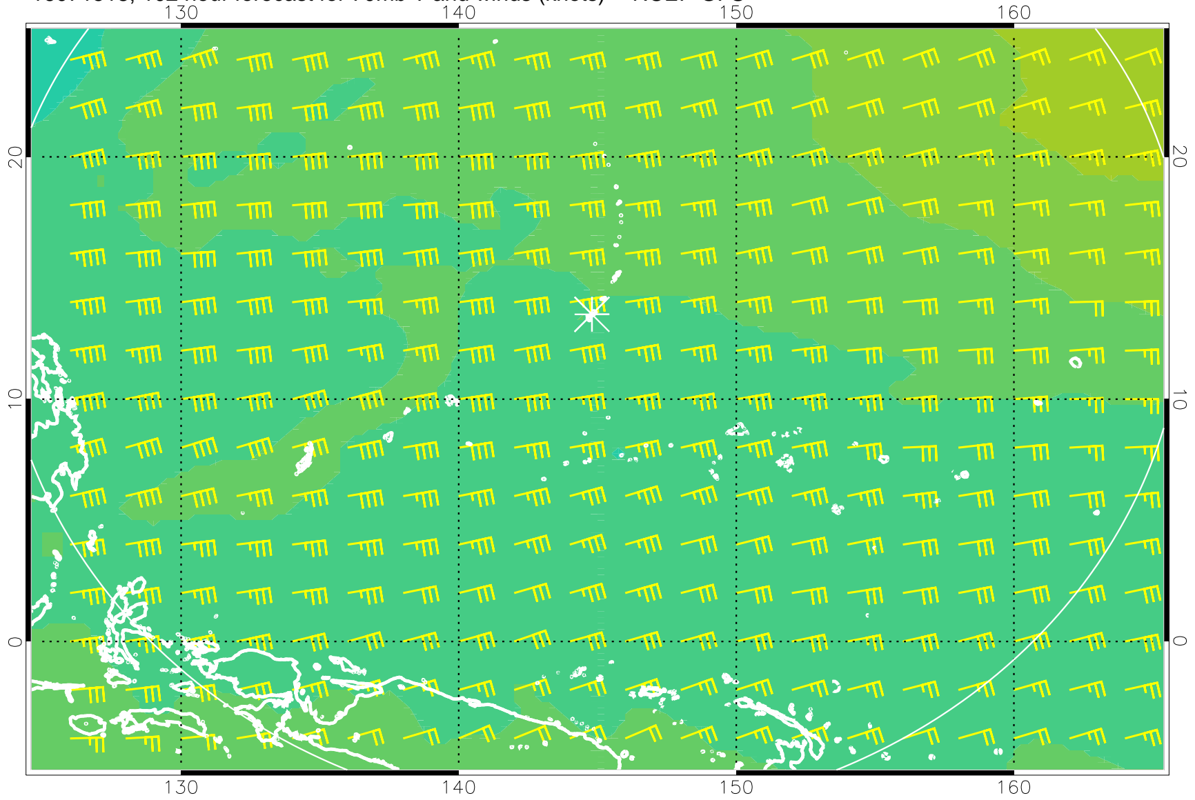
16071518, 102 hour forecast for 70mb T and winds (knots) -- NCEP GFS
