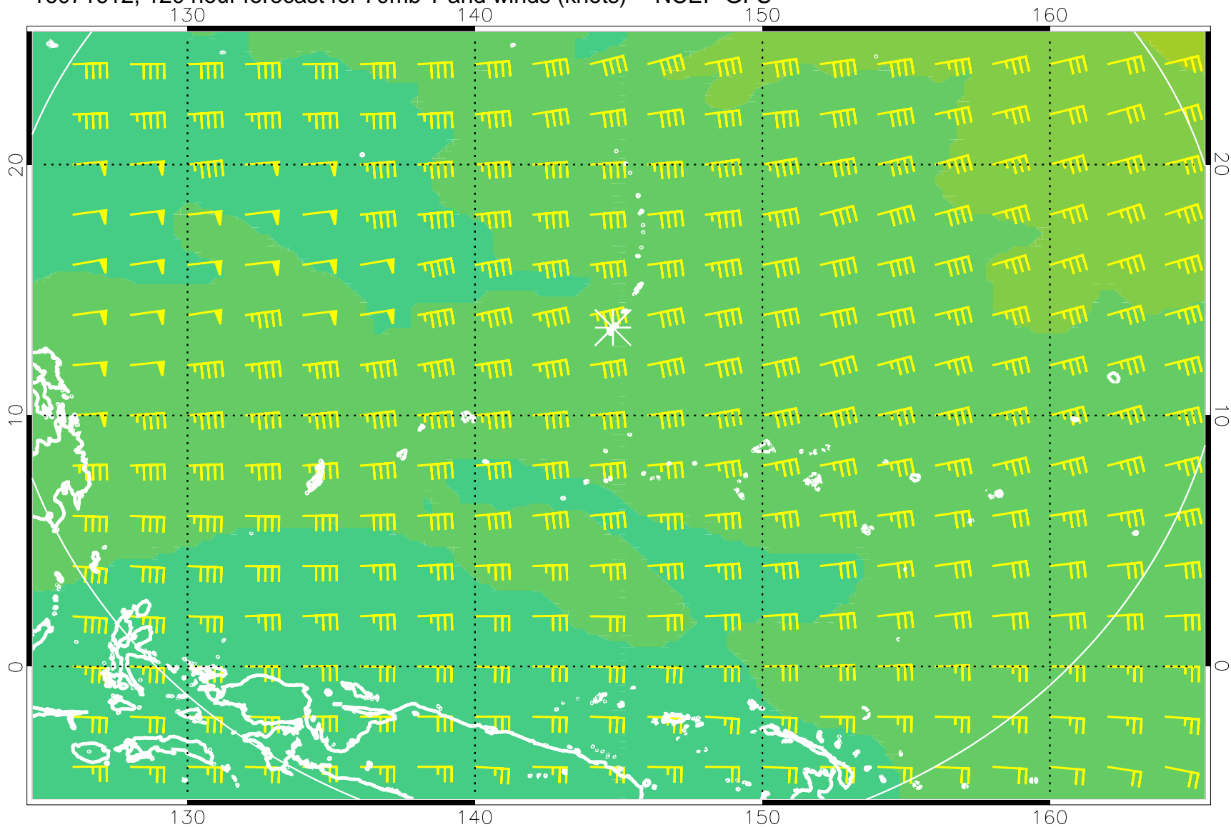
16071612, 120 hour forecast for 70mb T and winds (knots) -- NCEP GFS
