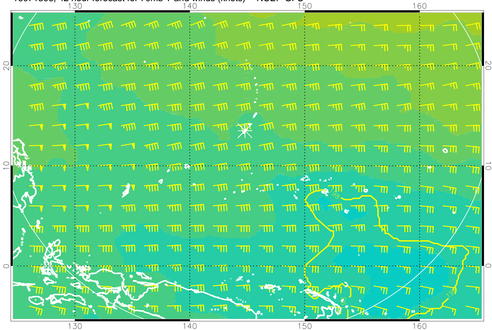
16071306, 42 hour forecast for 70mb T and winds (knots) -- NCEP GFS
