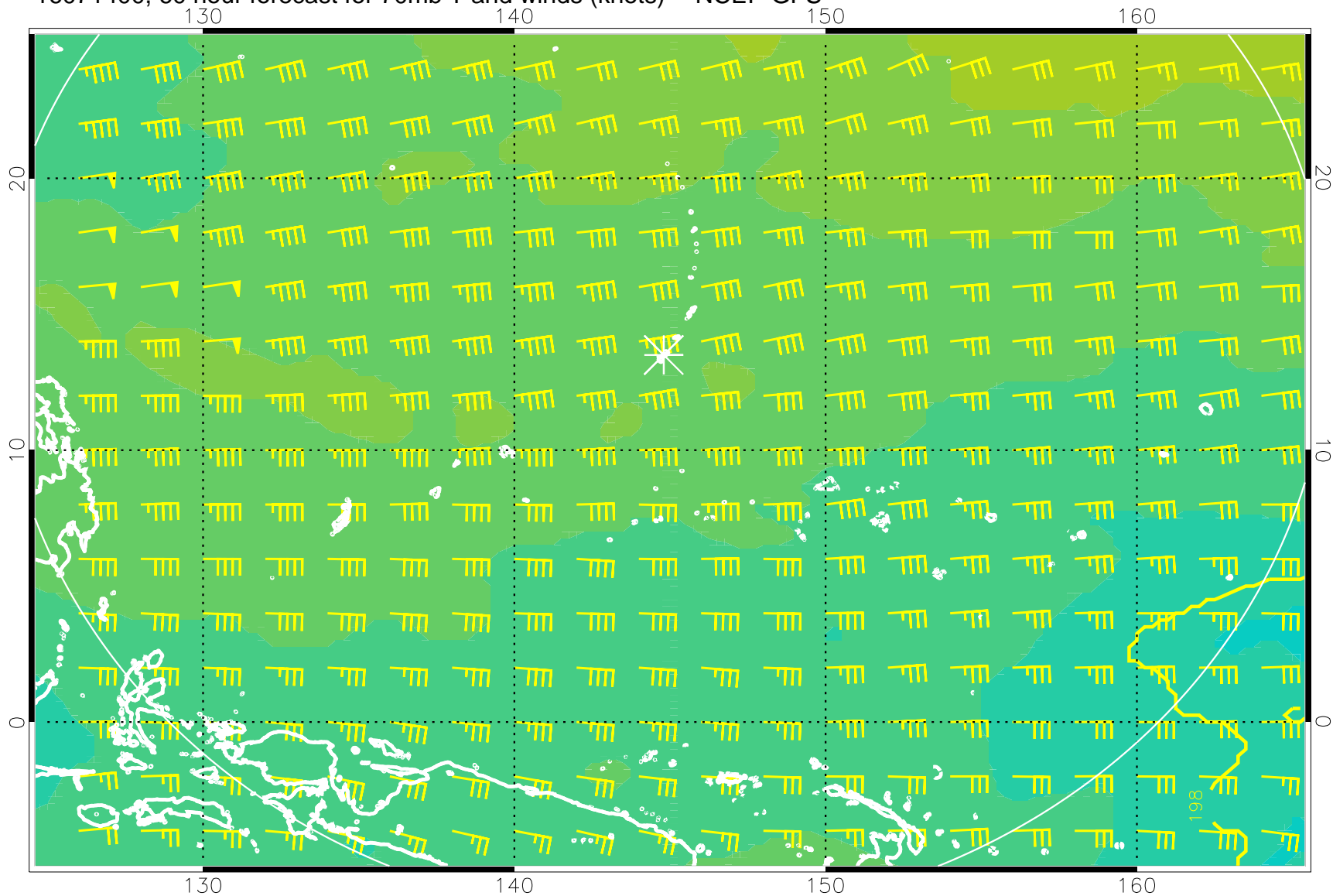
16071400, 60 hour forecast for 70mb T and winds (knots) -- NCEP GFS
