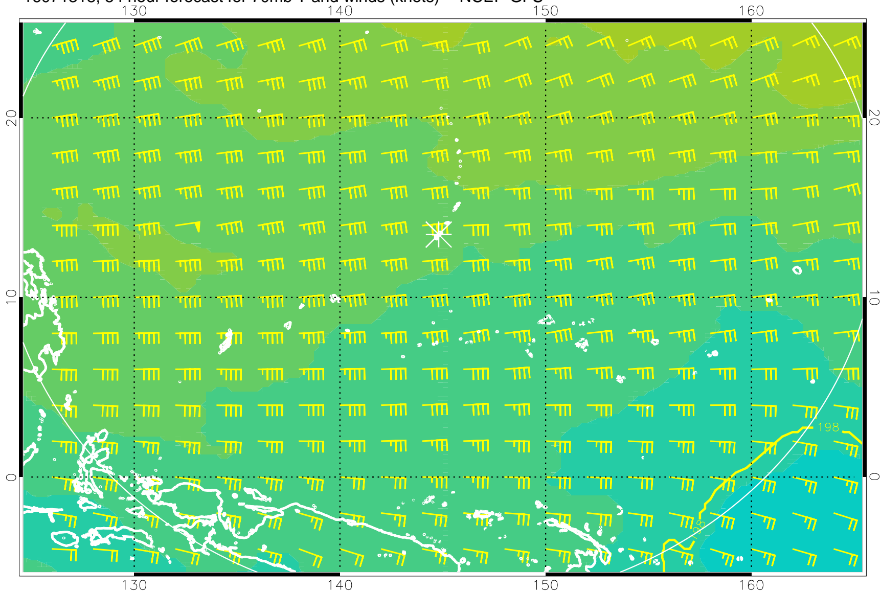
16071318, 54 hour forecast for 70mb T and winds (knots) -- NCEP GFS
