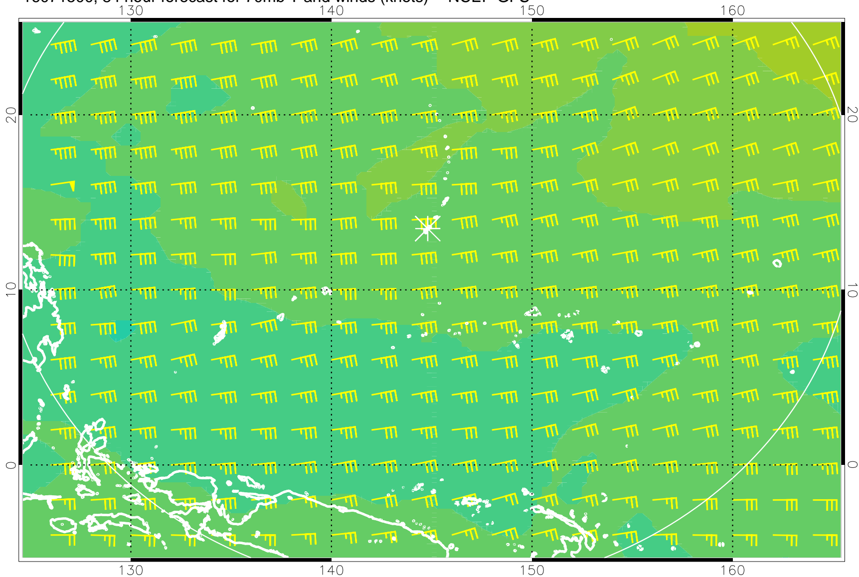
16071500, 84 hour forecast for 70mb T and winds (knots) -- NCEP GFS
