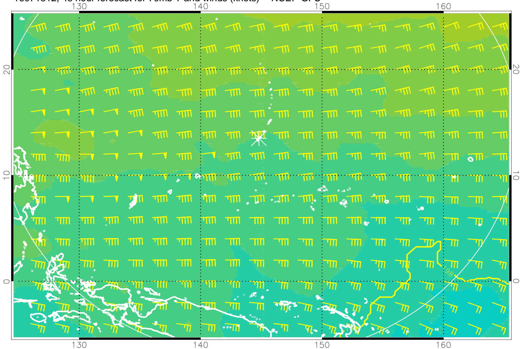
16071312, 48 hour forecast for 70mb T and winds (knots) -- NCEP GFS
