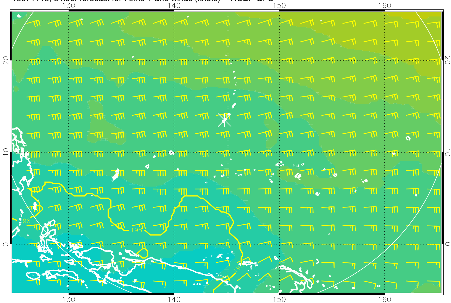
16071118, 6 hour forecast for 70mb T and winds (knots) -- NCEP GFS
