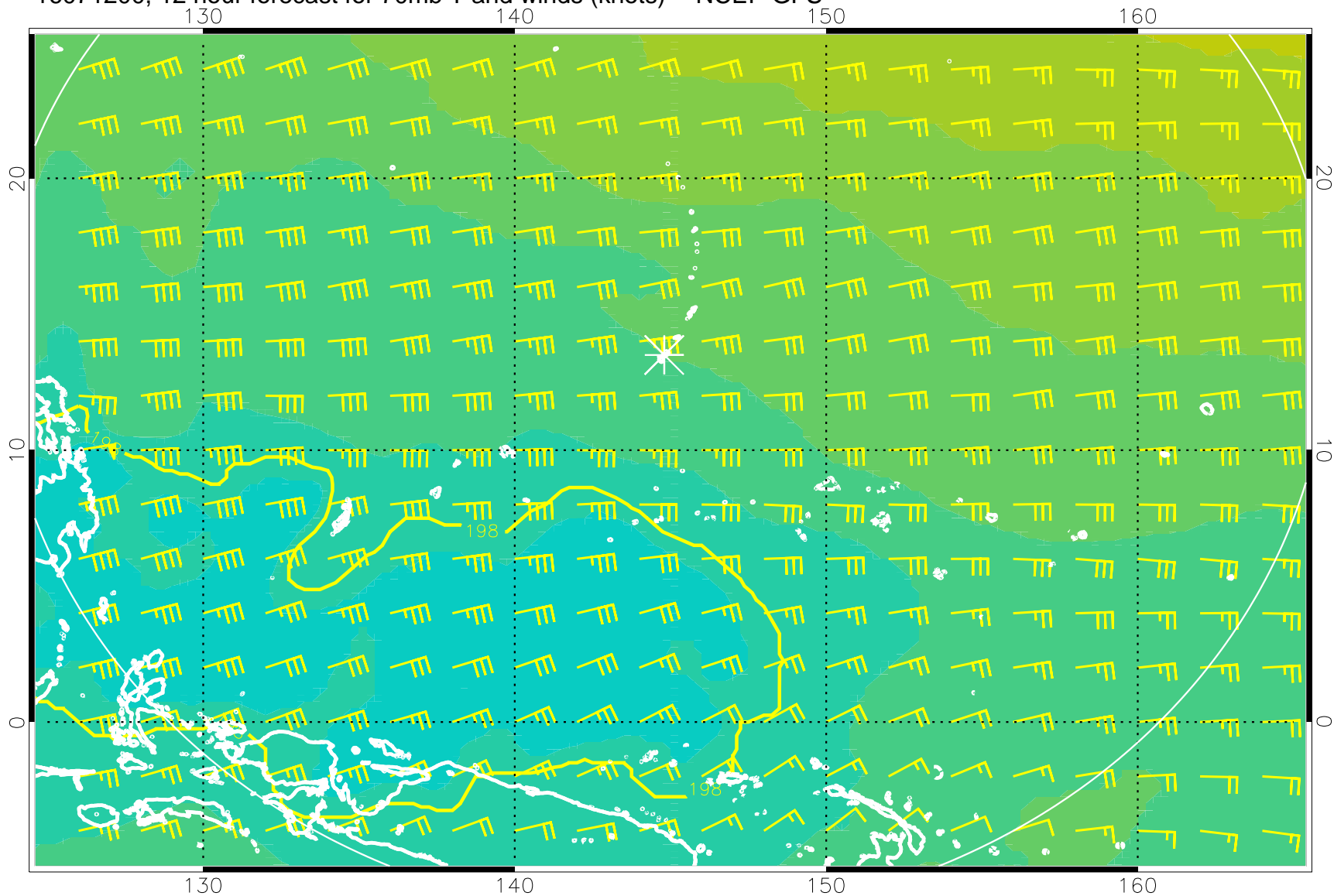
16071200, 12 hour forecast for 70mb T and winds (knots) -- NCEP GFS
