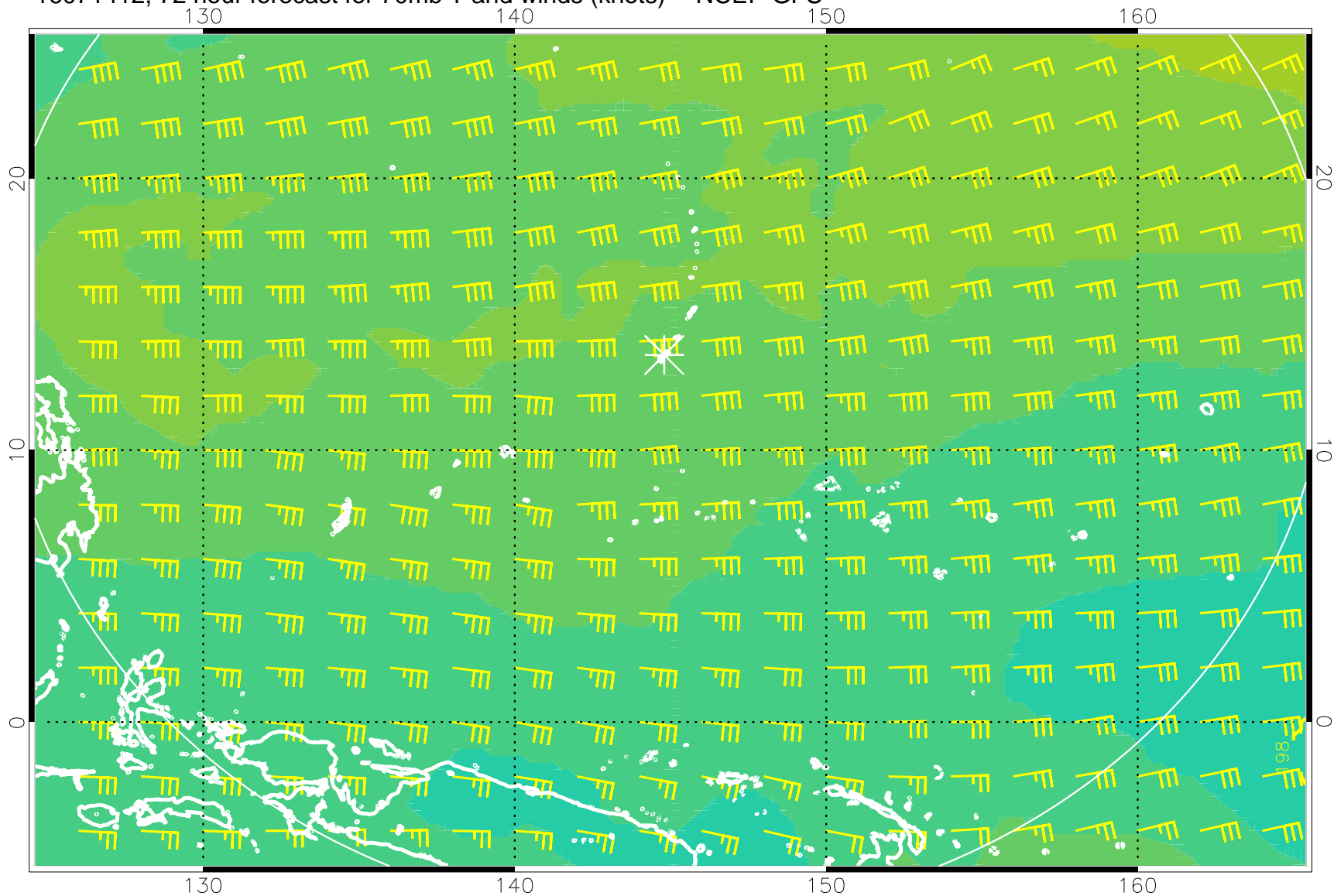
16071412, 72 hour forecast for 70mb T and winds (knots) -- NCEP GFS
