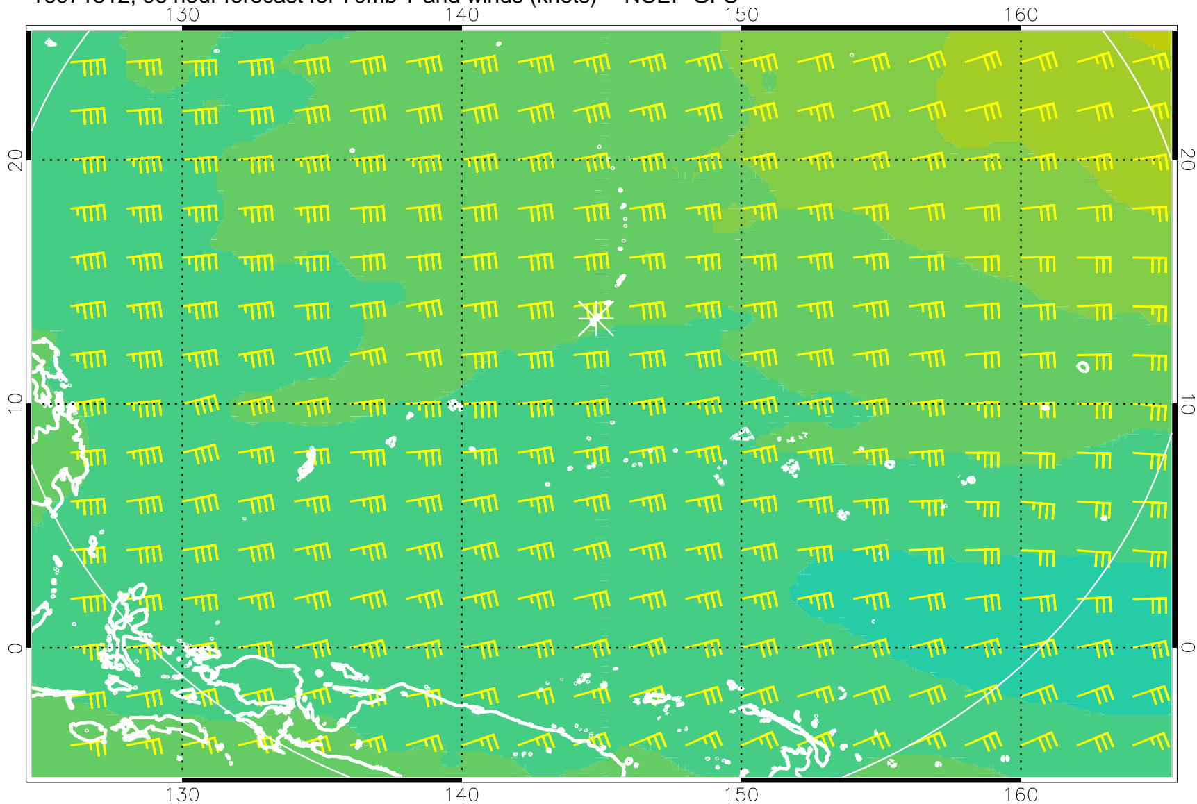
16071512, 96 hour forecast for 70mb T and winds (knots) -- NCEP GFS
