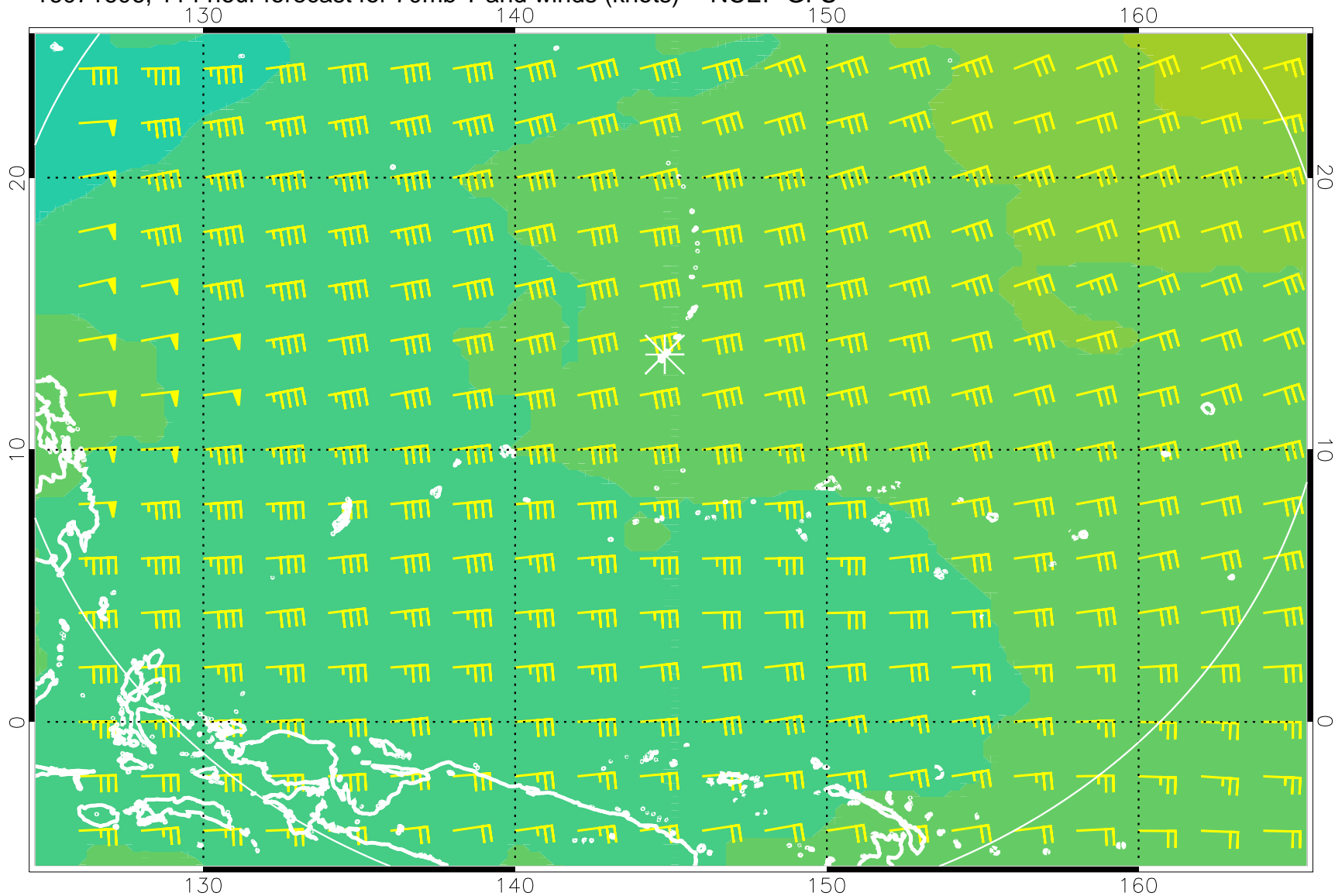
16071606, 114 hour forecast for 70mb T and winds (knots) -- NCEP GFS
