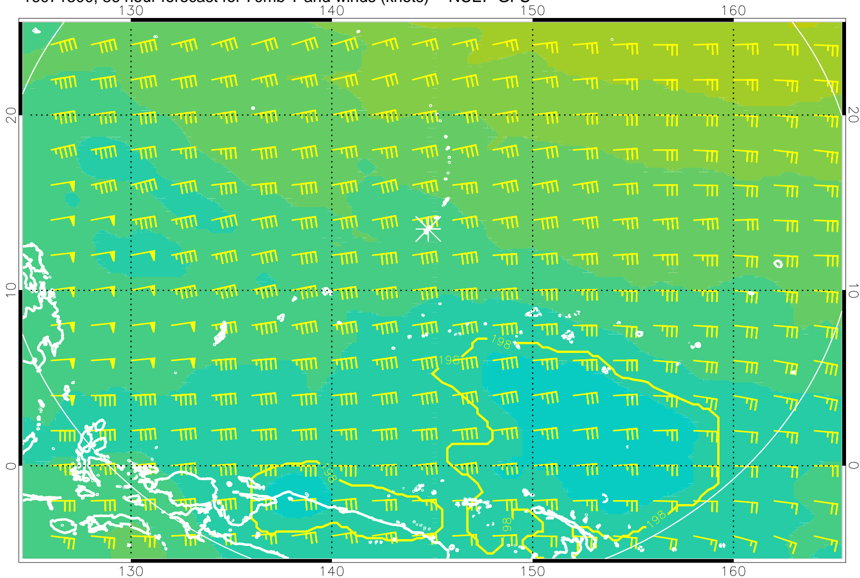
16071300, 36 hour forecast for 70mb T and winds (knots) -- NCEP GFS
