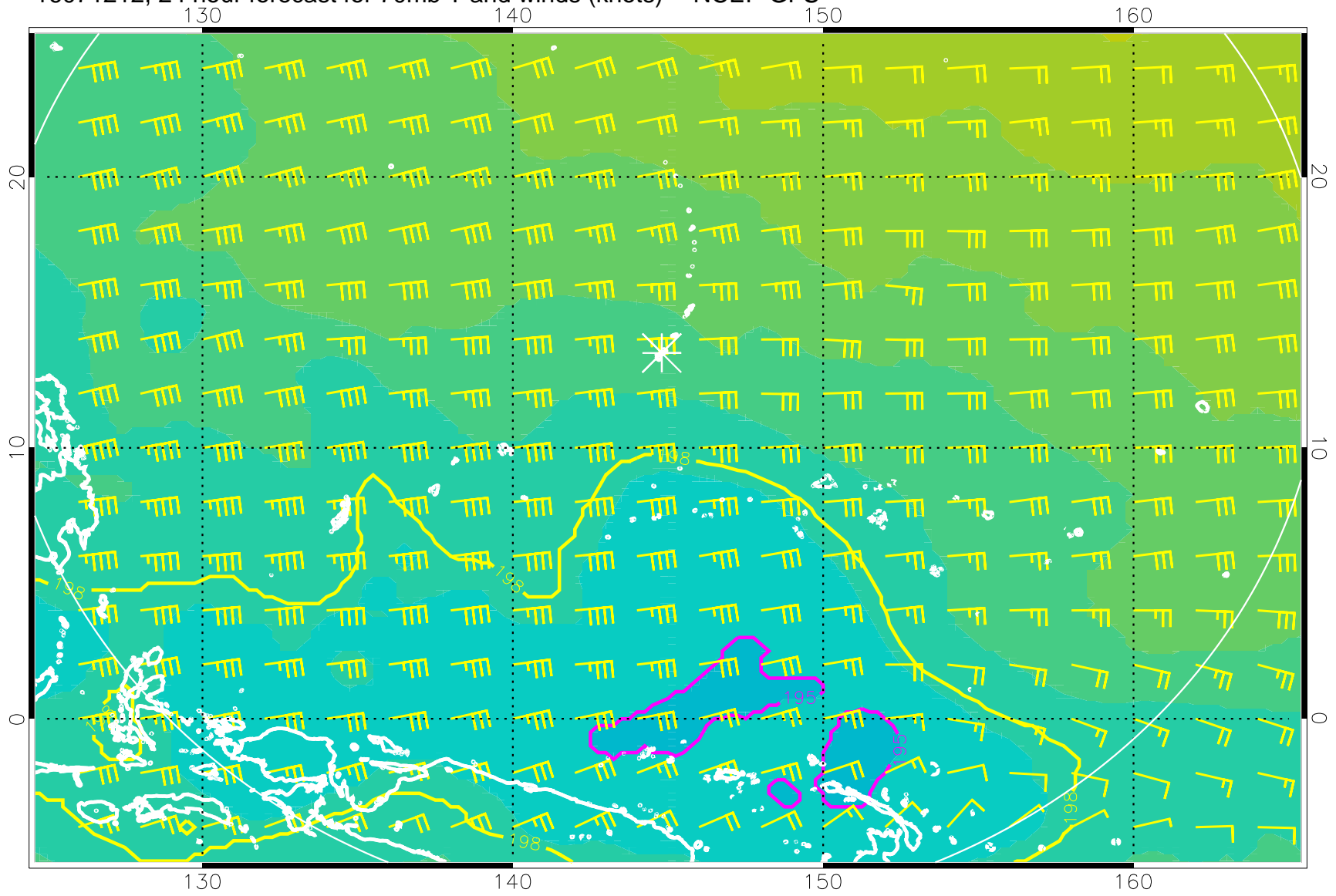
16071212, 24 hour forecast for 70mb T and winds (knots) -- NCEP GFS
