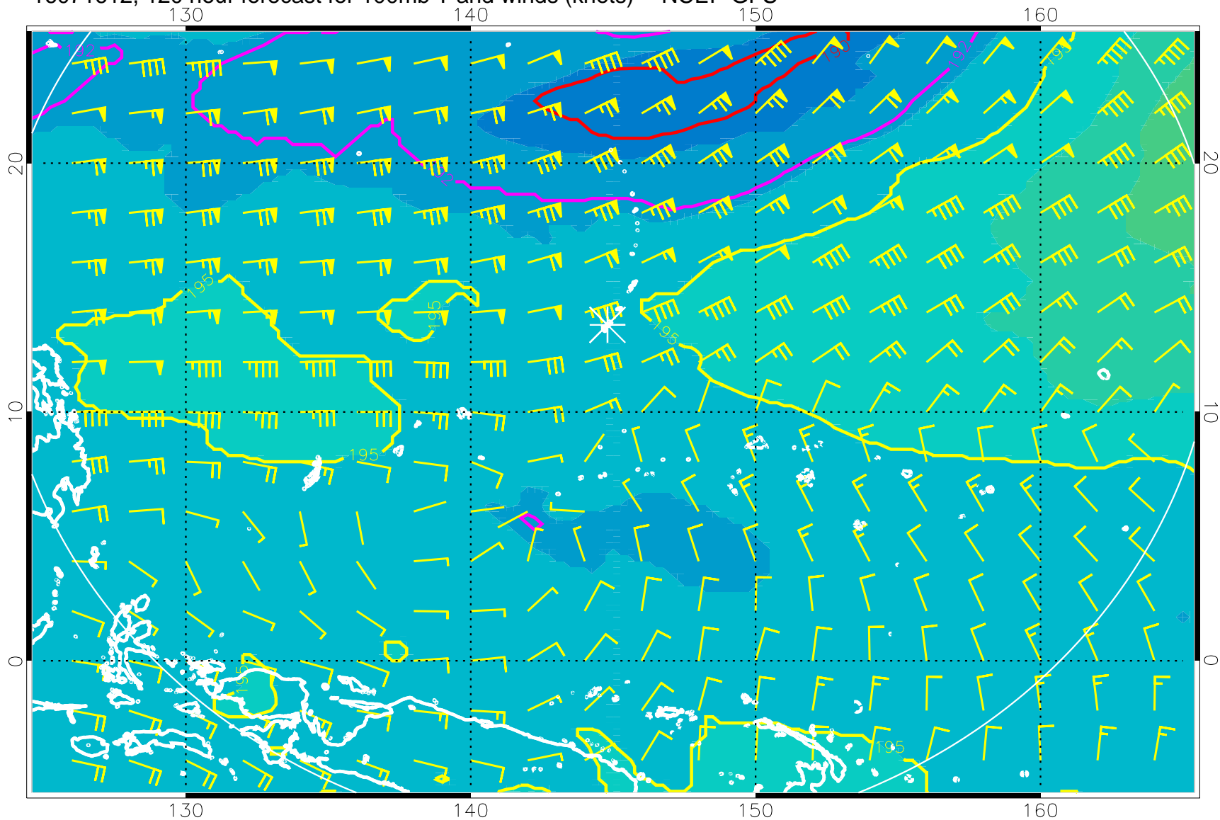
16071612, 120 hour forecast for 100mb T and winds (knots) -- NCEP GFS
