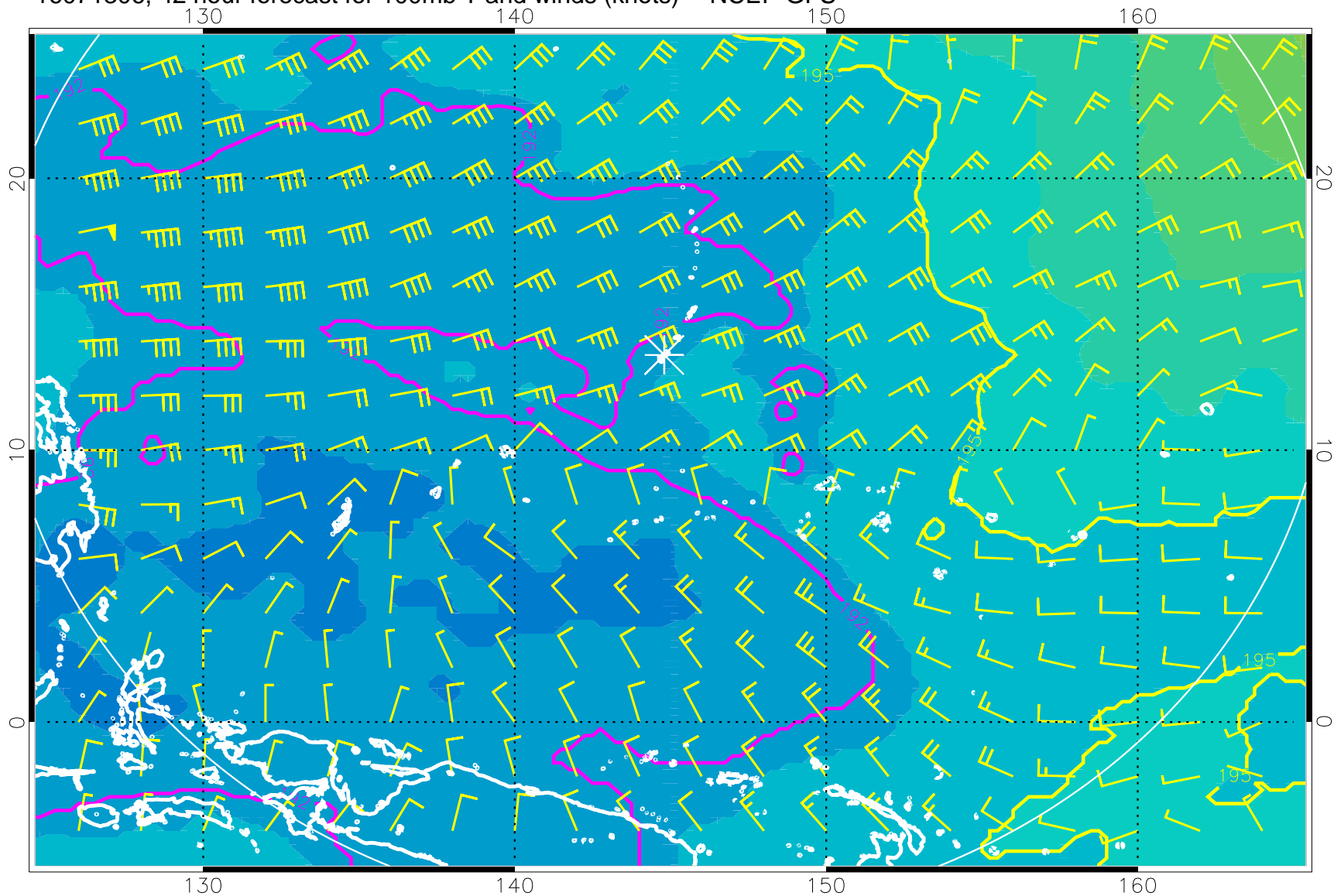
16071306, 42 hour forecast for 100mb T and winds (knots) -- NCEP GFS
