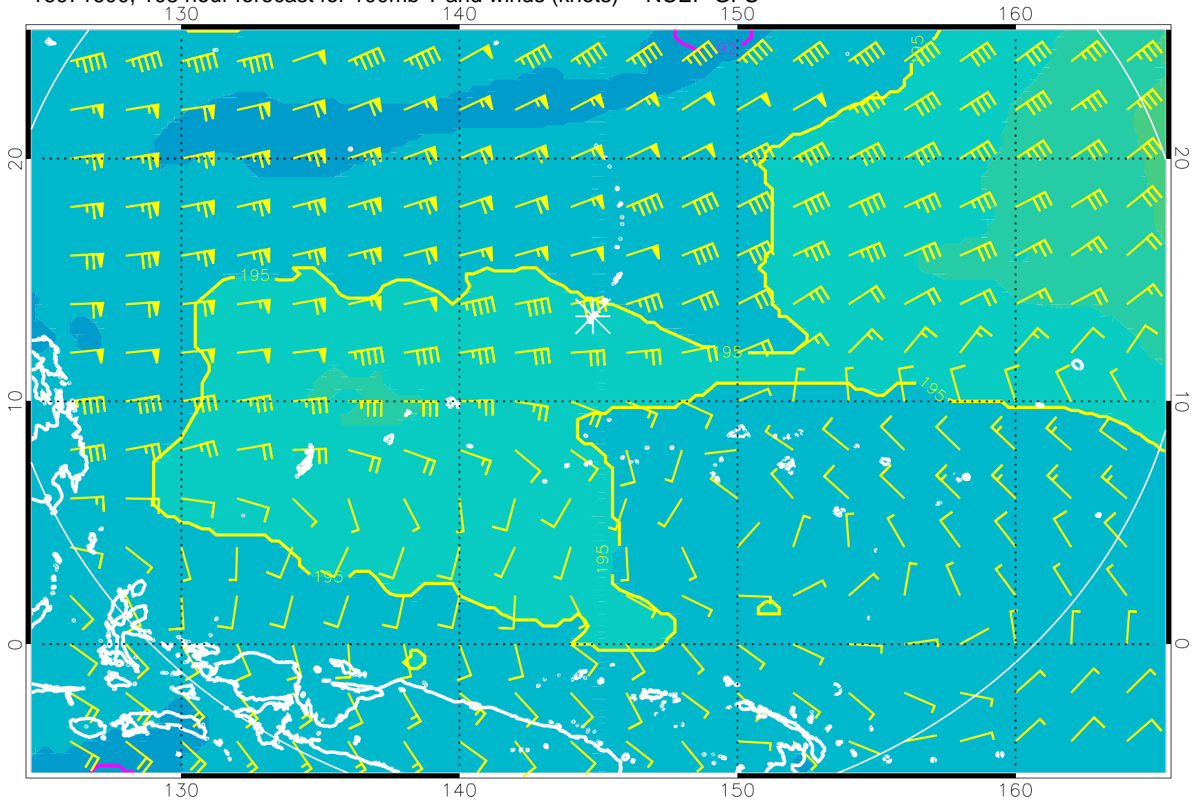
16071600, 108 hour forecast for 100mb T and winds (knots) -- NCEP GFS
