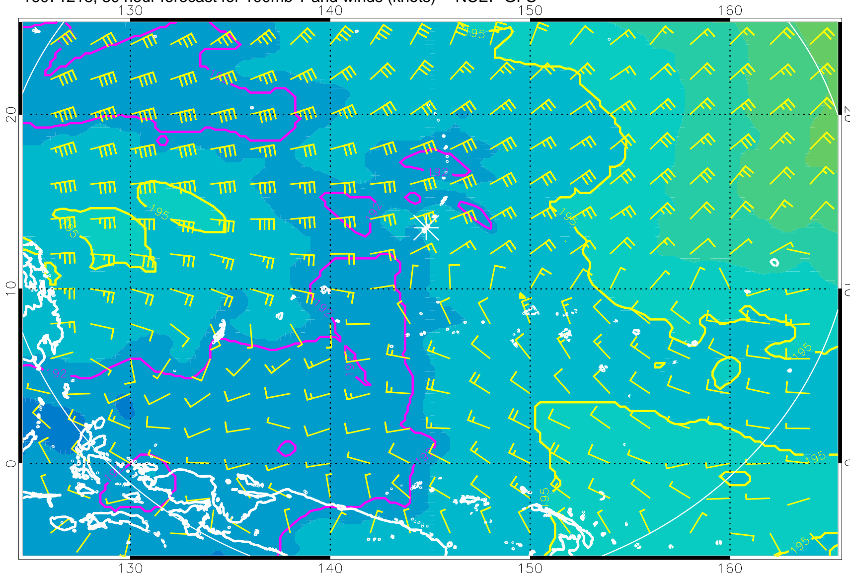
16071218, 30 hour forecast for 100mb T and winds (knots) -- NCEP GFS
