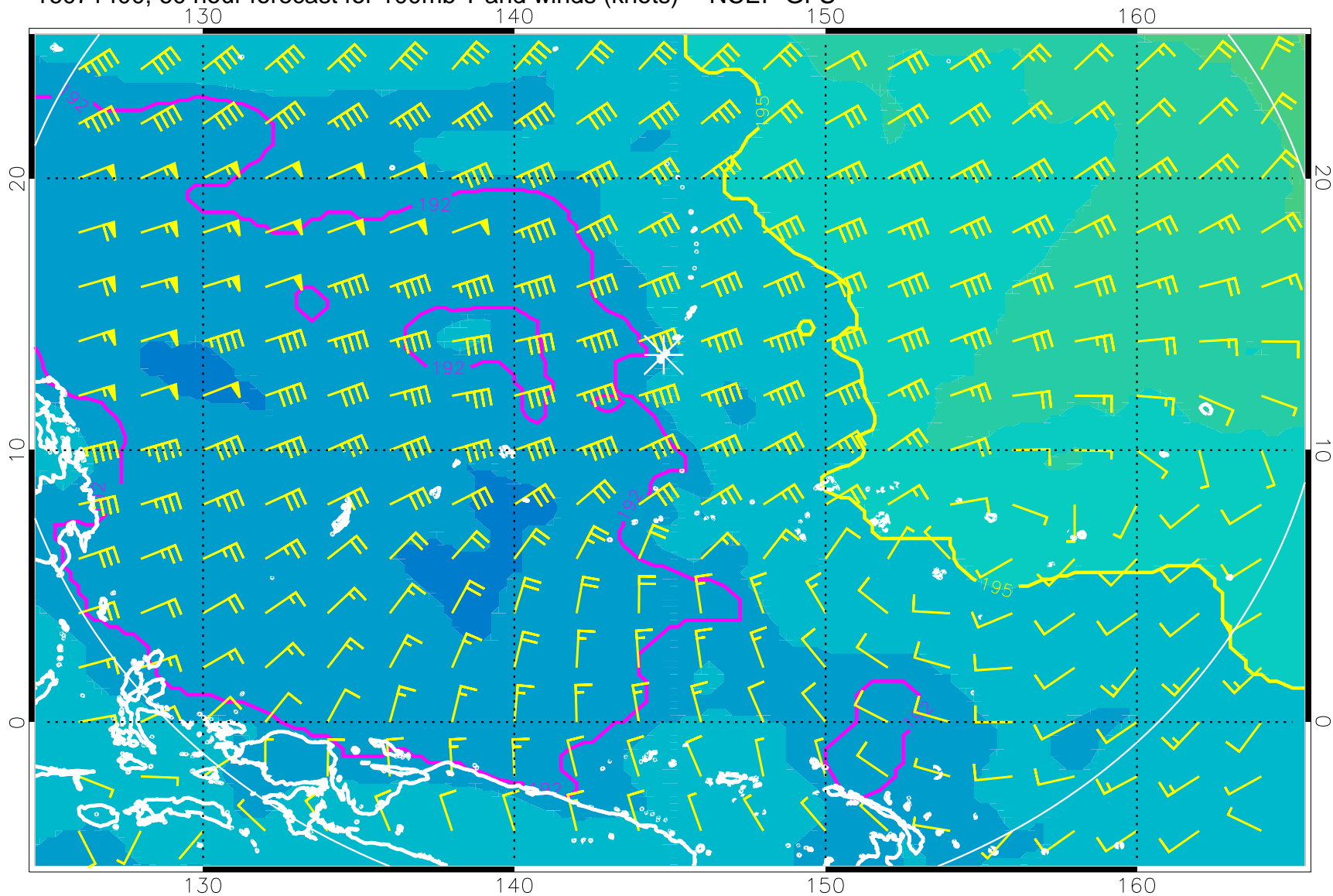
16071400, 60 hour forecast for 100mb T and winds (knots) -- NCEP GFS
