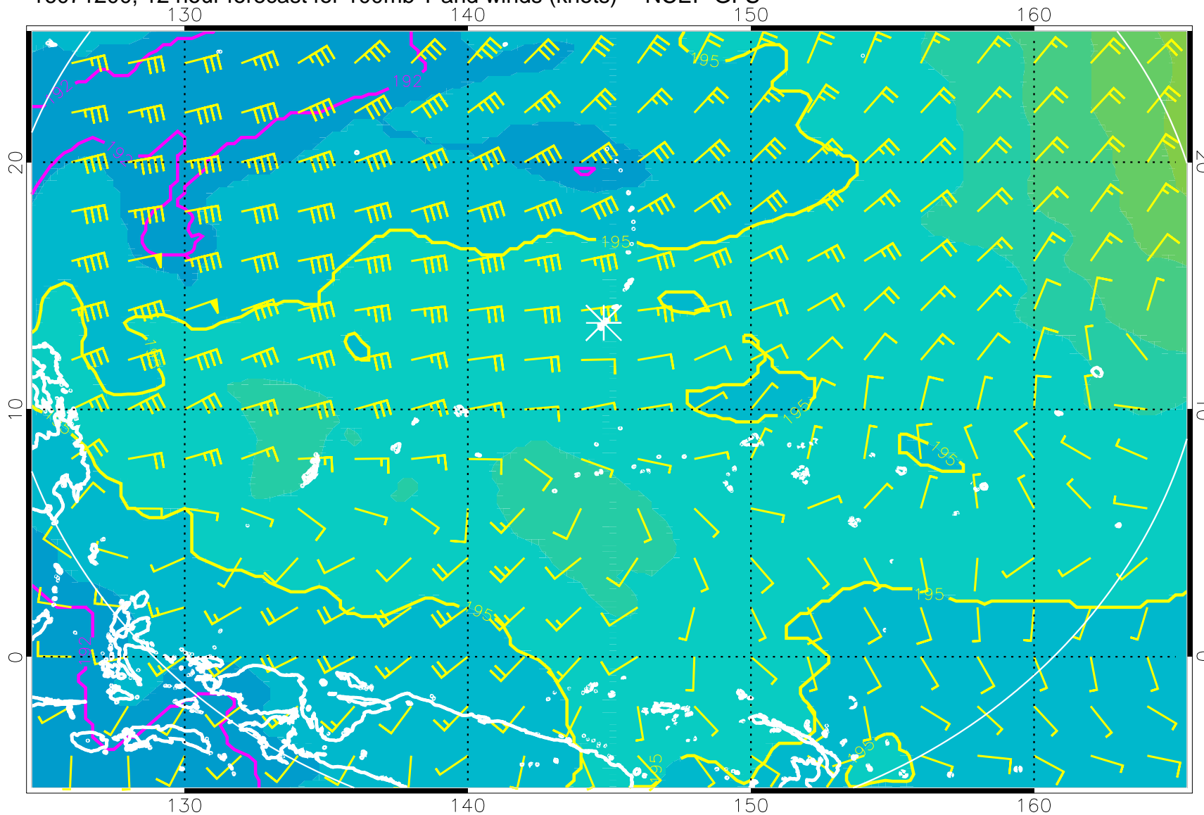
16071200, 12 hour forecast for 100mb T and winds (knots) -- NCEP GFS
