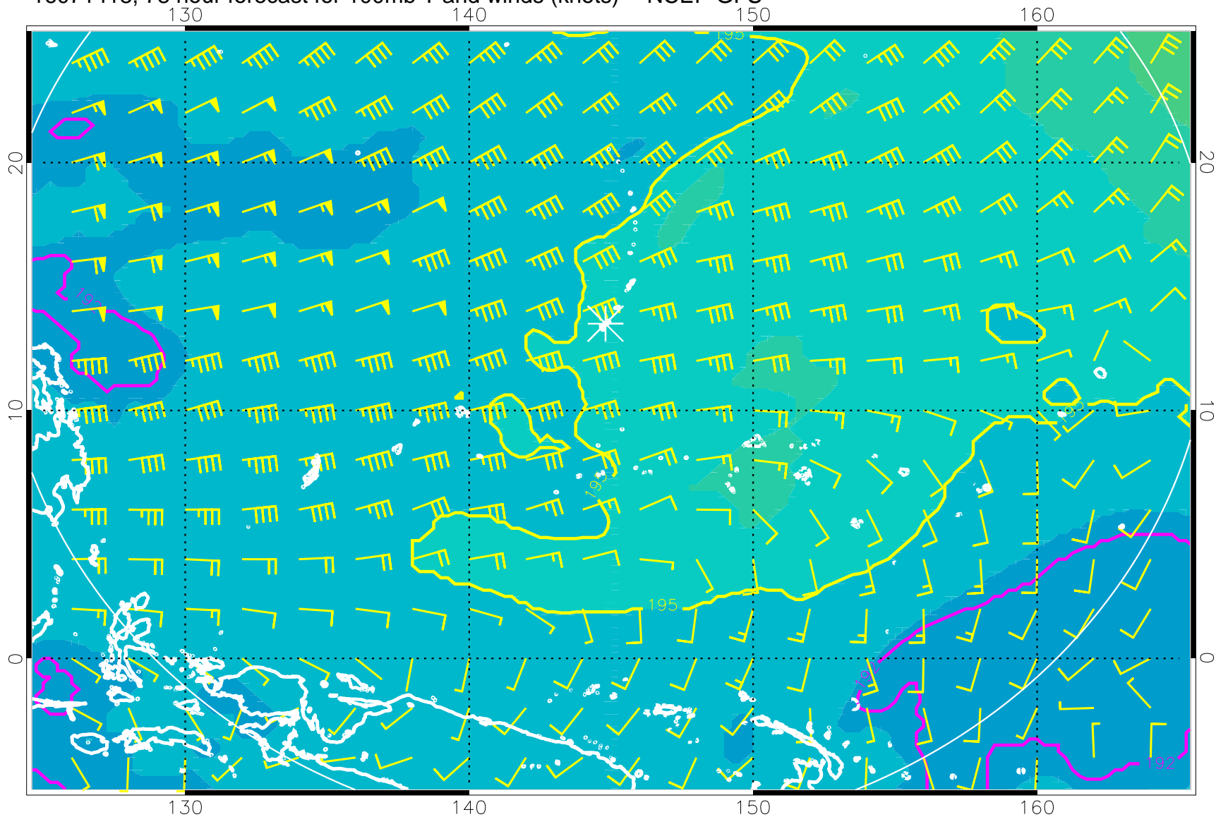
16071418, 78 hour forecast for 100mb T and winds (knots) -- NCEP GFS
