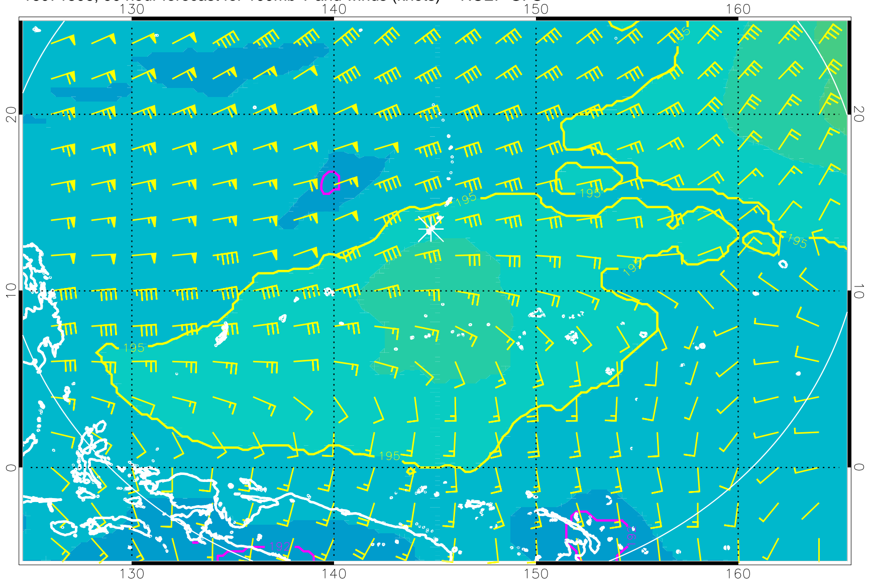
16071506, 90 hour forecast for 100mb T and winds (knots) -- NCEP GFS
