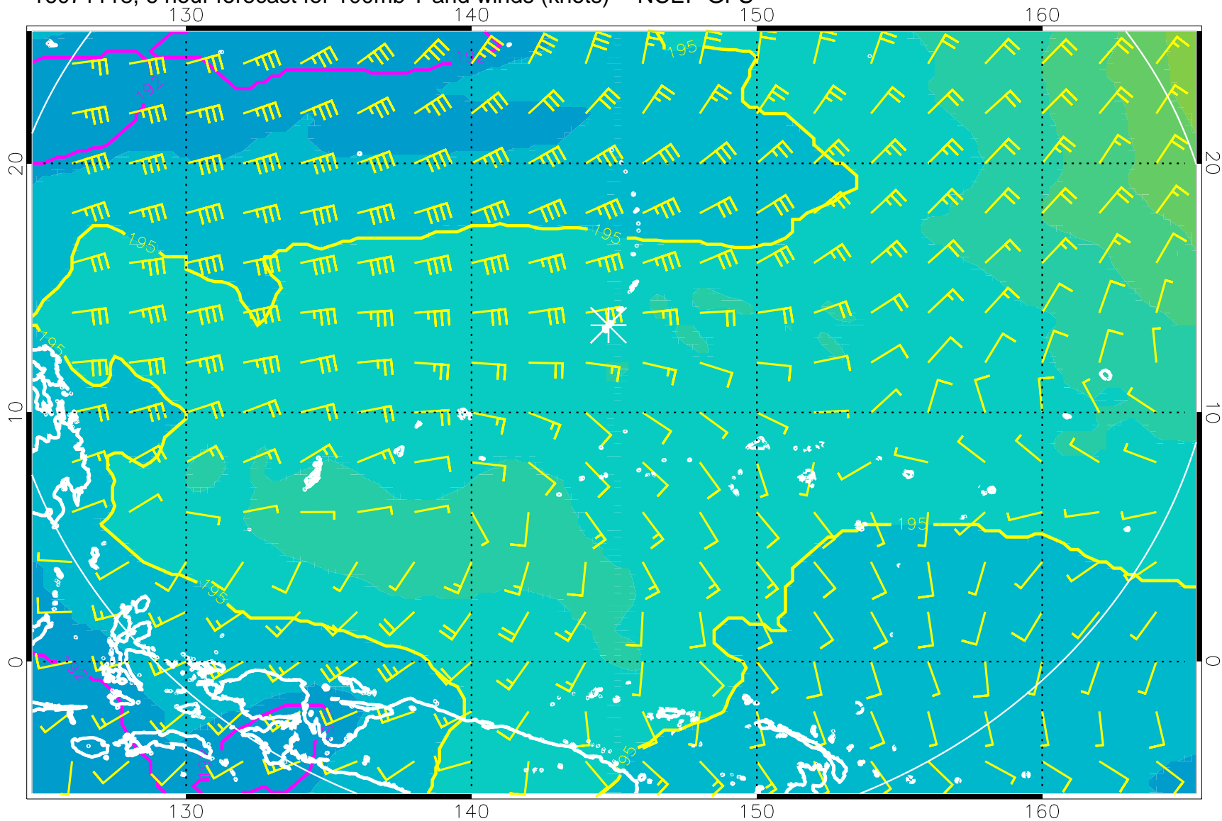
16071118, 6 hour forecast for 100mb T and winds (knots) -- NCEP GFS
