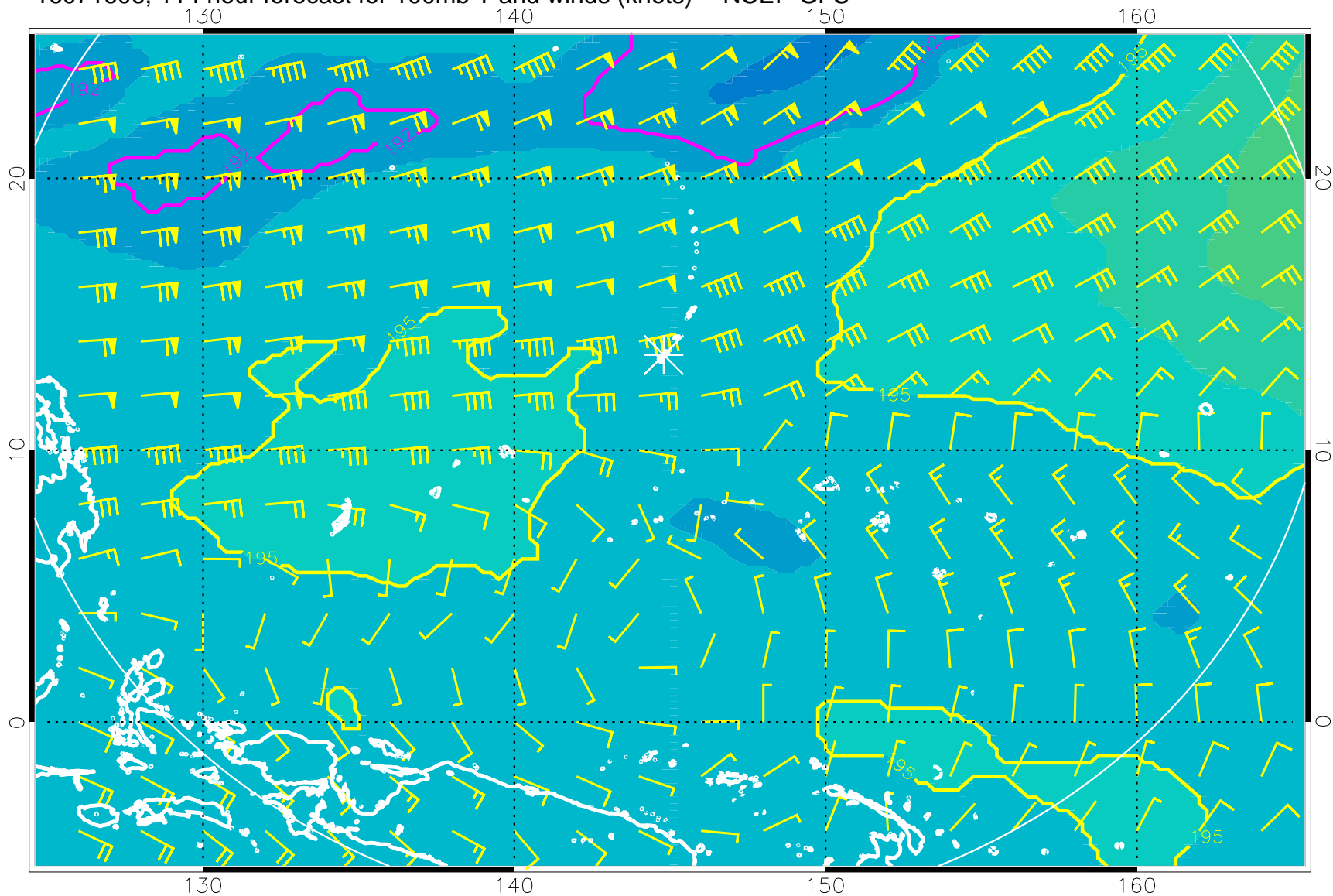
16071606, 114 hour forecast for 100mb T and winds (knots) -- NCEP GFS
