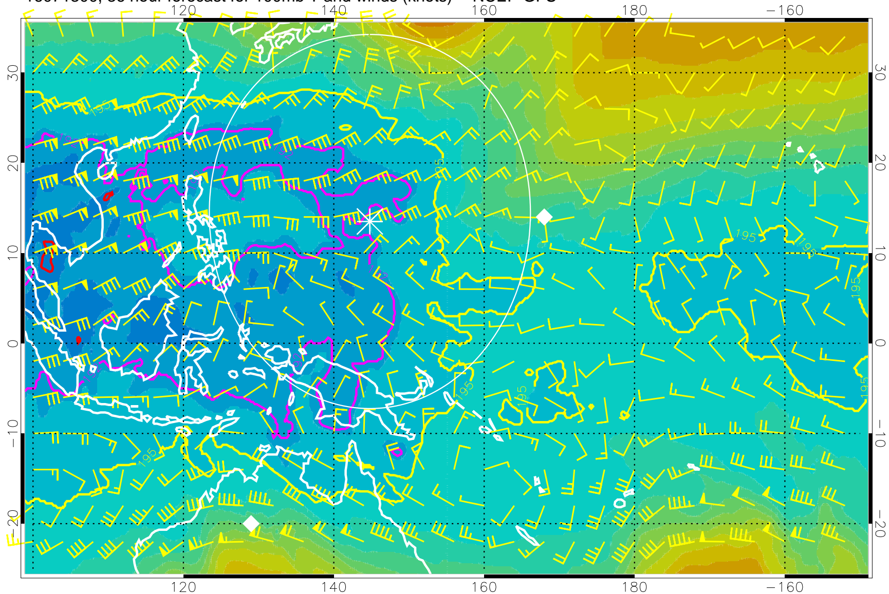
16071300, 36 hour forecast for 100mb T and winds (knots) -- NCEP GFS
