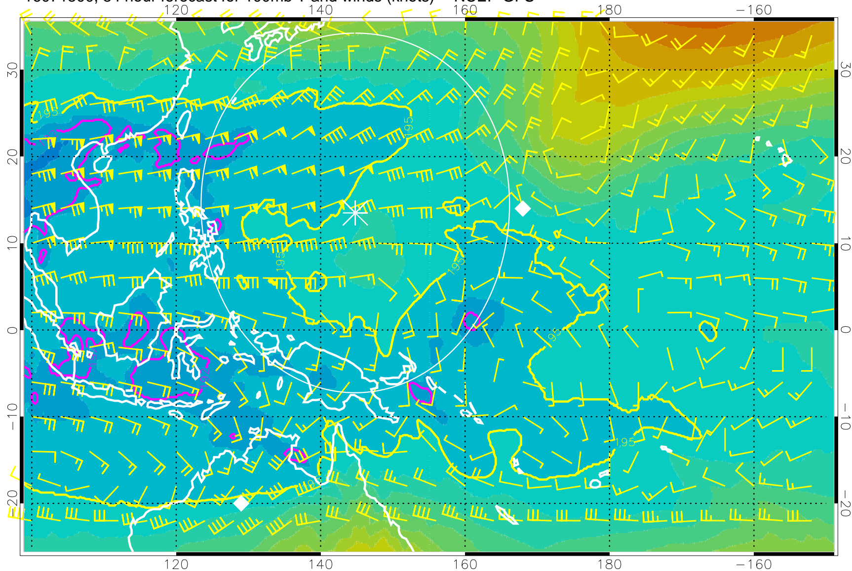
16071500, 84 hour forecast for 100mb T and winds (knots) -- NCEP GFS
