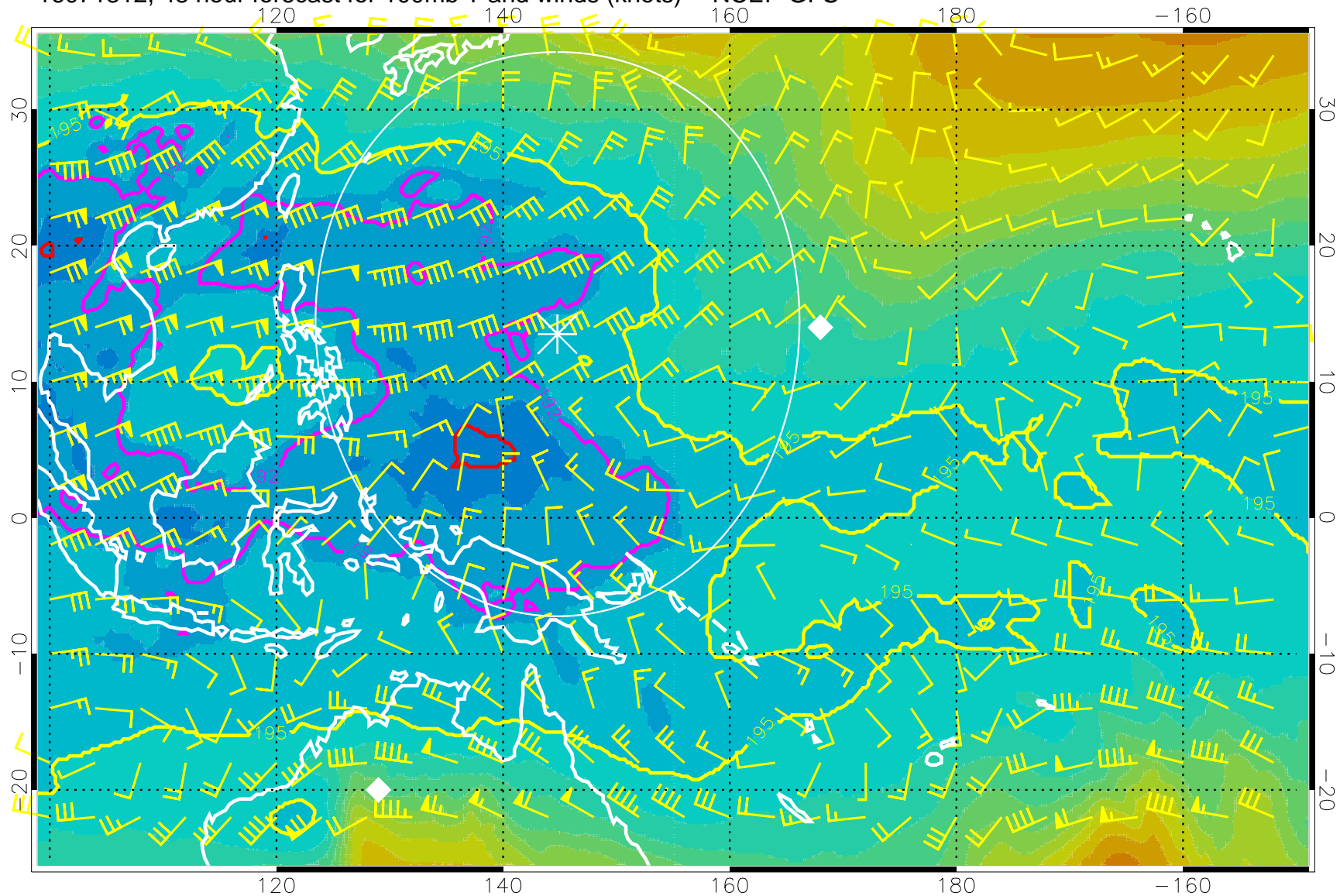
16071312, 48 hour forecast for 100mb T and winds (knots) -- NCEP GFS
