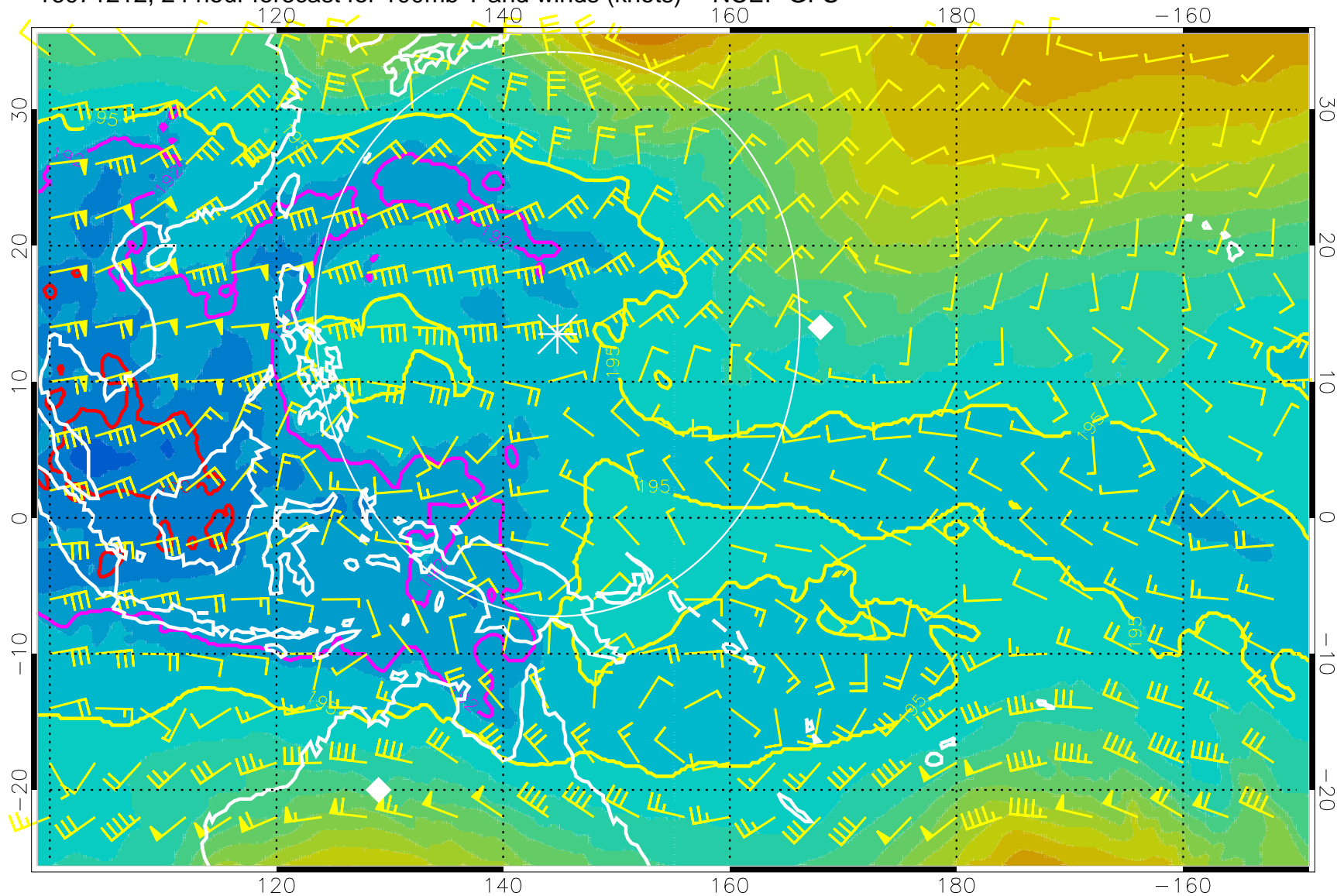
16071212, 24 hour forecast for 100mb T and winds (knots) -- NCEP GFS
