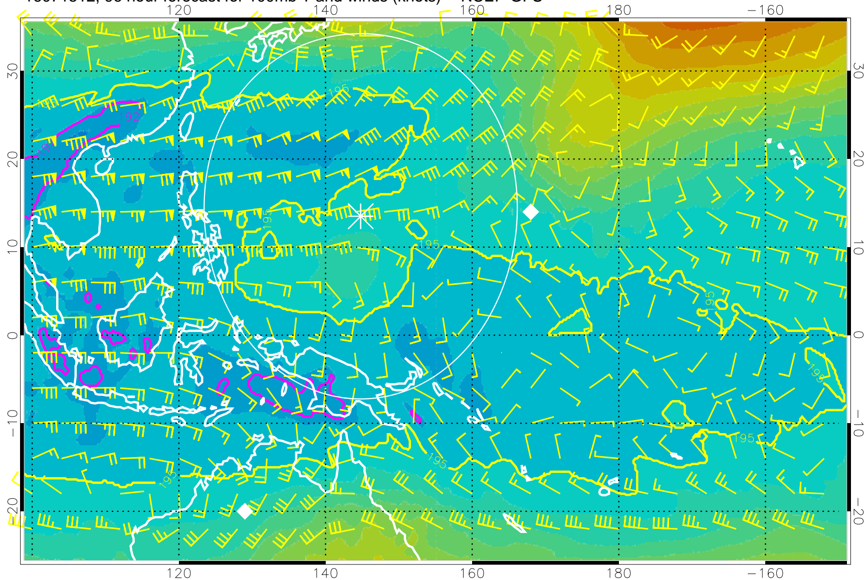
16071512, 96 hour forecast for 100mb T and winds (knots) -- NCEP GFS
