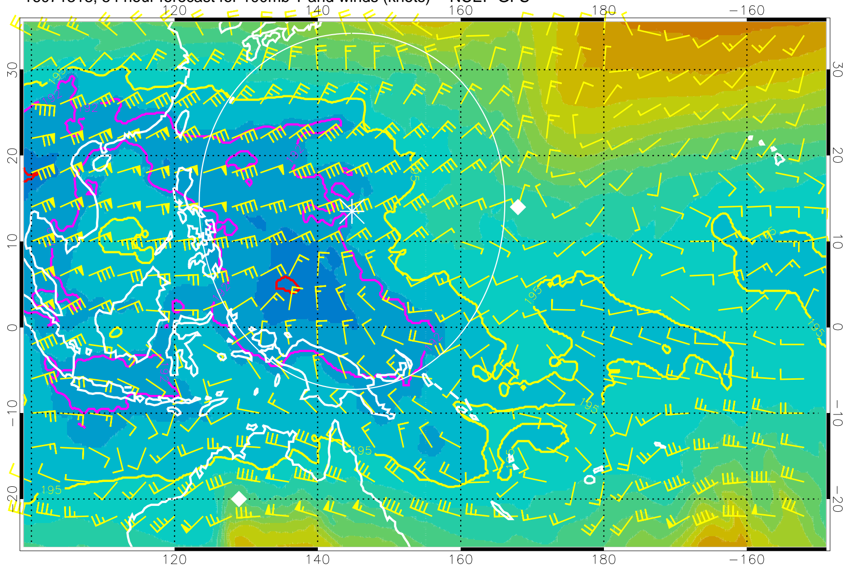
16071318, 54 hour forecast for 100mb T and winds (knots) -- NCEP GFS
