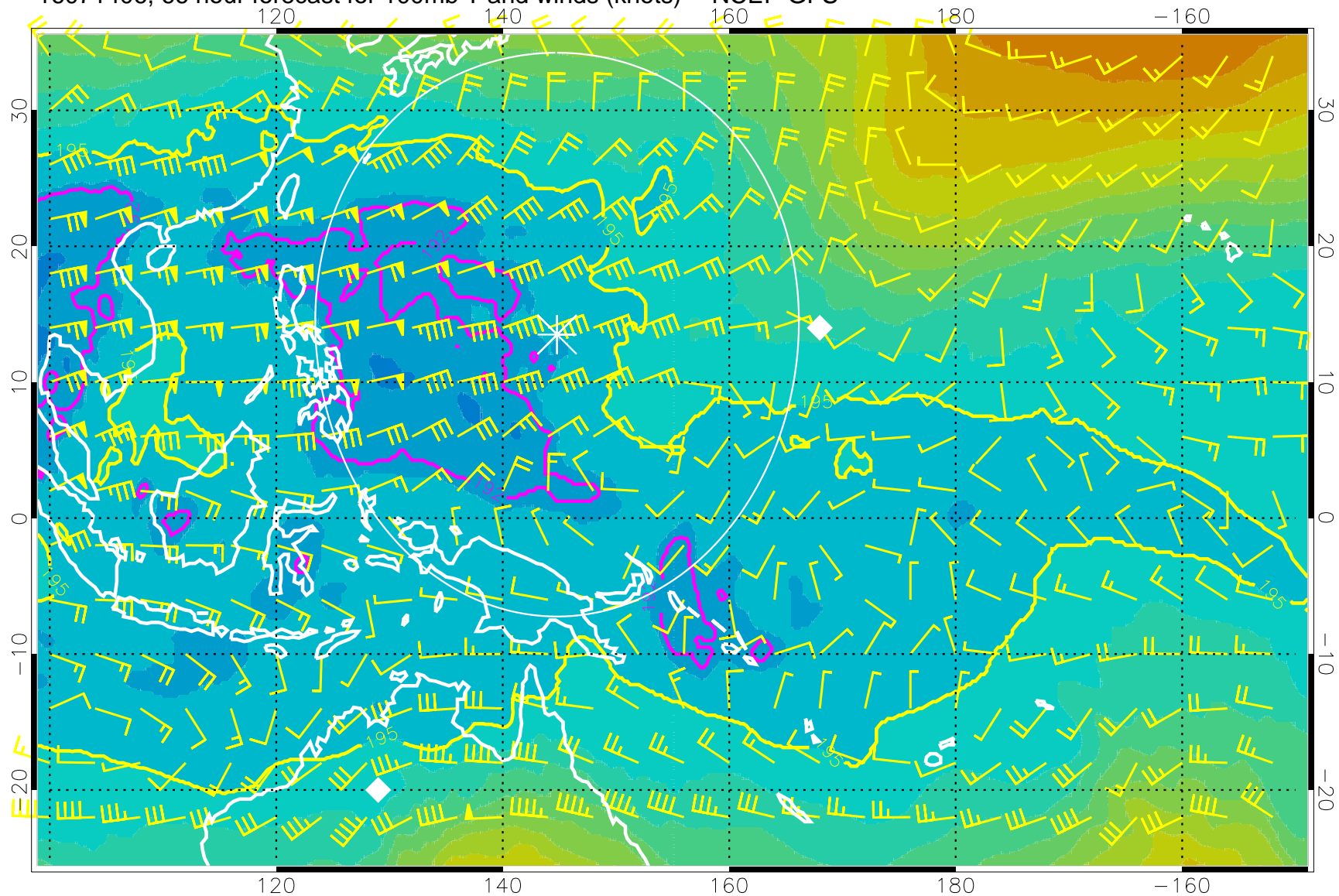
16071406, 66 hour forecast for 100mb T and winds (knots) -- NCEP GFS
