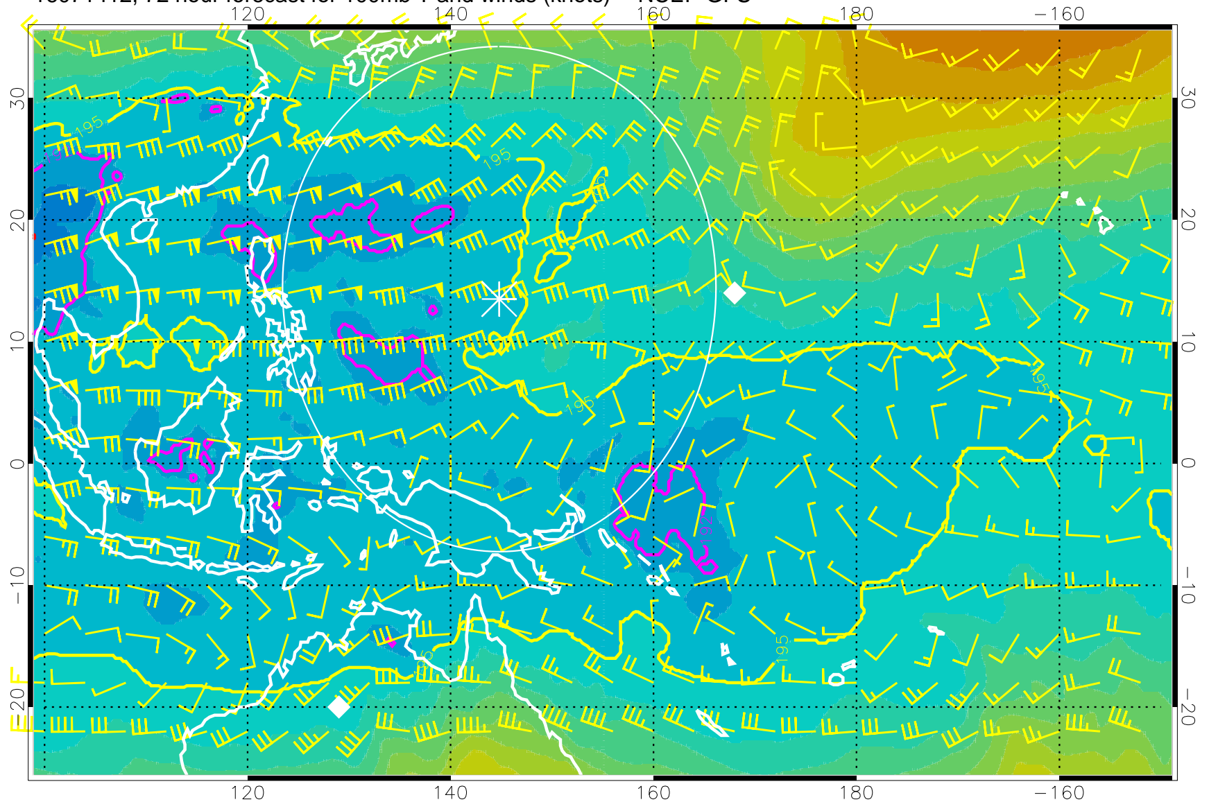
16071412, 72 hour forecast for 100mb T and winds (knots) -- NCEP GFS
