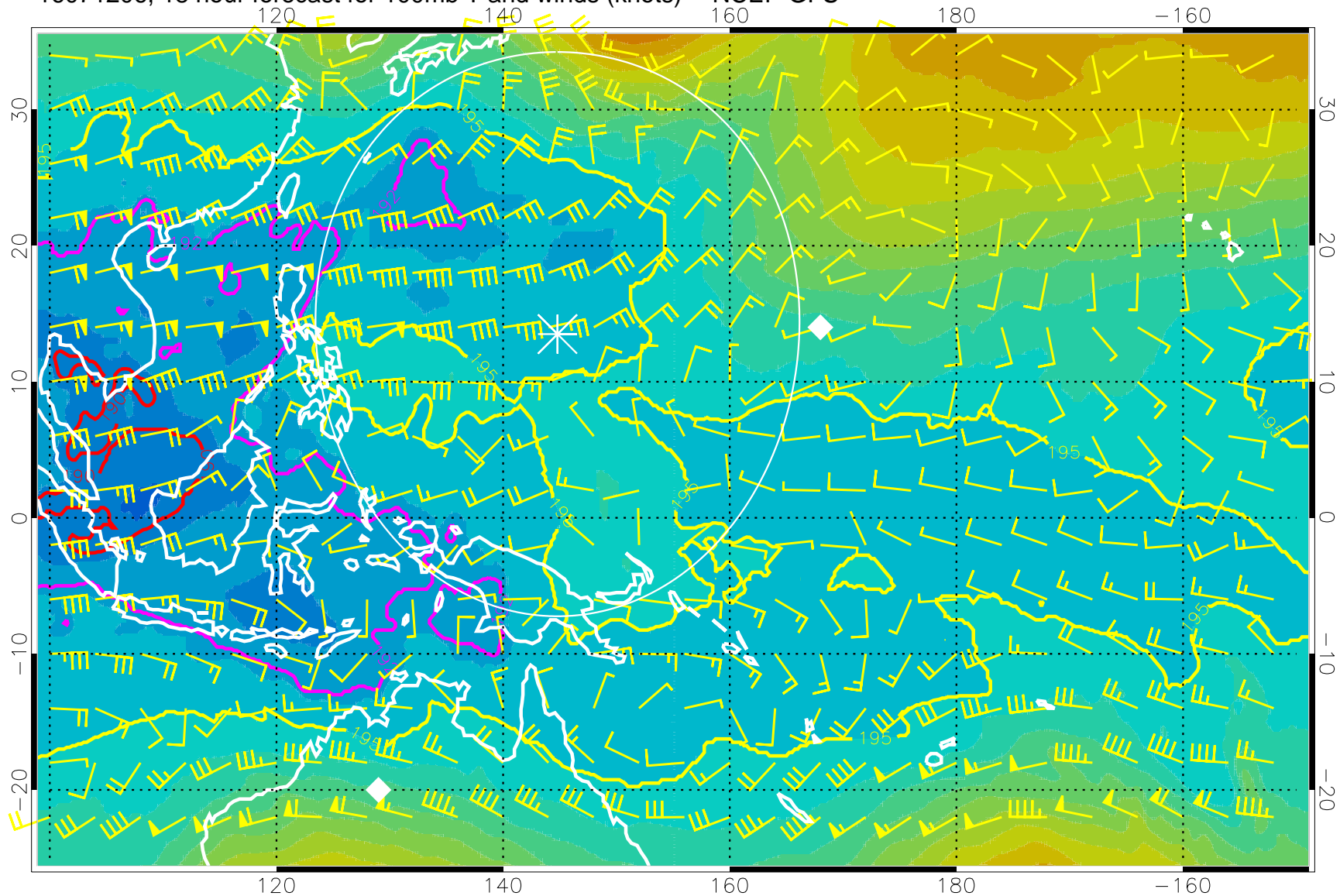
16071206, 18 hour forecast for 100mb T and winds (knots) -- NCEP GFS
