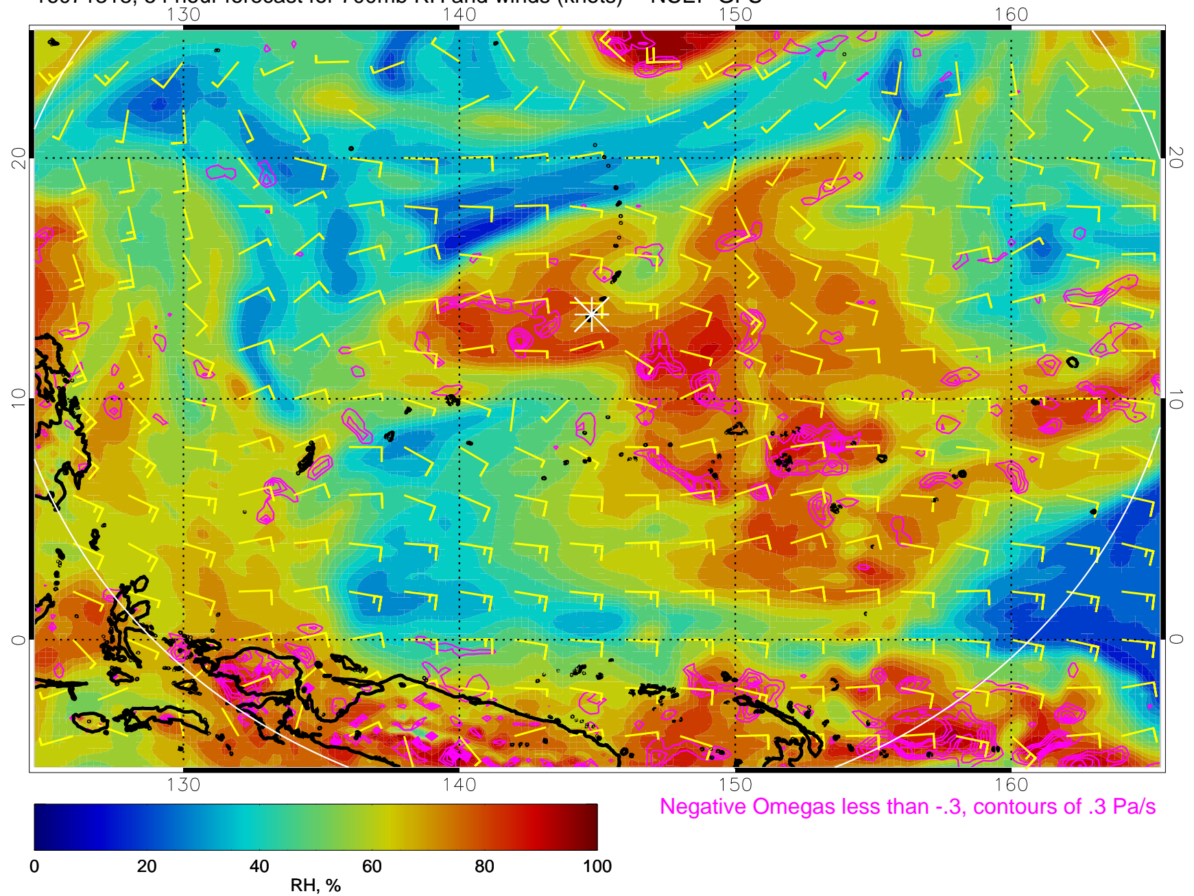
16071318, 54 hour forecast for 700mb RH and winds (knots) -- NCEP GFS
