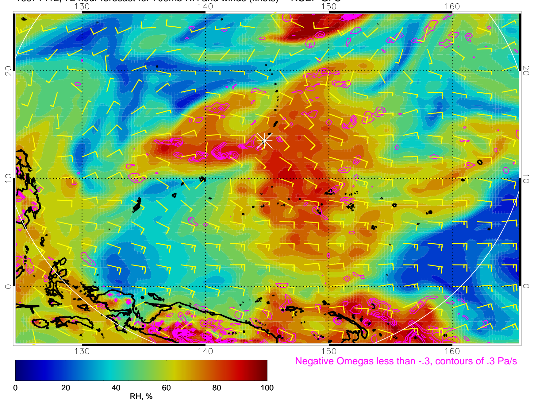
16071412, 72 hour forecast for 700mb RH and winds (knots) -- NCEP GFS
