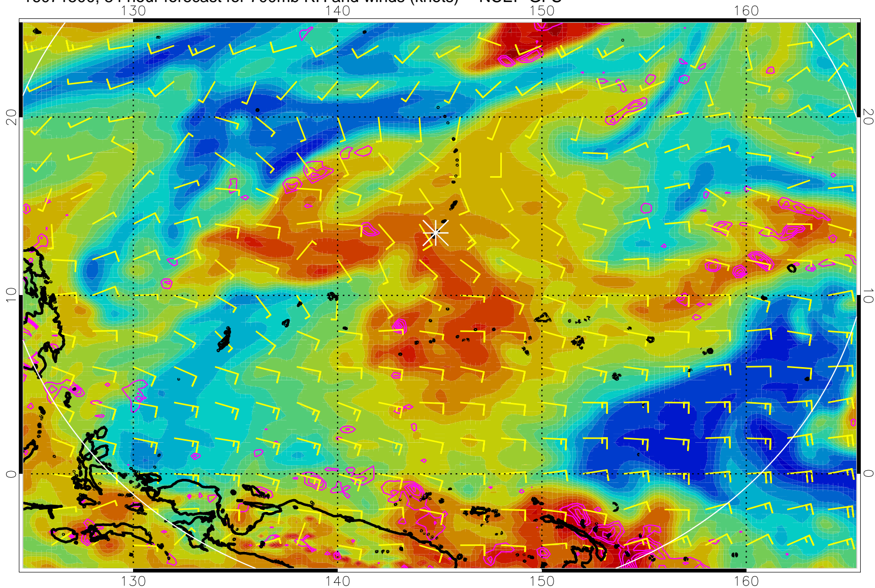
16071500, 84 hour forecast for 700mb RH and winds (knots) -- NCEP GFS
