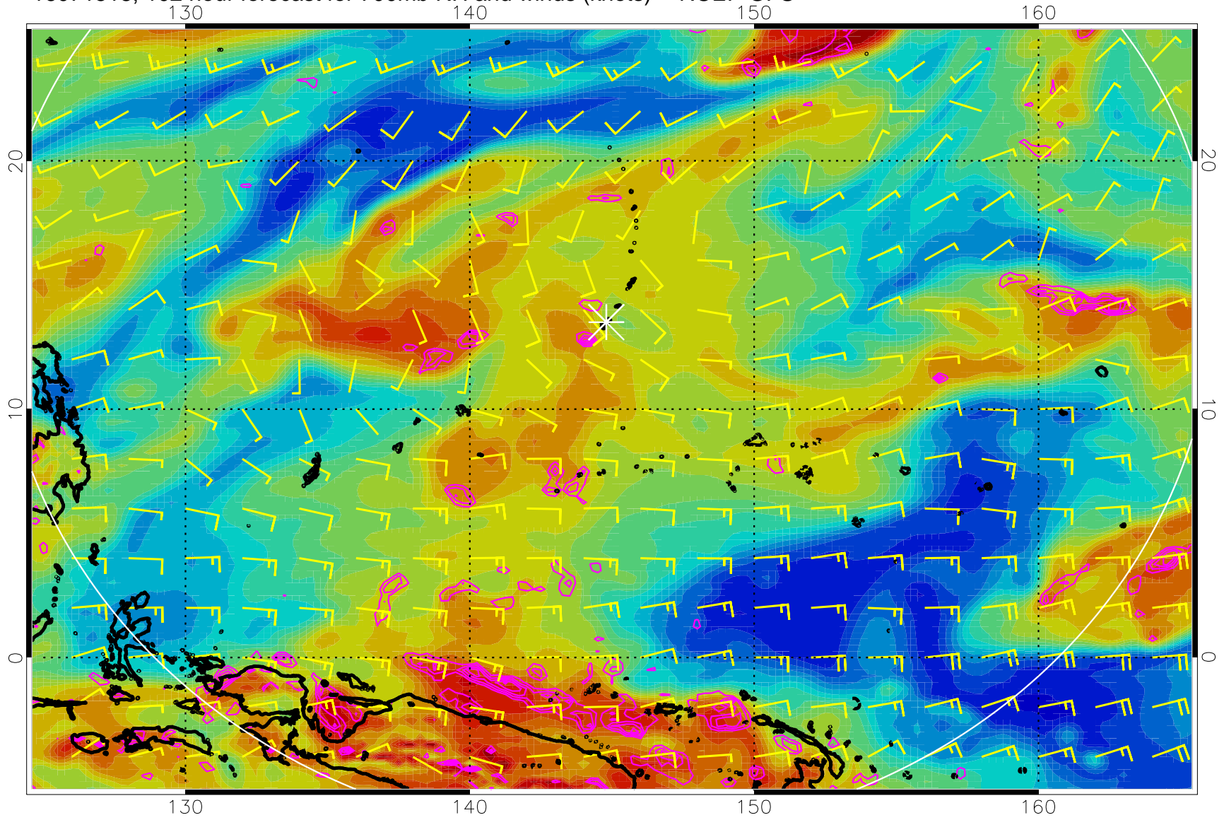
16071518, 102 hour forecast for 700mb RH and winds (knots) -- NCEP GFS
