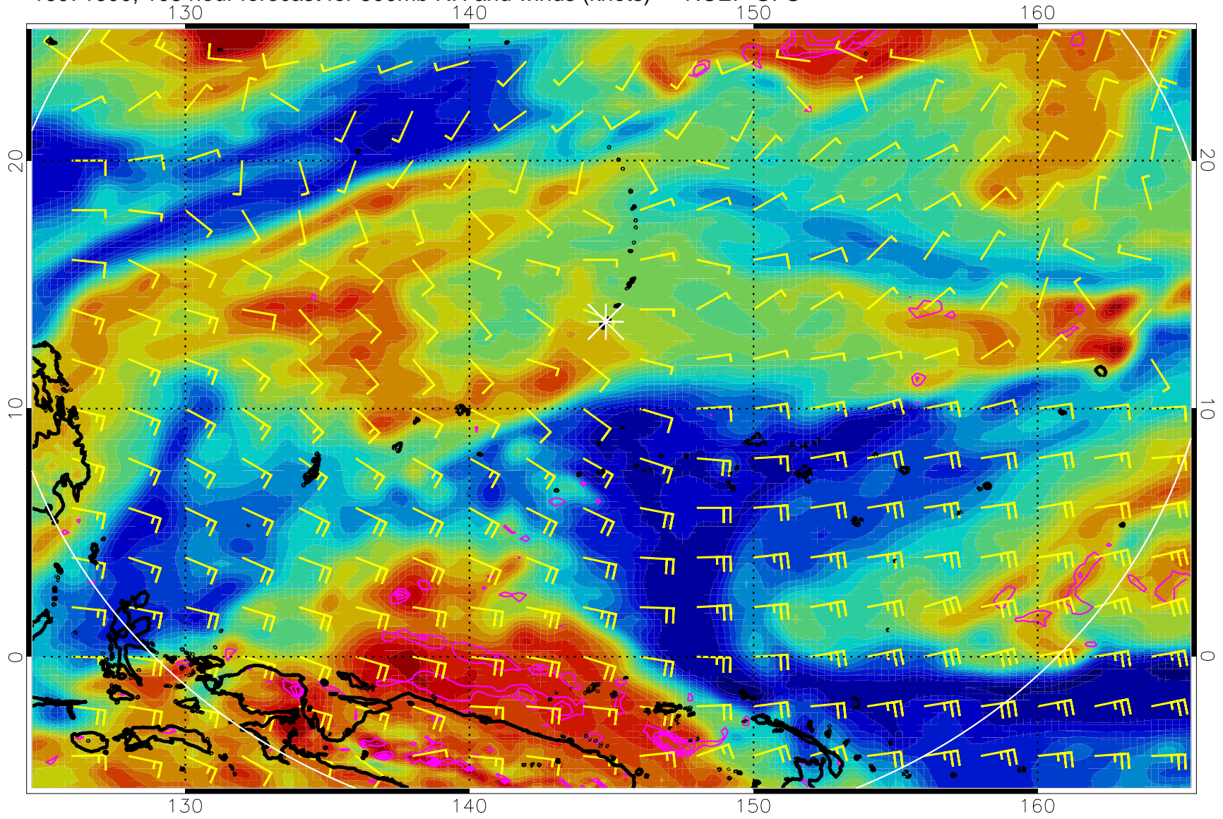
16071600, 108 hour forecast for 500mb RH and winds (knots) -- NCEP GFS
