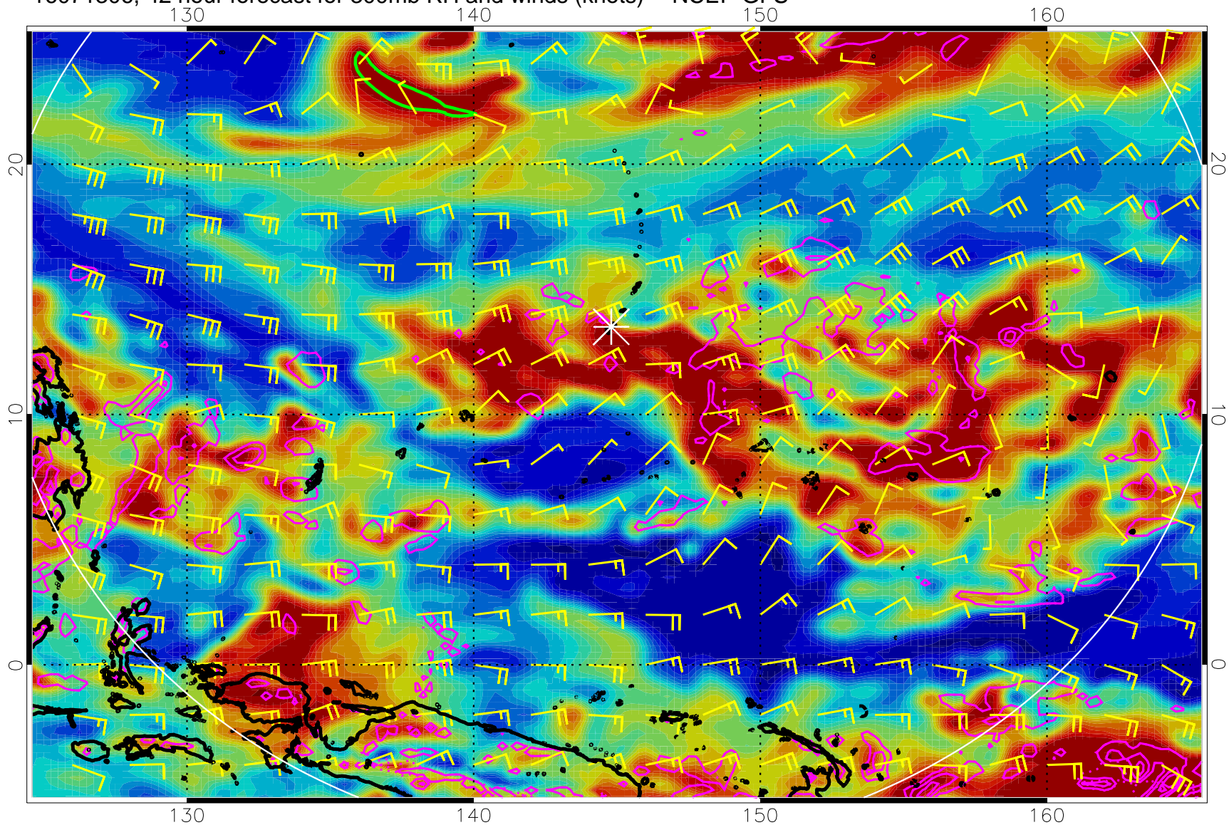
16071306, 42 hour forecast for 300mb RH and winds (knots) -- NCEP GFS
