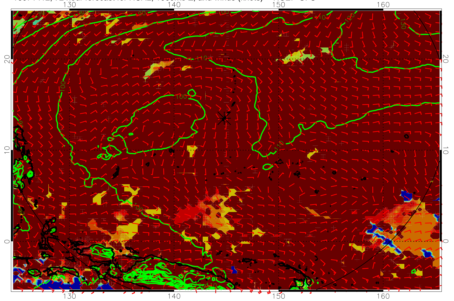
16071412, 72 hour forecast for HCAL, 1000mb Z, and winds (knots) -- NCEP GFS
