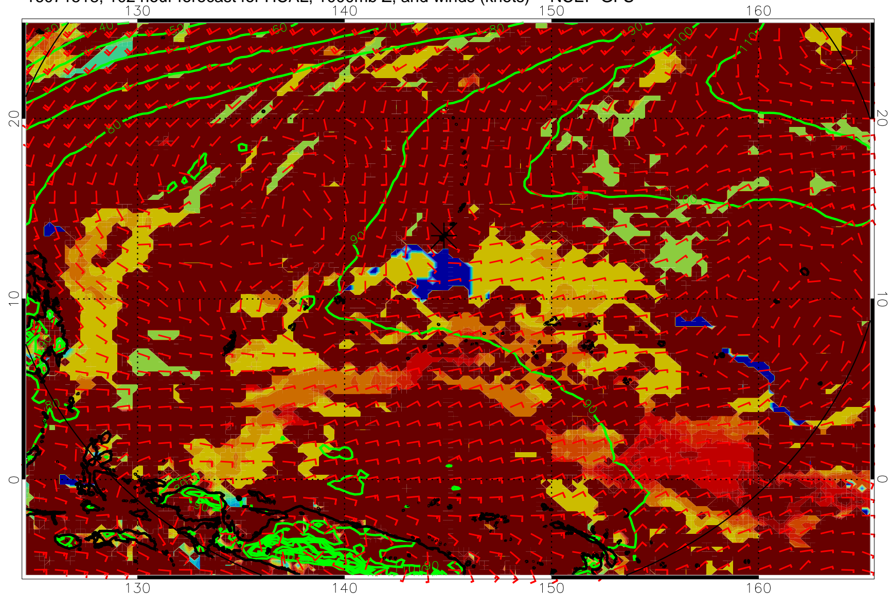
16071518, 102 hour forecast for HCAL, 1000mb Z, and winds (knots) -- NCEP GFS
