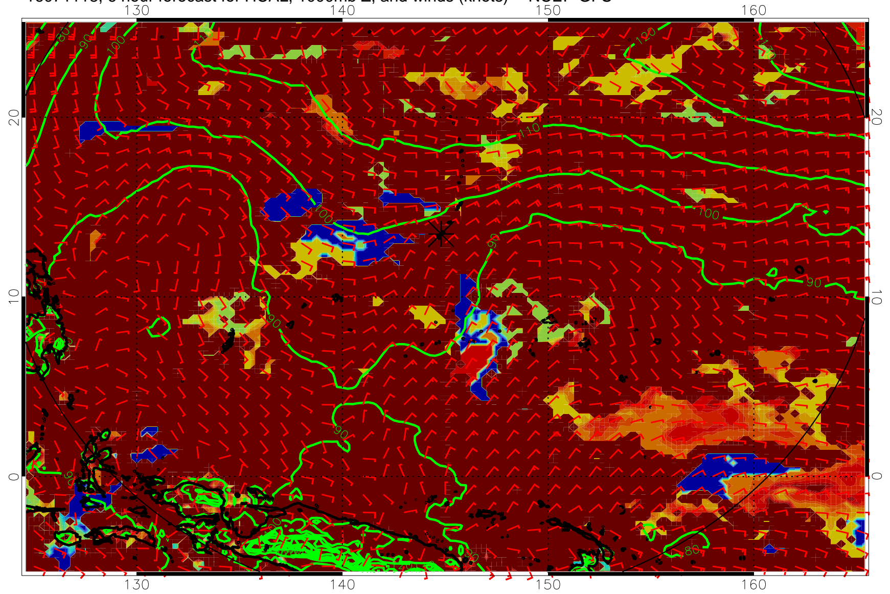
16071118, 6 hour forecast for HCAL, 1000mb Z, and winds (knots) -- NCEP GFS
