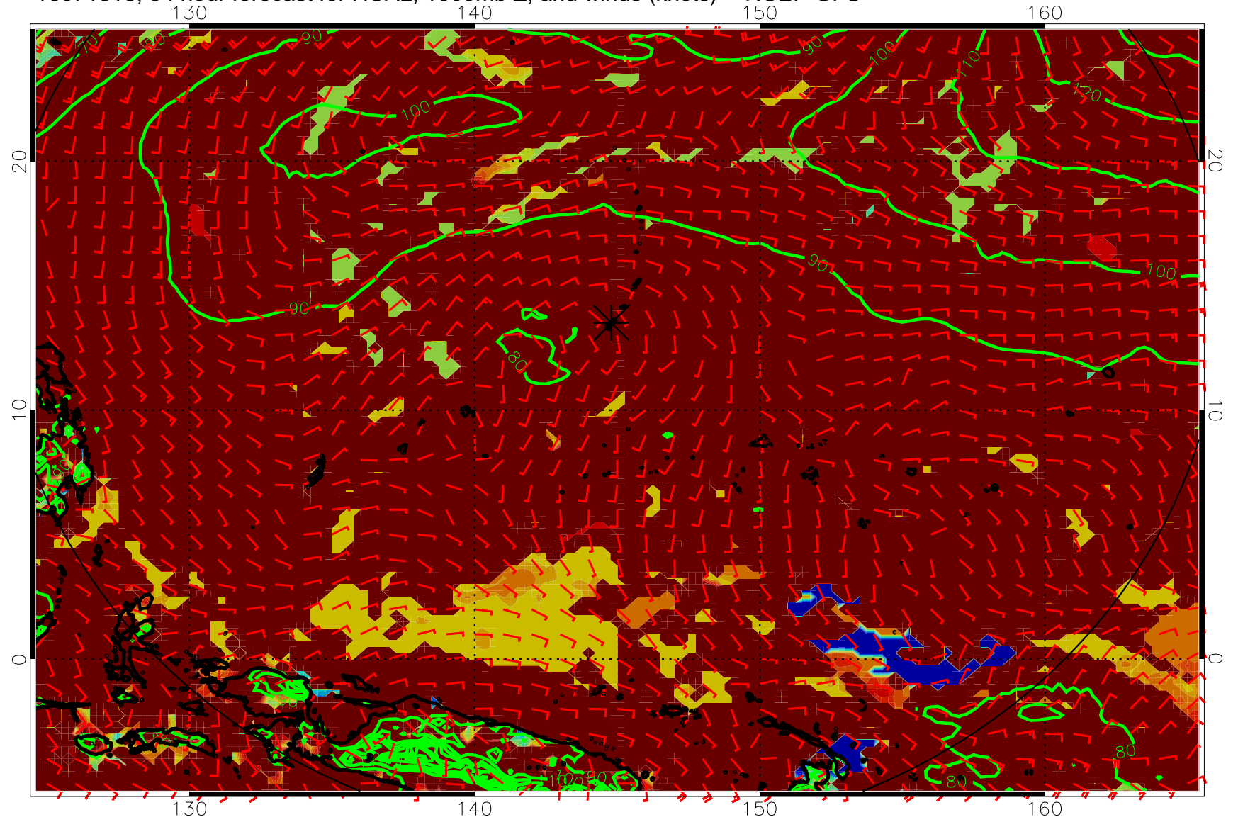
16071318, 54 hour forecast for HCAL, 1000mb Z, and winds (knots) -- NCEP GFS
