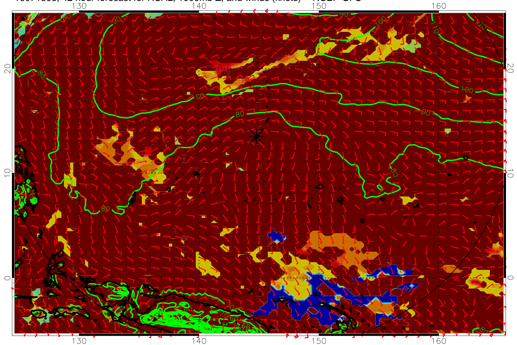
16071306, 42 hour forecast for HCAL, 1000mb Z, and winds (knots) -- NCEP GFS
