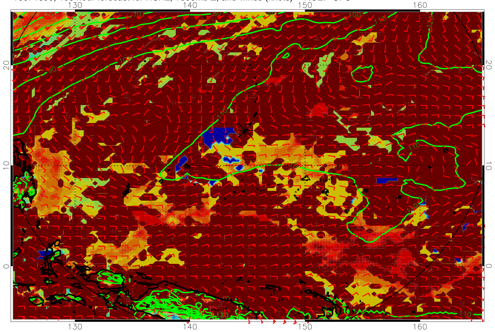
16071600, 108 hour forecast for HCAL, 1000mb Z, and winds (knots) -- NCEP GFS
