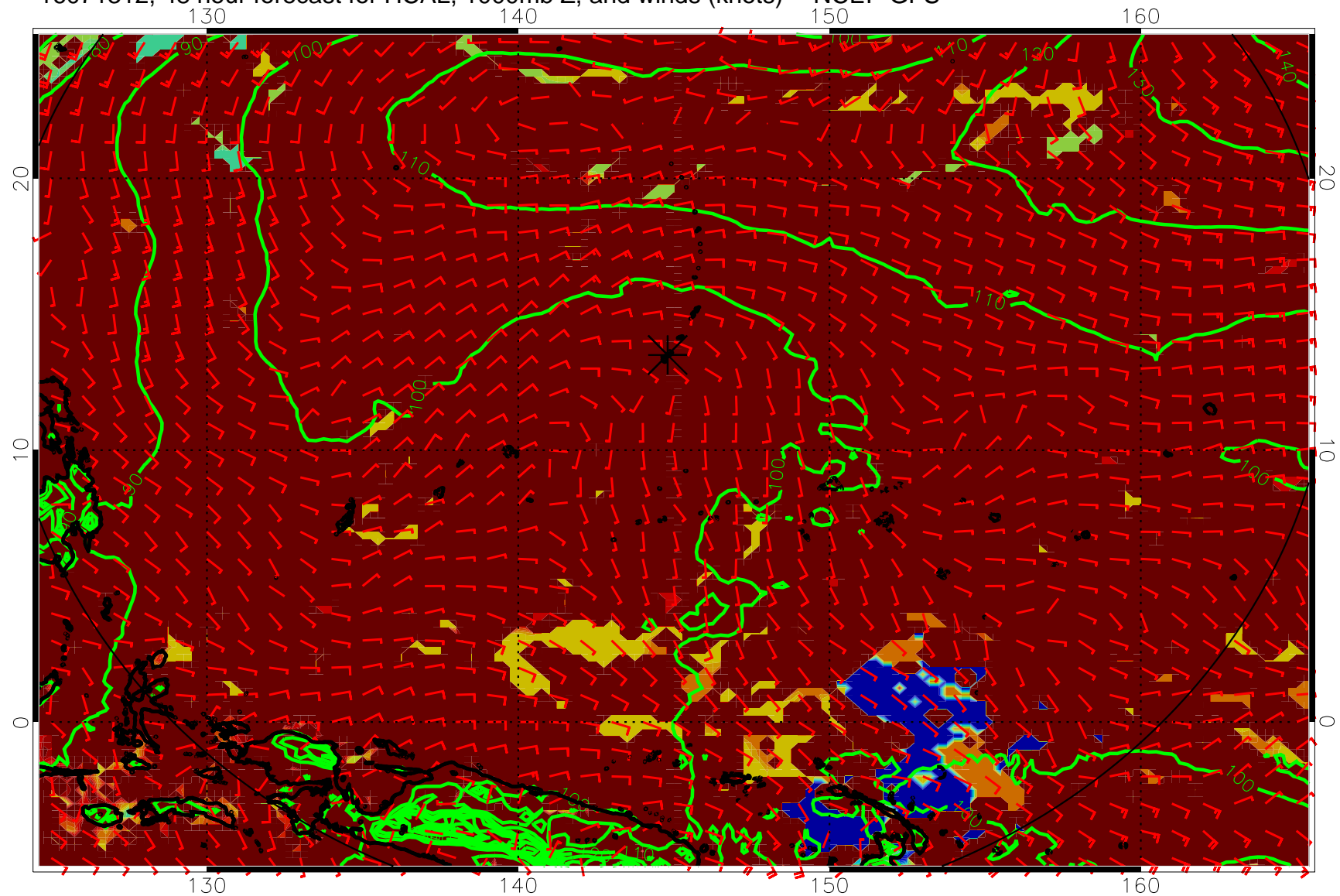
16071312, 48 hour forecast for HCAL, 1000mb Z, and winds (knots) -- NCEP GFS
