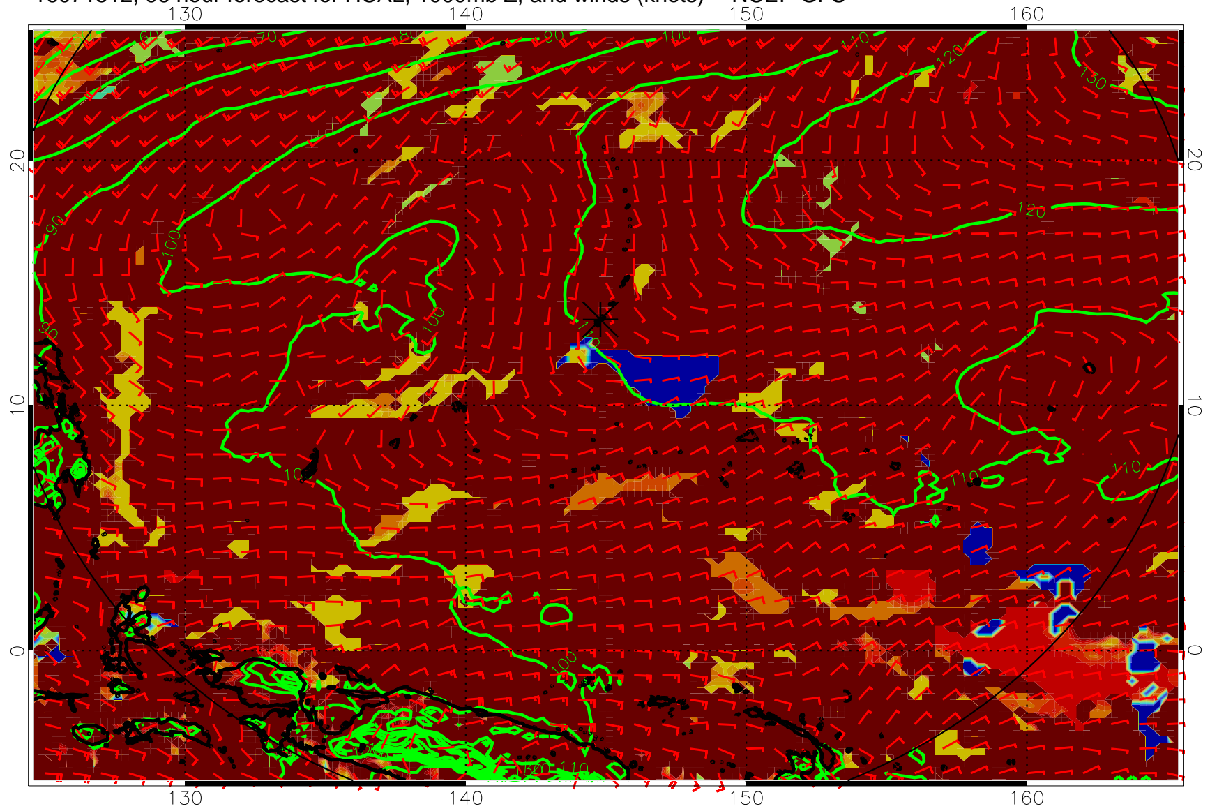
16071512, 96 hour forecast for HCAL, 1000mb Z, and winds (knots) -- NCEP GFS
