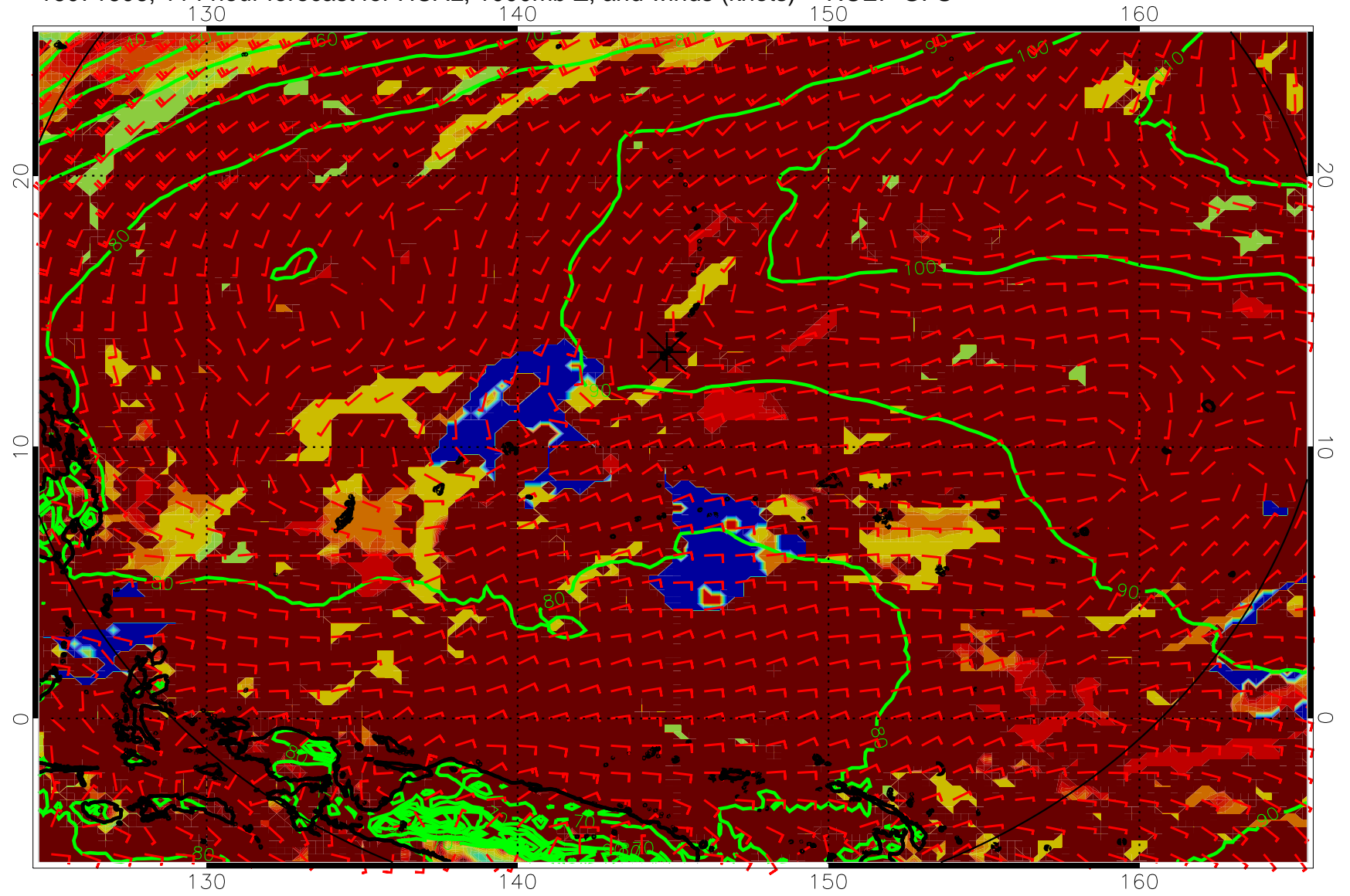
16071606, 114 hour forecast for HCAL, 1000mb Z, and winds (knots) -- NCEP GFS
