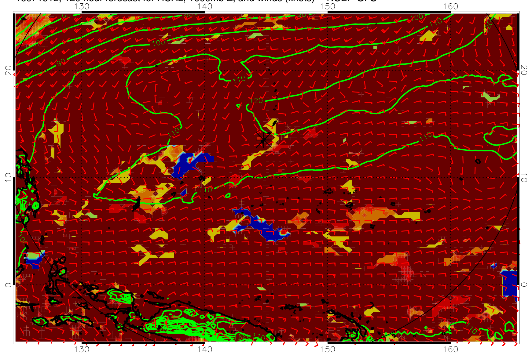
16071612, 120 hour forecast for HCAL, 1000mb Z, and winds (knots) -- NCEP GFS
