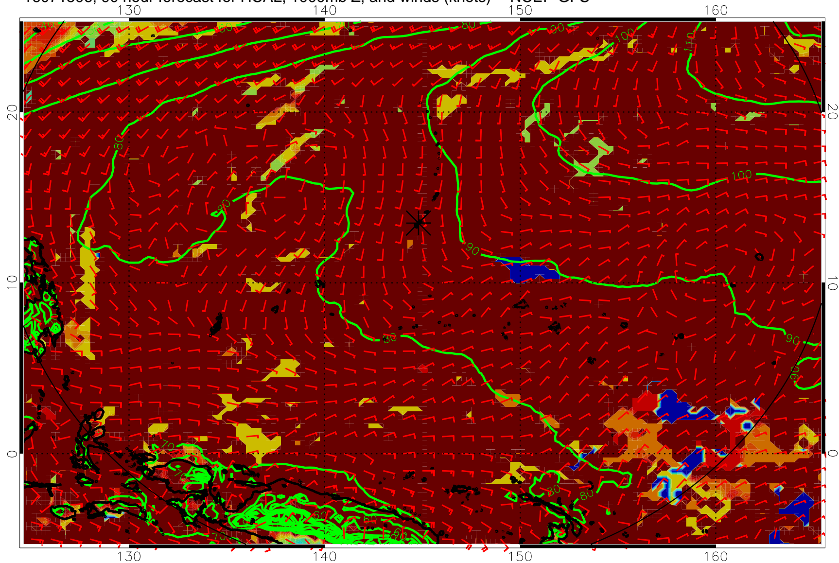
16071506, 90 hour forecast for HCAL, 1000mb Z, and winds (knots) -- NCEP GFS
