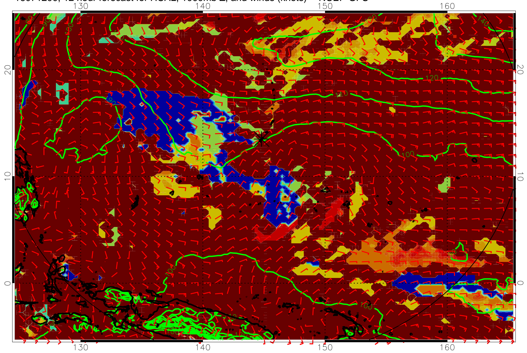
16071200, 12 hour forecast for HCAL, 1000mb Z, and winds (knots) -- NCEP GFS
