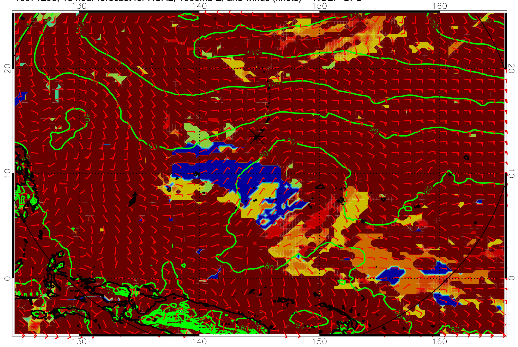
16071206, 18 hour forecast for HCAL, 1000mb Z, and winds (knots) -- NCEP GFS
