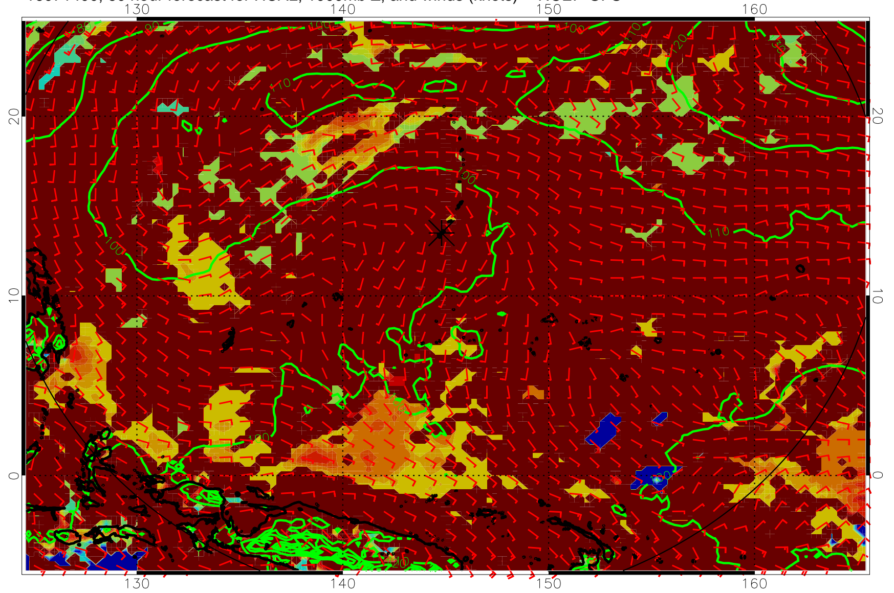
16071400, 60 hour forecast for HCAL, 1000mb Z, and winds (knots) -- NCEP GFS
