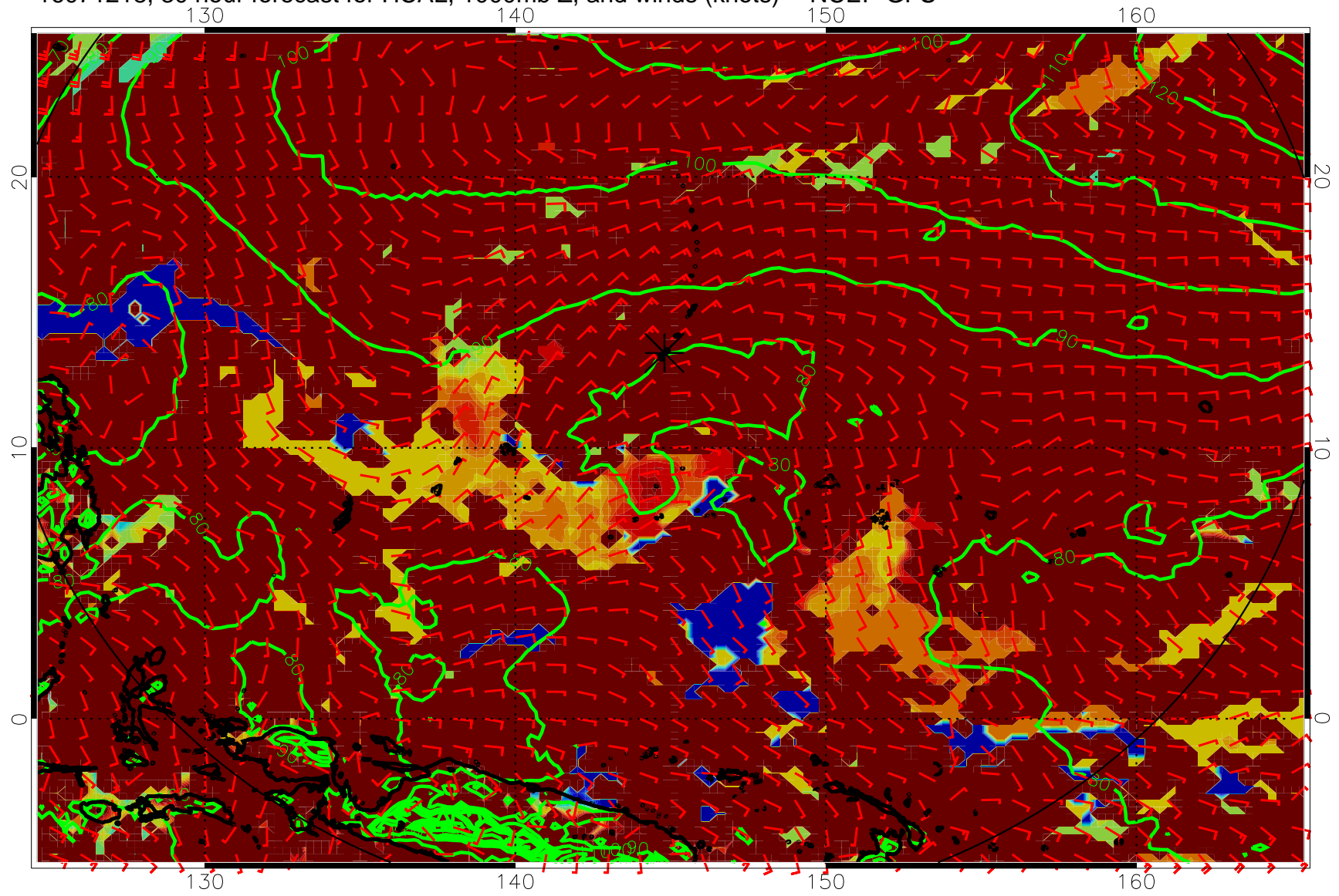
16071218, 30 hour forecast for HCAL, 1000mb Z, and winds (knots) -- NCEP GFS
