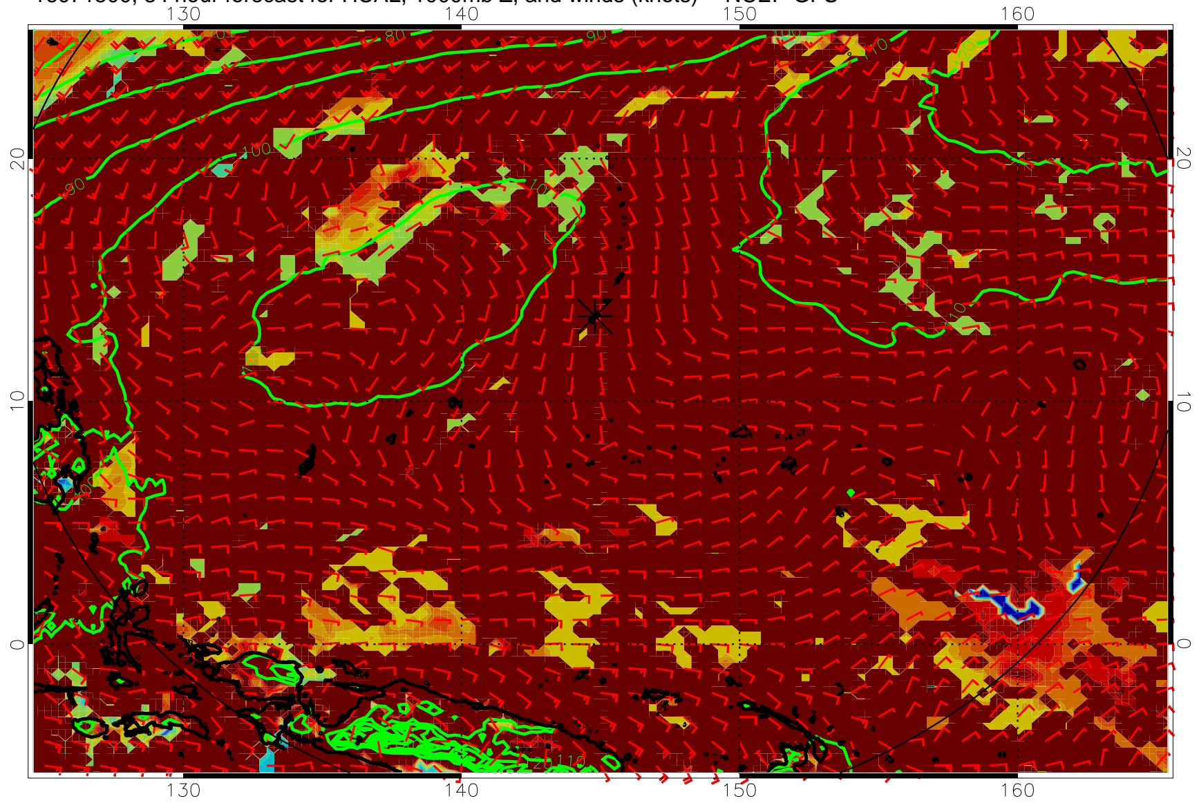
16071500, 84 hour forecast for HCAL, 1000mb Z, and winds (knots) -- NCEP GFS
