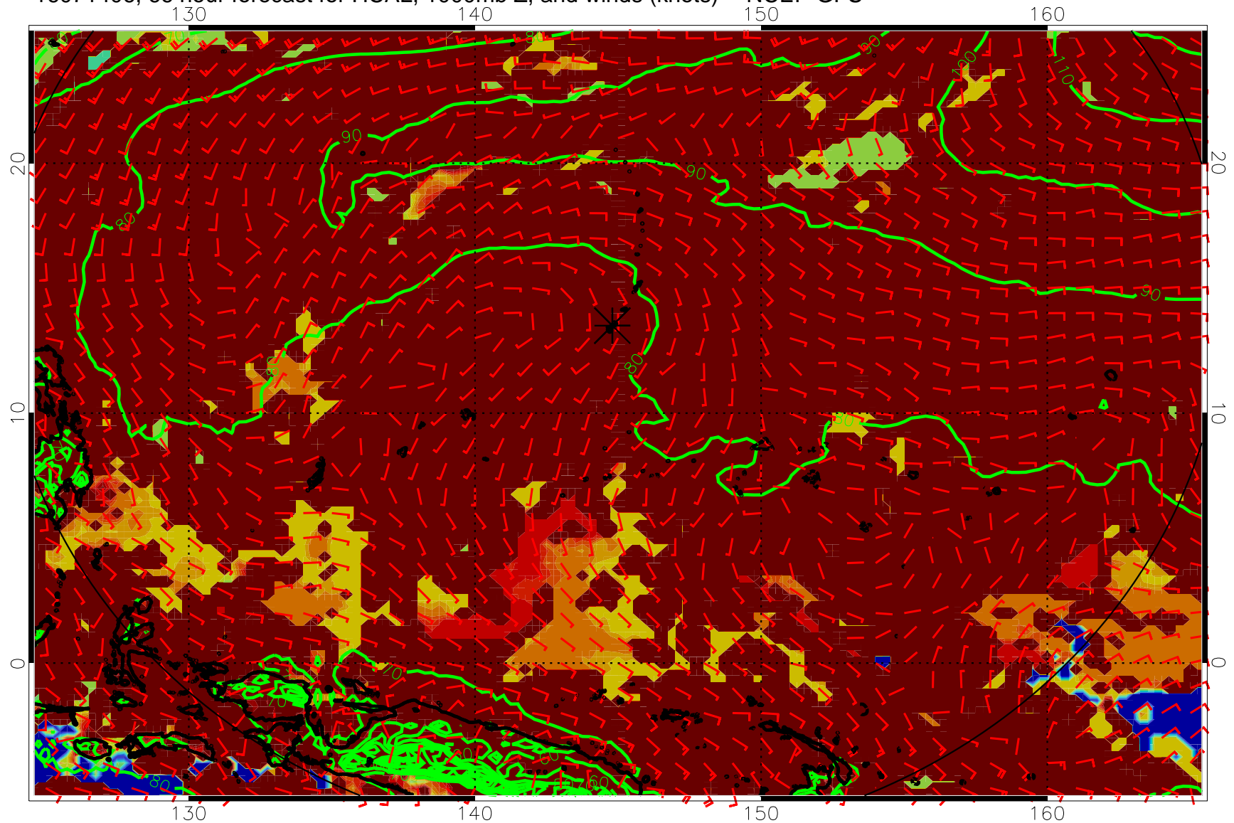
16071406, 66 hour forecast for HCAL, 1000mb Z, and winds (knots) -- NCEP GFS
