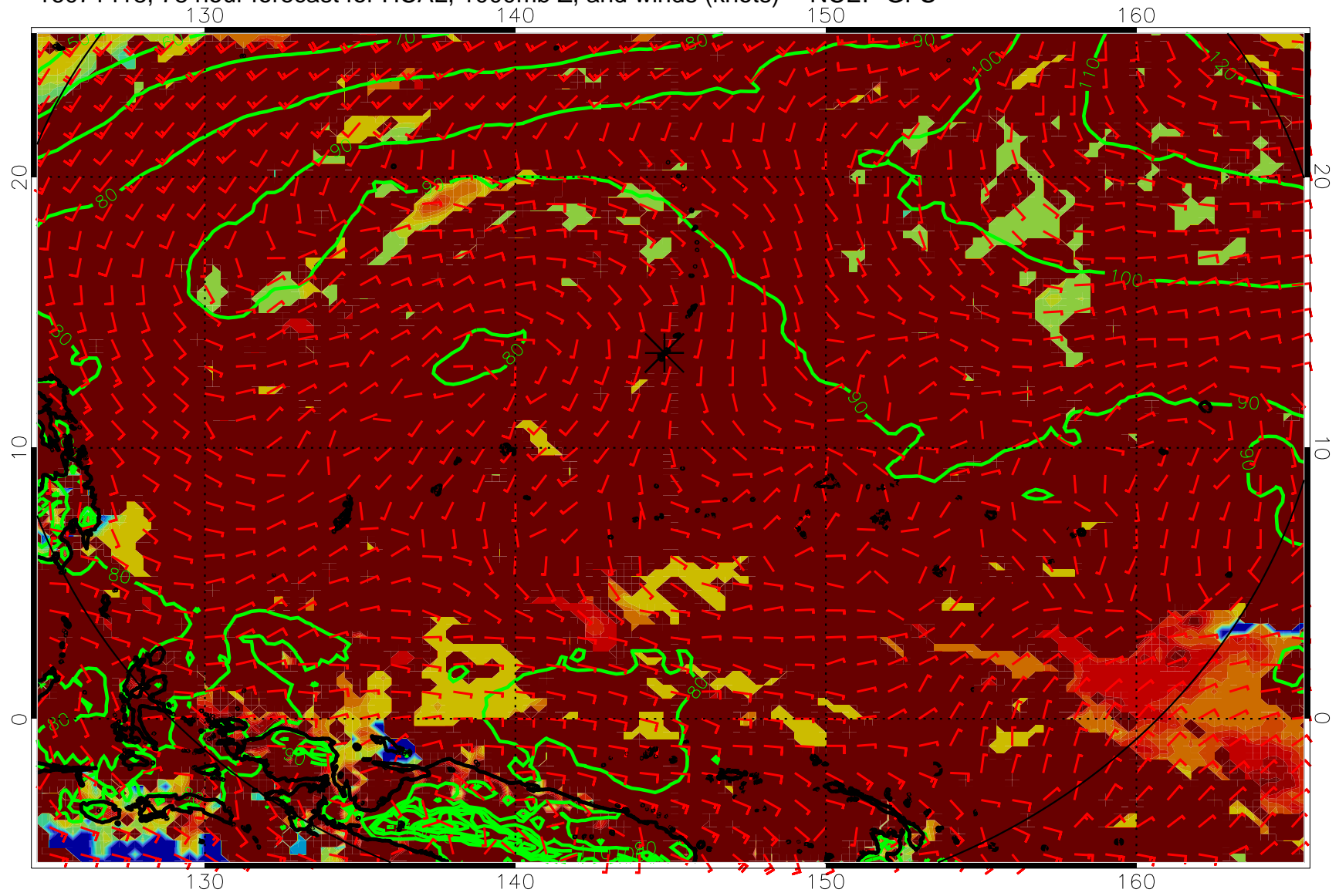
16071418, 78 hour forecast for HCAL, 1000mb Z, and winds (knots) -- NCEP GFS
