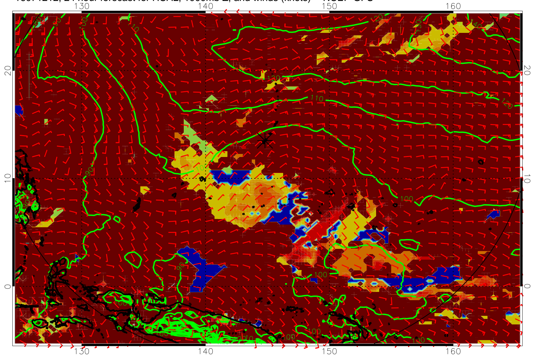
16071212, 24 hour forecast for HCAL, 1000mb Z, and winds (knots) -- NCEP GFS
