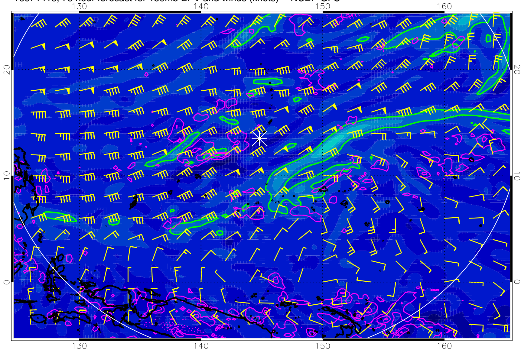
16071418, 78 hour forecast for 150mb EPV and winds (knots) -- NCEP GFS
