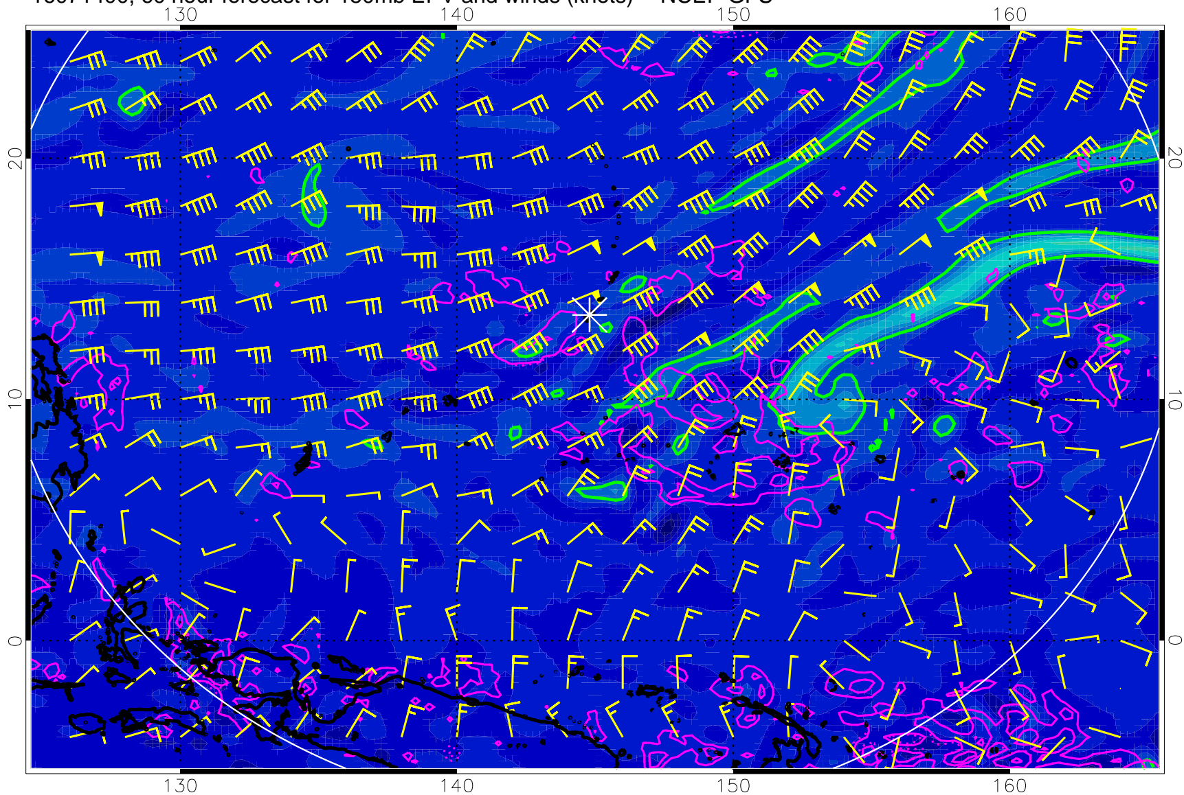
16071400, 60 hour forecast for 150mb EPV and winds (knots) -- NCEP GFS
