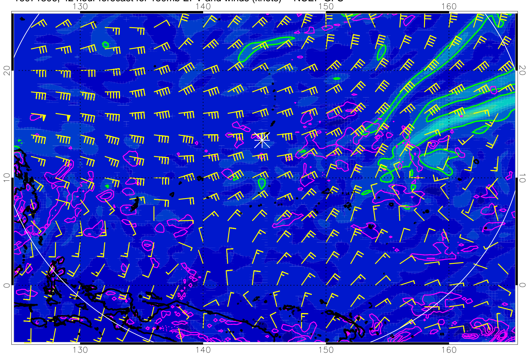
16071306, 42 hour forecast for 150mb EPV and winds (knots) -- NCEP GFS
