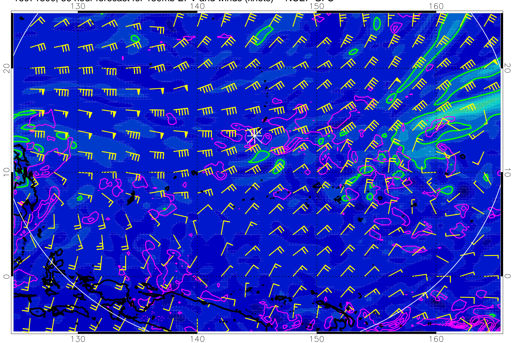
16071300, 36 hour forecast for 150mb EPV and winds (knots) -- NCEP GFS
