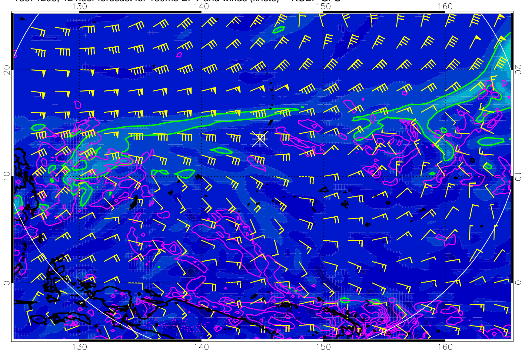
16071200, 12 hour forecast for 150mb EPV and winds (knots) -- NCEP GFS
