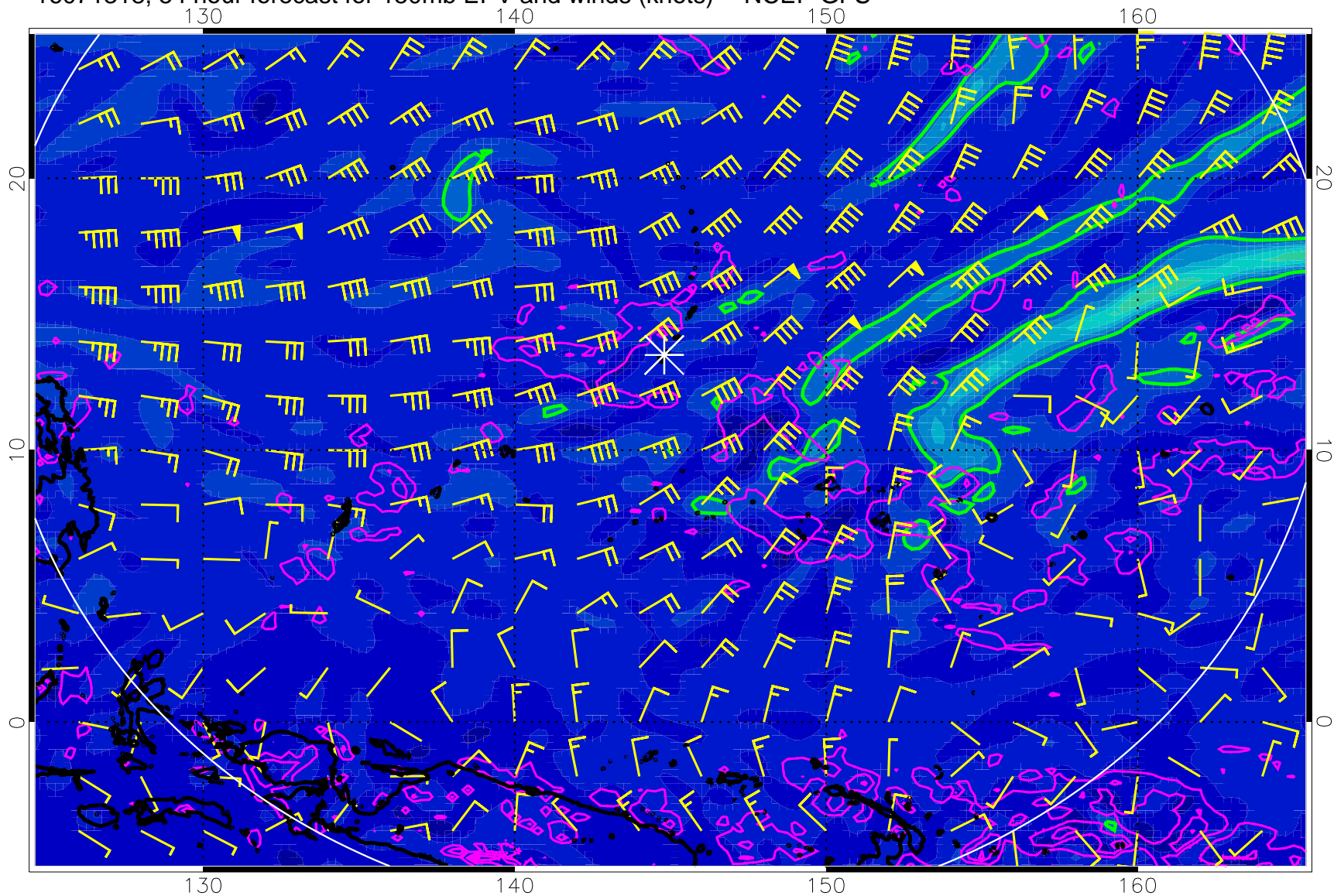
16071318, 54 hour forecast for 150mb EPV and winds (knots) -- NCEP GFS
