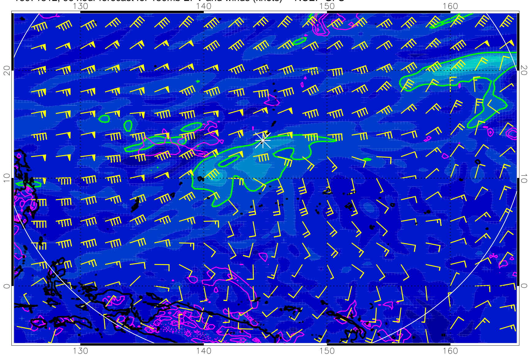
16071512, 96 hour forecast for 150mb EPV and winds (knots) -- NCEP GFS
