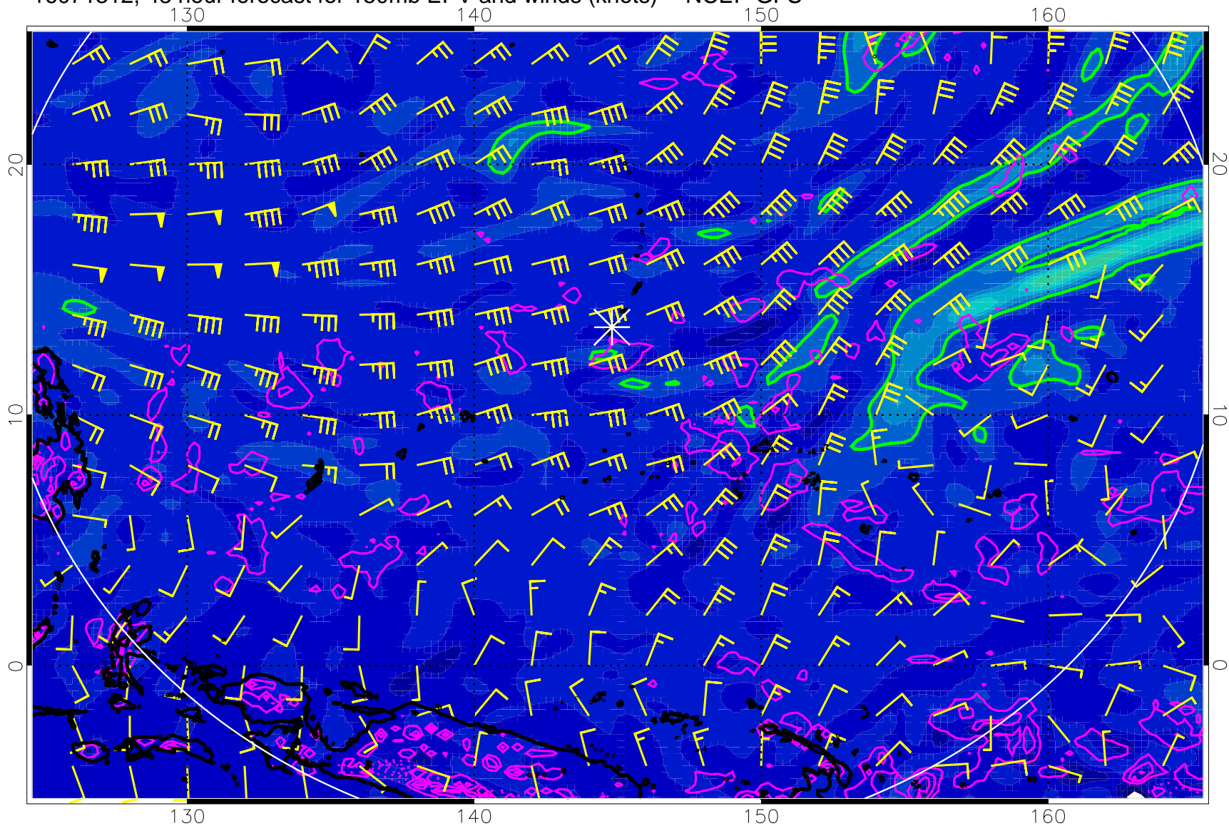
16071312, 48 hour forecast for 150mb EPV and winds (knots) -- NCEP GFS
