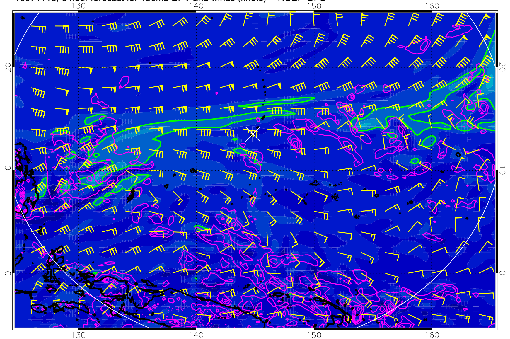
16071118, 6 hour forecast for 150mb EPV and winds (knots) -- NCEP GFS
