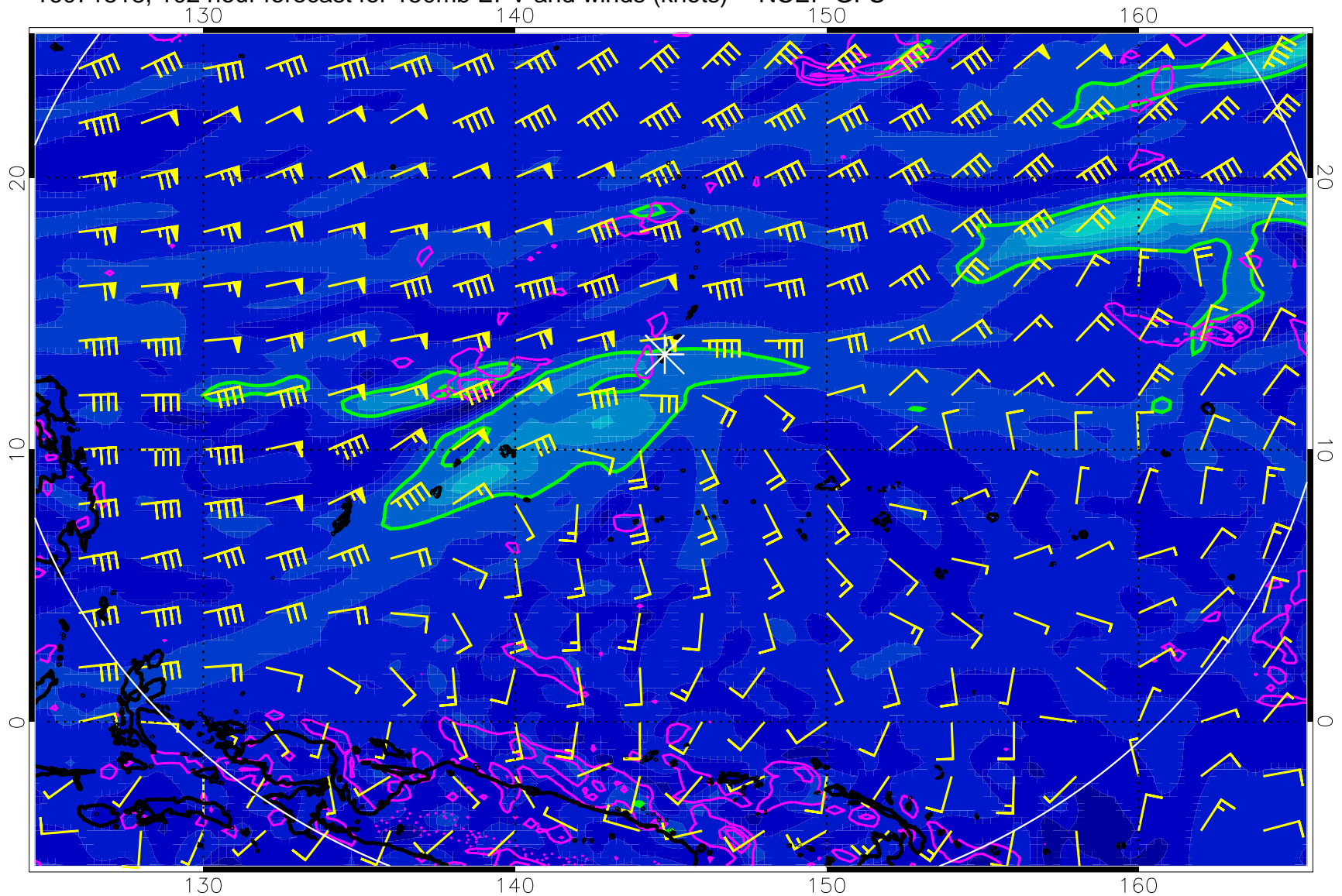
16071518, 102 hour forecast for 150mb EPV and winds (knots) -- NCEP GFS
