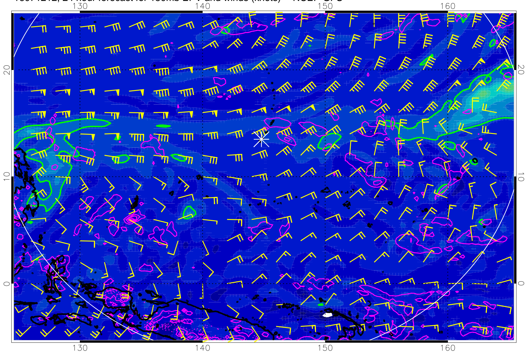
16071212, 24 hour forecast for 150mb EPV and winds (knots) -- NCEP GFS
