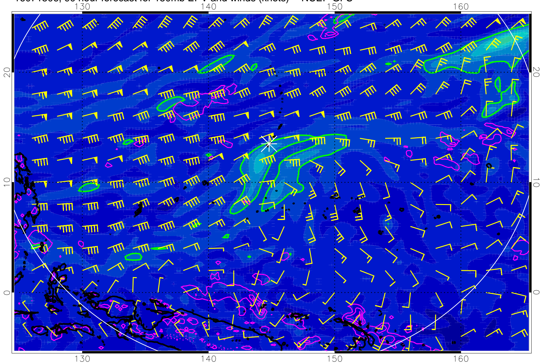
16071506, 90 hour forecast for 150mb EPV and winds (knots) -- NCEP GFS
