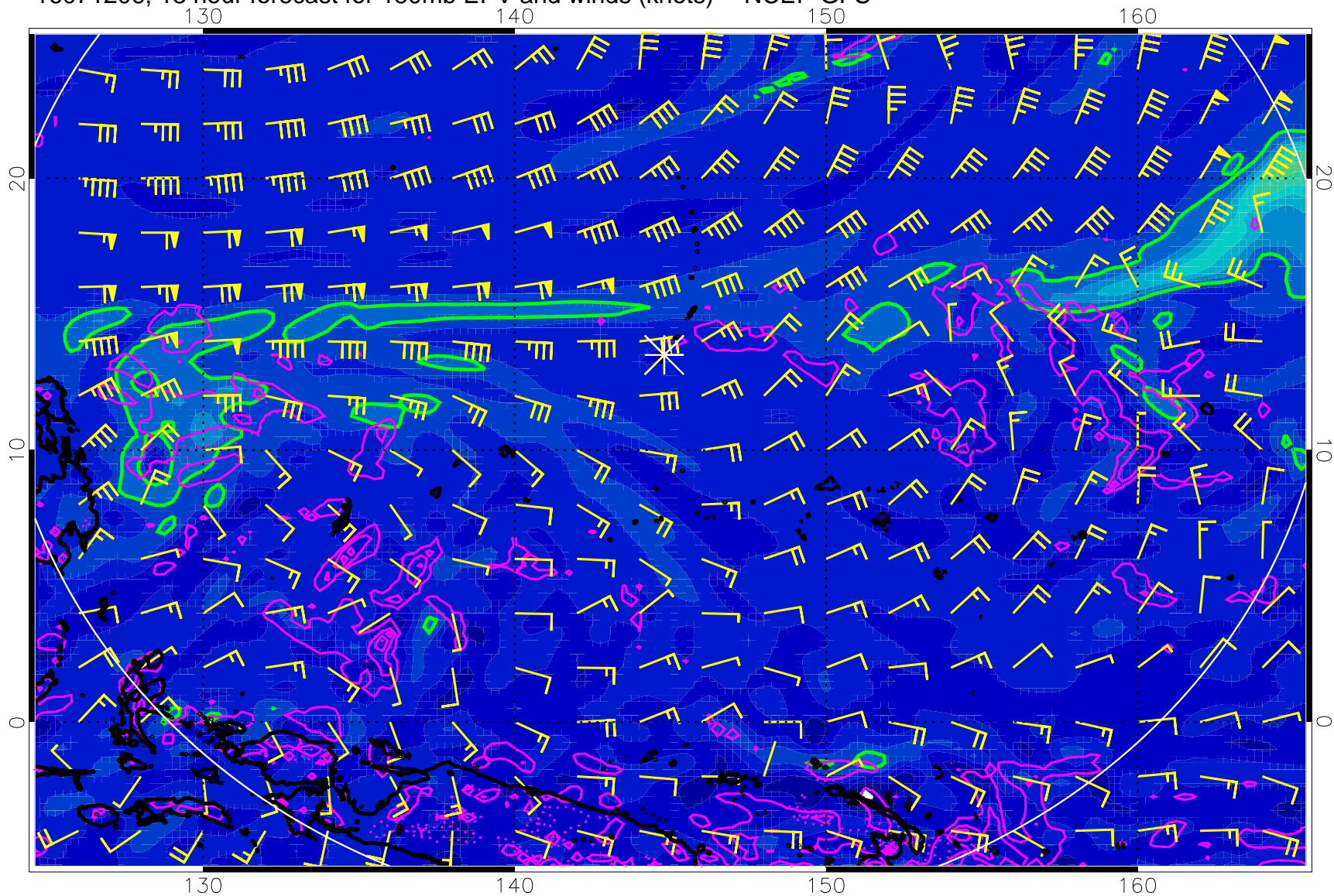
16071206, 18 hour forecast for 150mb EPV and winds (knots) -- NCEP GFS
