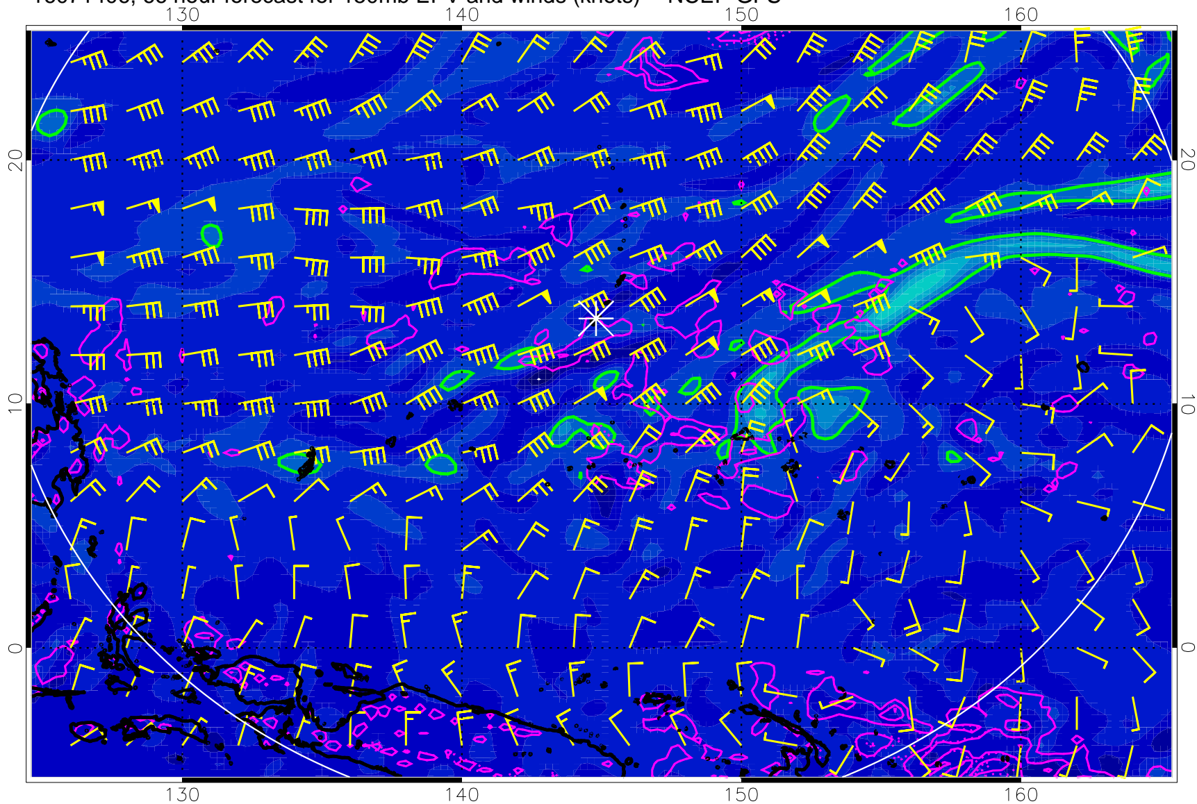
16071406, 66 hour forecast for 150mb EPV and winds (knots) -- NCEP GFS
