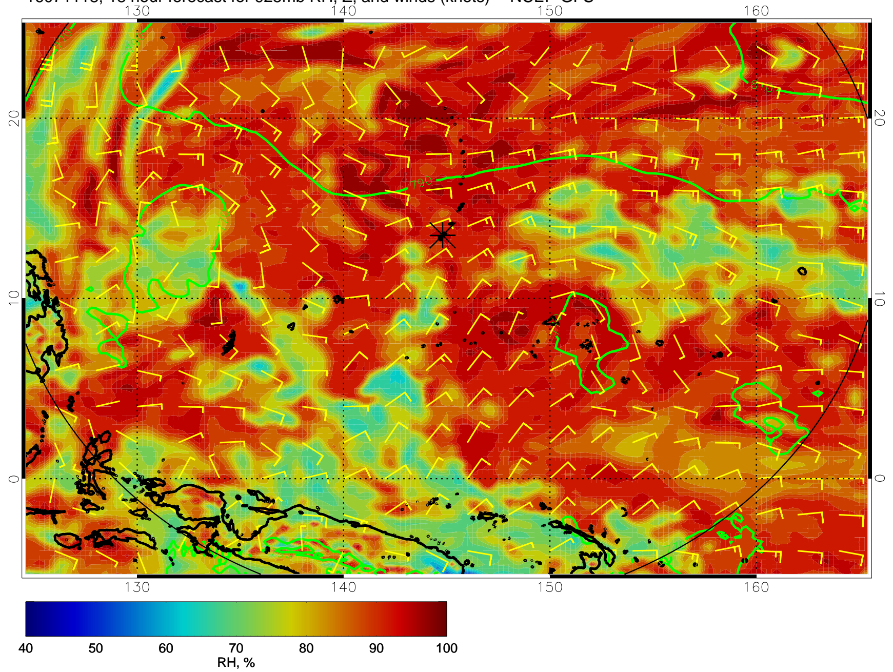
16071118, 18 hour forecast for 925mb RH, Z, and winds (knots) -- NCEP GFS
