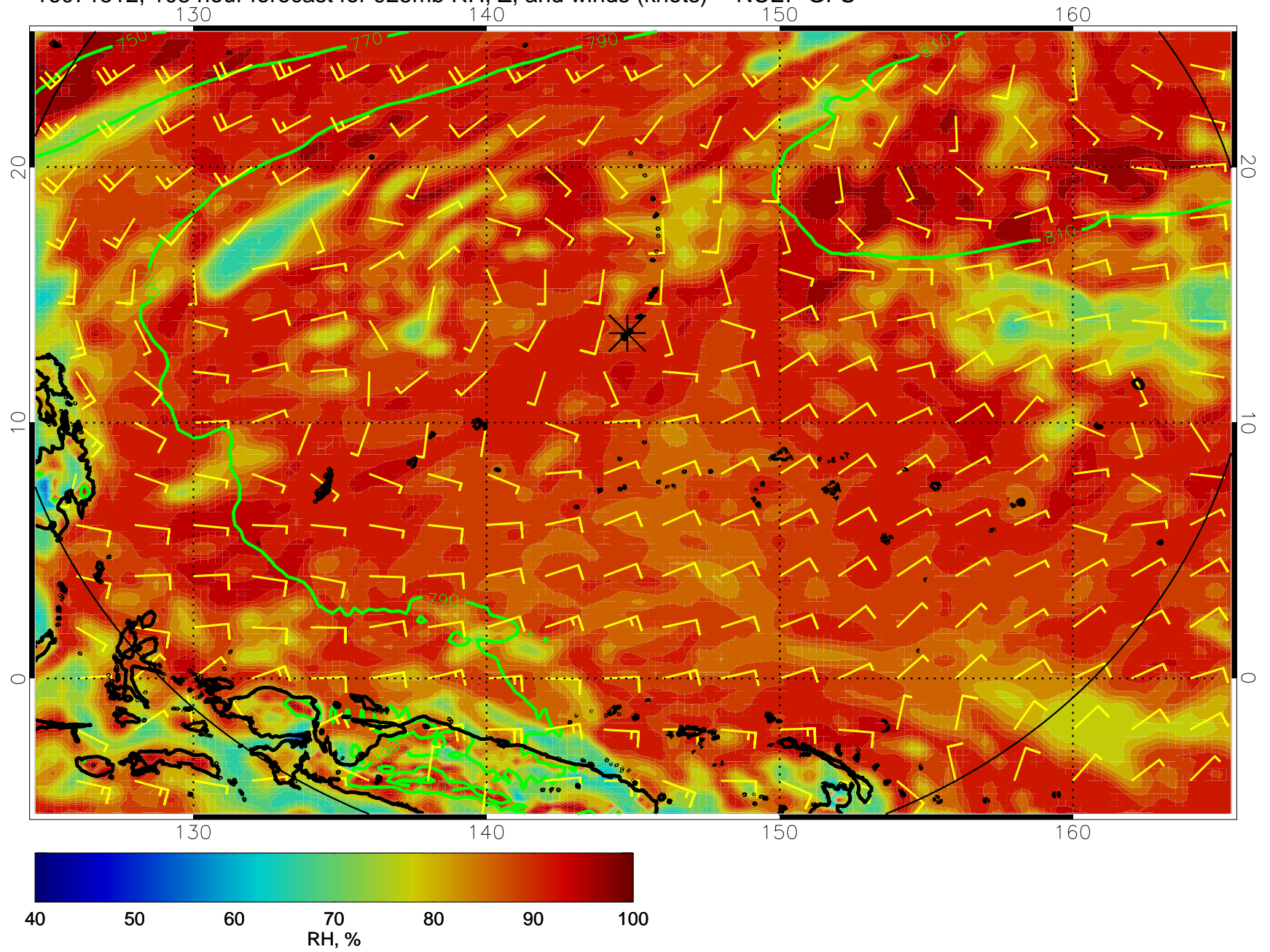
16071512, 108 hour forecast for 925mb RH, Z, and winds (knots) -- NCEP GFS
