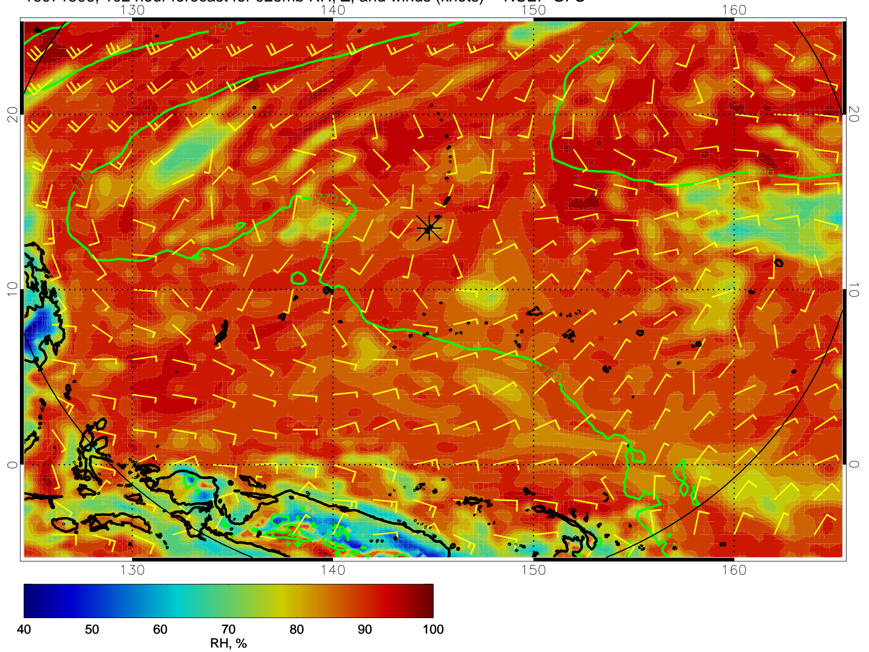
16071506, 102 hour forecast for 925mb RH, Z, and winds (knots) -- NCEP GFS
