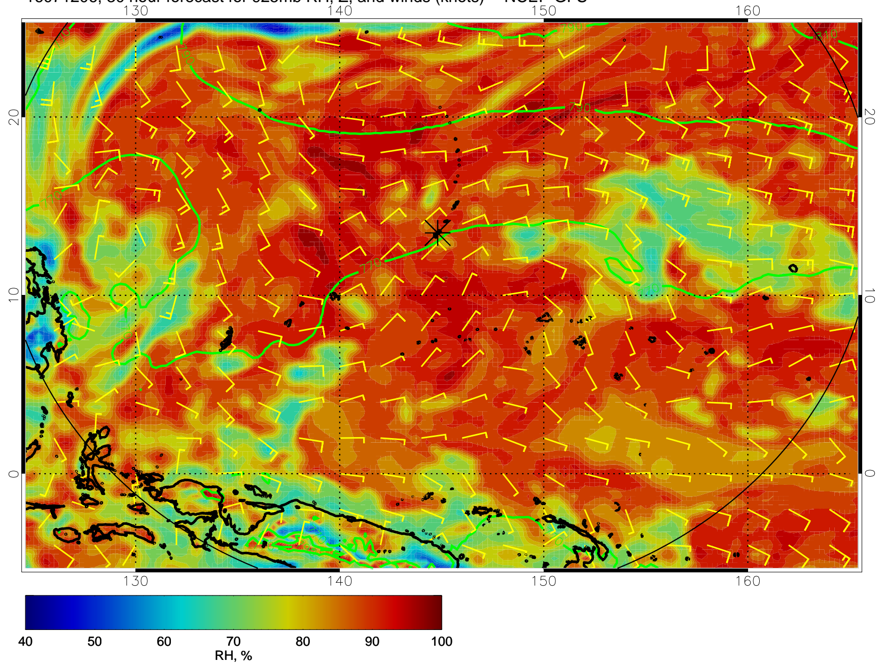
16071206, 30 hour forecast for 925mb RH, Z, and winds (knots) -- NCEP GFS
