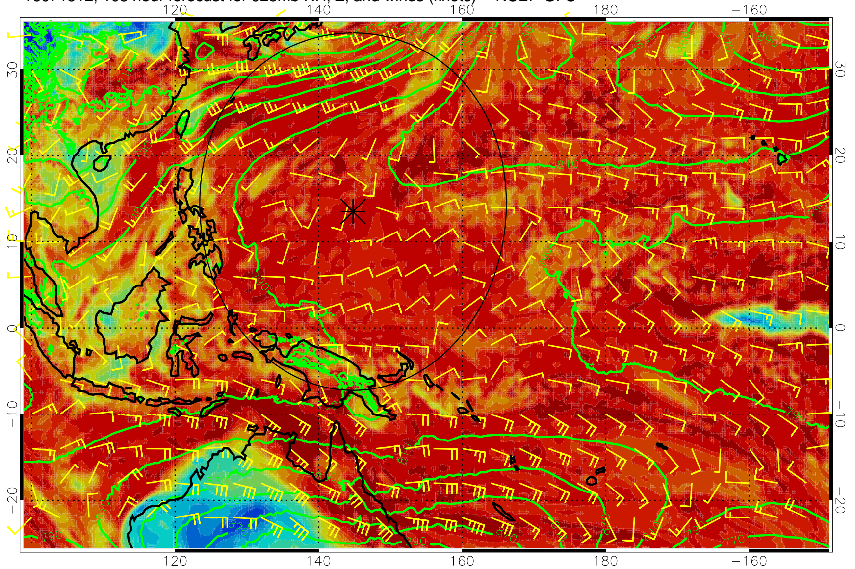
16071512, 108 hour forecast for 925mb RH, Z, and winds (knots) -- NCEP GFS
