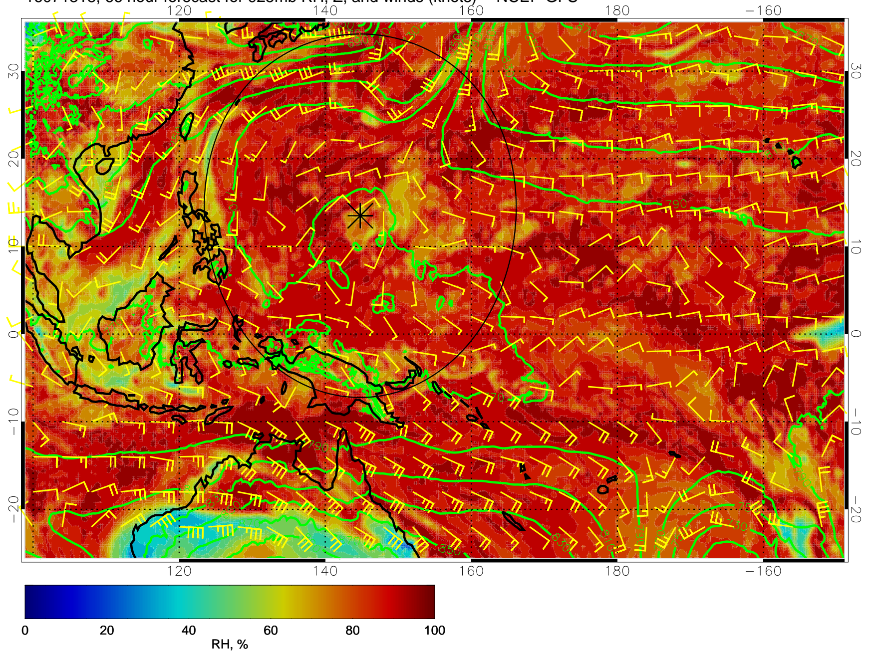
16071318, 66 hour forecast for 925mb RH, Z, and winds (knots) -- NCEP GFS
