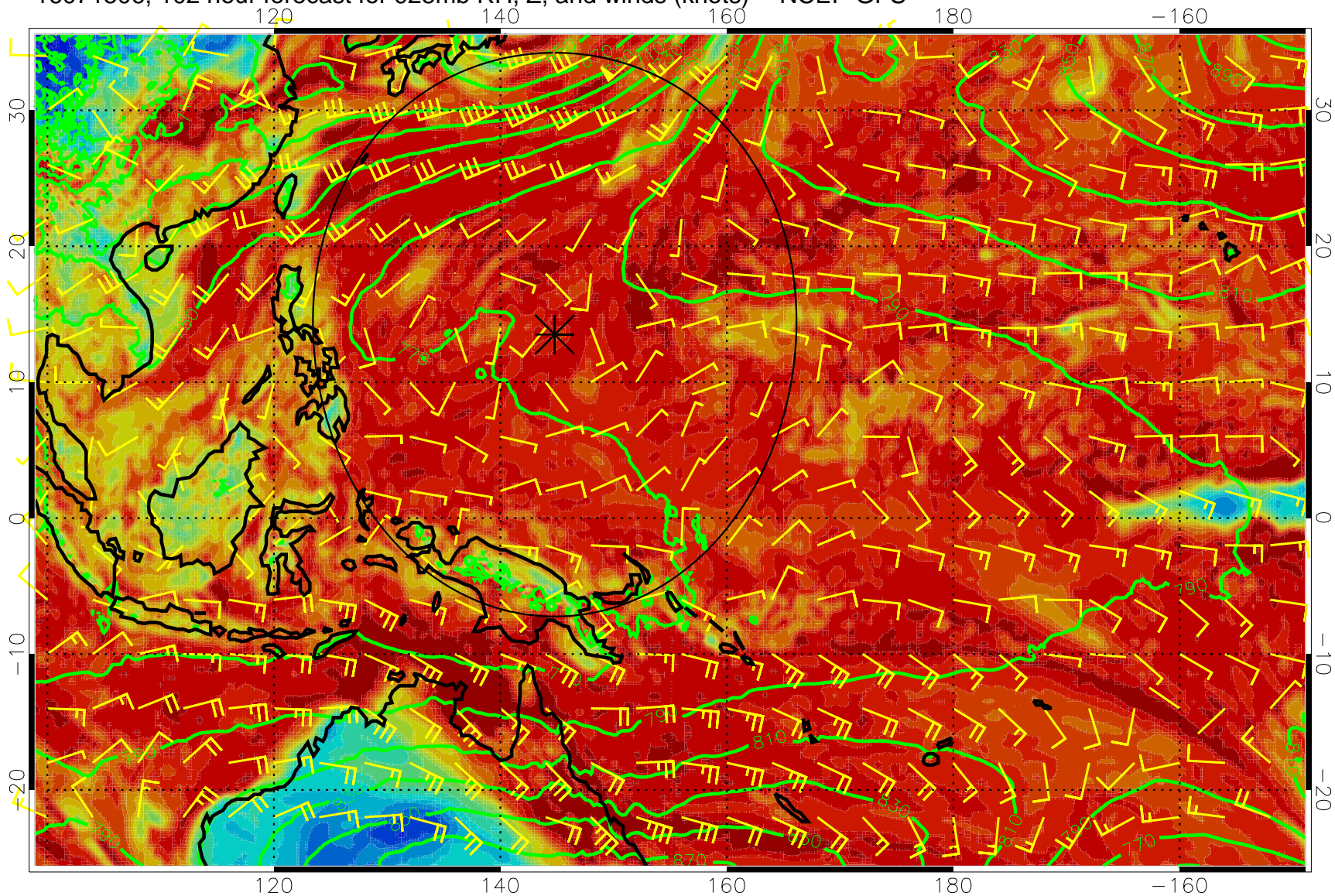
16071506, 102 hour forecast for 925mb RH, Z, and winds (knots) -- NCEP GFS
