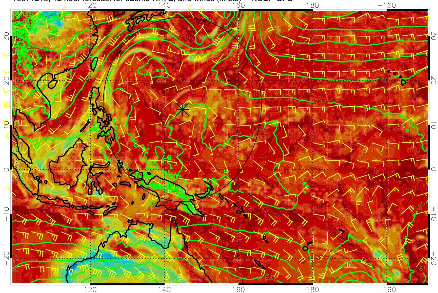
16071218, 42 hour forecast for 925mb RH, Z, and winds (knots) -- NCEP GFS
