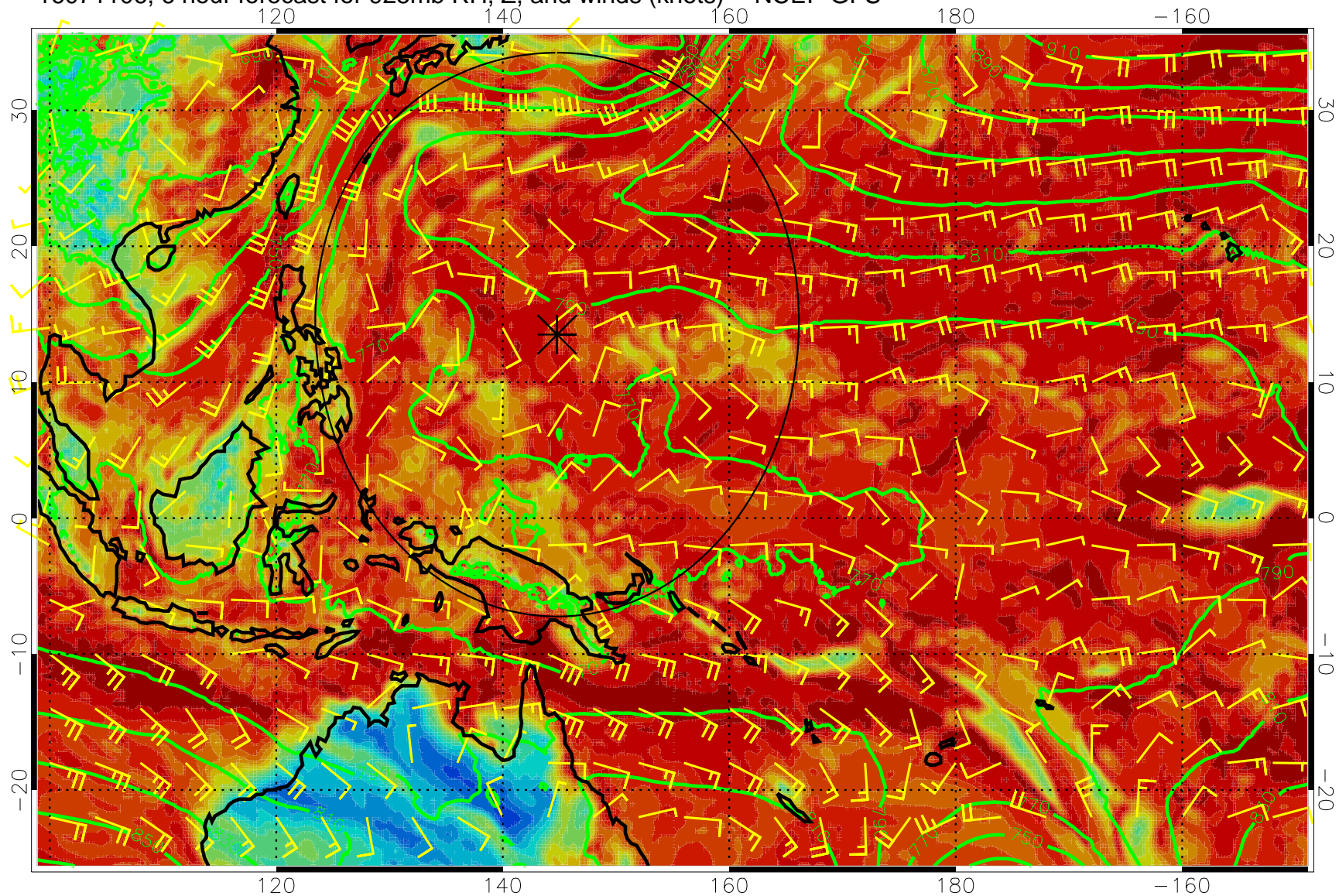
16071106, 6 hour forecast for 925mb RH, Z, and winds (knots) -- NCEP GFS
