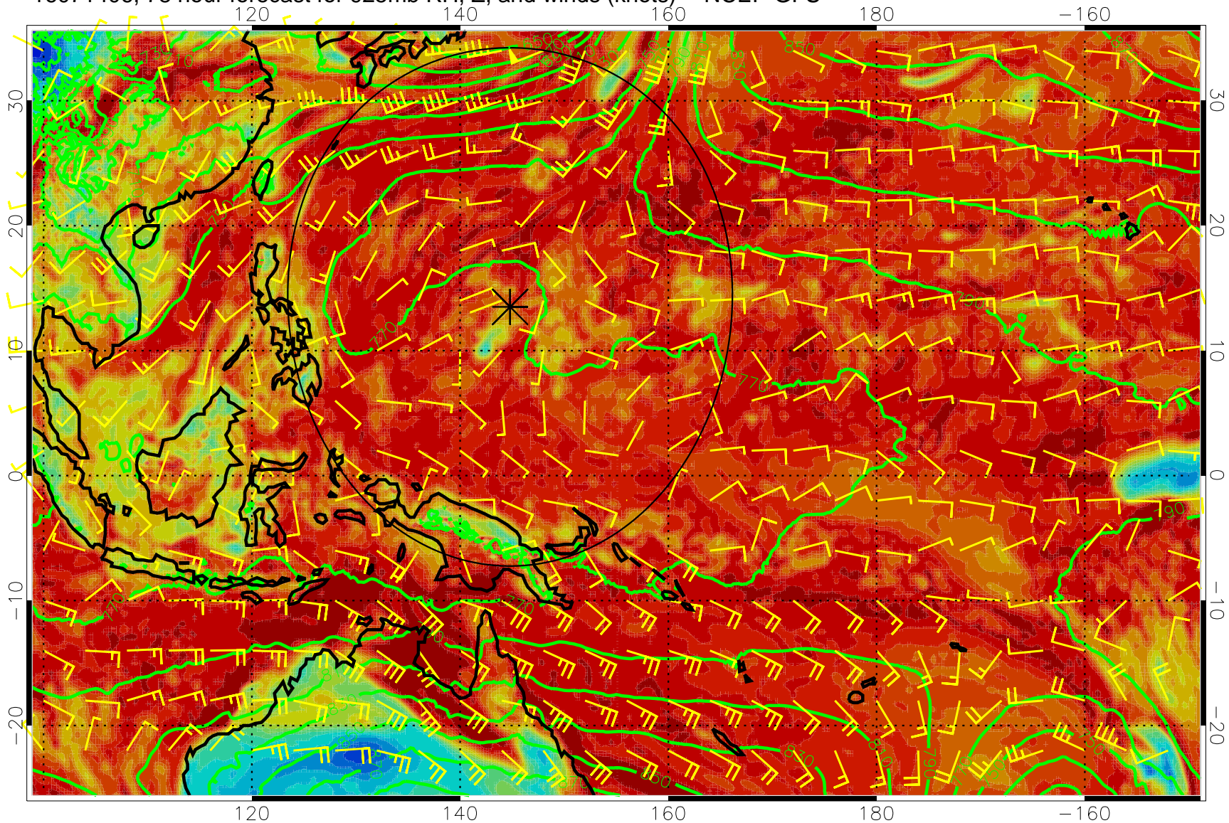
16071406, 78 hour forecast for 925mb RH, Z, and winds (knots) -- NCEP GFS
