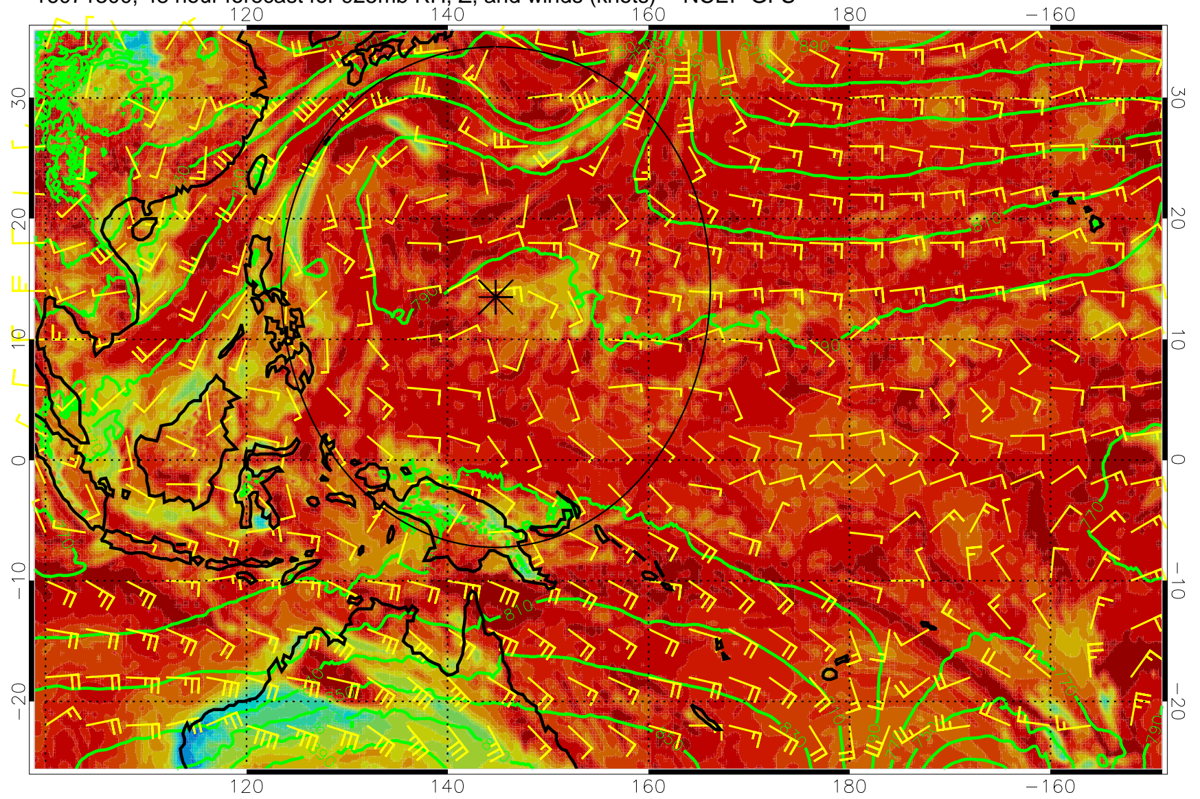
16071300, 48 hour forecast for 925mb RH, Z, and winds (knots) -- NCEP GFS
