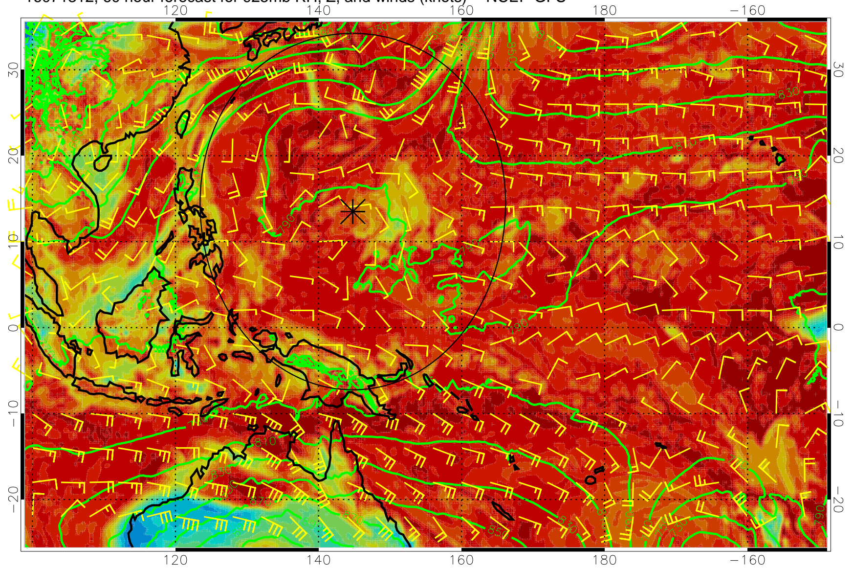
16071312, 60 hour forecast for 925mb RH, Z, and winds (knots) -- NCEP GFS
