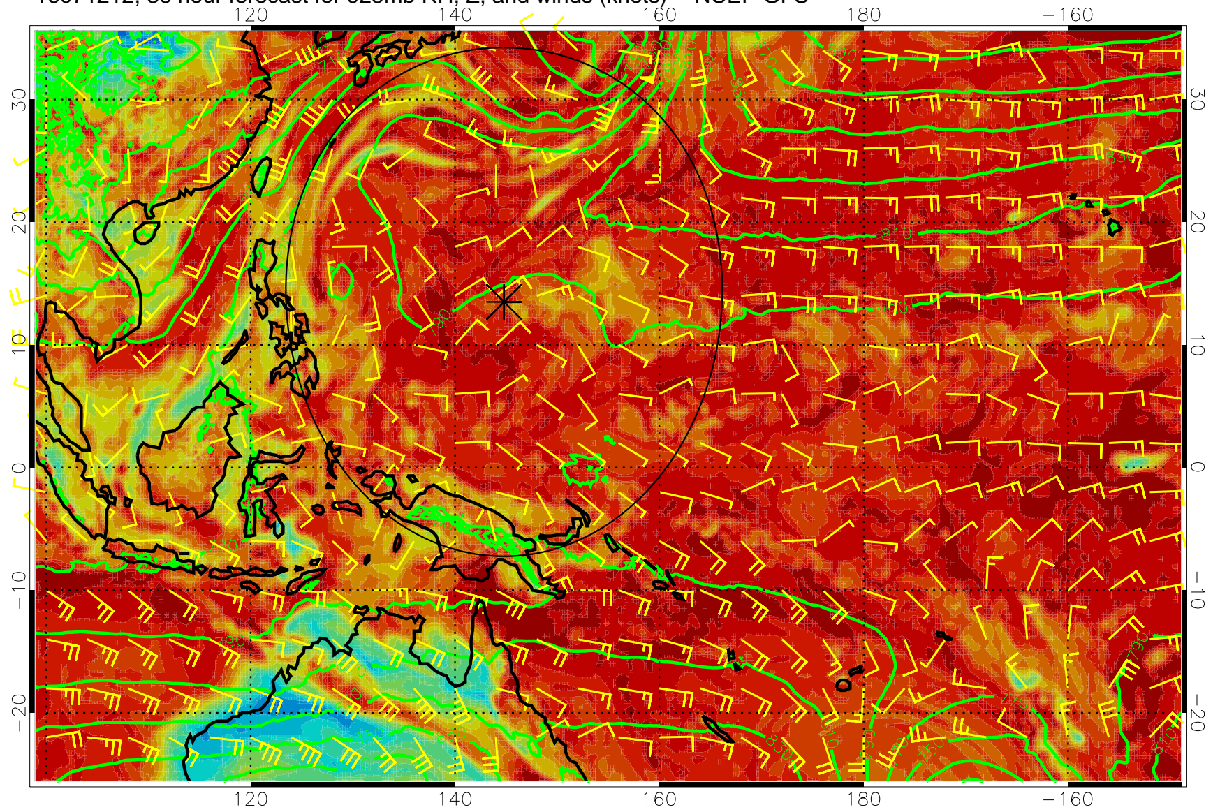
16071212, 36 hour forecast for 925mb RH, Z, and winds (knots) -- NCEP GFS
