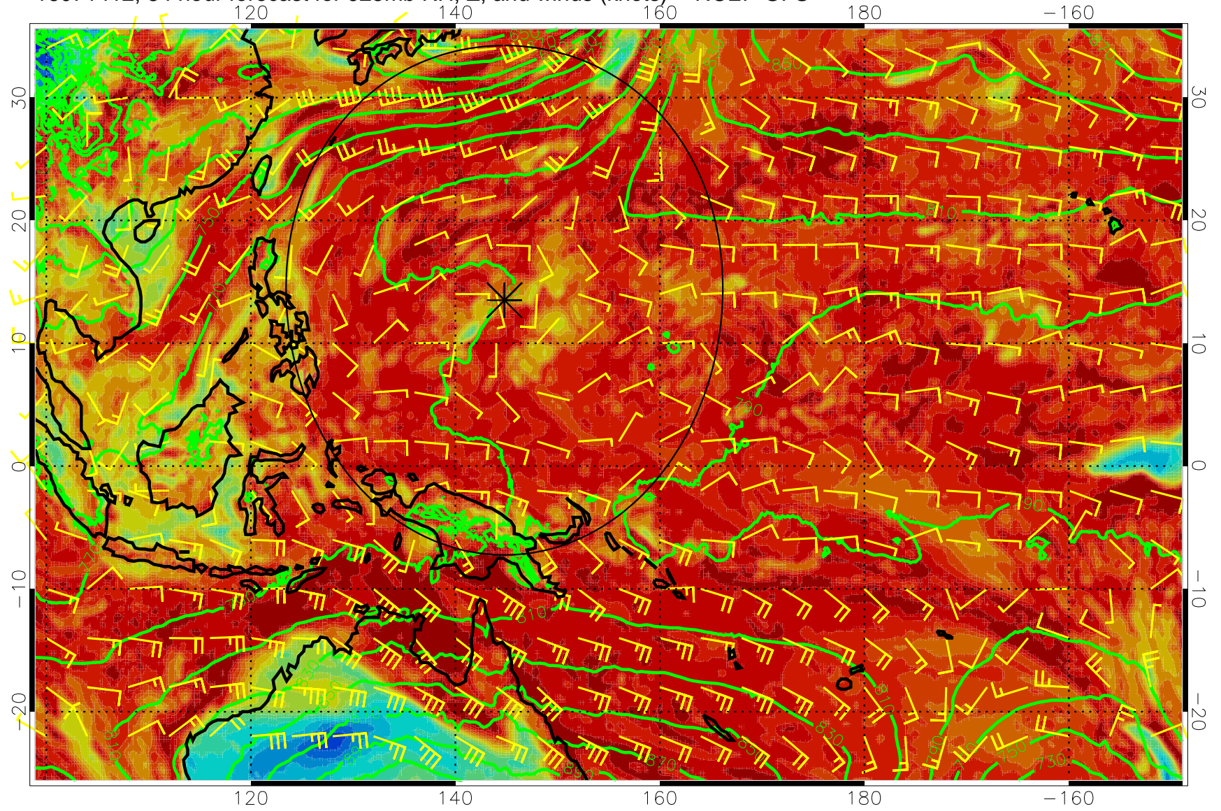
16071412, 84 hour forecast for 925mb RH, Z, and winds (knots) -- NCEP GFS
