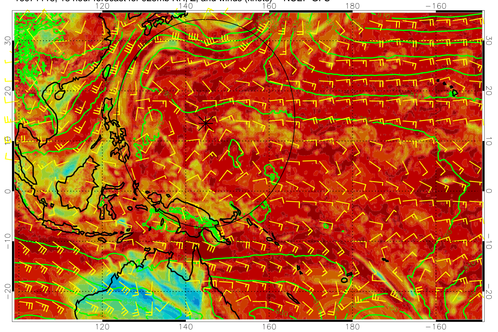
16071118, 18 hour forecast for 925mb RH, Z, and winds (knots) -- NCEP GFS
