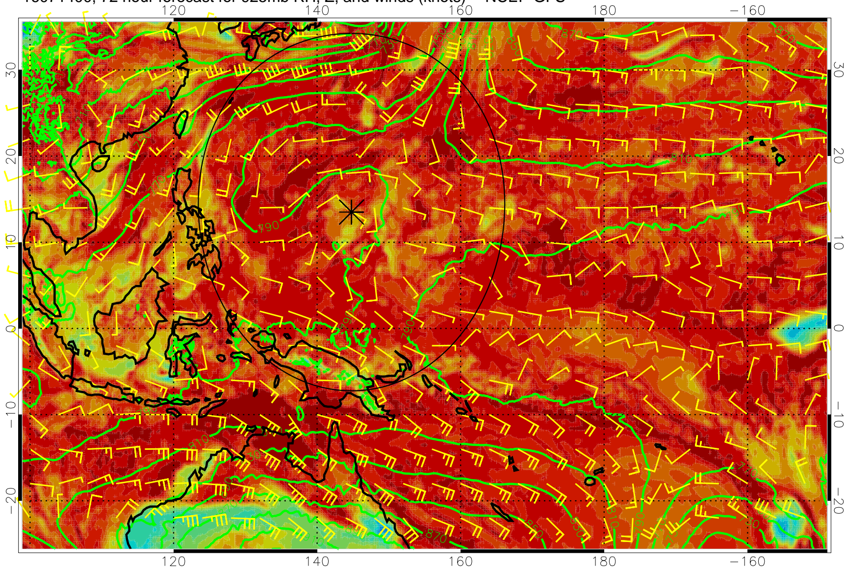
16071400, 72 hour forecast for 925mb RH, Z, and winds (knots) -- NCEP GFS
