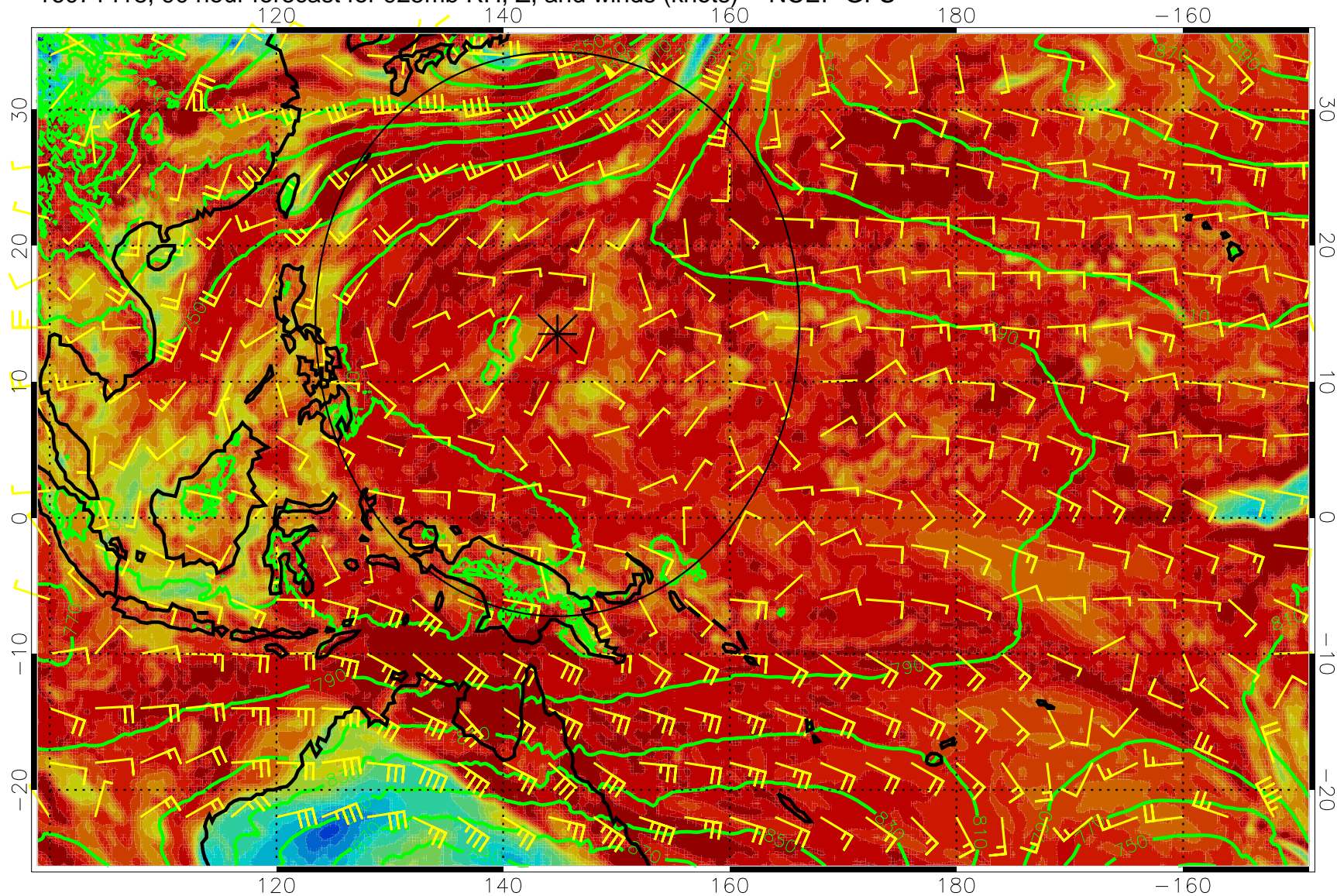
16071418, 90 hour forecast for 925mb RH, Z, and winds (knots) -- NCEP GFS
