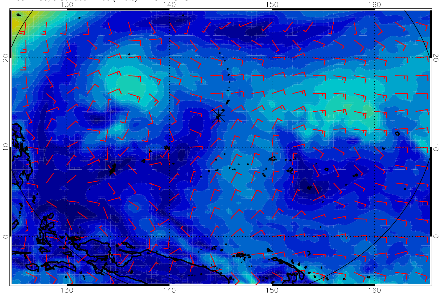
16071106, 6 Surface winds (knots) -- NCEP GFS
