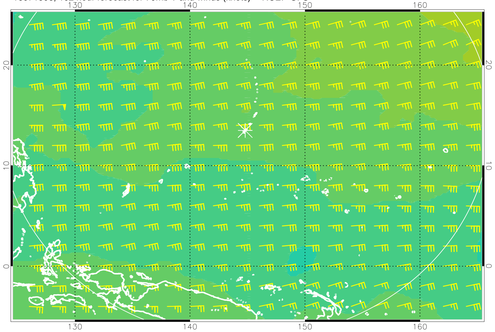
16071506, 102 hour forecast for 70mb T and winds (knots) -- NCEP GFS
