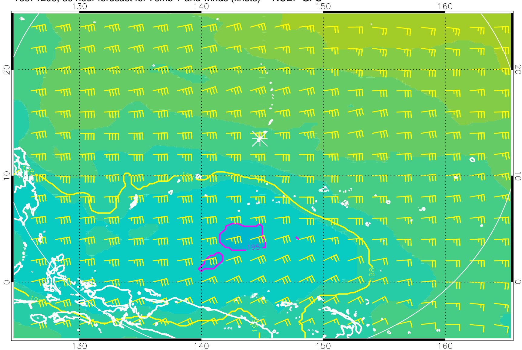
16071206, 30 hour forecast for 70mb T and winds (knots) -- NCEP GFS
