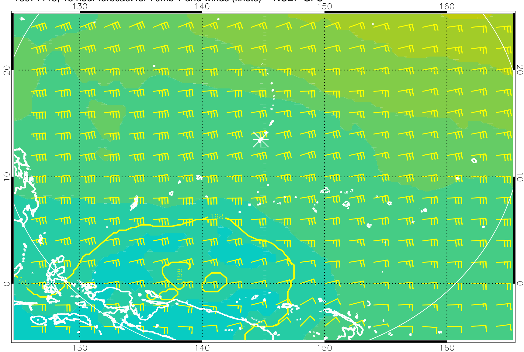
16071118, 18 hour forecast for 70mb T and winds (knots) -- NCEP GFS
