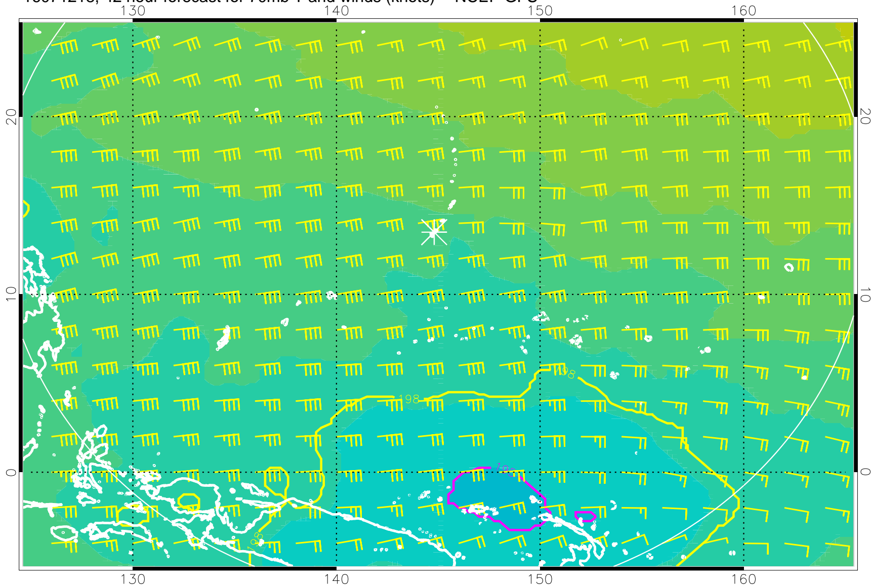
16071218, 42 hour forecast for 70mb T and winds (knots) -- NCEP GFS
