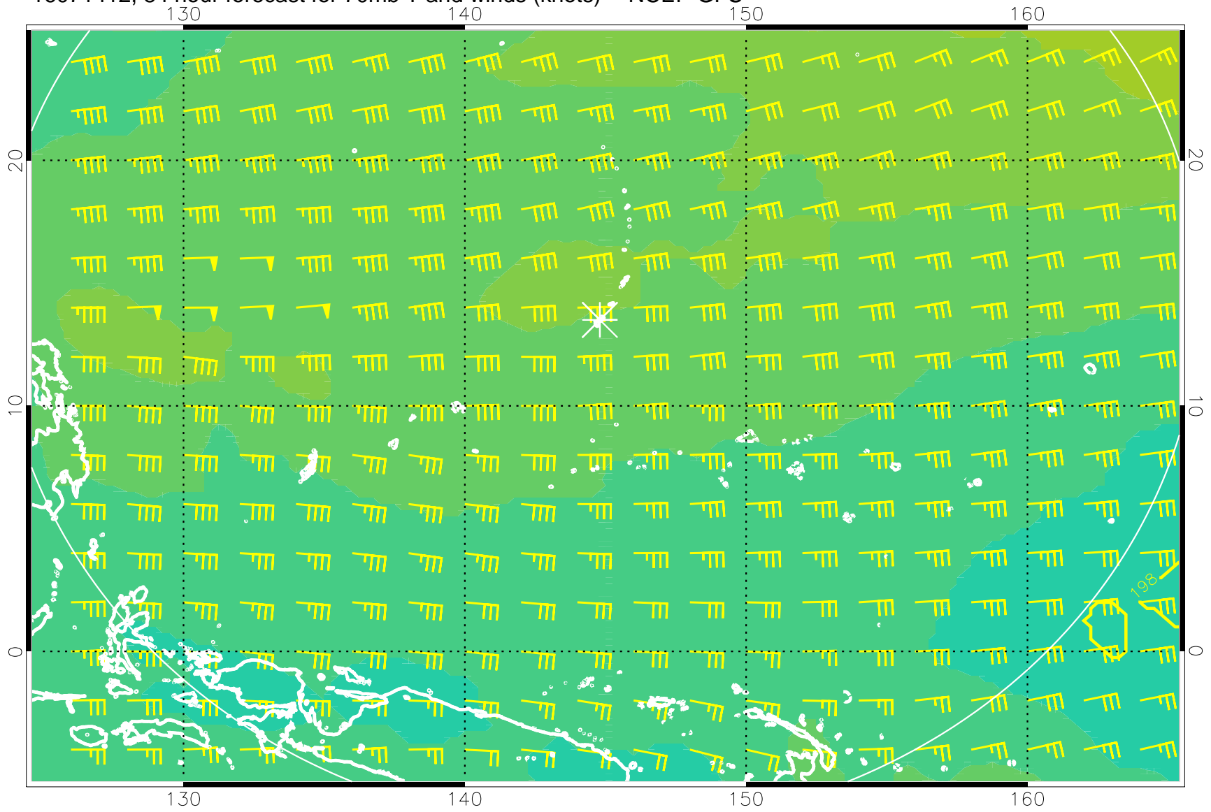
16071412, 84 hour forecast for 70mb T and winds (knots) -- NCEP GFS
