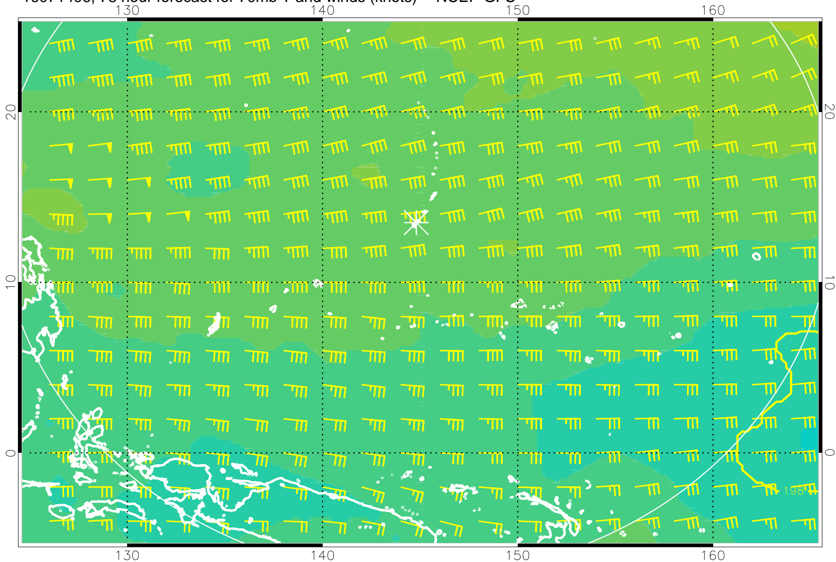
16071406, 78 hour forecast for 70mb T and winds (knots) -- NCEP GFS
