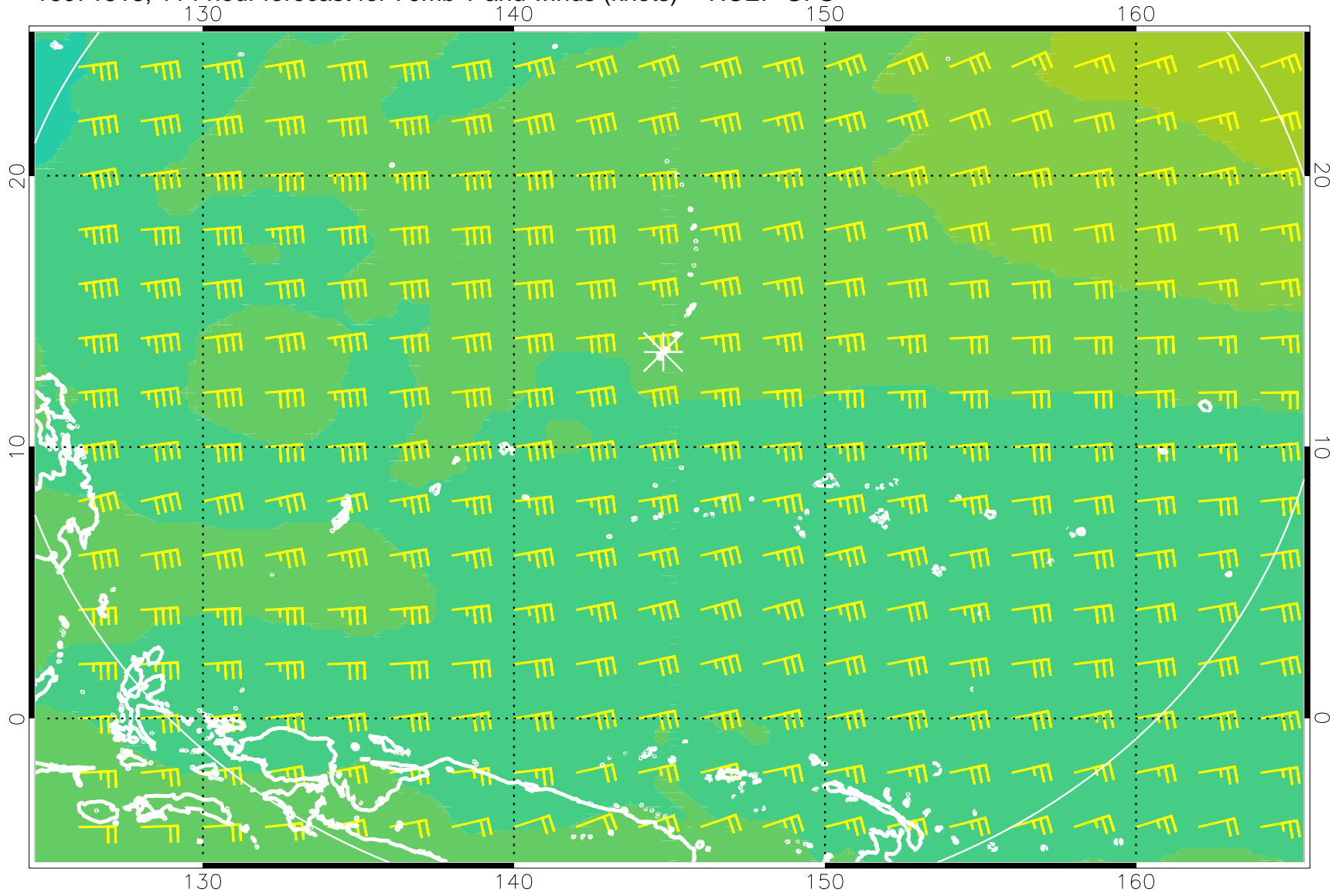
16071518, 114 hour forecast for 70mb T and winds (knots) -- NCEP GFS
