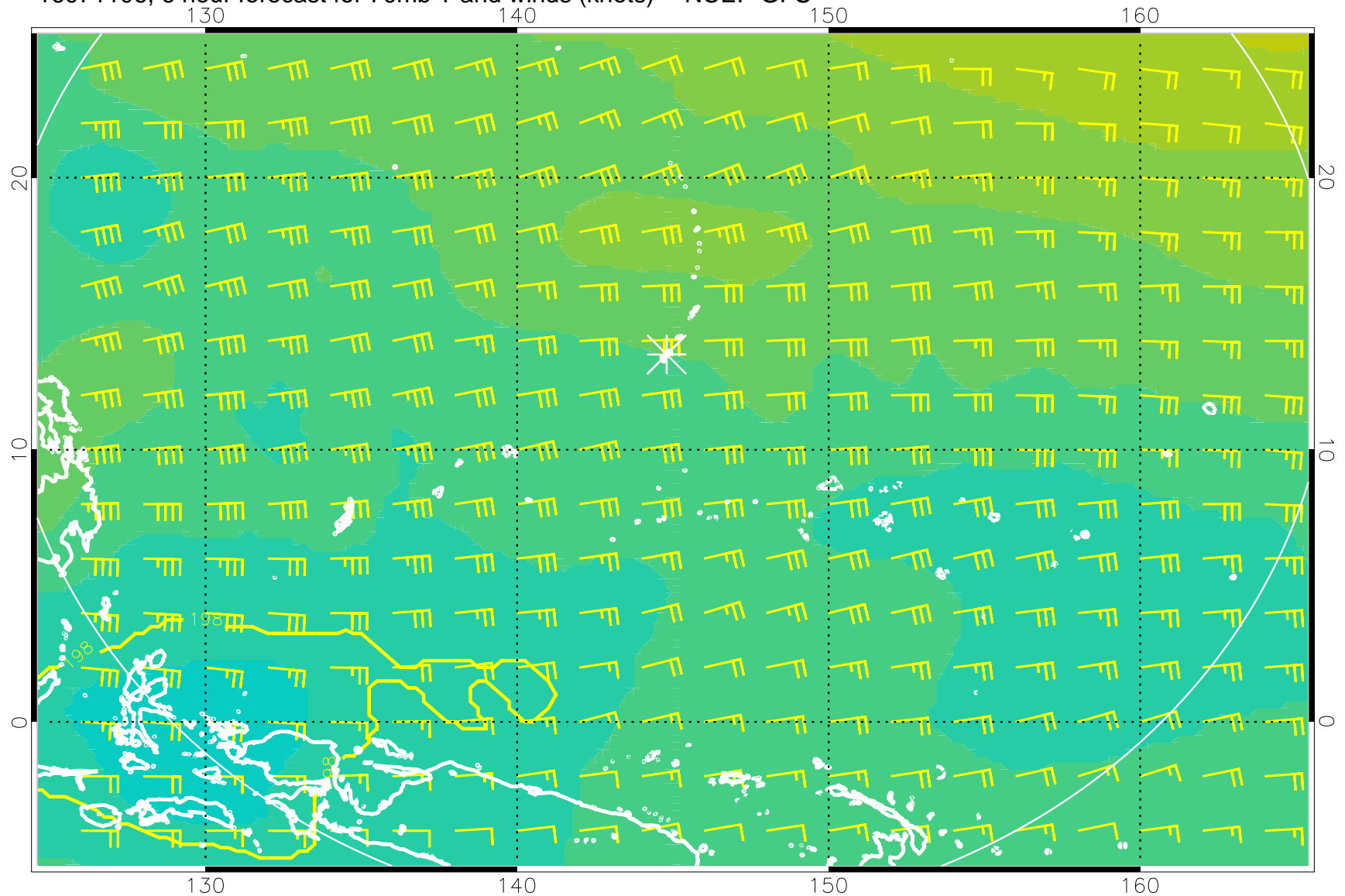
16071106, 6 hour forecast for 70mb T and winds (knots) -- NCEP GFS
