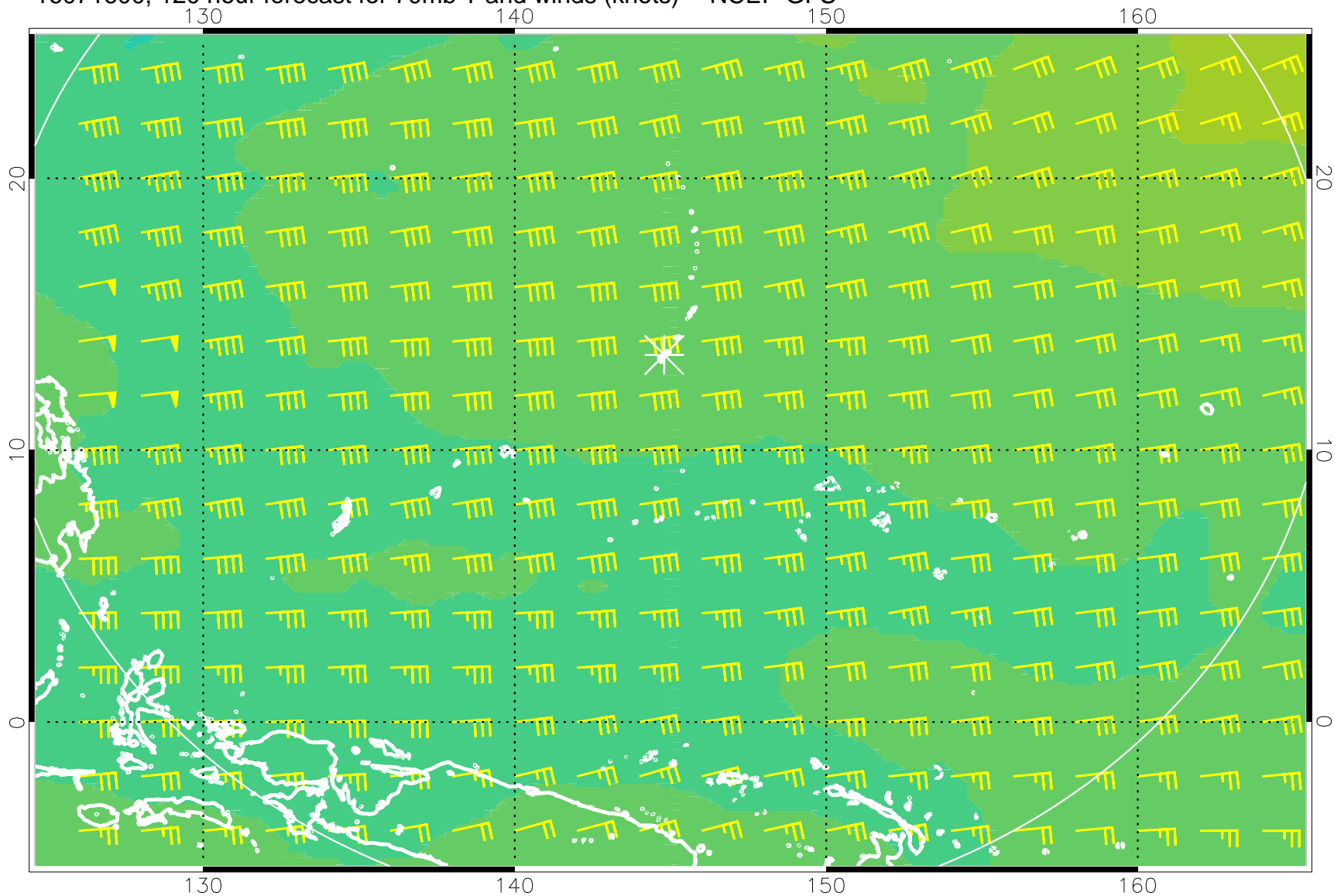
16071600, 120 hour forecast for 70mb T and winds (knots) -- NCEP GFS
