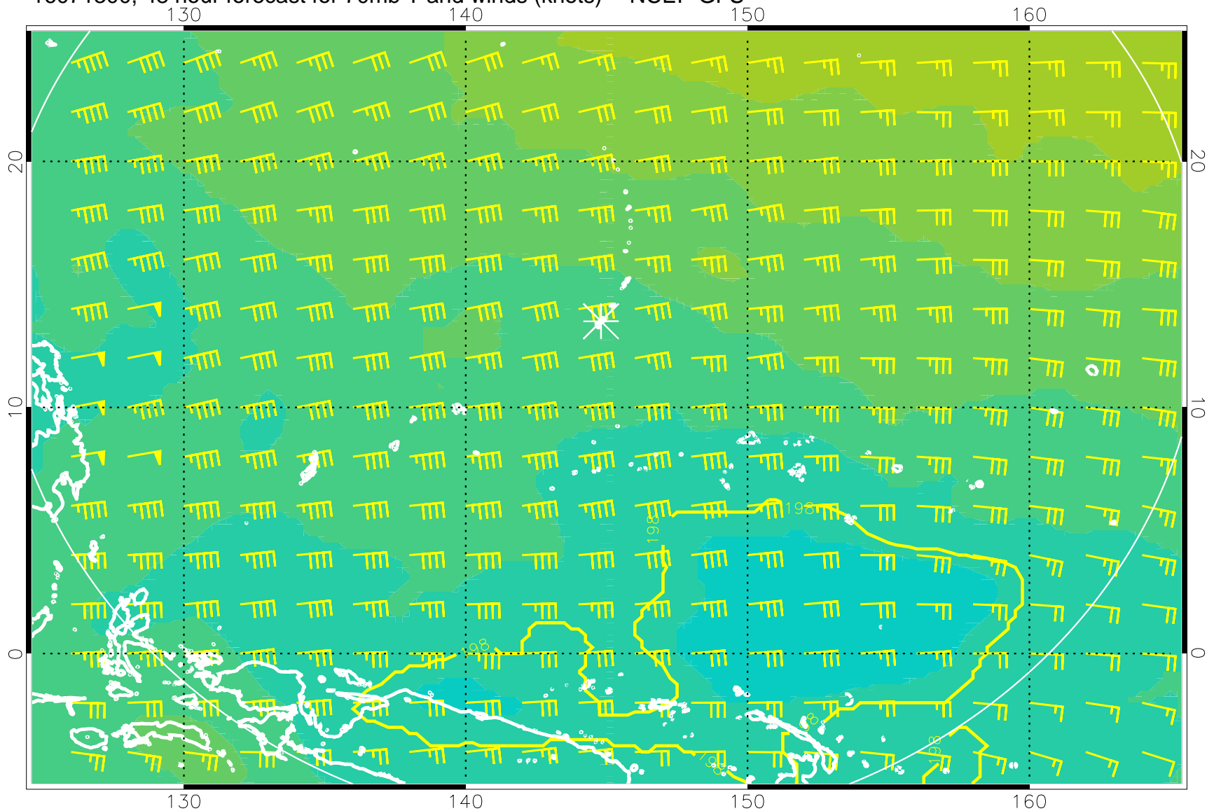
16071300, 48 hour forecast for 70mb T and winds (knots) -- NCEP GFS
