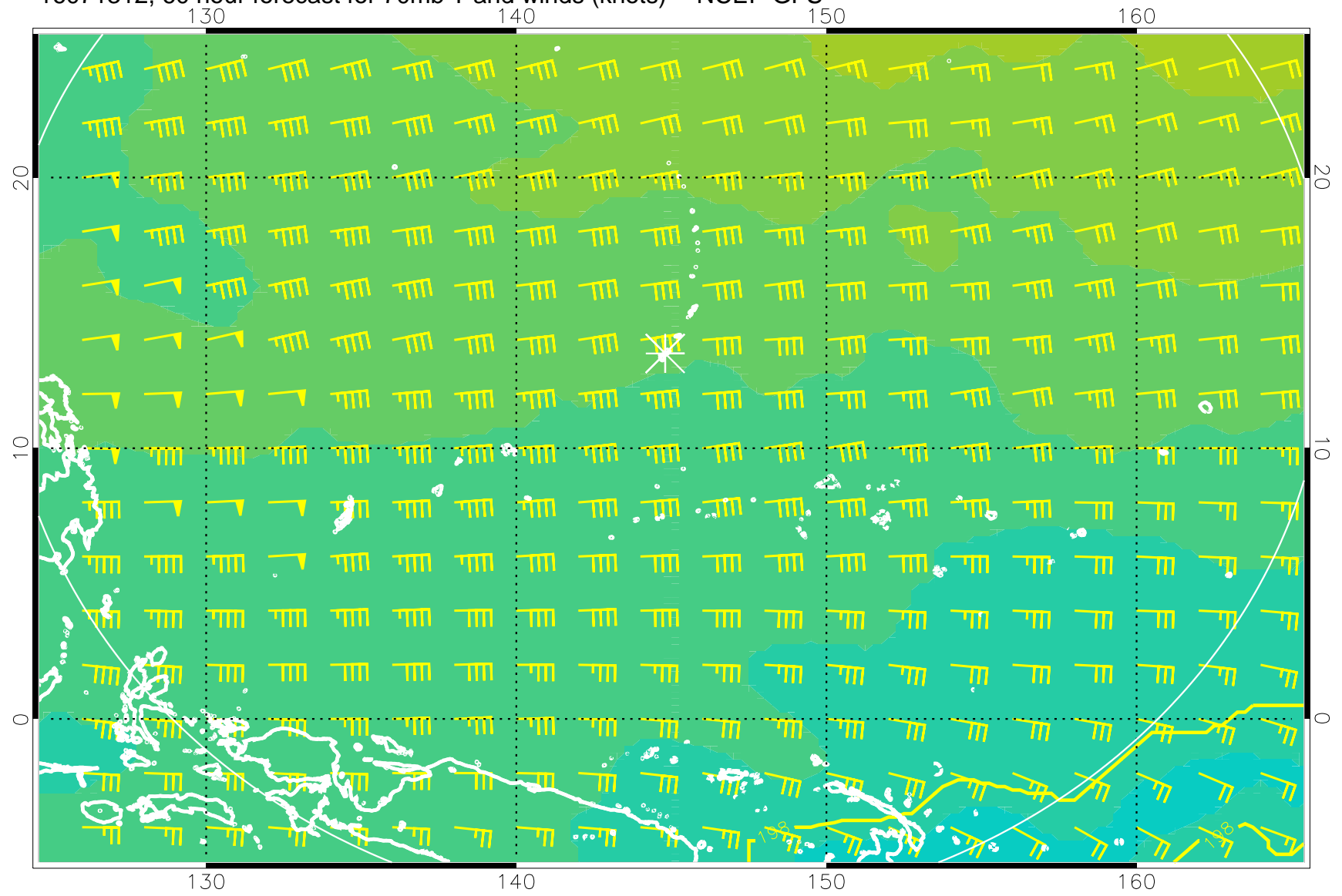
16071312, 60 hour forecast for 70mb T and winds (knots) -- NCEP GFS
