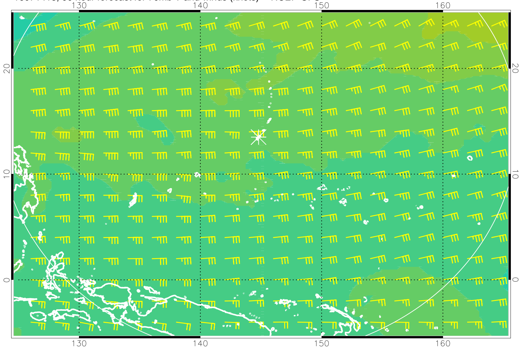
16071418, 90 hour forecast for 70mb T and winds (knots) -- NCEP GFS
