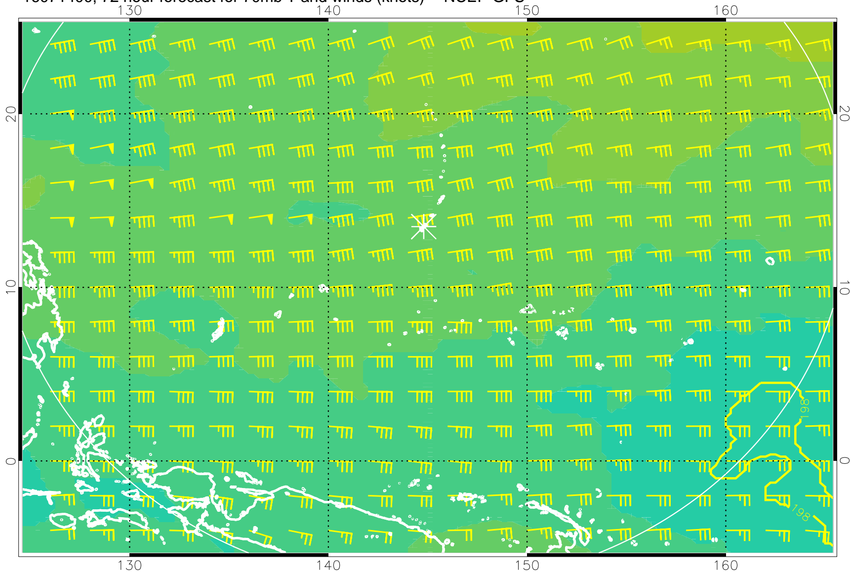
16071400, 72 hour forecast for 70mb T and winds (knots) -- NCEP GFS
