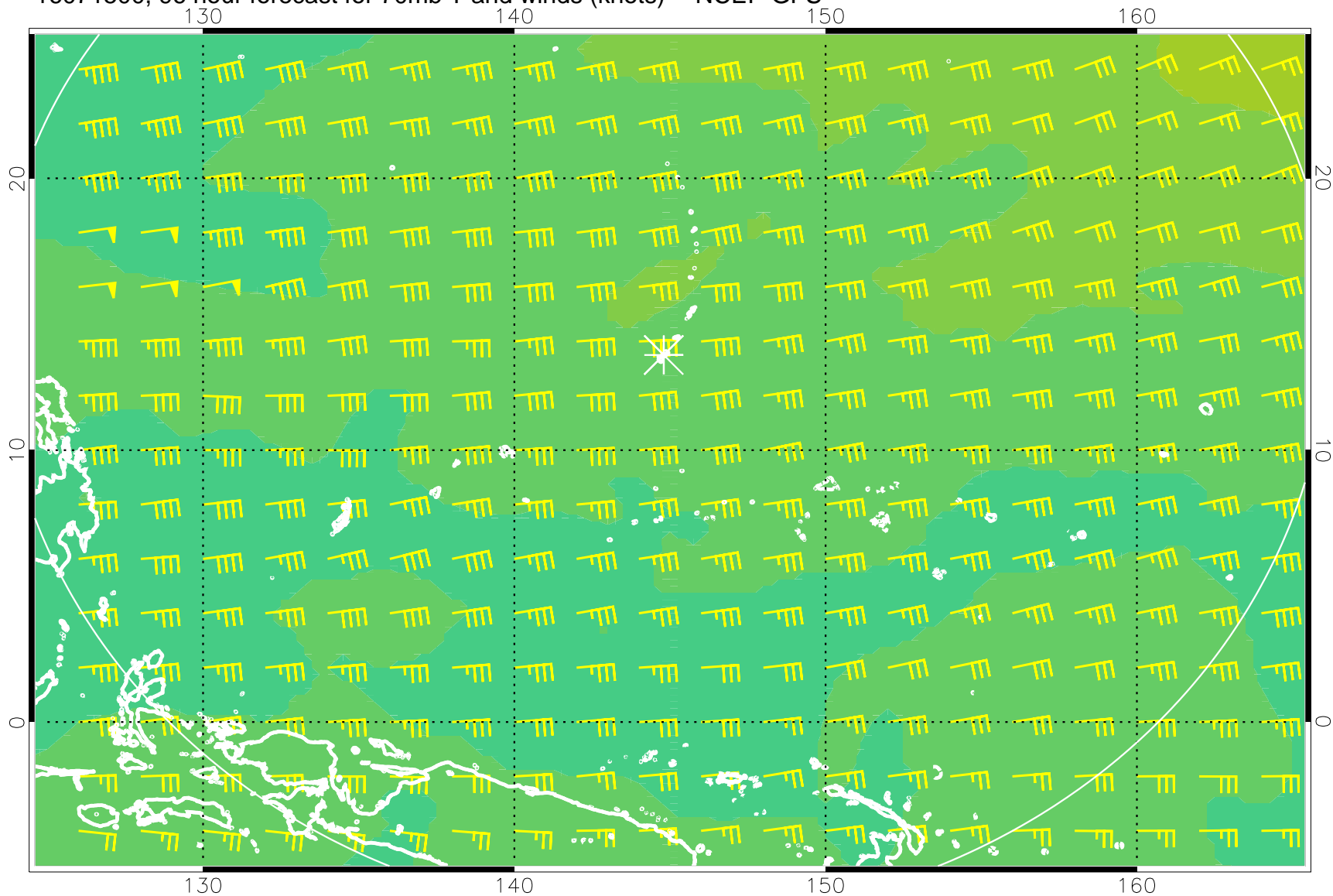
16071500, 96 hour forecast for 70mb T and winds (knots) -- NCEP GFS
