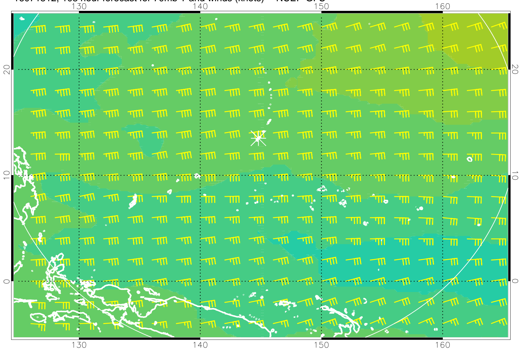
16071512, 108 hour forecast for 70mb T and winds (knots) -- NCEP GFS
