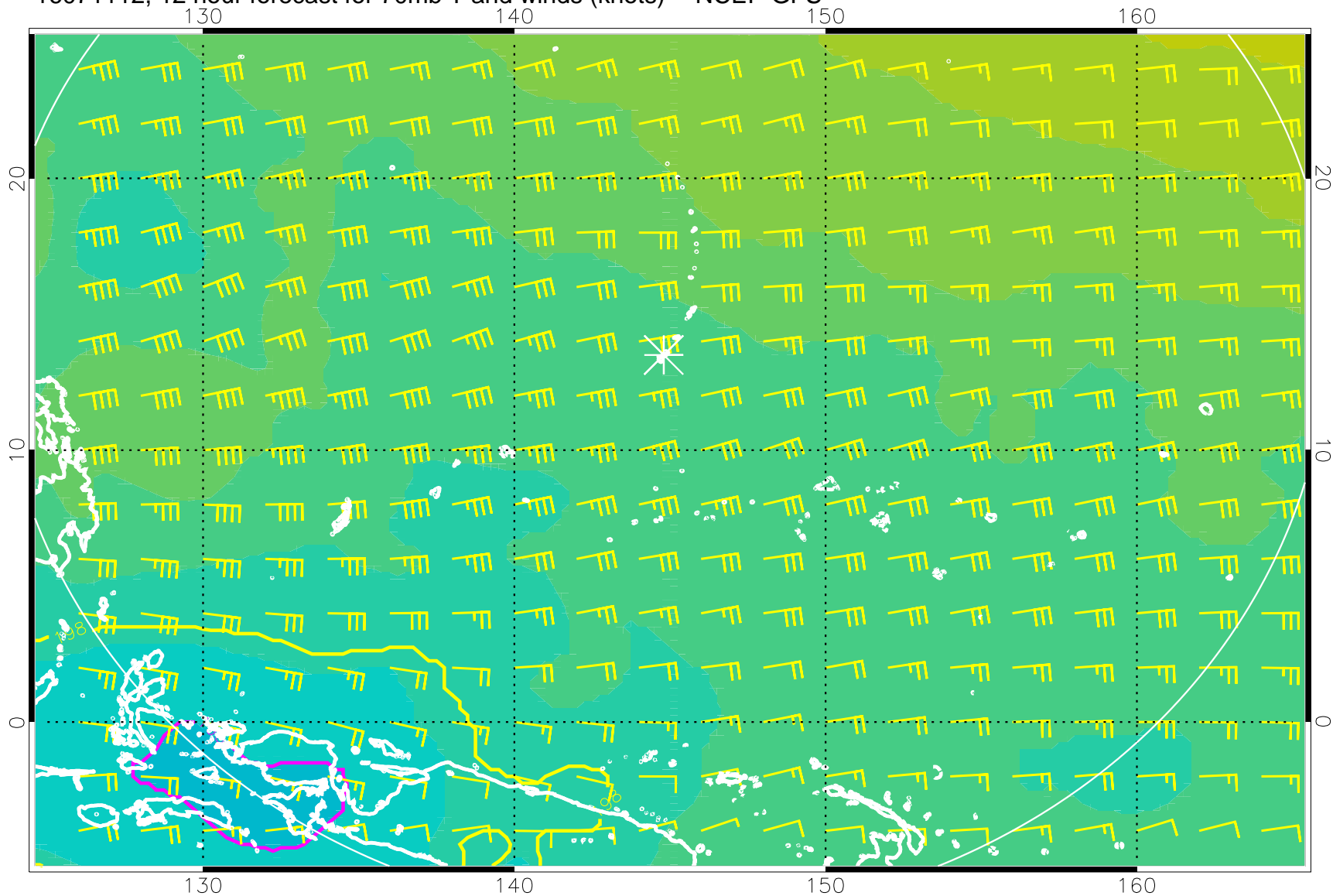
16071112, 12 hour forecast for 70mb T and winds (knots) -- NCEP GFS
