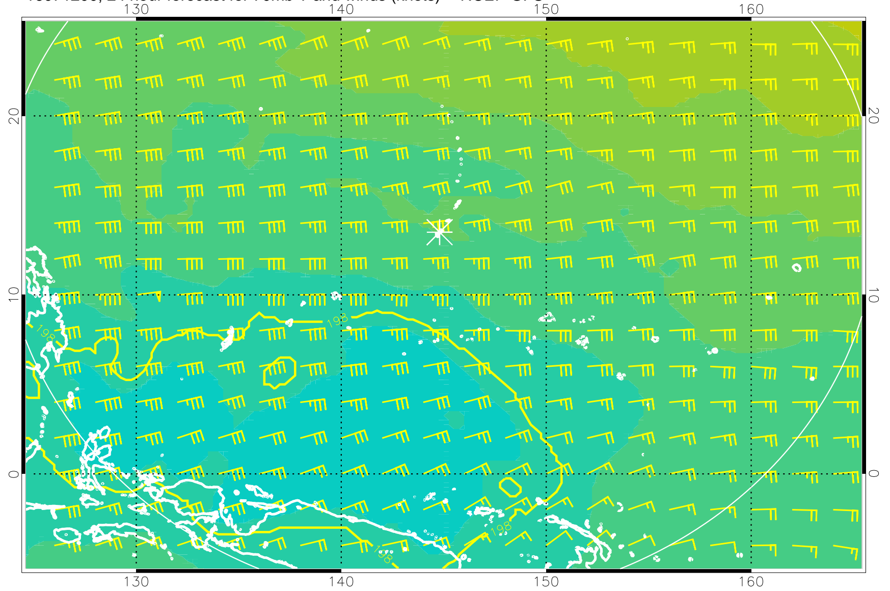
16071200, 24 hour forecast for 70mb T and winds (knots) -- NCEP GFS
