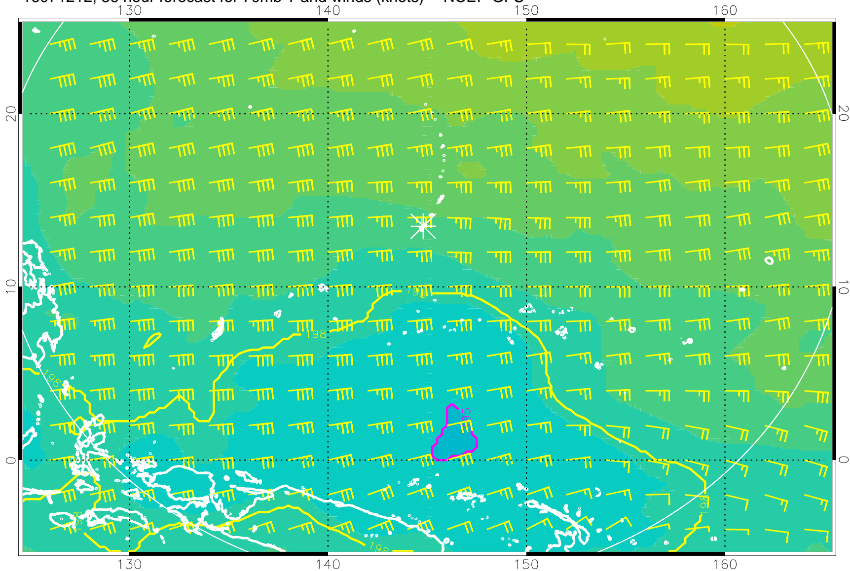
16071212, 36 hour forecast for 70mb T and winds (knots) -- NCEP GFS
