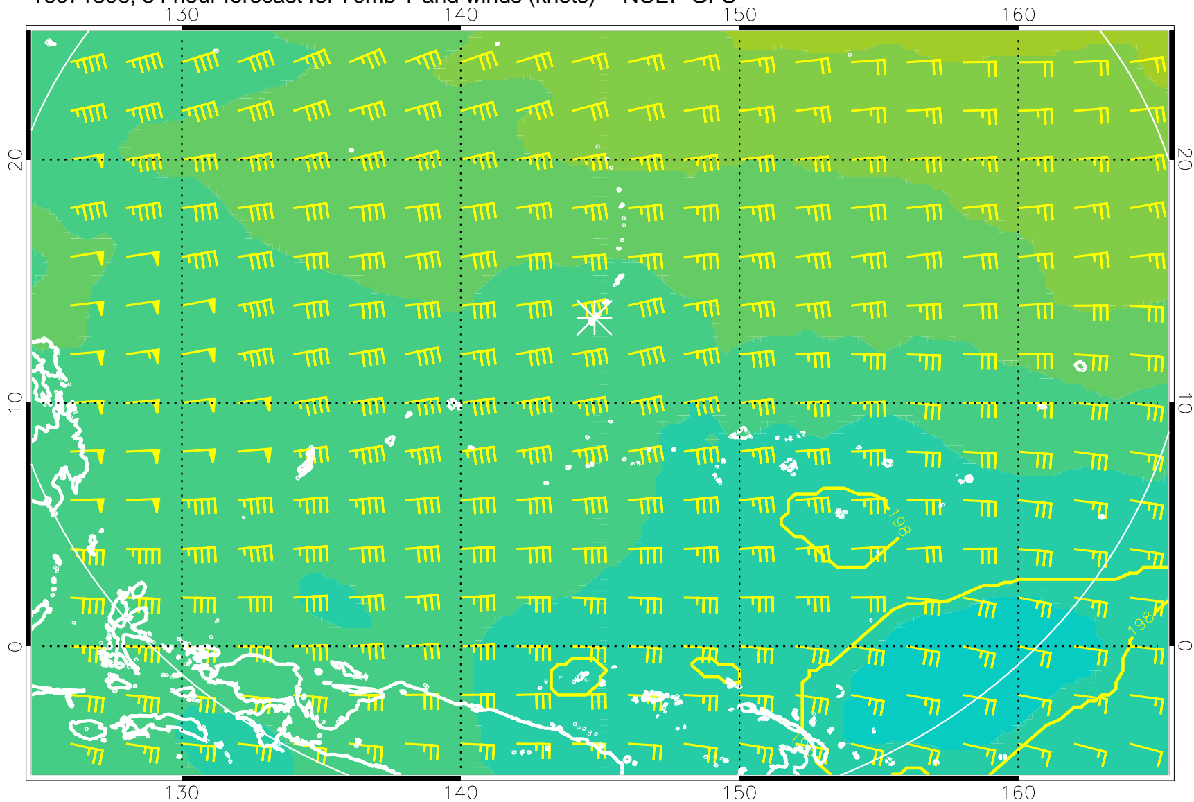
16071306, 54 hour forecast for 70mb T and winds (knots) -- NCEP GFS
