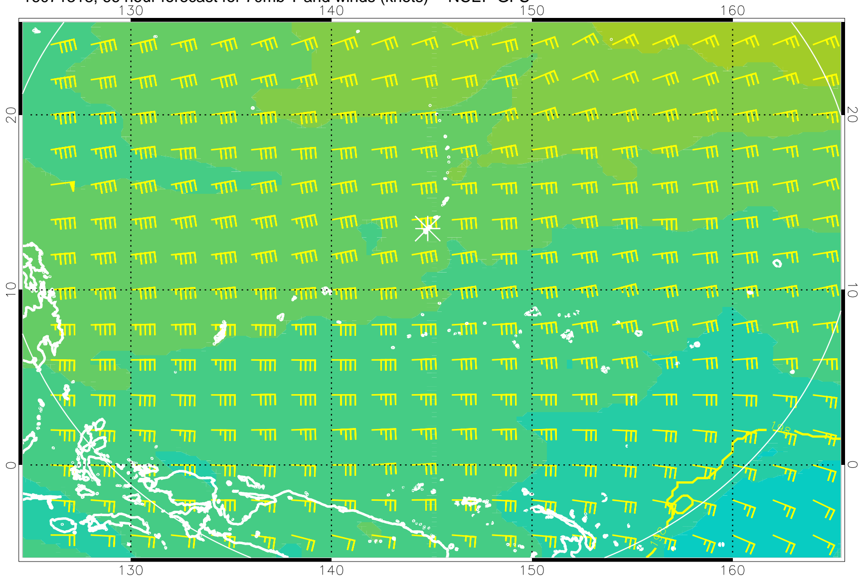
16071318, 66 hour forecast for 70mb T and winds (knots) -- NCEP GFS
