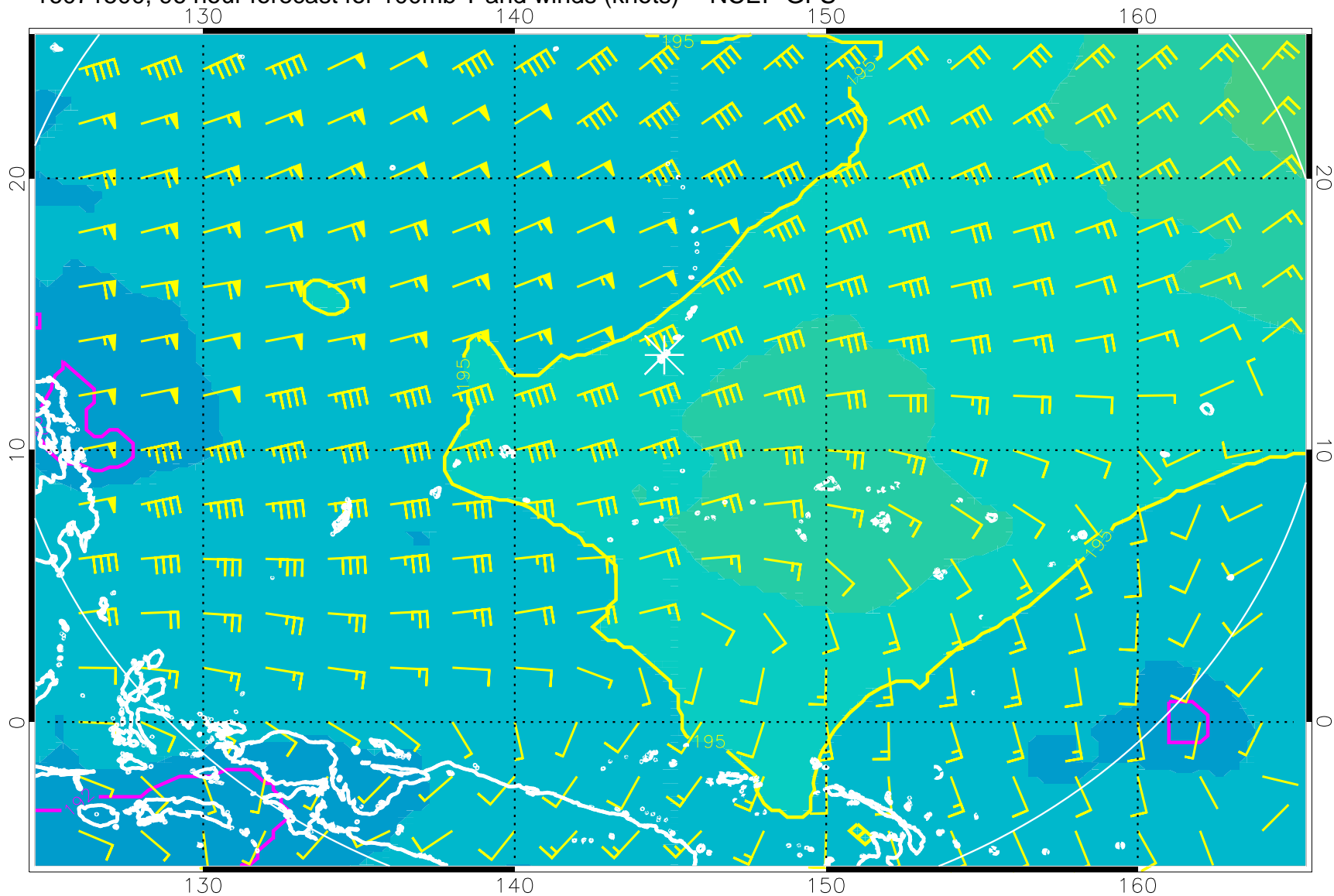
16071500, 96 hour forecast for 100mb T and winds (knots) -- NCEP GFS
