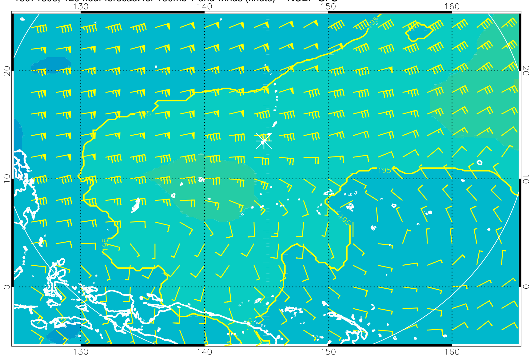
16071600, 120 hour forecast for 100mb T and winds (knots) -- NCEP GFS
