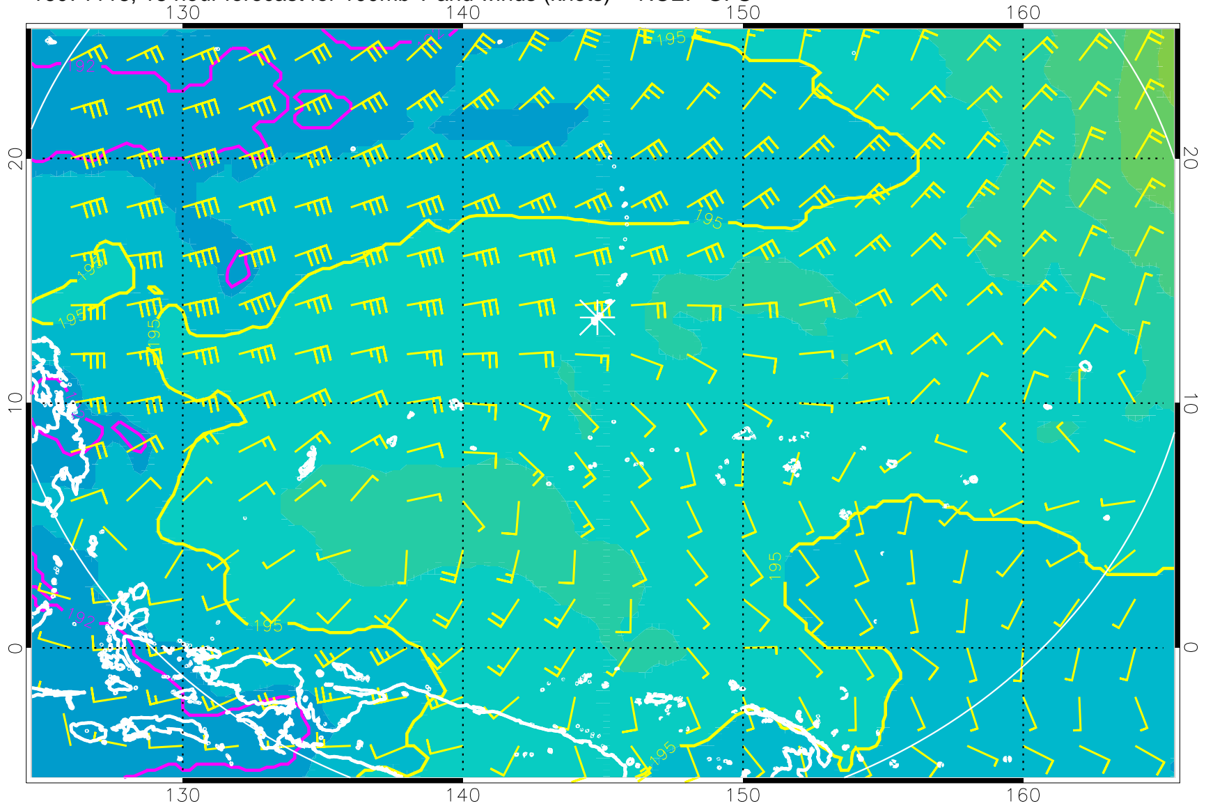
16071118, 18 hour forecast for 100mb T and winds (knots) -- NCEP GFS
