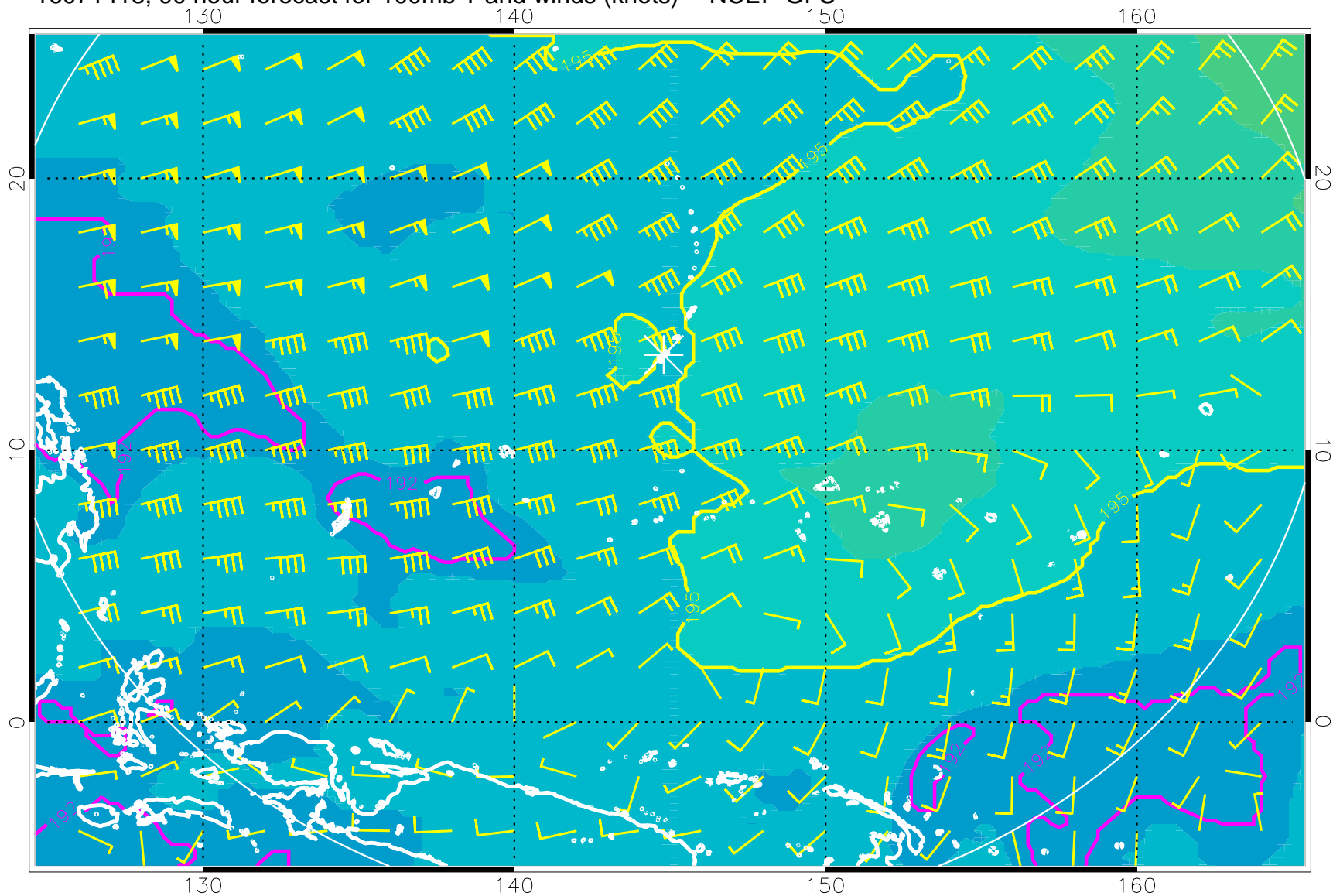
16071418, 90 hour forecast for 100mb T and winds (knots) -- NCEP GFS
