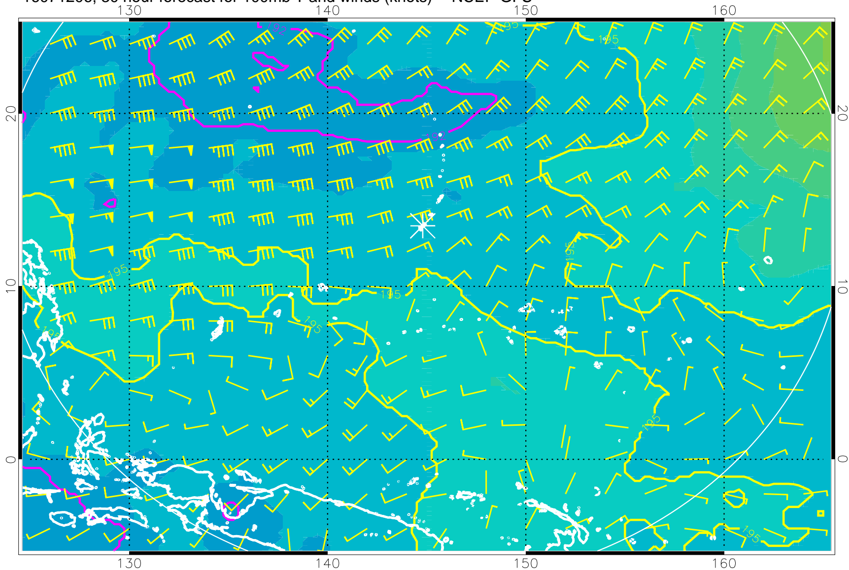
16071206, 30 hour forecast for 100mb T and winds (knots) -- NCEP GFS
