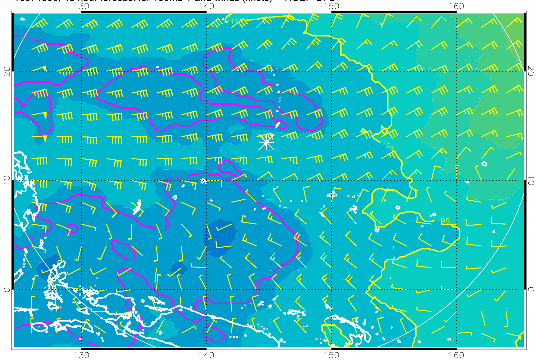
16071300, 48 hour forecast for 100mb T and winds (knots) -- NCEP GFS
