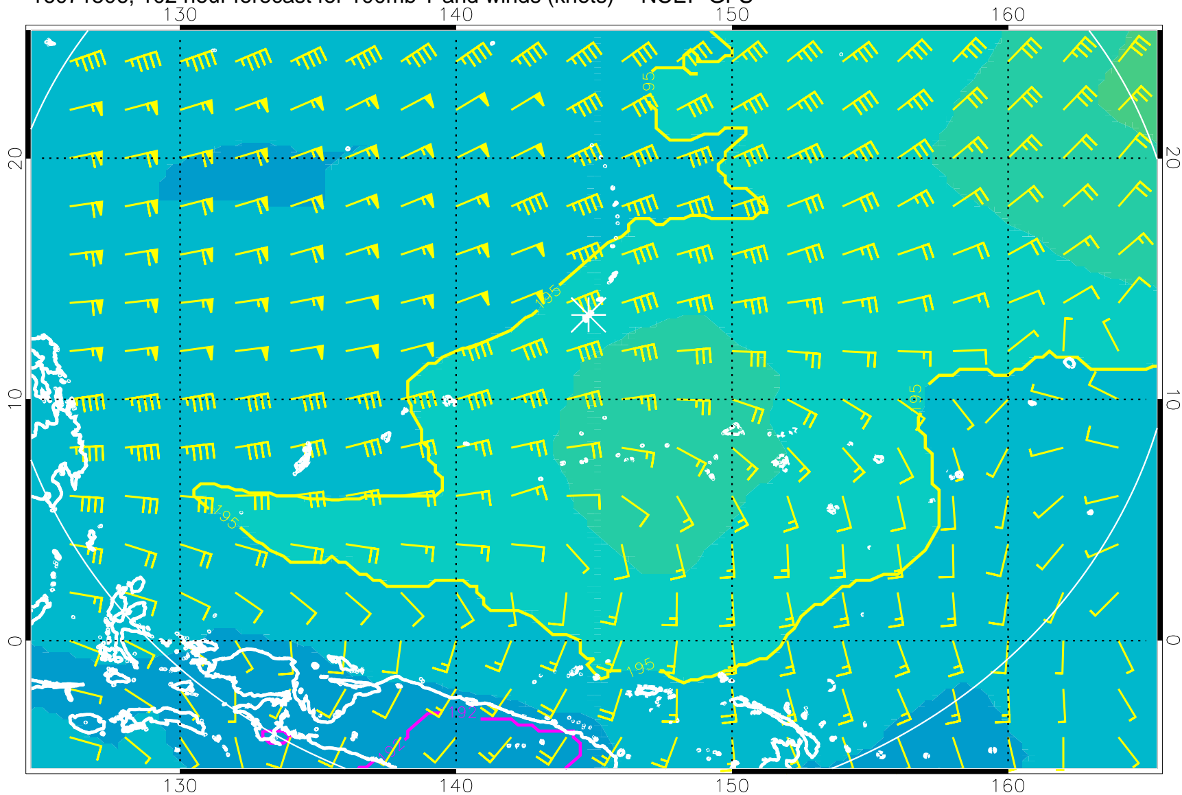
16071506, 102 hour forecast for 100mb T and winds (knots) -- NCEP GFS
