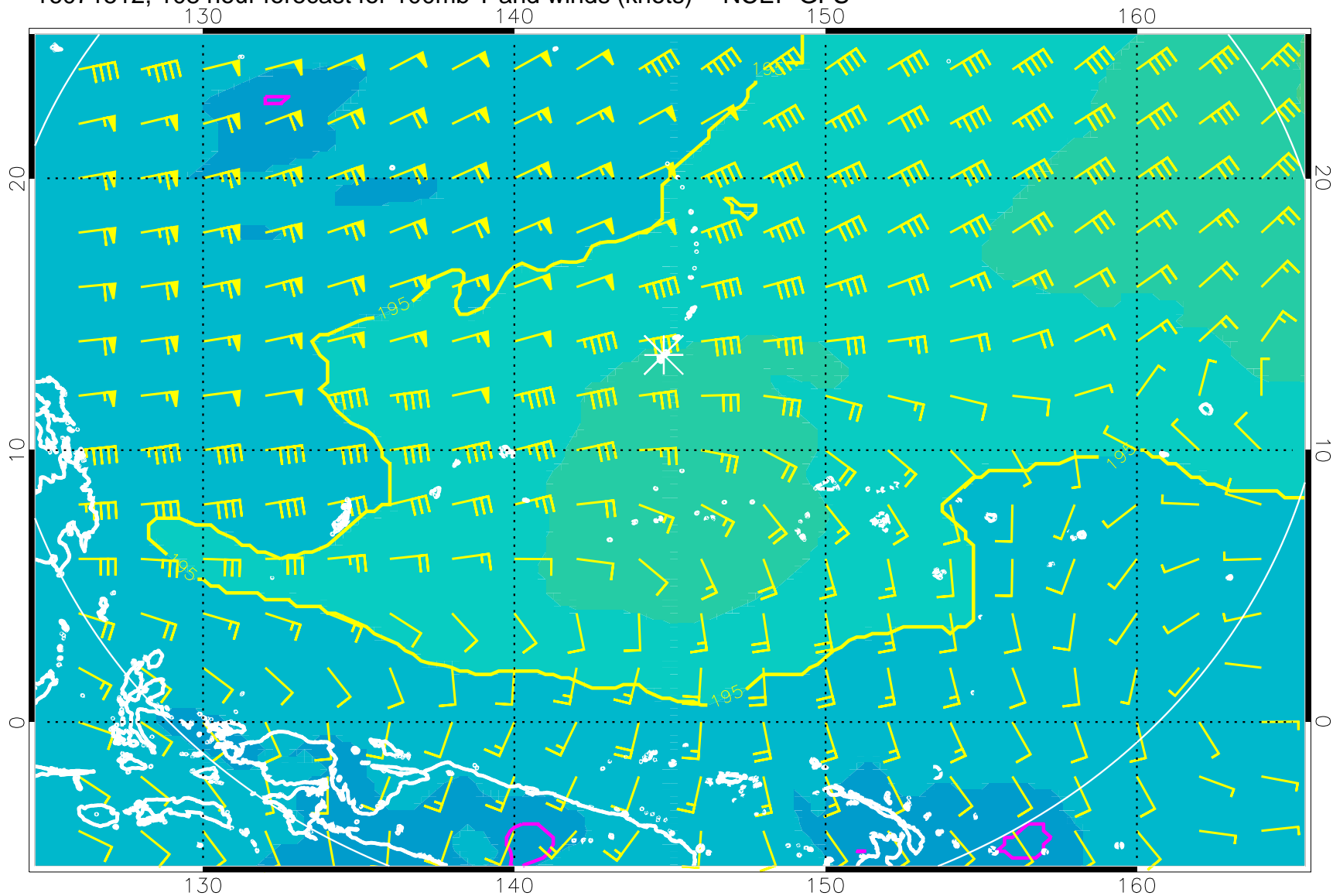
16071512, 108 hour forecast for 100mb T and winds (knots) -- NCEP GFS
