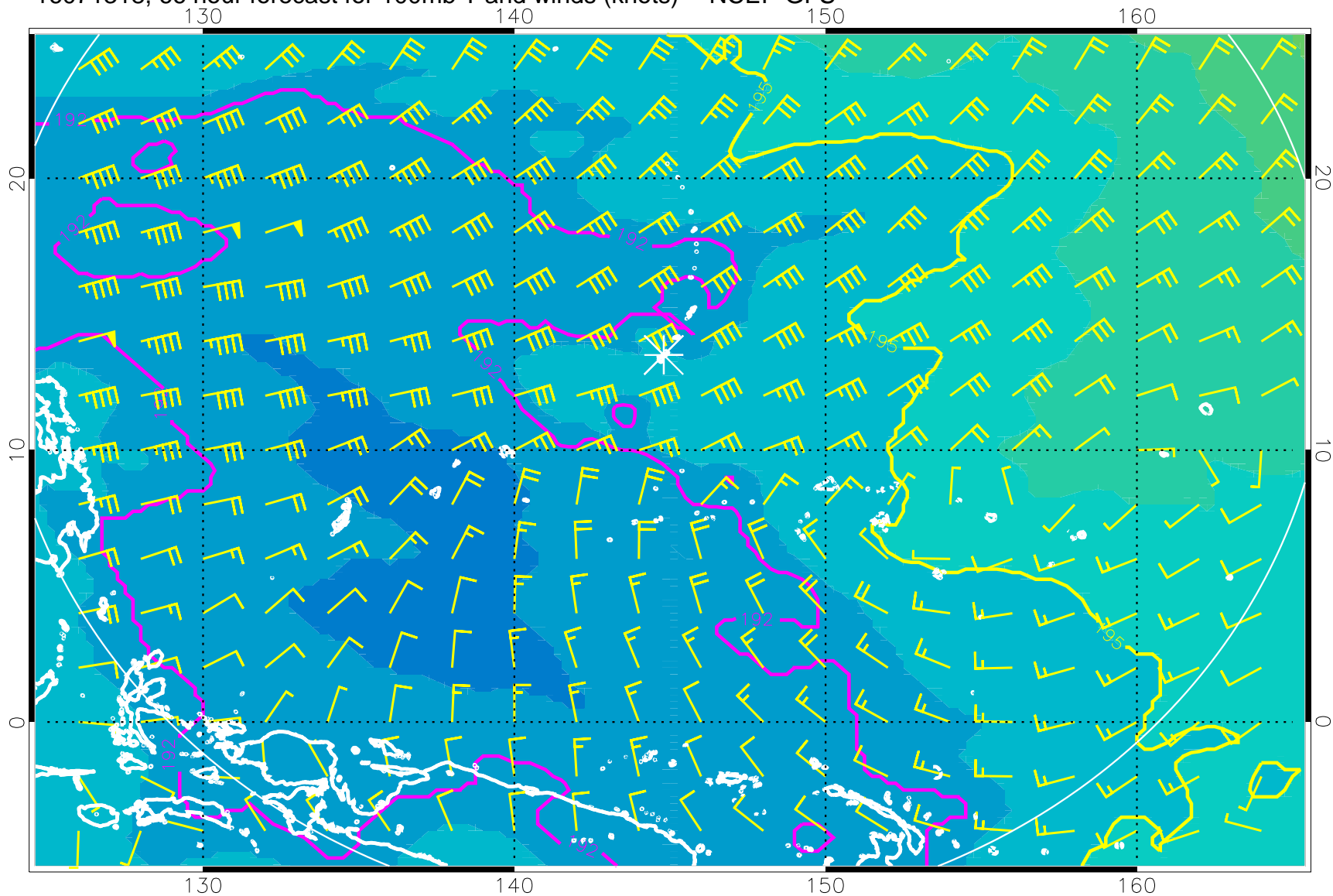
16071318, 66 hour forecast for 100mb T and winds (knots) -- NCEP GFS
