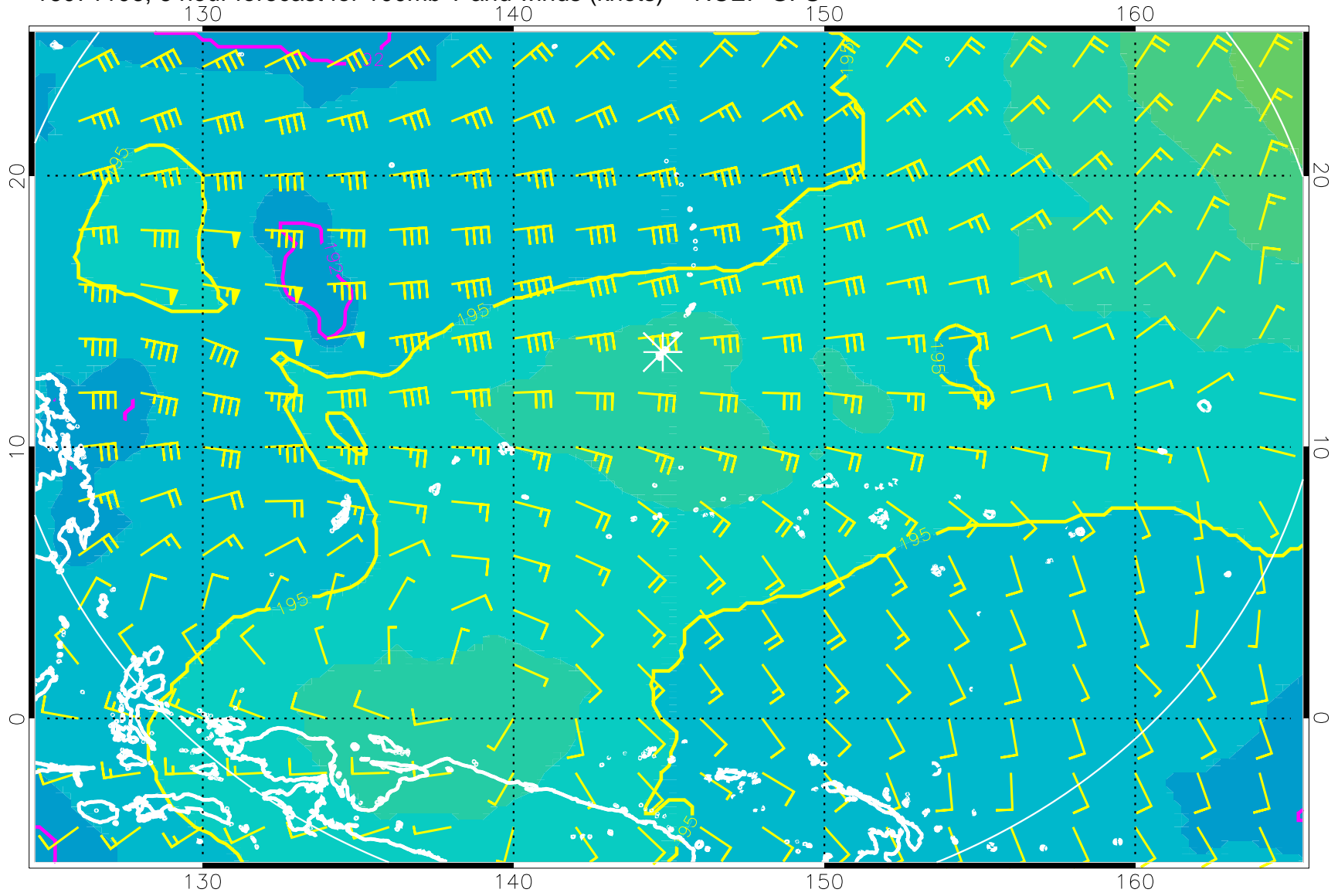
16071106, 6 hour forecast for 100mb T and winds (knots) -- NCEP GFS
