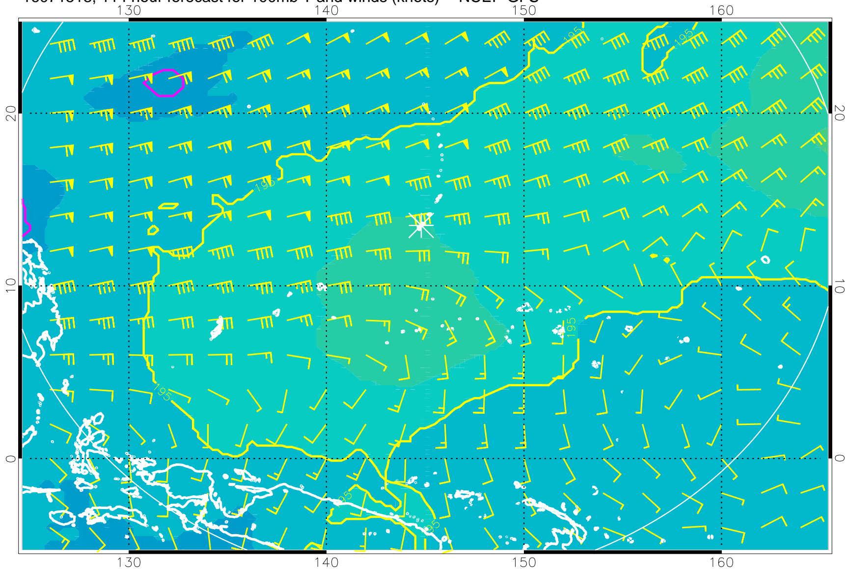
16071518, 114 hour forecast for 100mb T and winds (knots) -- NCEP GFS
