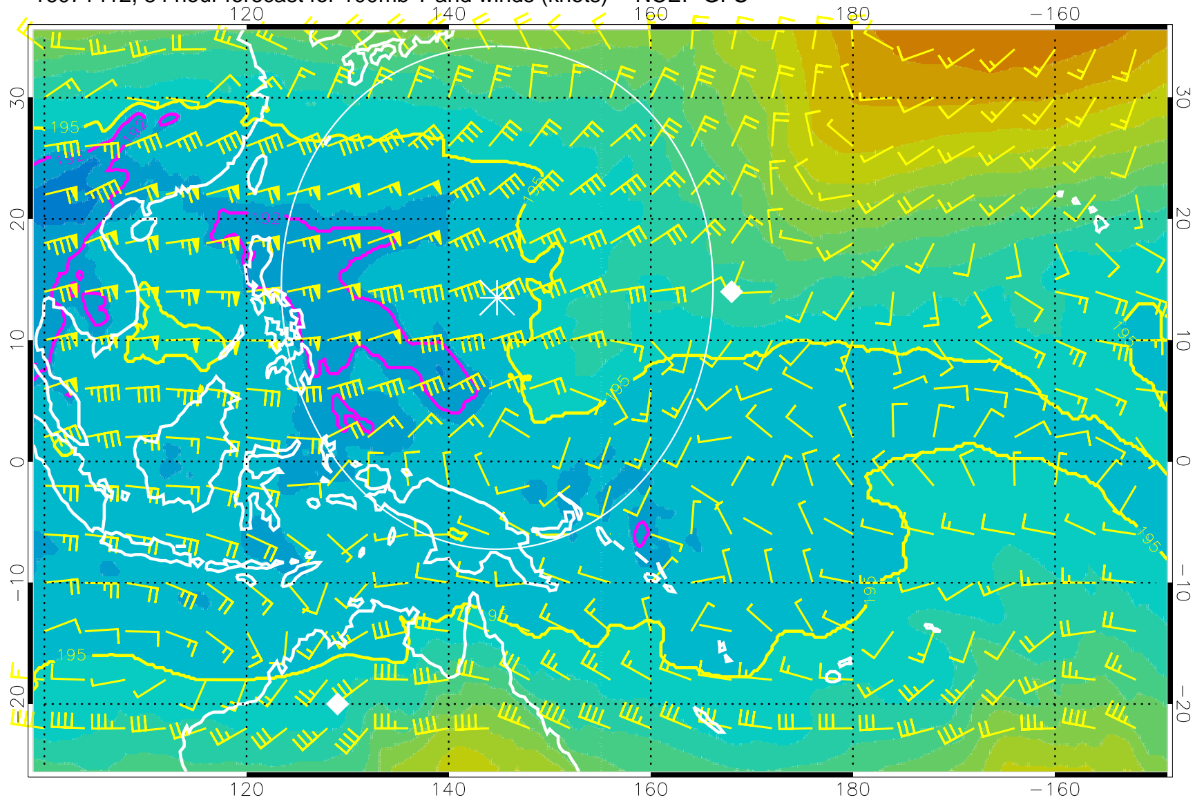
16071412, 84 hour forecast for 100mb T and winds (knots) -- NCEP GFS
