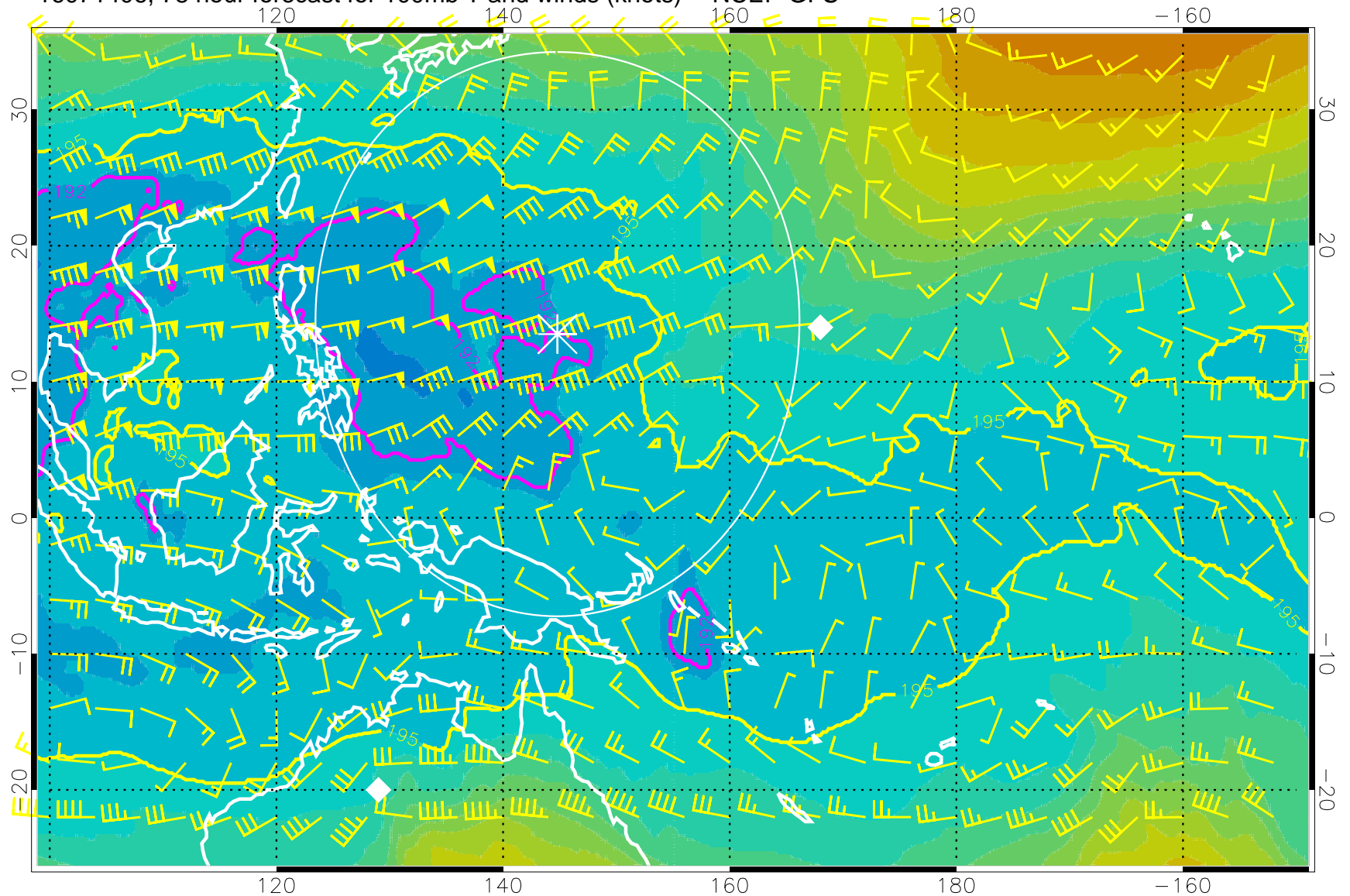
16071406, 78 hour forecast for 100mb T and winds (knots) -- NCEP GFS
