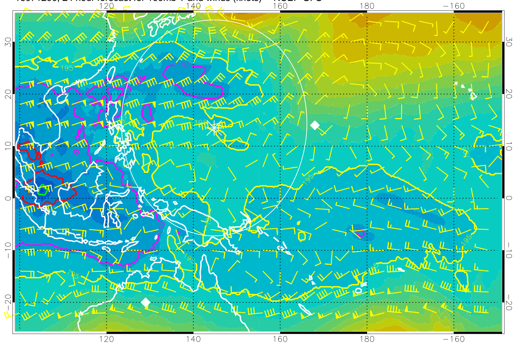
16071200, 24 hour forecast for 100mb T and winds (knots) -- NCEP GFS
