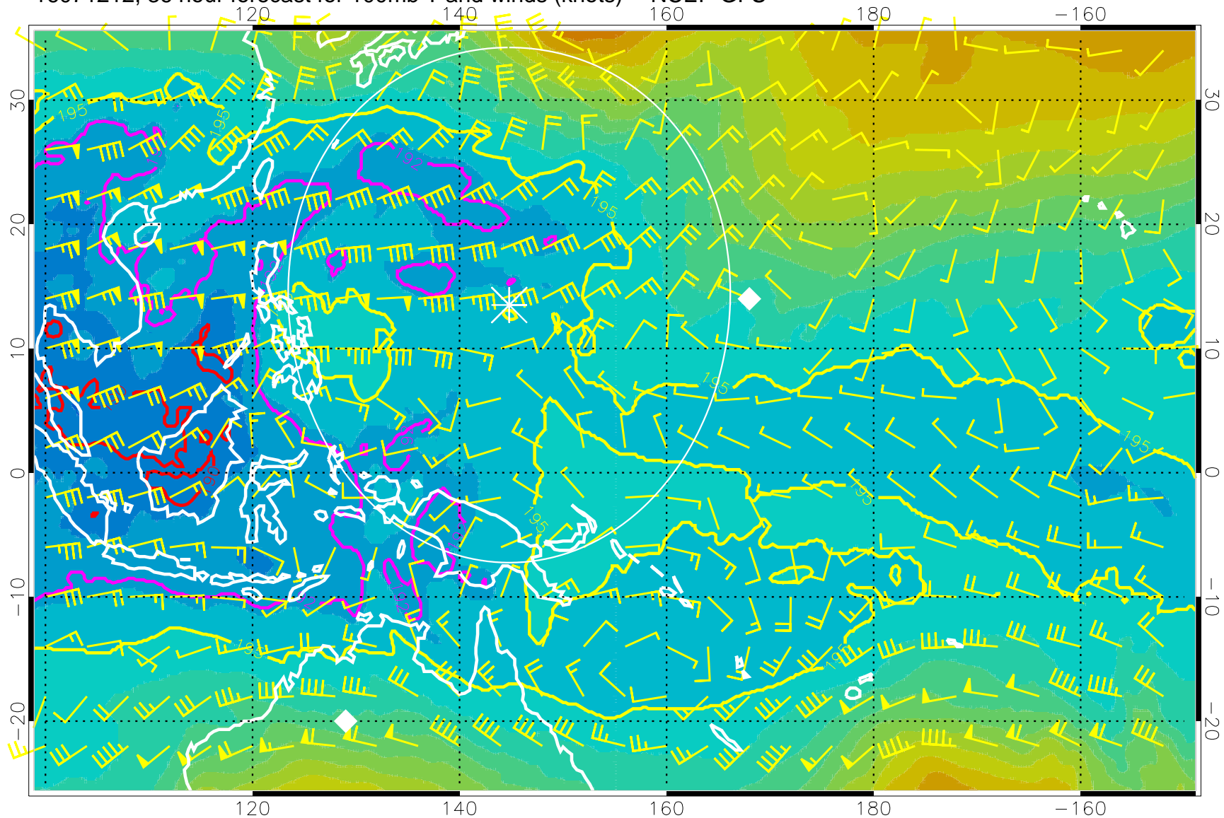
16071212, 36 hour forecast for 100mb T and winds (knots) -- NCEP GFS
