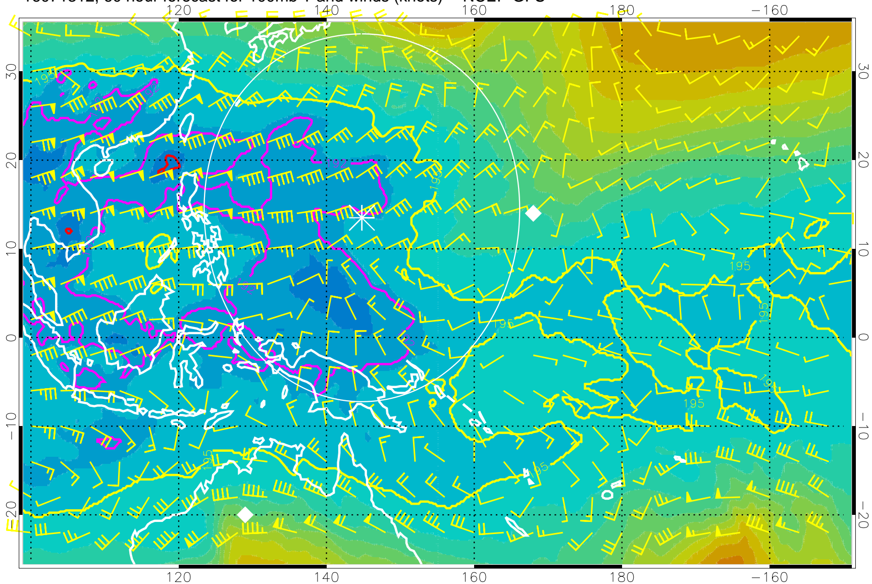
16071312, 60 hour forecast for 100mb T and winds (knots) -- NCEP GFS
