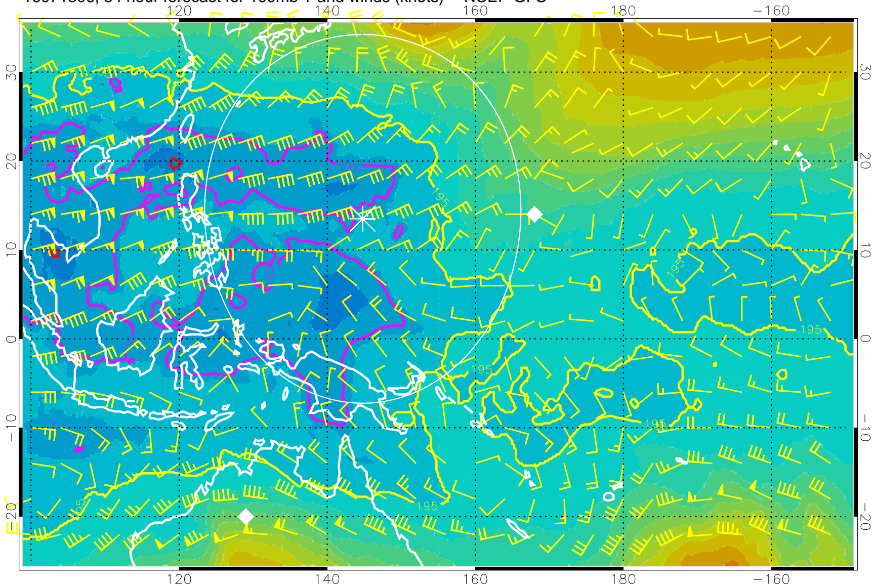
16071306, 54 hour forecast for 100mb T and winds (knots) -- NCEP GFS
