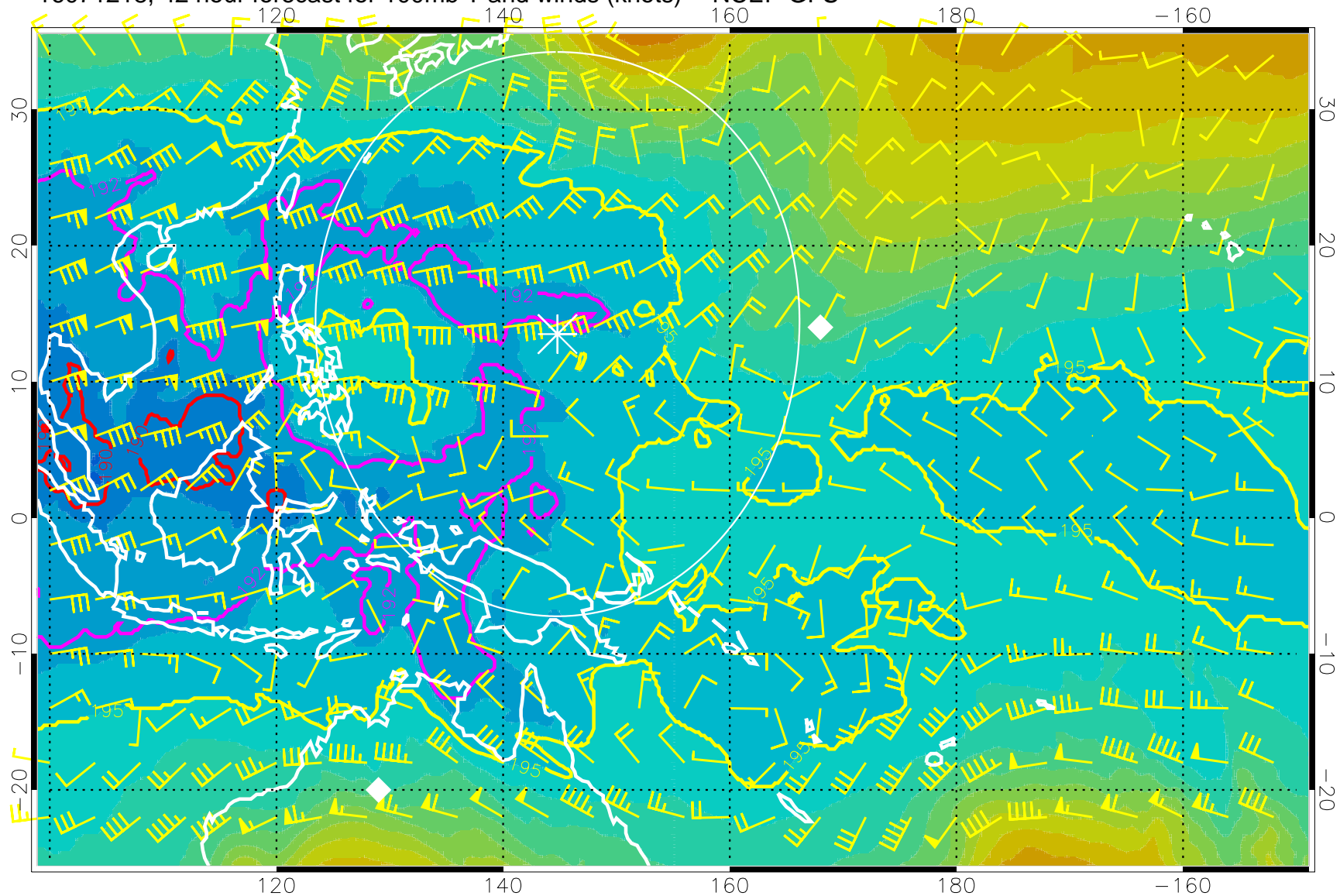
16071218, 42 hour forecast for 100mb T and winds (knots) -- NCEP GFS
