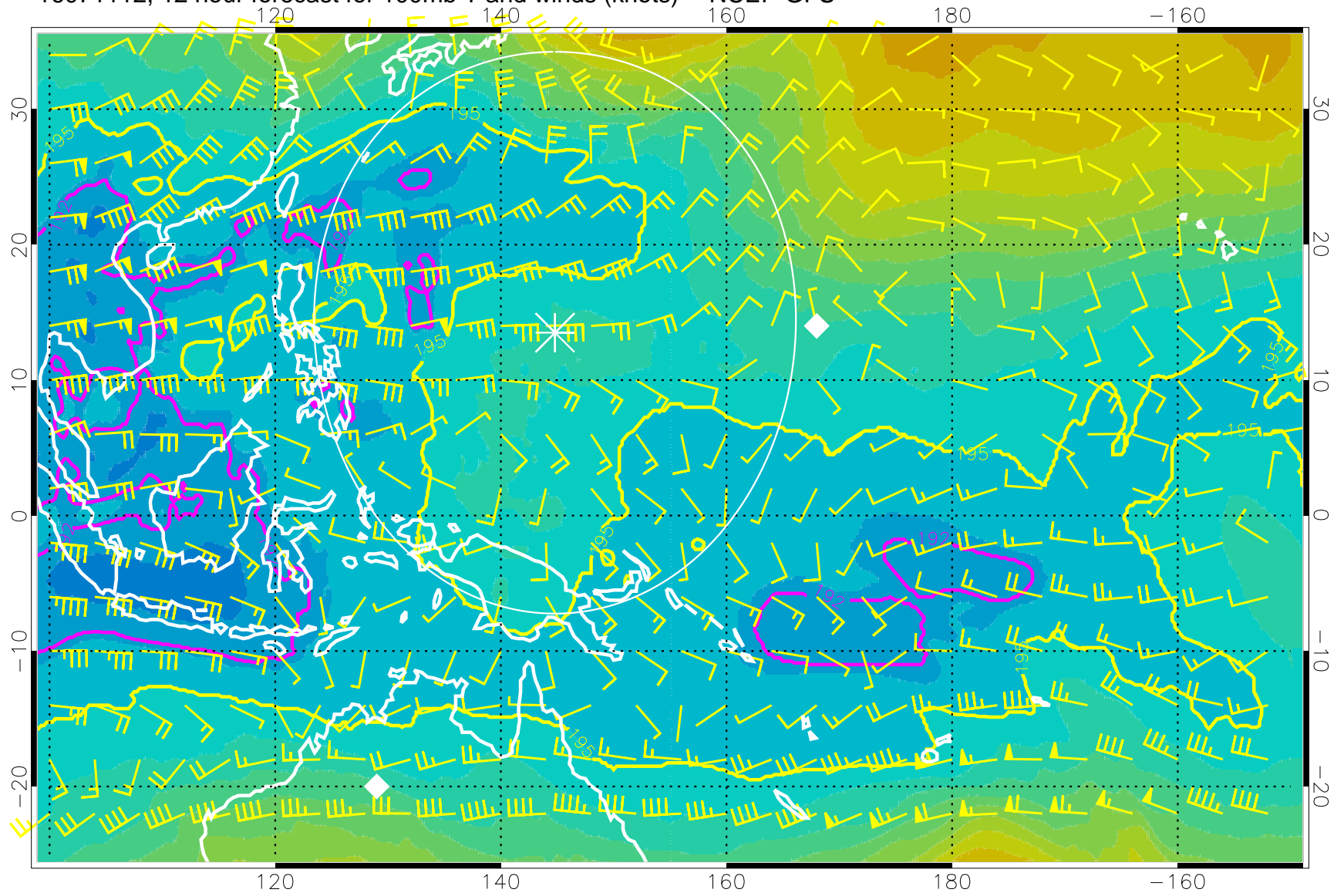
16071112, 12 hour forecast for 100mb T and winds (knots) -- NCEP GFS
