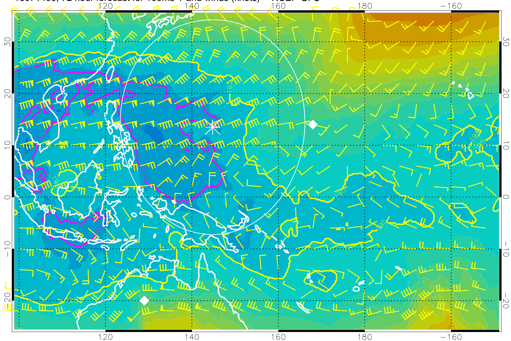
16071400, 72 hour forecast for 100mb T and winds (knots) -- NCEP GFS
