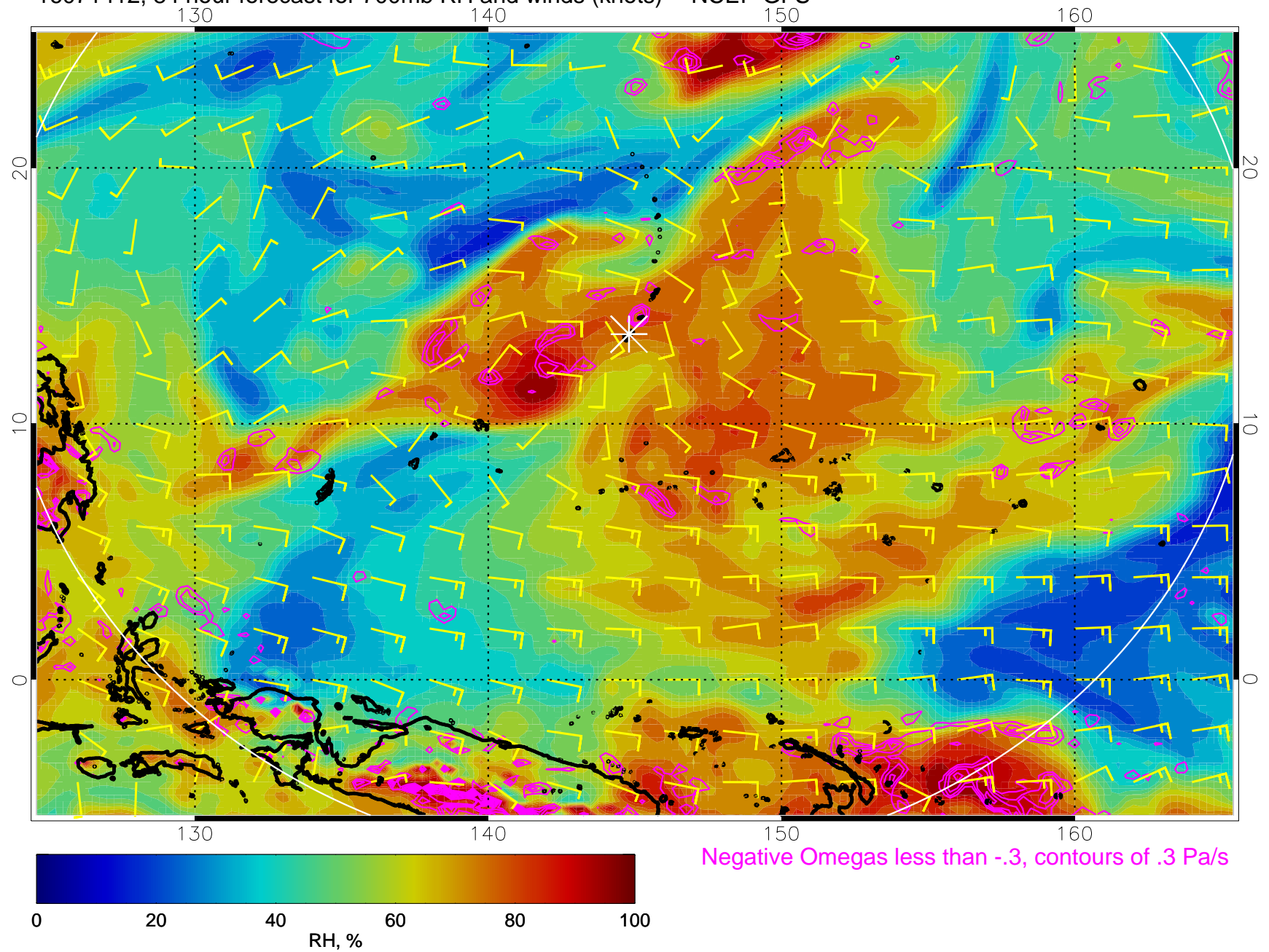
16071412, 84 hour forecast for 700mb RH and winds (knots) -- NCEP GFS
