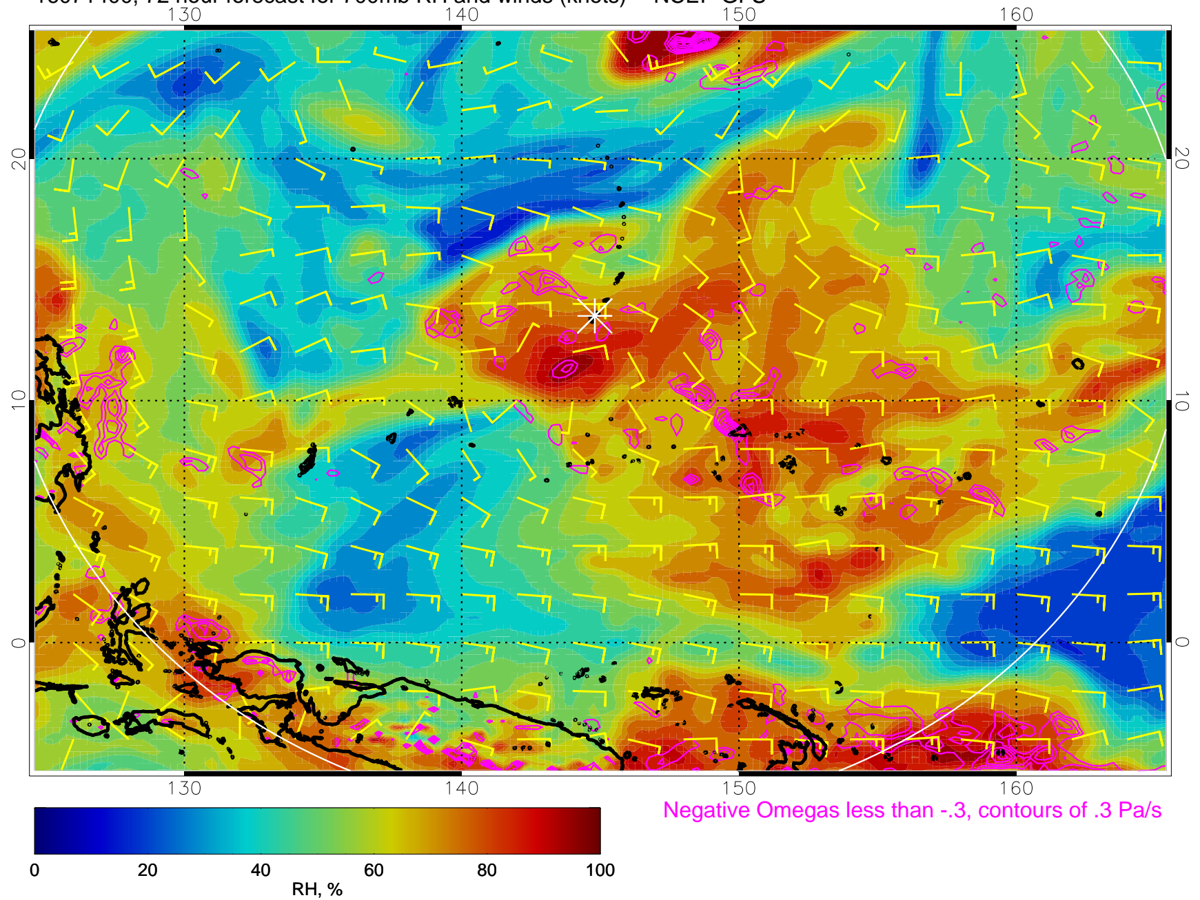
16071400, 72 hour forecast for 700mb RH and winds (knots) -- NCEP GFS
