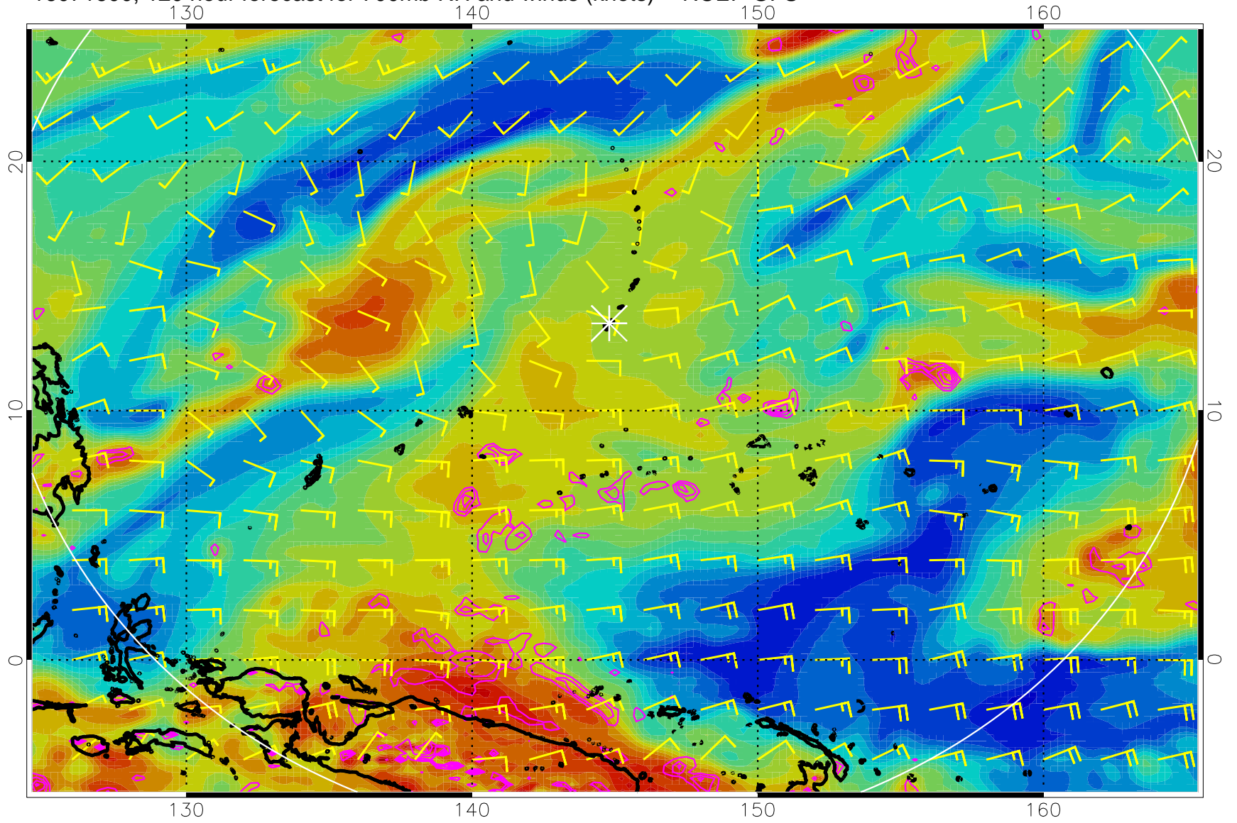
16071600, 120 hour forecast for 700mb RH and winds (knots) -- NCEP GFS
