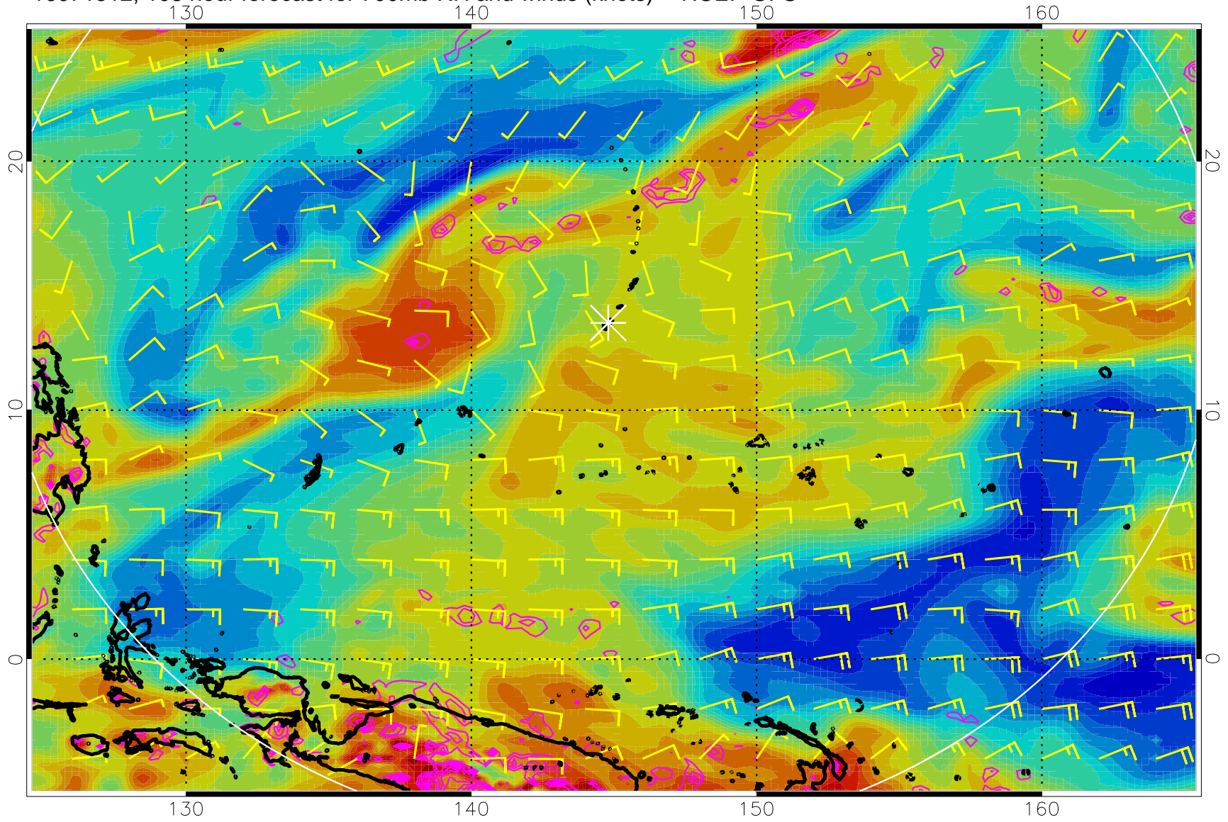
16071512, 108 hour forecast for 700mb RH and winds (knots) -- NCEP GFS
