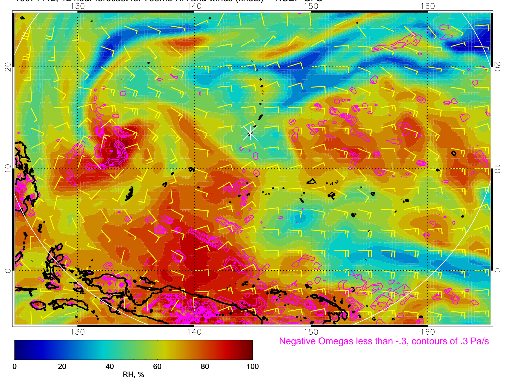
16071112, 12 hour forecast for 700mb RH and winds (knots) -- NCEP GFS
