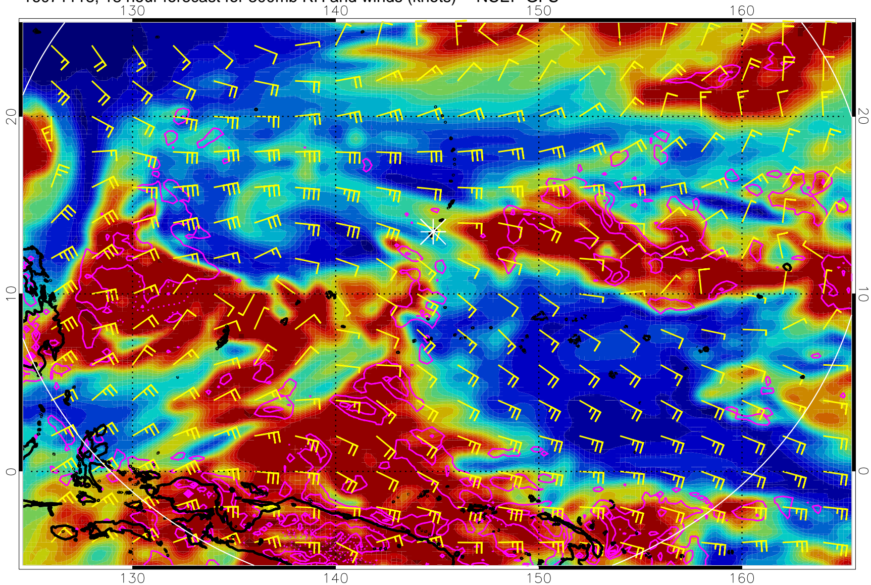
16071118, 18 hour forecast for 300mb RH and winds (knots) -- NCEP GFS
