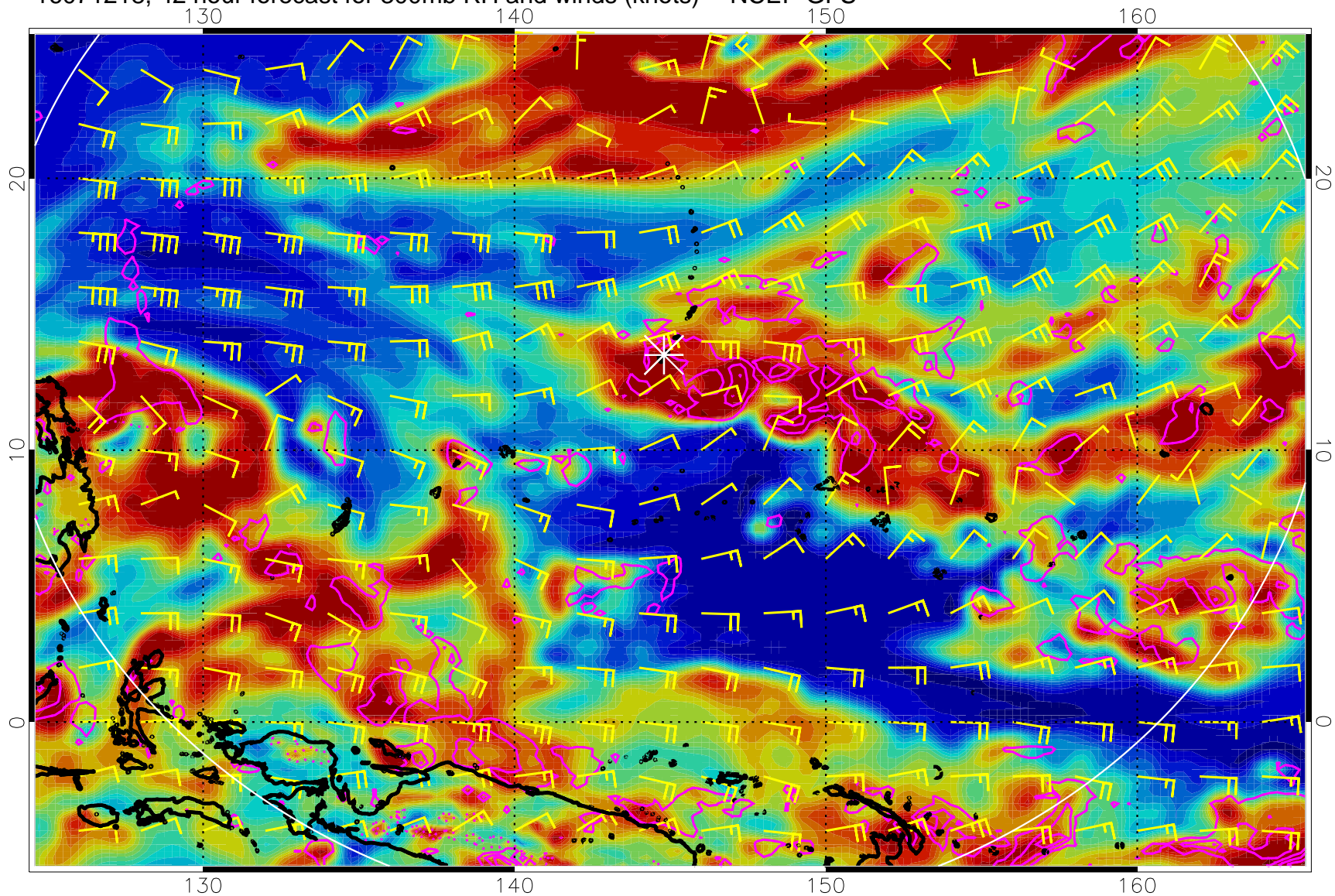
16071218, 42 hour forecast for 300mb RH and winds (knots) -- NCEP GFS
