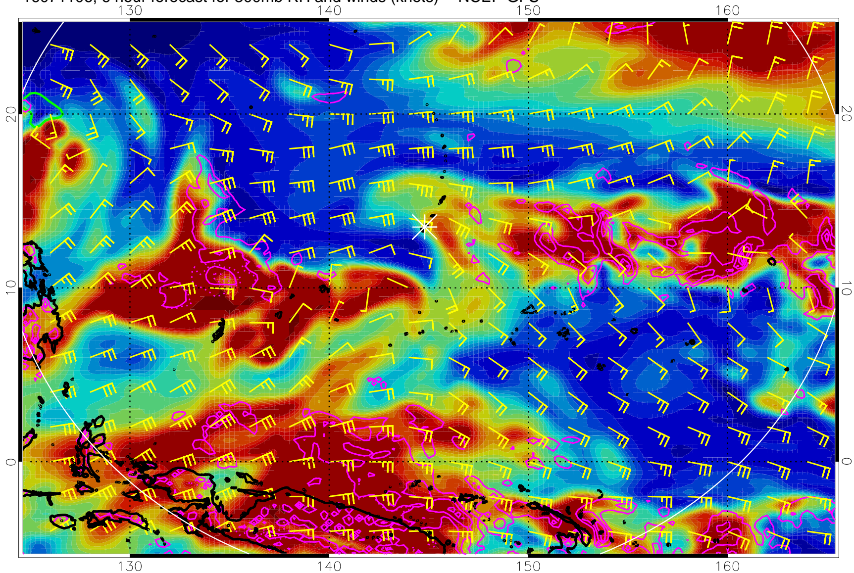
16071106, 6 hour forecast for 300mb RH and winds (knots) -- NCEP GFS
