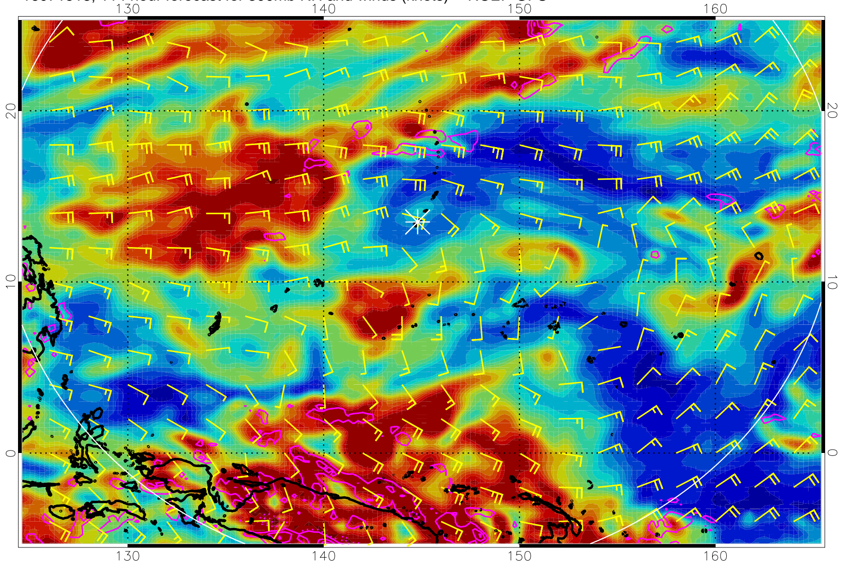
16071518, 114 hour forecast for 300mb RH and winds (knots) -- NCEP GFS
