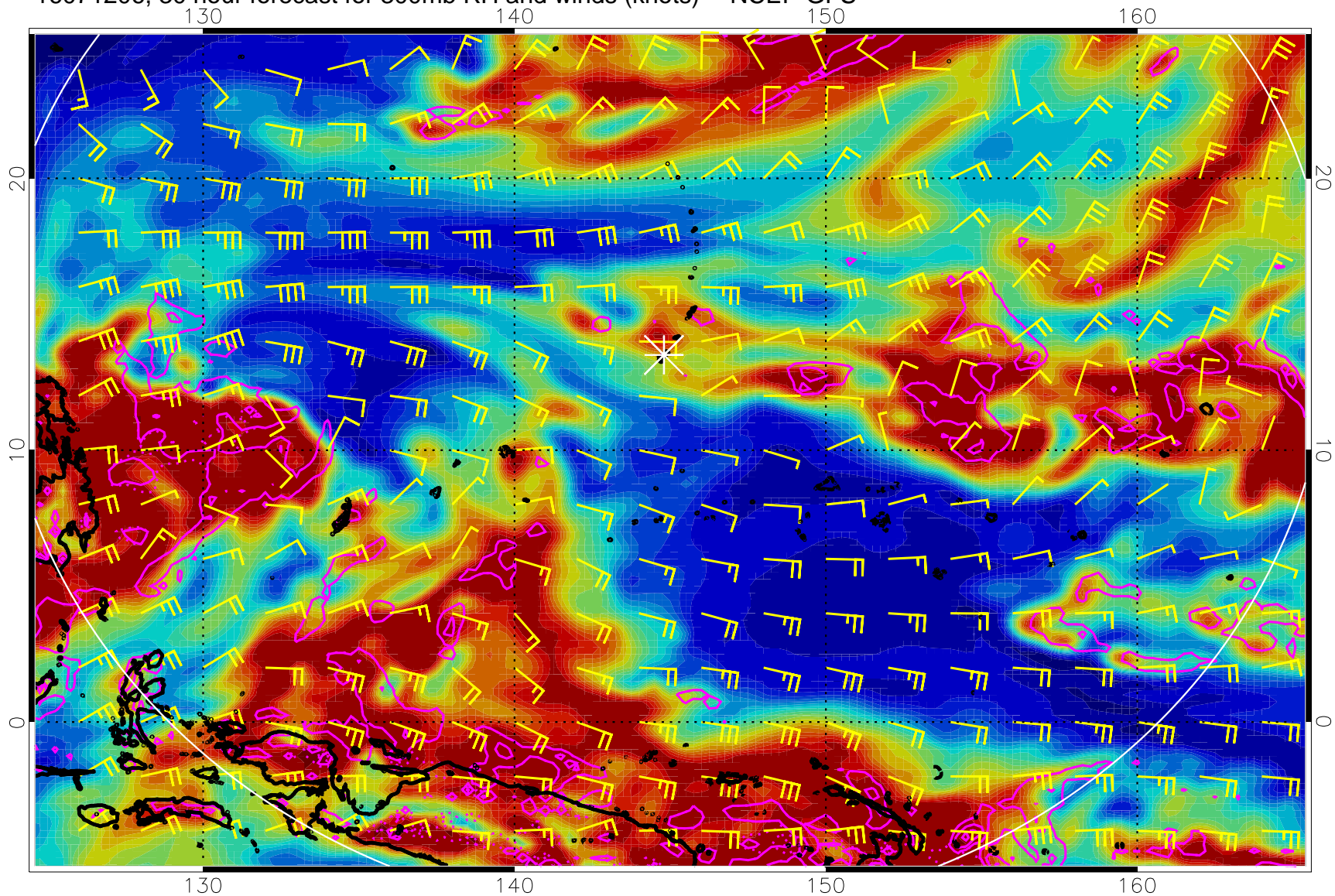
16071206, 30 hour forecast for 300mb RH and winds (knots) -- NCEP GFS
