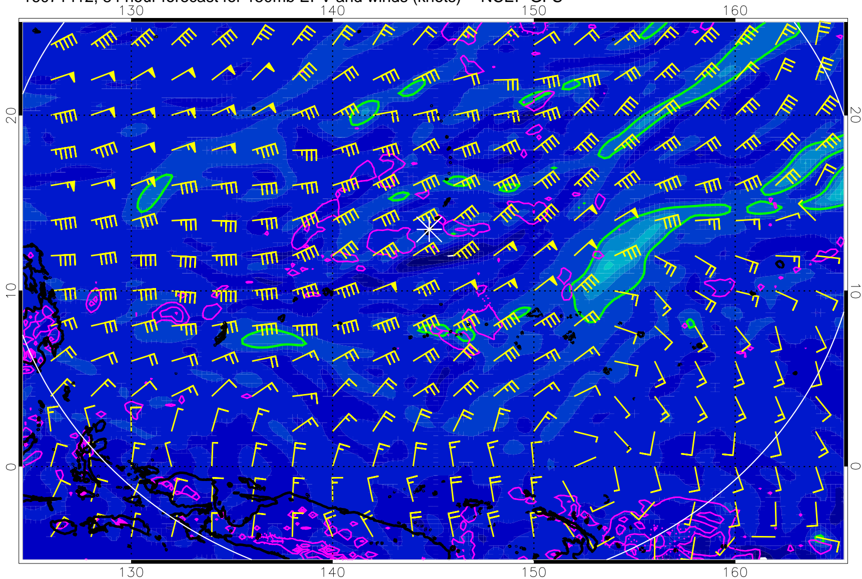
16071412, 84 hour forecast for 150mb EPV and winds (knots) -- NCEP GFS
