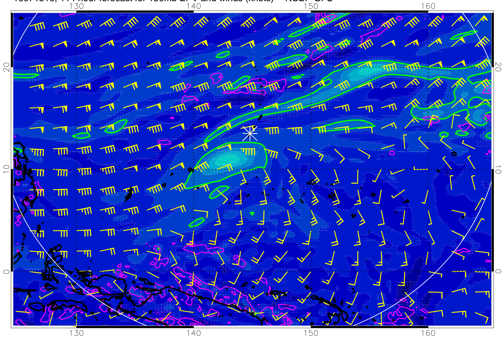
16071518, 114 hour forecast for 150mb EPV and winds (knots) -- NCEP GFS
