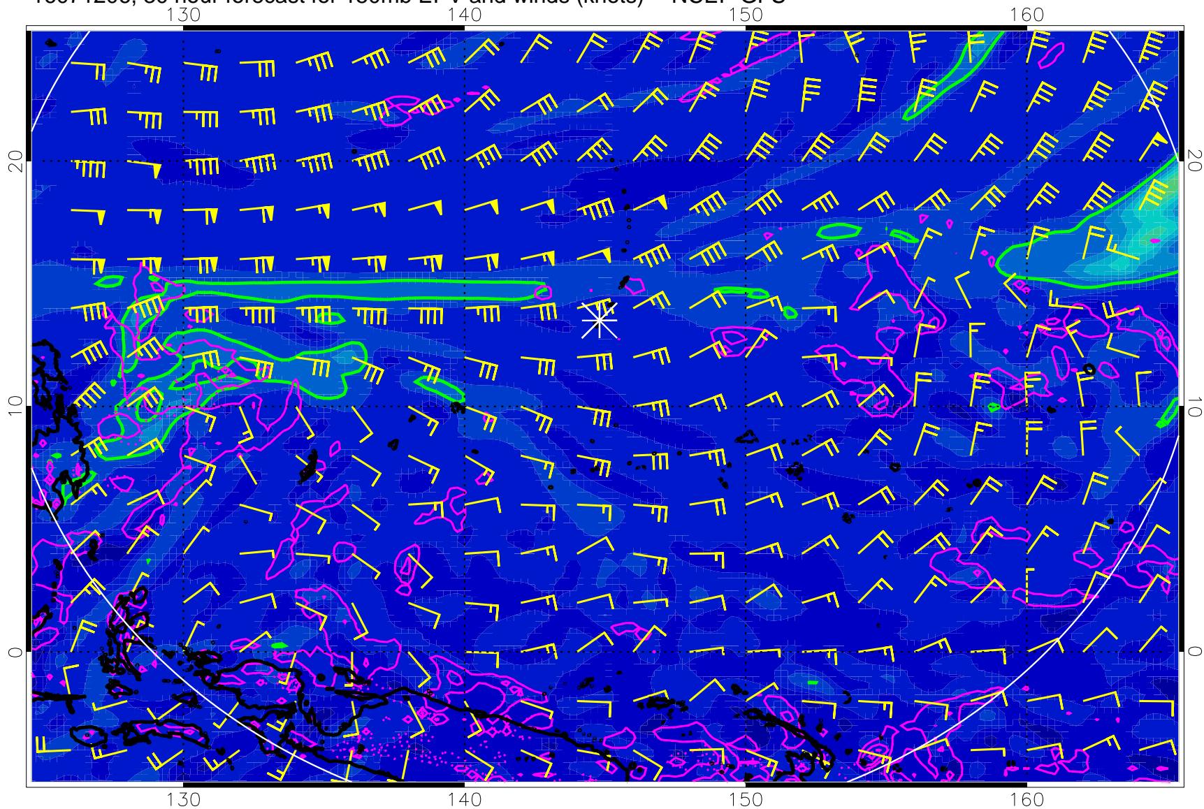
16071206, 30 hour forecast for 150mb EPV and winds (knots) -- NCEP GFS
