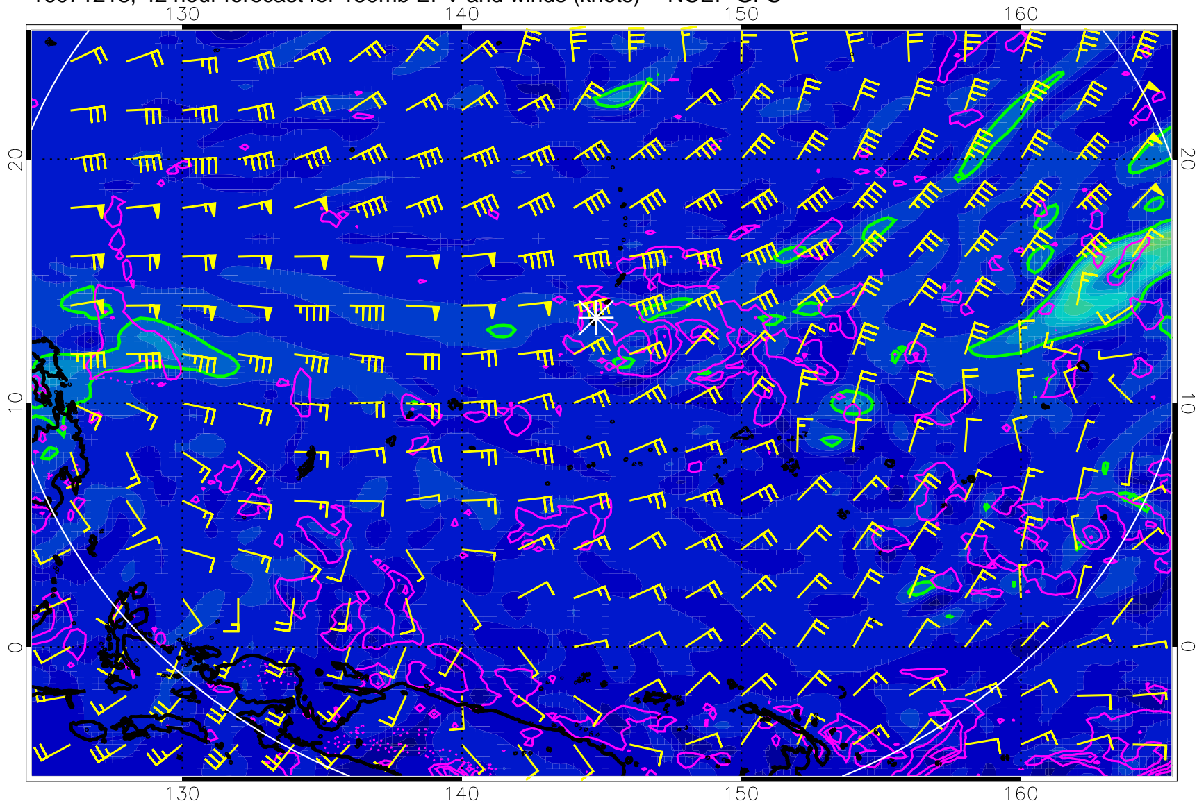
16071218, 42 hour forecast for 150mb EPV and winds (knots) -- NCEP GFS
