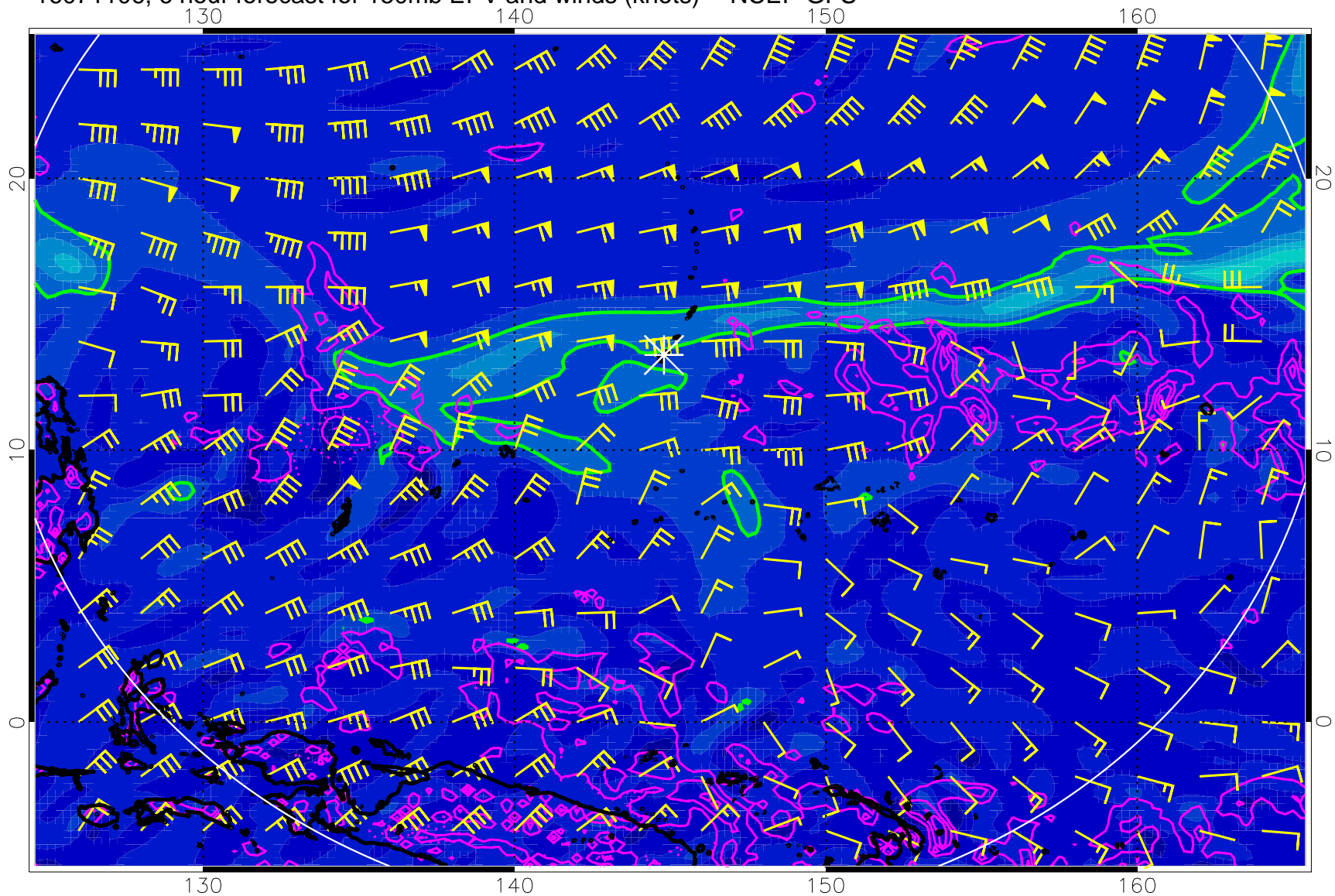
16071106, 6 hour forecast for 150mb EPV and winds (knots) -- NCEP GFS
