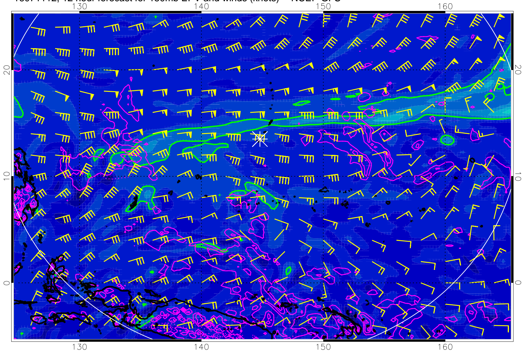
16071112, 12 hour forecast for 150mb EPV and winds (knots) -- NCEP GFS
