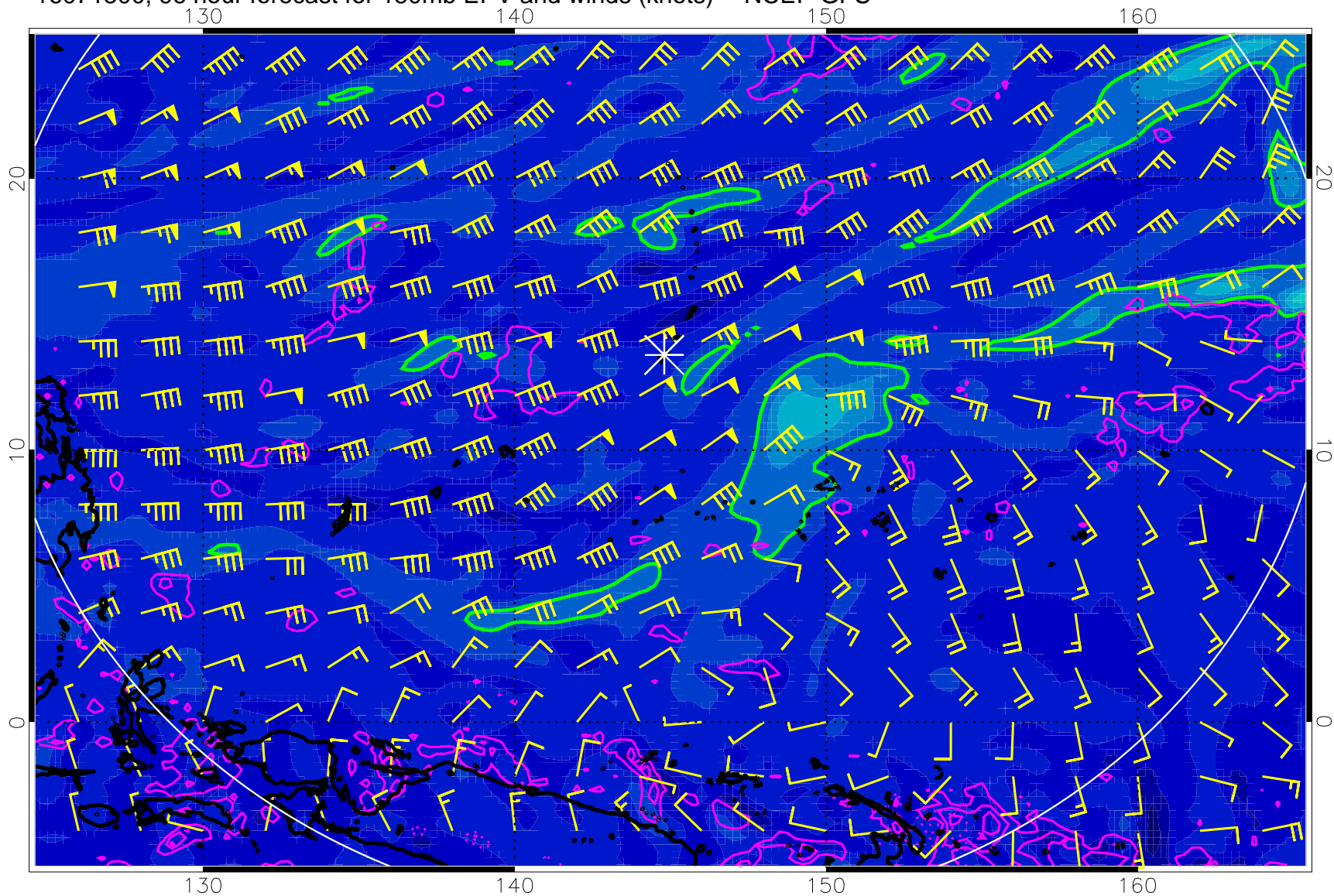
16071500, 96 hour forecast for 150mb EPV and winds (knots) -- NCEP GFS
