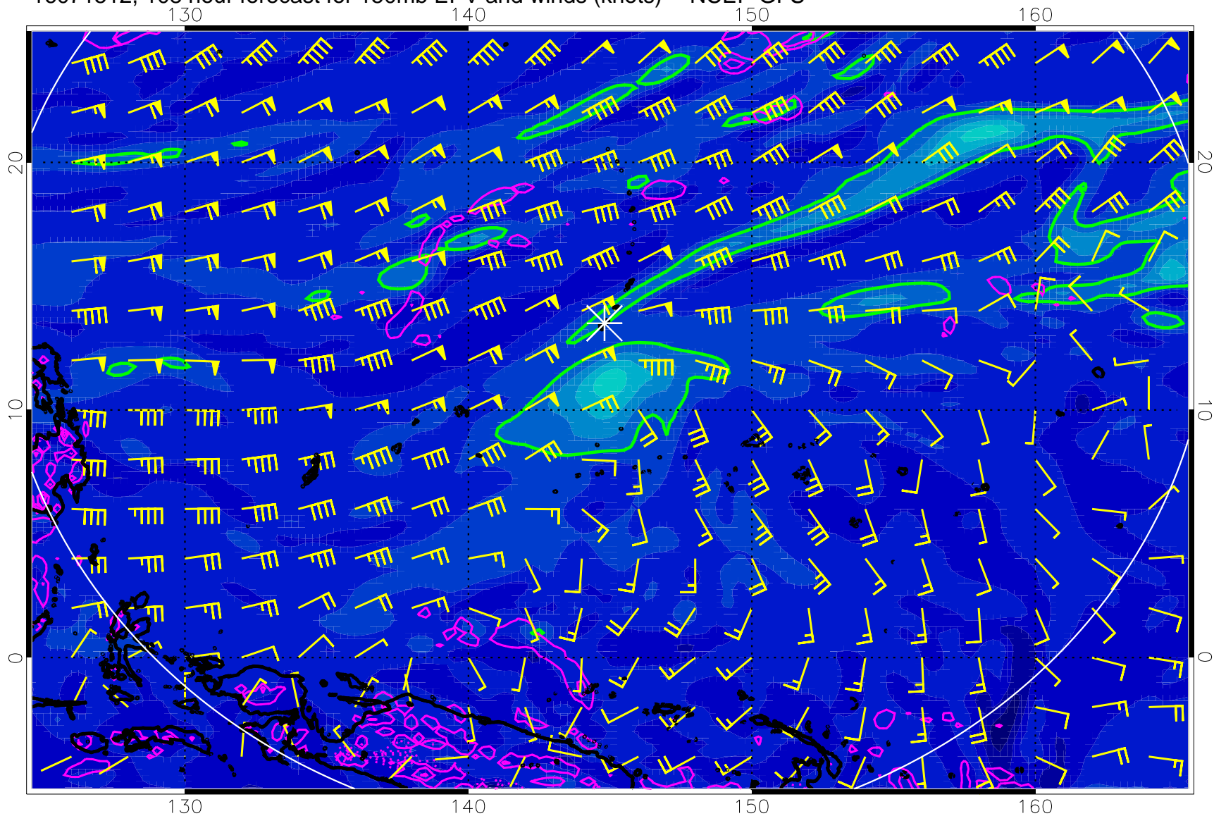
16071512, 108 hour forecast for 150mb EPV and winds (knots) -- NCEP GFS
