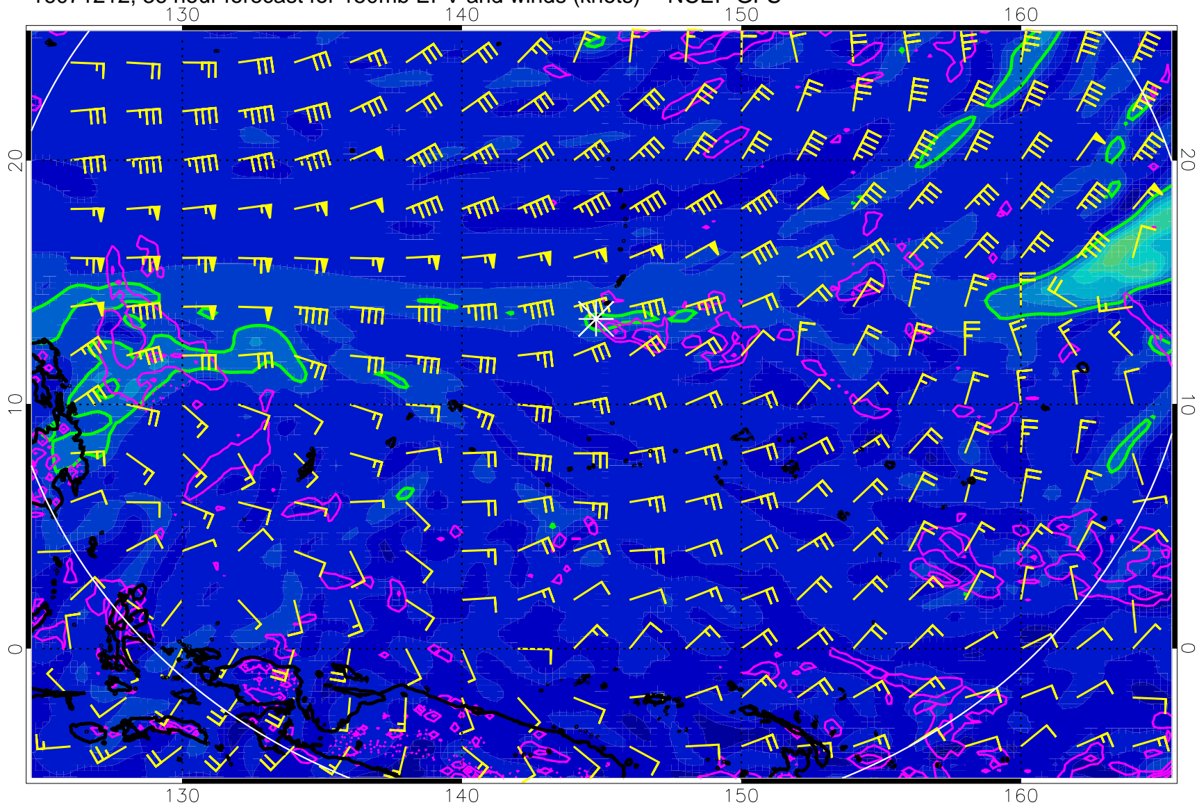
16071212, 36 hour forecast for 150mb EPV and winds (knots) -- NCEP GFS
