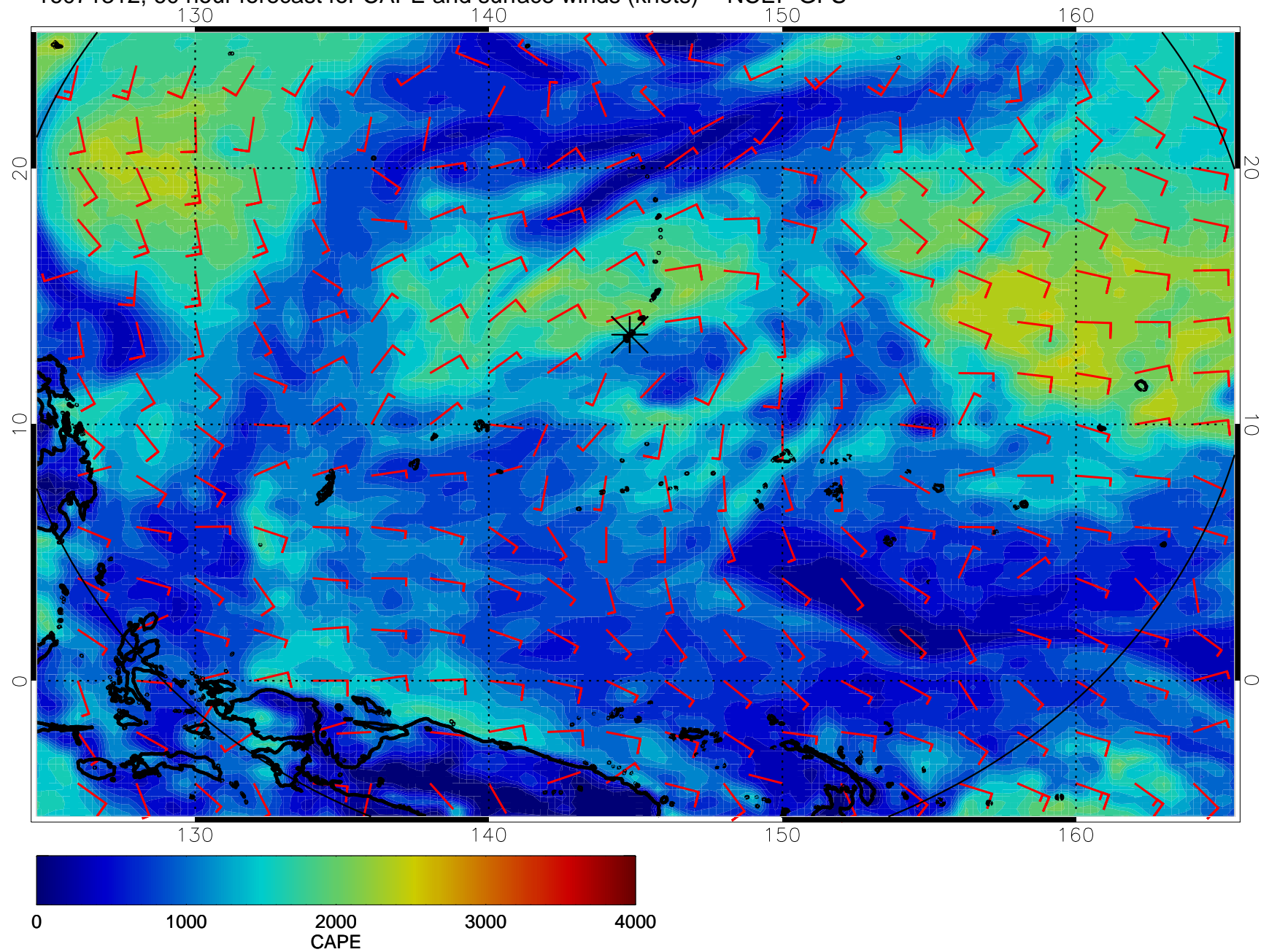
16071312, 60 hour forecast for CAPE and surface winds (knots) -- NCEP GFS
