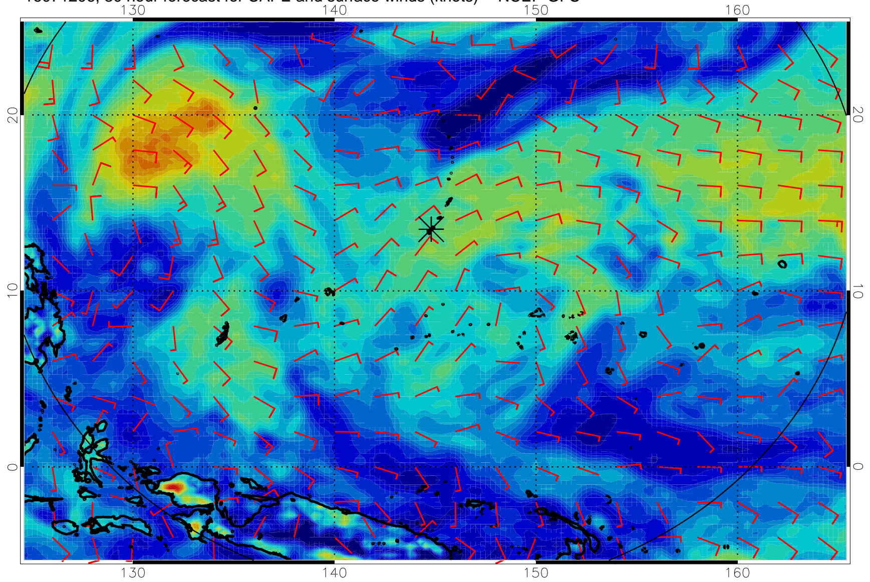
16071206, 30 hour forecast for CAPE and surface winds (knots) -- NCEP GFS
