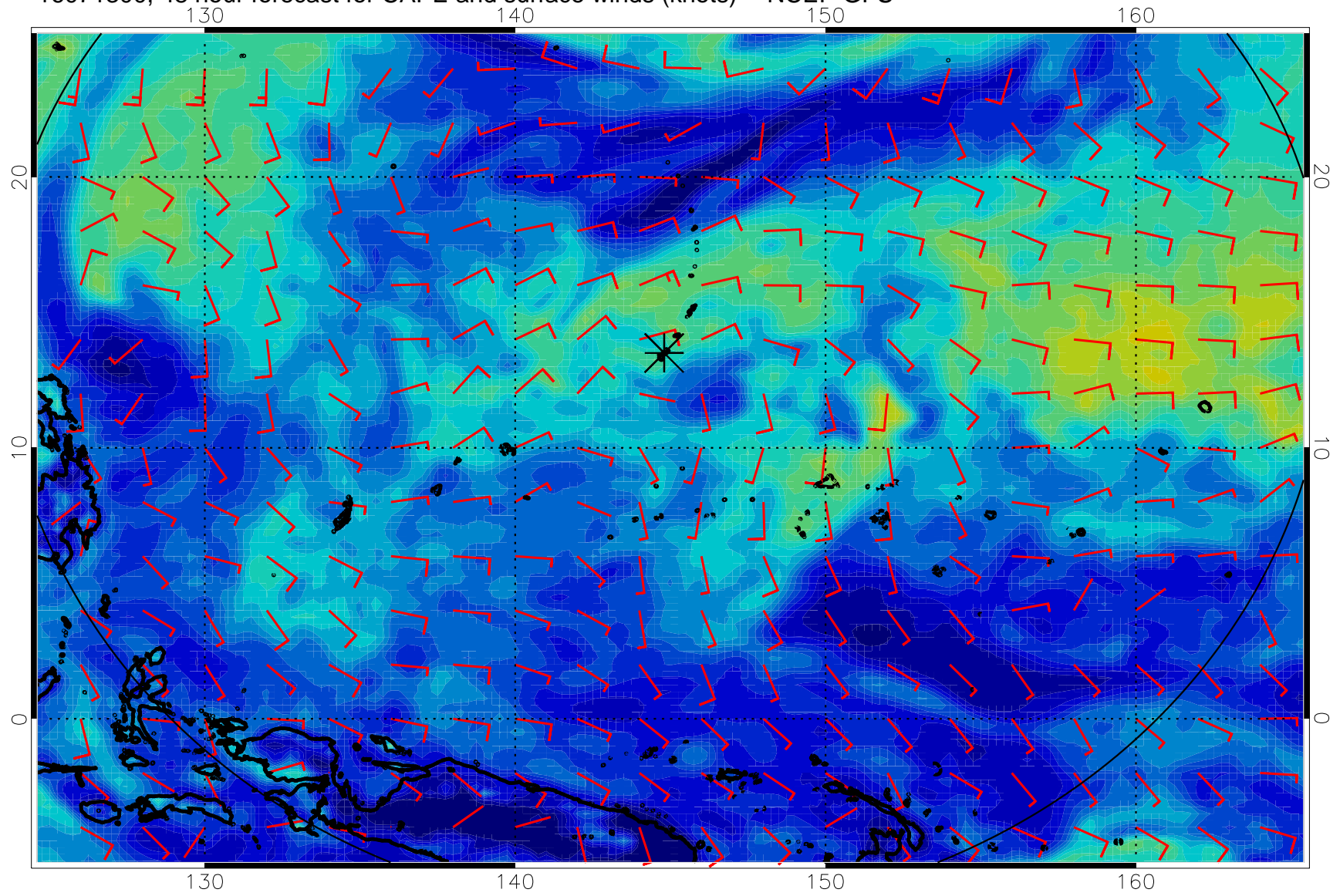
16071300, 48 hour forecast for CAPE and surface winds (knots) -- NCEP GFS
