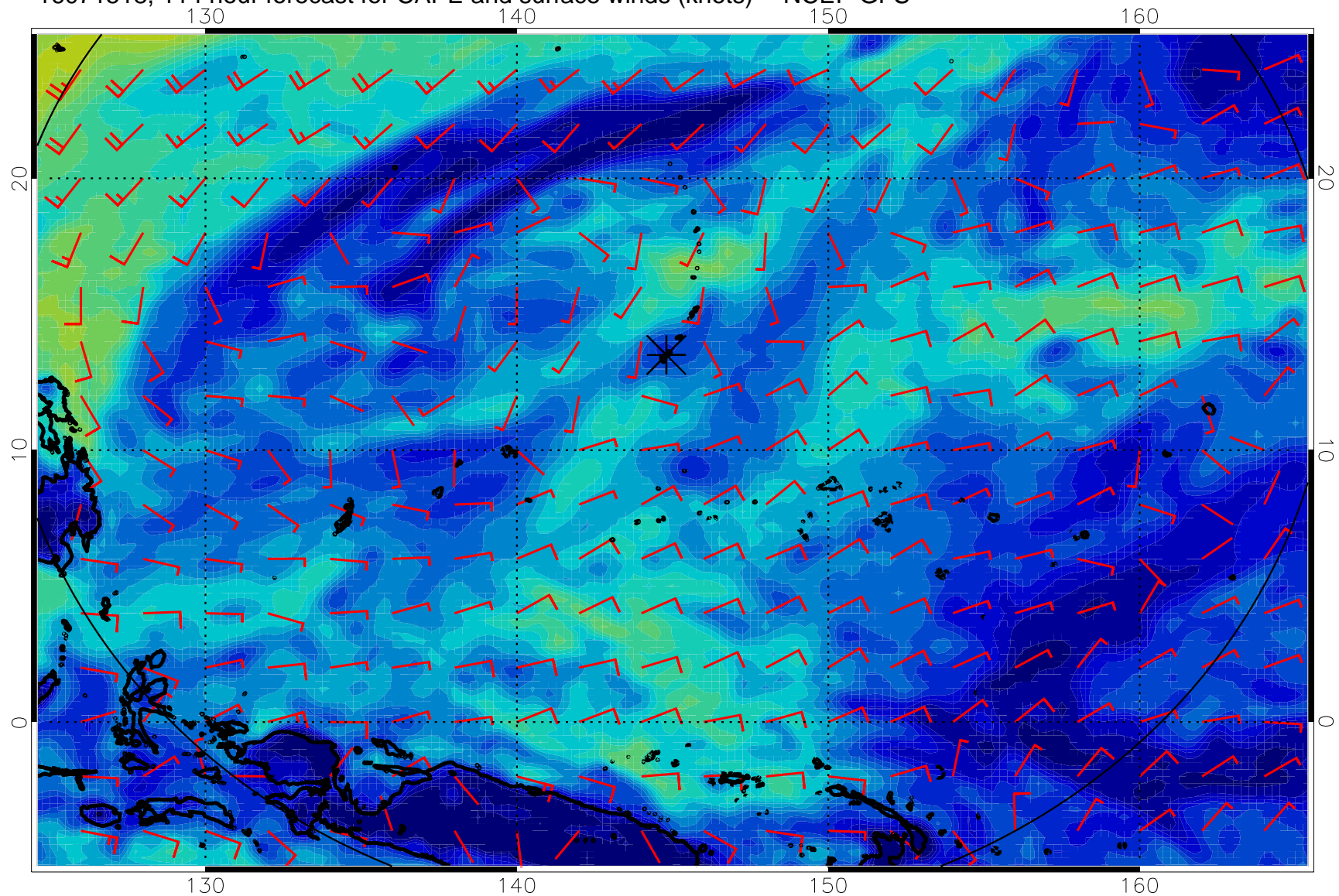
16071518, 114 hour forecast for CAPE and surface winds (knots) -- NCEP GFS
