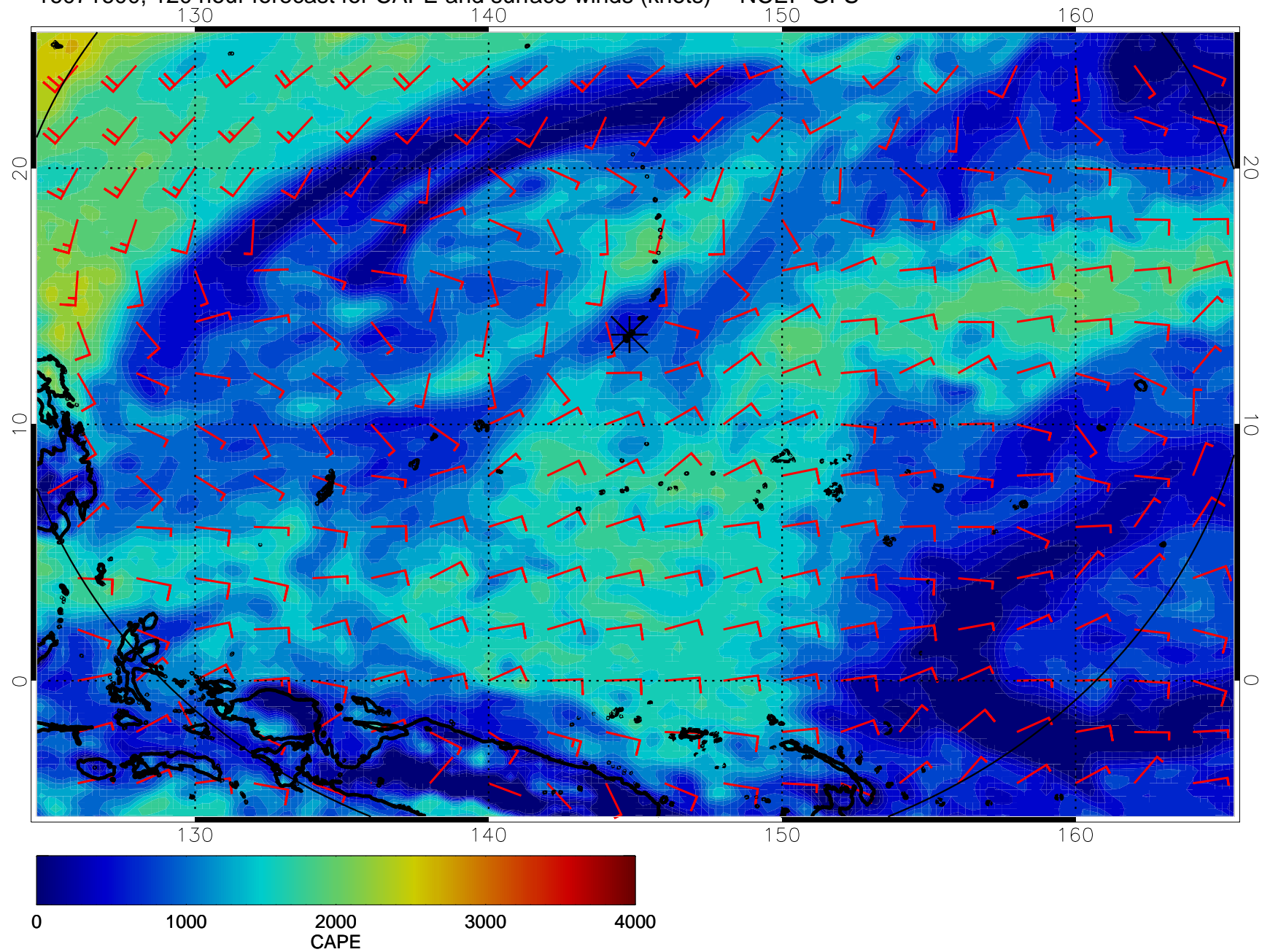
16071600, 120 hour forecast for CAPE and surface winds (knots) -- NCEP GFS
