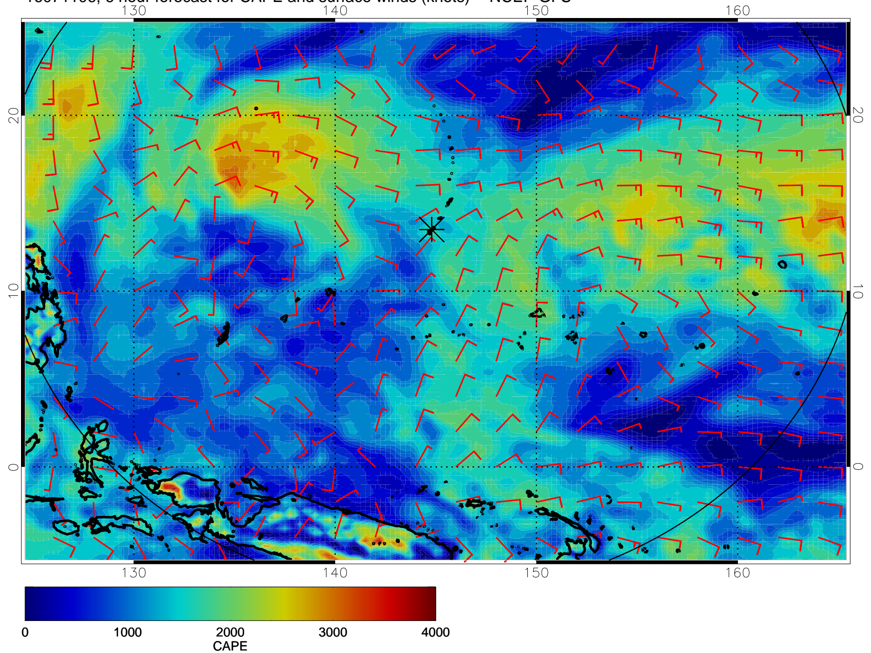
16071106, 6 hour forecast for CAPE and surface winds (knots) -- NCEP GFS
