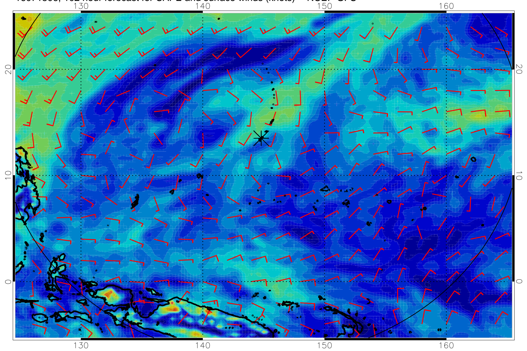
16071506, 102 hour forecast for CAPE and surface winds (knots) -- NCEP GFS
