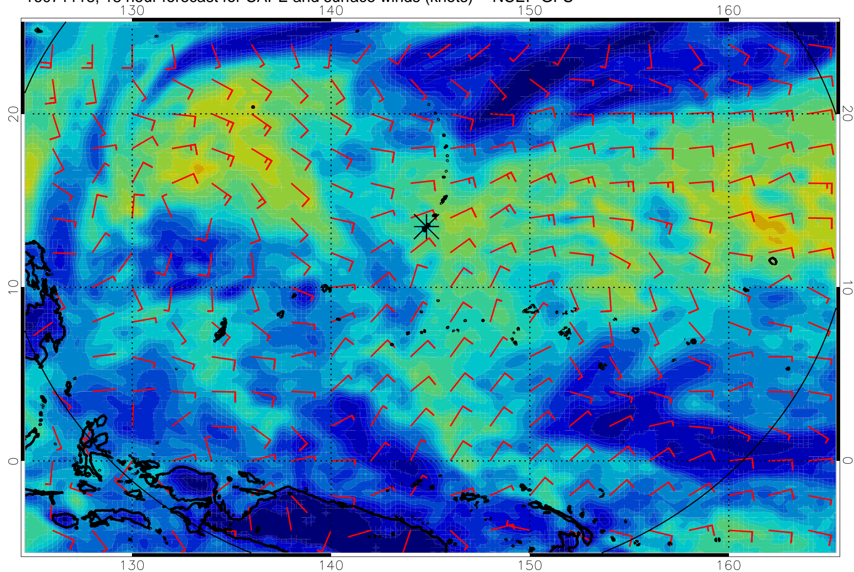
16071118, 18 hour forecast for CAPE and surface winds (knots) -- NCEP GFS
