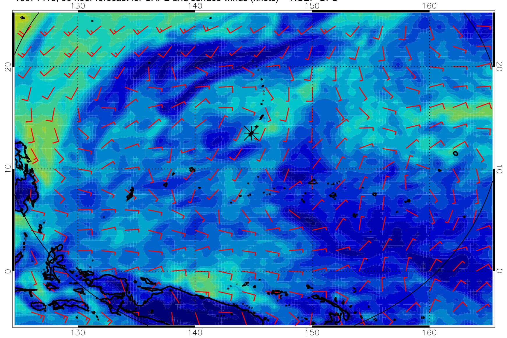
16071418, 90 hour forecast for CAPE and surface winds (knots) -- NCEP GFS
