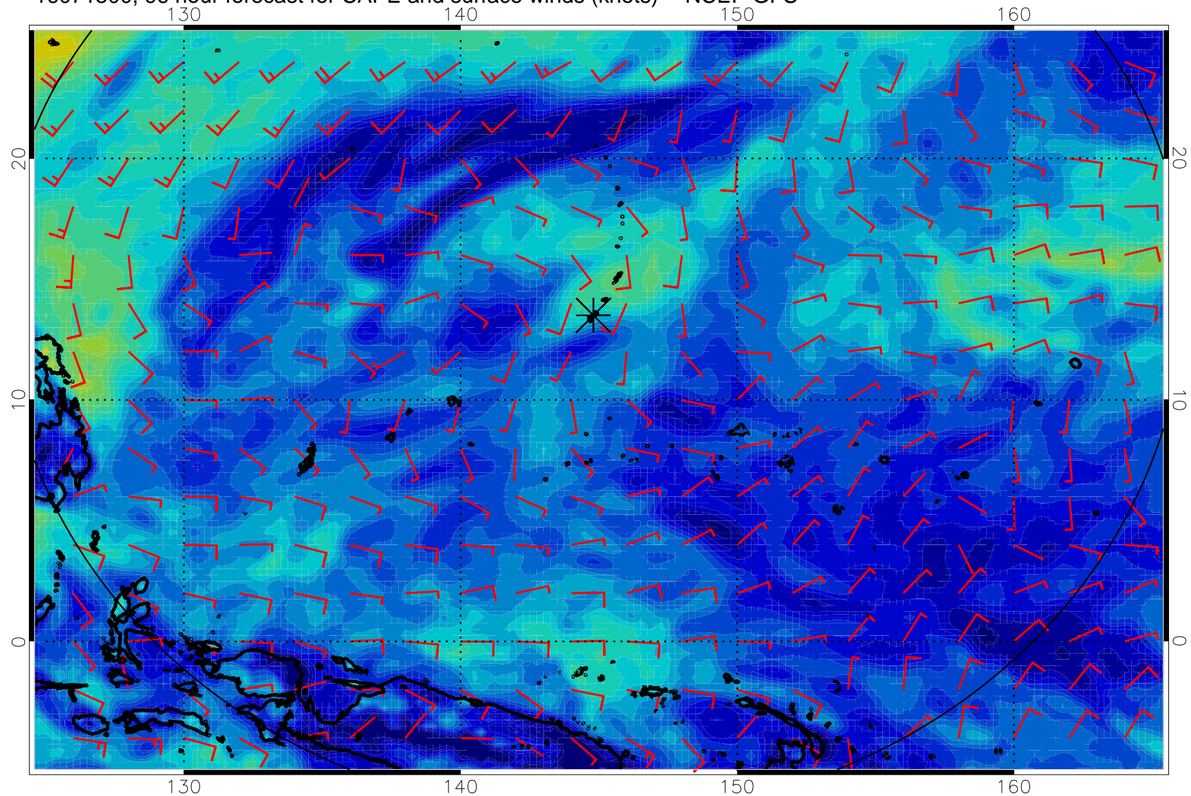
16071500, 96 hour forecast for CAPE and surface winds (knots) -- NCEP GFS
