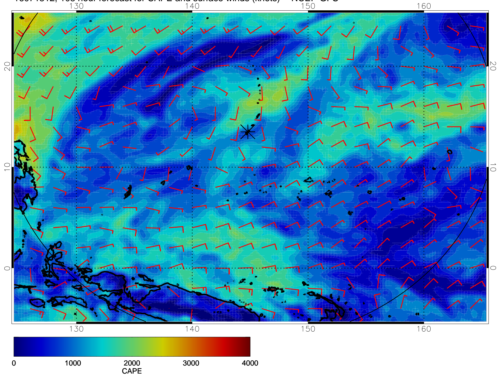
16071512, 108 hour forecast for CAPE and surface winds (knots) -- NCEP GFS
