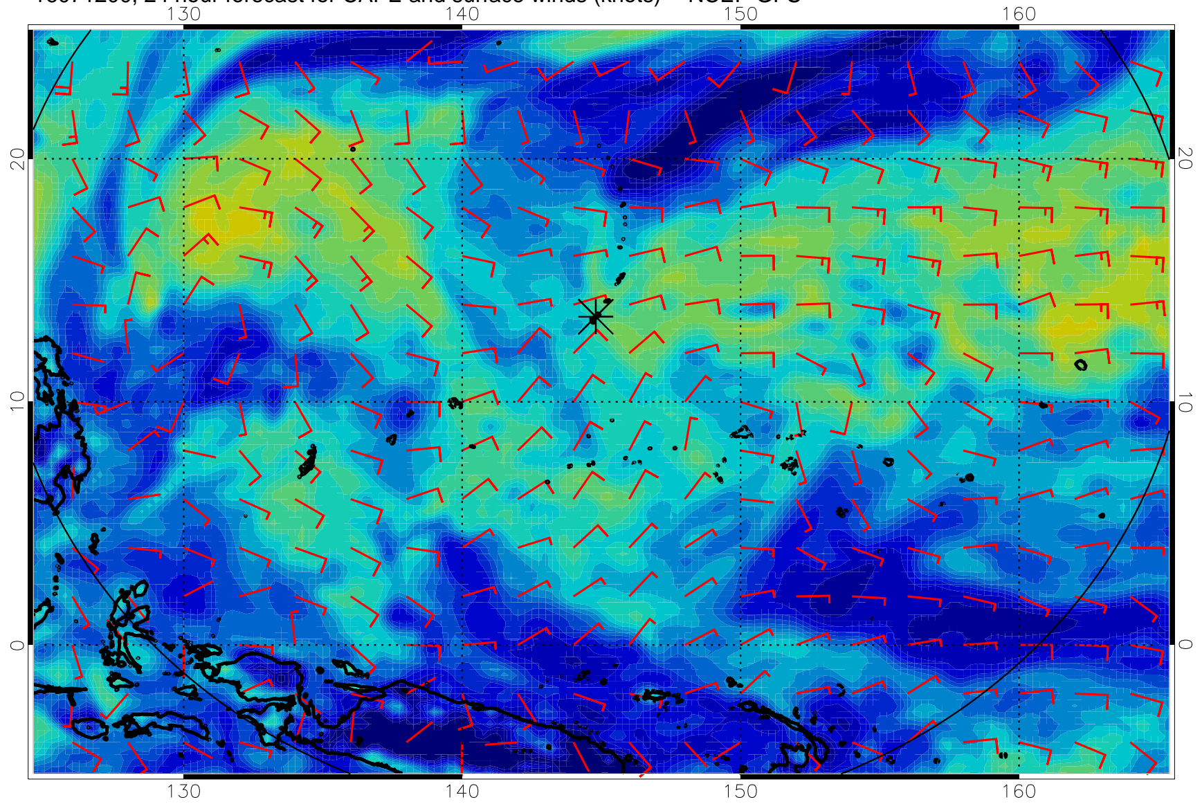
16071200, 24 hour forecast for CAPE and surface winds (knots) -- NCEP GFS
