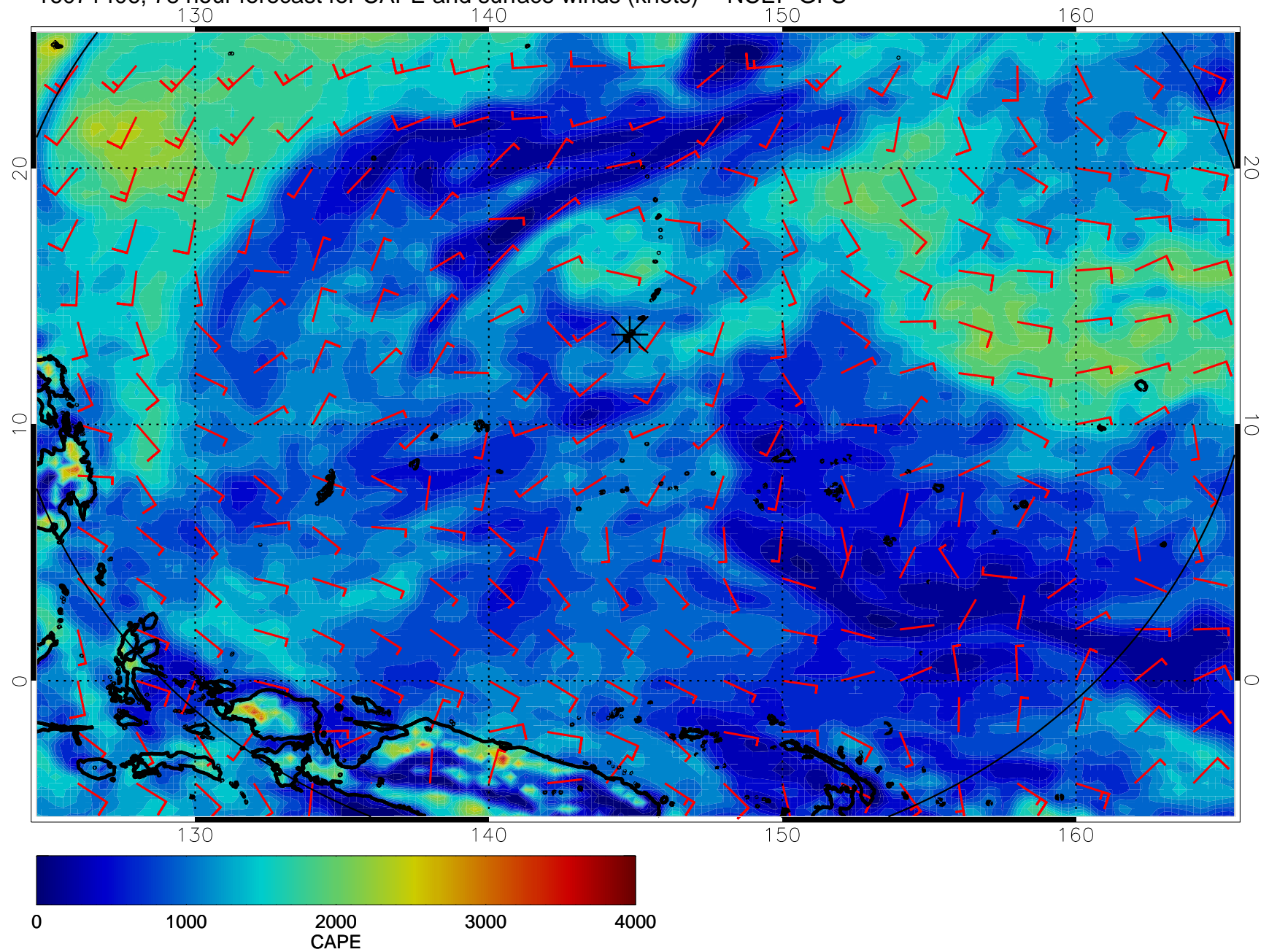
16071406, 78 hour forecast for CAPE and surface winds (knots) -- NCEP GFS
