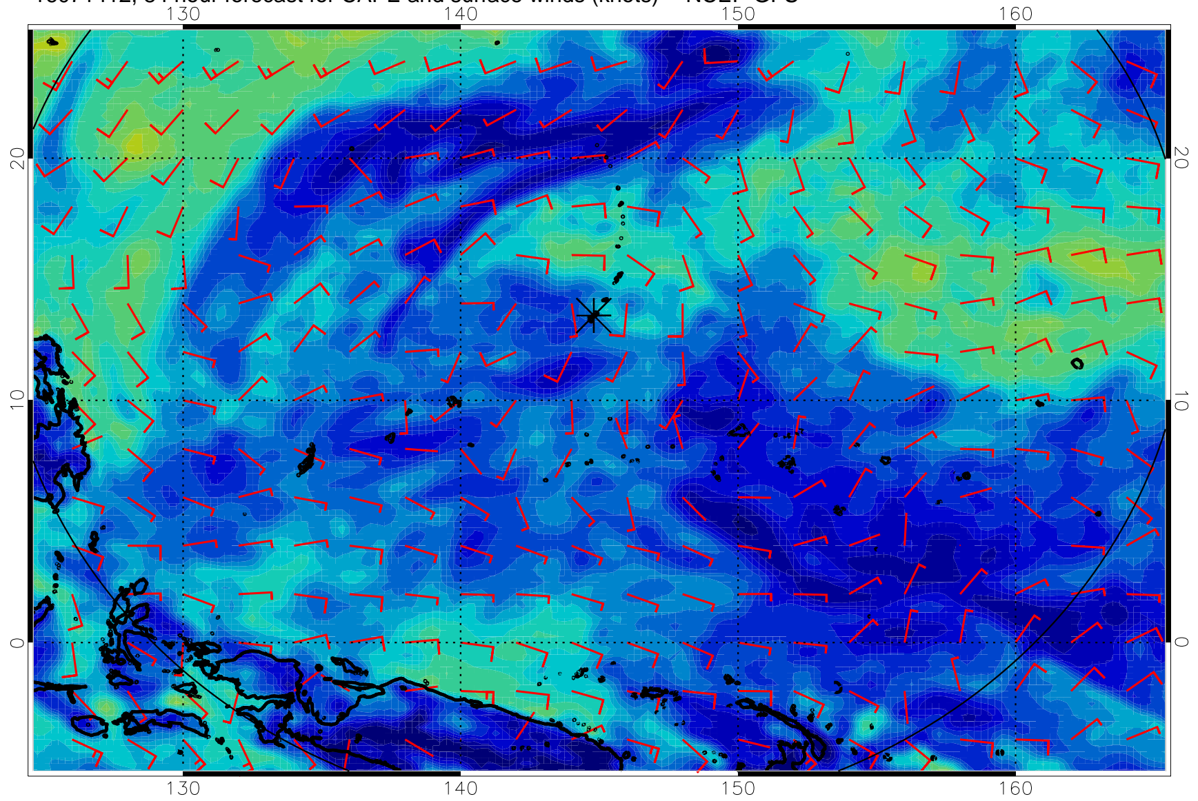
16071412, 84 hour forecast for CAPE and surface winds (knots) -- NCEP GFS
