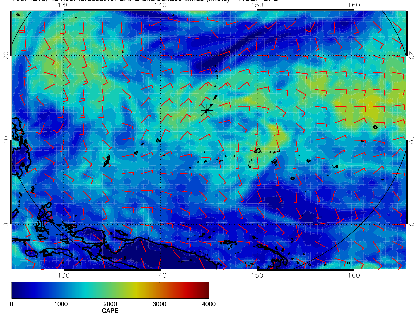
16071218, 42 hour forecast for CAPE and surface winds (knots) -- NCEP GFS
