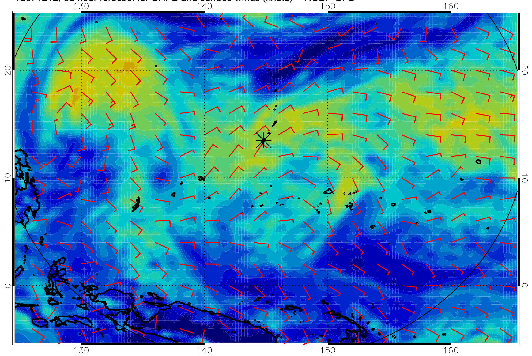
16071212, 36 hour forecast for CAPE and surface winds (knots) -- NCEP GFS
