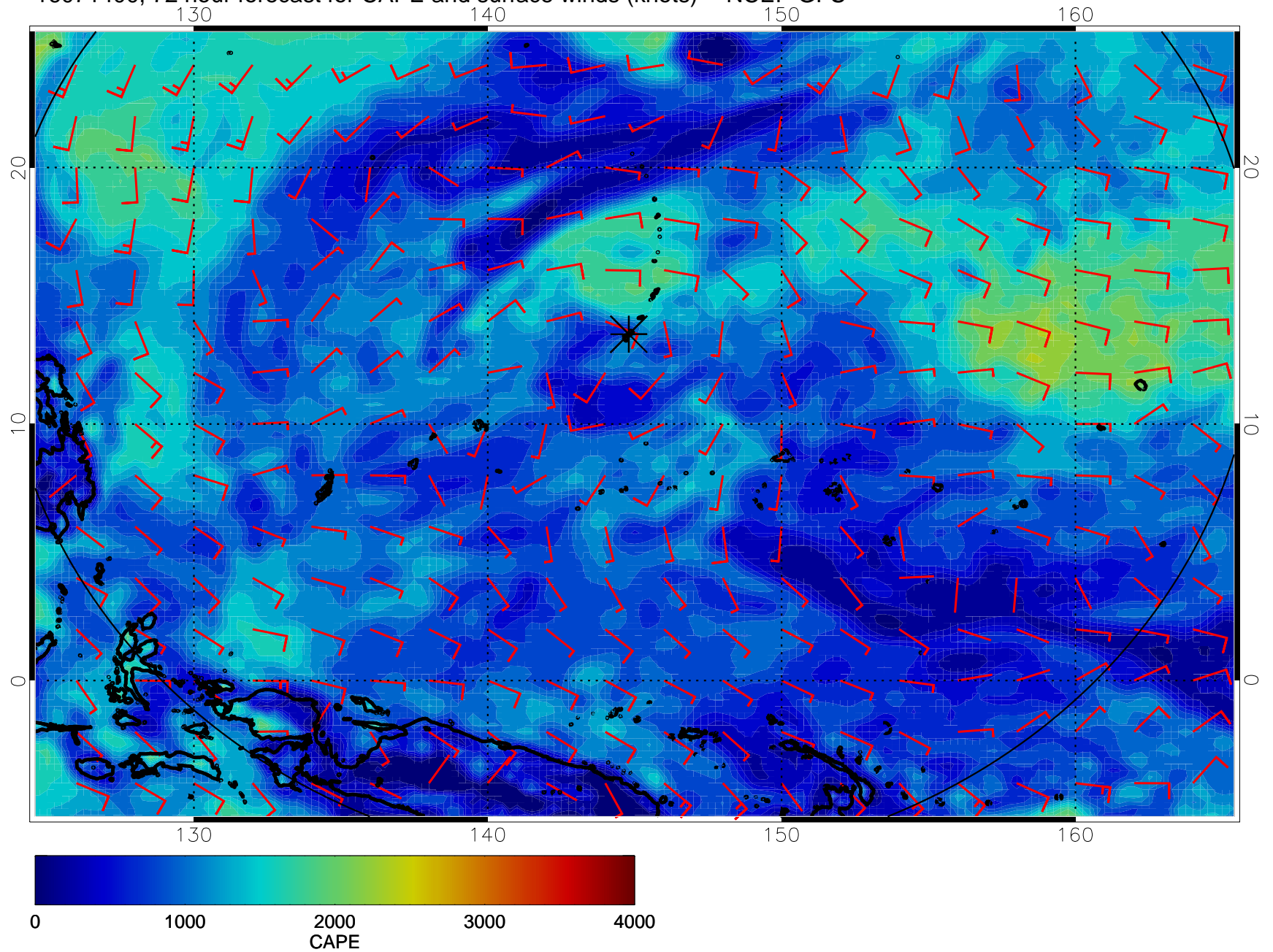
16071400, 72 hour forecast for CAPE and surface winds (knots) -- NCEP GFS
