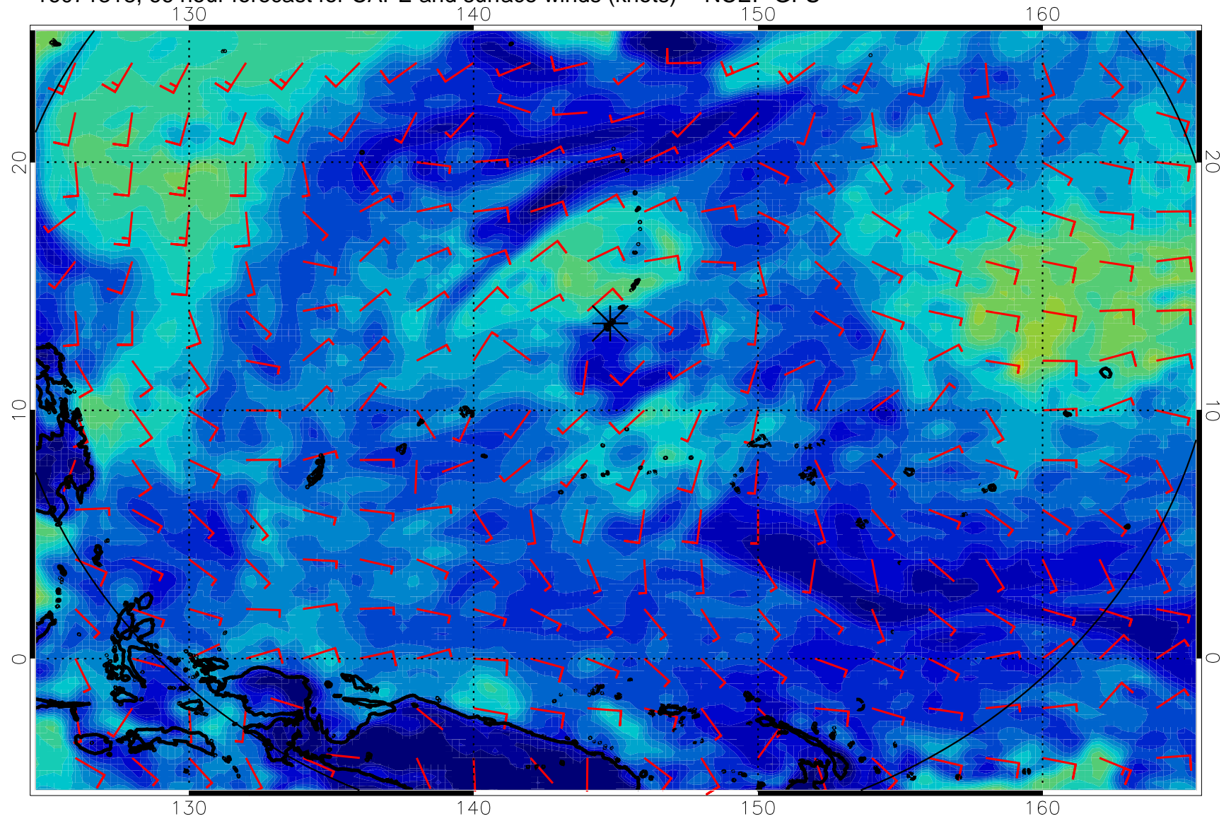
16071318, 66 hour forecast for CAPE and surface winds (knots) -- NCEP GFS
