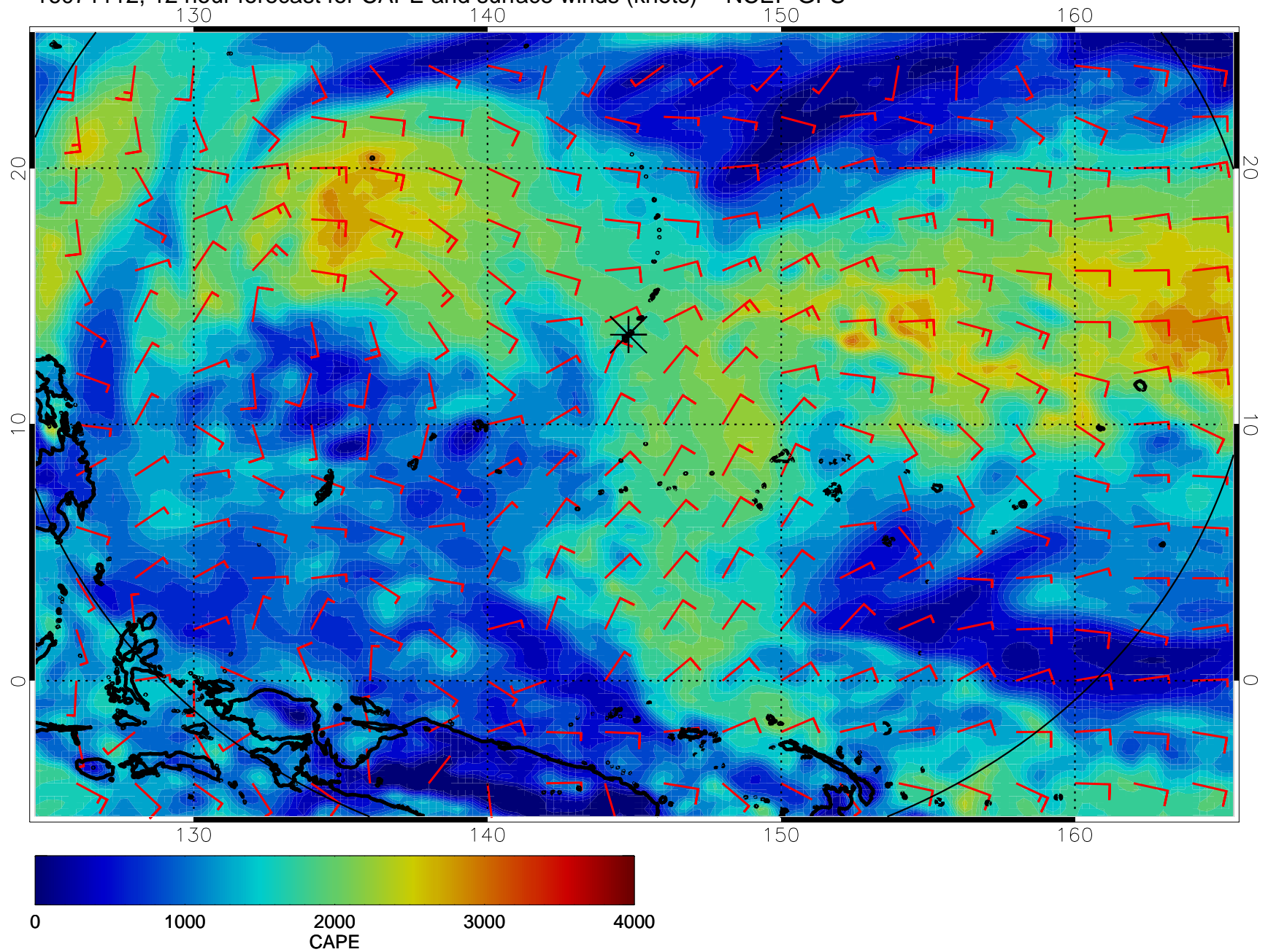
16071112, 12 hour forecast for CAPE and surface winds (knots) -- NCEP GFS
