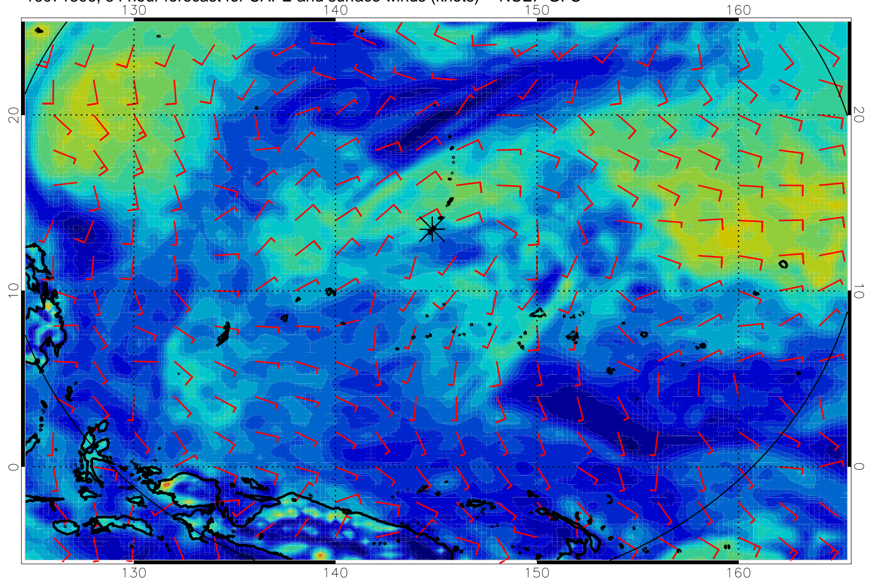
16071306, 54 hour forecast for CAPE and surface winds (knots) -- NCEP GFS
