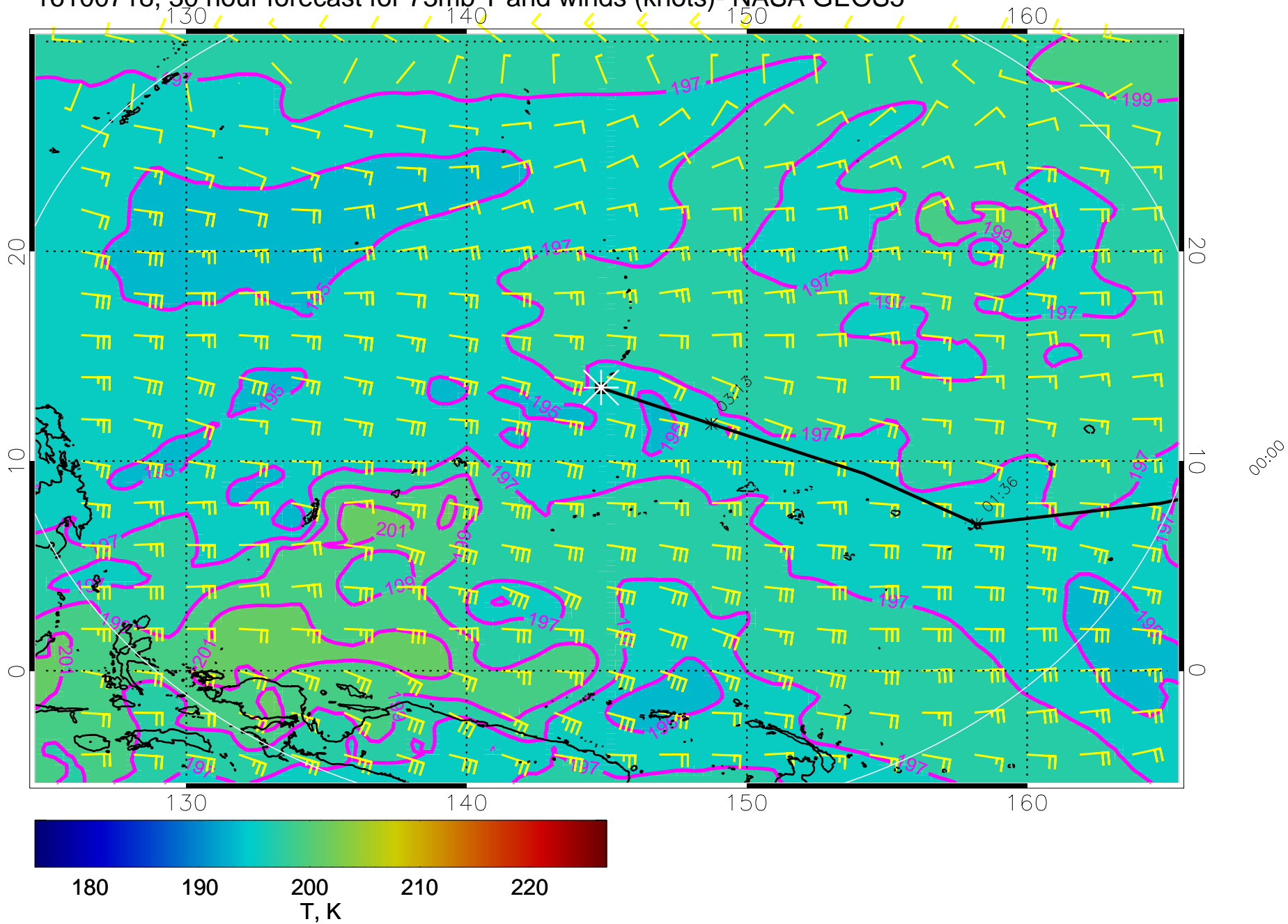
16100718, 30 hour forecast for 73mb T and winds (knots)- NASA GEOS5
