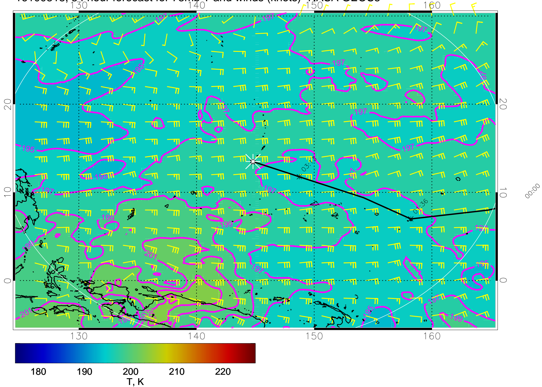
16100818, 54 hour forecast for 73mb T and winds (knots)- NASA GEOS5
