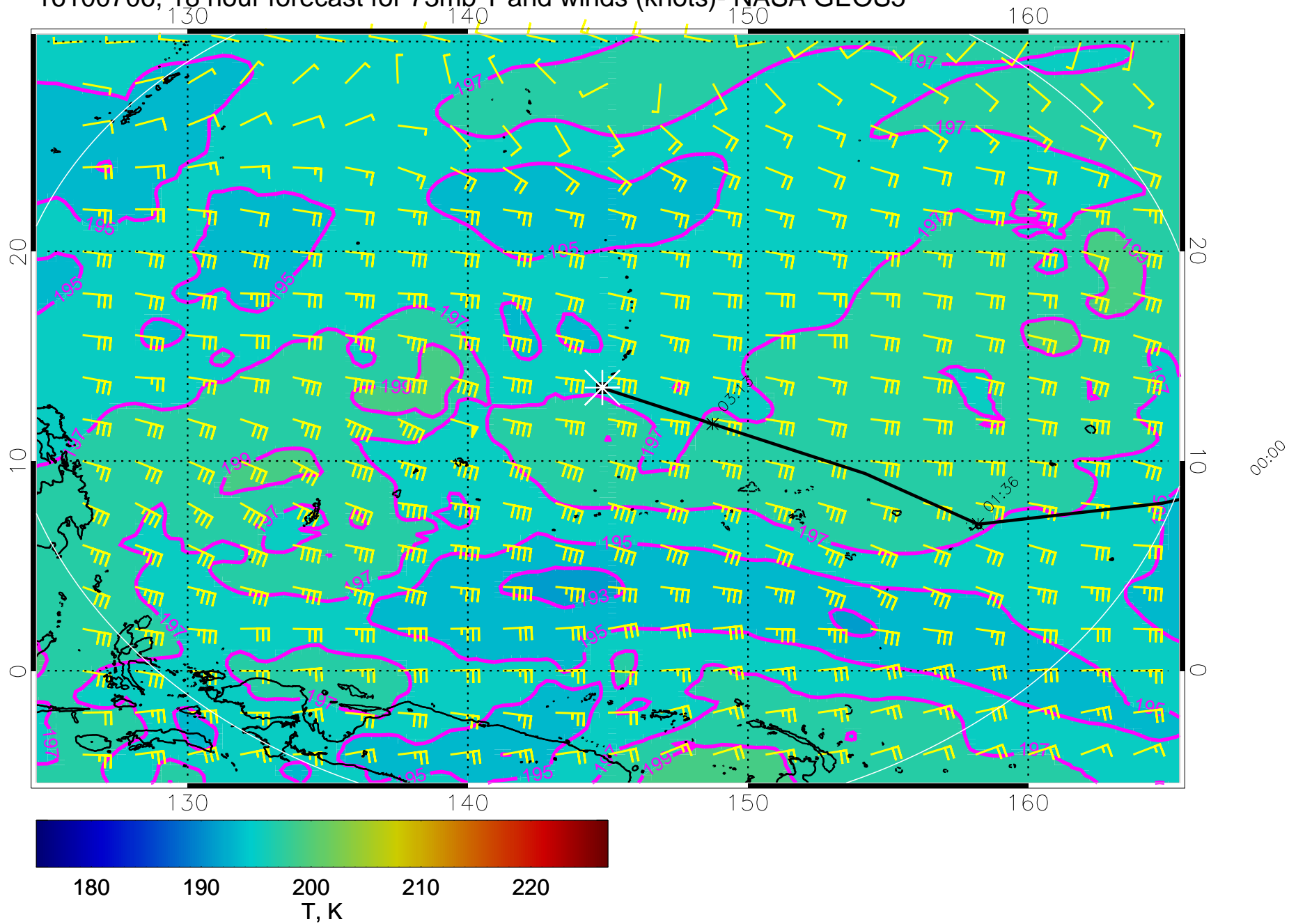
16100706, 18 hour forecast for 73mb T and winds (knots)- NASA GEOS5
