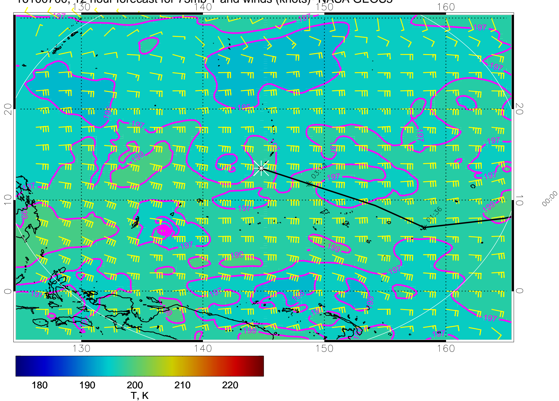
16100700, 12 hour forecast for 73mb T and winds (knots)- NASA GEOS5
