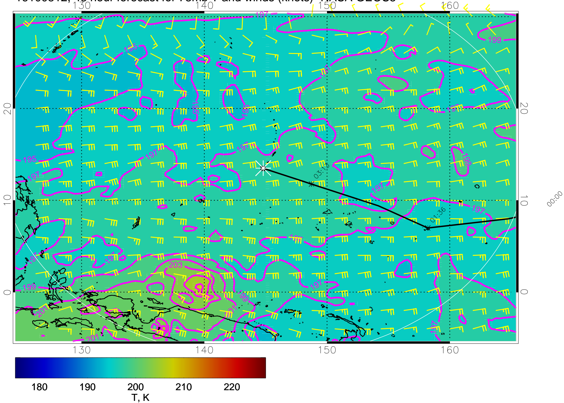
16100812, 48 hour forecast for 73mb T and winds (knots)- NASA GEOS5
