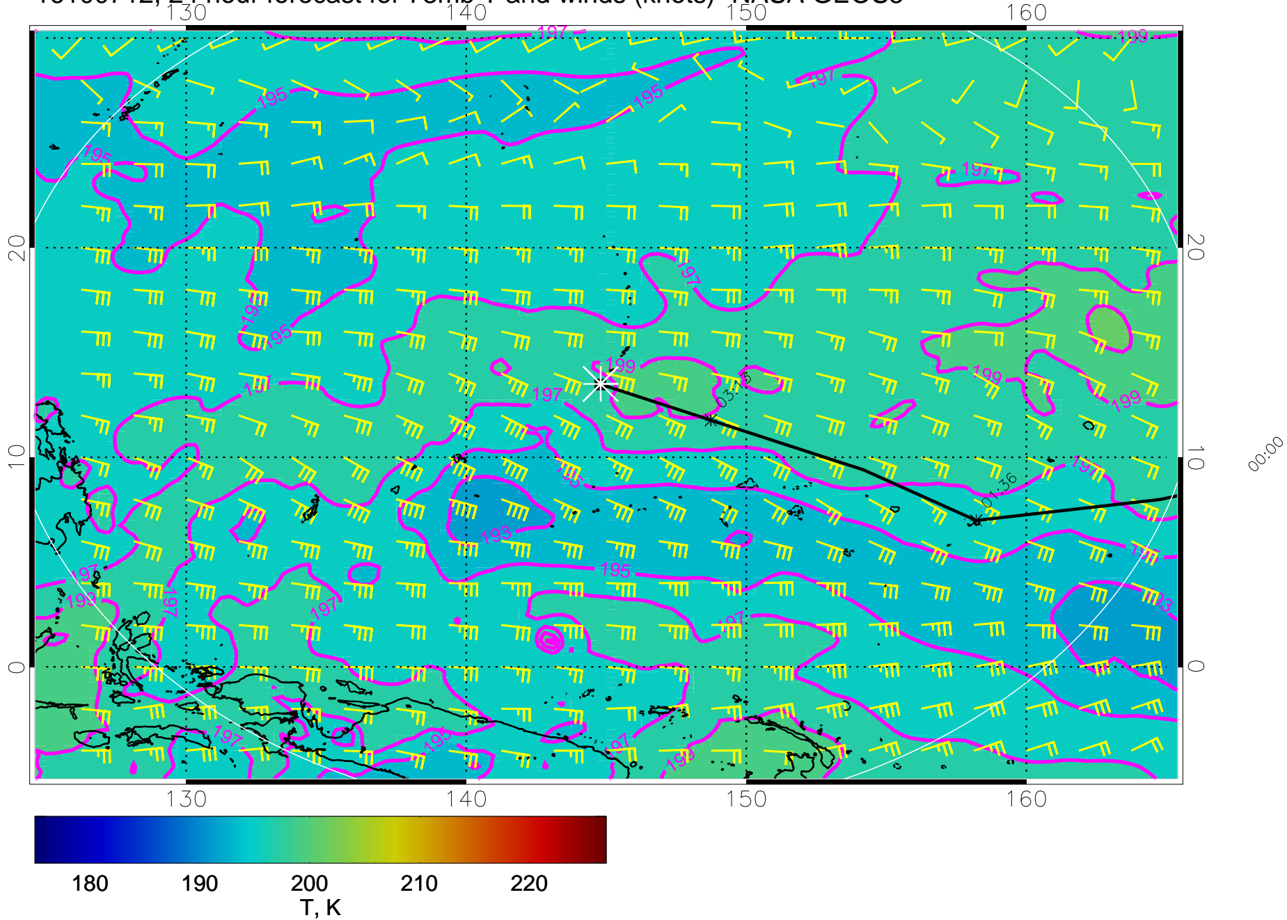
16100712, 24 hour forecast for 73mb T and winds (knots)- NASA GEOS5
