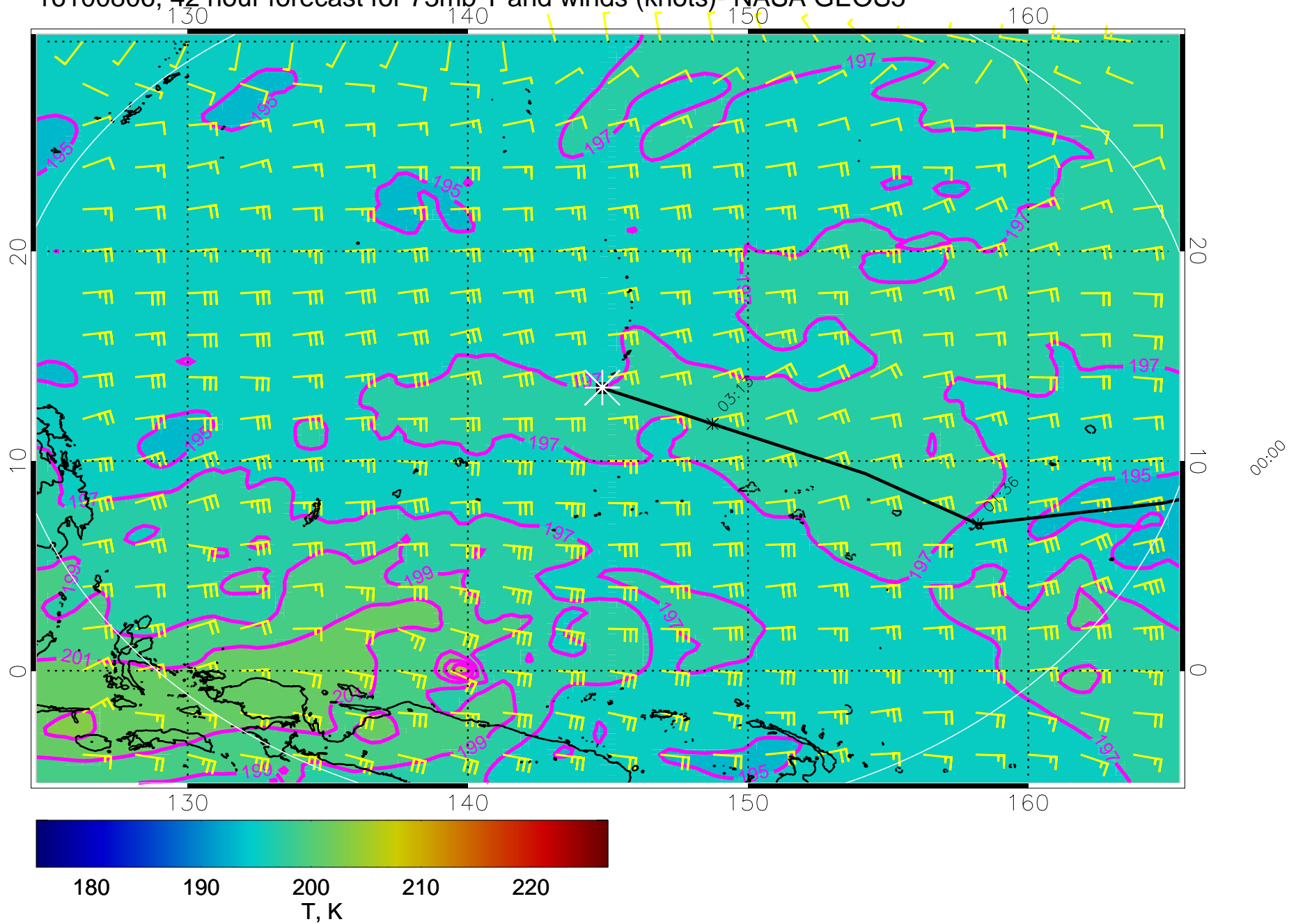
16100806, 42 hour forecast for 73mb T and winds (knots)- NASA GEOS5
