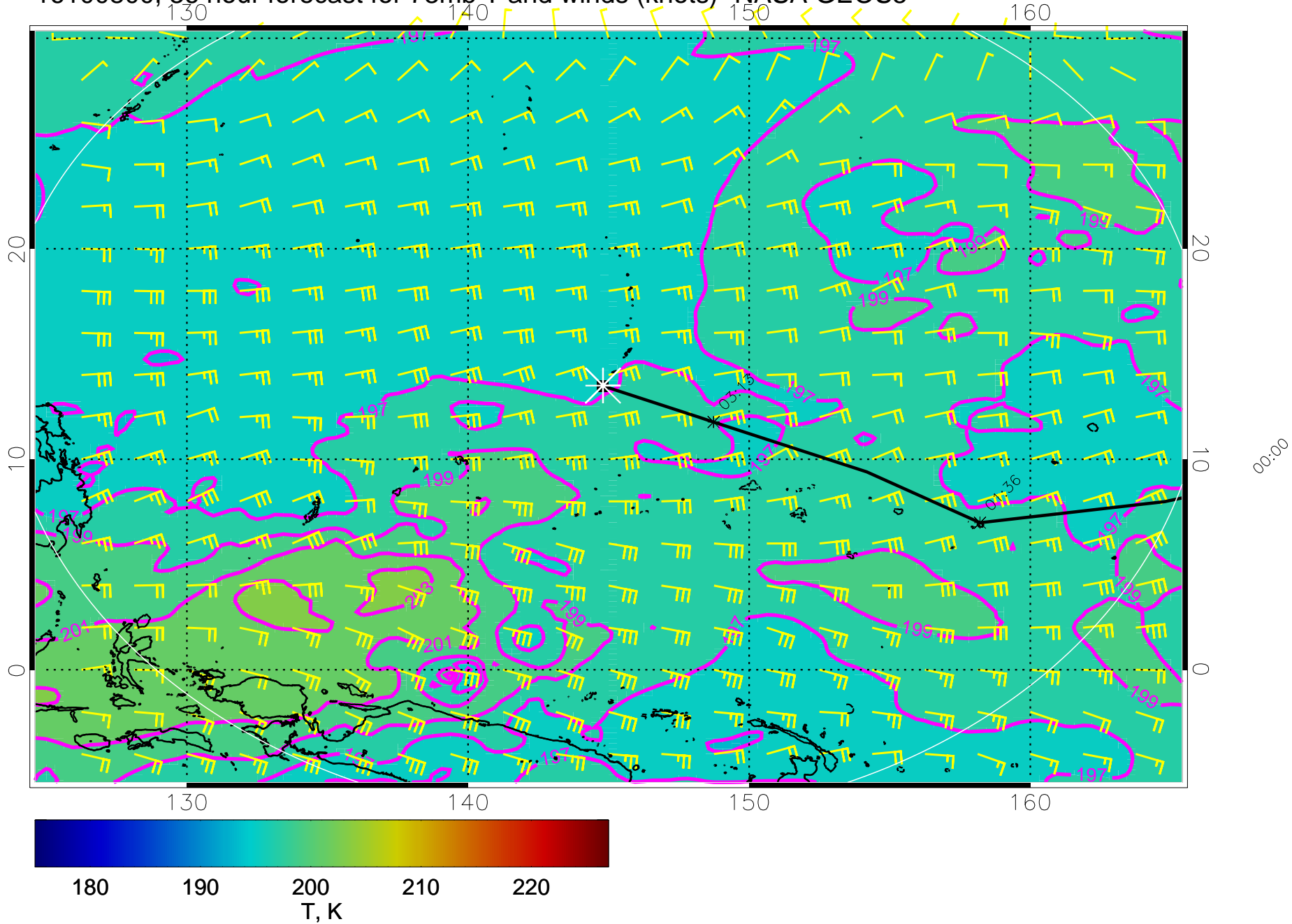
16100800, 36 hour forecast for 73mb T and winds (knots)- NASA GEOS5
