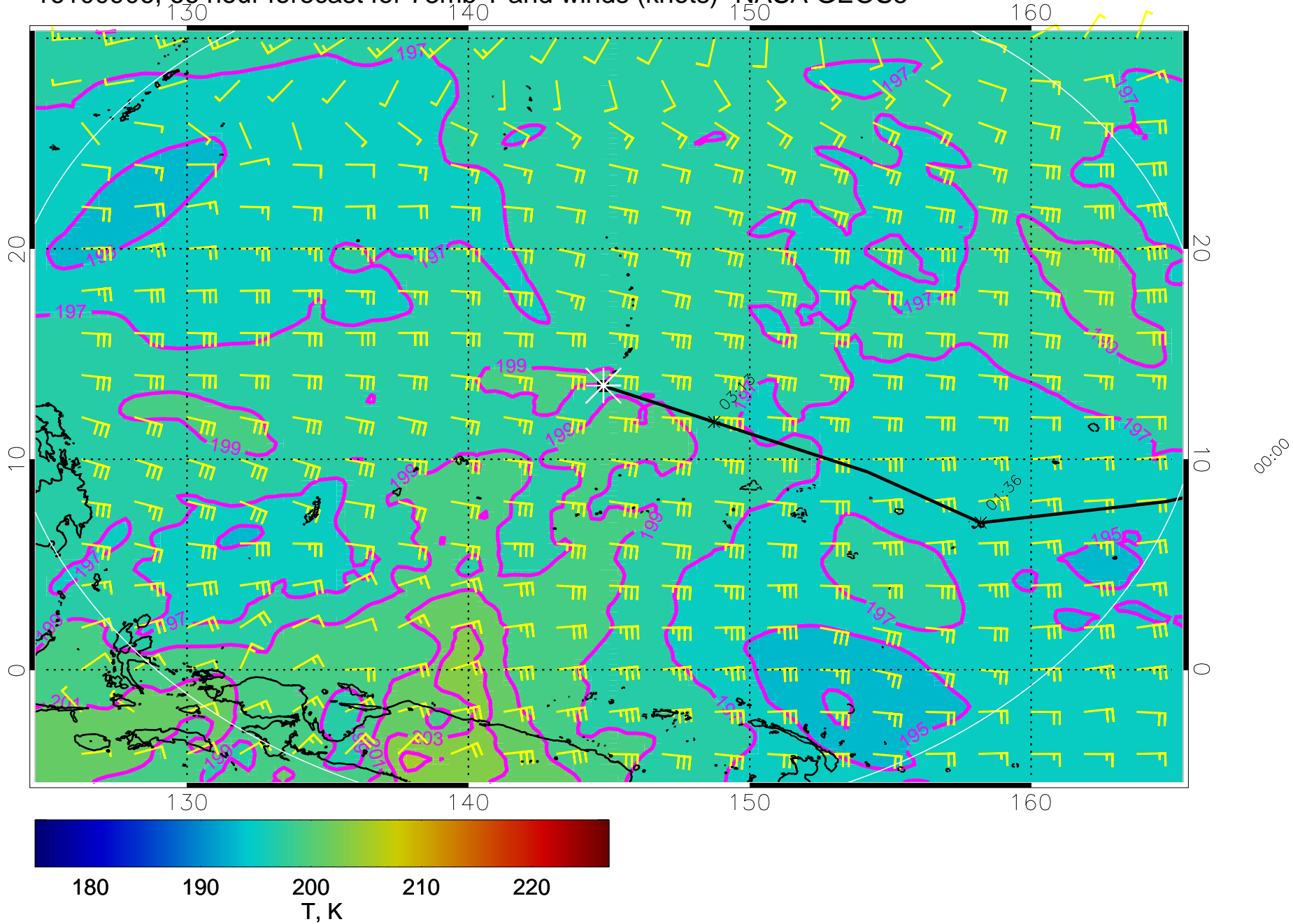
16100906, 66 hour forecast for 73mb T and winds (knots)- NASA GEOS5
