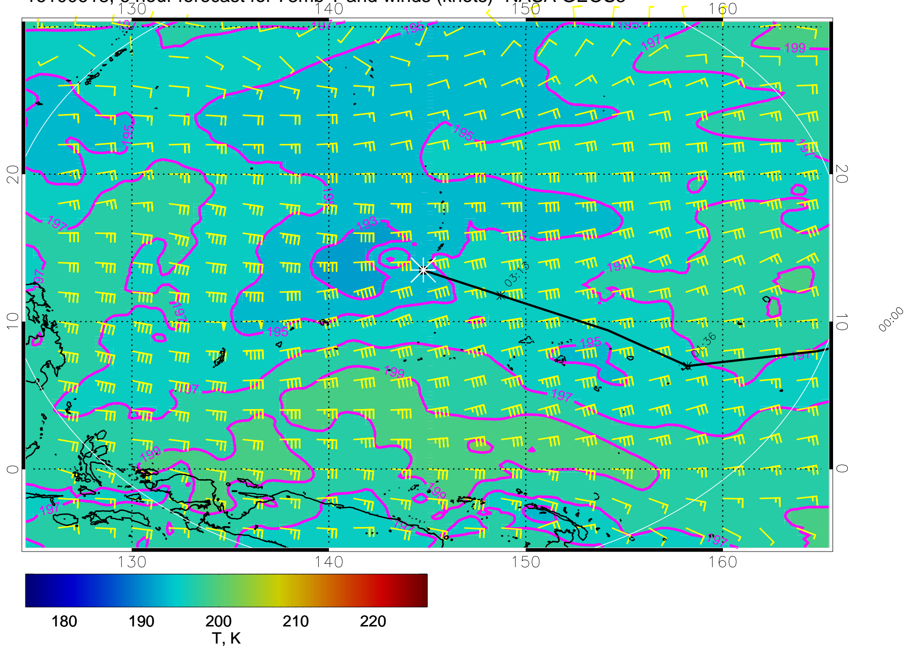
16100618, 6 hour forecast for 73mb T and winds (knots)- NASA GEOS5
