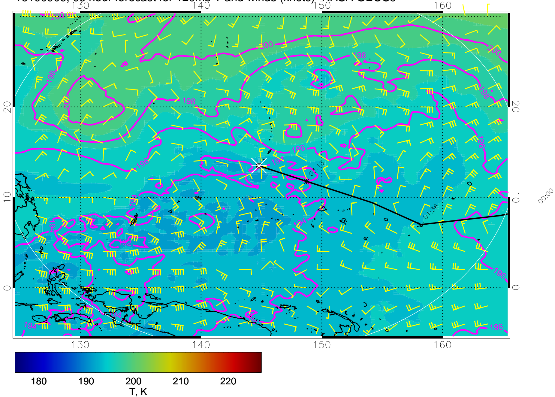
16100906, 66 hour forecast for 120mb T and winds (knots)- NASA GEOS5
