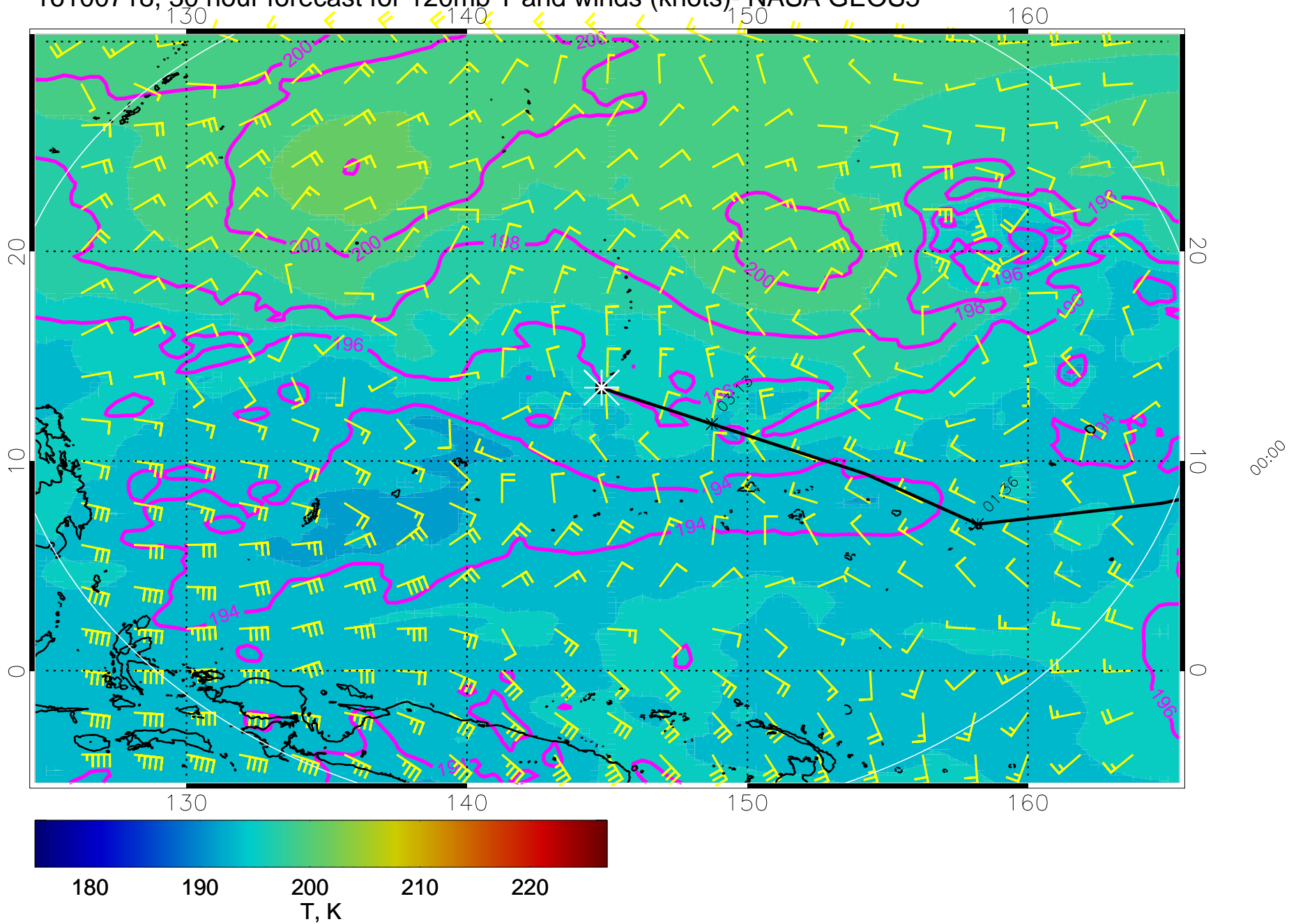
16100718, 30 hour forecast for 120mb T and winds (knots)- NASA GEOS5
