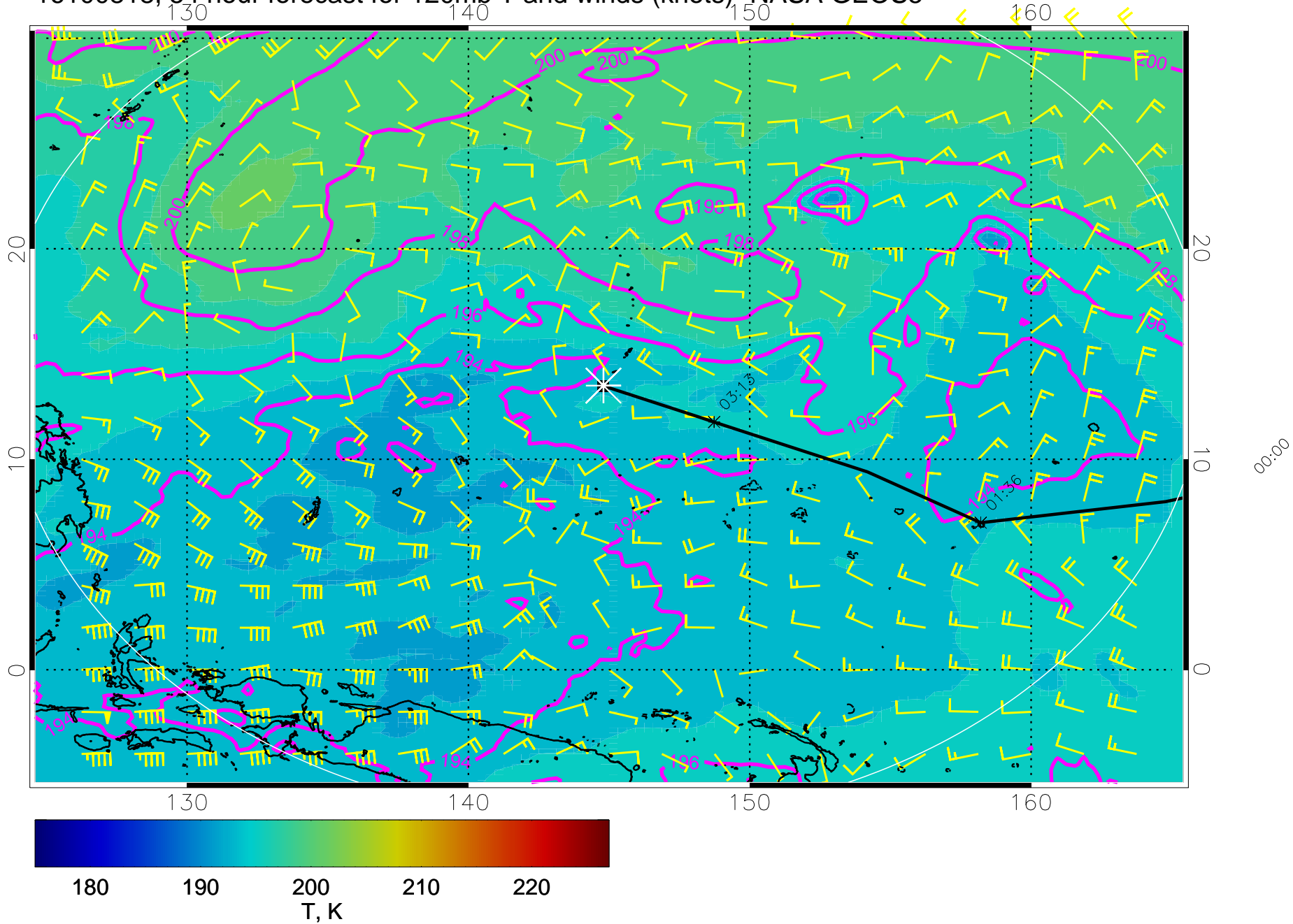
16100818, 54 hour forecast for 120mb T and winds (knots)- NASA GEOS5
