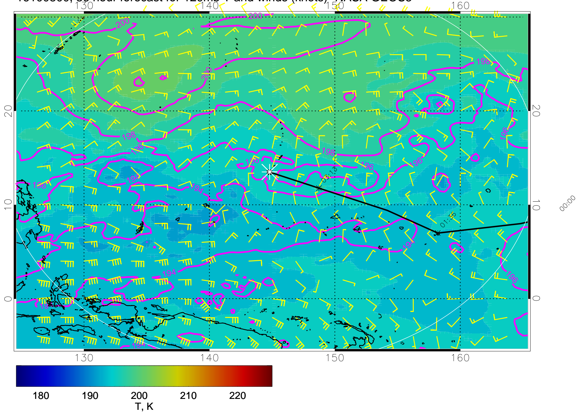
16100800, 36 hour forecast for 120mb T and winds (knots)- NASA GEOS5
