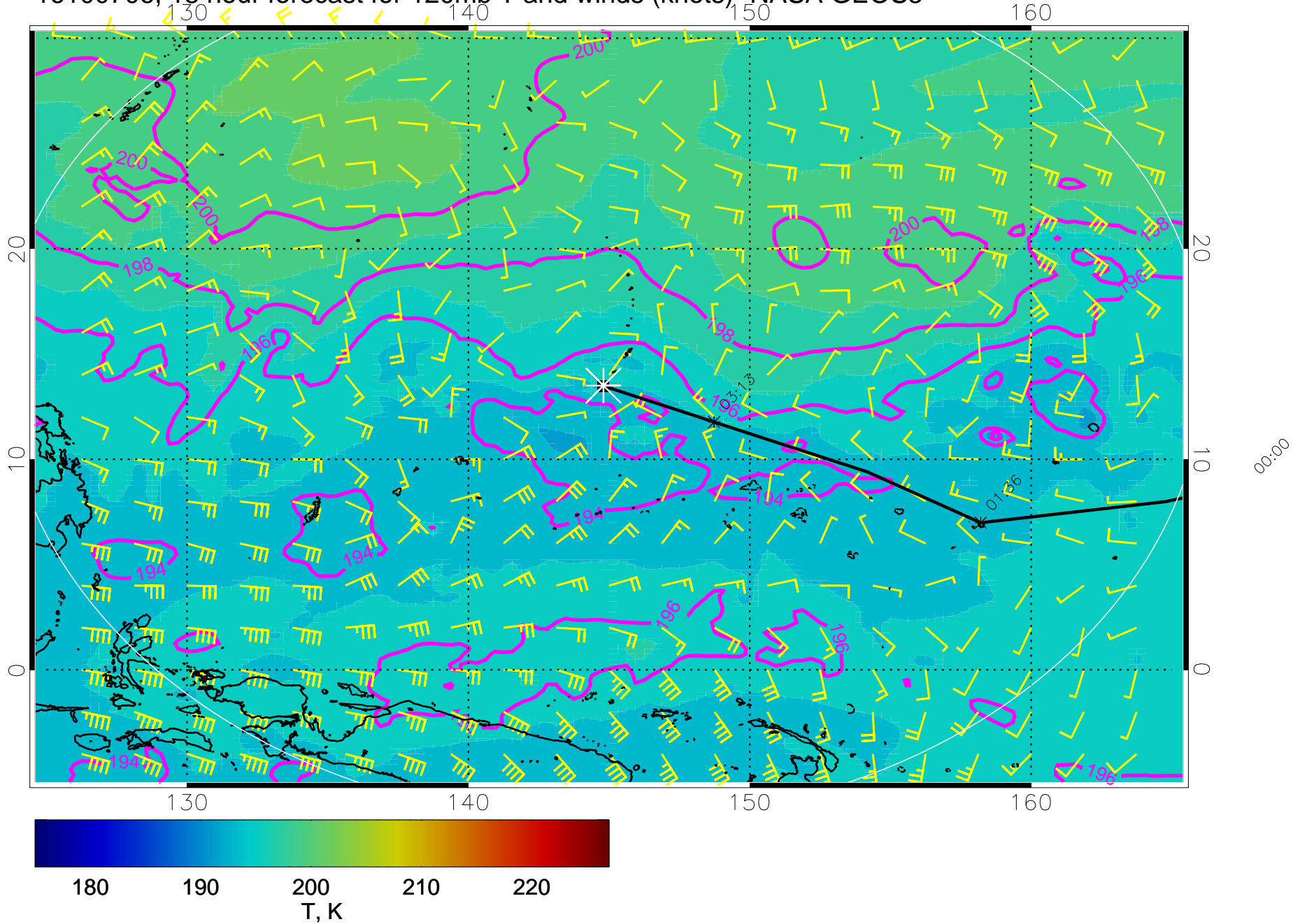
16100706, 18 hour forecast for 120mb T and winds (knots)- NASA GEOS5
