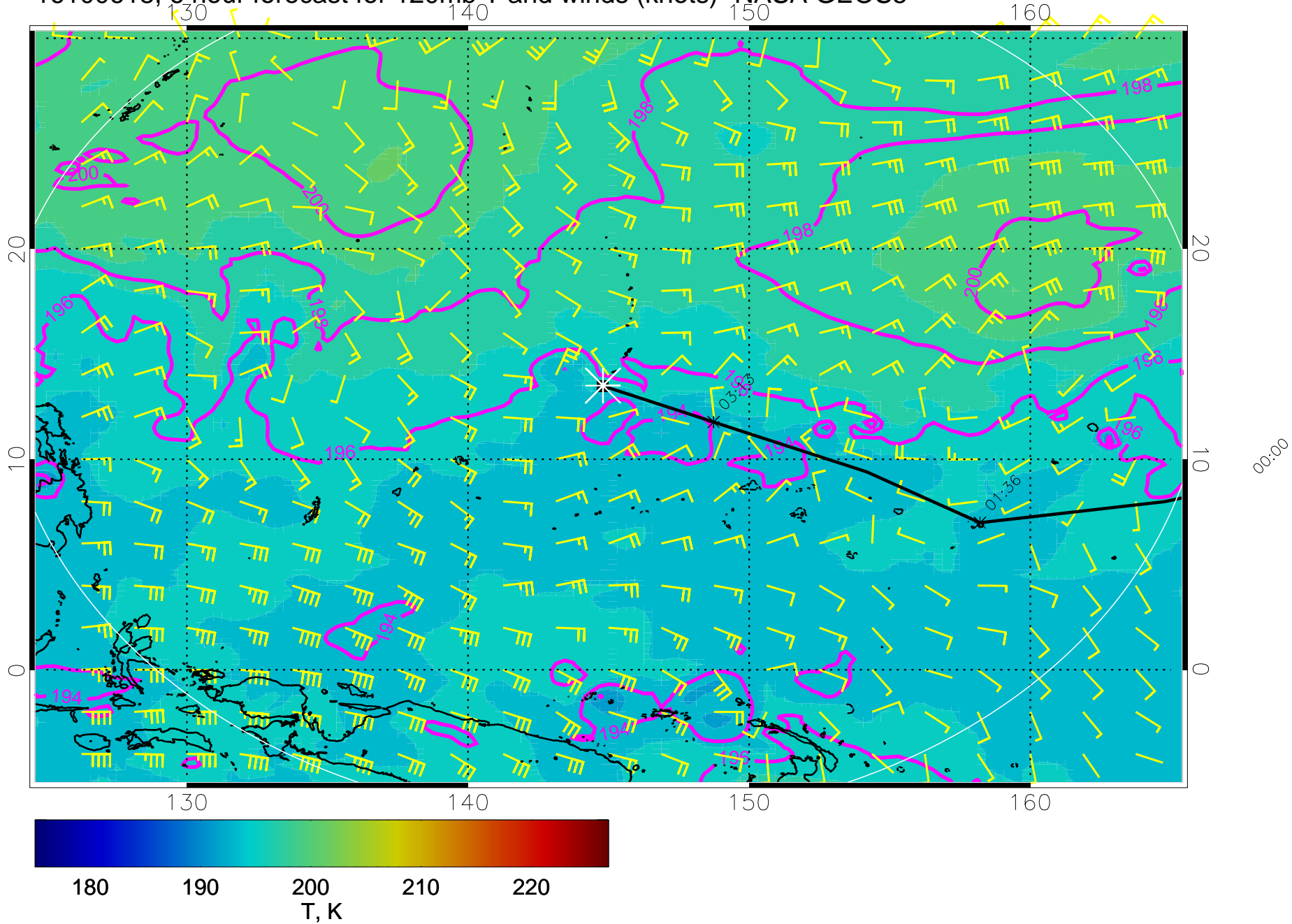
16100618, 6 hour forecast for 120mb T and winds (knots)- NASA GEOS5
