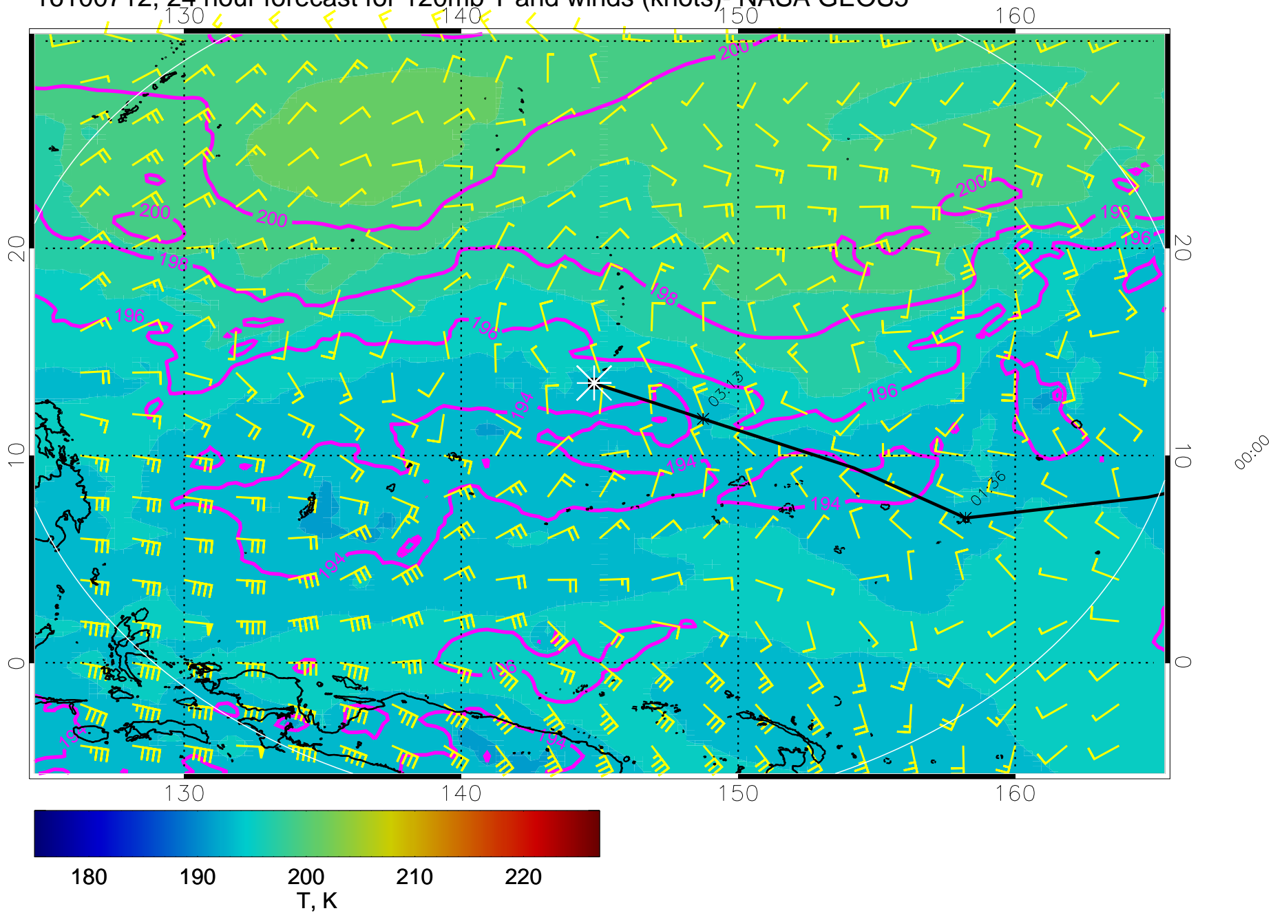
16100712, 24 hour forecast for 120mb T and winds (knots)- NASA GEOS5
