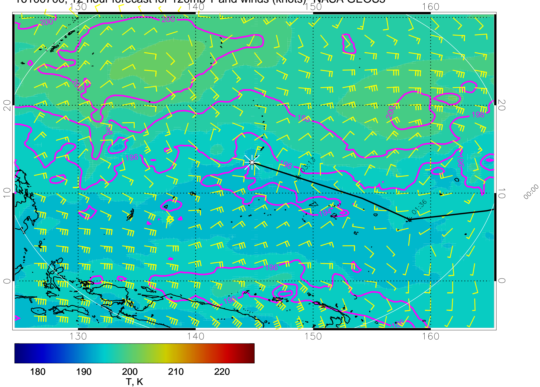
16100700, 12 hour forecast for 120mb T and winds (knots)- NASA GEOS5
