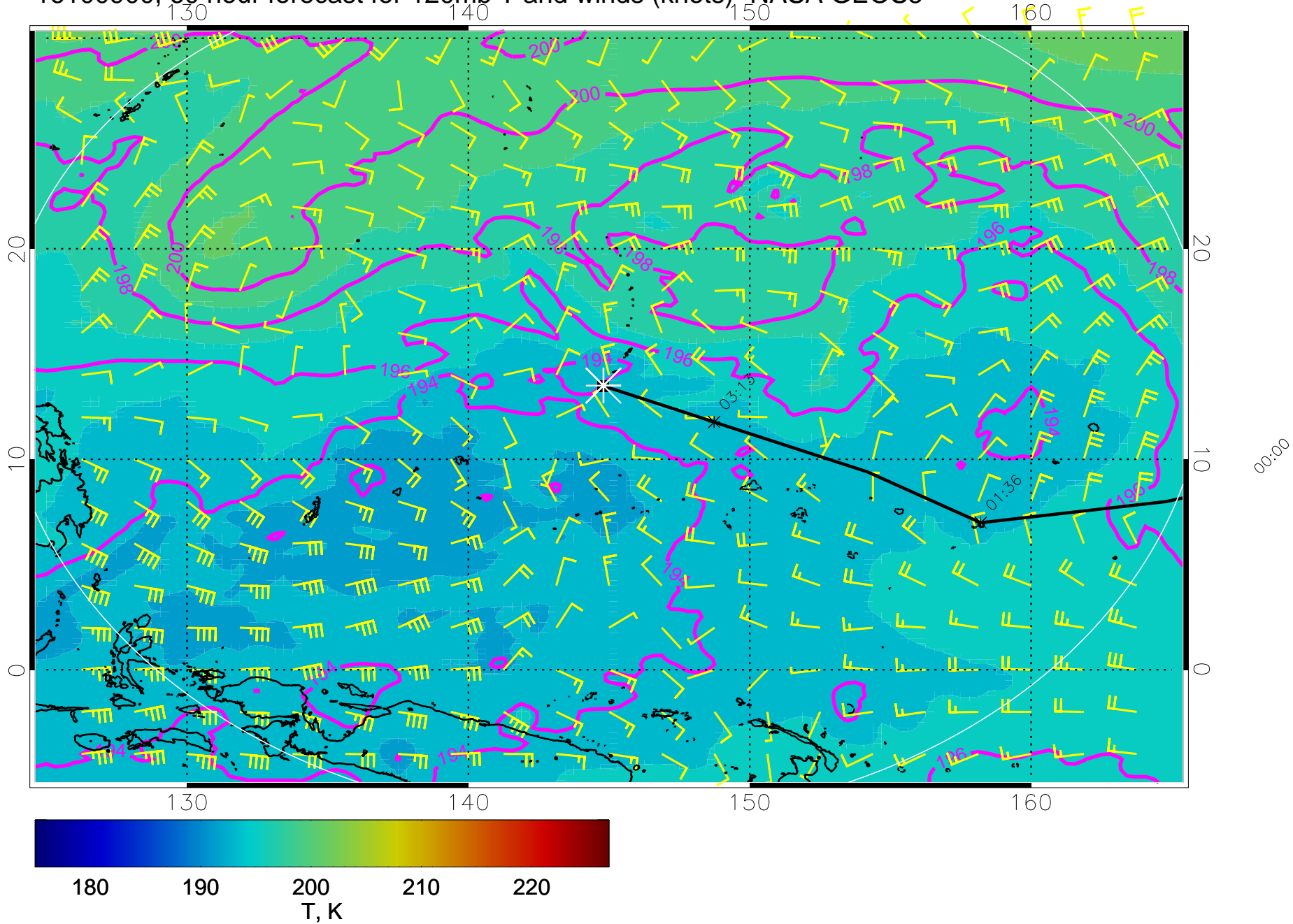
16100900, 60 hour forecast for 120mb T and winds (knots)- NASA GEOS5
