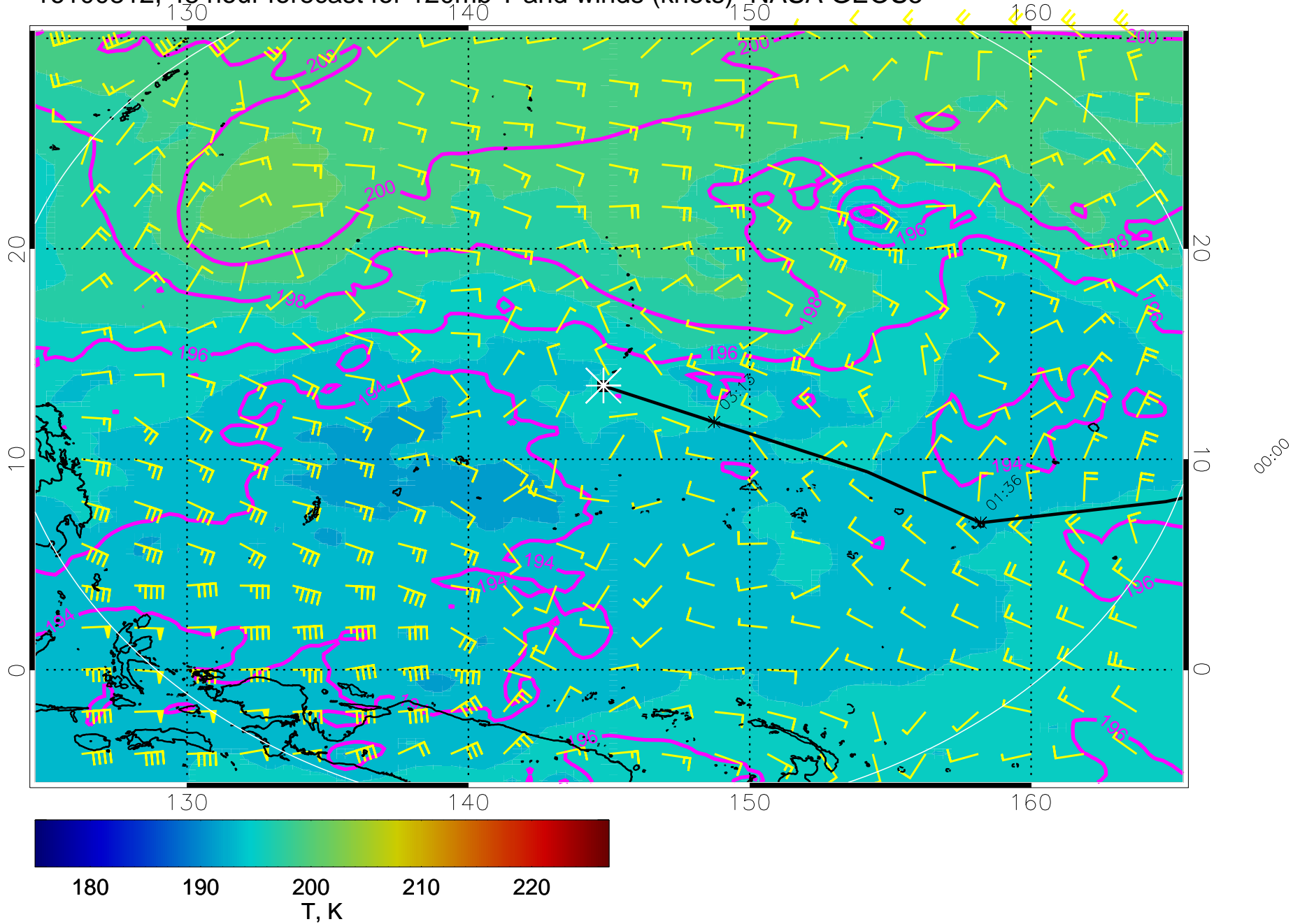
16100812, 48 hour forecast for 120mb T and winds (knots)- NASA GEOS5
