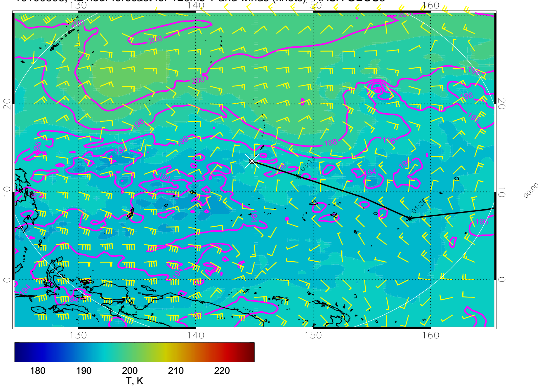
16100806, 42 hour forecast for 120mb T and winds (knots)- NASA GEOS5
