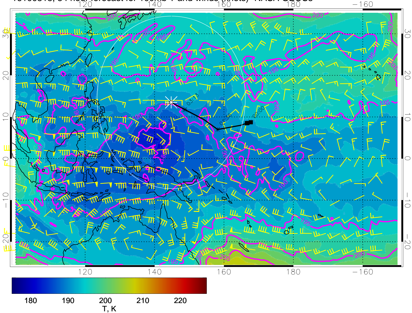
16100818, 54 hour forecast for 100mb T and winds (knots)- NASA GEOS5
