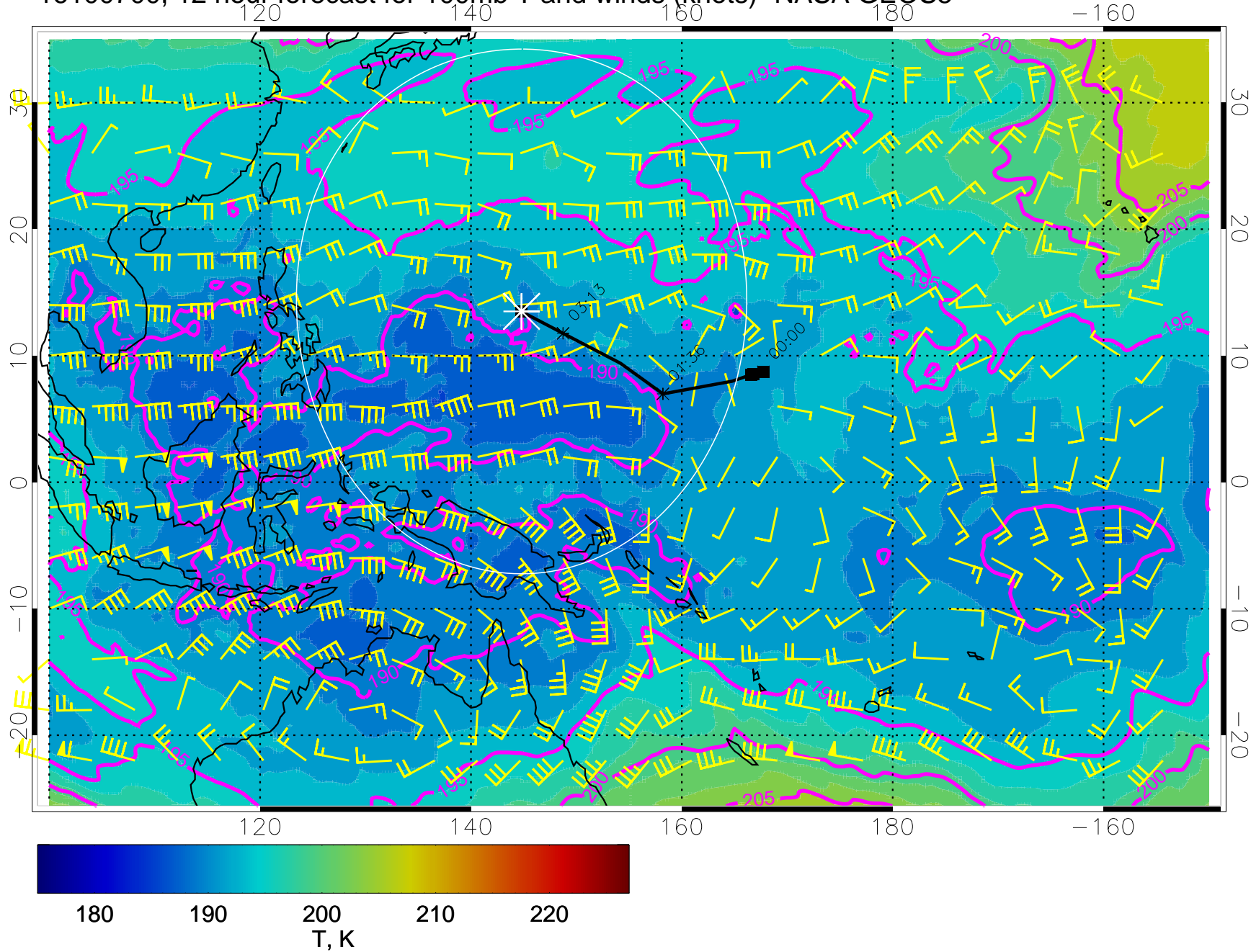
16100700, 12 hour forecast for 100mb T and winds (knots)- NASA GEOS5
