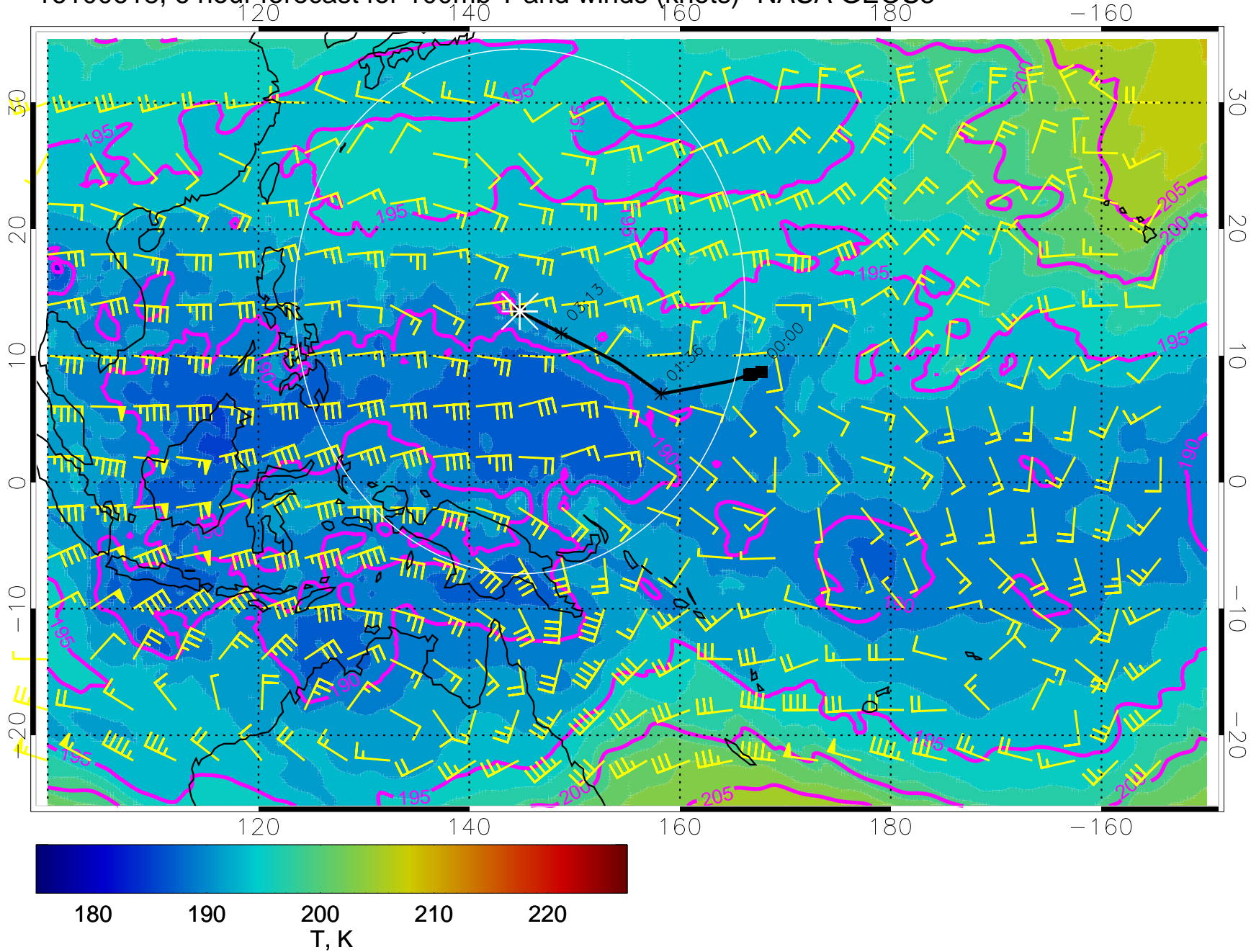
16100618, 6 hour forecast for 100mb T and winds (knots)- NASA GEOS5
