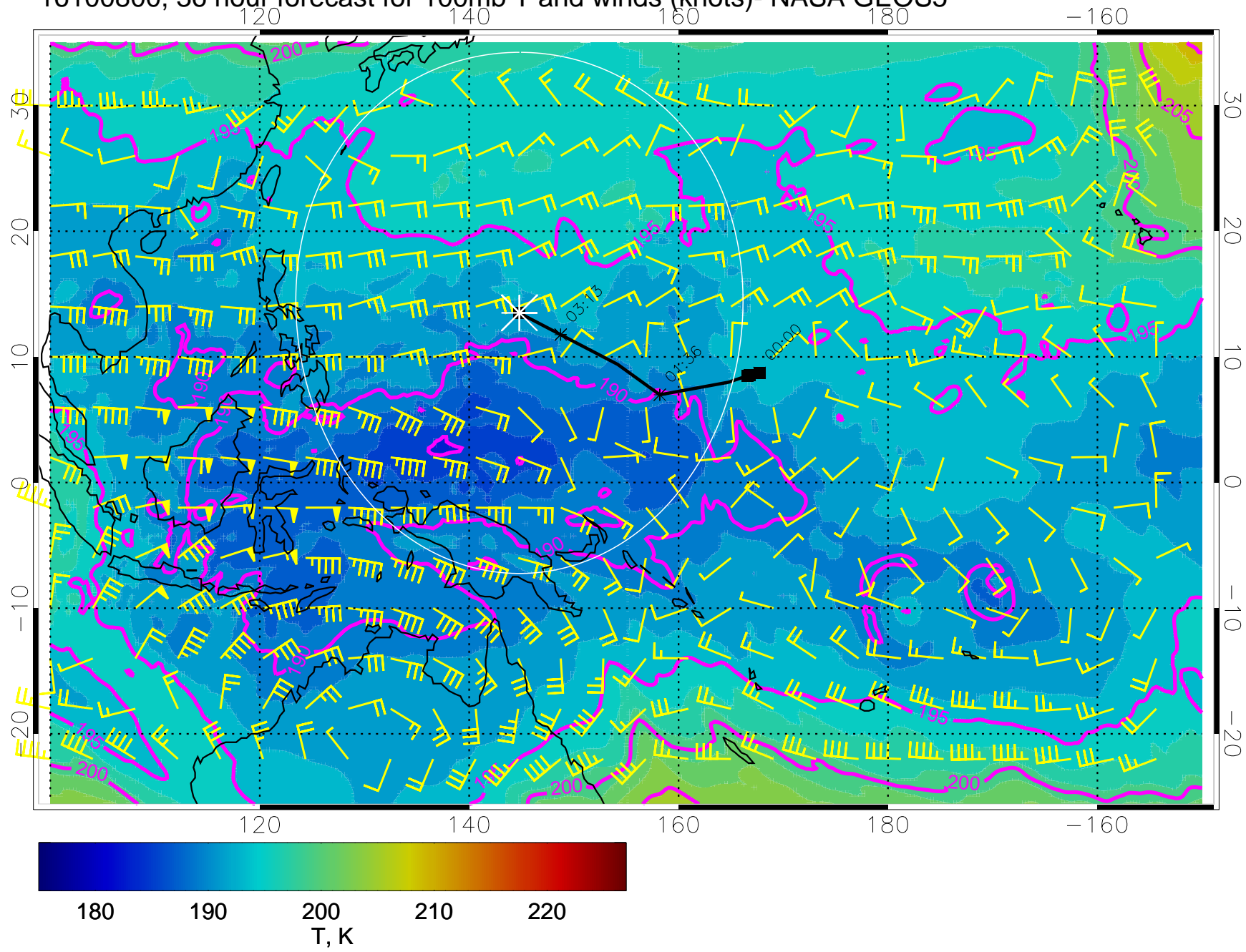
16100800, 36 hour forecast for 100mb T and winds (knots)- NASA GEOS5
