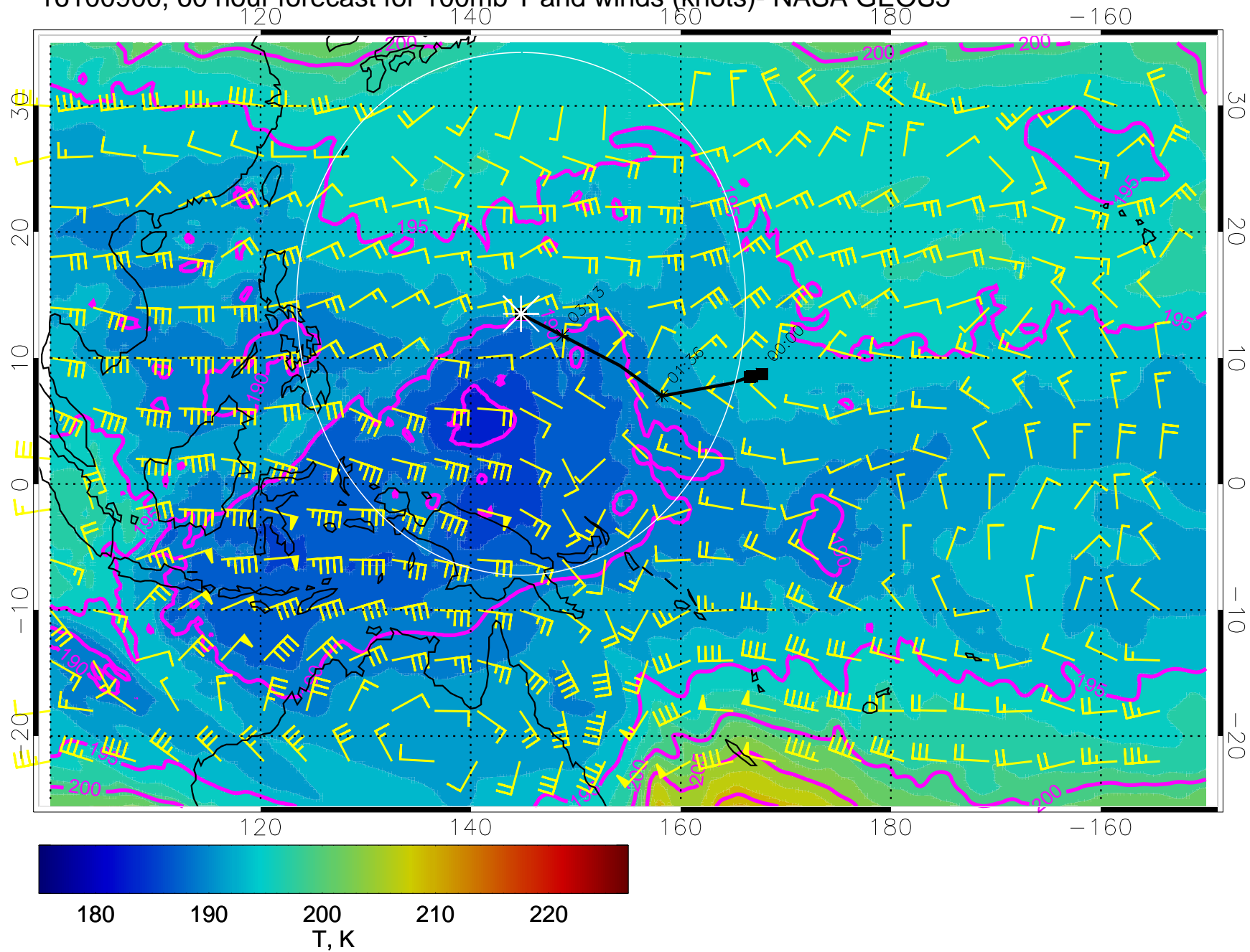
16100900, 60 hour forecast for 100mb T and winds (knots)- NASA GEOS5
