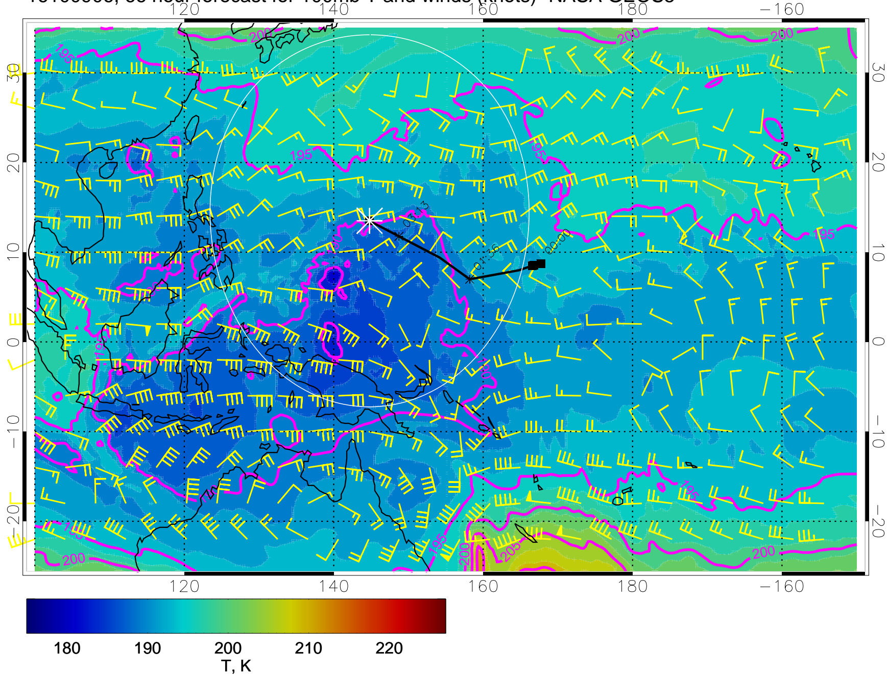
16100906, 66 hour forecast for 100mb T and winds (knots)- NASA GEOS5
