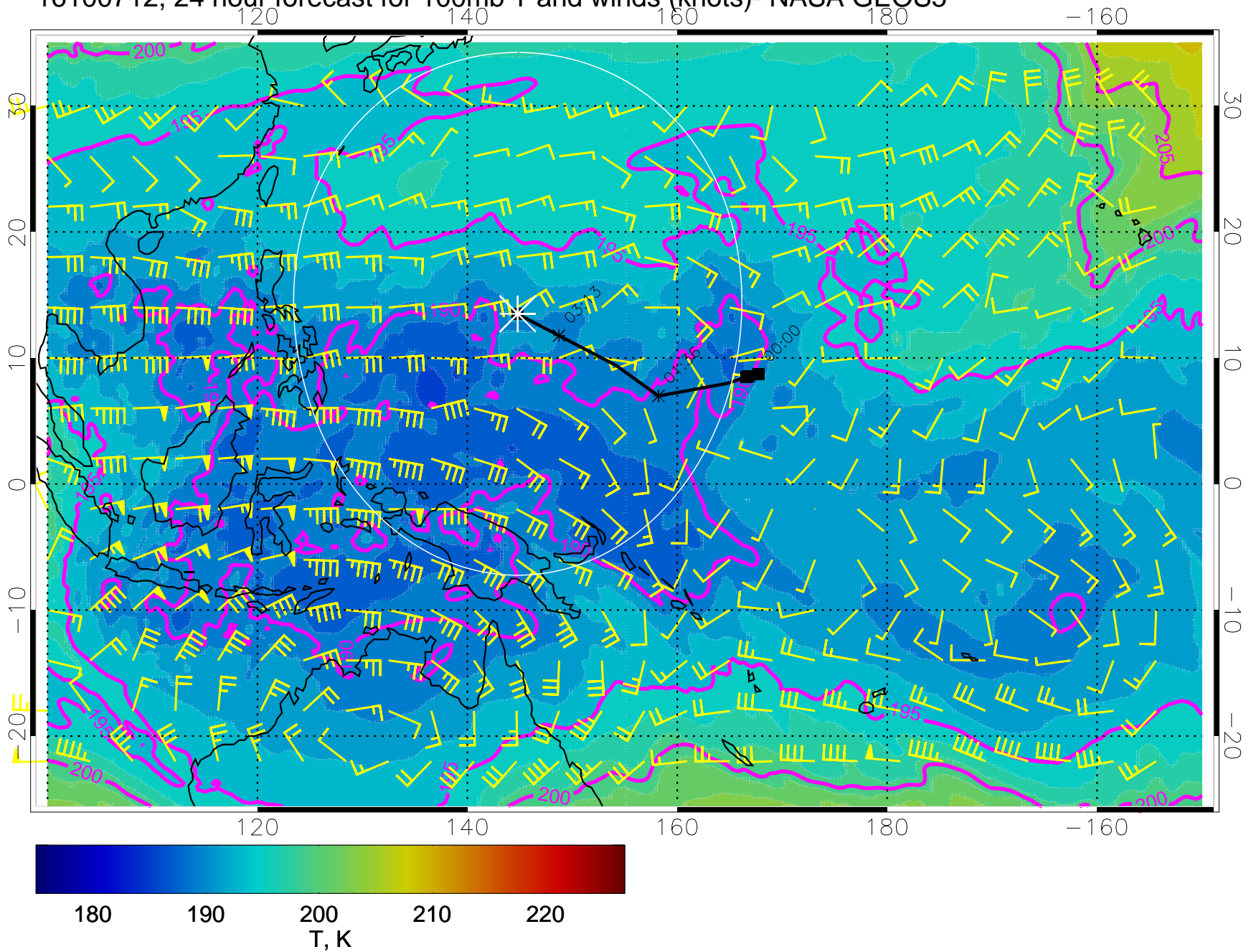
16100712, 24 hour forecast for 100mb T and winds (knots)- NASA GEOS5
