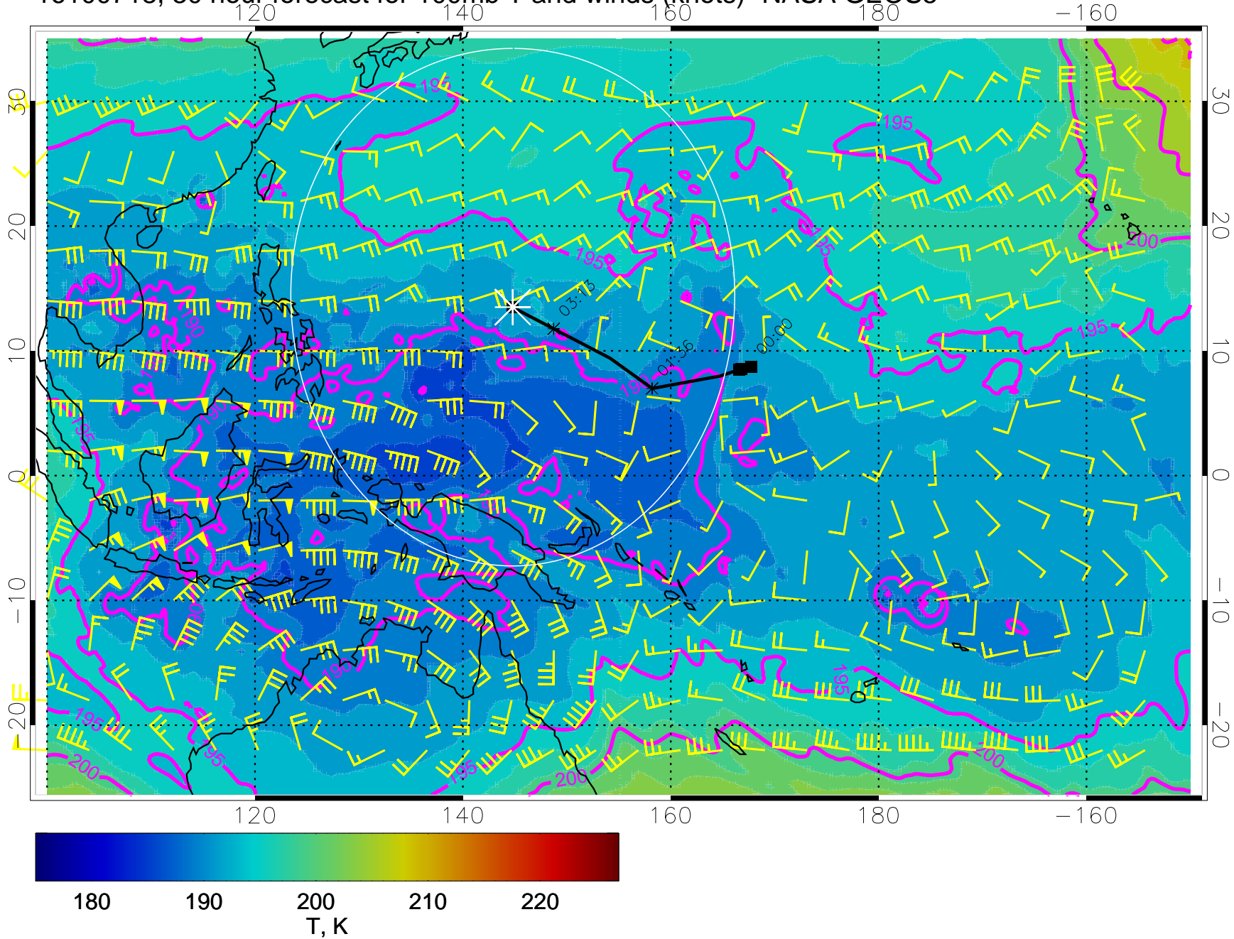
16100718, 30 hour forecast for 100mb T and winds (knots)- NASA GEOS5
