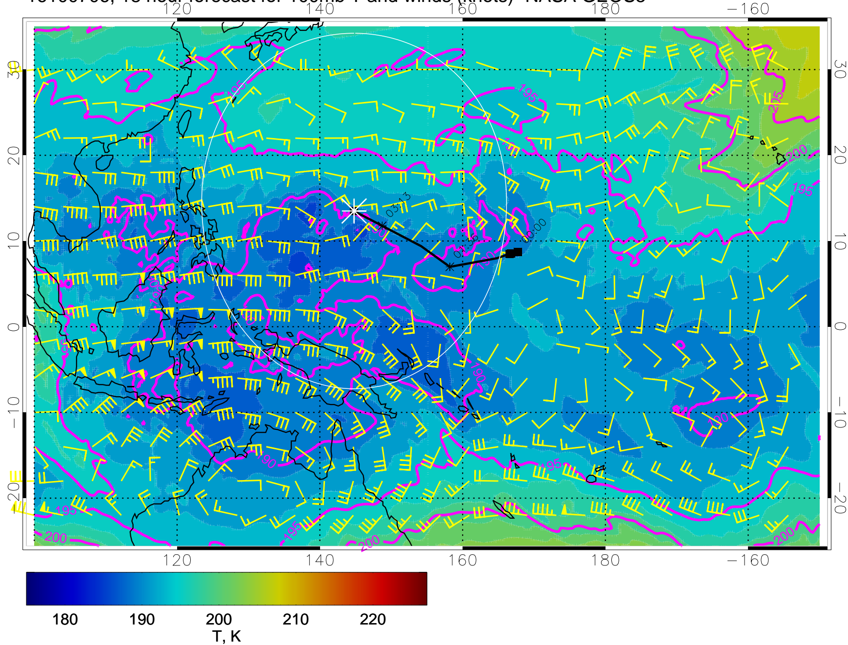
16100706, 18 hour forecast for 100mb T and winds (knots)- NASA GEOS5
