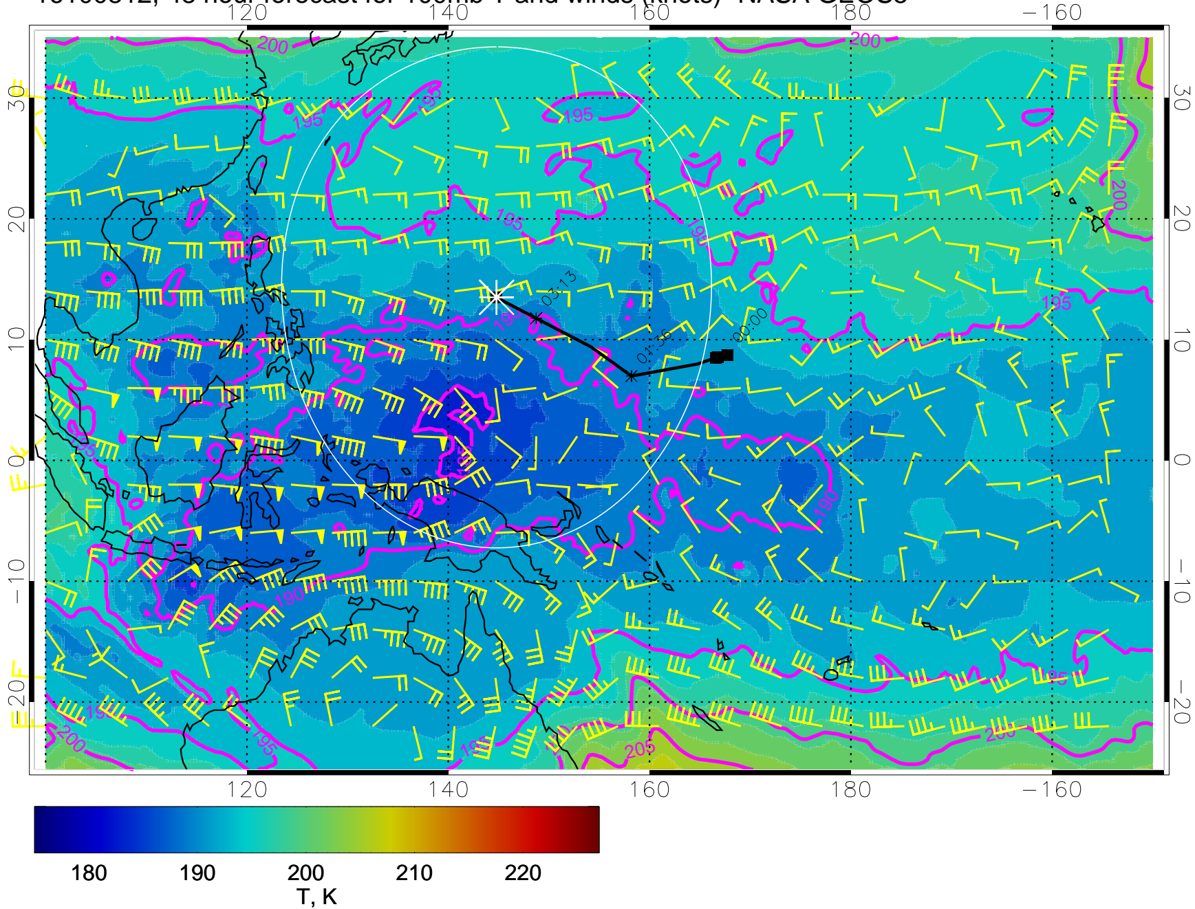
16100812, 48 hour forecast for 100mb T and winds (knots)- NASA GEOS5
