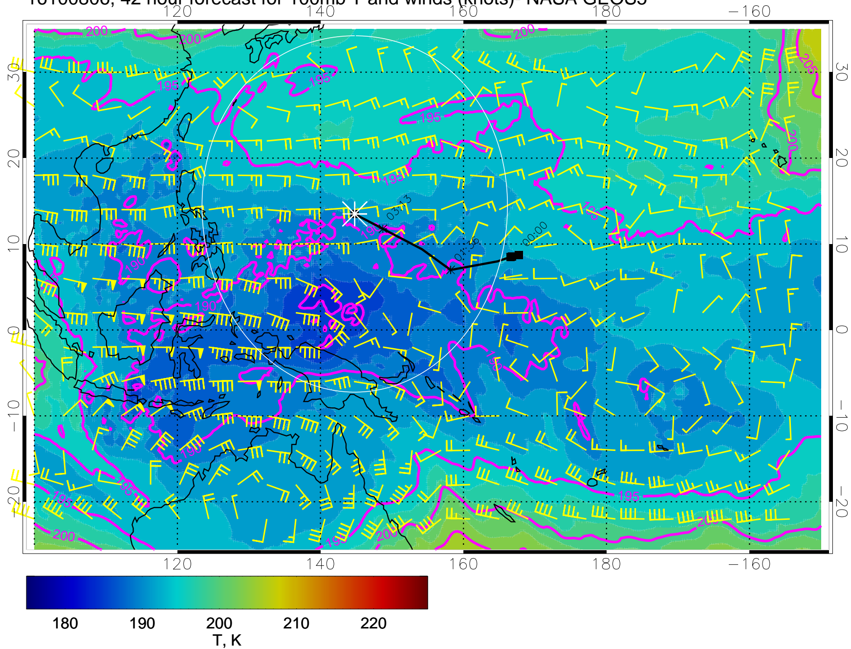
16100806, 42 hour forecast for 100mb T and winds (knots)- NASA GEOS5
