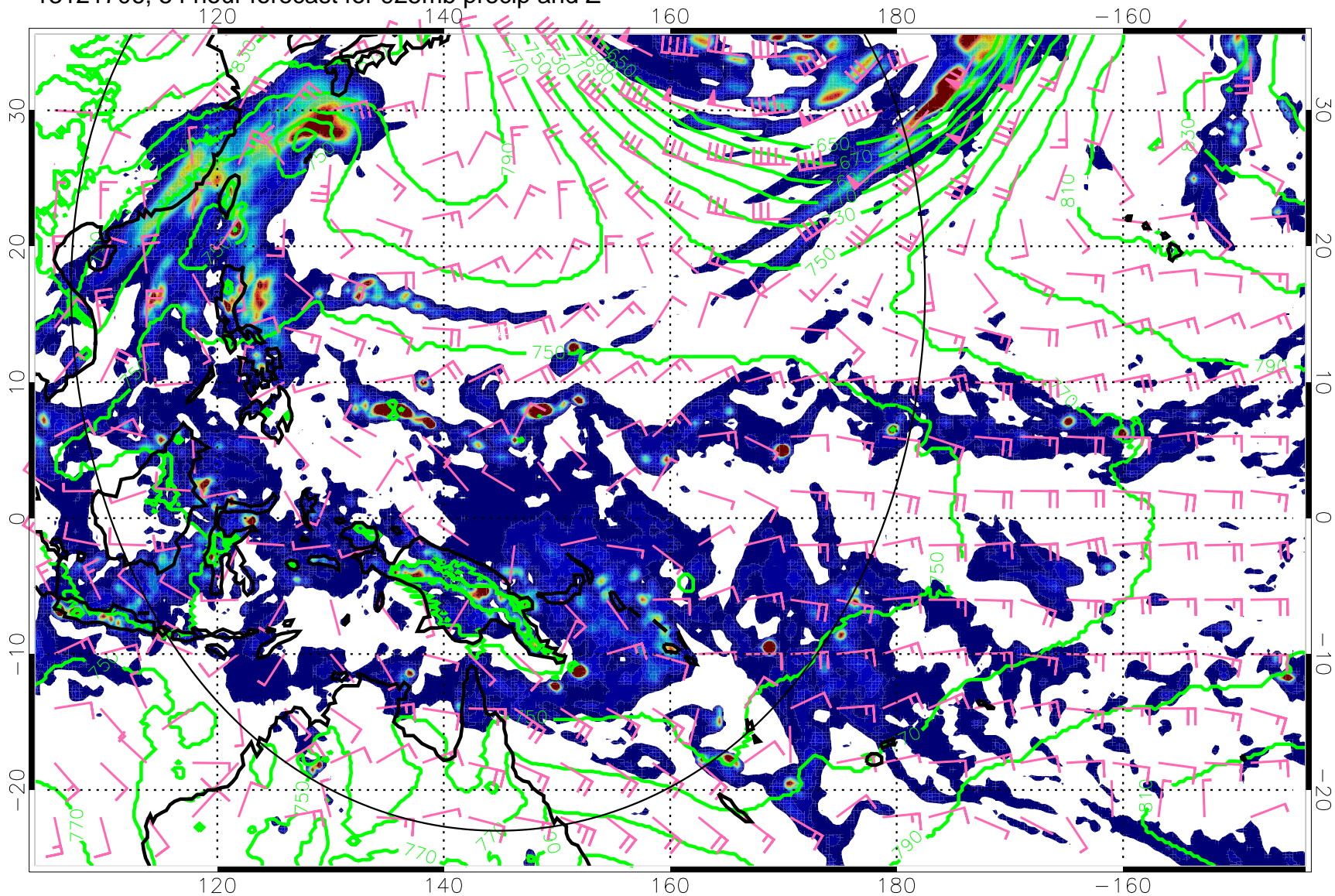
13121706, 54 hour forecast for 925mb precip and Z
