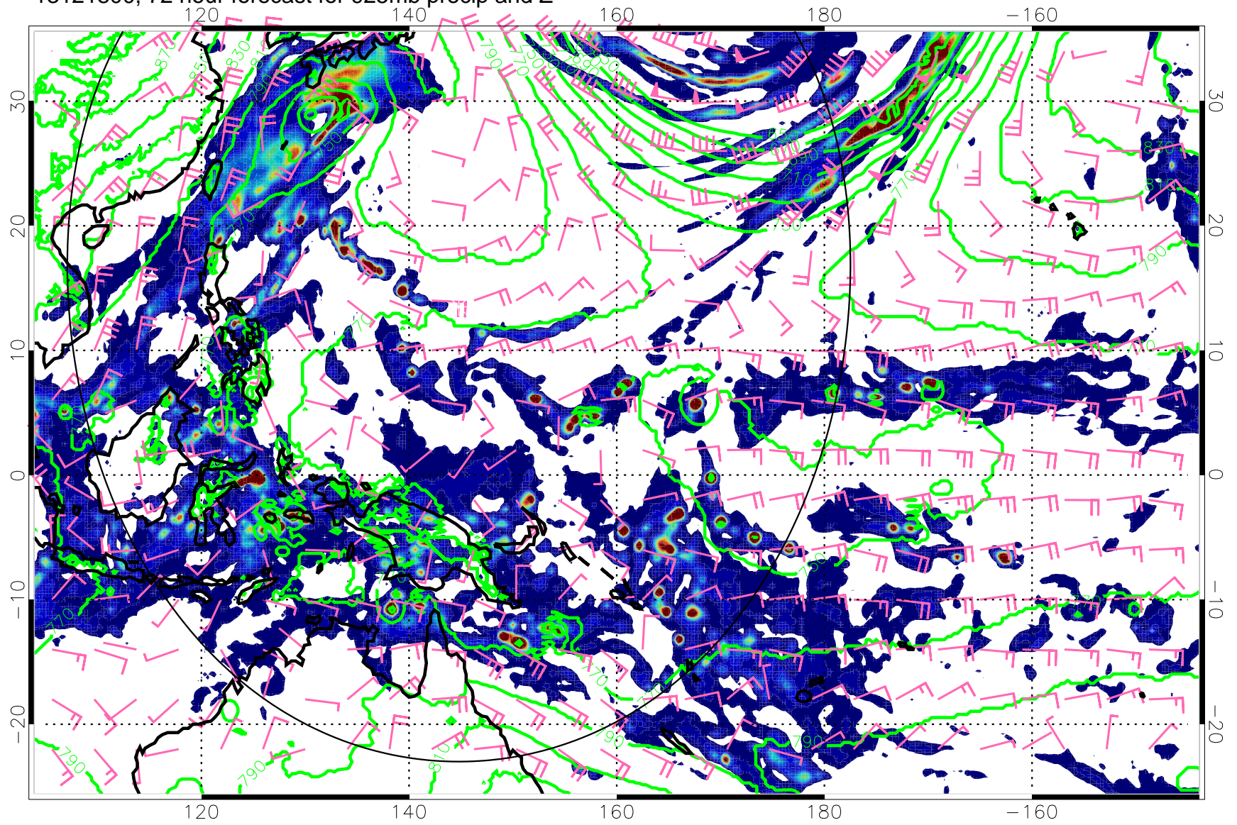
13121800, 72 hour forecast for 925mb precip and Z
