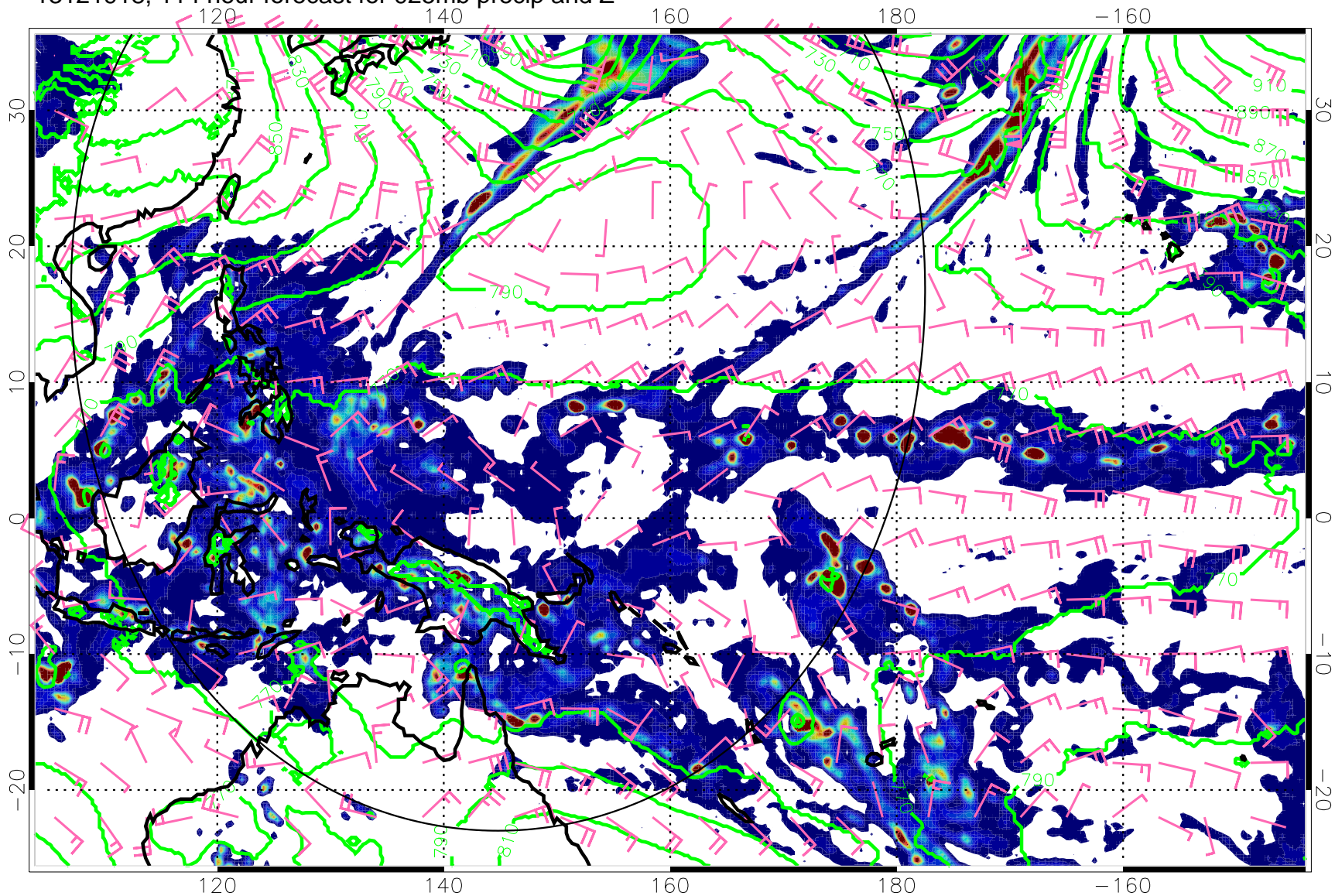
13121918, 114 hour forecast for 925mb precip and Z
