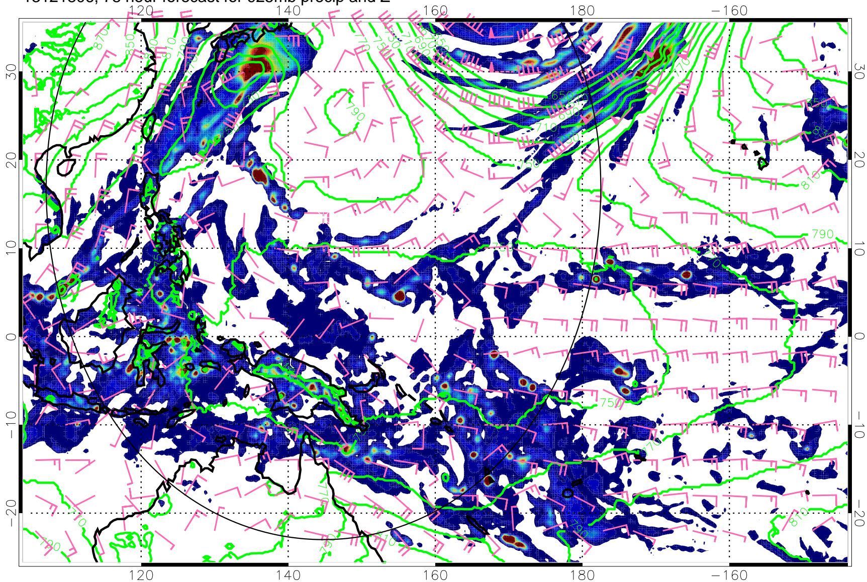
13121806, 78 hour forecast for 925mb precip and Z
