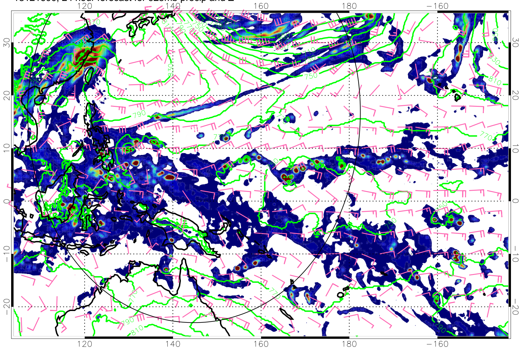
13121600, 24 hour forecast for 925mb precip and Z
