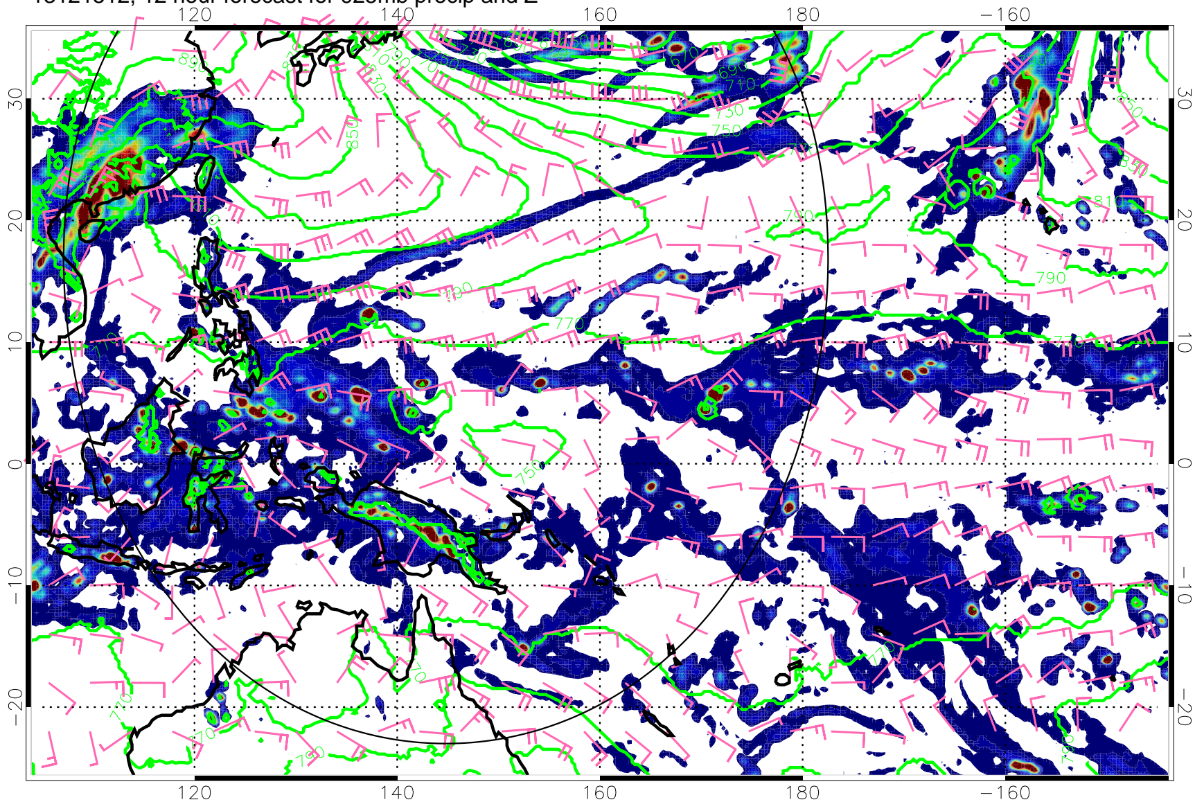
13121512, 12 hour forecast for 925mb precip and Z
