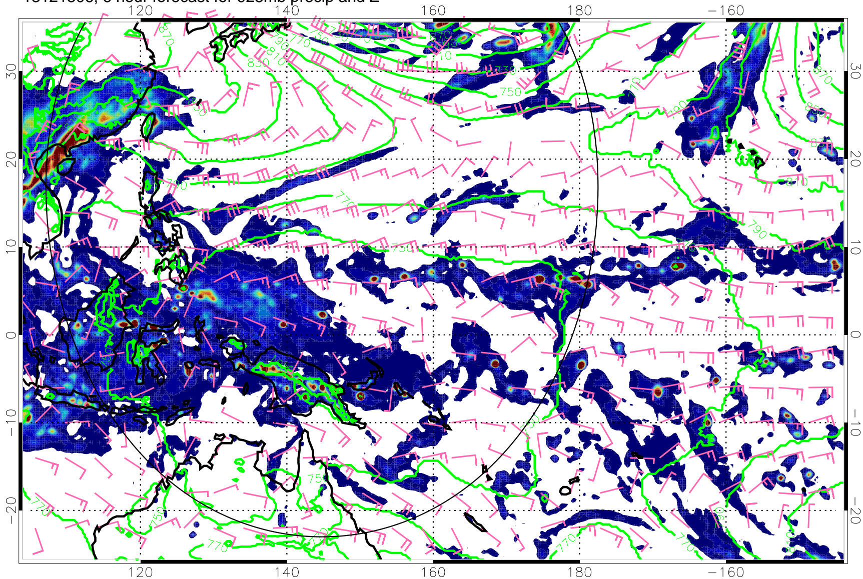
13121506, 6 hour forecast for 925mb precip and Z
