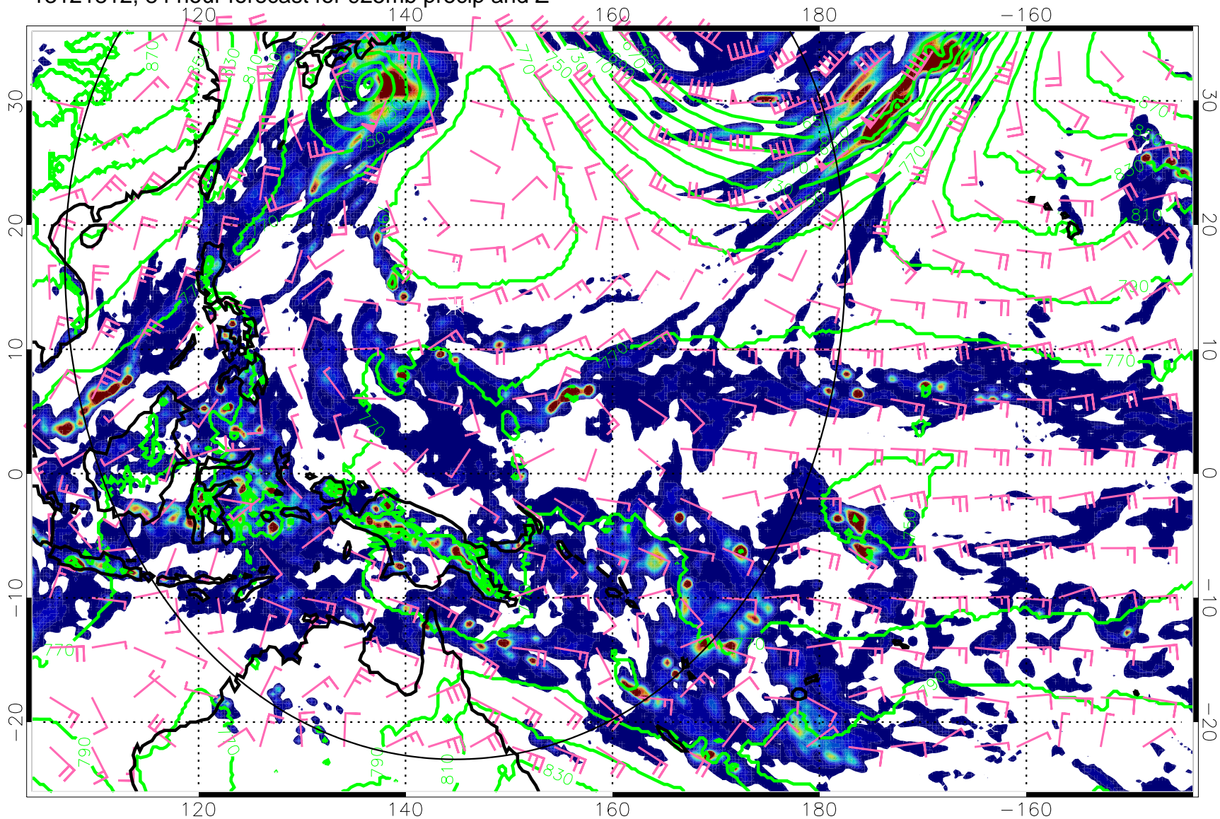
13121812, 84 hour forecast for 925mb precip and Z
