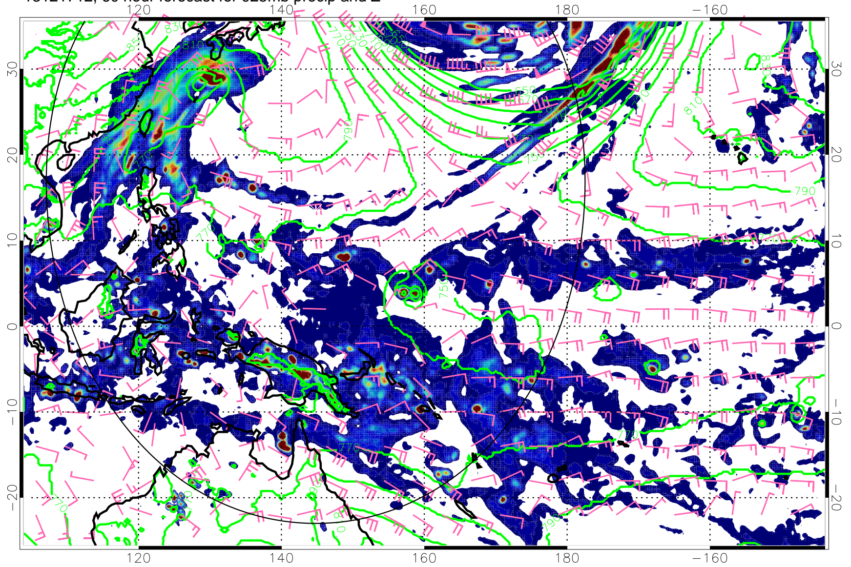
13121712, 60 hour forecast for 925mb precip and Z
