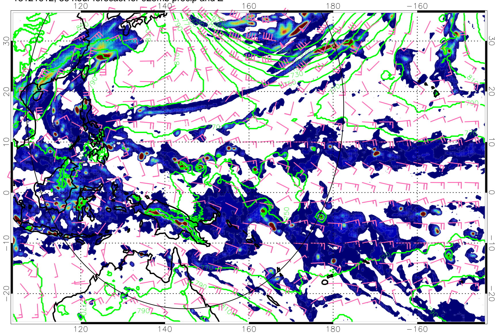
13121612, 36 hour forecast for 925mb precip and Z
