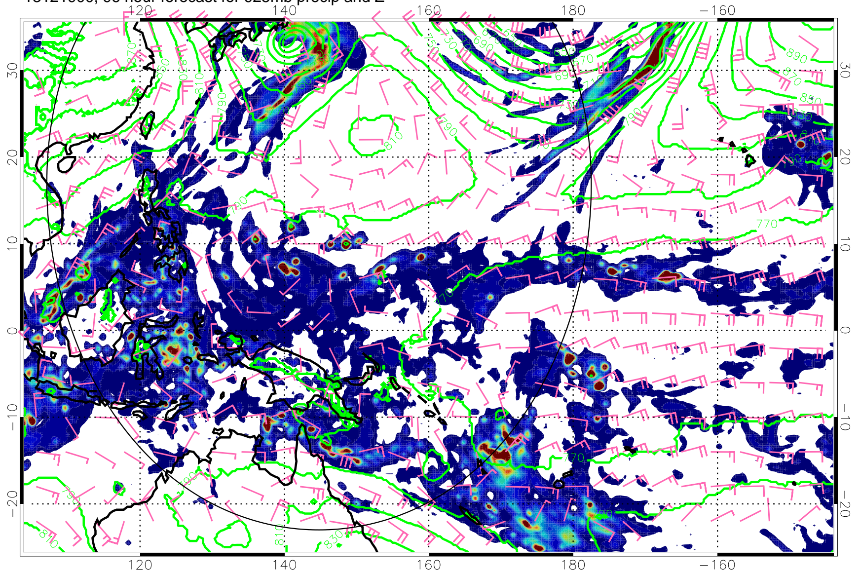
13121900, 96 hour forecast for 925mb precip and Z
