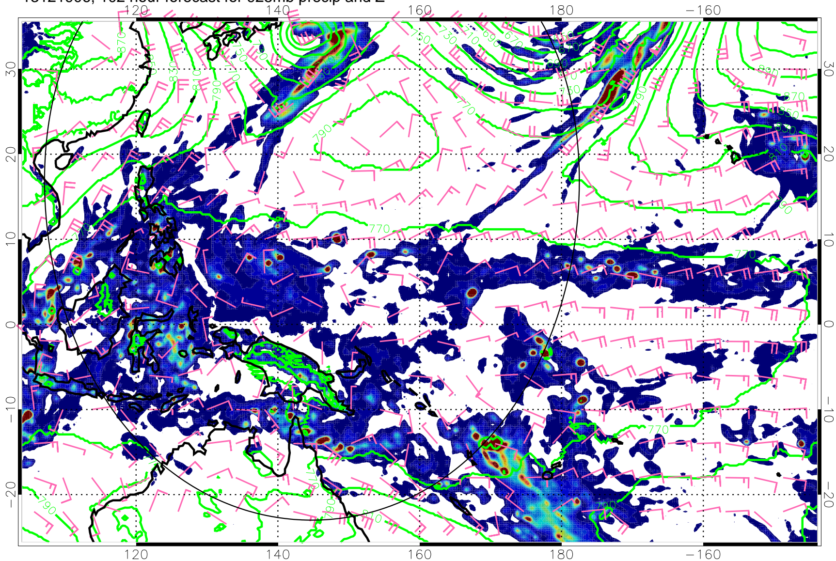
13121906, 102 hour forecast for 925mb precip and Z
