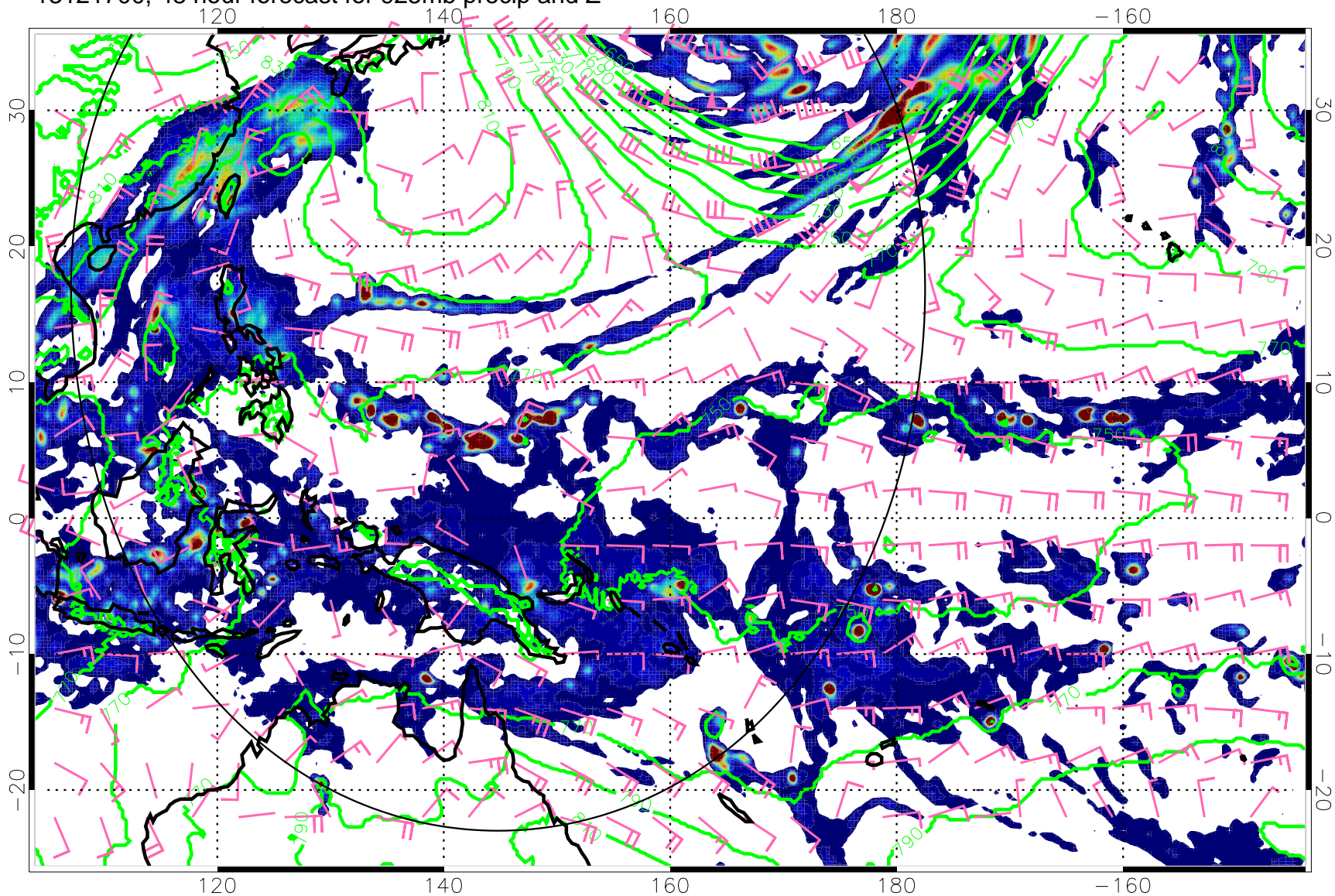
13121700, 48 hour forecast for 925mb precip and Z
