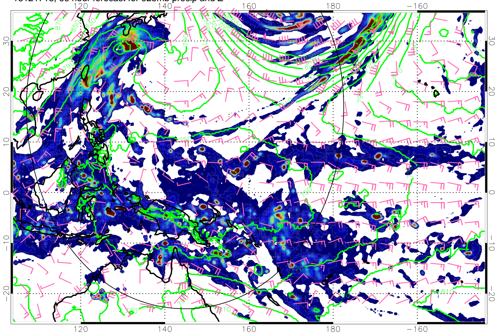
13121718, 66 hour forecast for 925mb precip and Z
