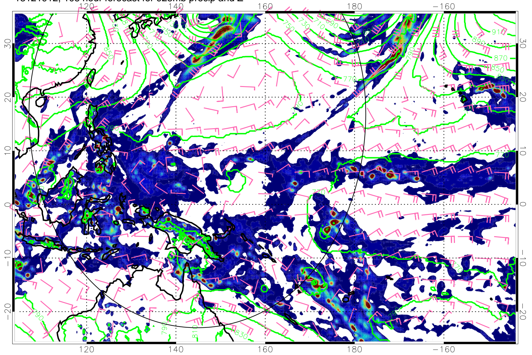
13121912, 108 hour forecast for 925mb precip and Z
