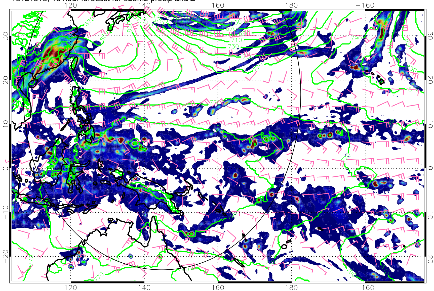
13121518, 18 hour forecast for 925mb precip and Z
