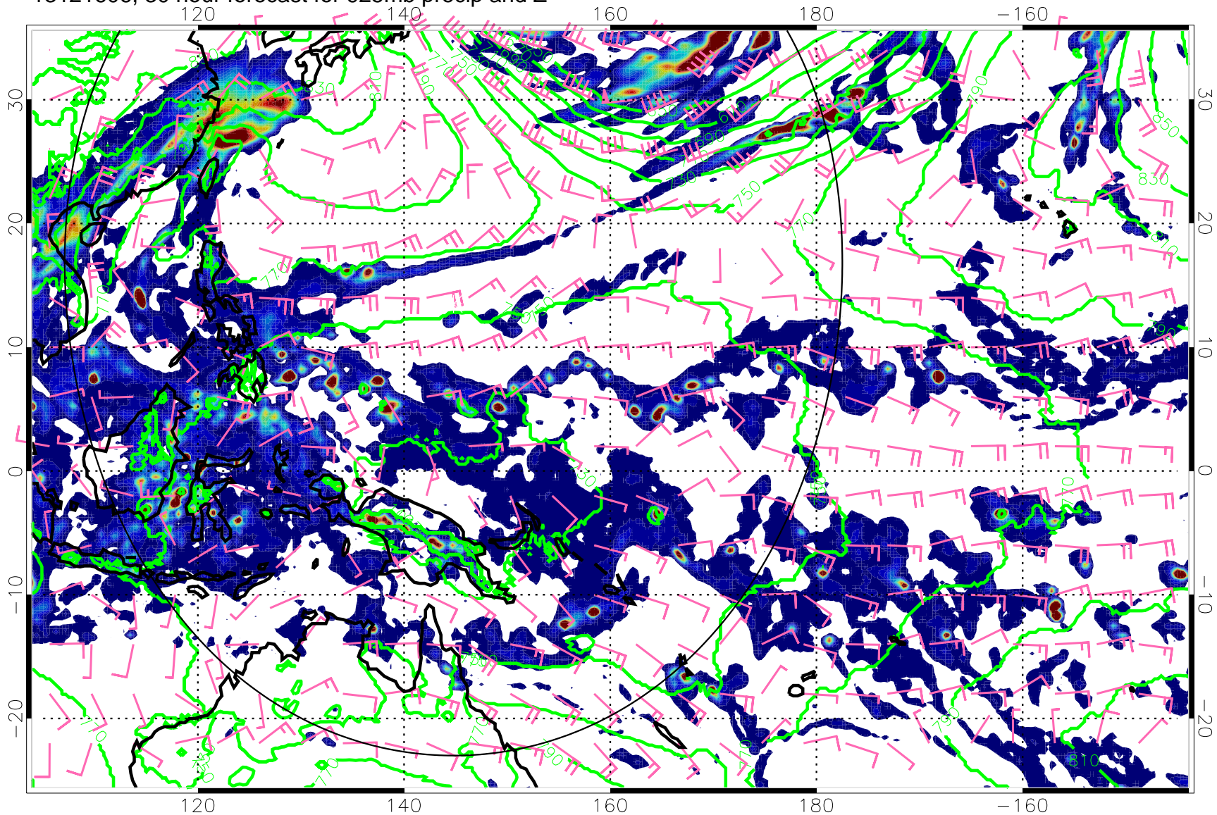
13121606, 30 hour forecast for 925mb precip and Z
