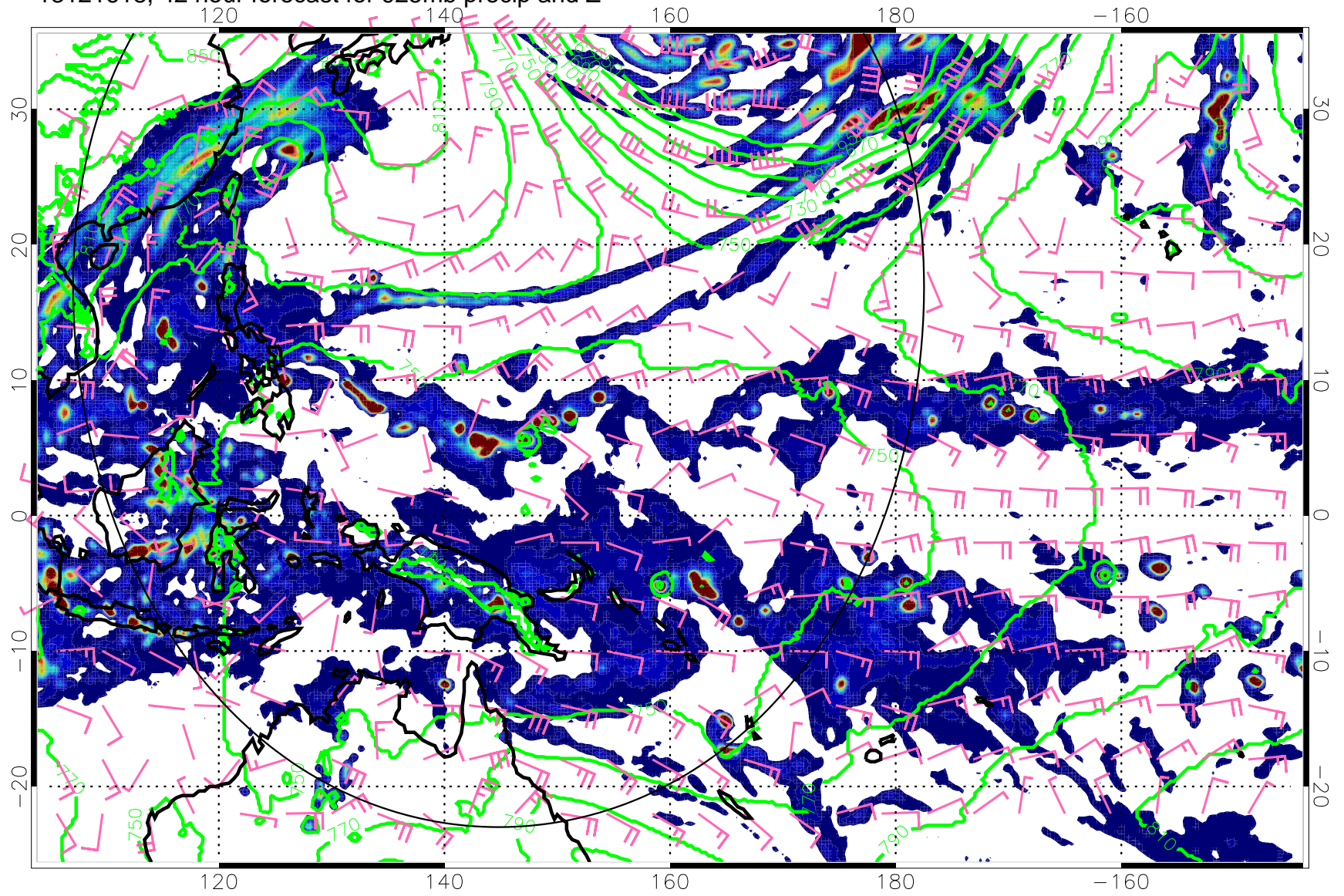
13121618, 42 hour forecast for 925mb precip and Z
