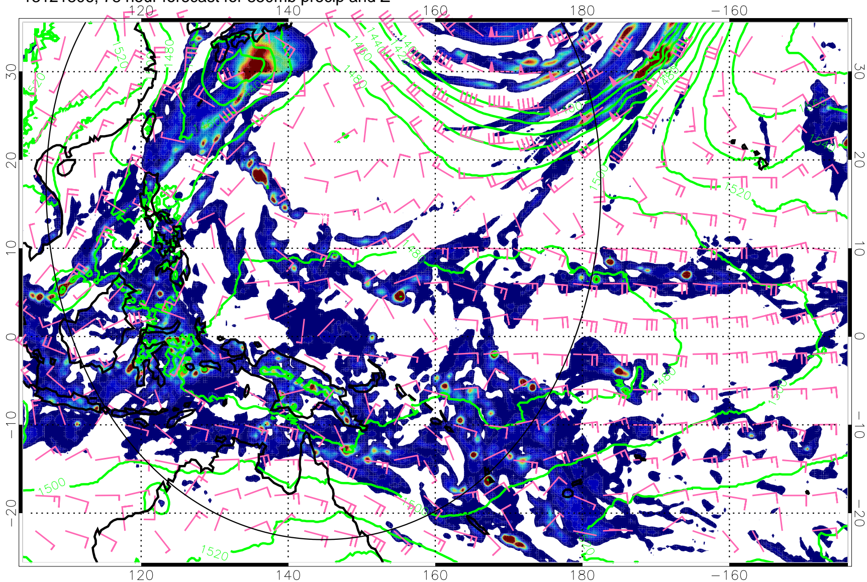
13121806, 78 hour forecast for 850mb precip and Z
