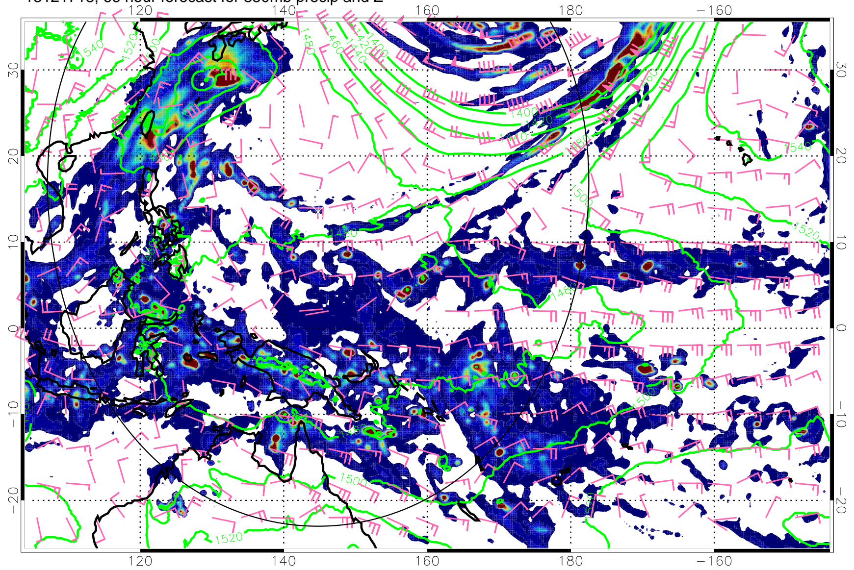
13121718, 66 hour forecast for 850mb precip and Z
