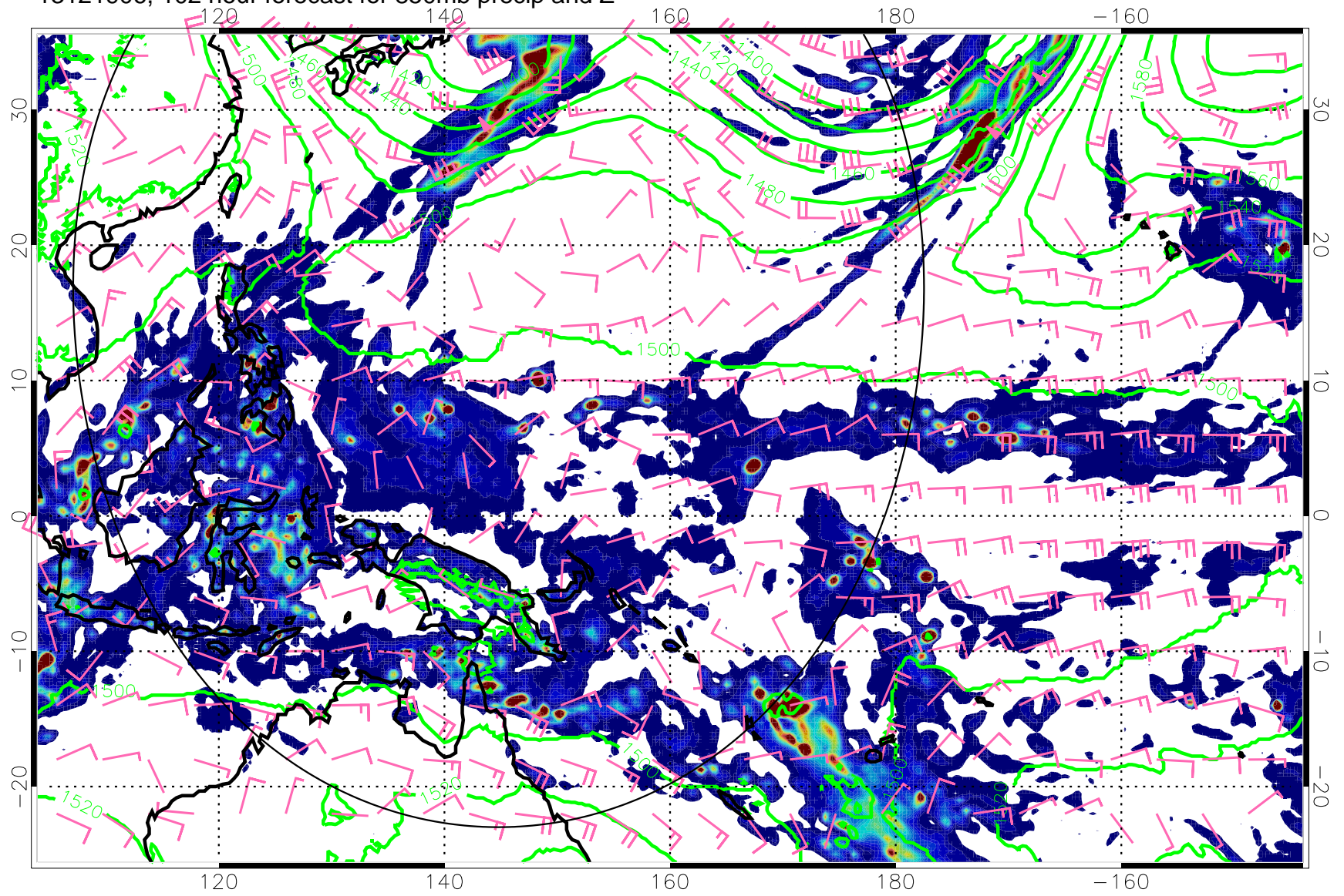
13121906, 102 hour forecast for 850mb precip and Z
