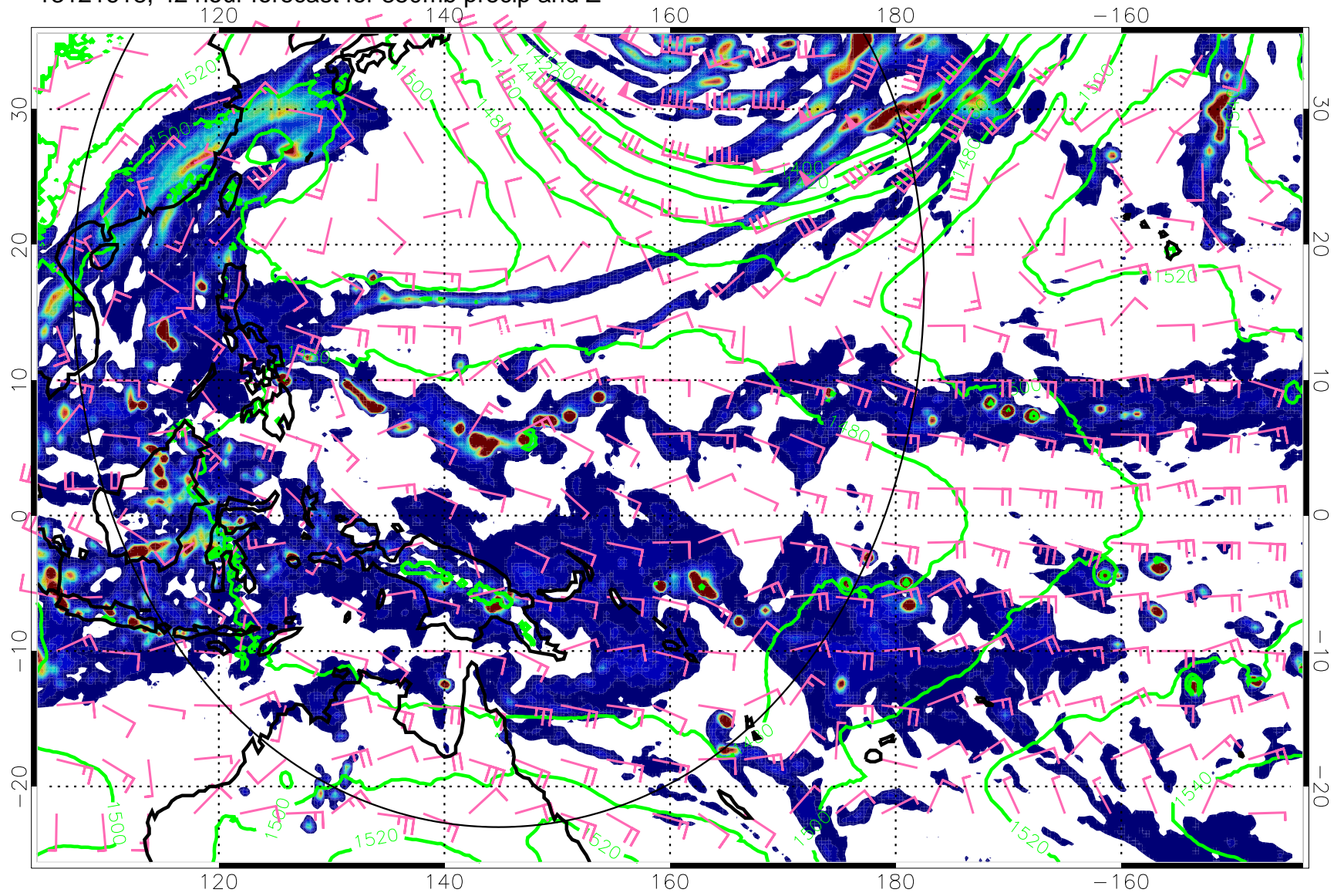
13121618, 42 hour forecast for 850mb precip and Z
