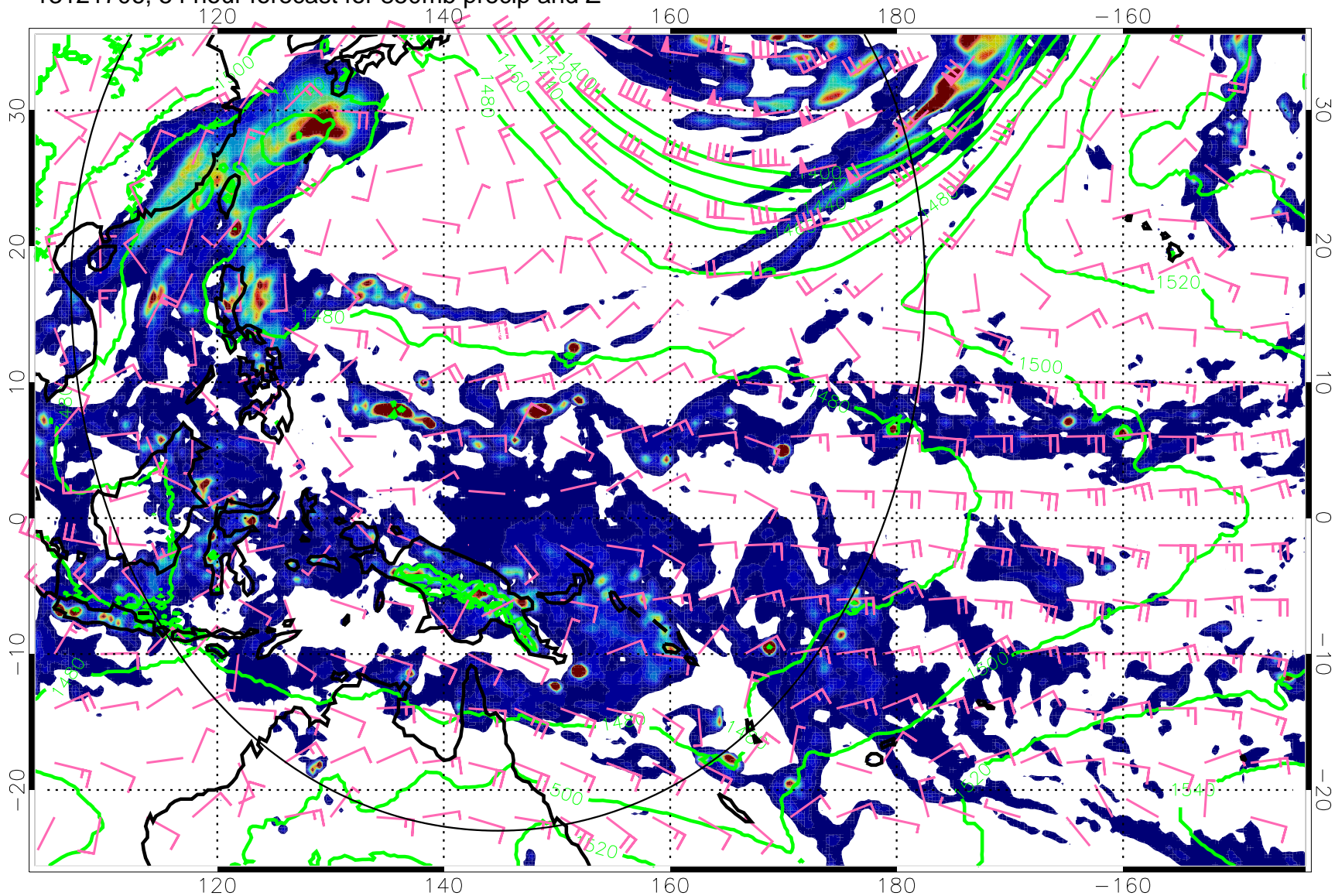
13121706, 54 hour forecast for 850mb precip and Z
