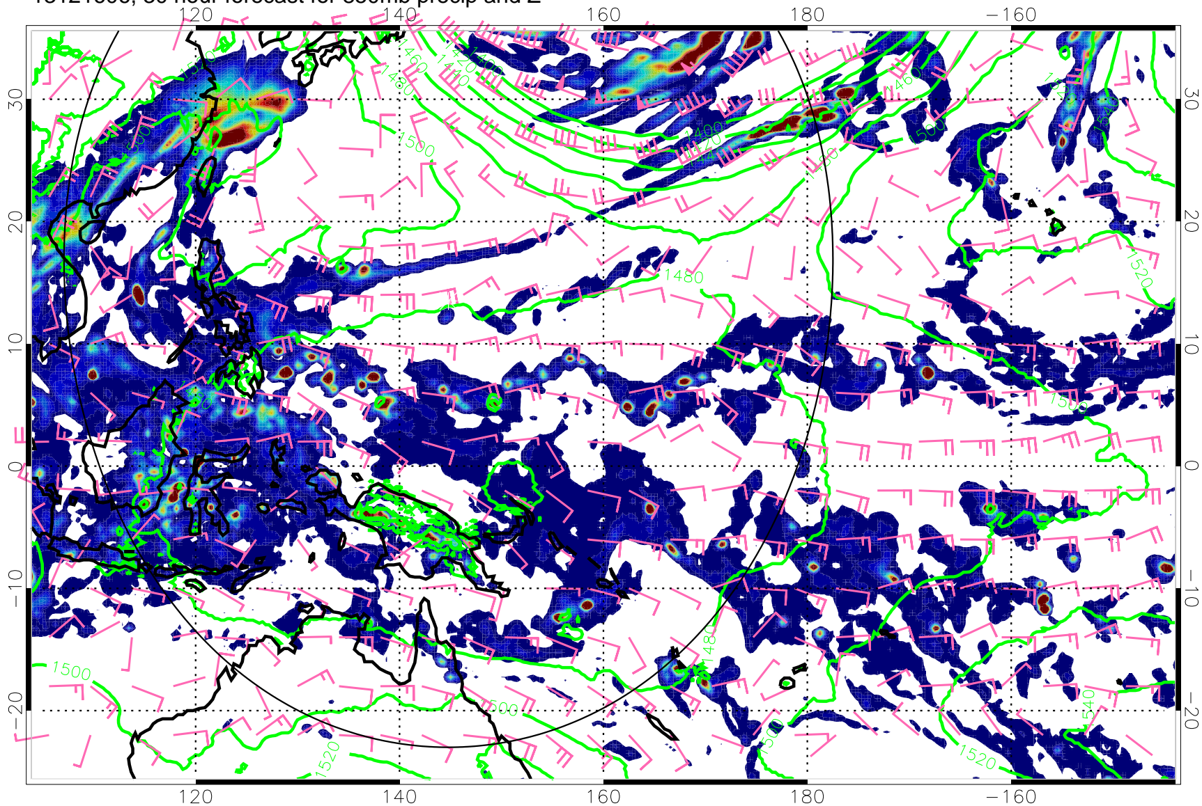
13121606, 30 hour forecast for 850mb precip and Z
