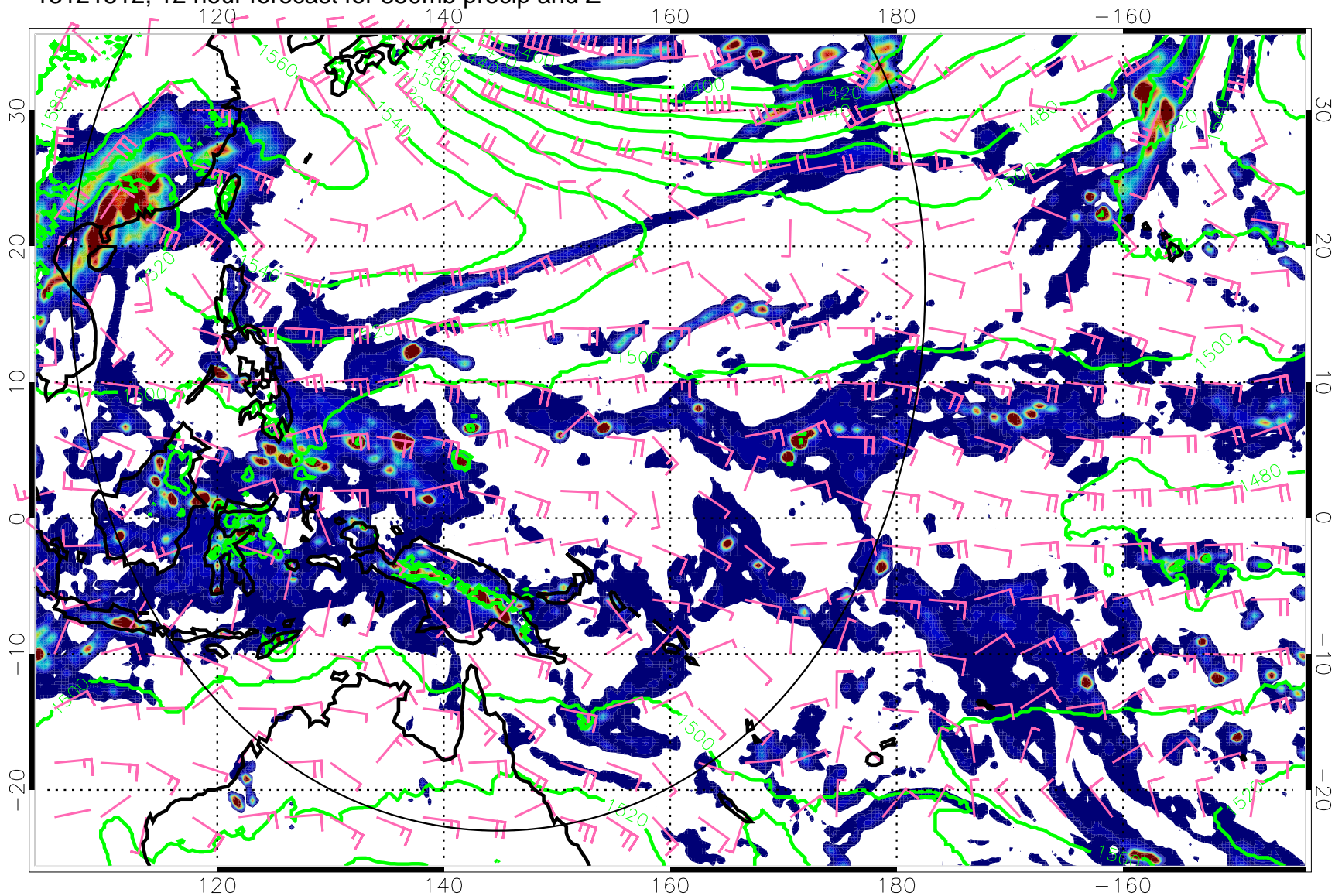
13121512, 12 hour forecast for 850mb precip and Z
