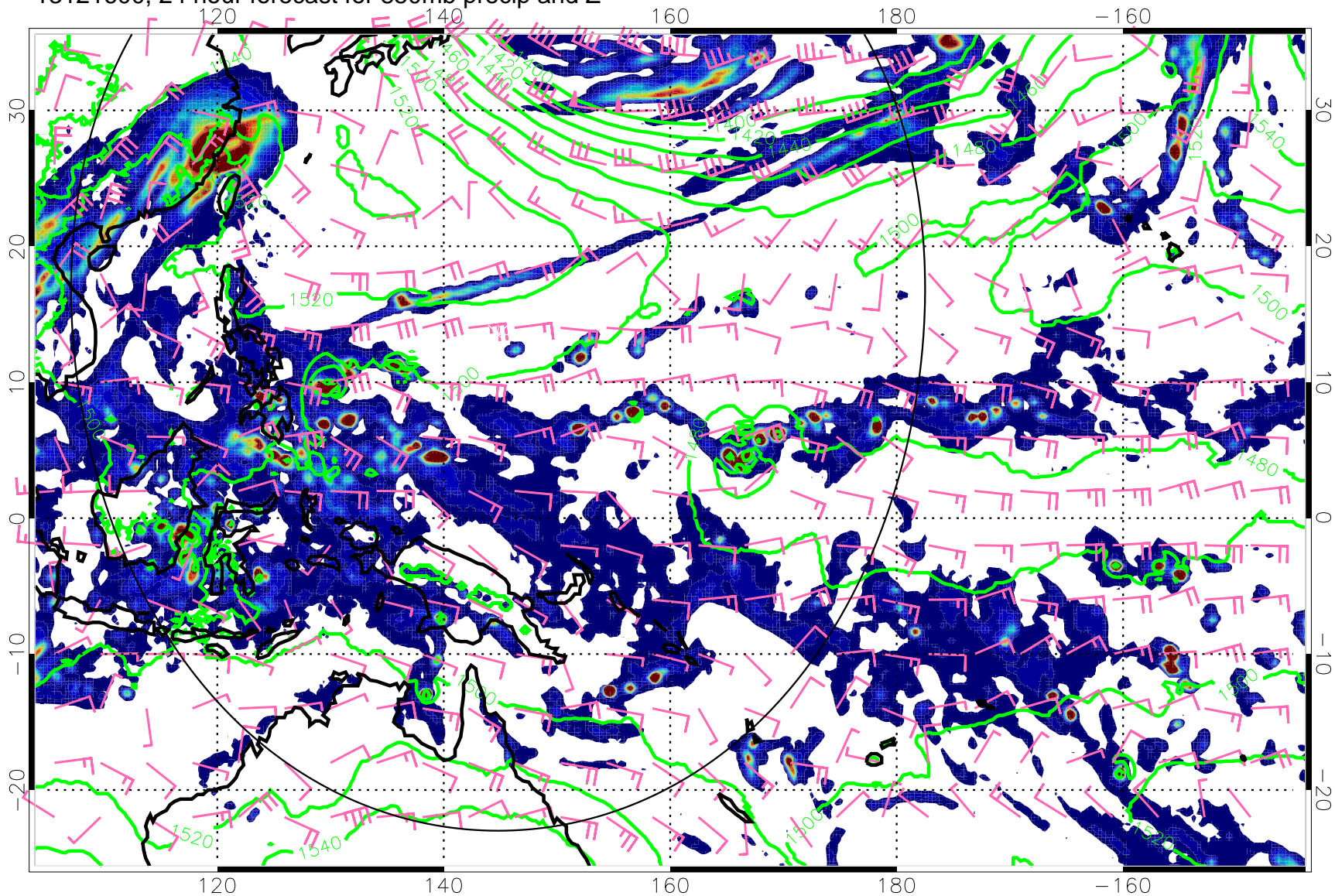
13121600, 24 hour forecast for 850mb precip and Z
