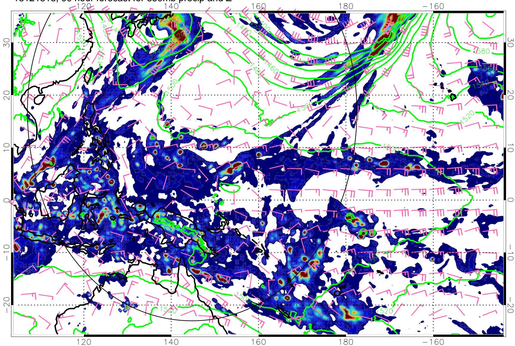
13121818, 90 hour forecast for 850mb precip and Z
