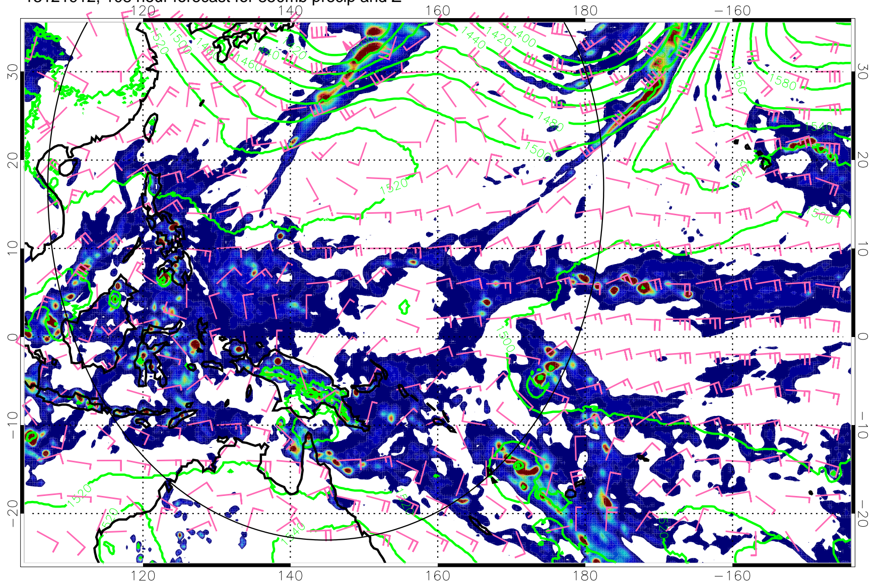
13121912, 108 hour forecast for 850mb precip and Z
