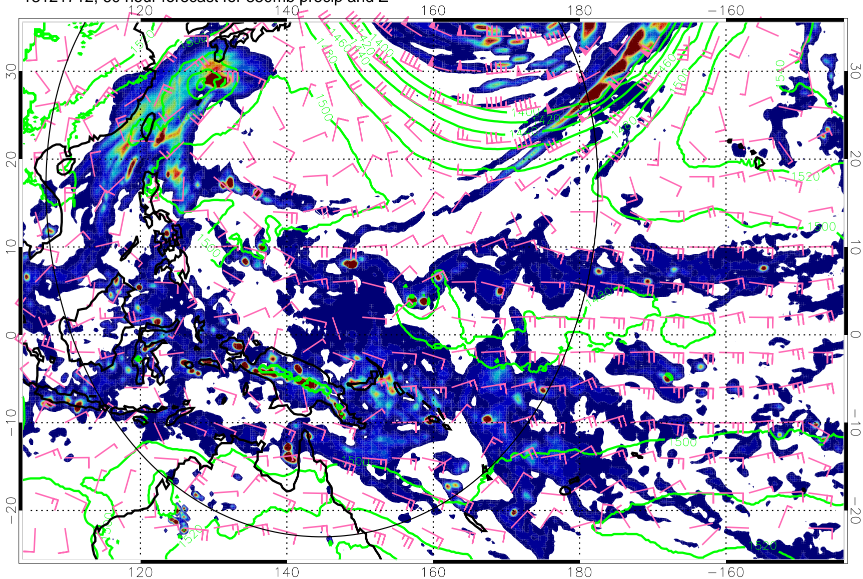
13121712, 60 hour forecast for 850mb precip and Z
