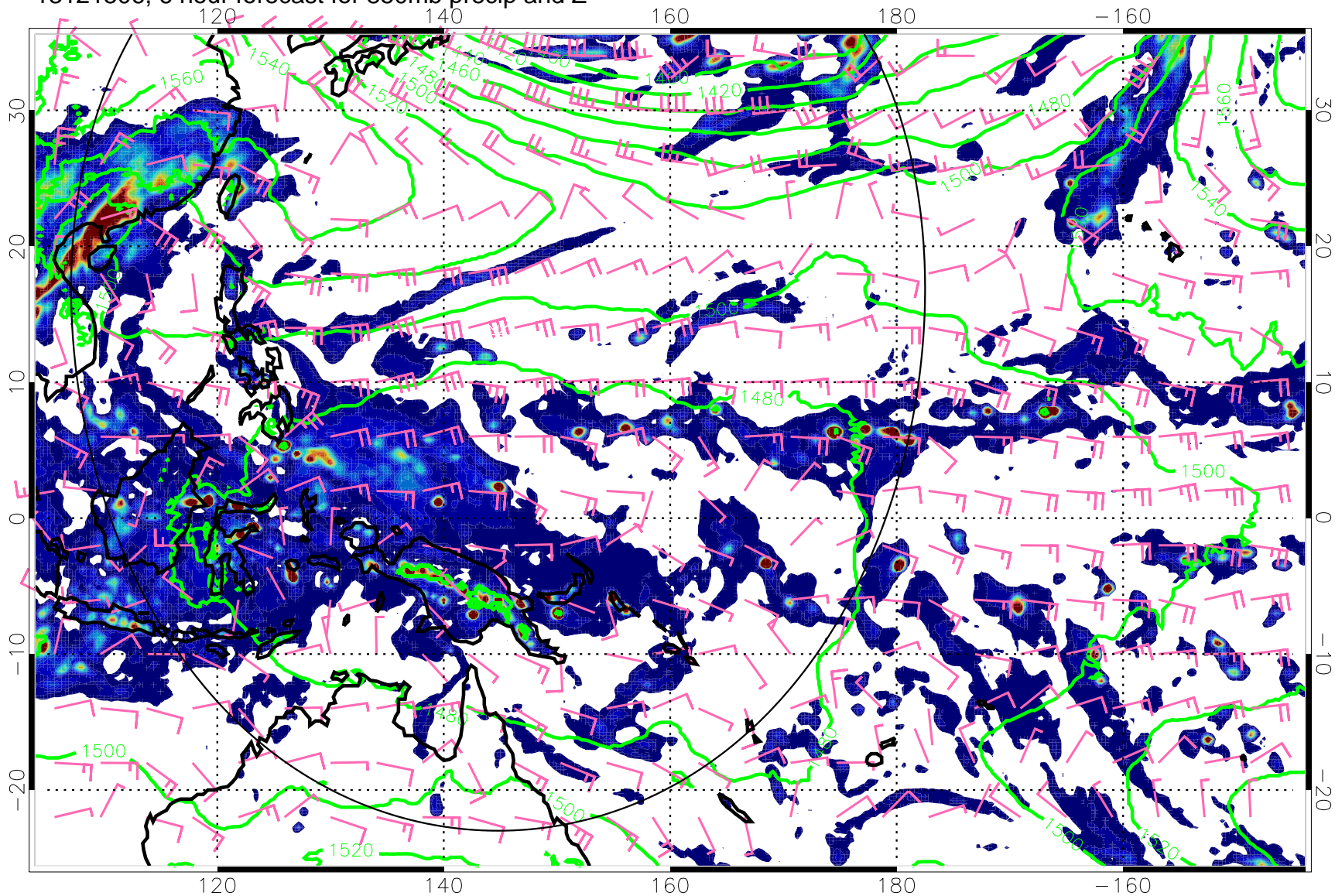
13121506, 6 hour forecast for 850mb precip and Z
