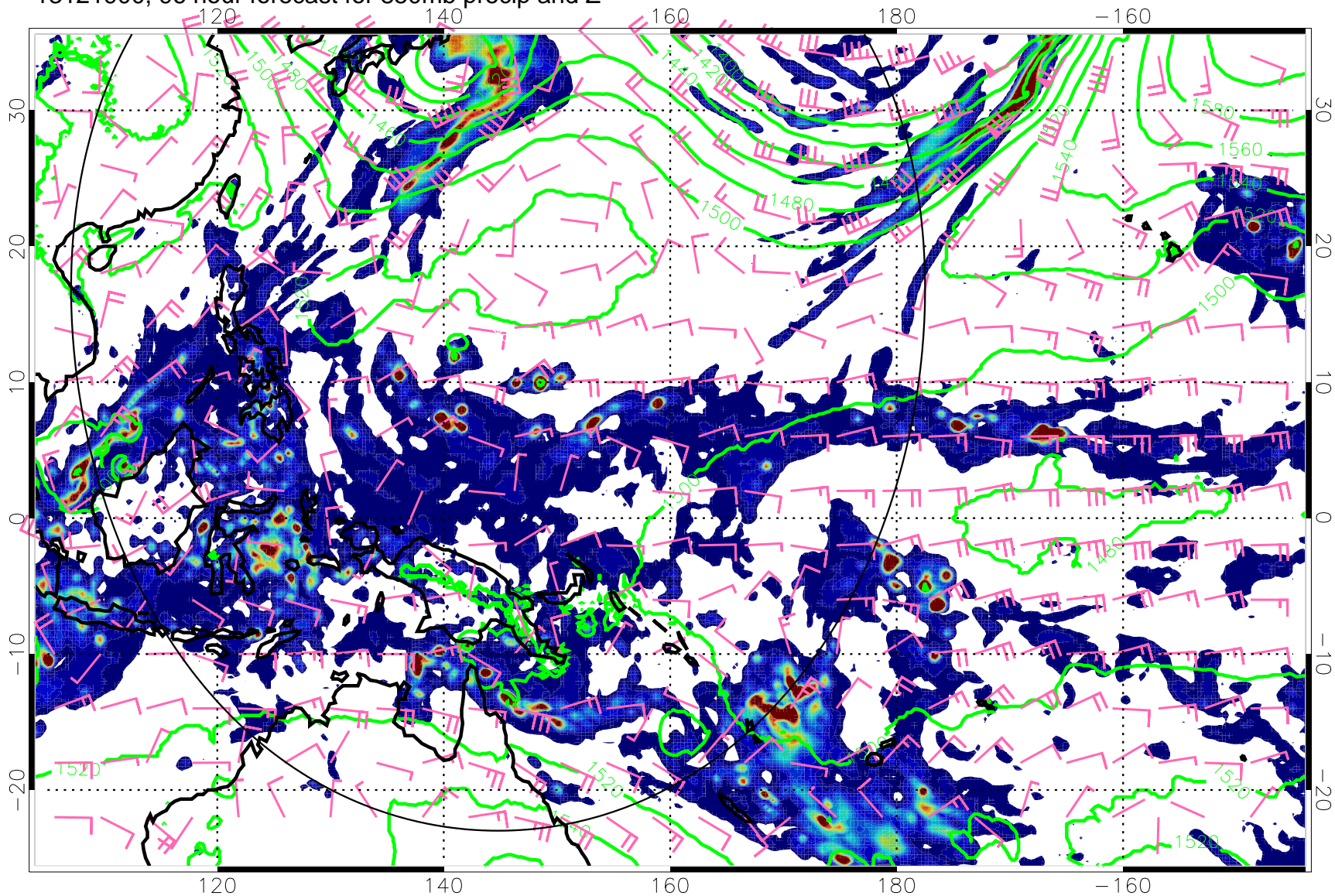
13121900, 96 hour forecast for 850mb precip and Z
