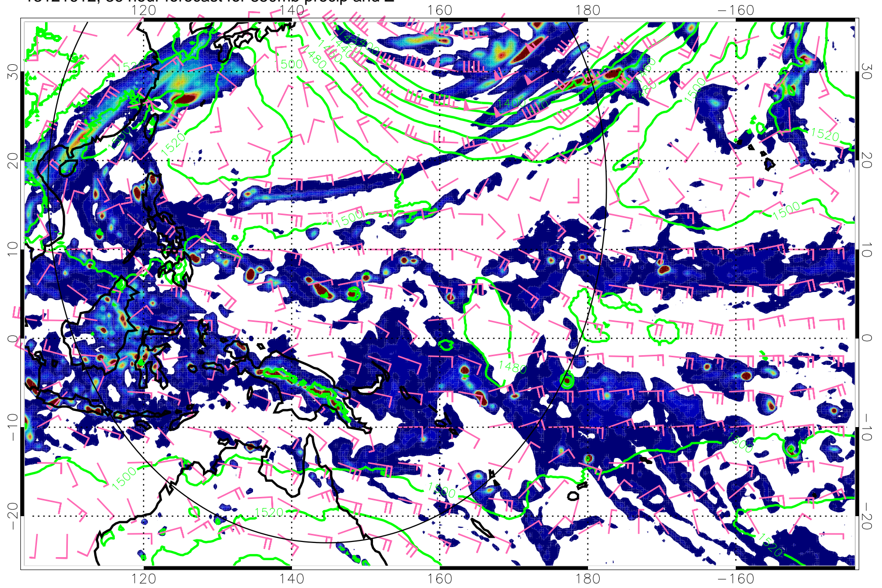
13121612, 36 hour forecast for 850mb precip and Z
