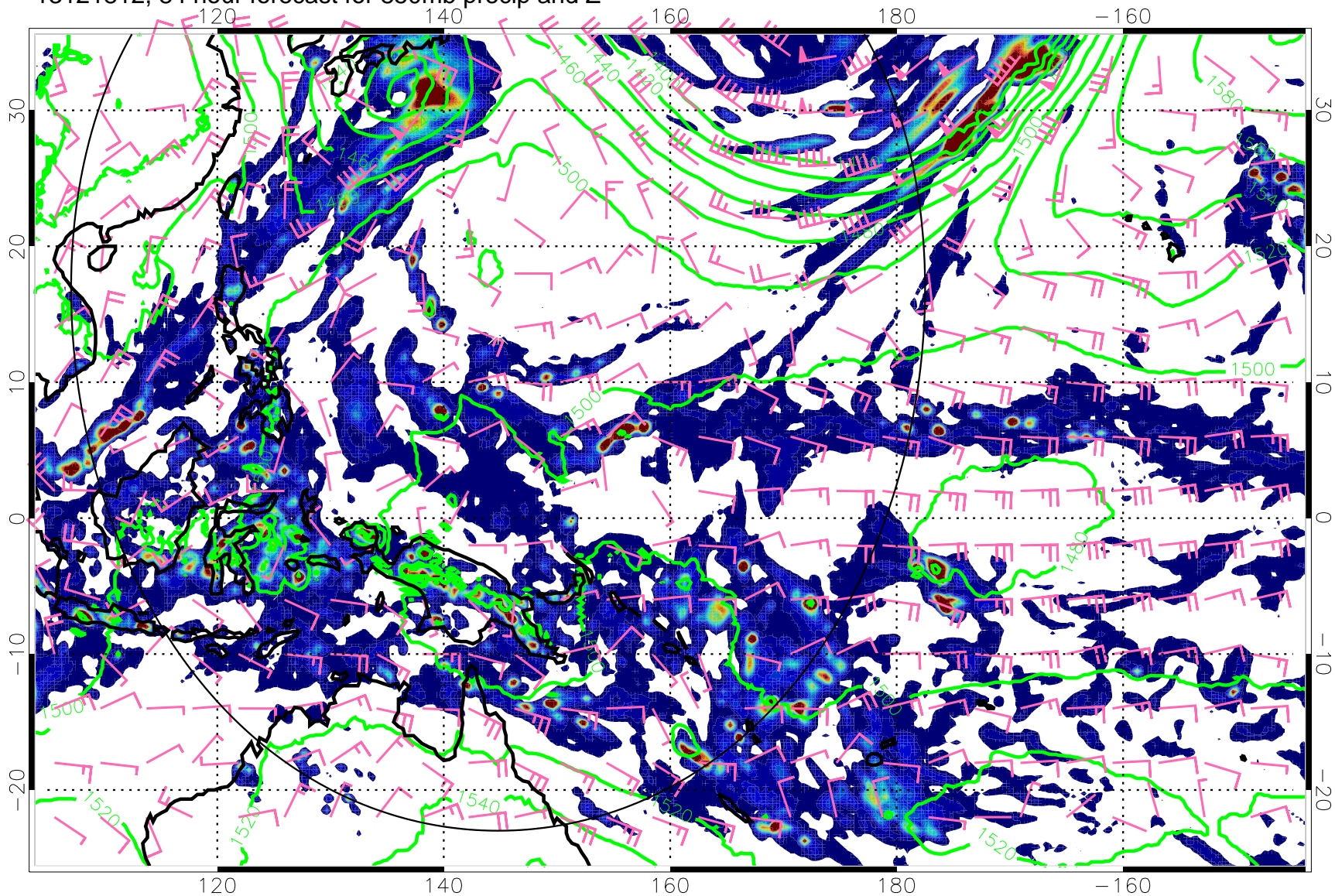
13121812, 84 hour forecast for 850mb precip and Z
