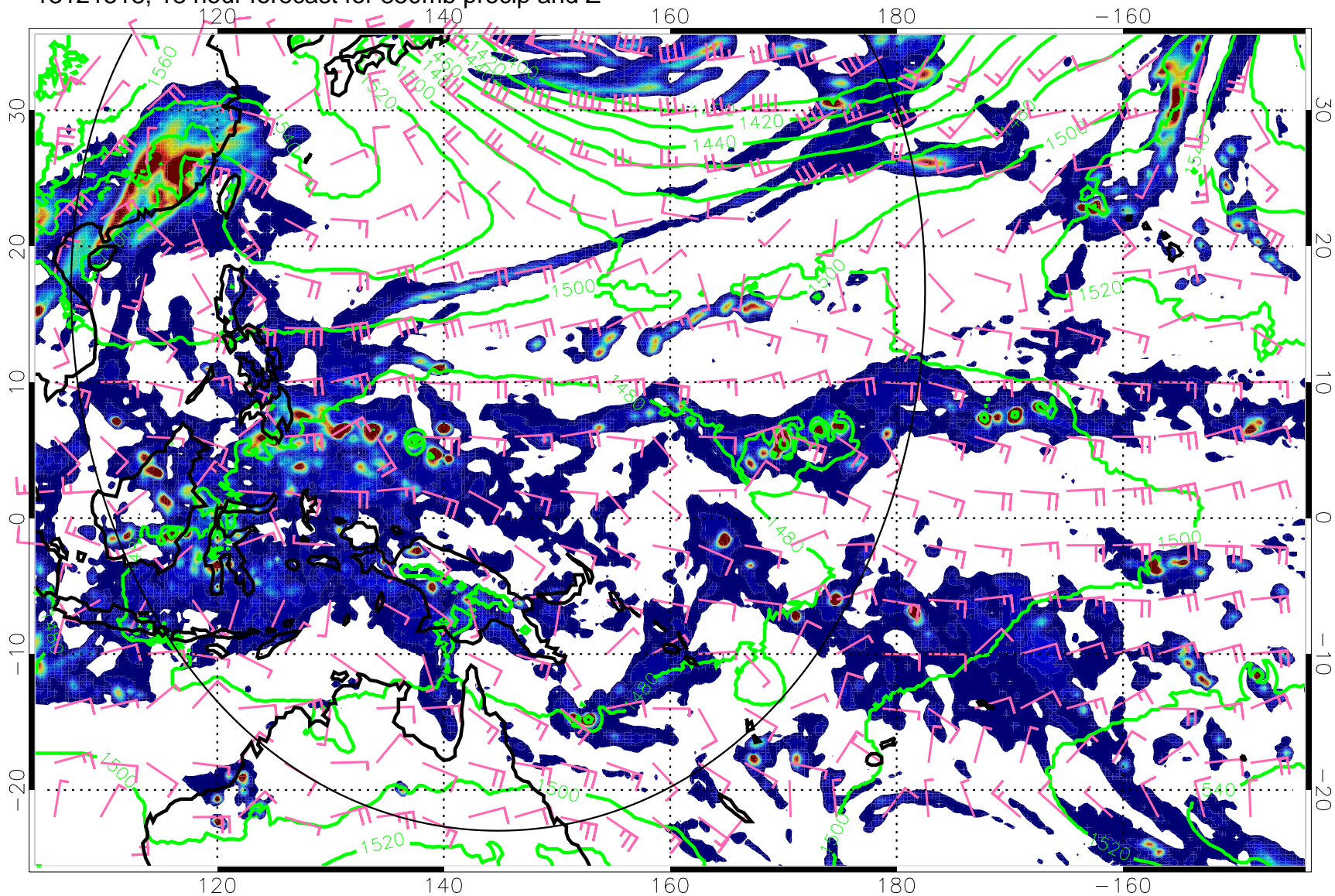
13121518, 18 hour forecast for 850mb precip and Z
