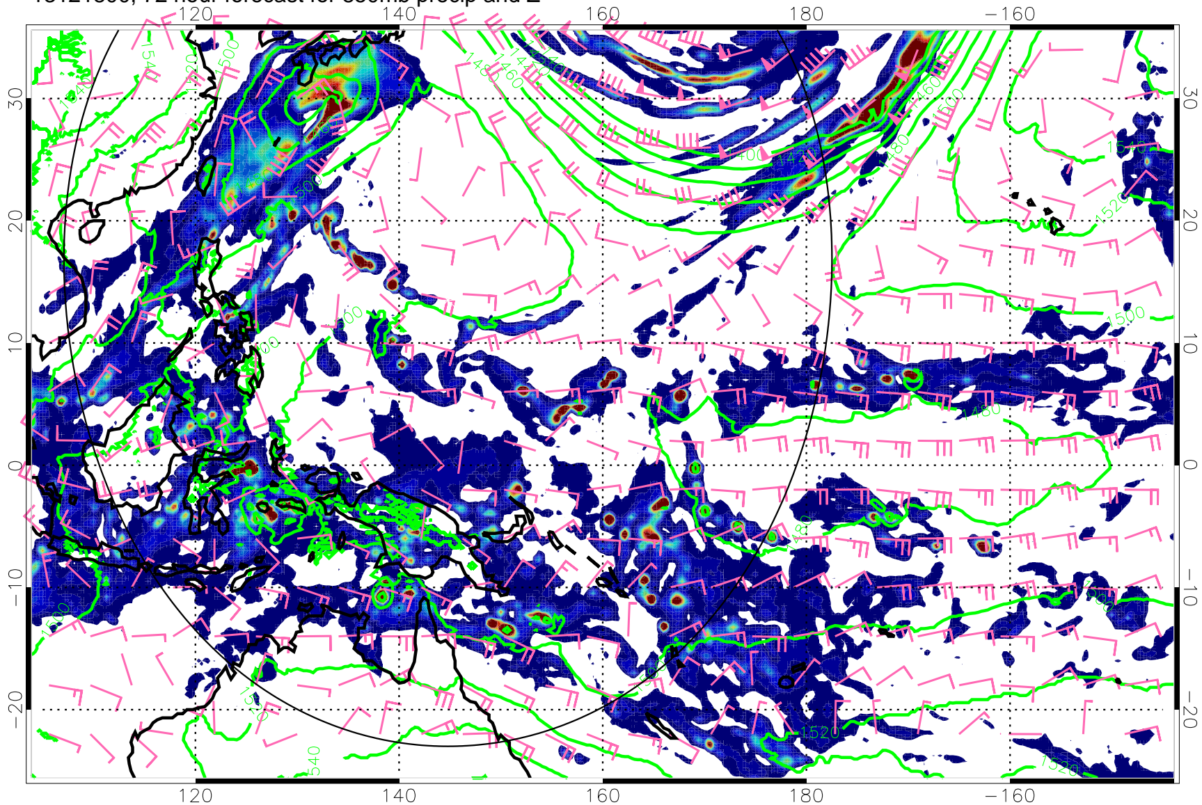
13121800, 72 hour forecast for 850mb precip and Z
