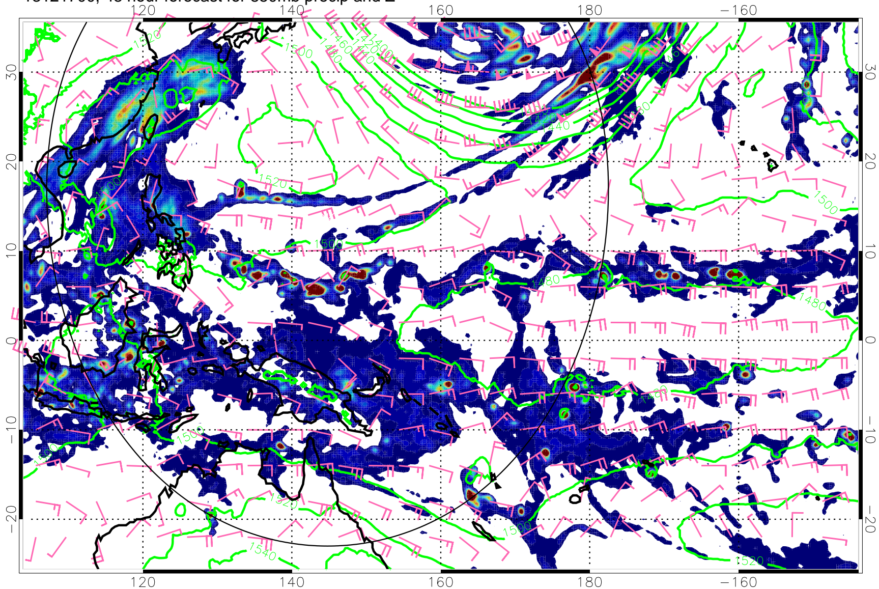
13121700, 48 hour forecast for 850mb precip and Z
