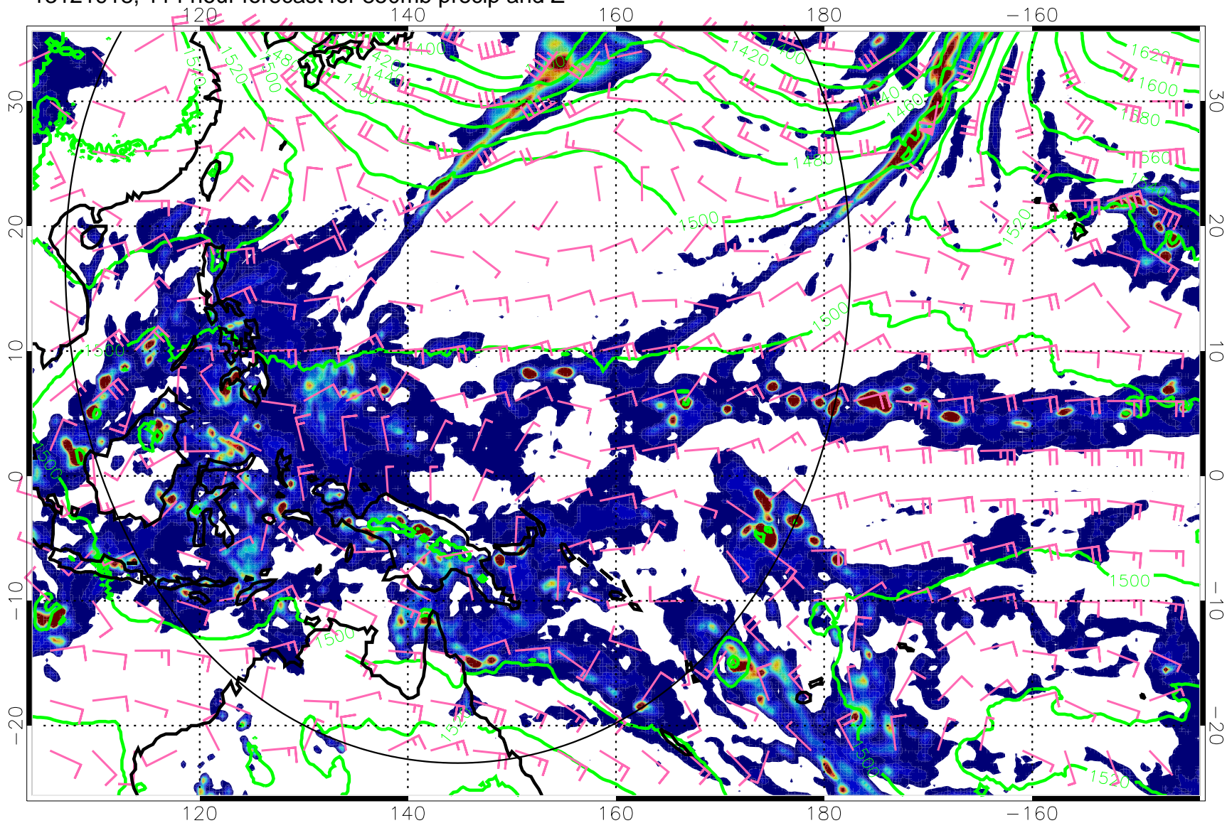
13121918, 114 hour forecast for 850mb precip and Z
