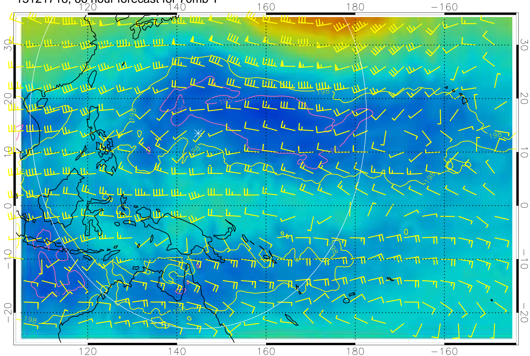
13121718, 66 hour forecast for 70mb T
