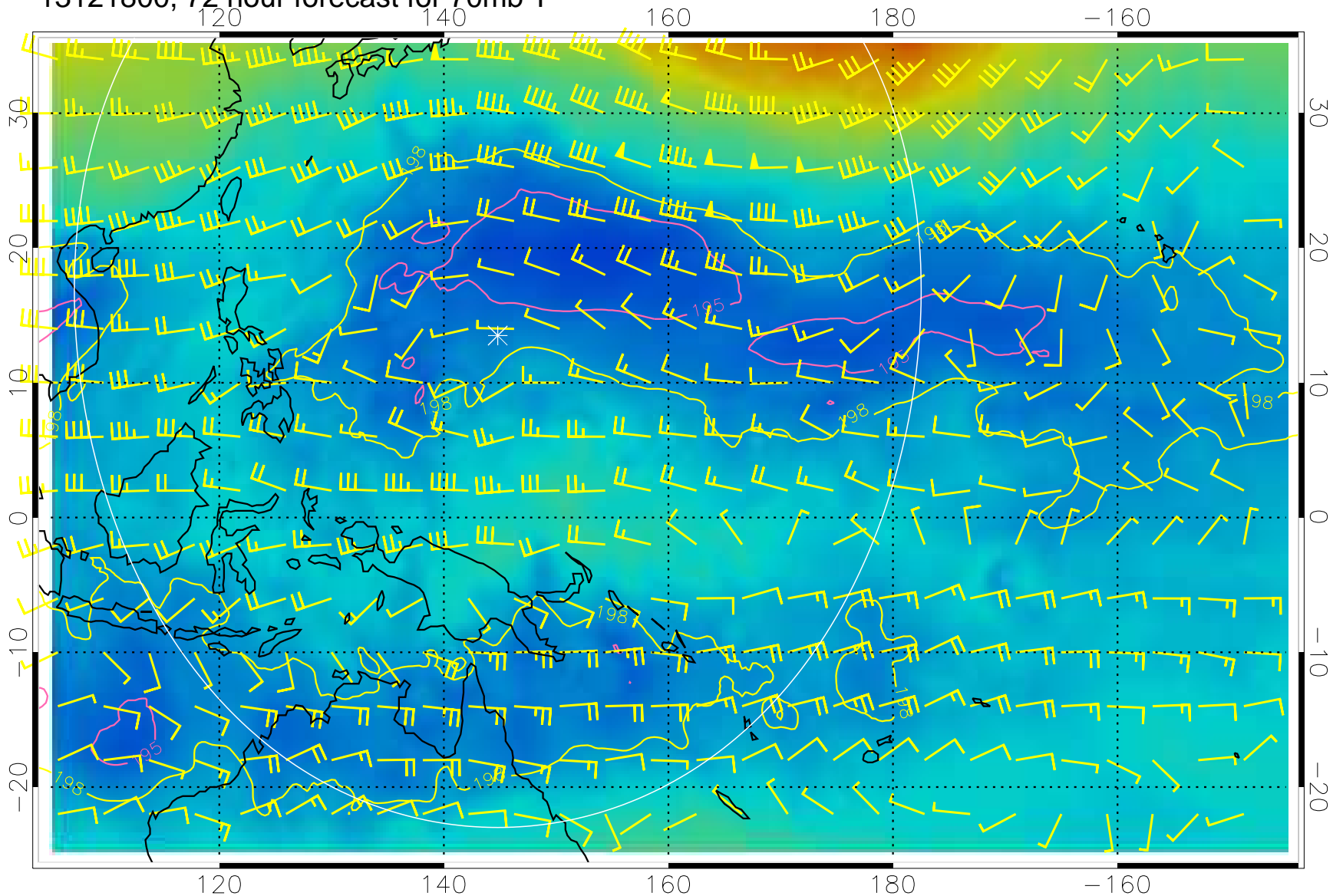
13121800, 72 hour forecast for 70mb T
