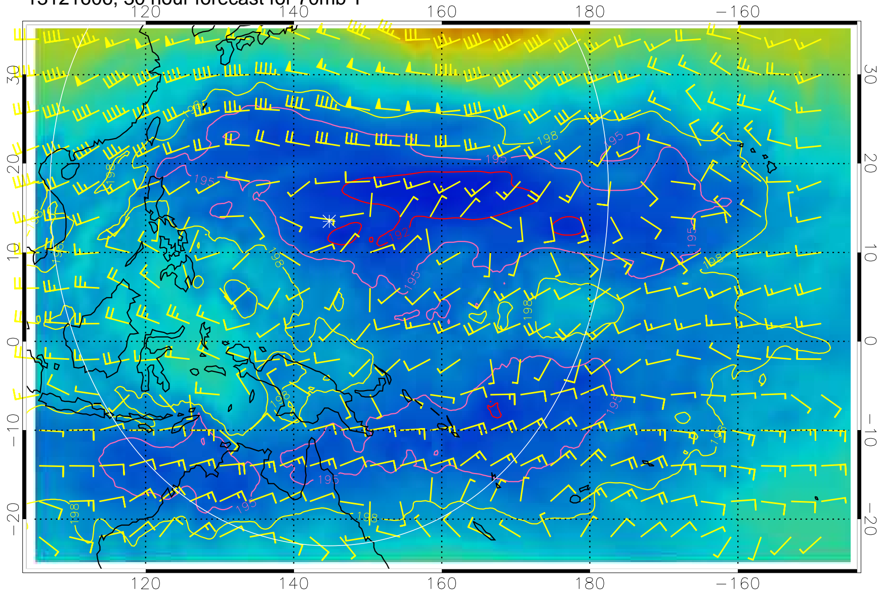
13121606, 30 hour forecast for 70mb T
