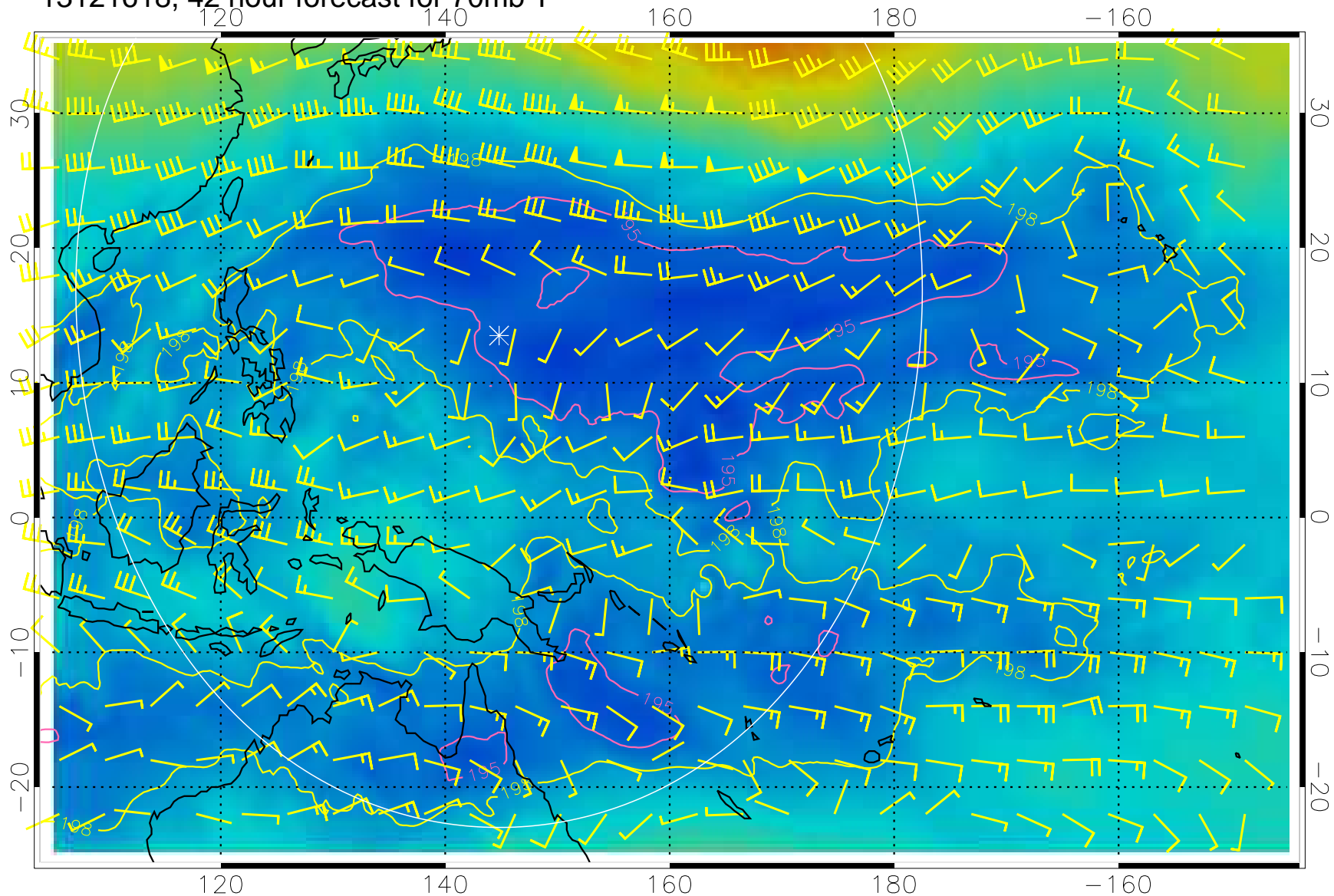
13121618, 42 hour forecast for 70mb T
