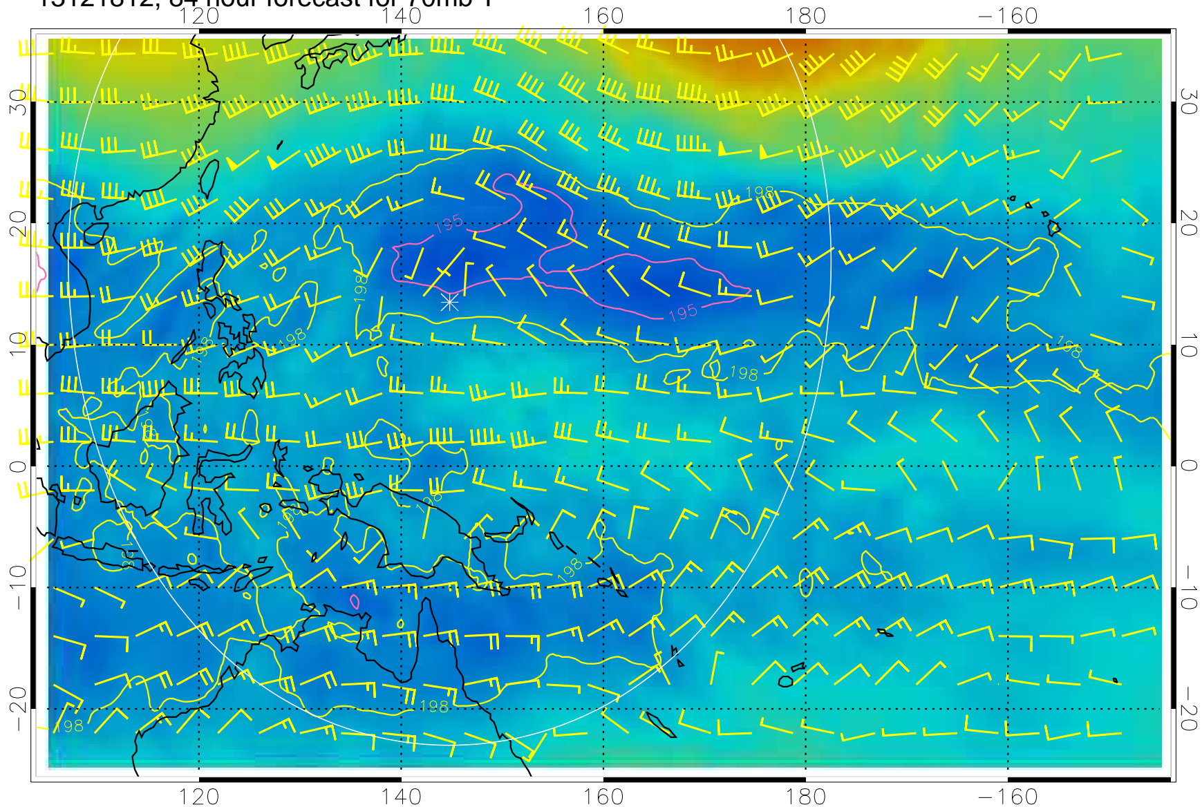
13121812, 84 hour forecast for 70mb T
