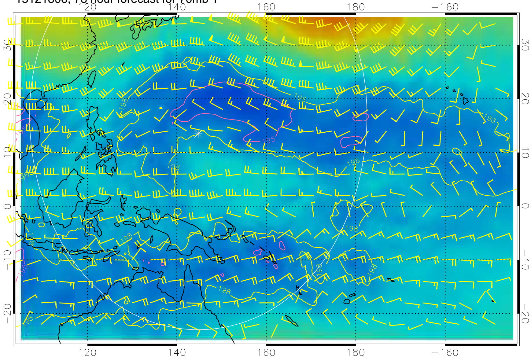
13121806, 78 hour forecast for 70mb T
