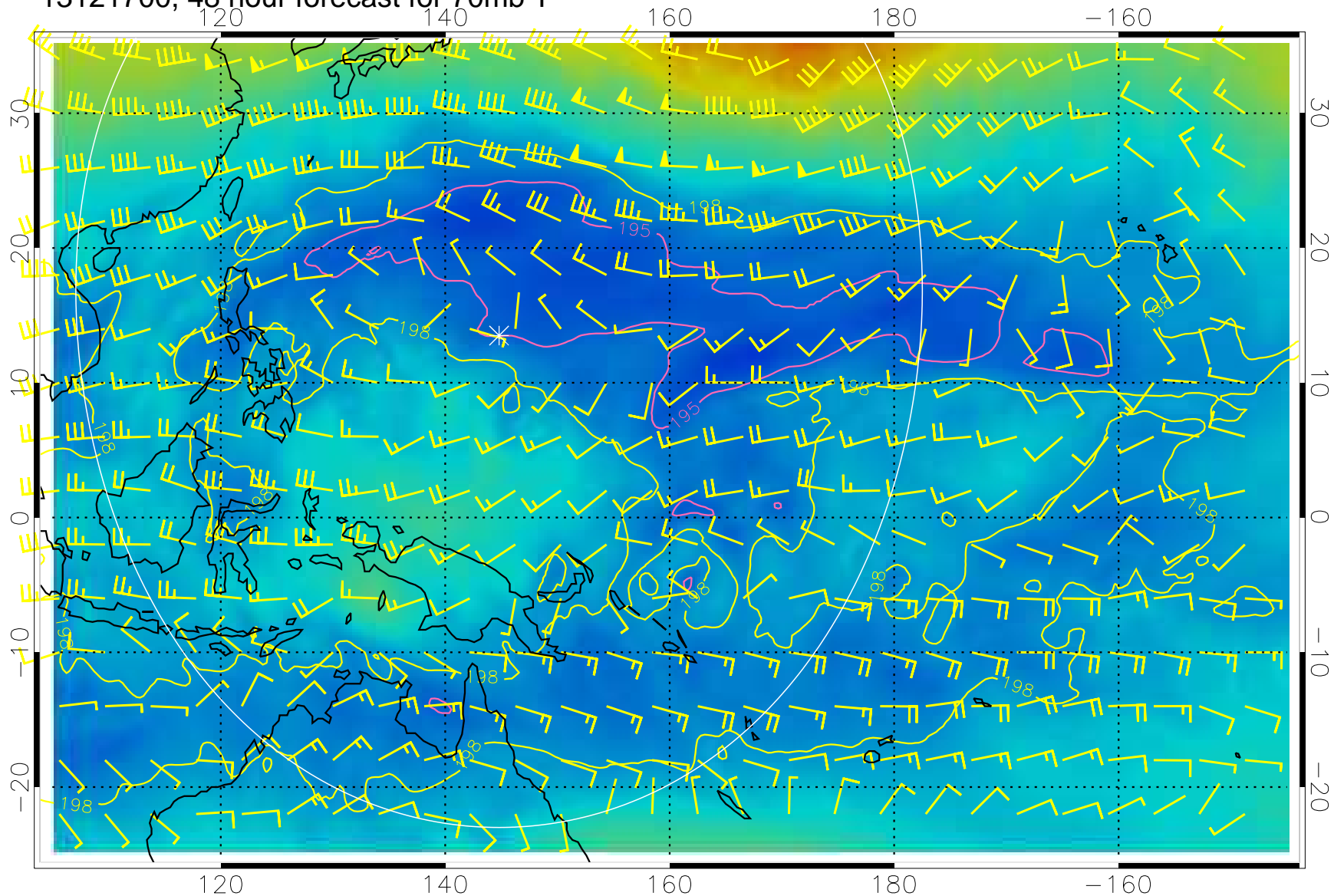
13121700, 48 hour forecast for 70mb T
