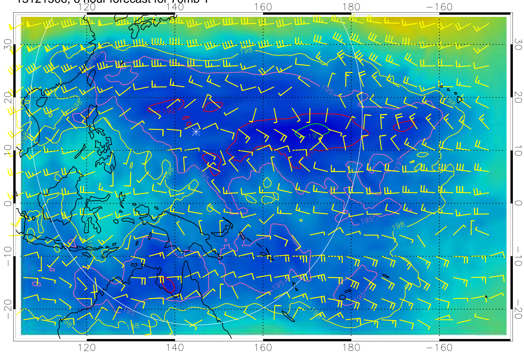
13121506, 6 hour forecast for 70mb T
