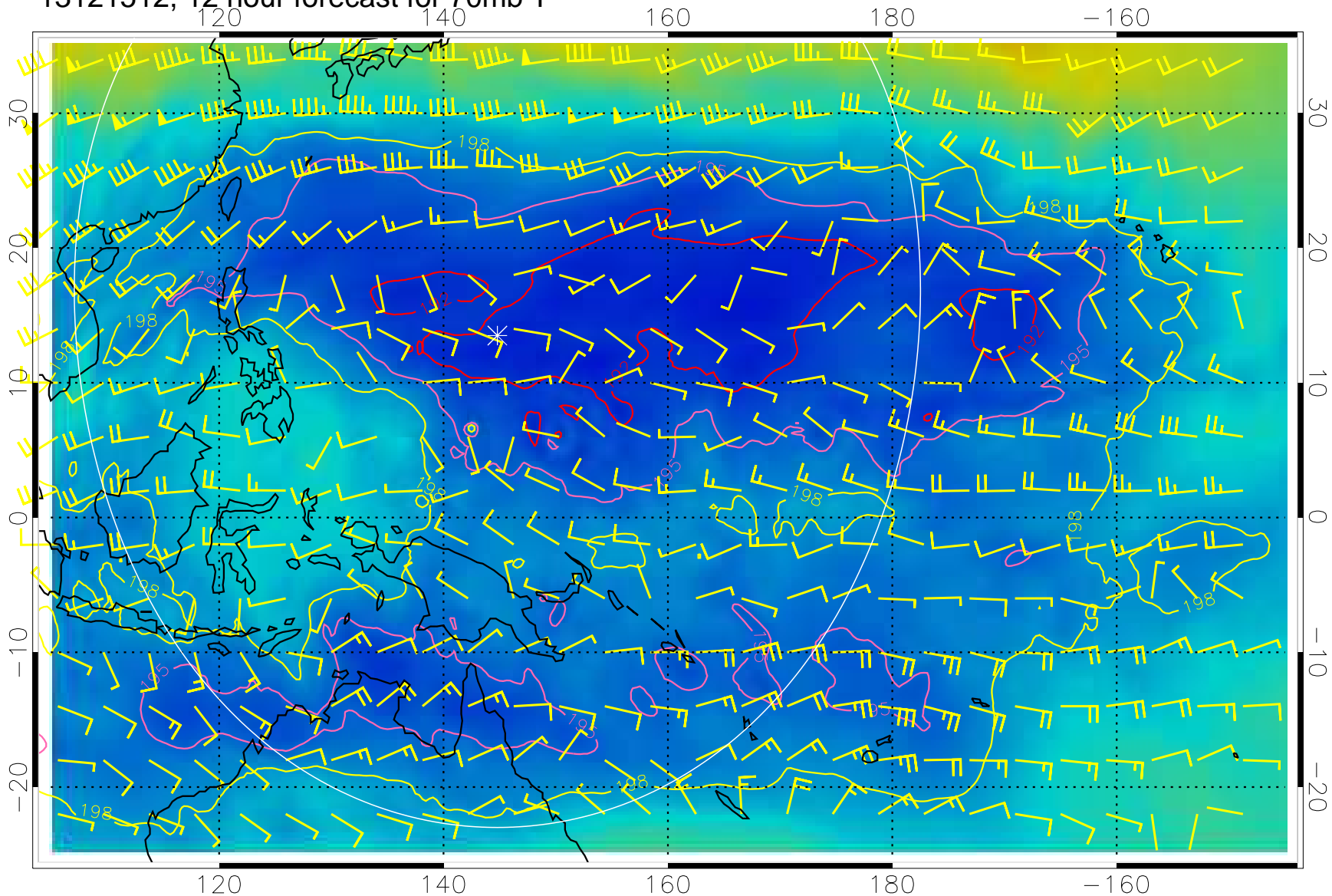
13121512, 12 hour forecast for 70mb T
