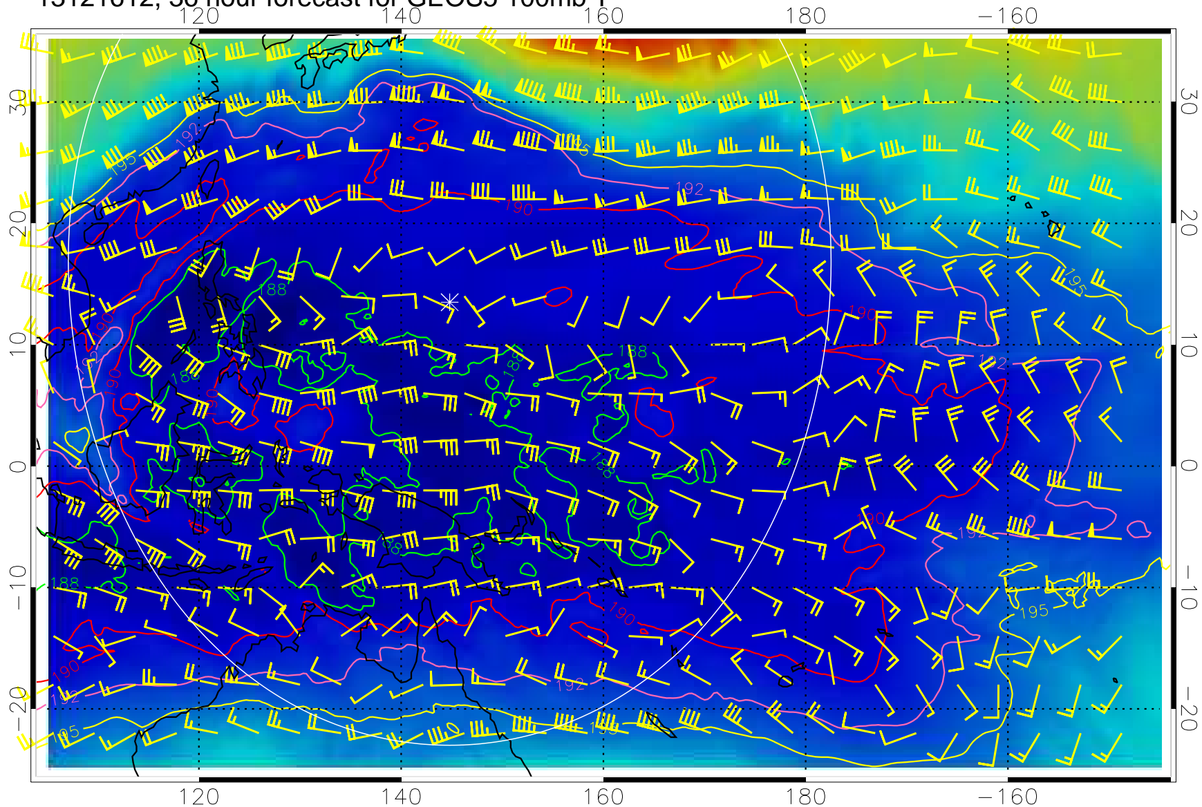
13121612, 36 hour forecast for GEOS5 100mb T
