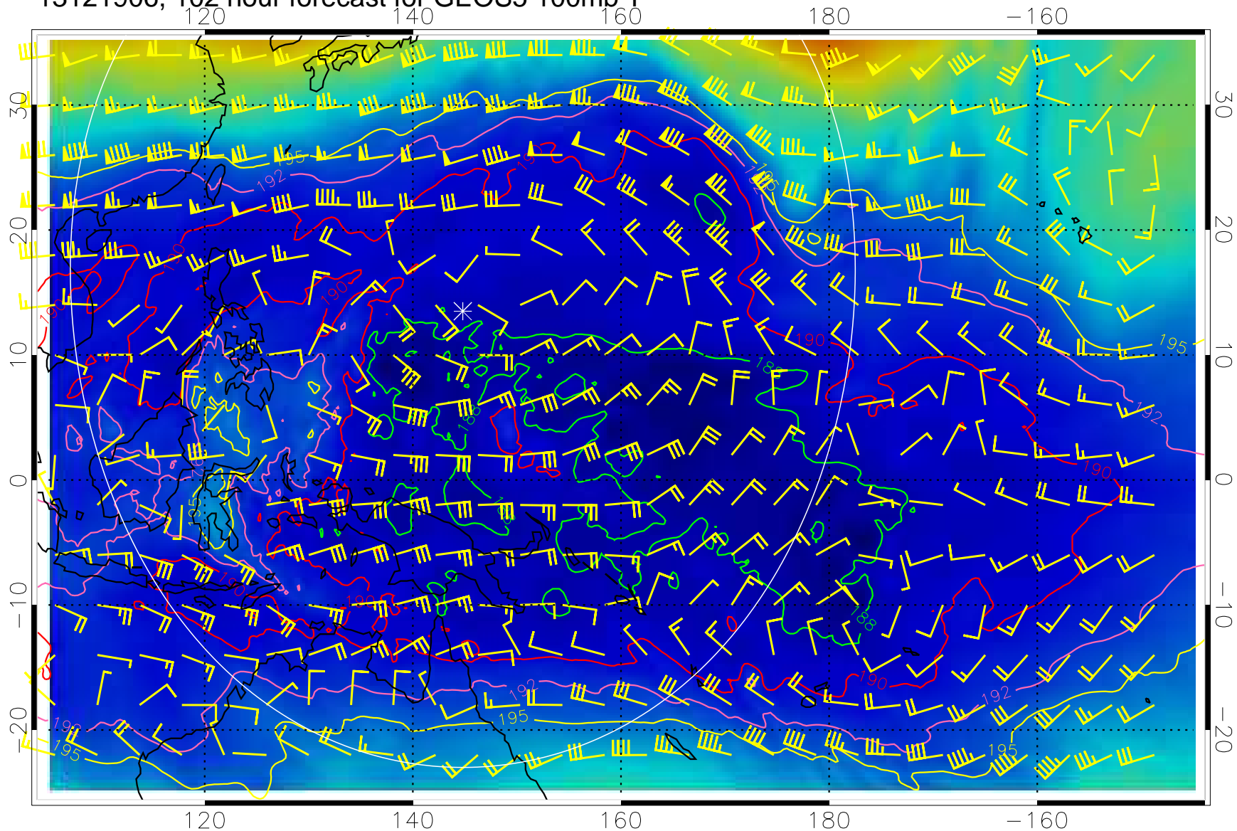
13121906, 102 hour forecast for GEOS5 100mb T
