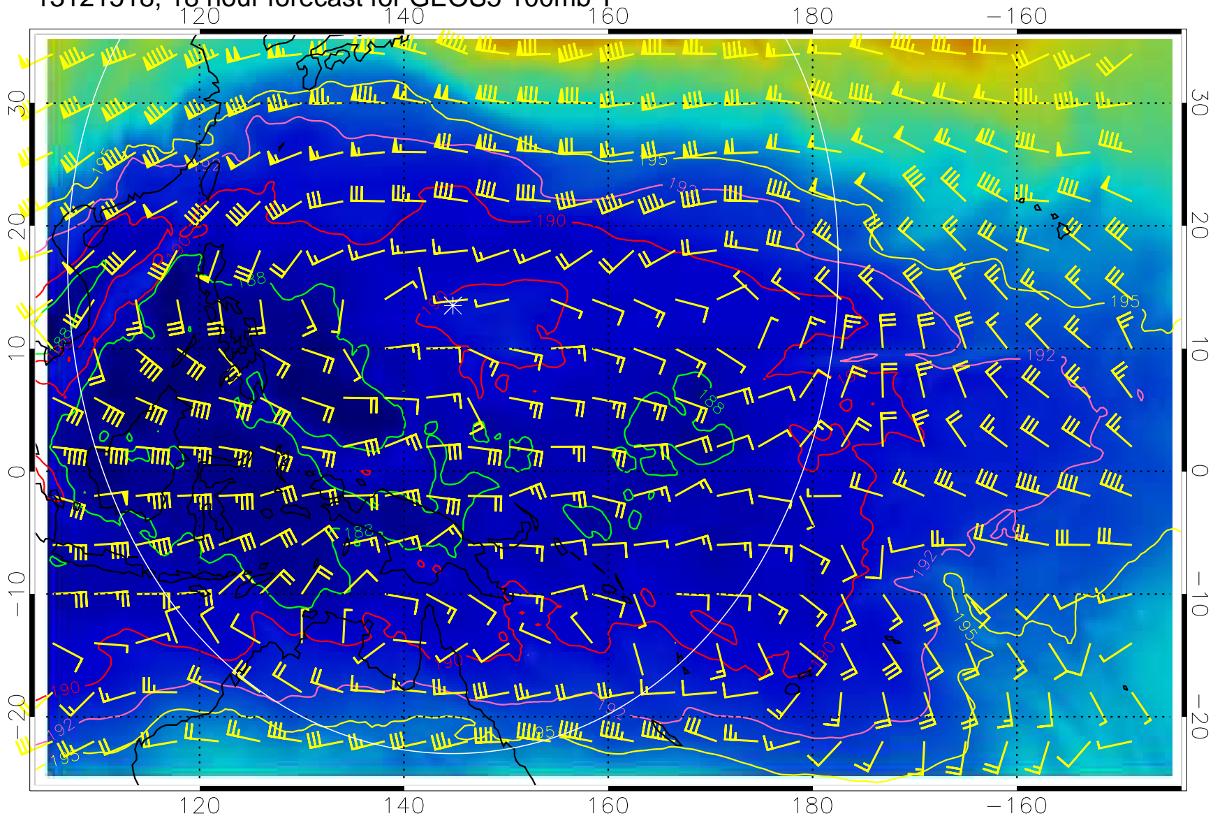
13121518, 18 hour forecast for GEOS5 100mb T
