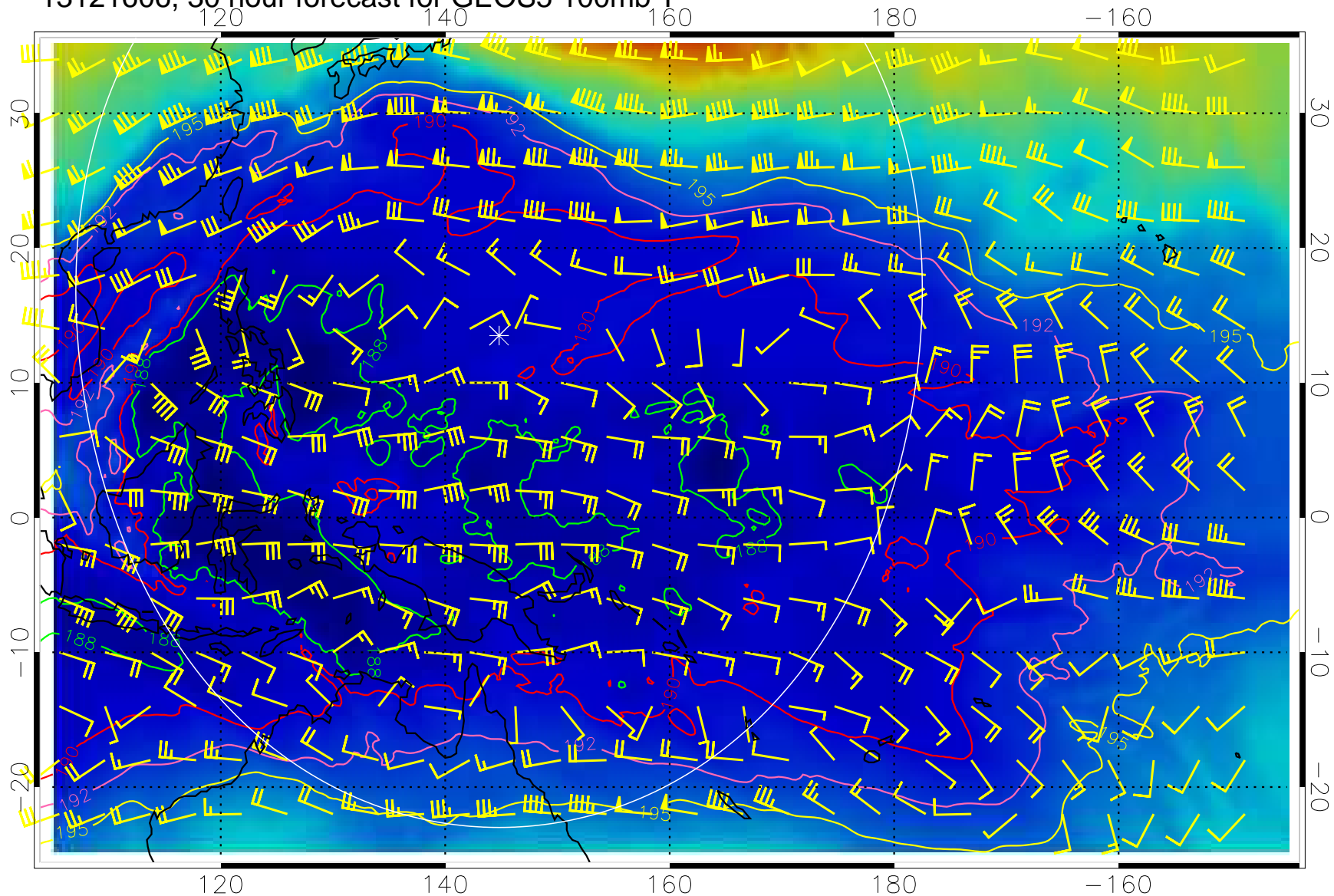
13121606, 30 hour forecast for GEOS5 100mb T
