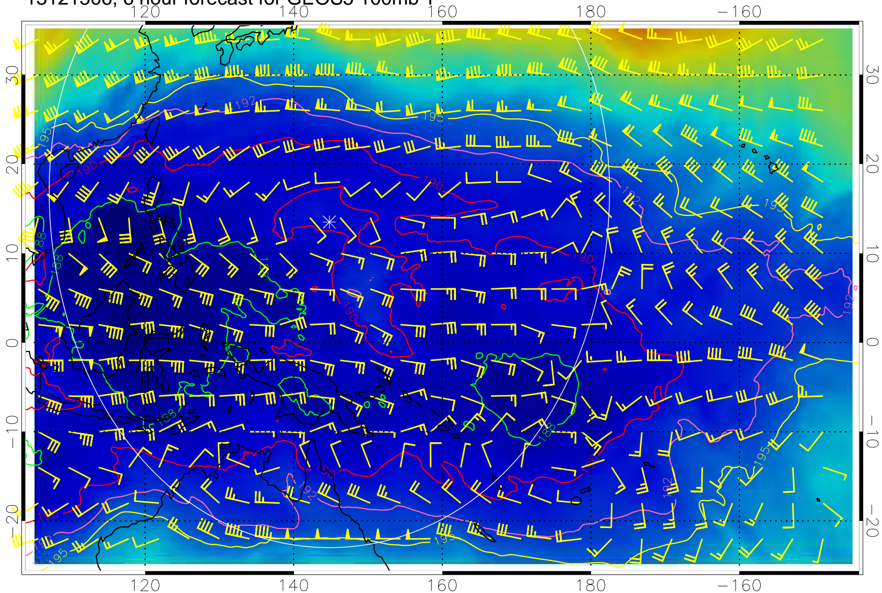
13121506, 6 hour forecast for GEOS5 100mb T
