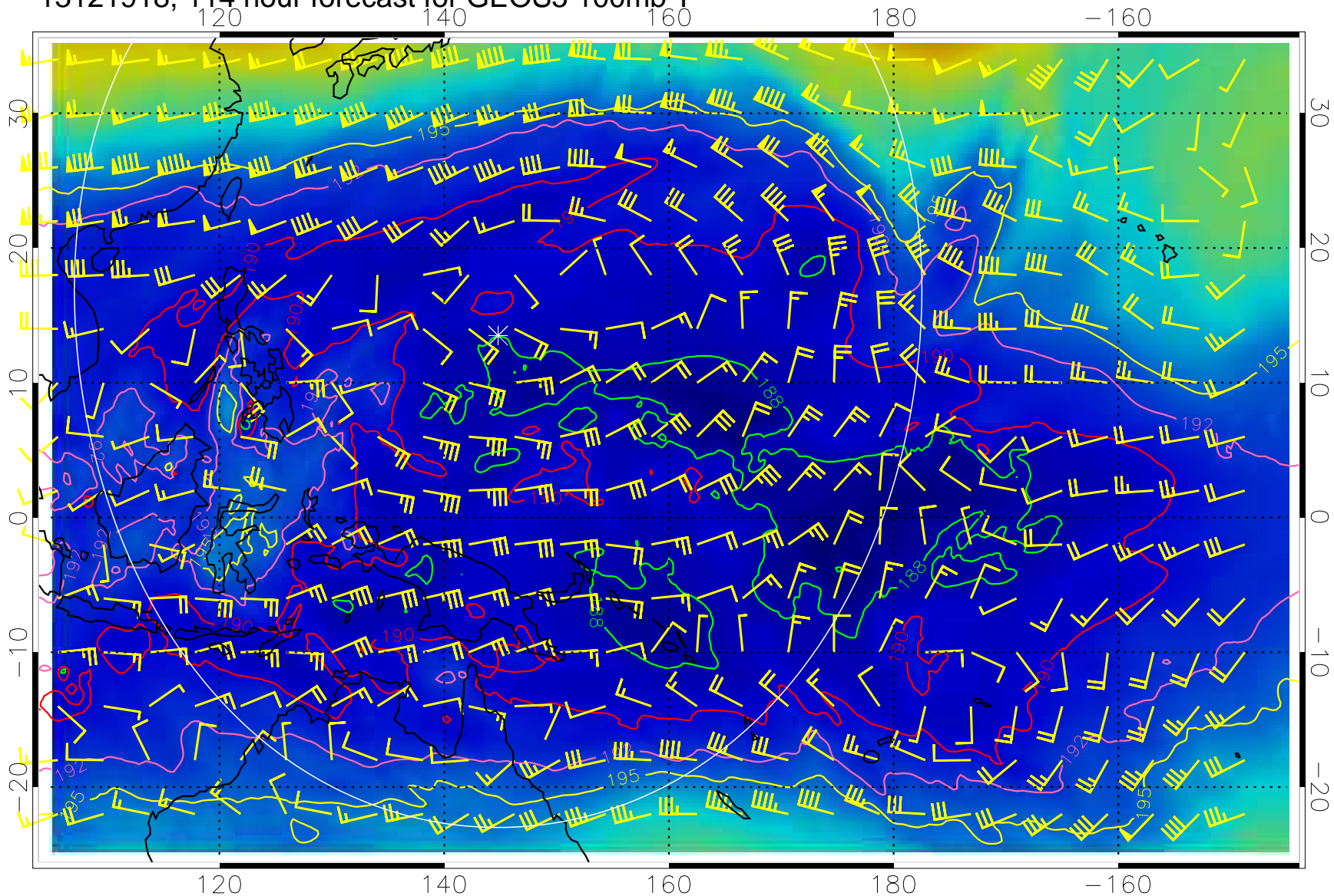
13121918, 114 hour forecast for GEOS5 100mb T
