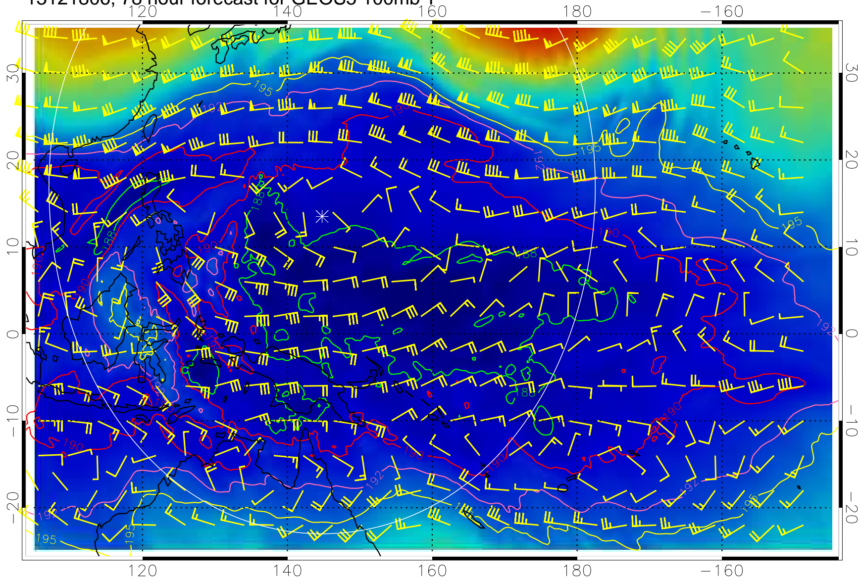
13121806, 78 hour forecast for GEOS5 100mb T
