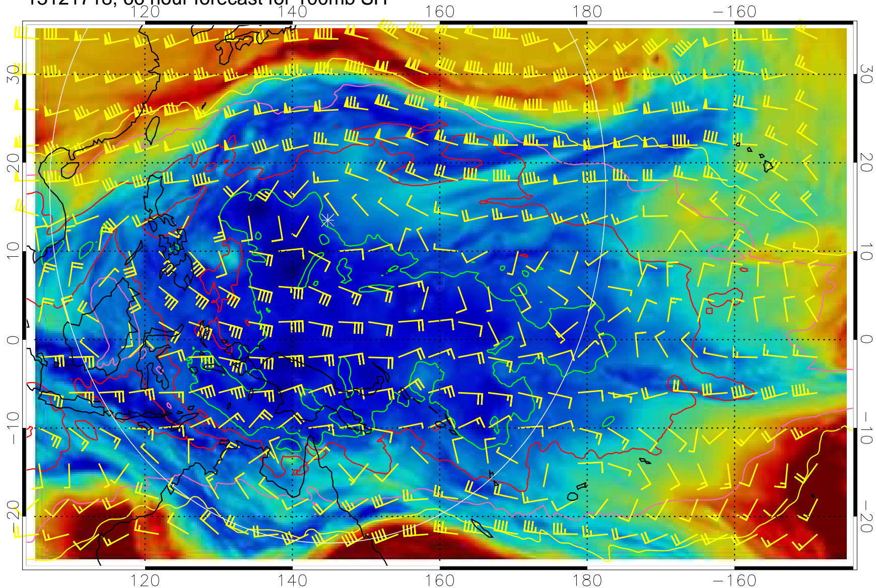
13121718, 66 hour forecast for 100mb SH
