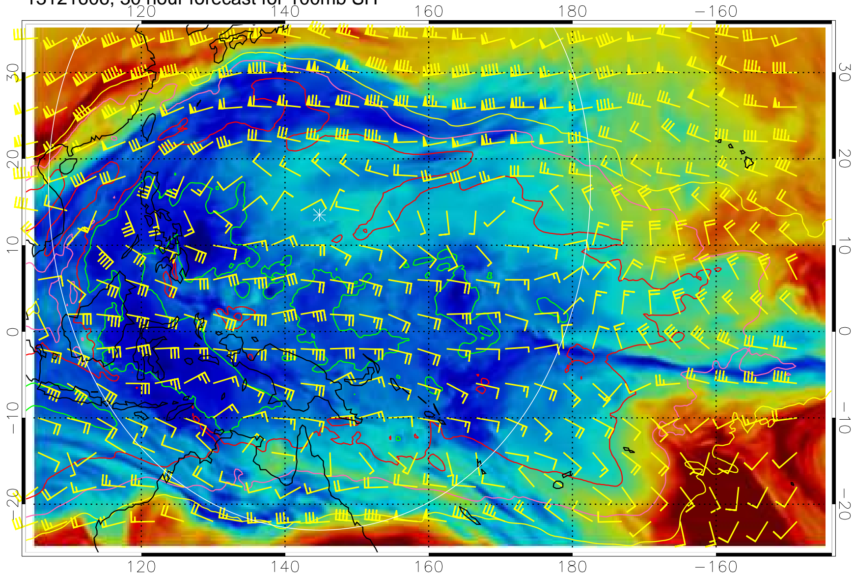
13121606, 30 hour forecast for 100mb SH
