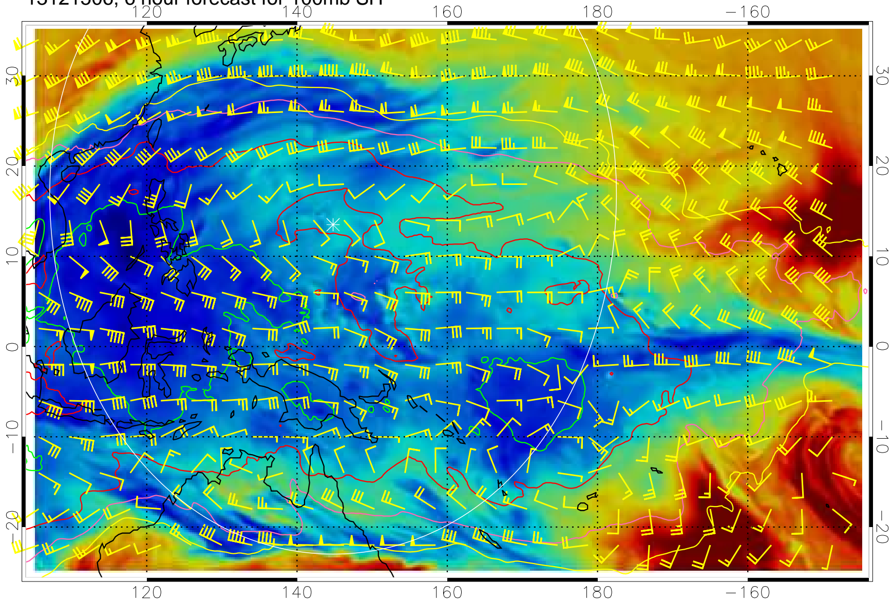
13121506, 6 hour forecast for 100mb SH
