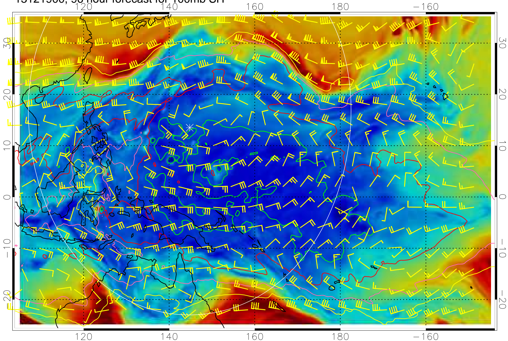
13121900, 96 hour forecast for 100mb SH
