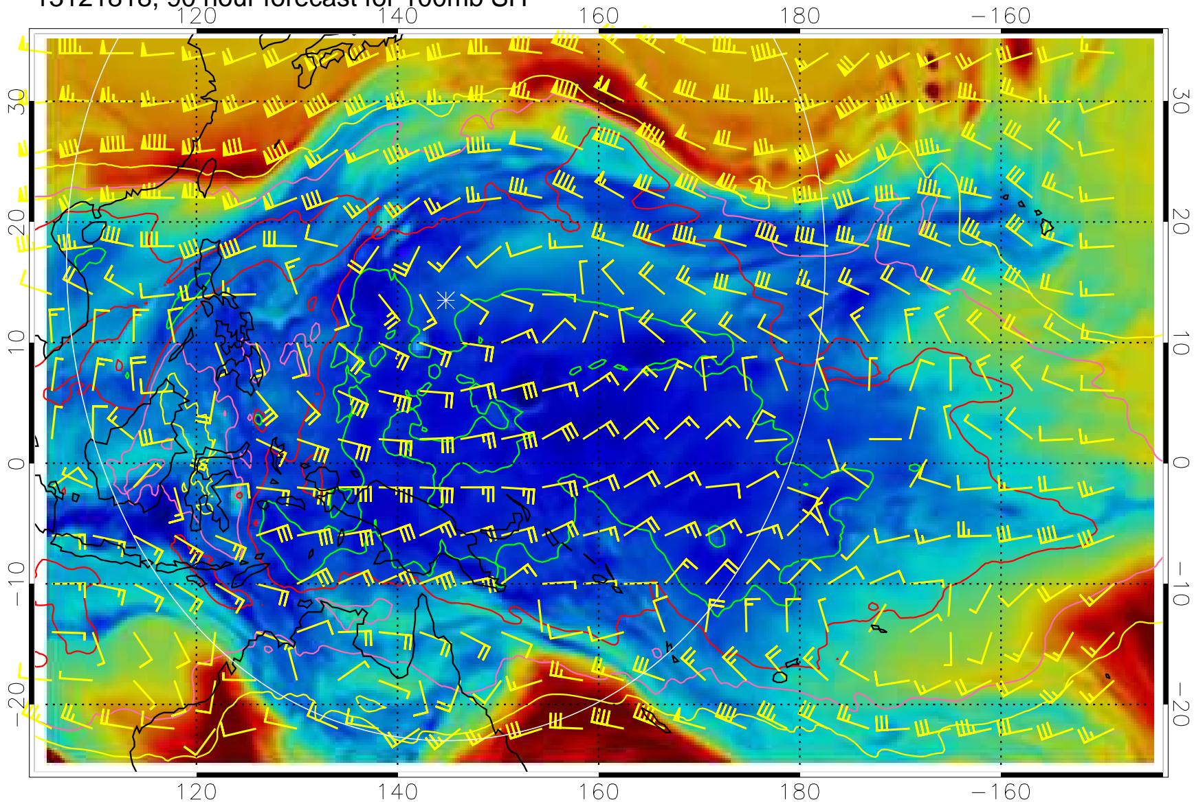
13121818, 90 hour forecast for 100mb SH
