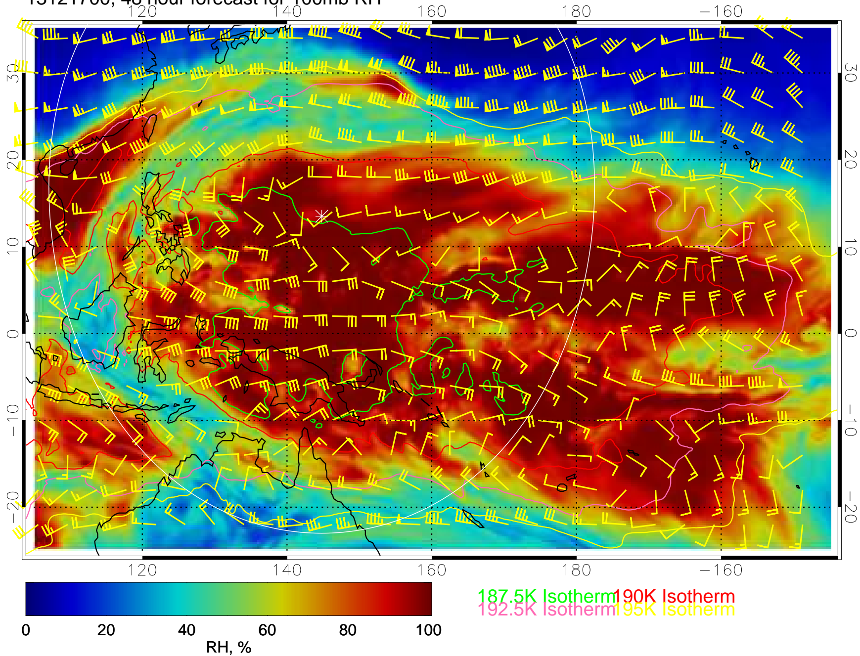
13121700, 48 hour forecast for 100mb RH
