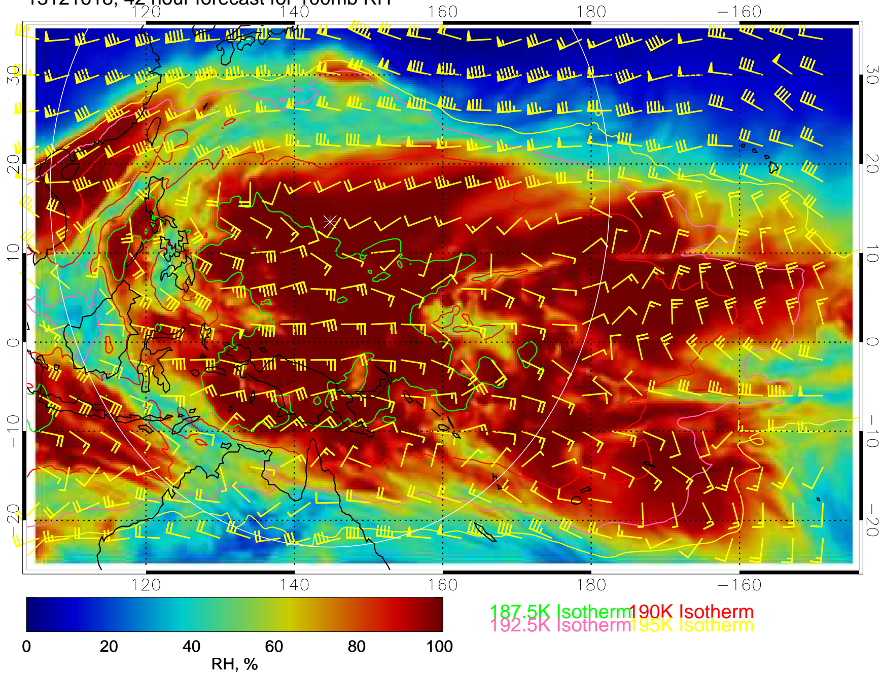
13121618, 42 hour forecast for 100mb RH
