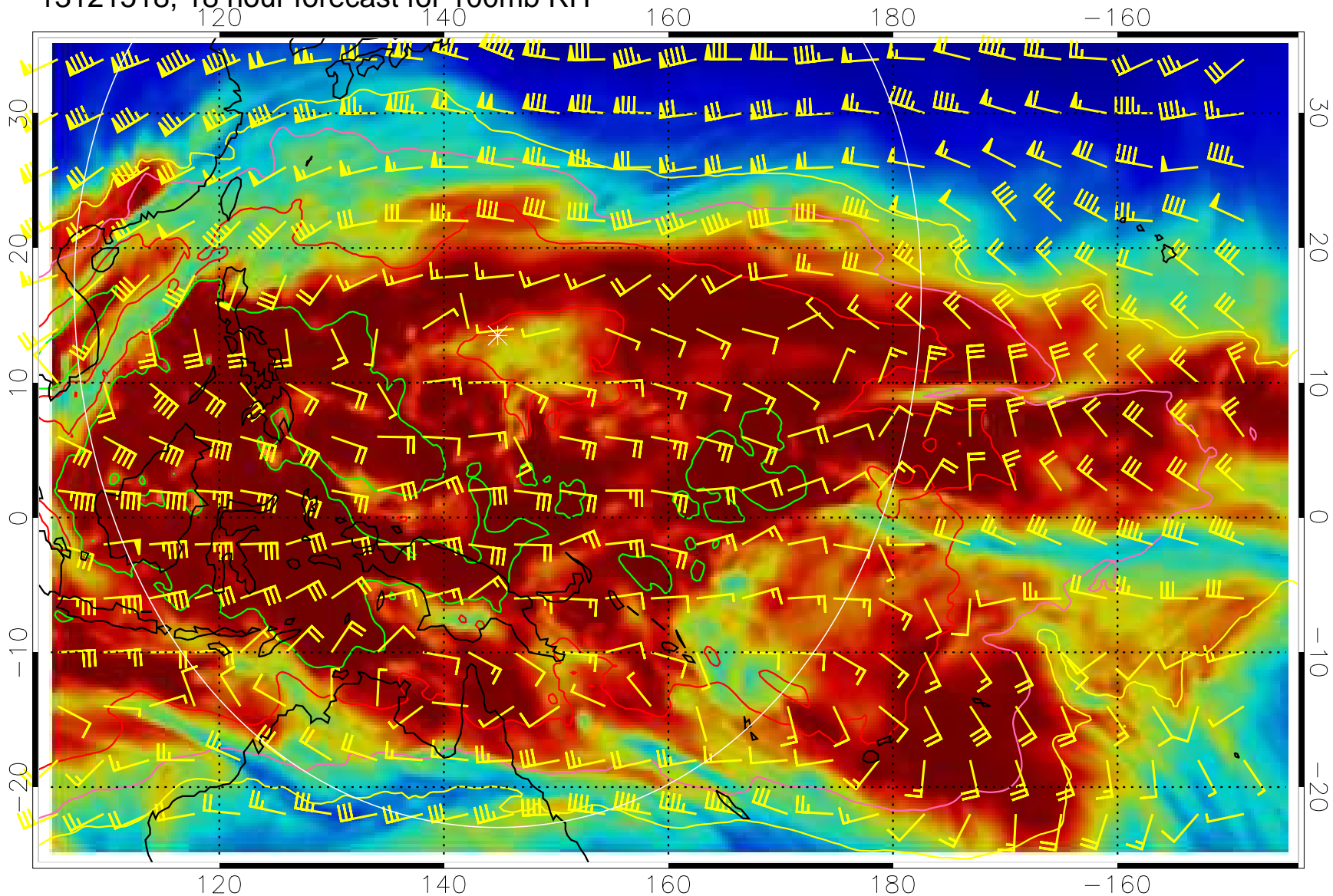
13121518, 18 hour forecast for 100mb RH
