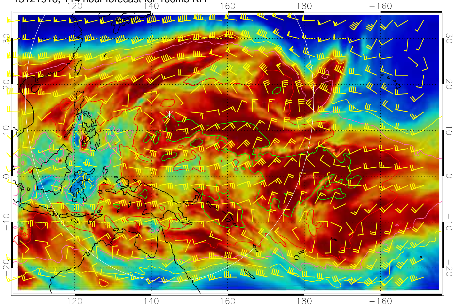
13121918, 114 hour forecast for 100mb RH
