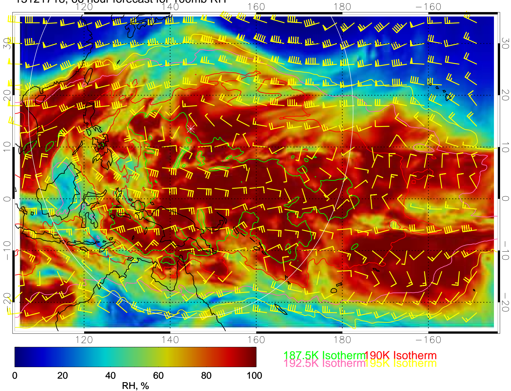
13121718, 66 hour forecast for 100mb RH
