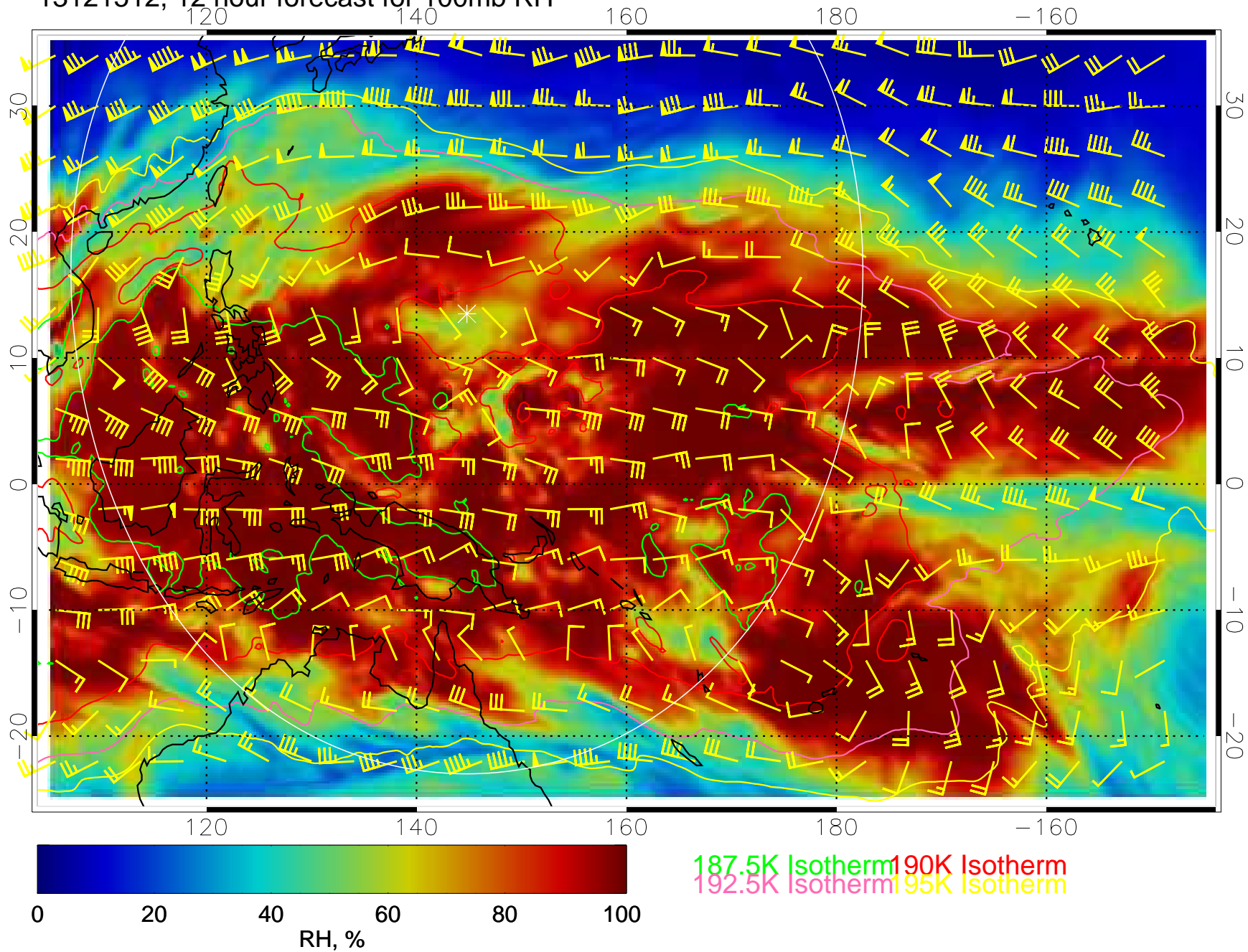
13121512, 12 hour forecast for 100mb RH
