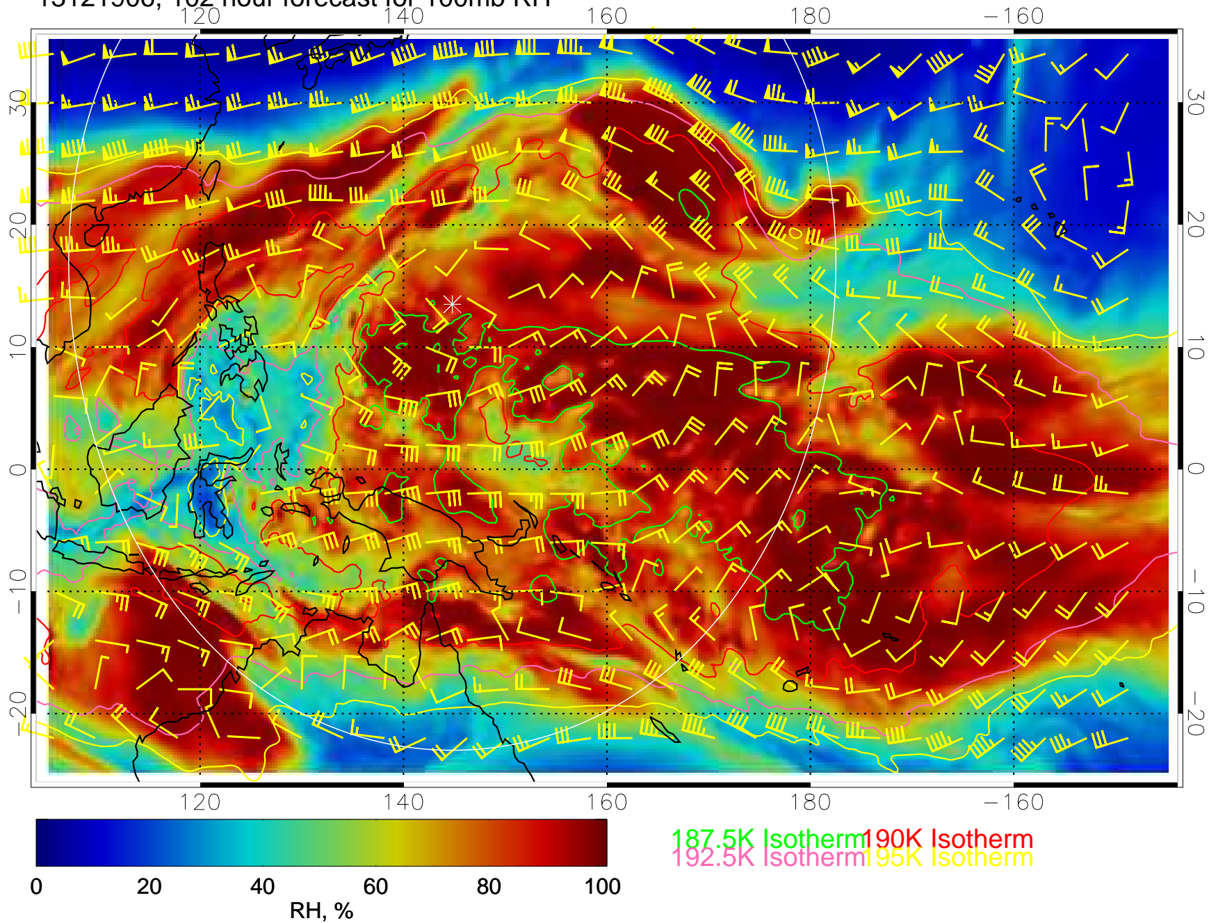
13121906, 102 hour forecast for 100mb RH
