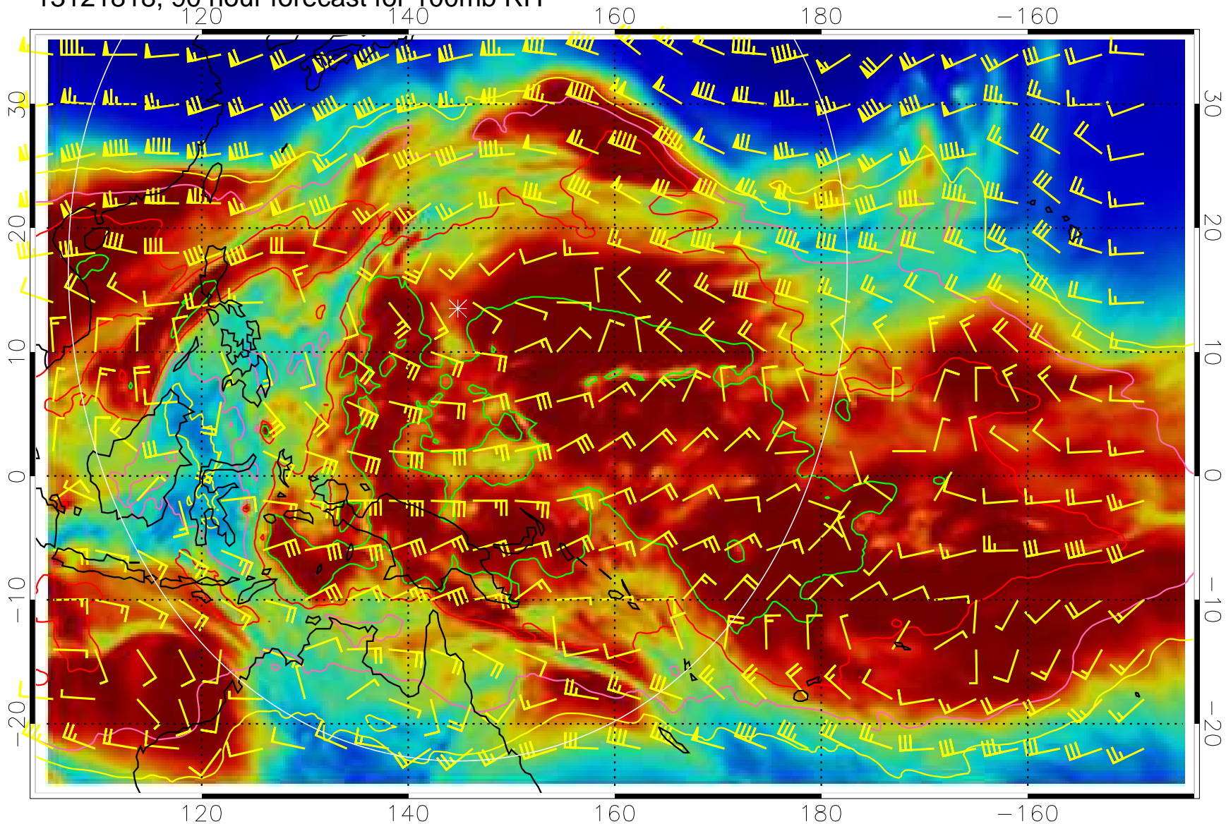
13121818, 90 hour forecast for 100mb RH
