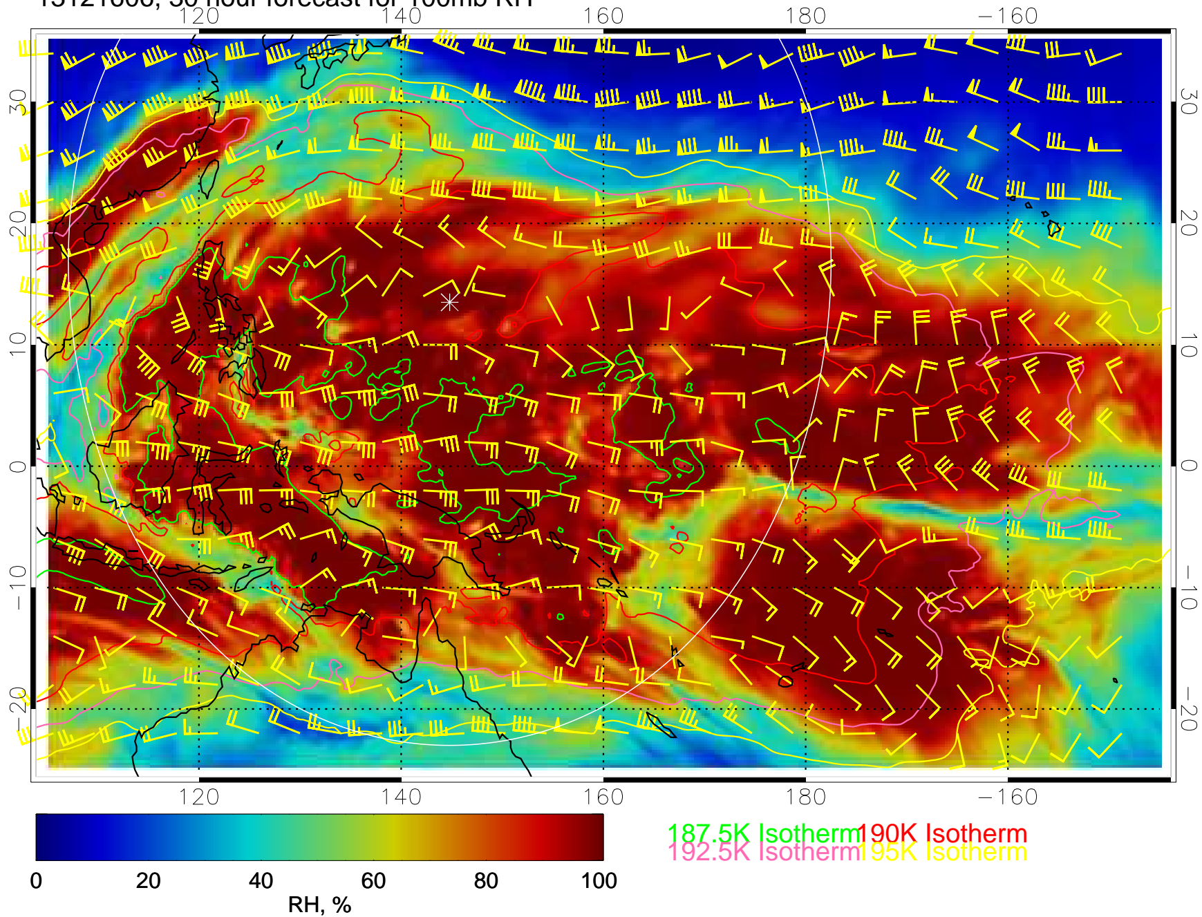
13121606, 30 hour forecast for 100mb RH
