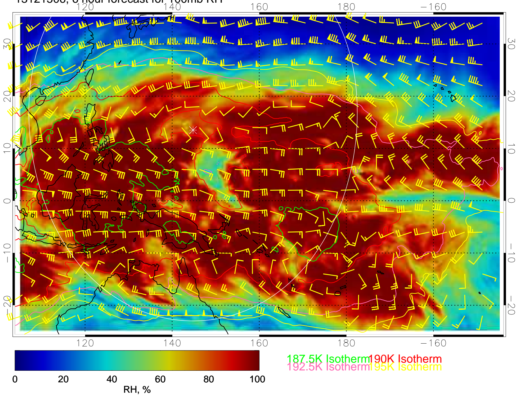
13121506, 6 hour forecast for 100mb RH
