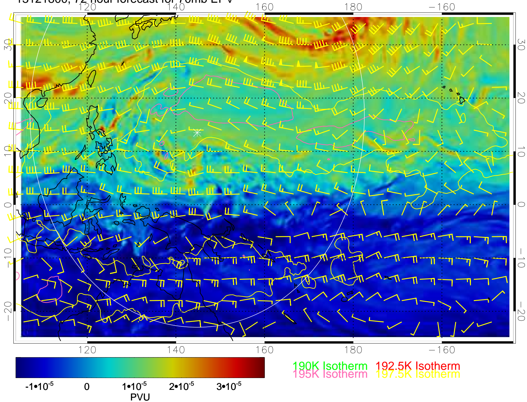
13121800, 72 hour forecast for 70mb EPV
