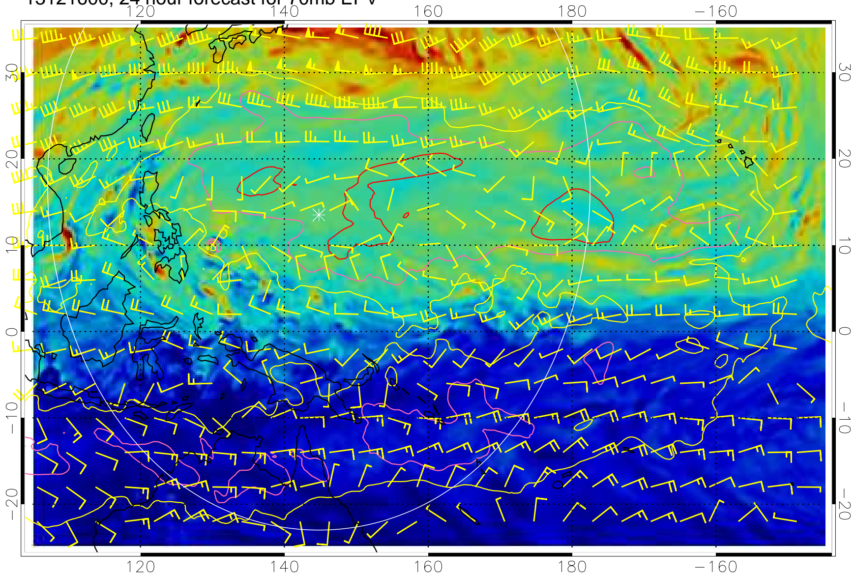
13121600, 24 hour forecast for 70mb EPV
