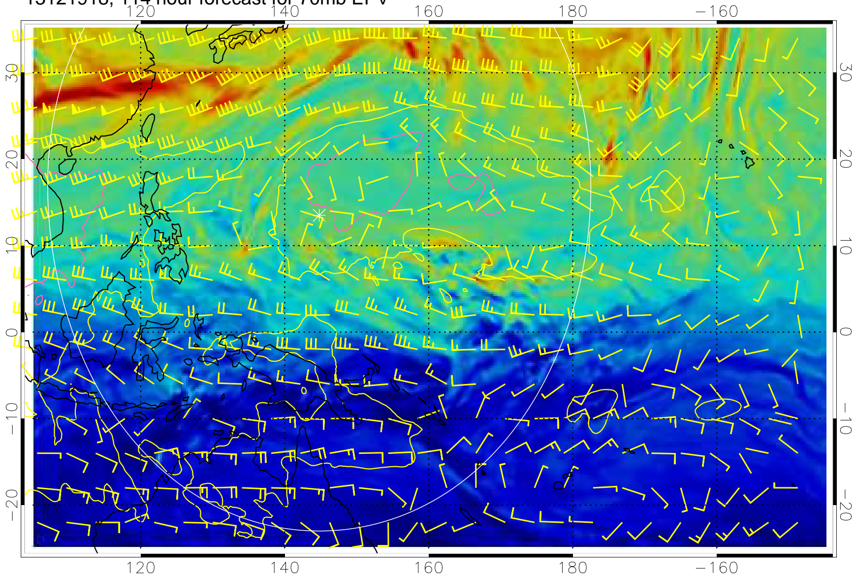
13121918, 114 hour forecast for 70mb EPV
