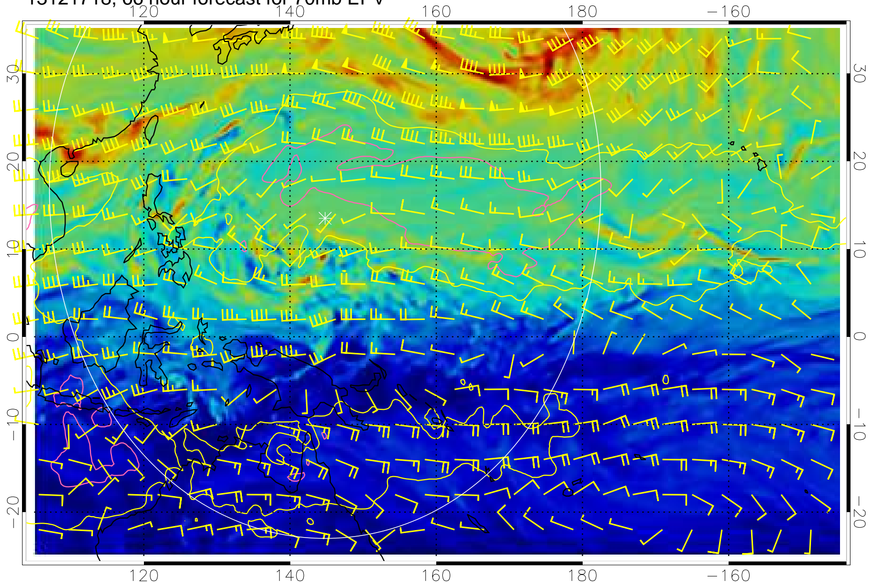
13121718, 66 hour forecast for 70mb EPV
