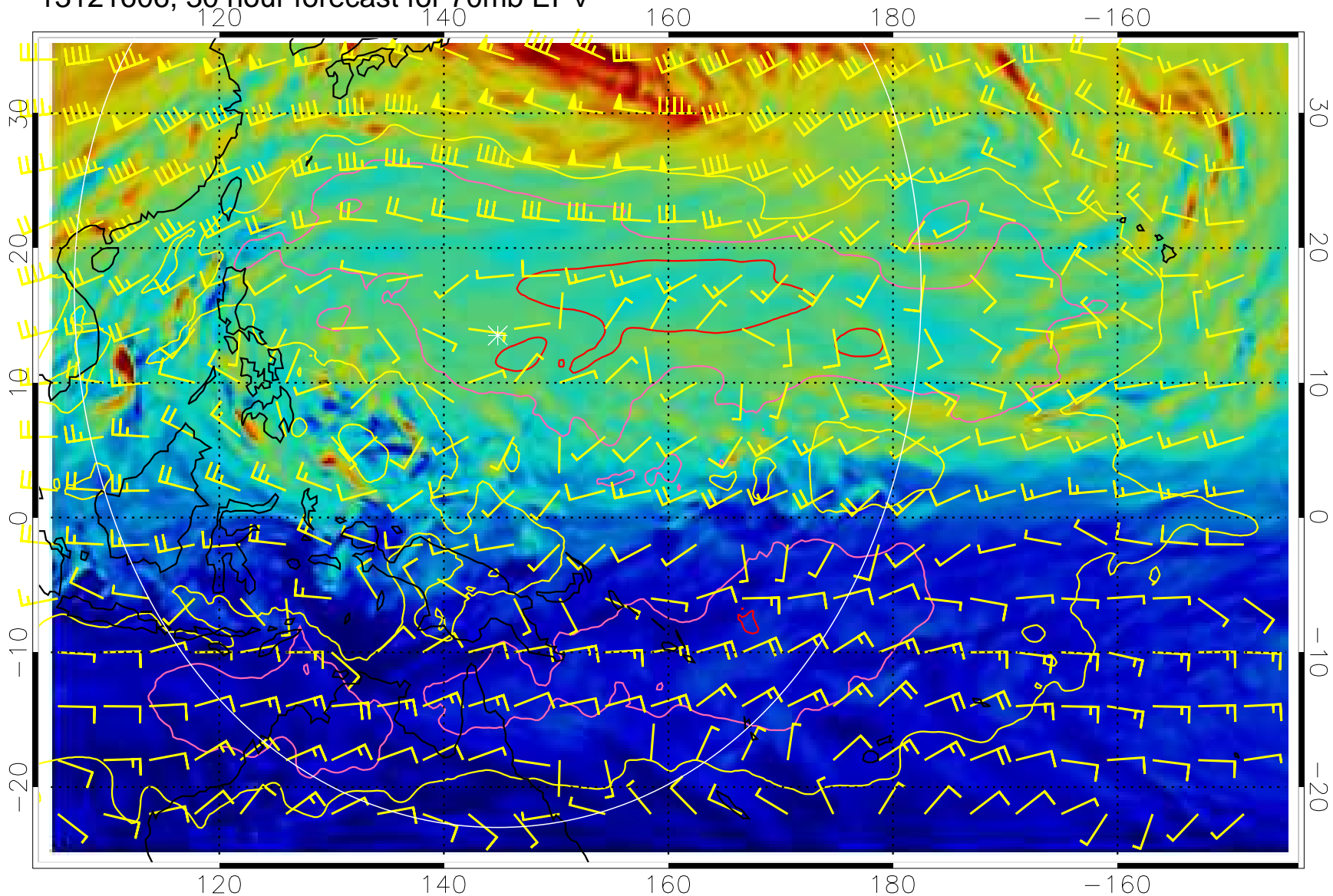
13121606, 30 hour forecast for 70mb EPV
