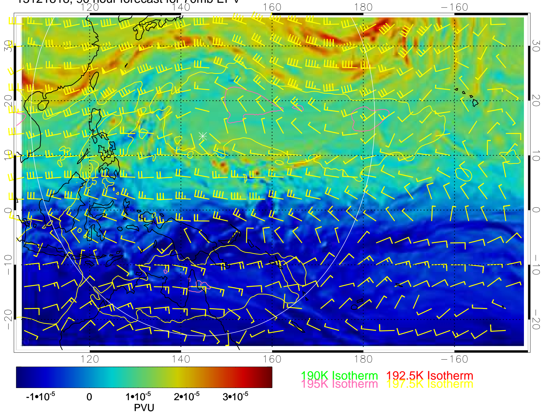
13121818, 90 hour forecast for 70mb EPV
