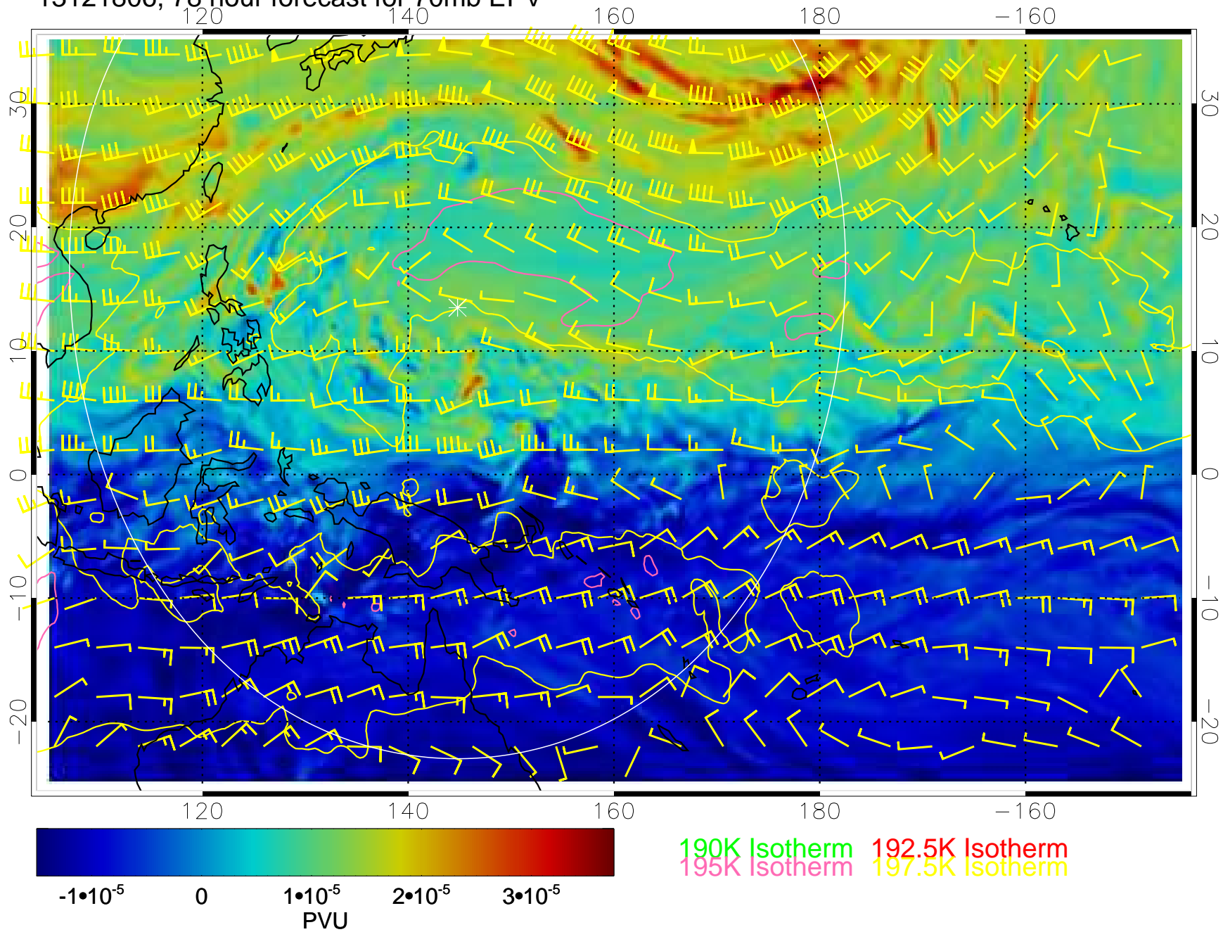
13121806, 78 hour forecast for 70mb EPV
