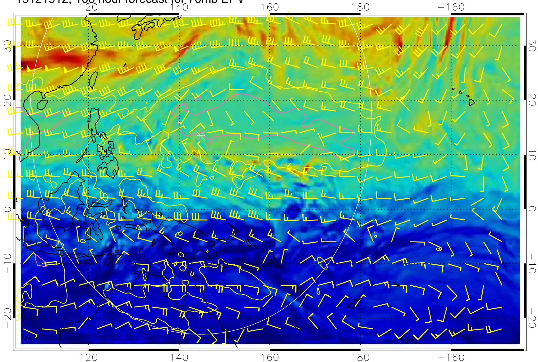
13121912, 108 hour forecast for 70mb EPV
