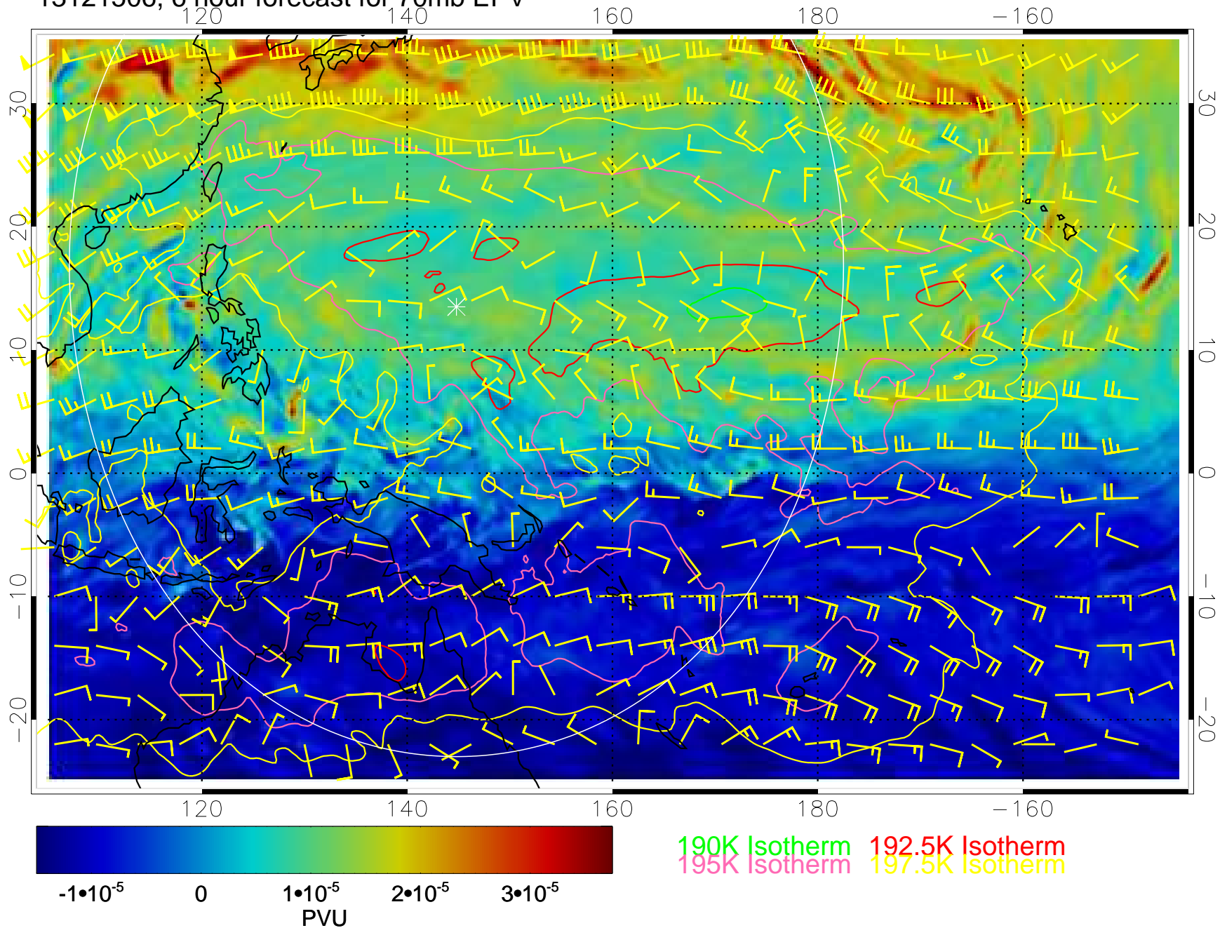
13121506, 6 hour forecast for 70mb EPV
