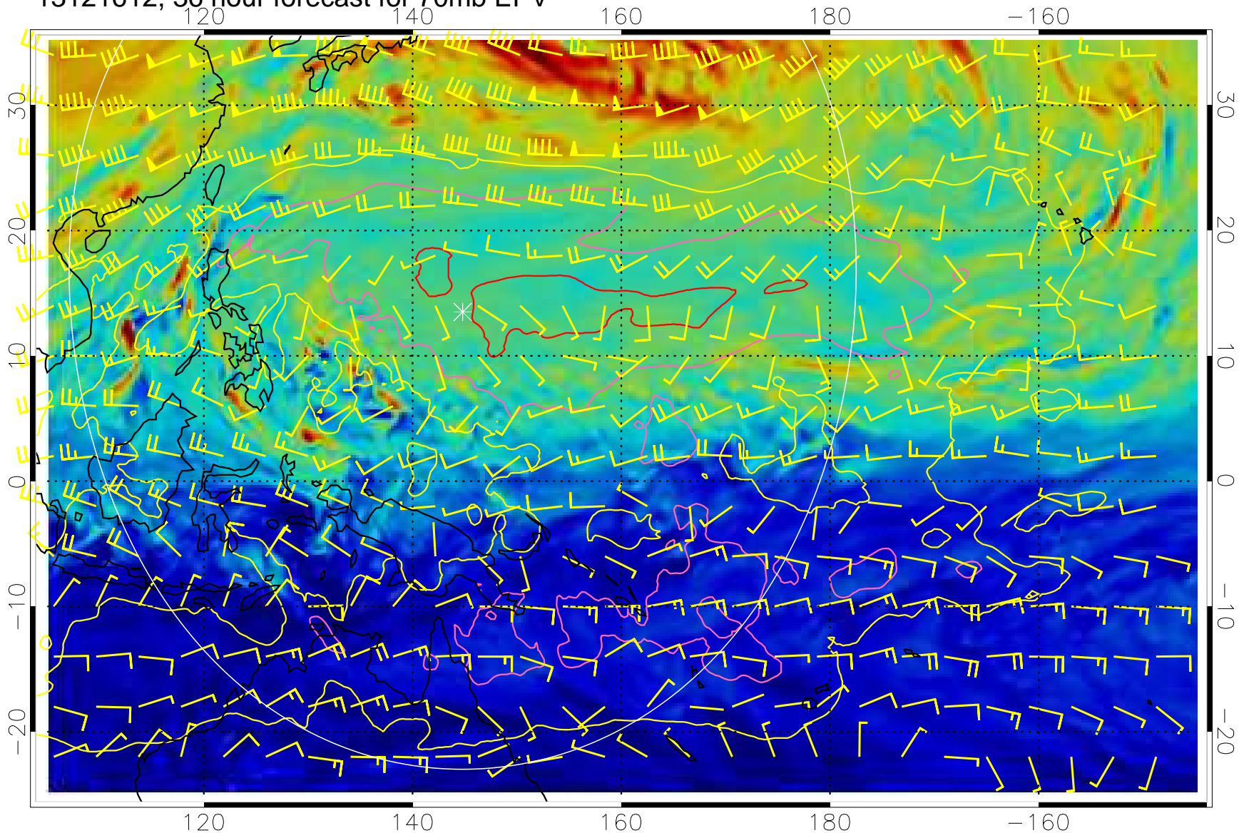
13121612, 36 hour forecast for 70mb EPV
