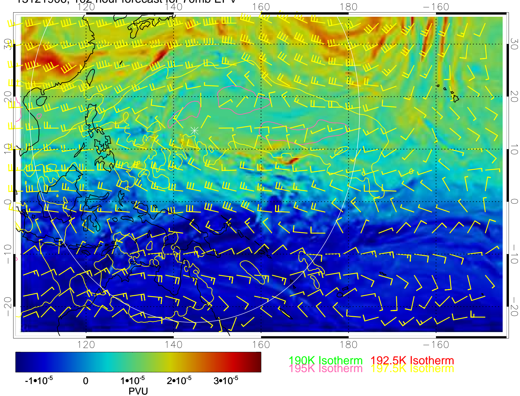
13121906, 102 hour forecast for 70mb EPV
