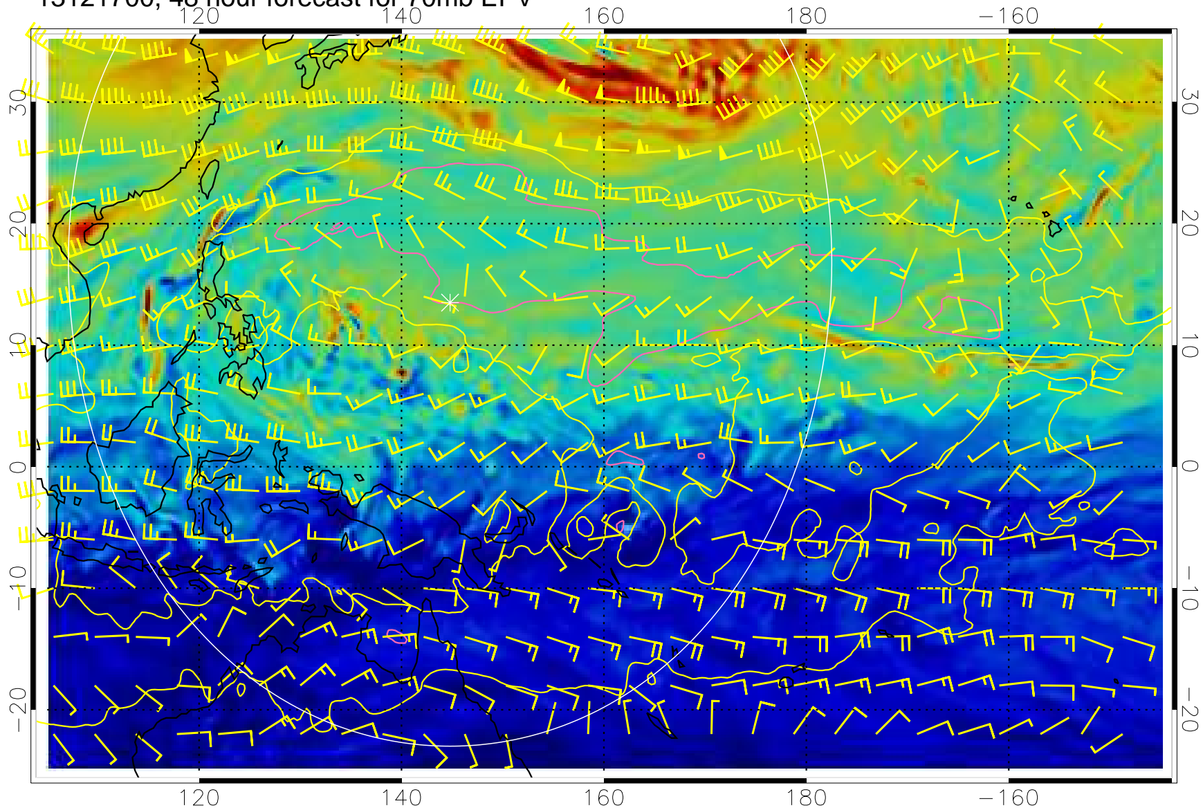
13121700, 48 hour forecast for 70mb EPV
