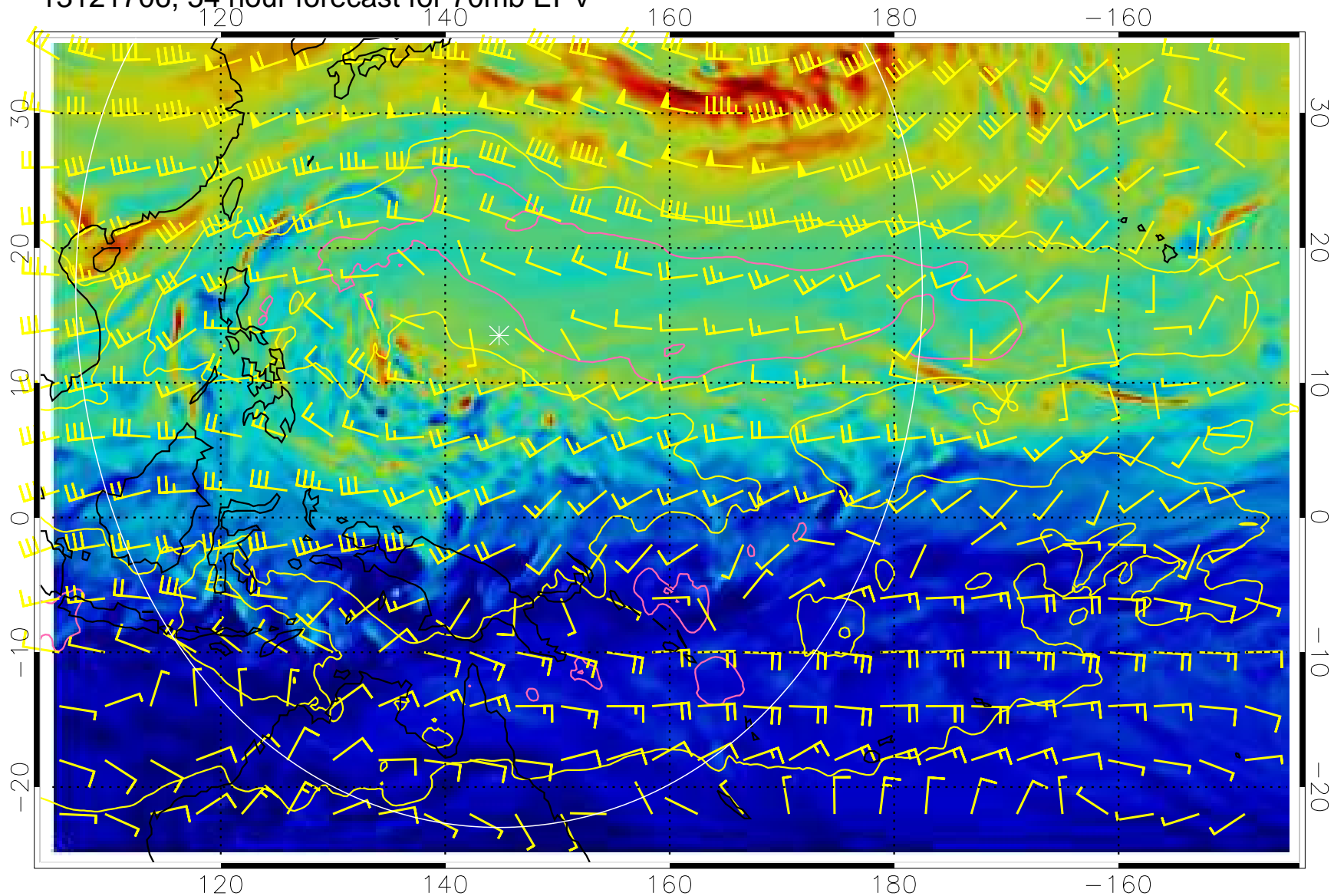
13121706, 54 hour forecast for 70mb EPV
