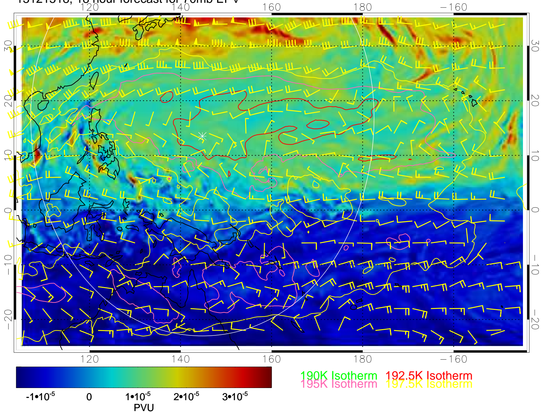
13121518, 18 hour forecast for 70mb EPV
