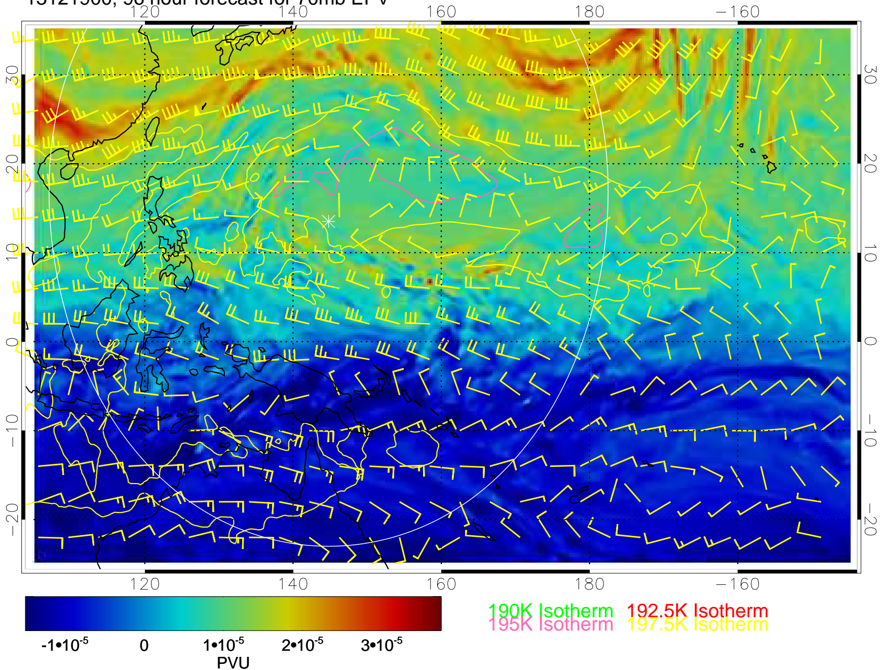
13121900, 96 hour forecast for 70mb EPV
