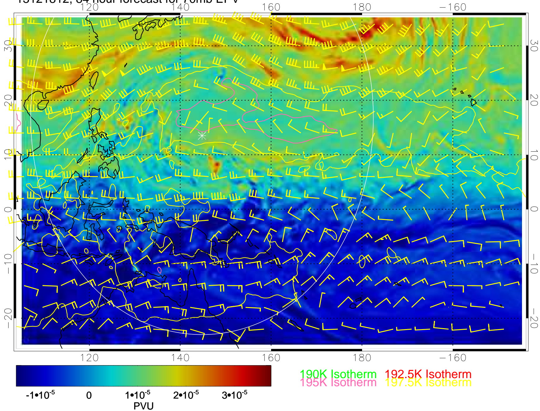
13121812, 84 hour forecast for 70mb EPV
