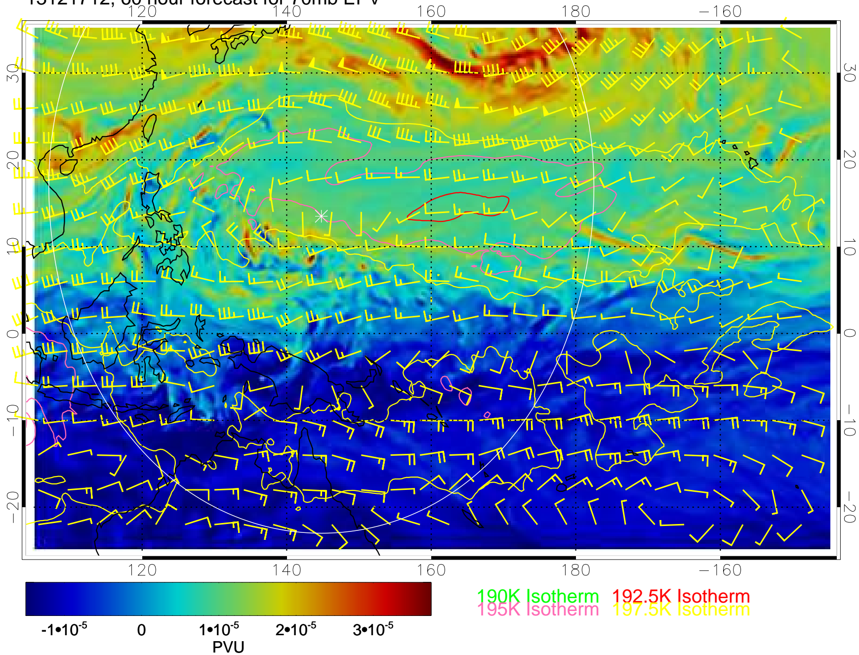
13121712, 60 hour forecast for 70mb EPV
