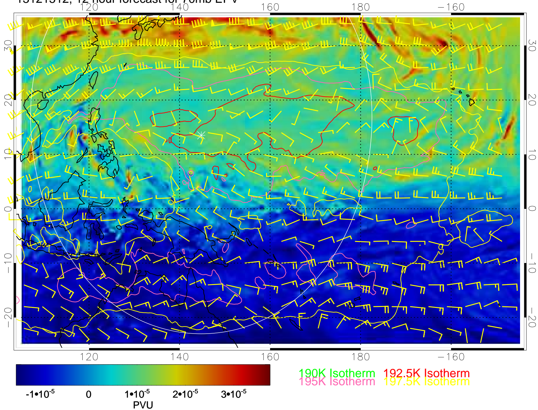
13121512, 12 hour forecast for 70mb EPV
