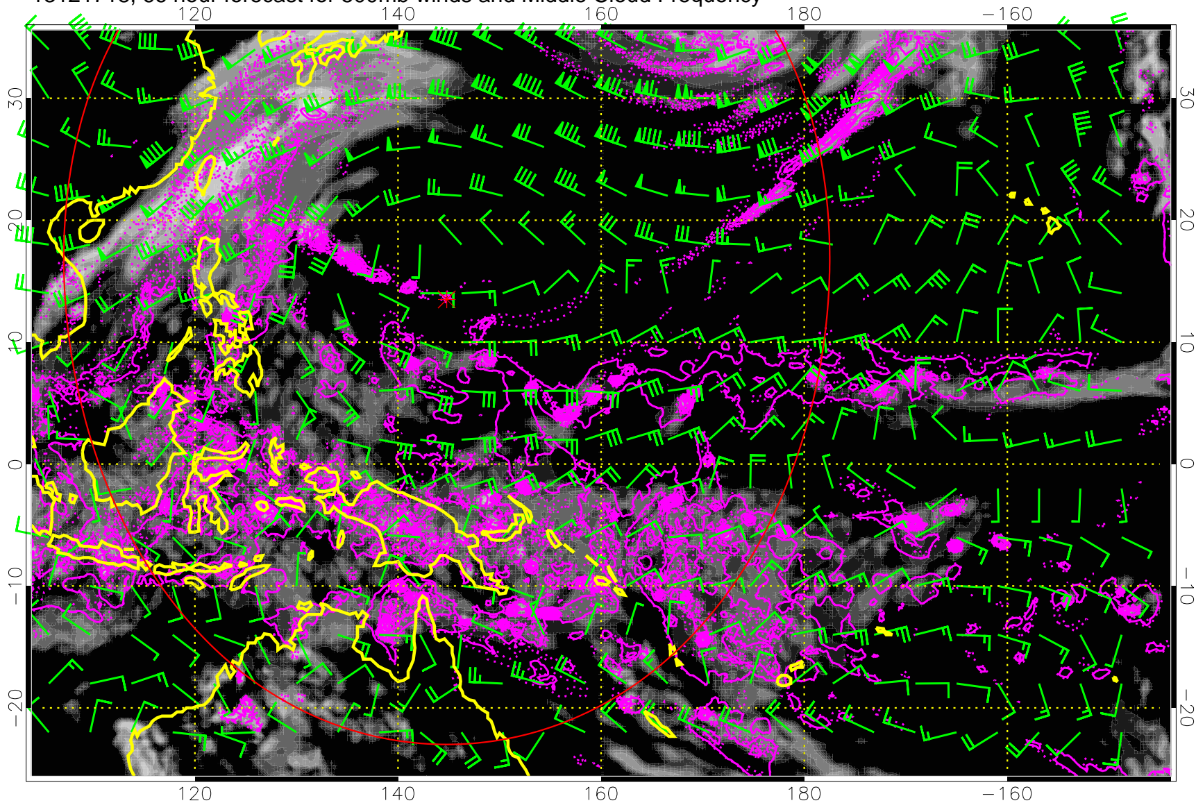
13121718, 66 hour forecast for 500mb winds and Middle Cloud Frequency
