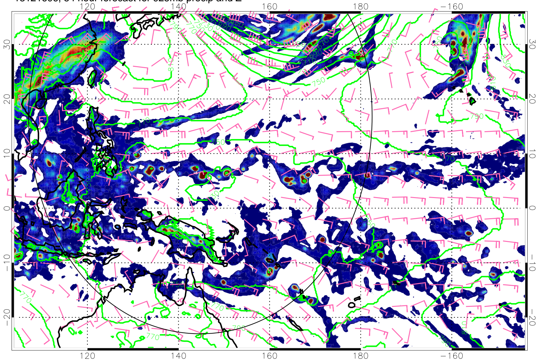
13121606, 54 hour forecast for 925mb precip and Z
