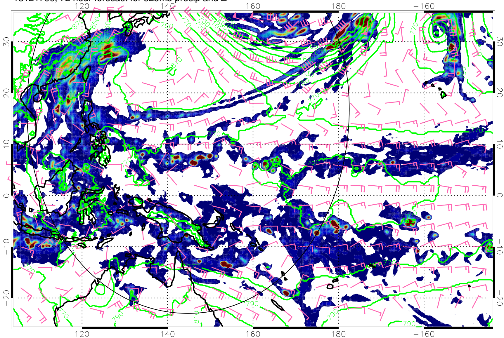
13121700, 72 hour forecast for 925mb precip and Z
