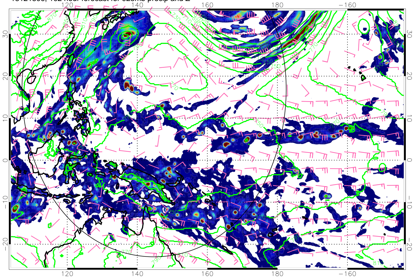
13121806, 102 hour forecast for 925mb precip and Z
