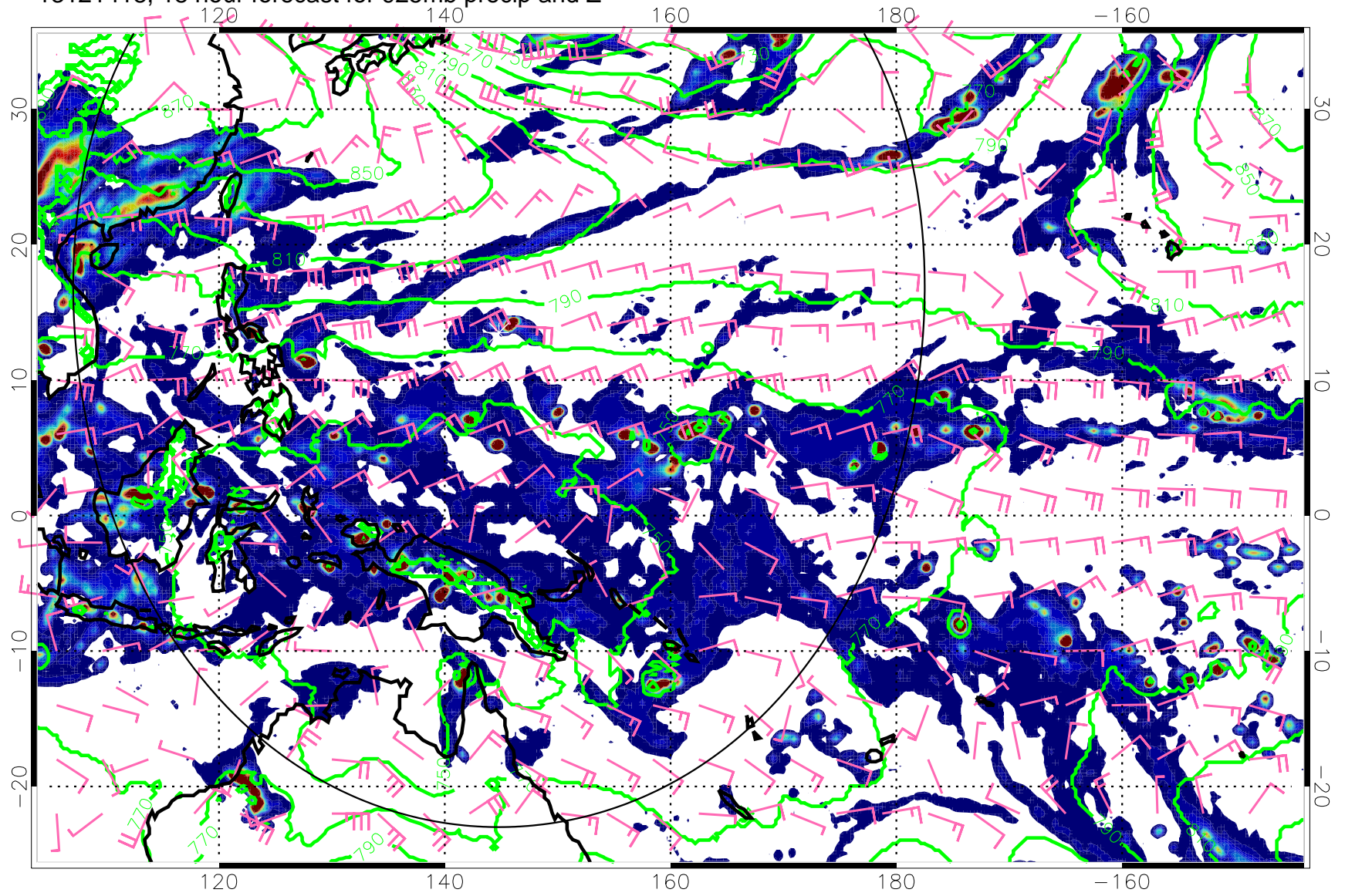
13121418, 18 hour forecast for 925mb precip and Z
