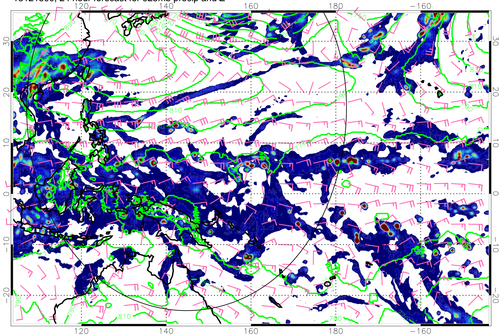
13121500, 24 hour forecast for 925mb precip and Z
