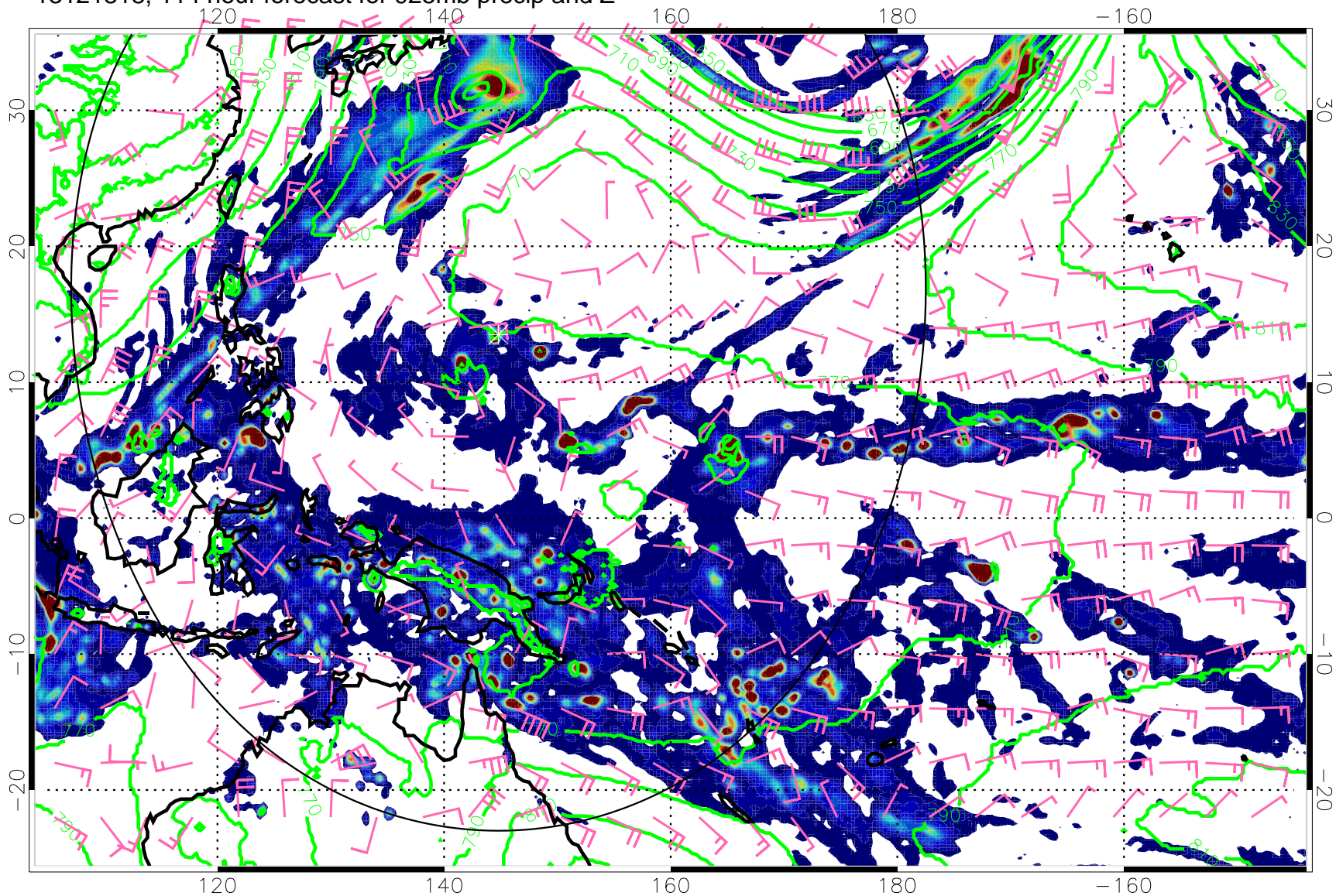
13121818, 114 hour forecast for 925mb precip and Z
