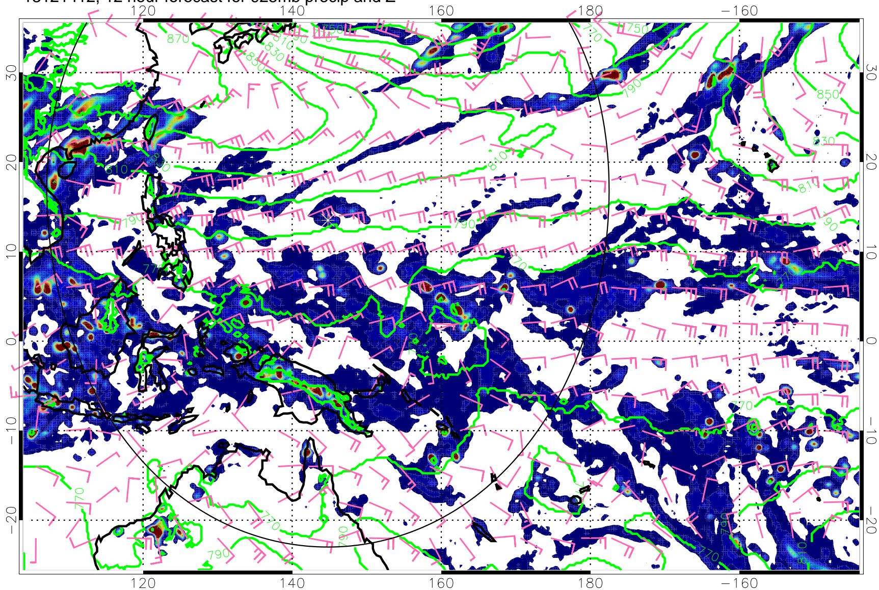
13121412, 12 hour forecast for 925mb precip and Z
