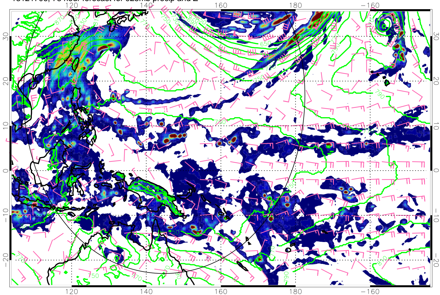
13121706, 78 hour forecast for 925mb precip and Z
