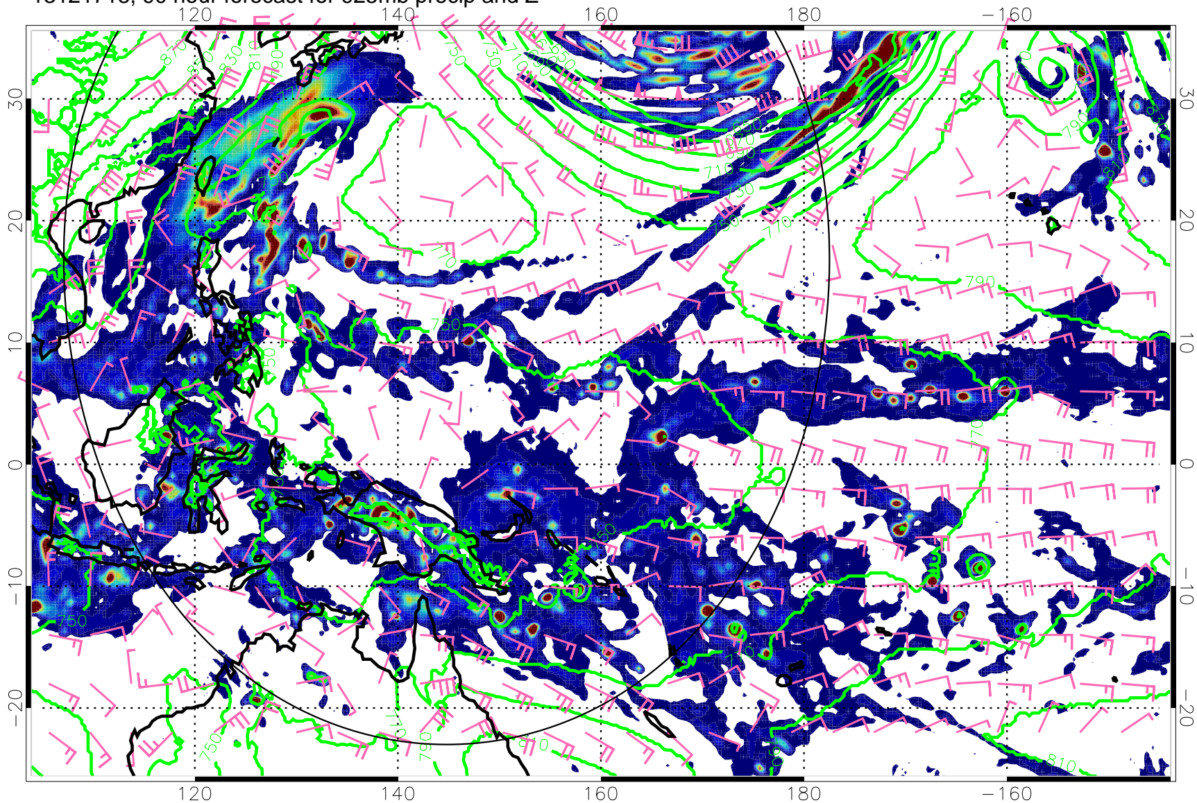
13121718, 90 hour forecast for 925mb precip and Z
