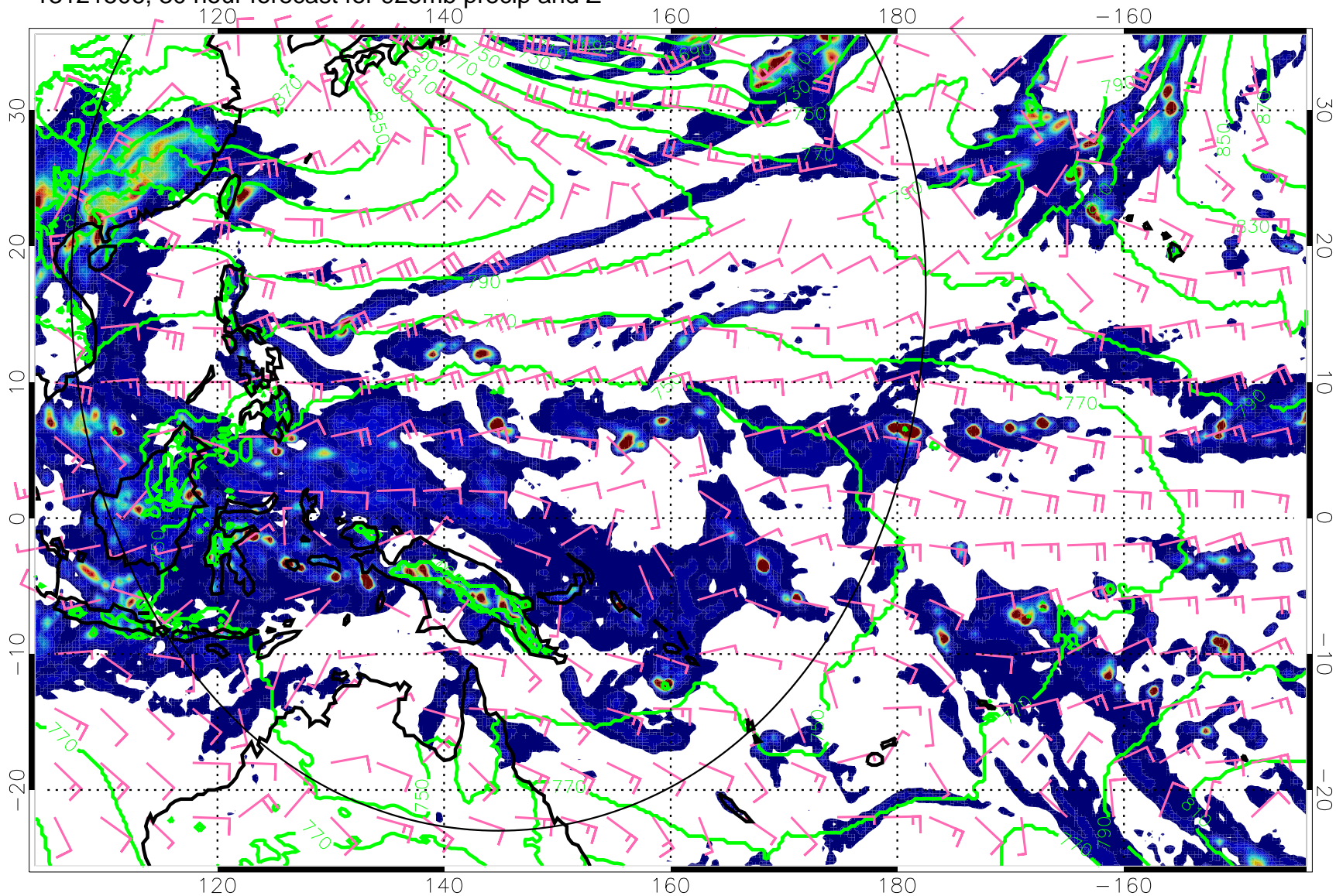
13121506, 30 hour forecast for 925mb precip and Z
