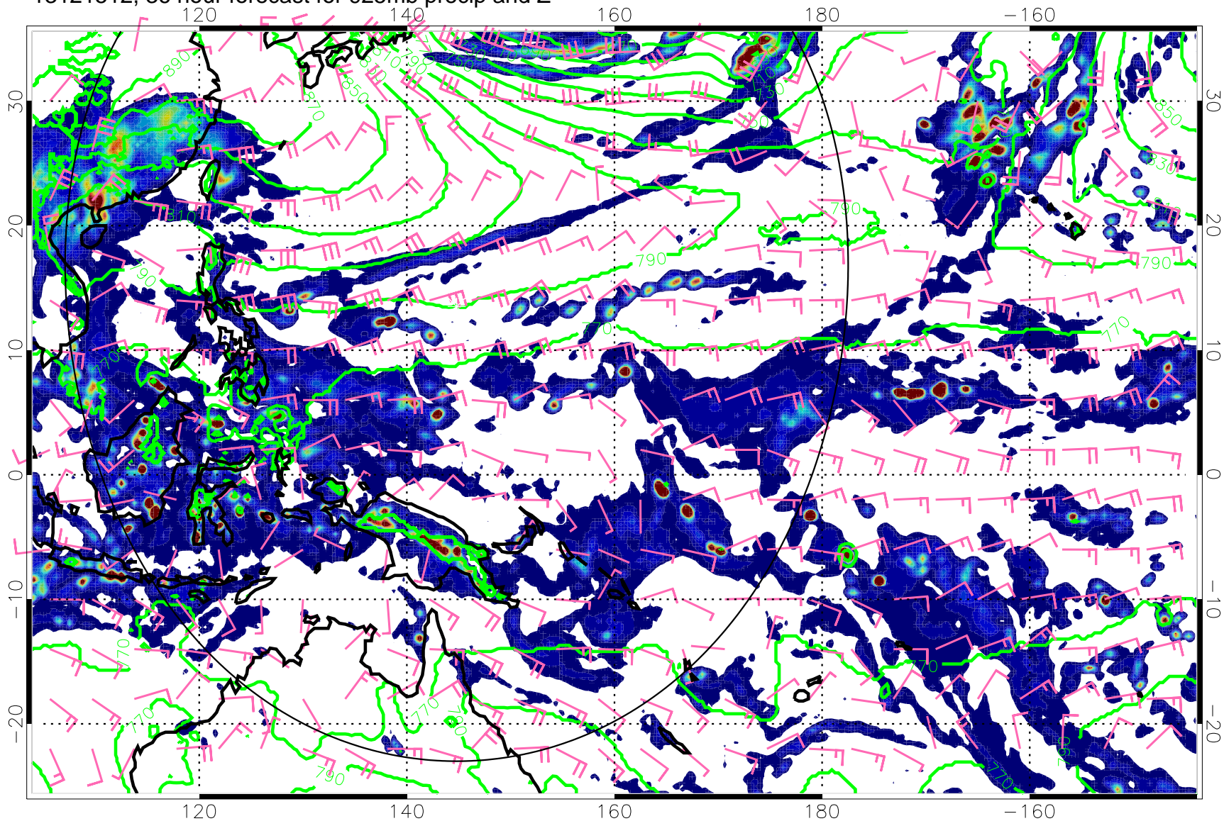
13121512, 36 hour forecast for 925mb precip and Z
