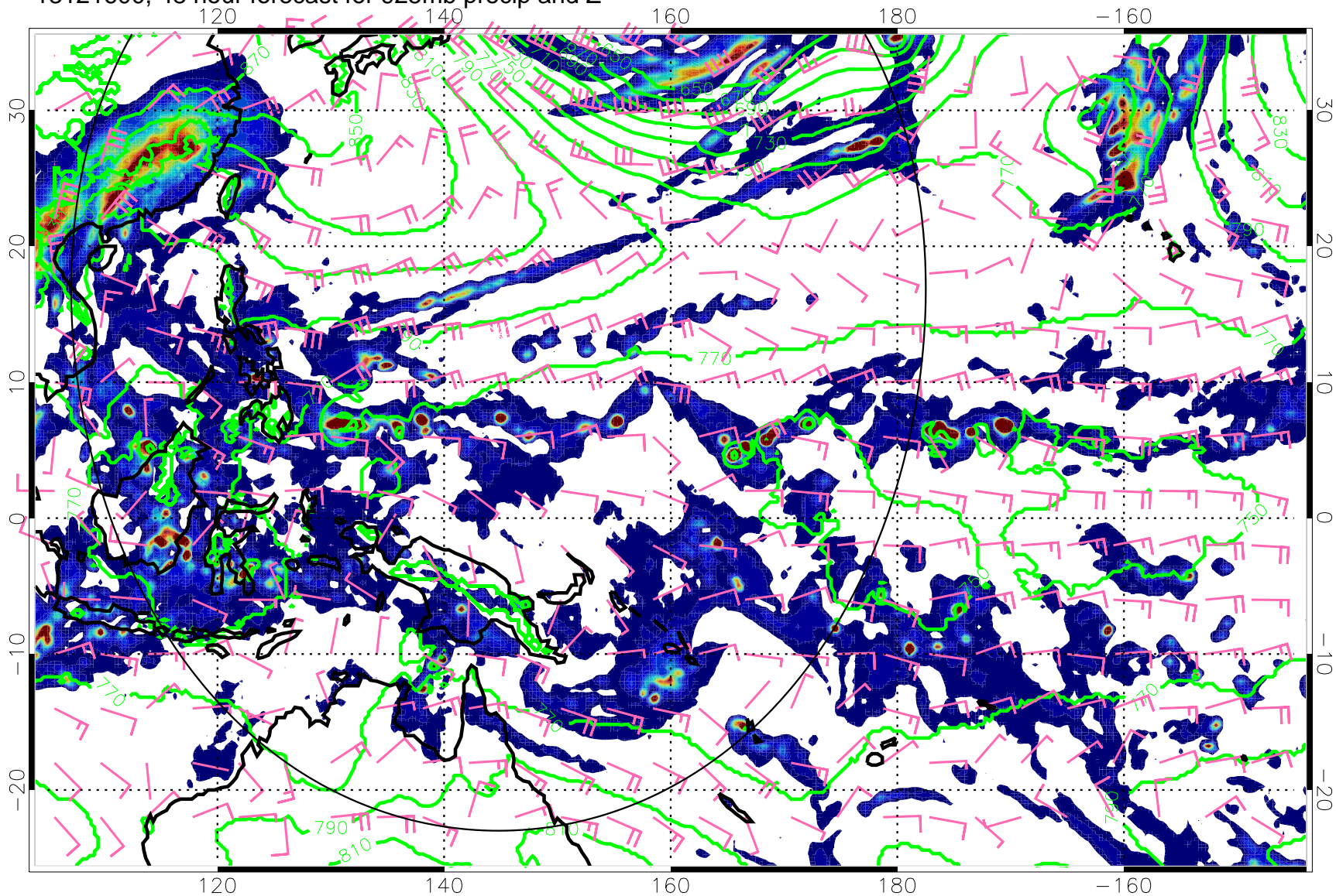
13121600, 48 hour forecast for 925mb precip and Z
