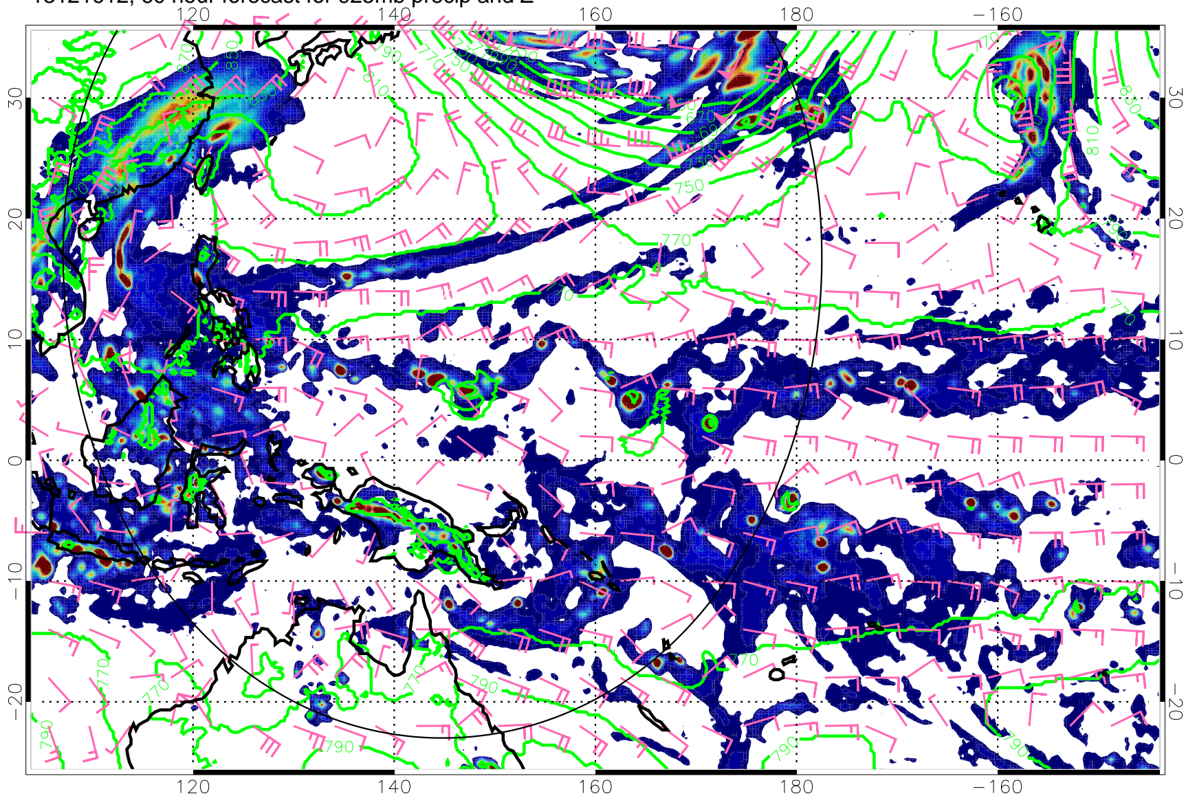
13121612, 60 hour forecast for 925mb precip and Z
