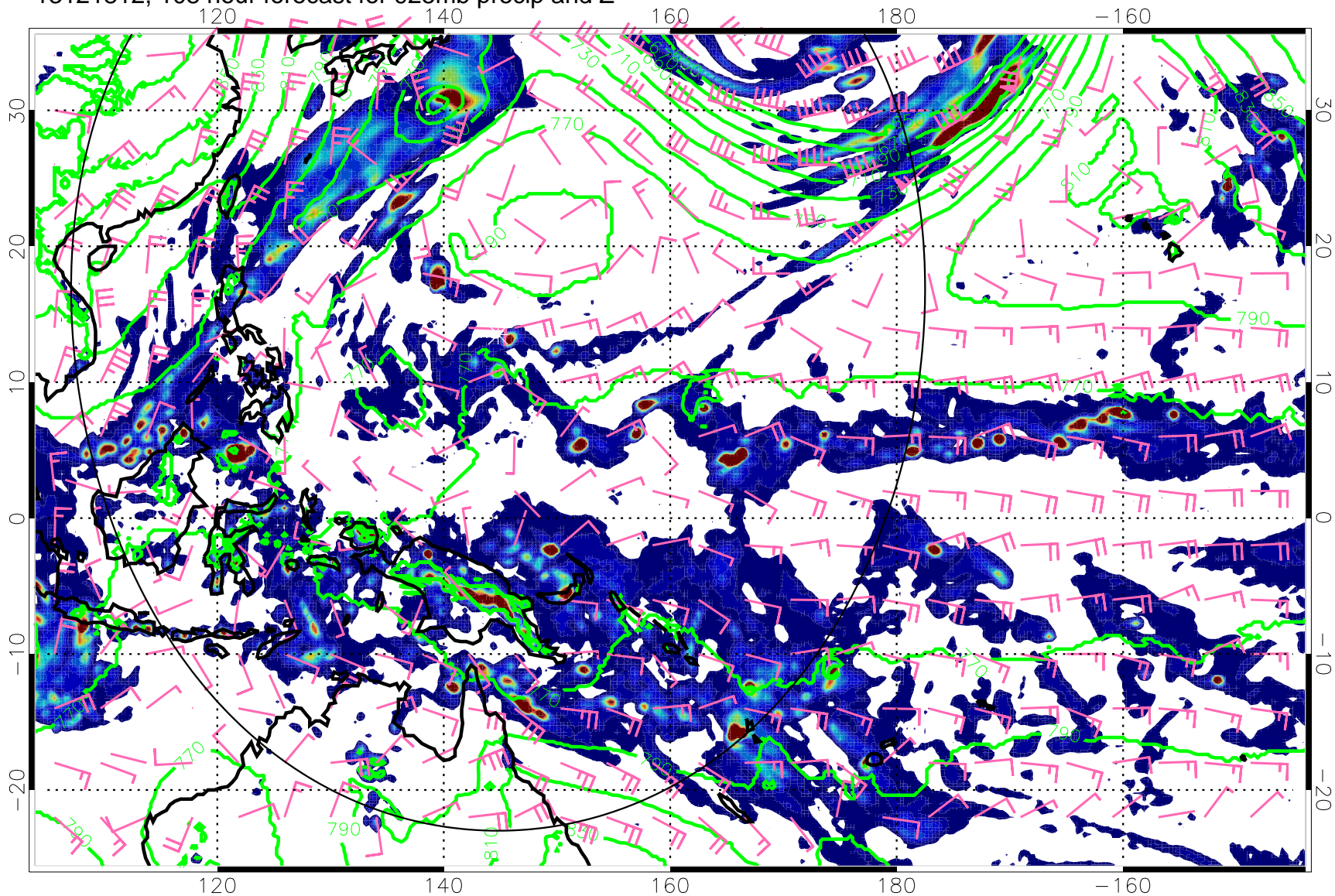
13121812, 108 hour forecast for 925mb precip and Z
