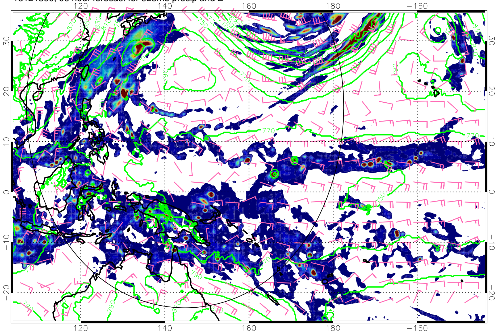
13121800, 96 hour forecast for 925mb precip and Z
