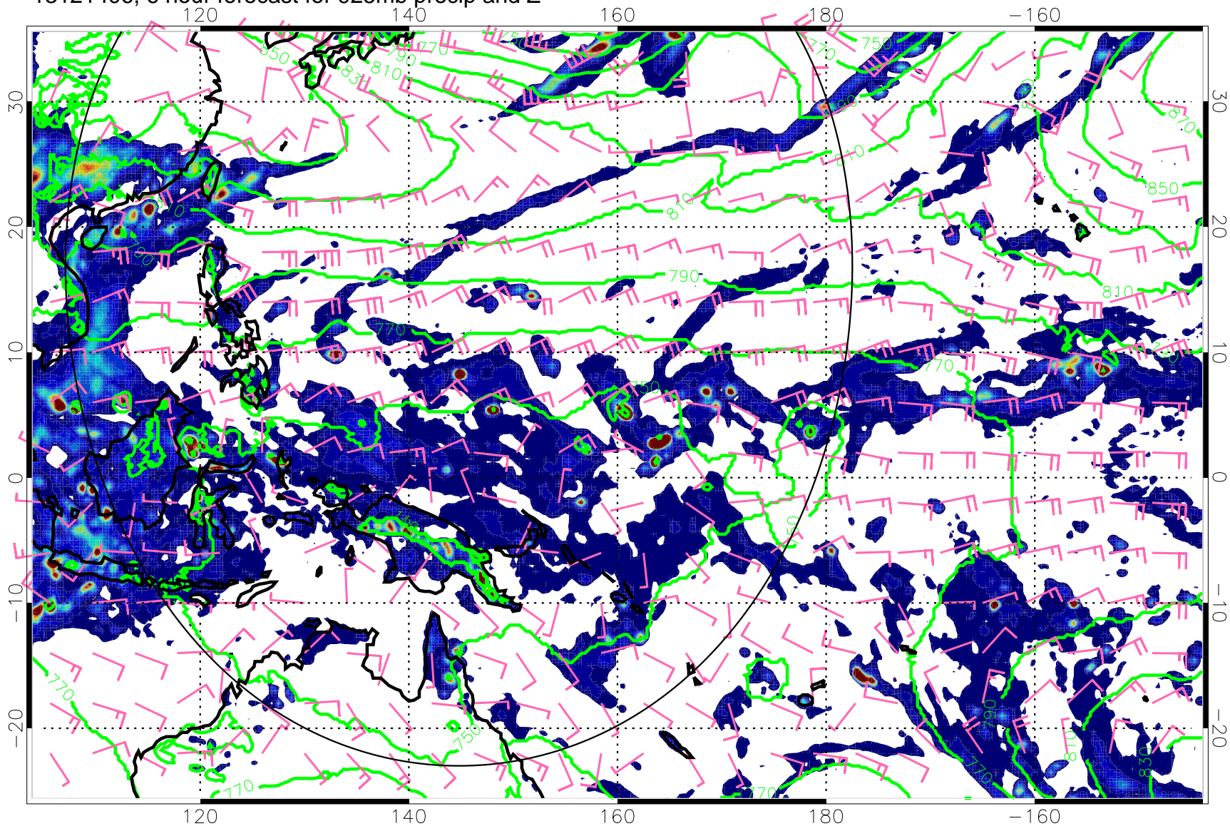
13121406, 6 hour forecast for 925mb precip and Z
