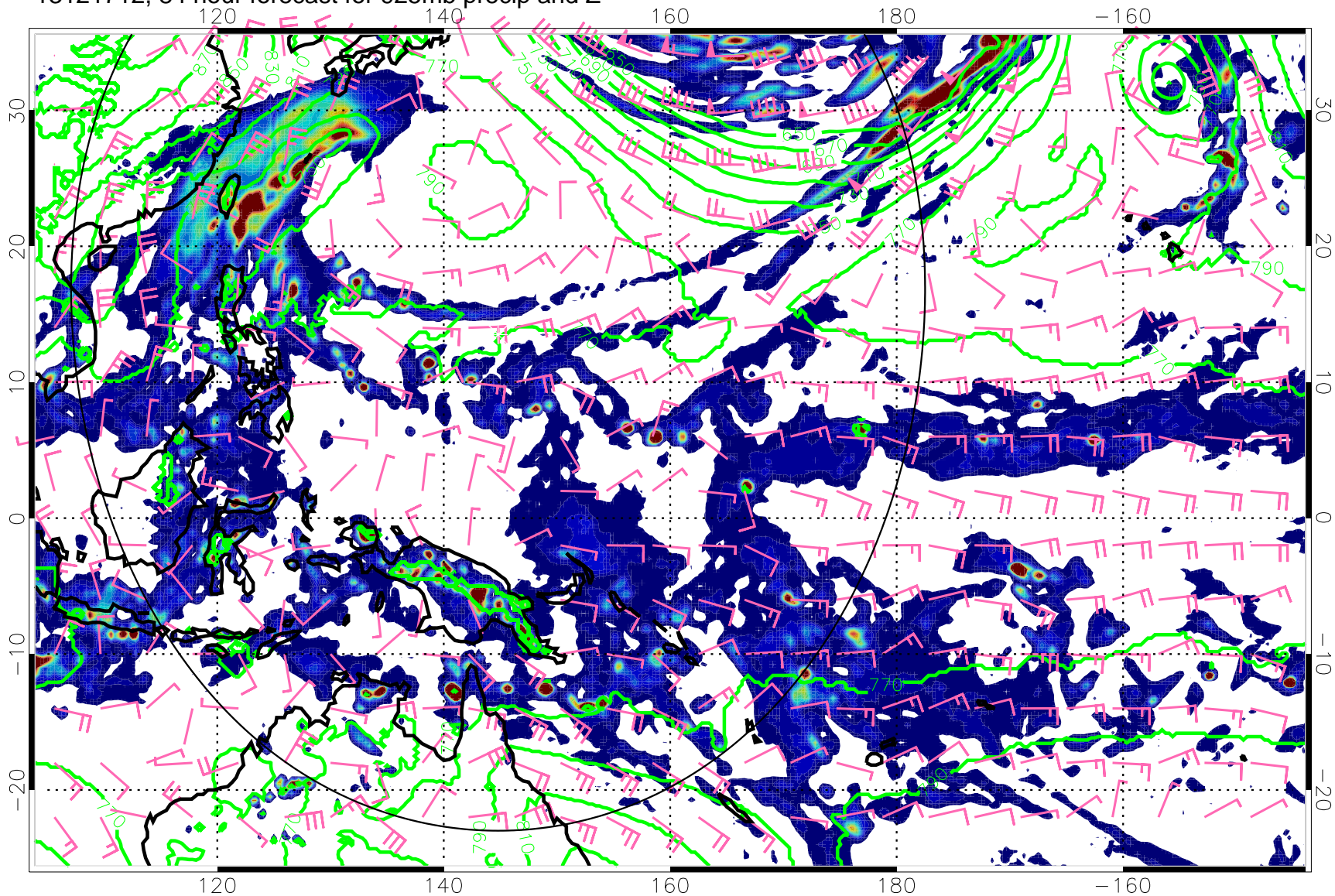
13121712, 84 hour forecast for 925mb precip and Z
