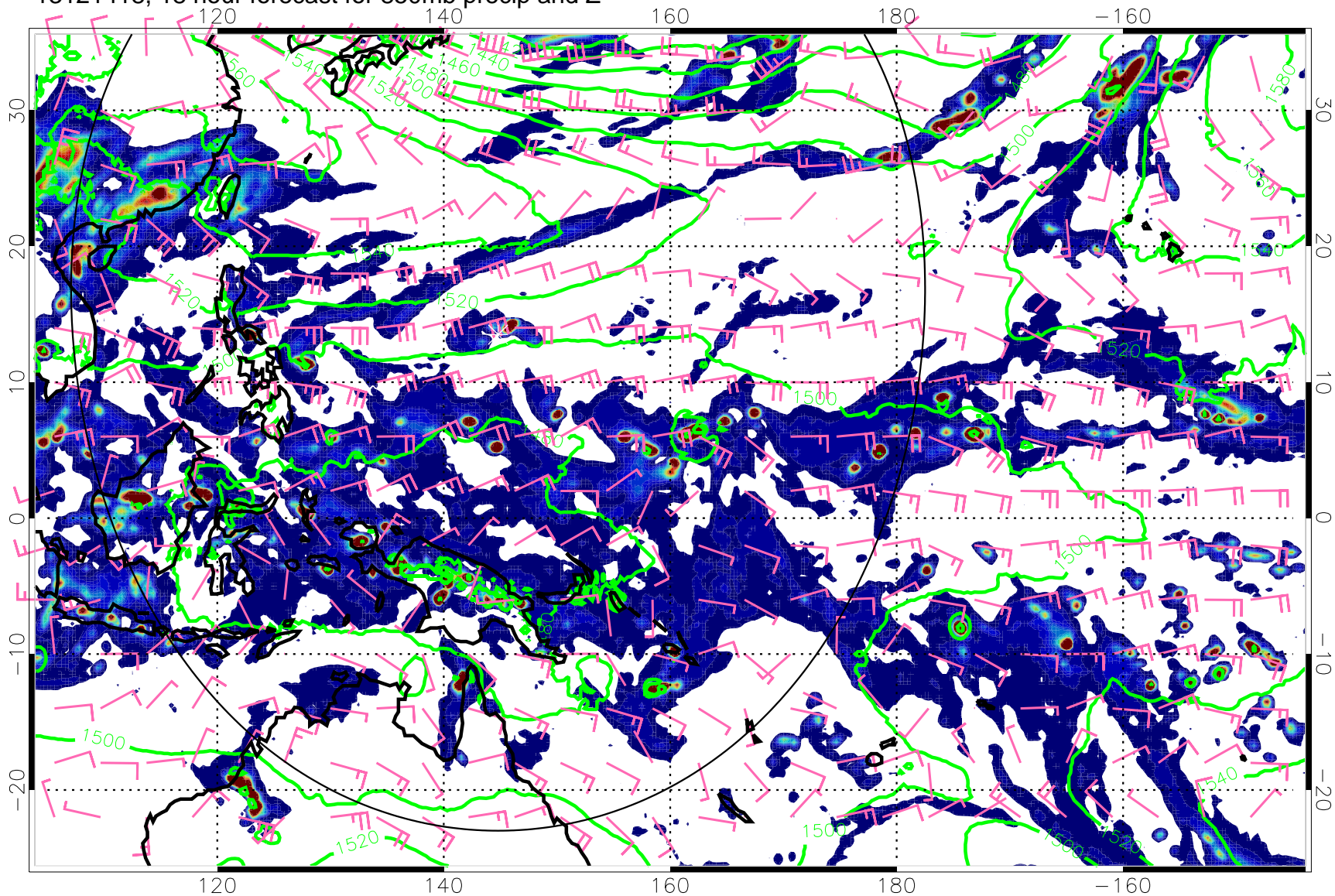
13121418, 18 hour forecast for 850mb precip and Z
