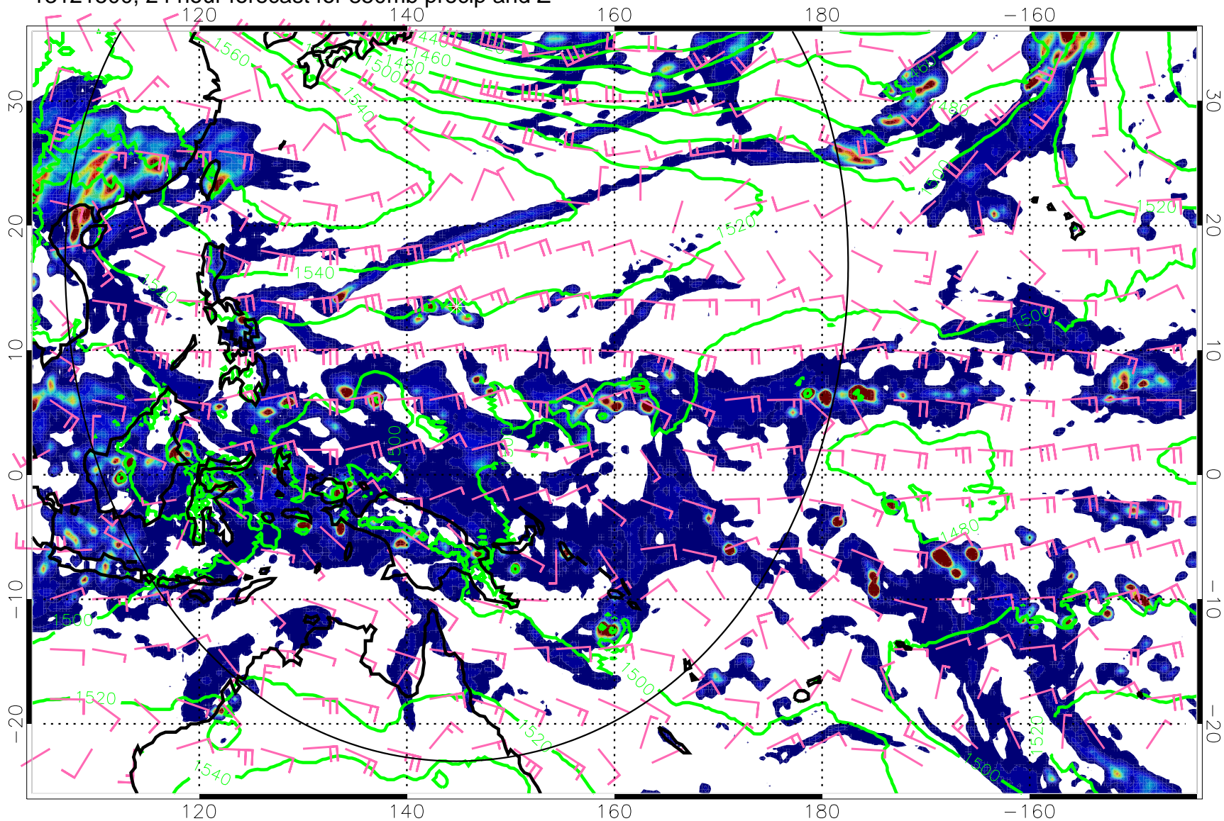
13121500, 24 hour forecast for 850mb precip and Z
