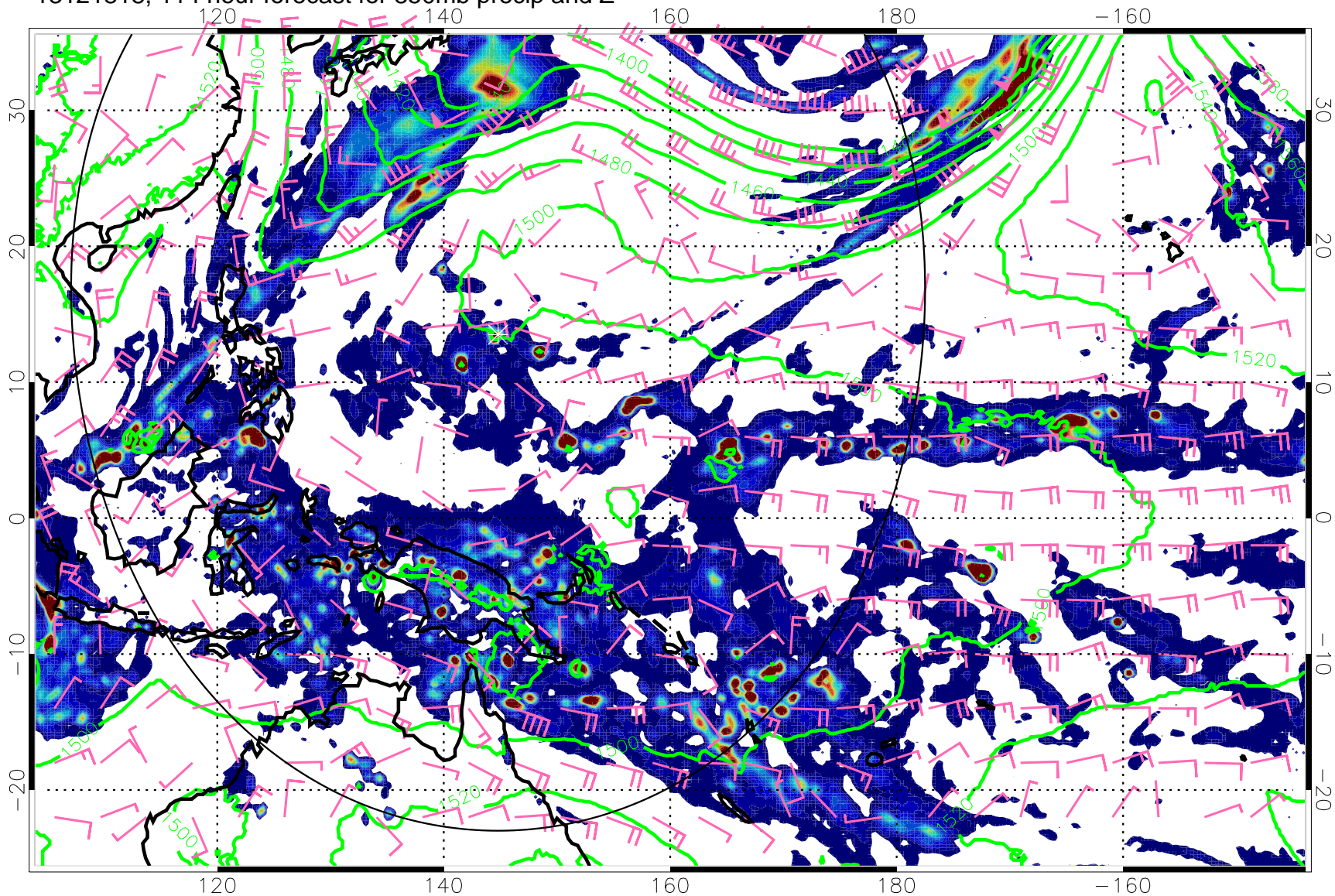
13121818, 114 hour forecast for 850mb precip and Z
