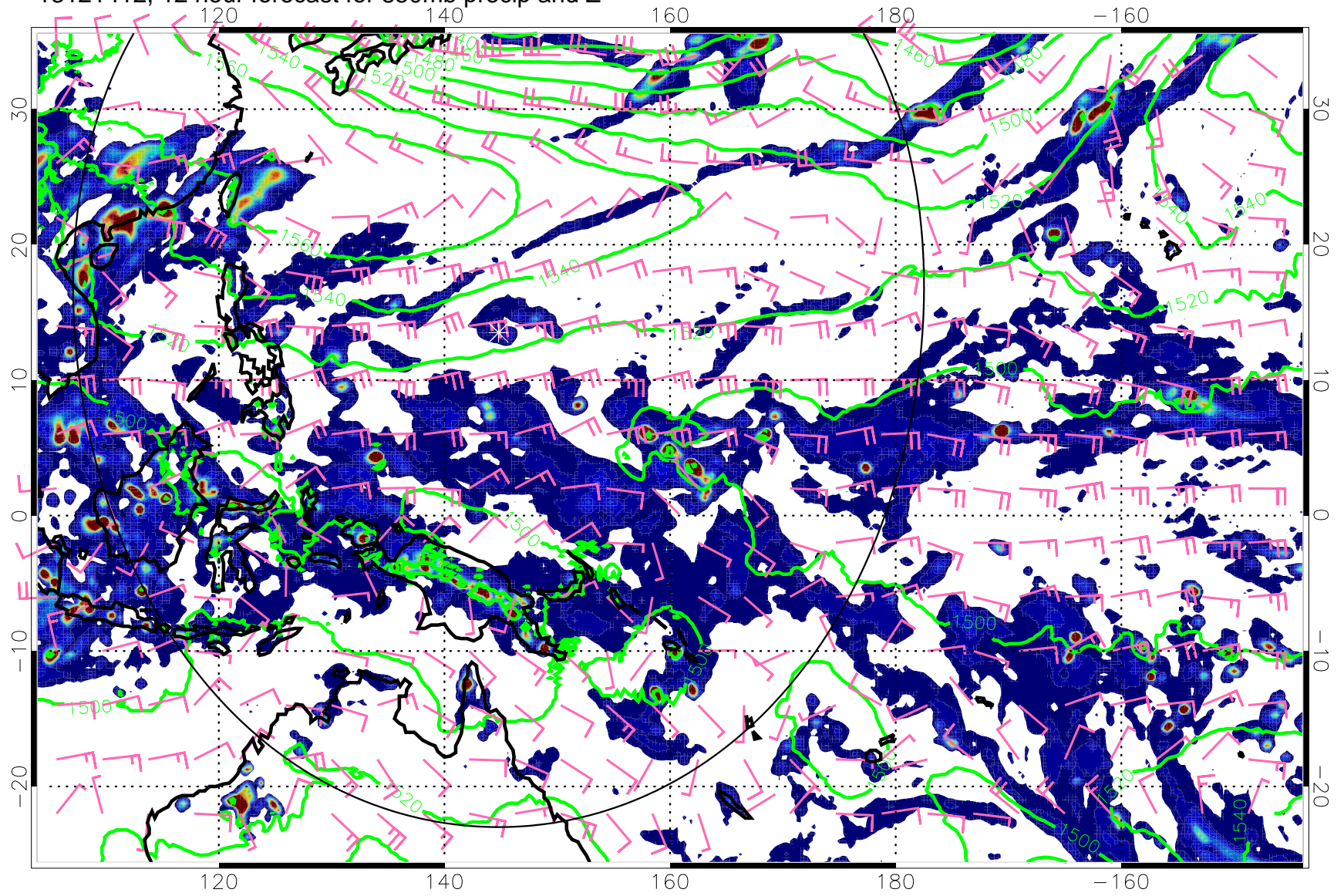
13121412, 12 hour forecast for 850mb precip and Z
