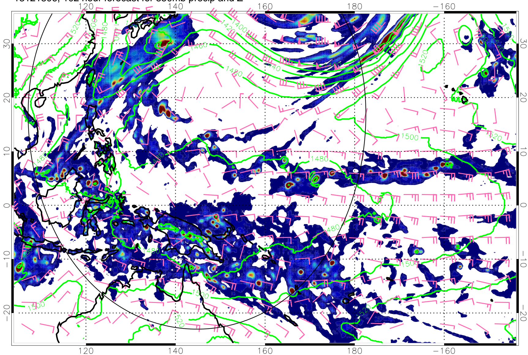
13121806, 102 hour forecast for 850mb precip and Z
