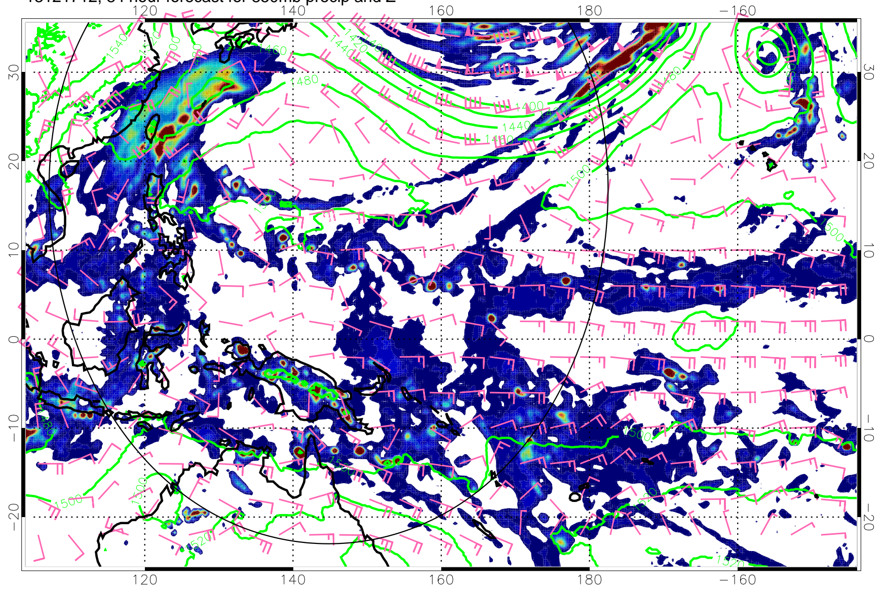
13121712, 84 hour forecast for 850mb precip and Z
