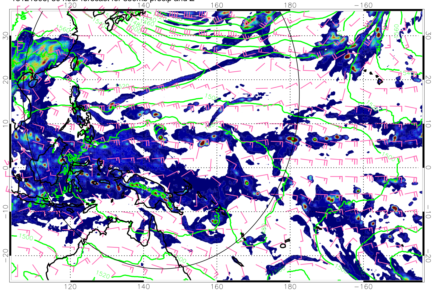
13121506, 30 hour forecast for 850mb precip and Z
