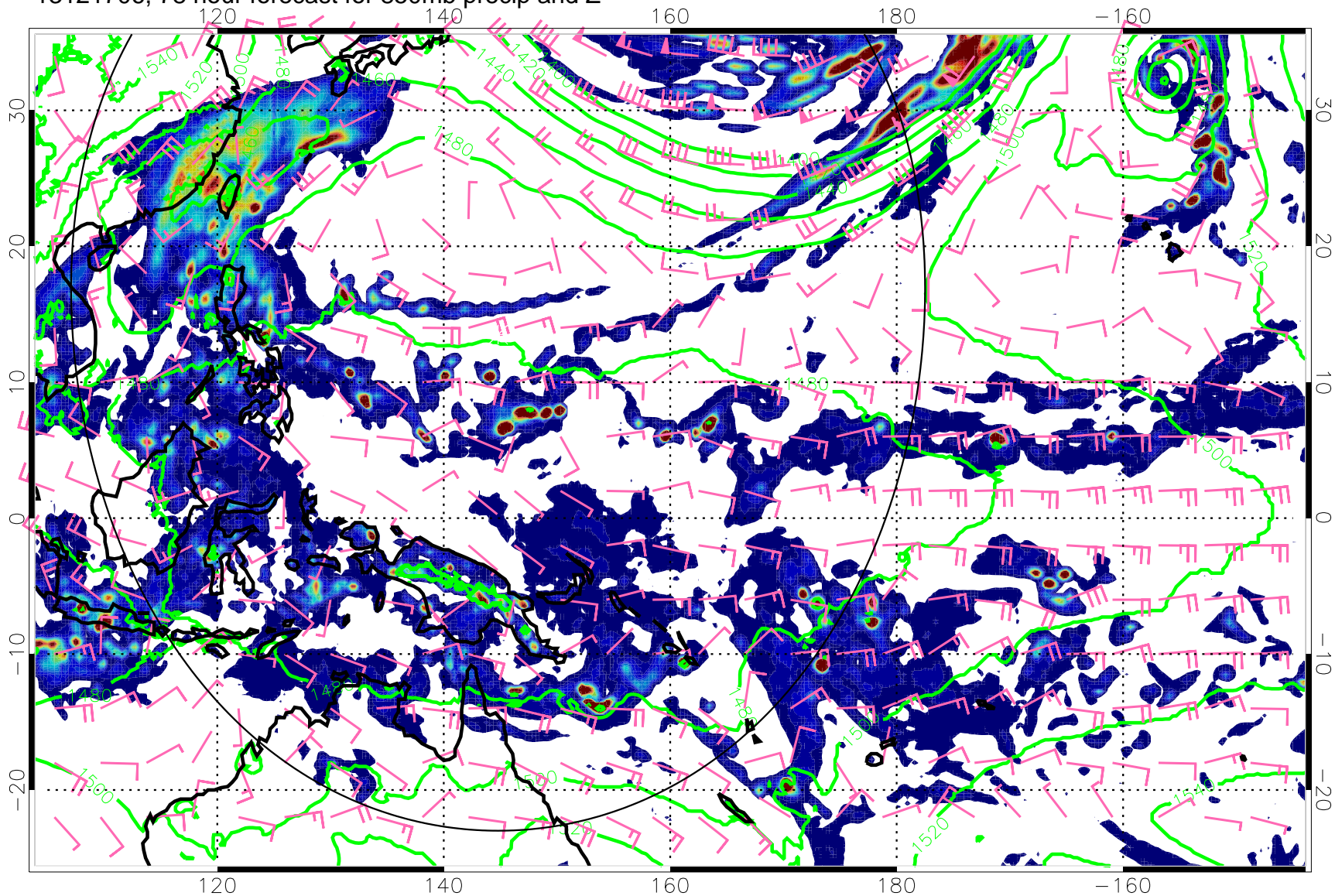
13121706, 78 hour forecast for 850mb precip and Z
