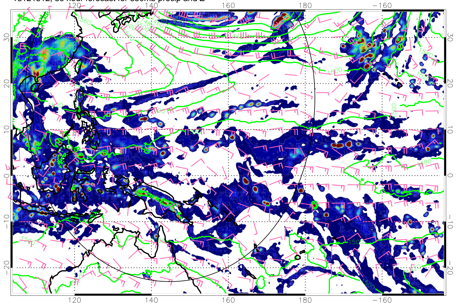
13121512, 36 hour forecast for 850mb precip and Z
