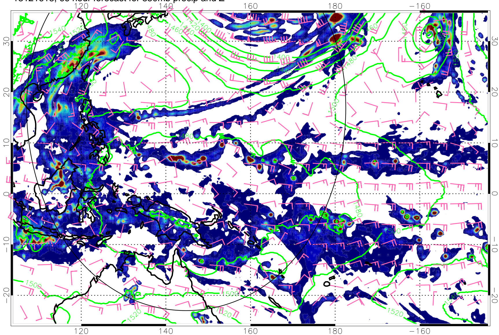
13121618, 66 hour forecast for 850mb precip and Z
