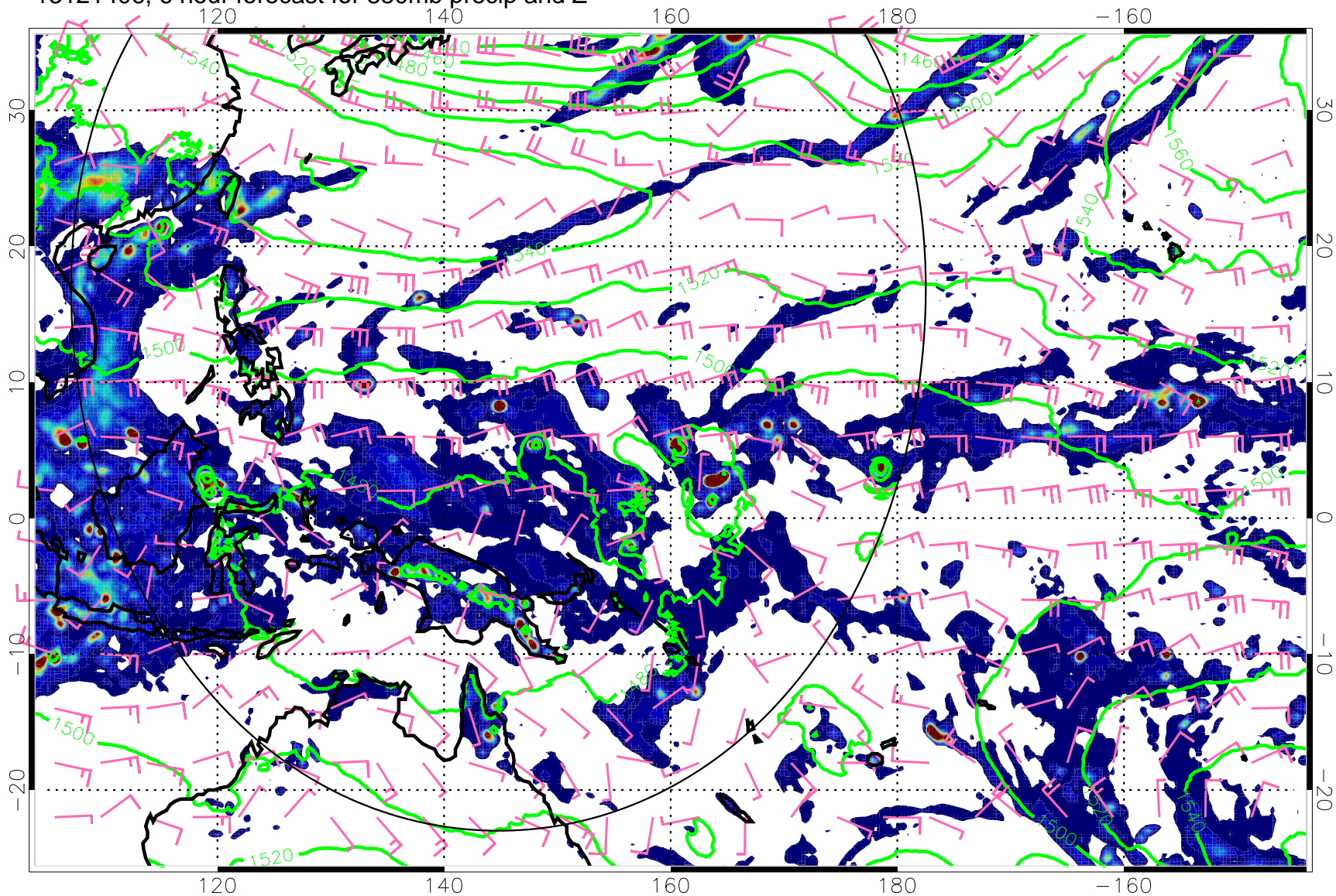
13121406, 6 hour forecast for 850mb precip and Z
