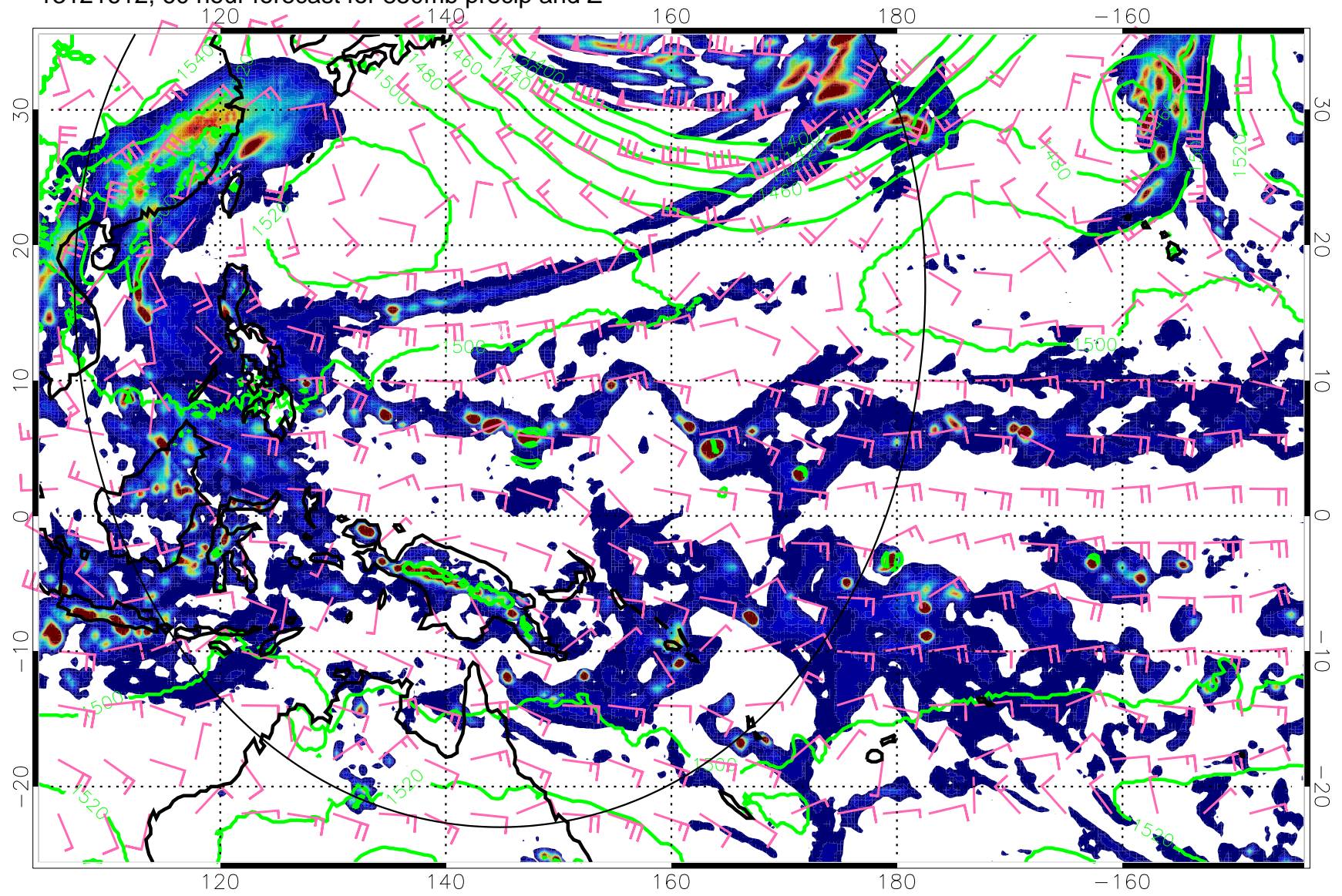
13121612, 60 hour forecast for 850mb precip and Z
