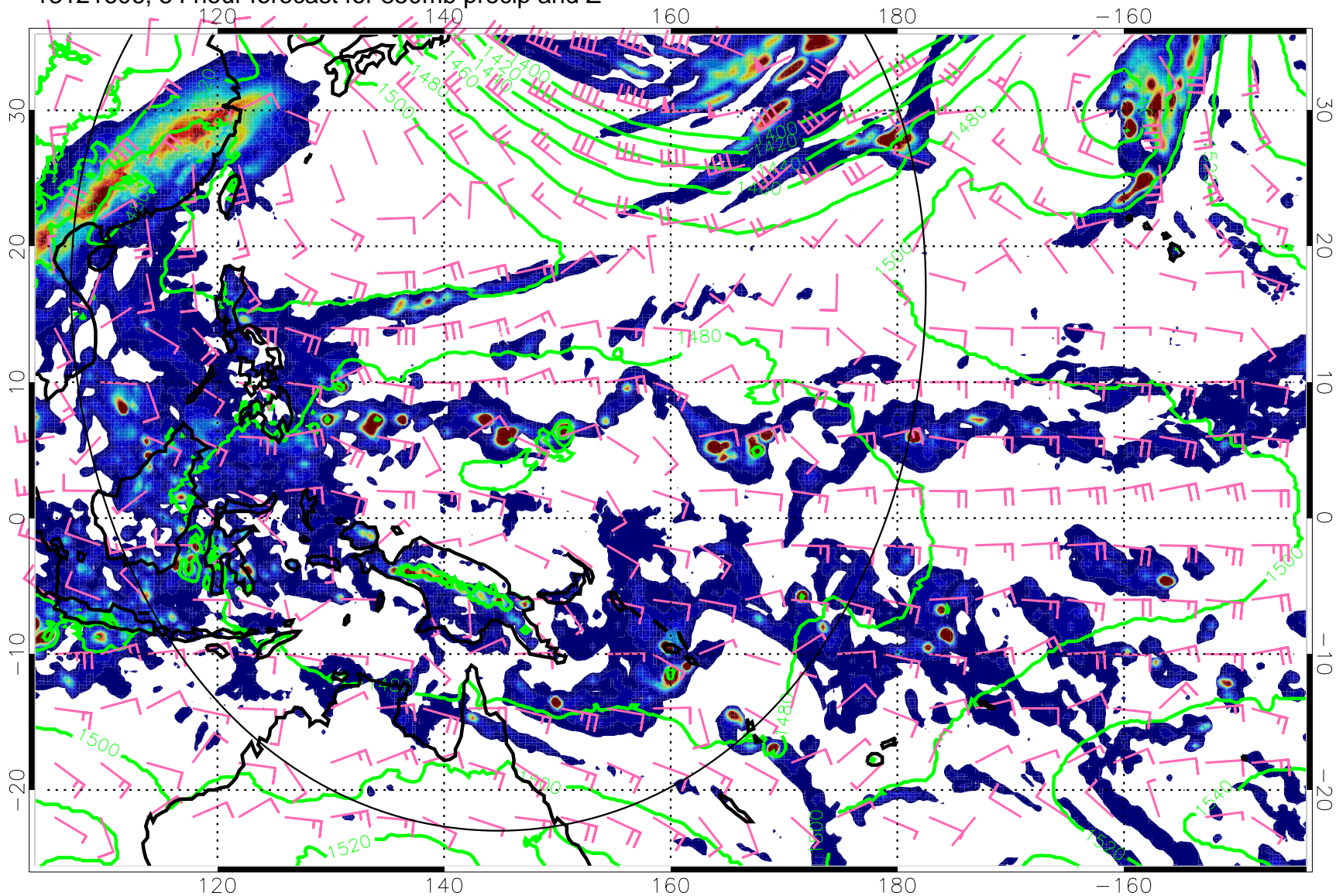
13121606, 54 hour forecast for 850mb precip and Z
