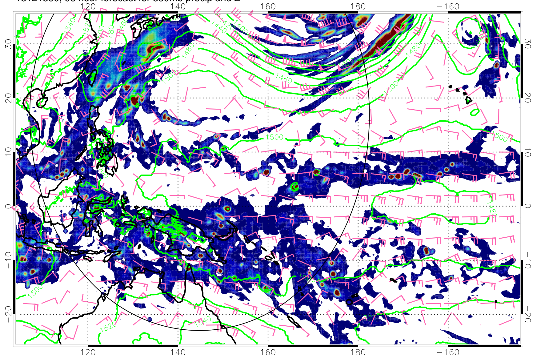
13121800, 96 hour forecast for 850mb precip and Z
