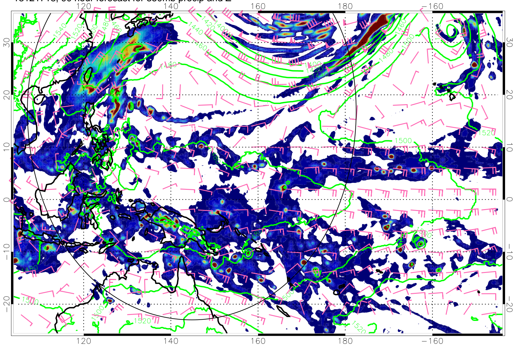
13121718, 90 hour forecast for 850mb precip and Z
