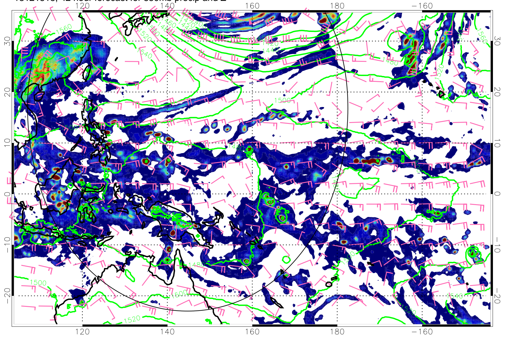
13121518, 42 hour forecast for 850mb precip and Z
