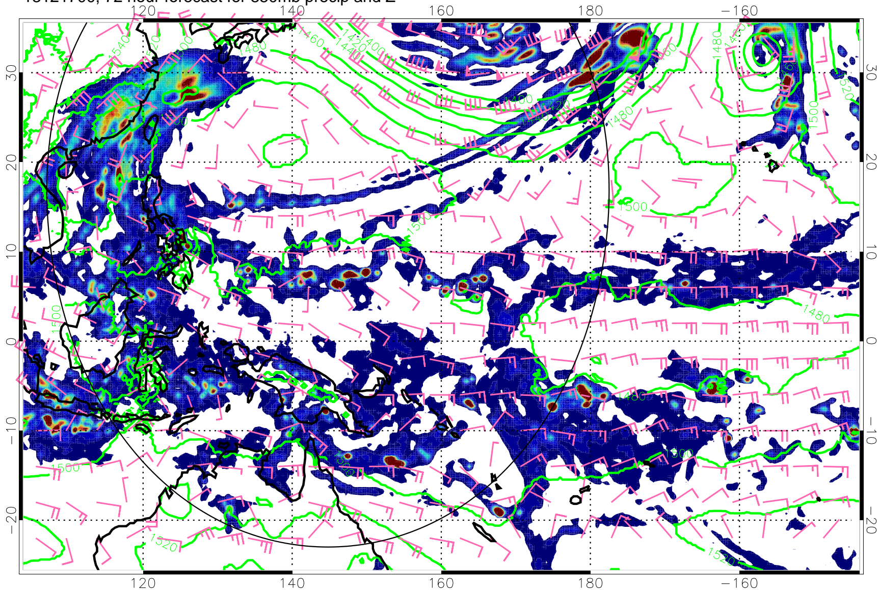
13121700, 72 hour forecast for 850mb precip and Z
