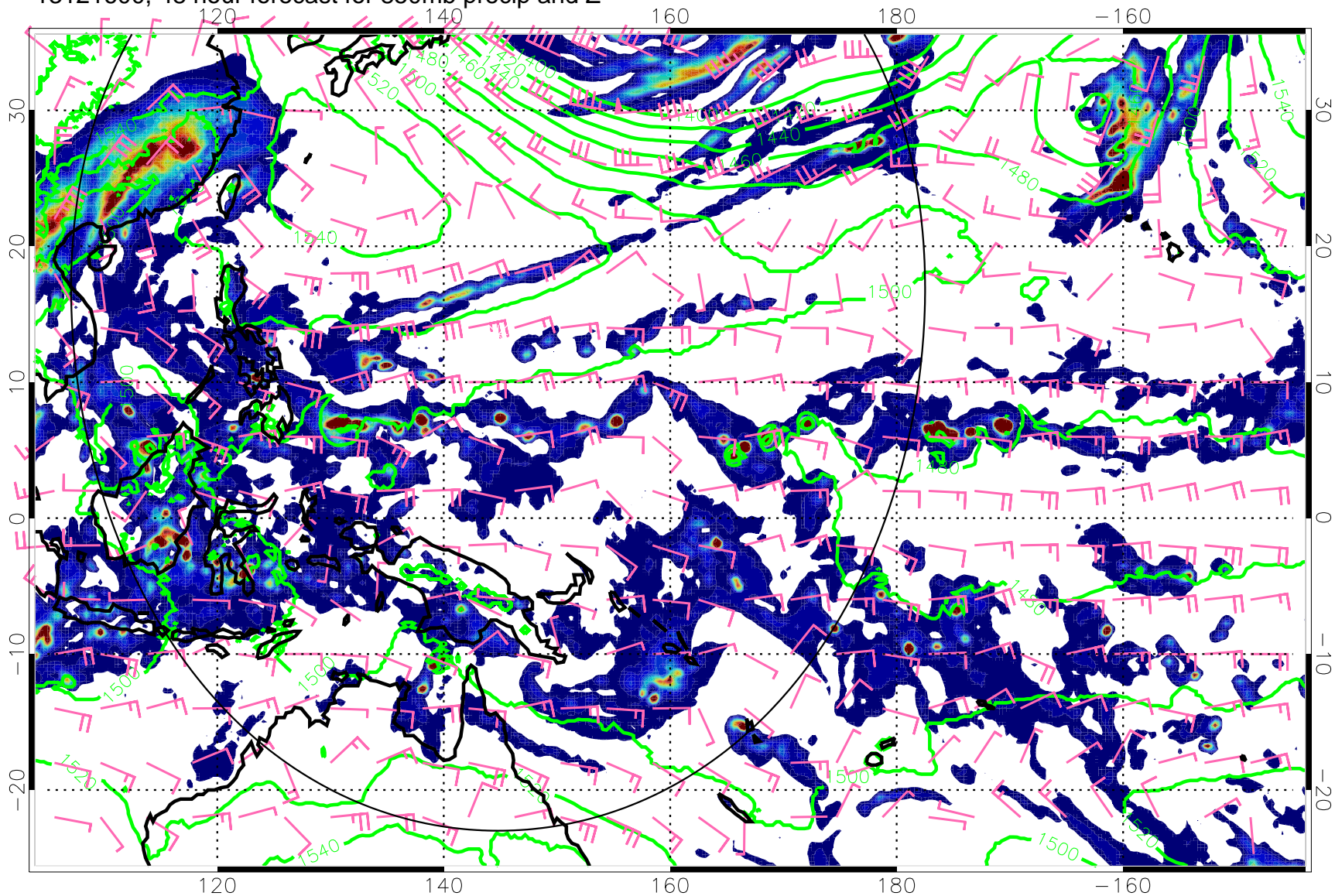
13121600, 48 hour forecast for 850mb precip and Z
