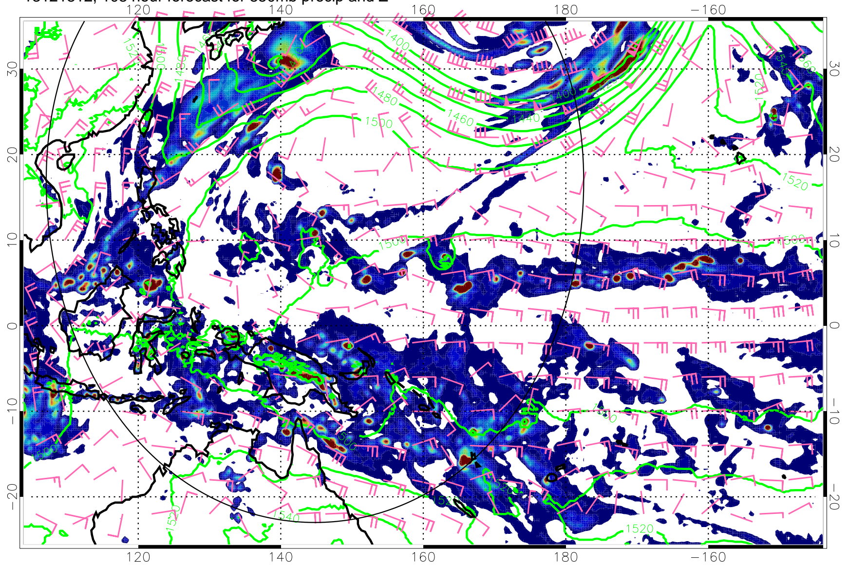
13121812, 108 hour forecast for 850mb precip and Z
