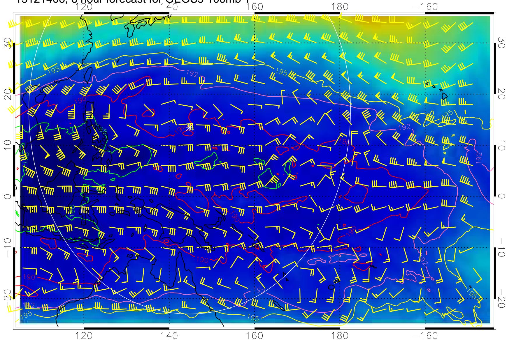
13121406, 6 hour forecast for GEOS5 100mb T
