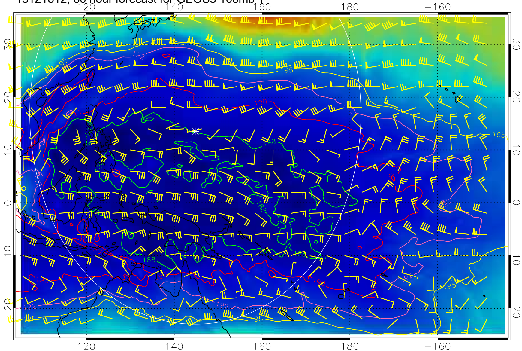
13121612, 60 hour forecast for GEOS5 100mb T
