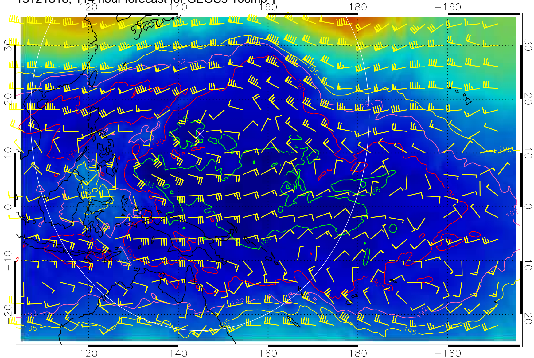
13121818, 114 hour forecast for GEOS5 100mb T
