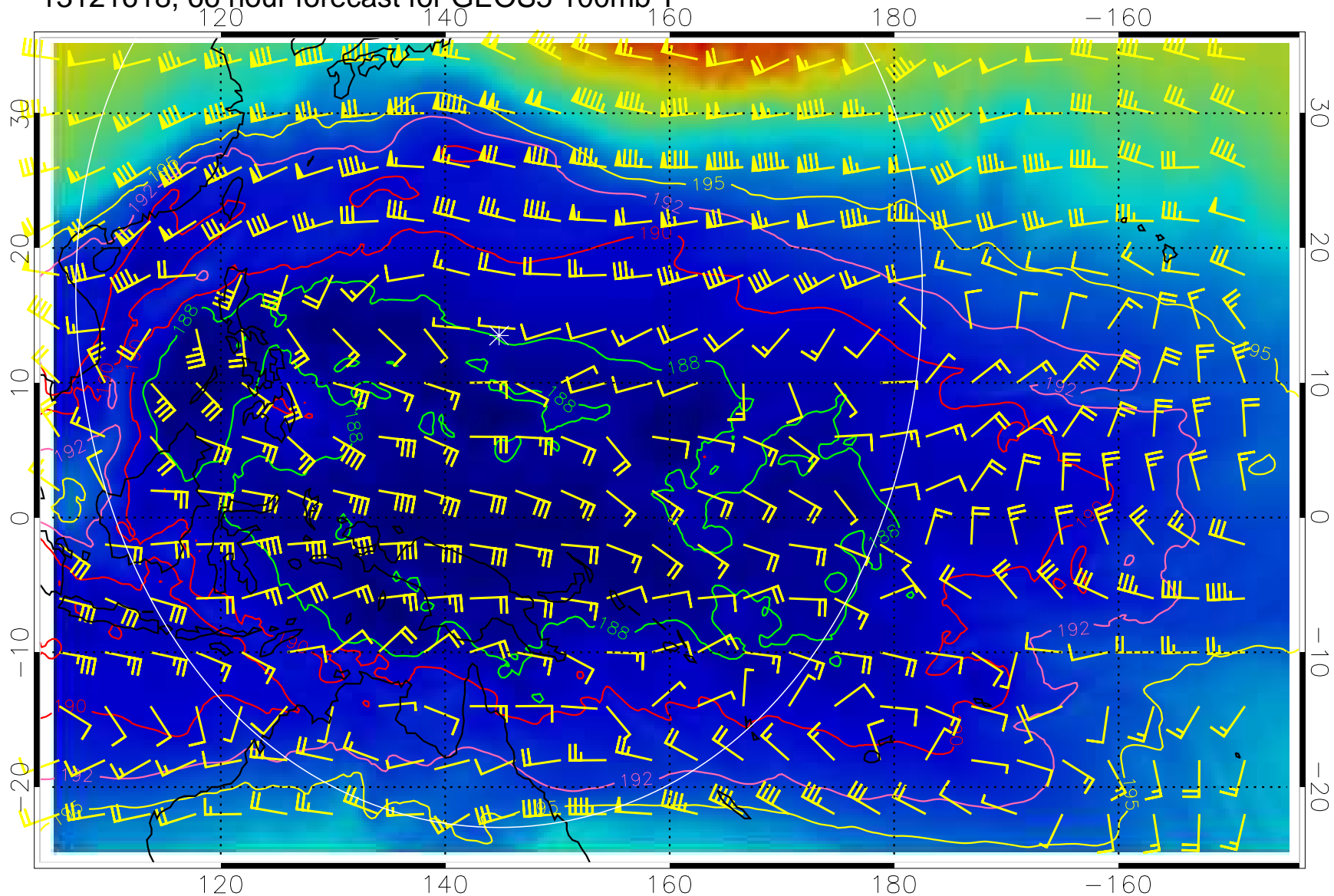
13121618, 66 hour forecast for GEOS5 100mb T
