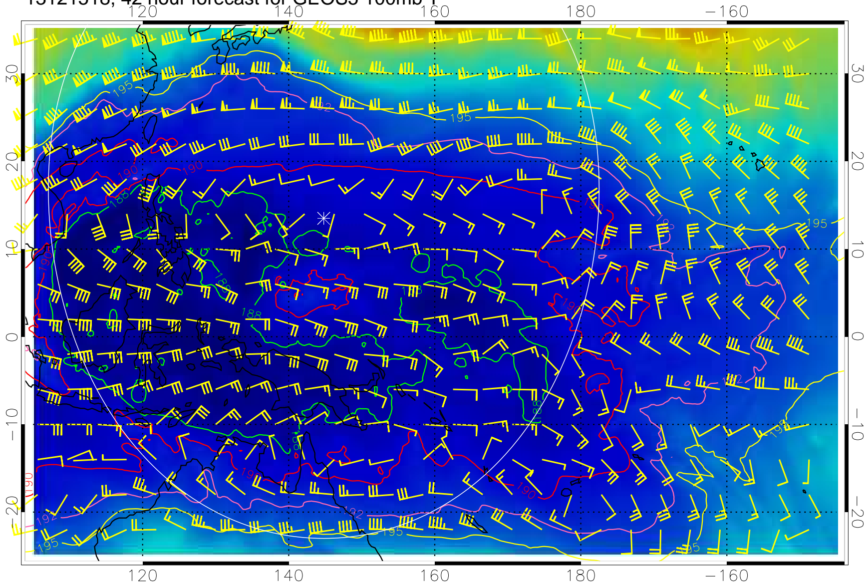
13121518, 42 hour forecast for GEOS5 100mb T
