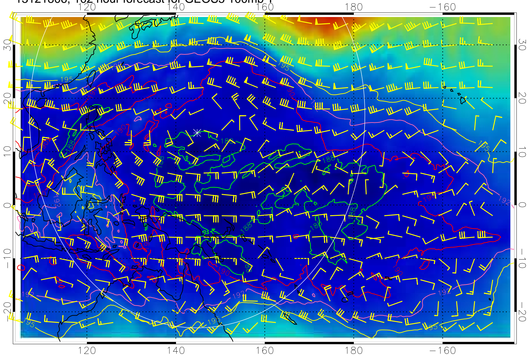
13121806, 102 hour forecast for GEOS5 100mb T
