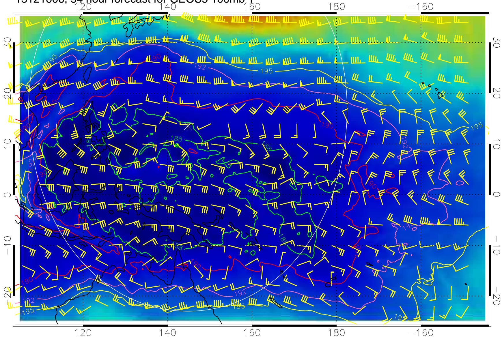
13121606, 54 hour forecast for GEOS5 100mb T
