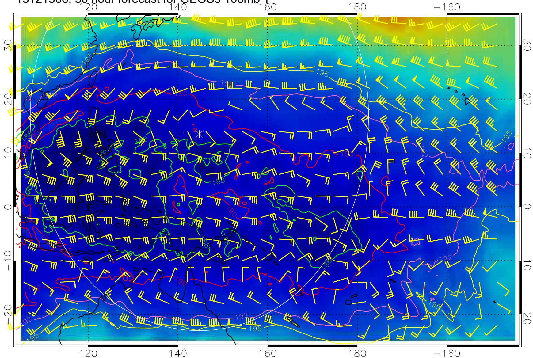
13121506, 30 hour forecast for GEOS5 100mb T
