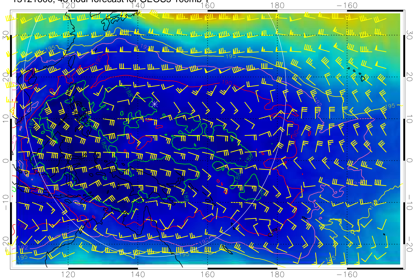
13121600, 48 hour forecast for GEOS5 100mb T
