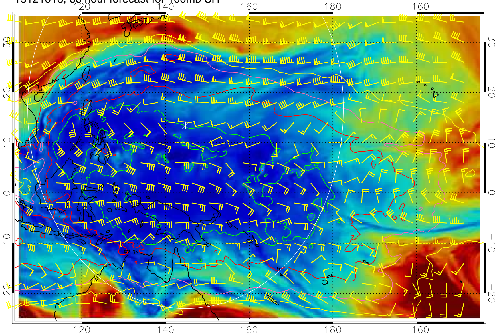
13121618, 66 hour forecast for 100mb SH
