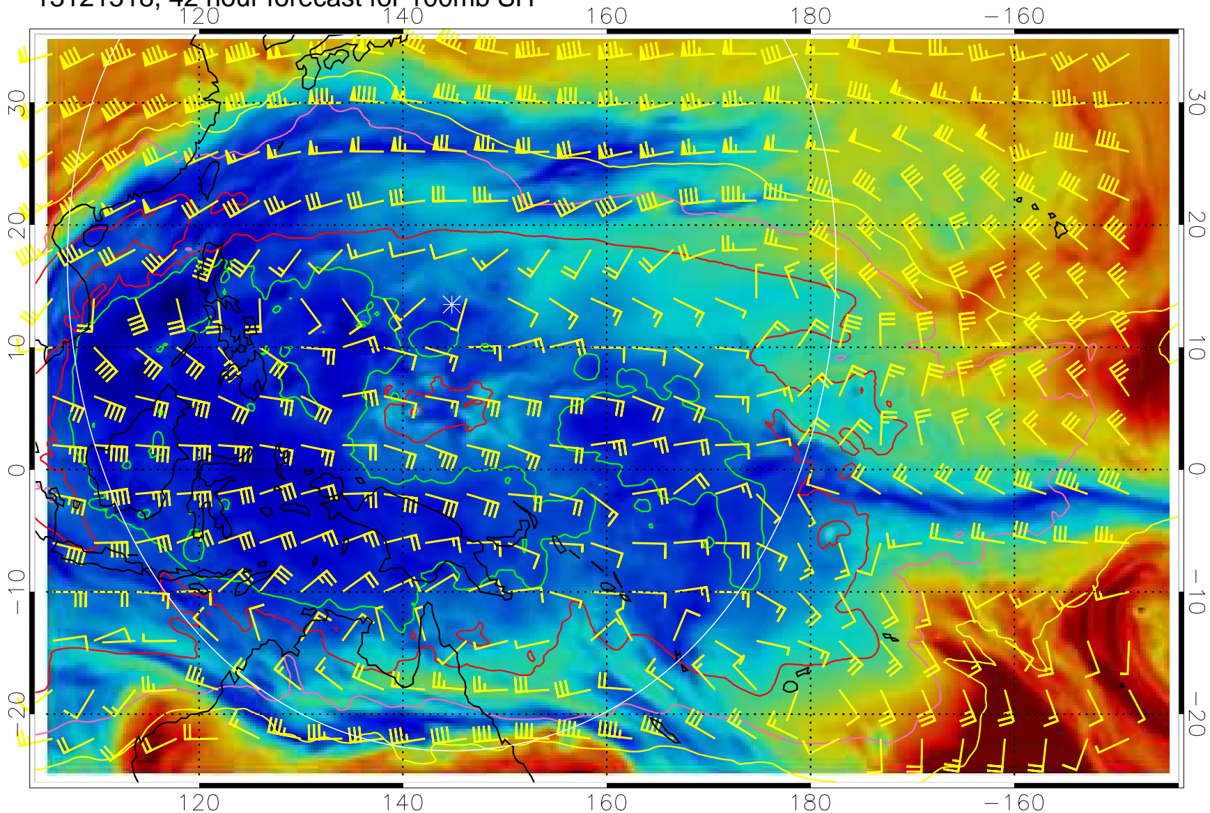
13121518, 42 hour forecast for 100mb SH
