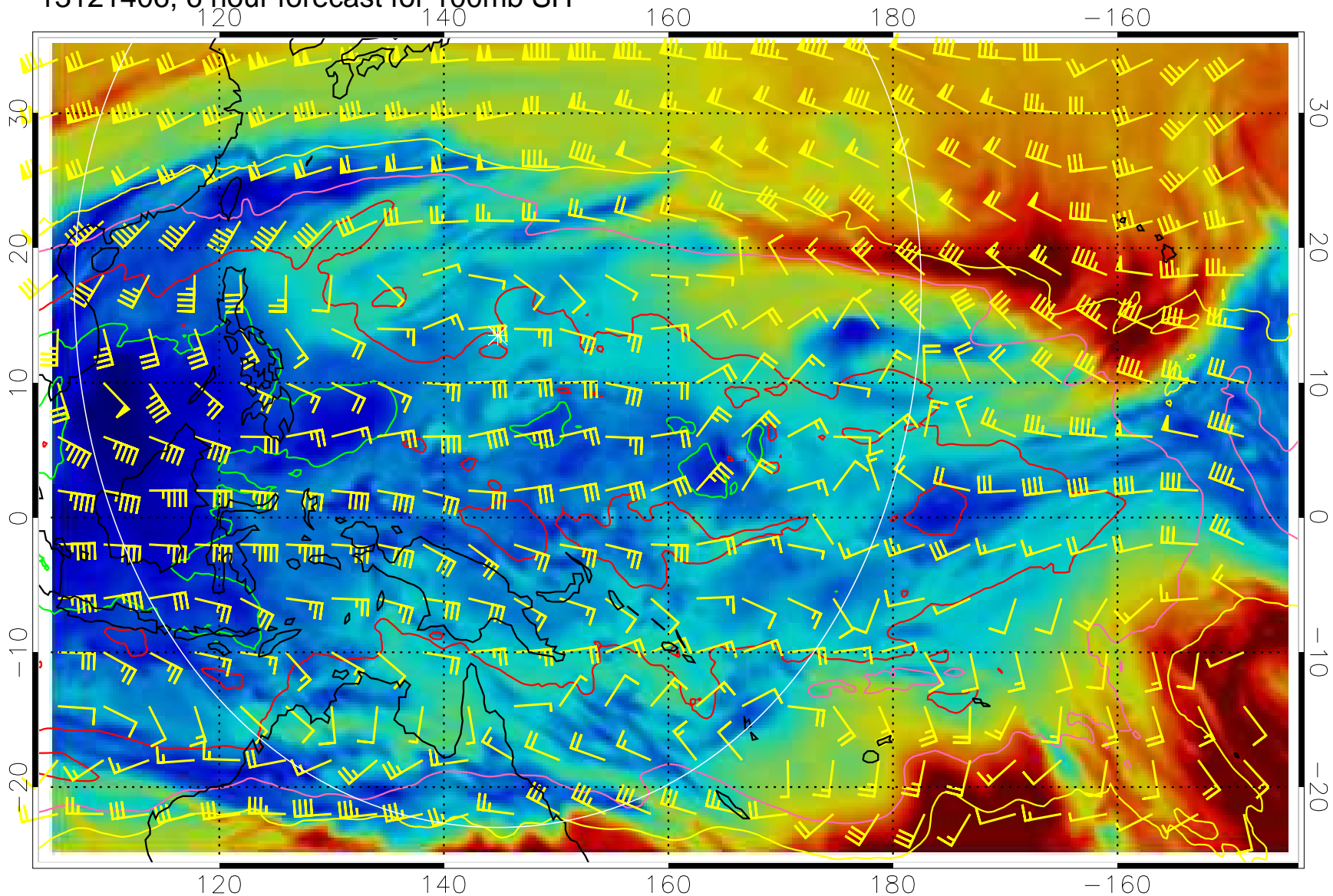
13121406, 6 hour forecast for 100mb SH
