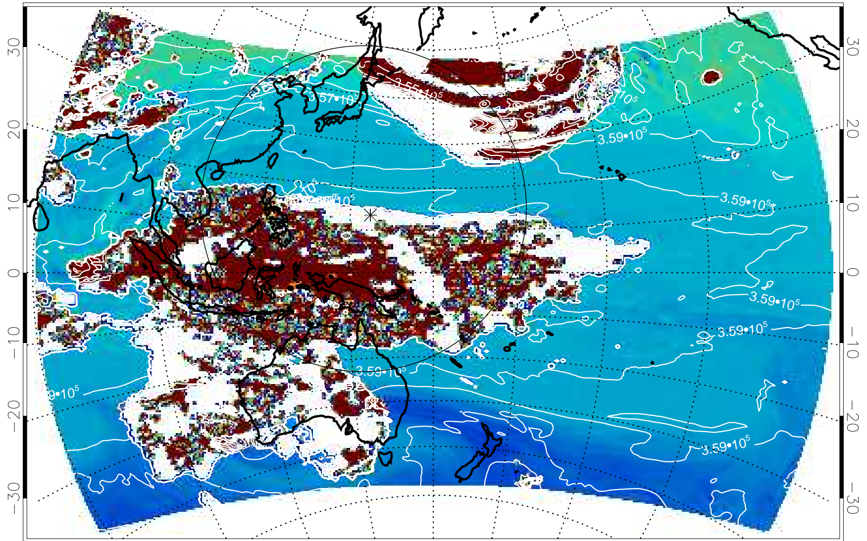
380K Montgomery Streamfunction, white
