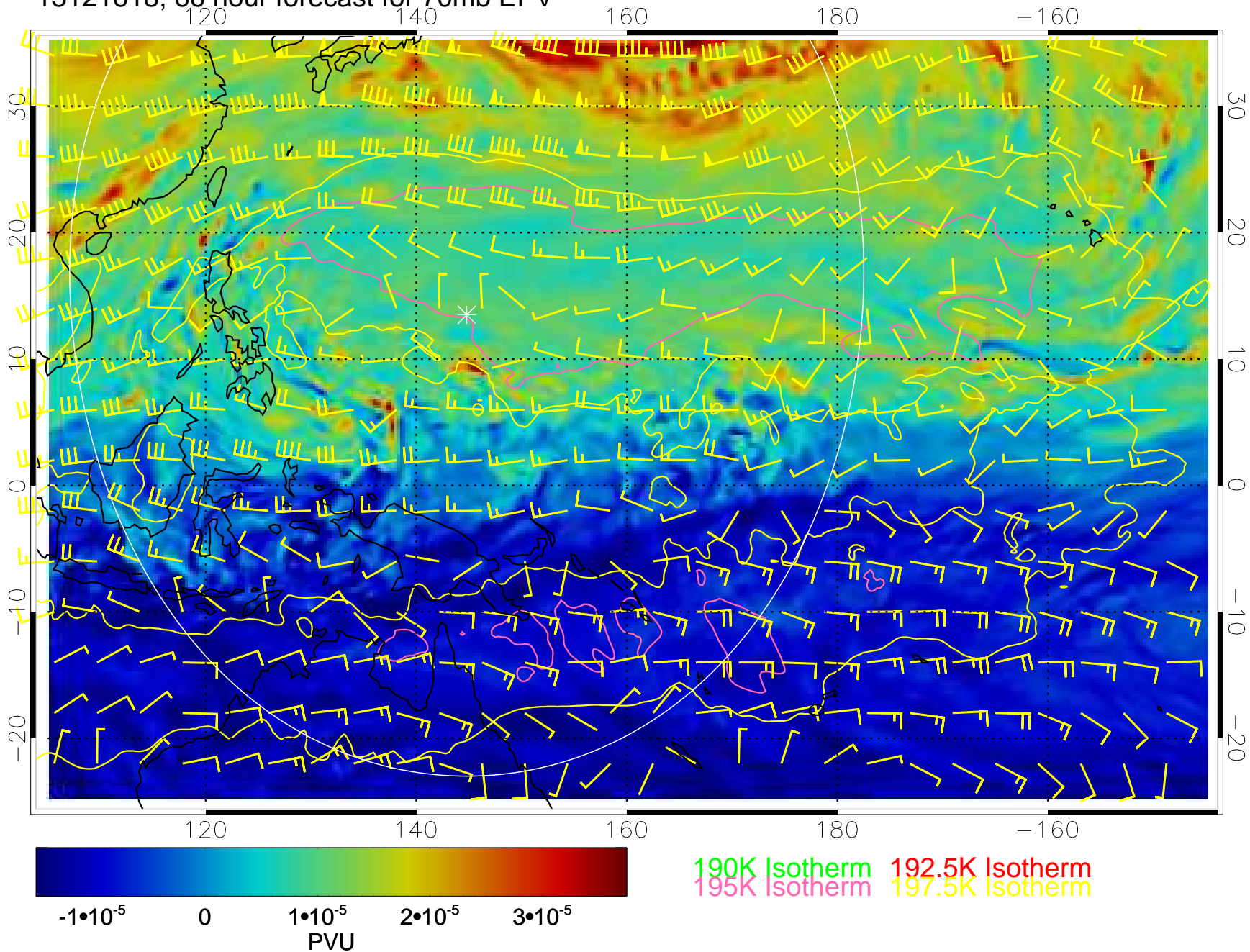
13121618, 66 hour forecast for 70mb EPV
