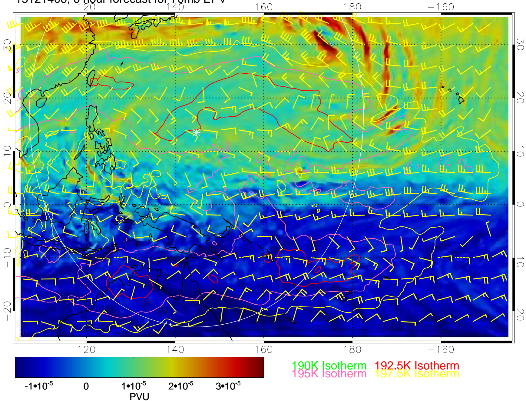
13121406, 6 hour forecast for 70mb EPV
