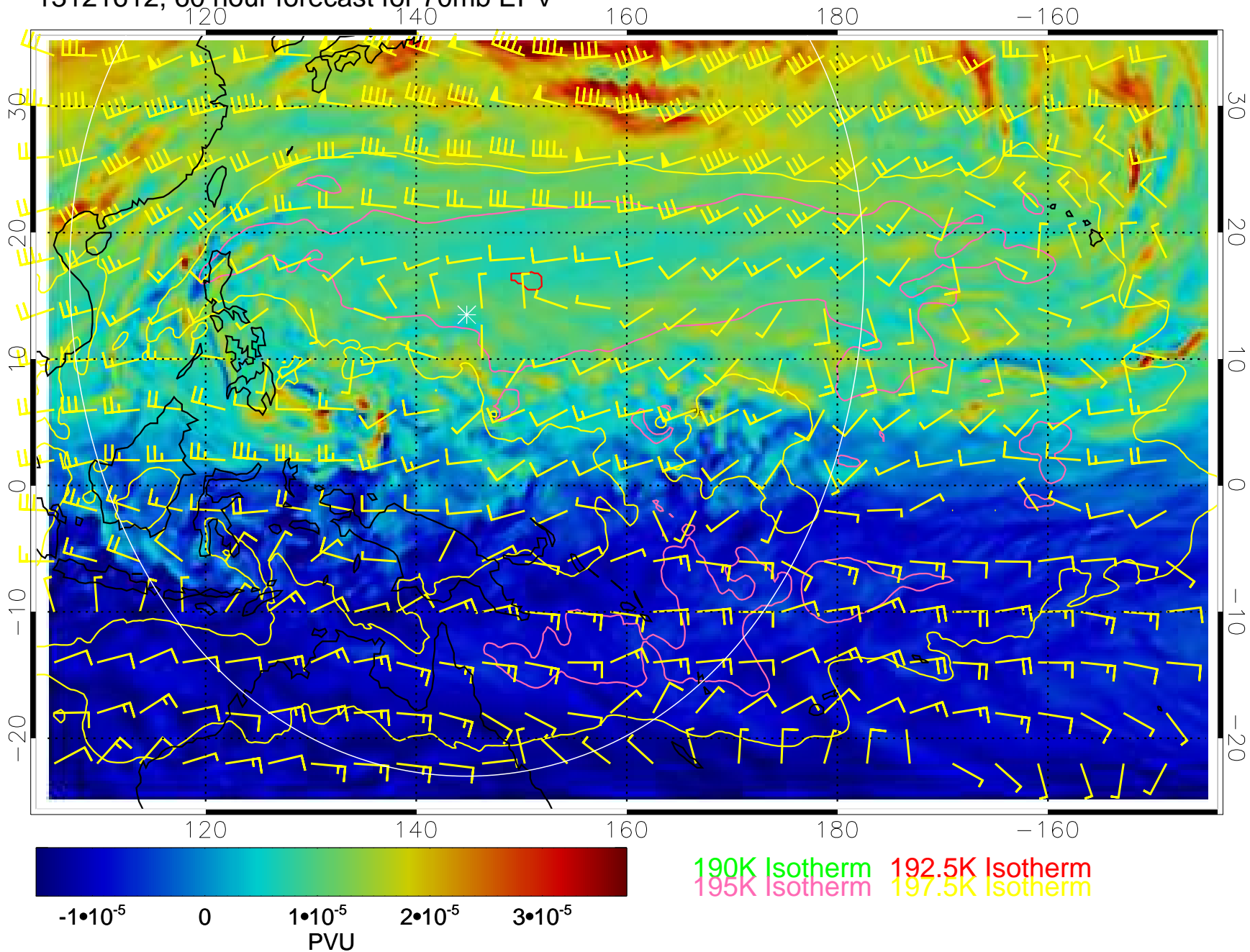
13121612, 60 hour forecast for 70mb EPV
