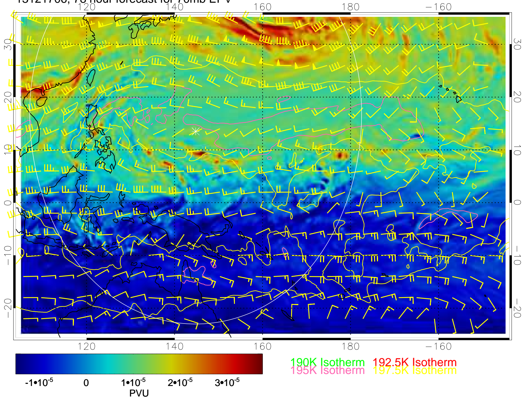
13121706, 78 hour forecast for 70mb EPV
