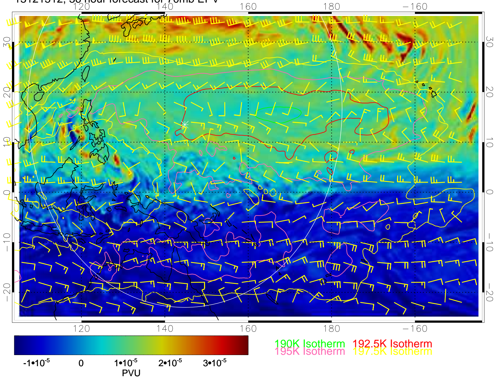
13121512, 36 hour forecast for 70mb EPV
