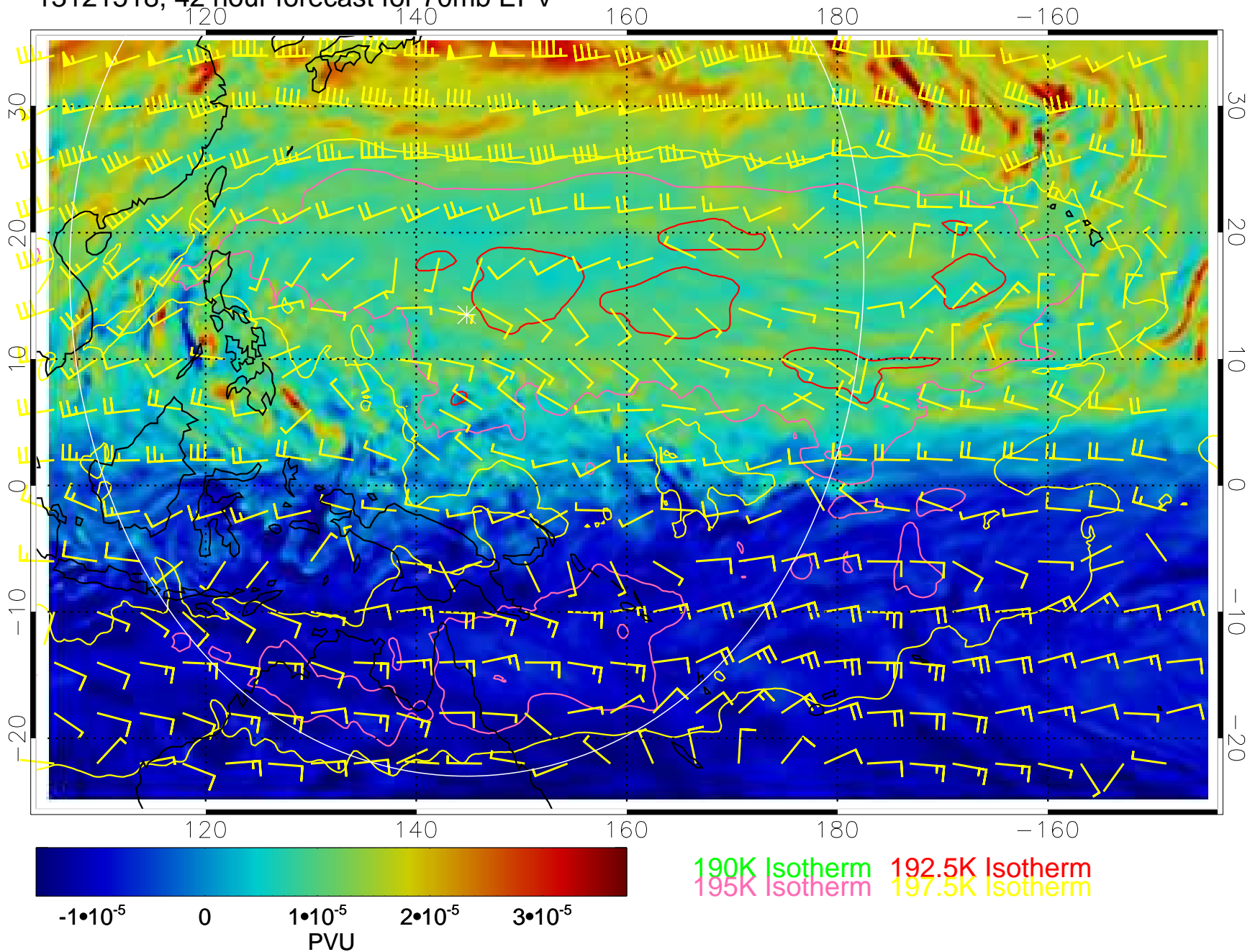
13121518, 42 hour forecast for 70mb EPV
