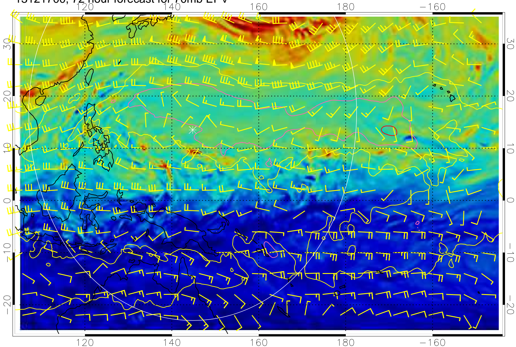
13121700, 72 hour forecast for 70mb EPV
