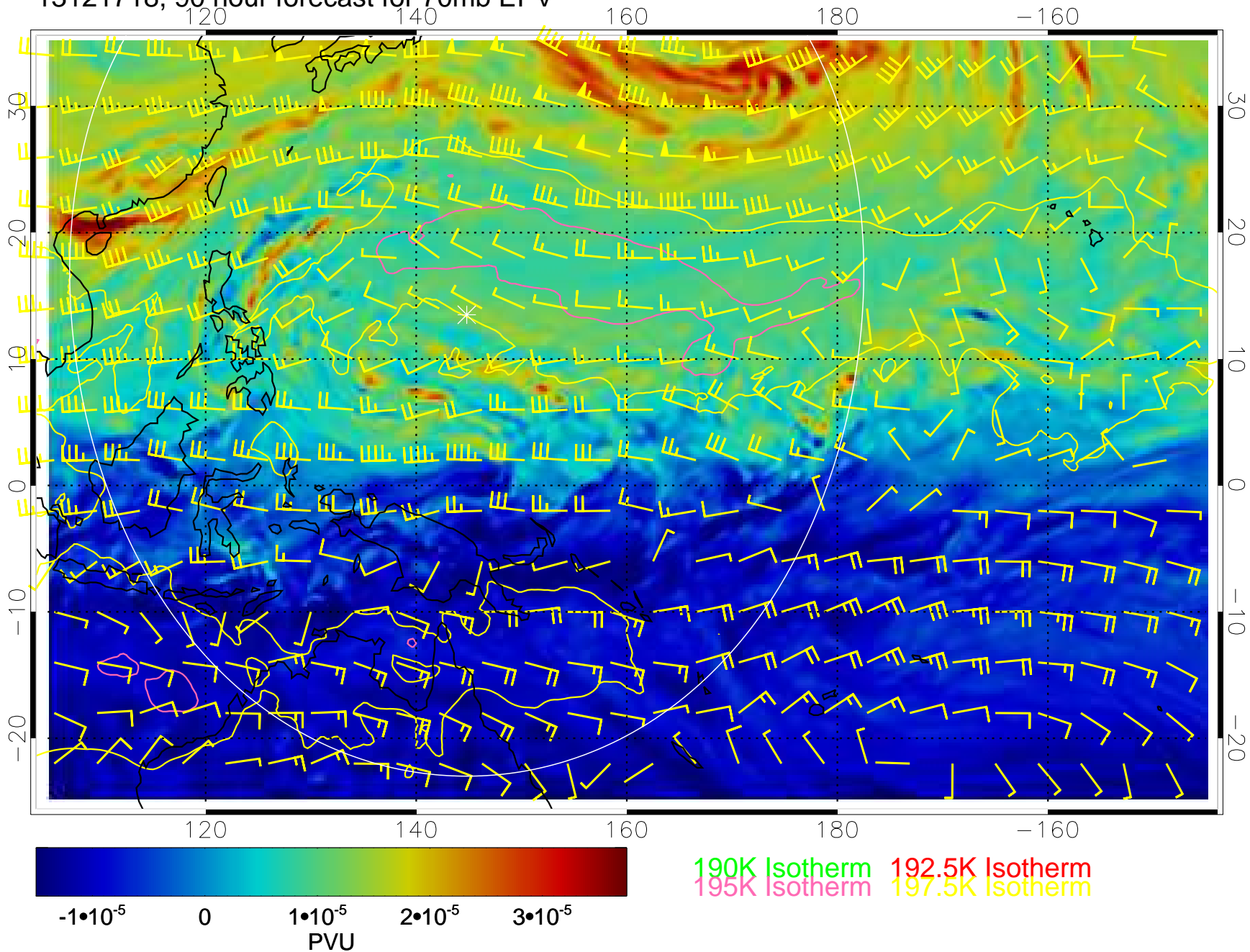
13121718, 90 hour forecast for 70mb EPV
