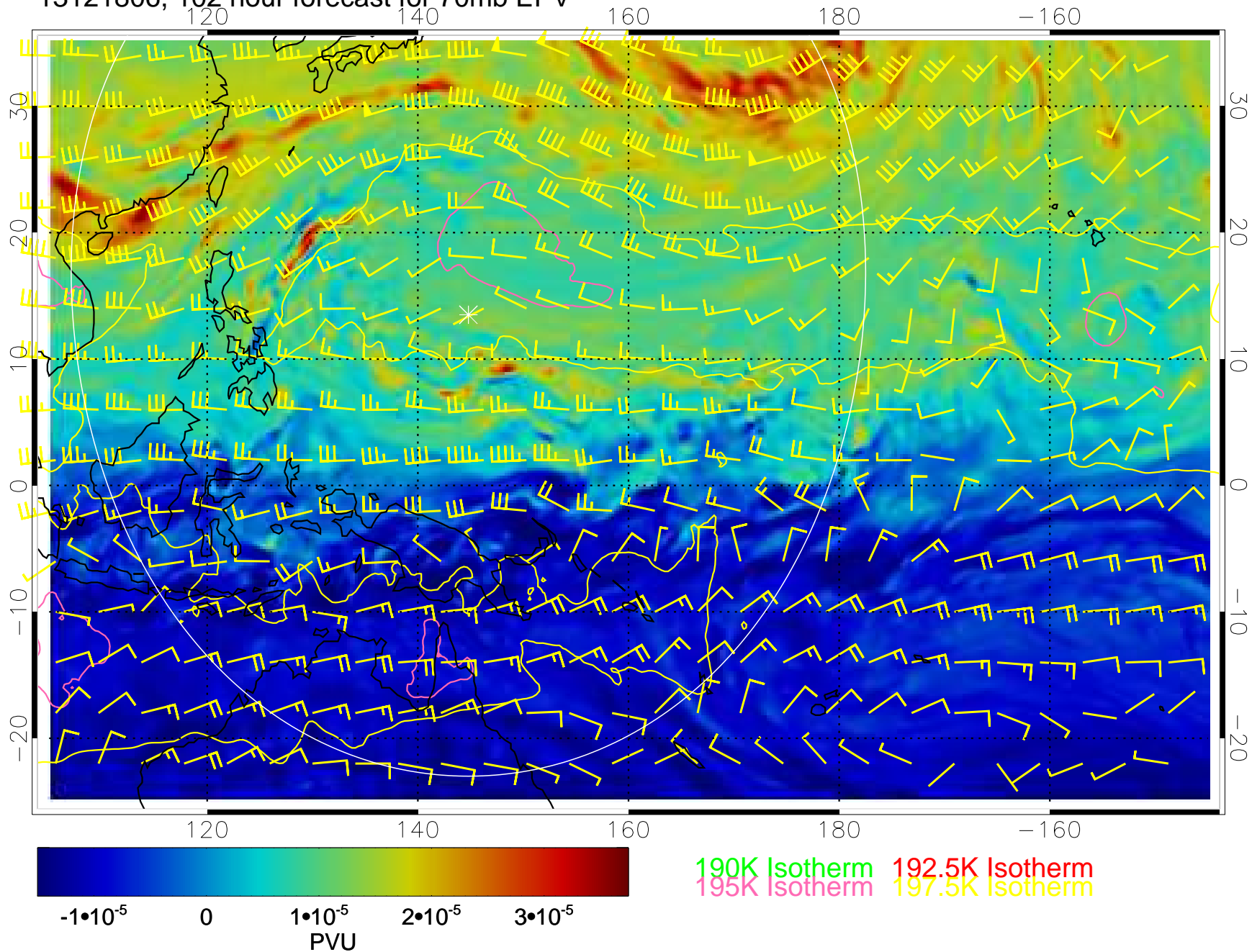
13121806, 102 hour forecast for 70mb EPV
