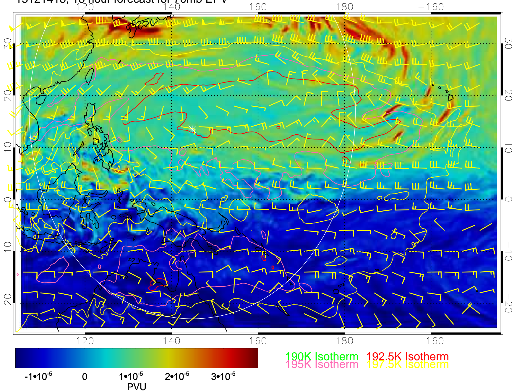
13121418, 18 hour forecast for 70mb EPV
