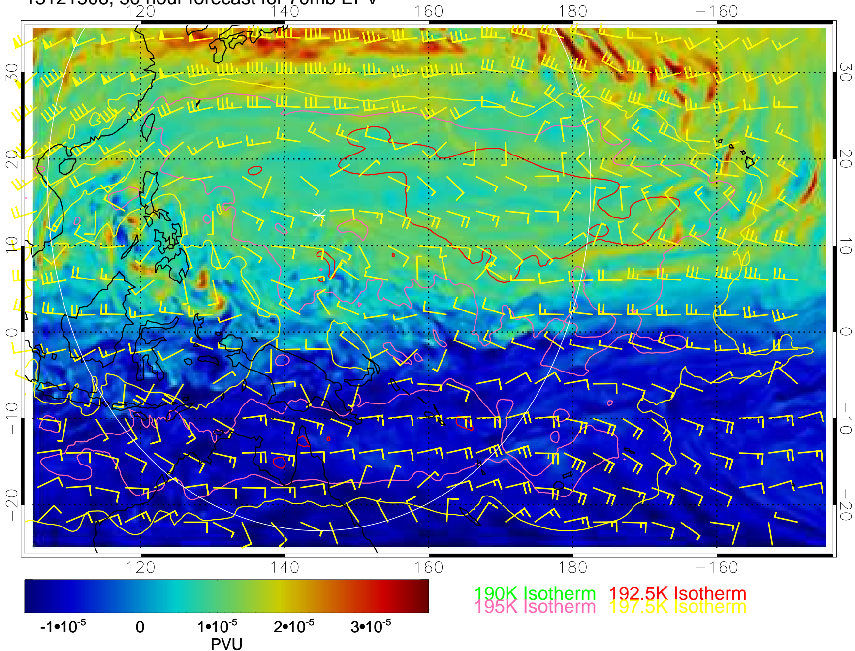
13121506, 30 hour forecast for 70mb EPV
