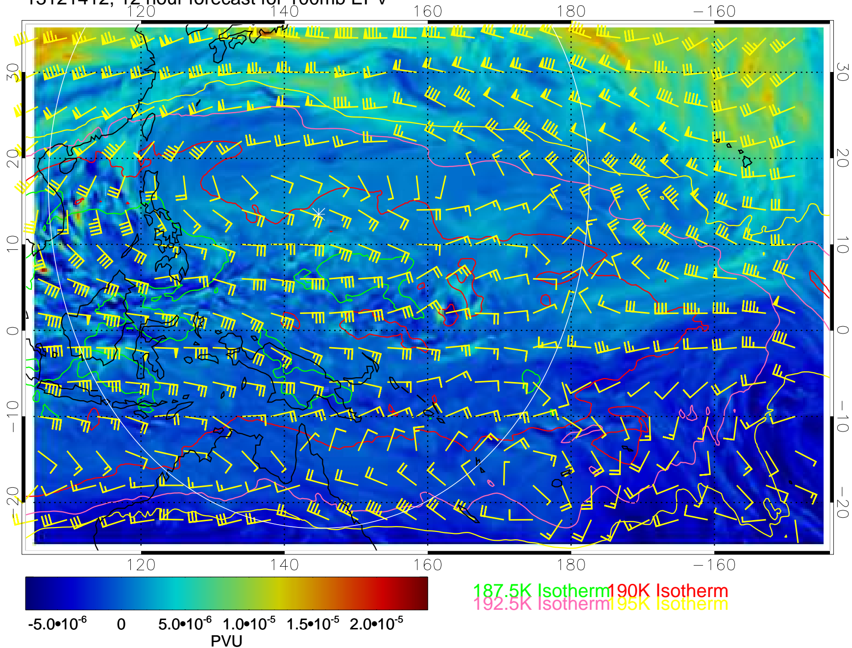
13121412, 12 hour forecast for 100mb EPV
