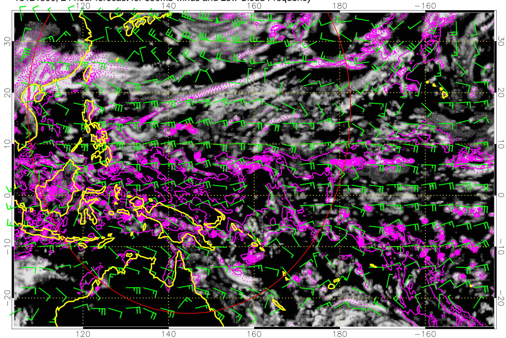
13121500, 24 hour forecast for 850mb winds and Low Cloud Frequency
