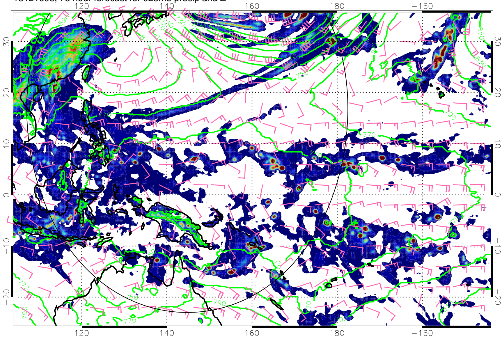
13121606, 78 hour forecast for 925mb precip and Z
