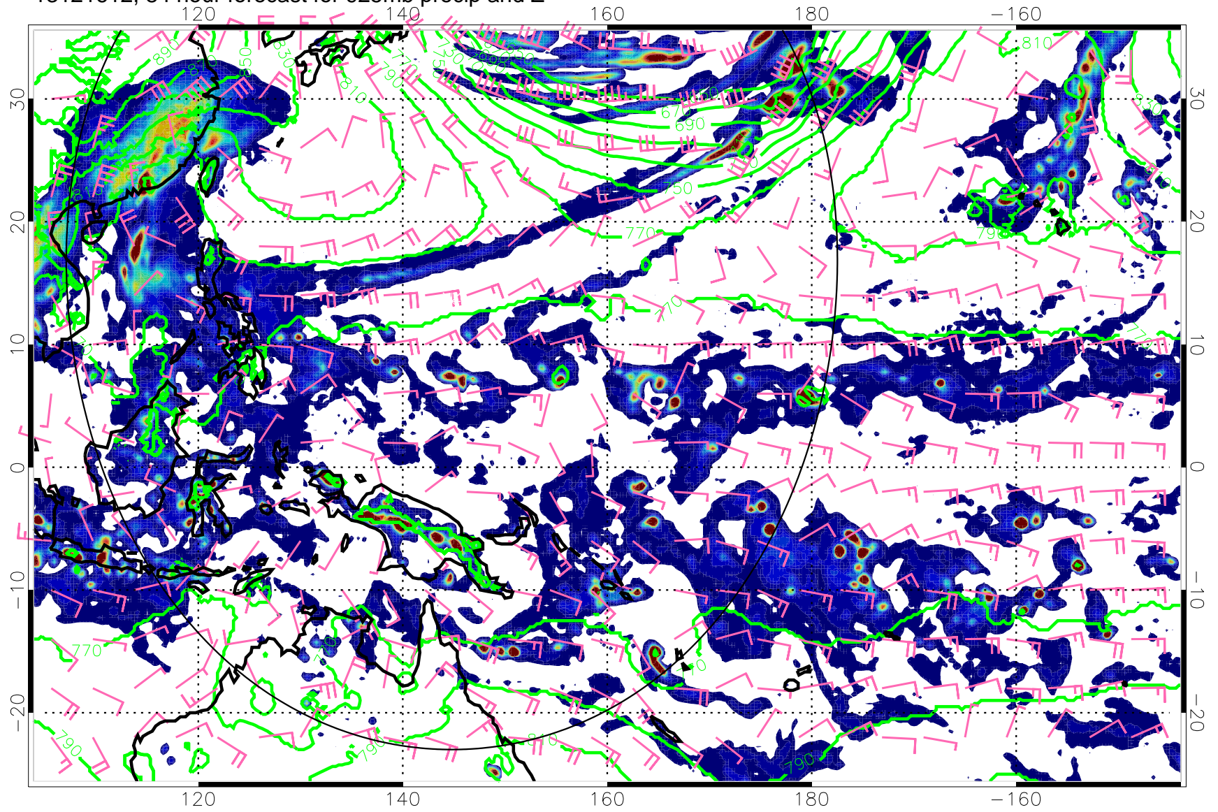
13121612, 84 hour forecast for 925mb precip and Z
