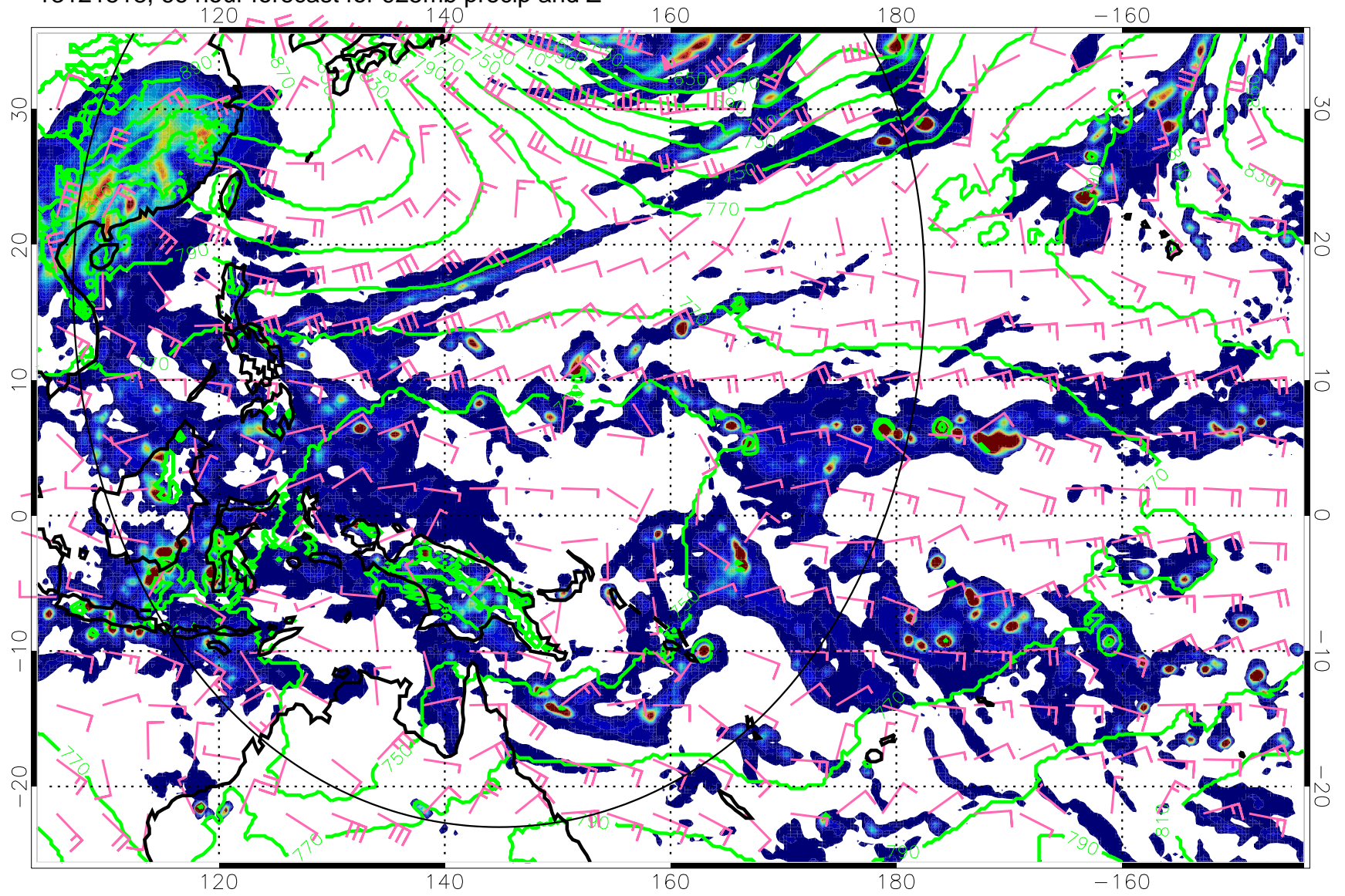
13121518, 66 hour forecast for 925mb precip and Z
