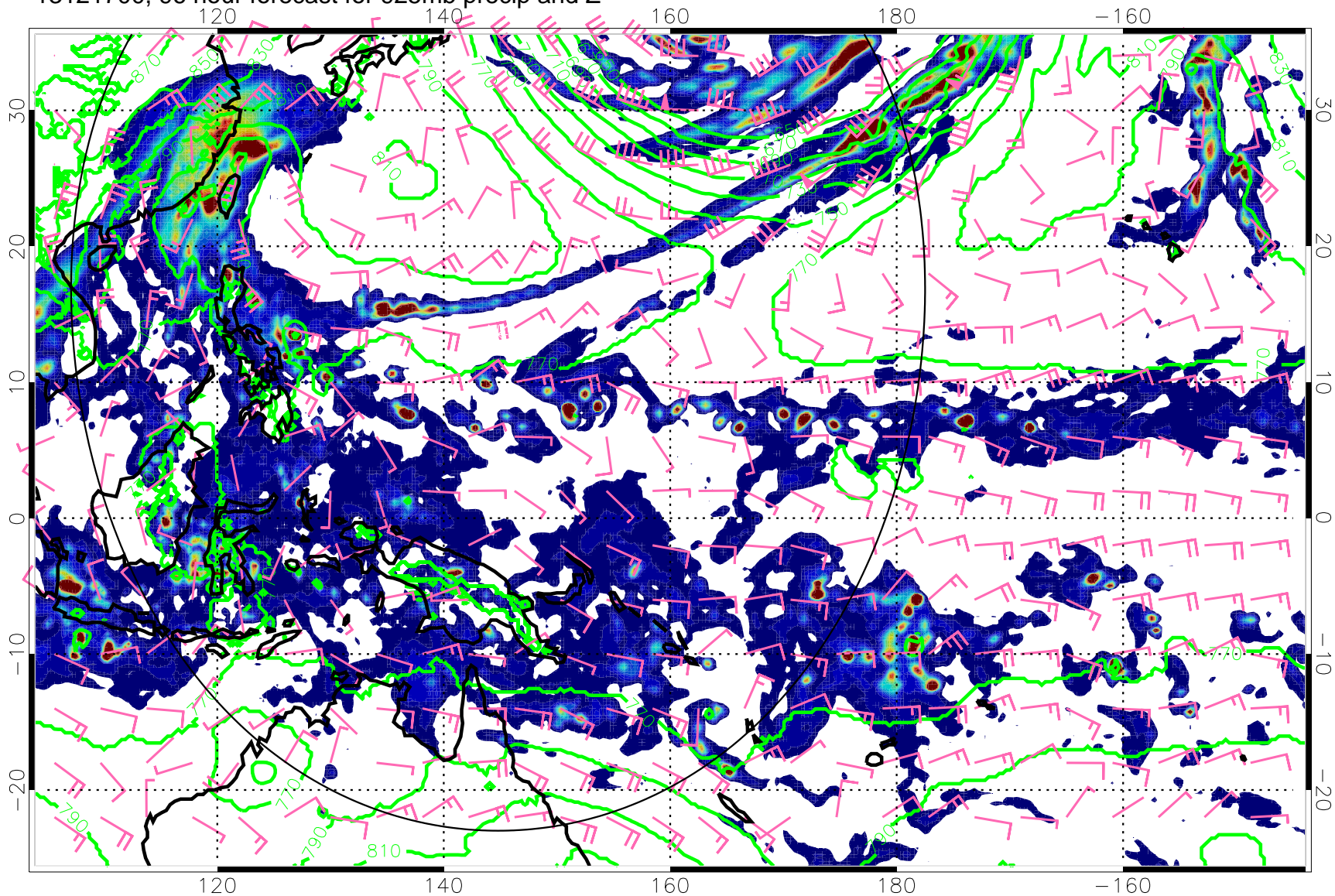
13121700, 96 hour forecast for 925mb precip and Z
