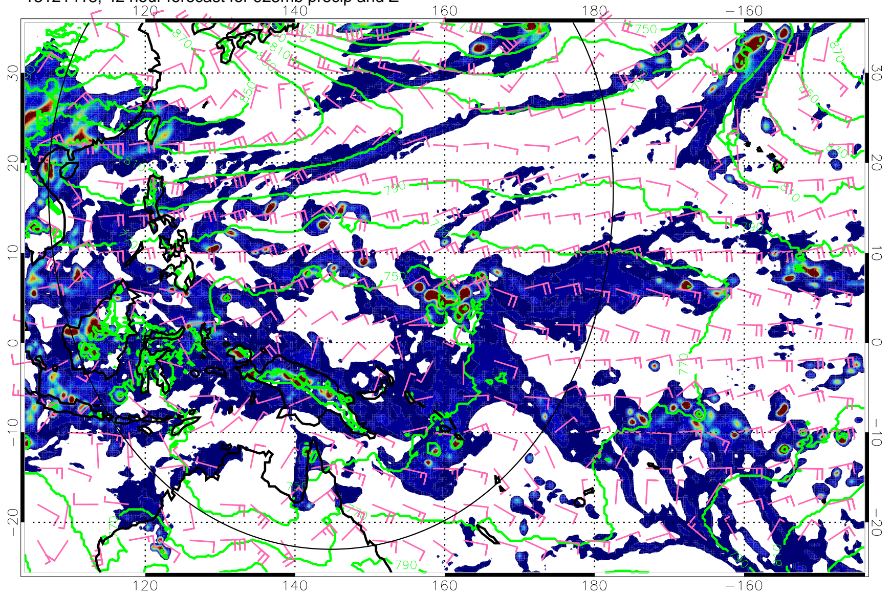
13121418, 42 hour forecast for 925mb precip and Z
