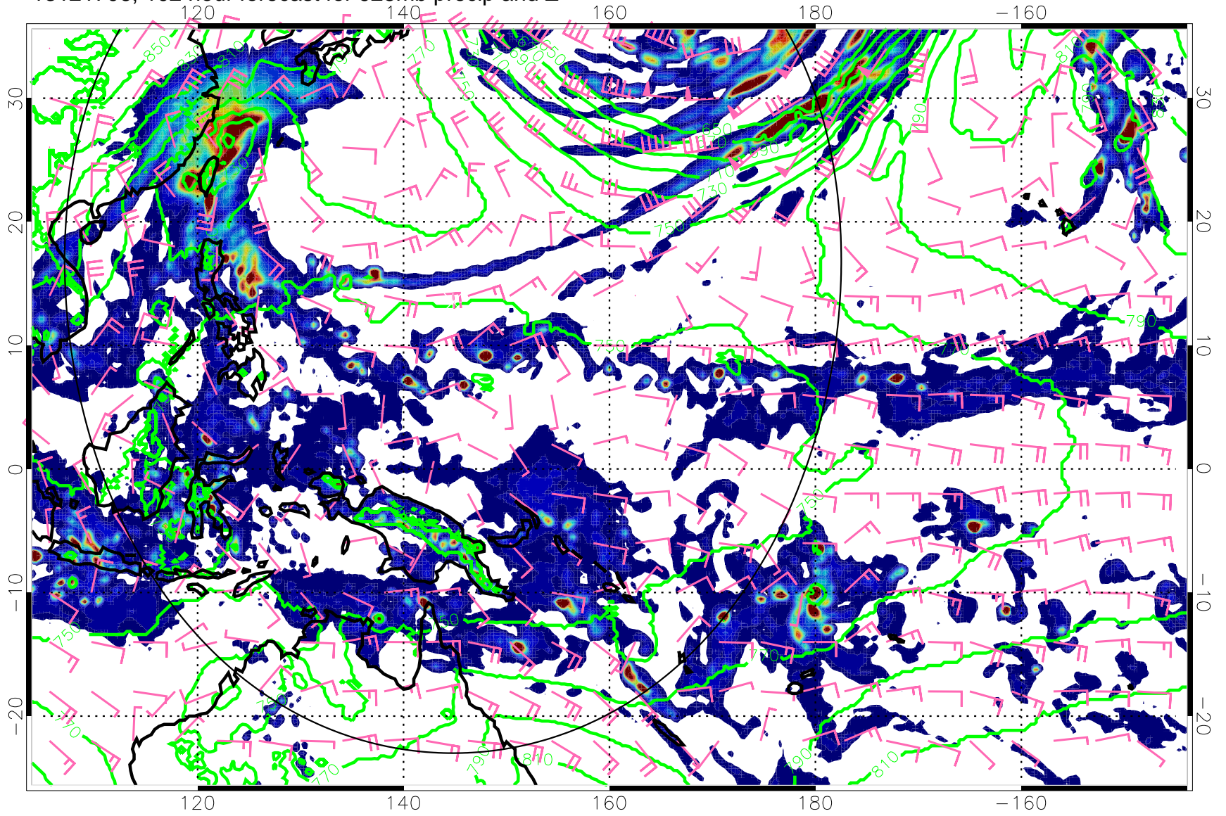
13121706, 102 hour forecast for 925mb precip and Z
