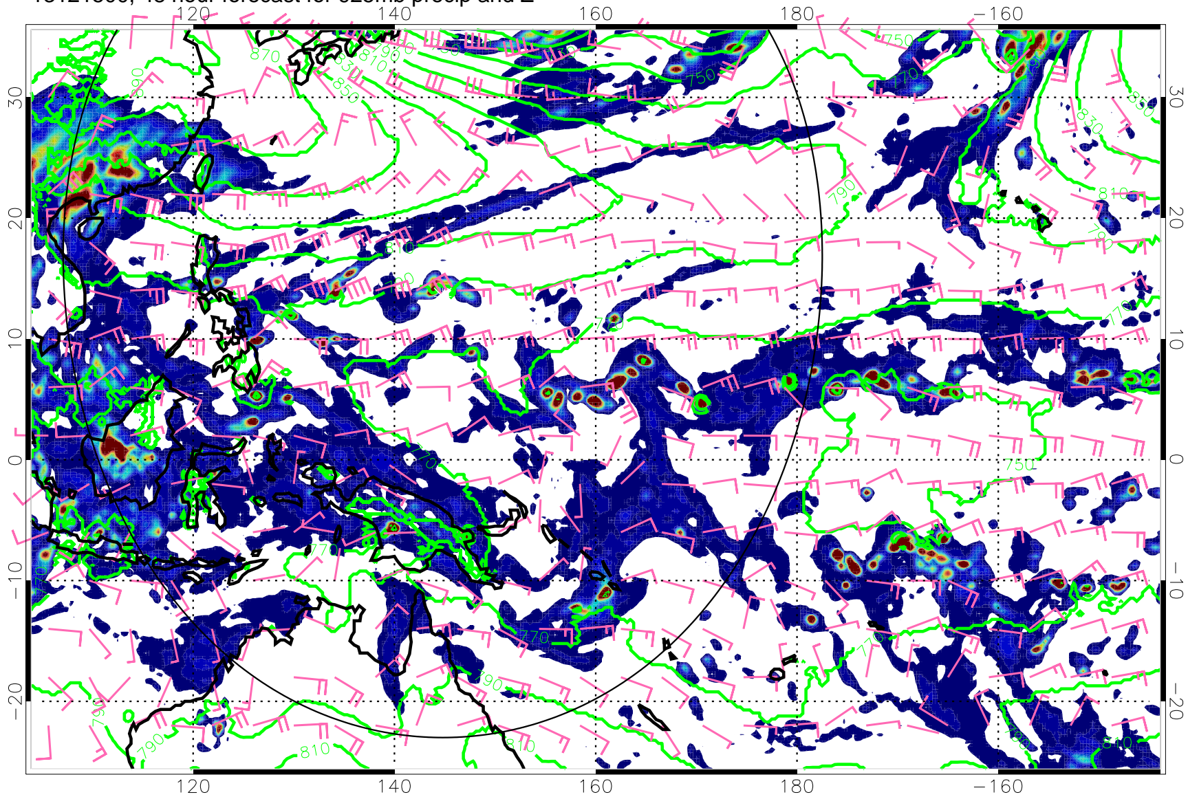
13121500, 48 hour forecast for 925mb precip and Z
