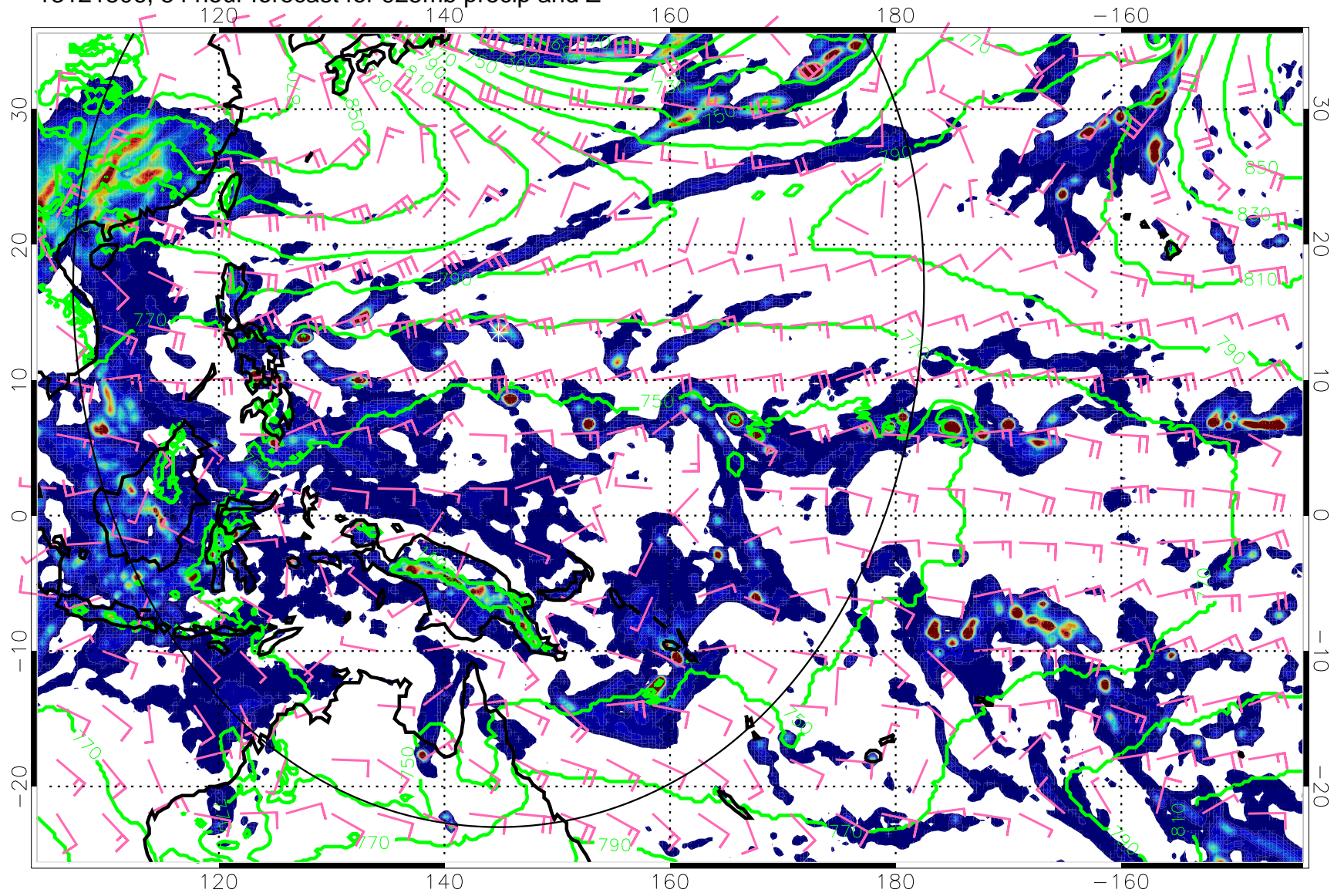
13121506, 54 hour forecast for 925mb precip and Z
