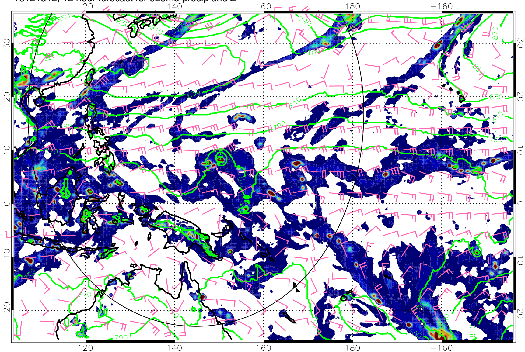
13121312, 12 hour forecast for 925mb precip and Z
