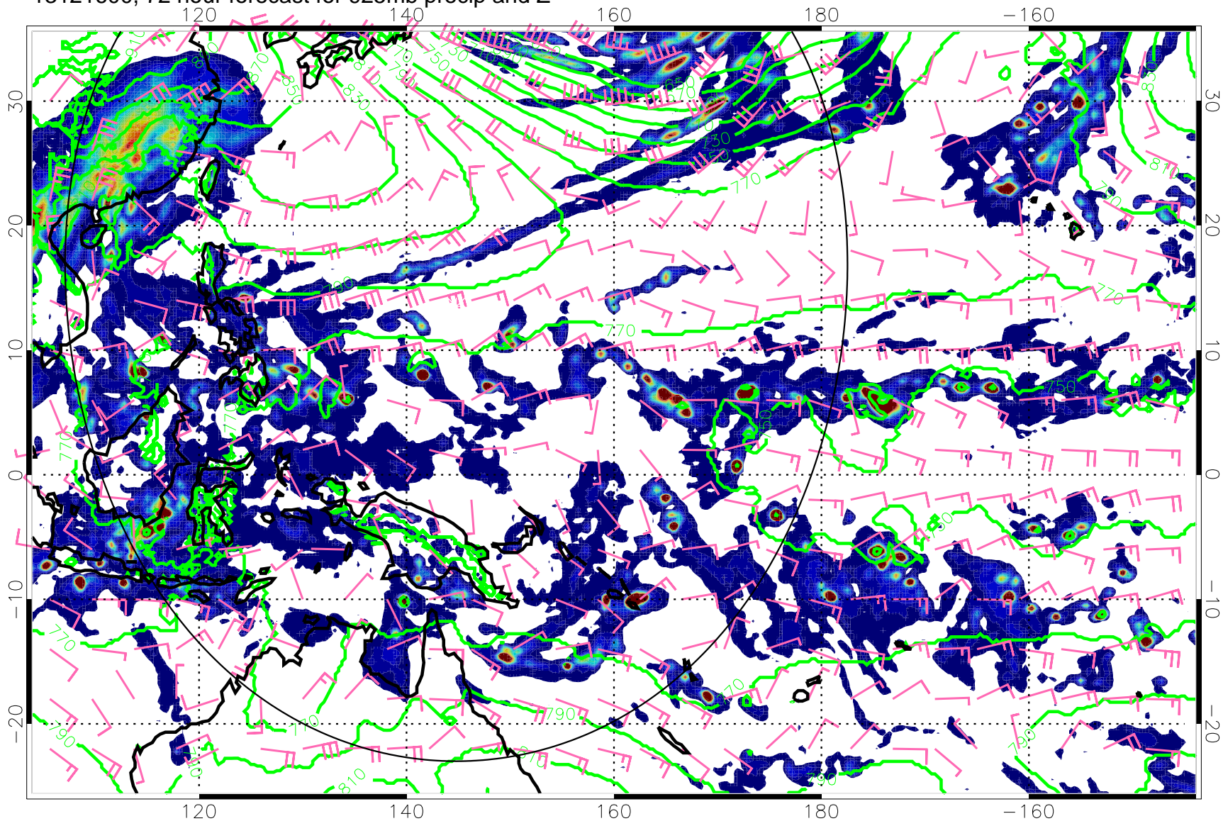
13121600, 72 hour forecast for 925mb precip and Z
