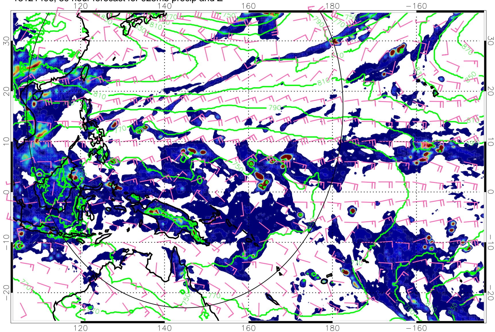
13121406, 30 hour forecast for 925mb precip and Z
