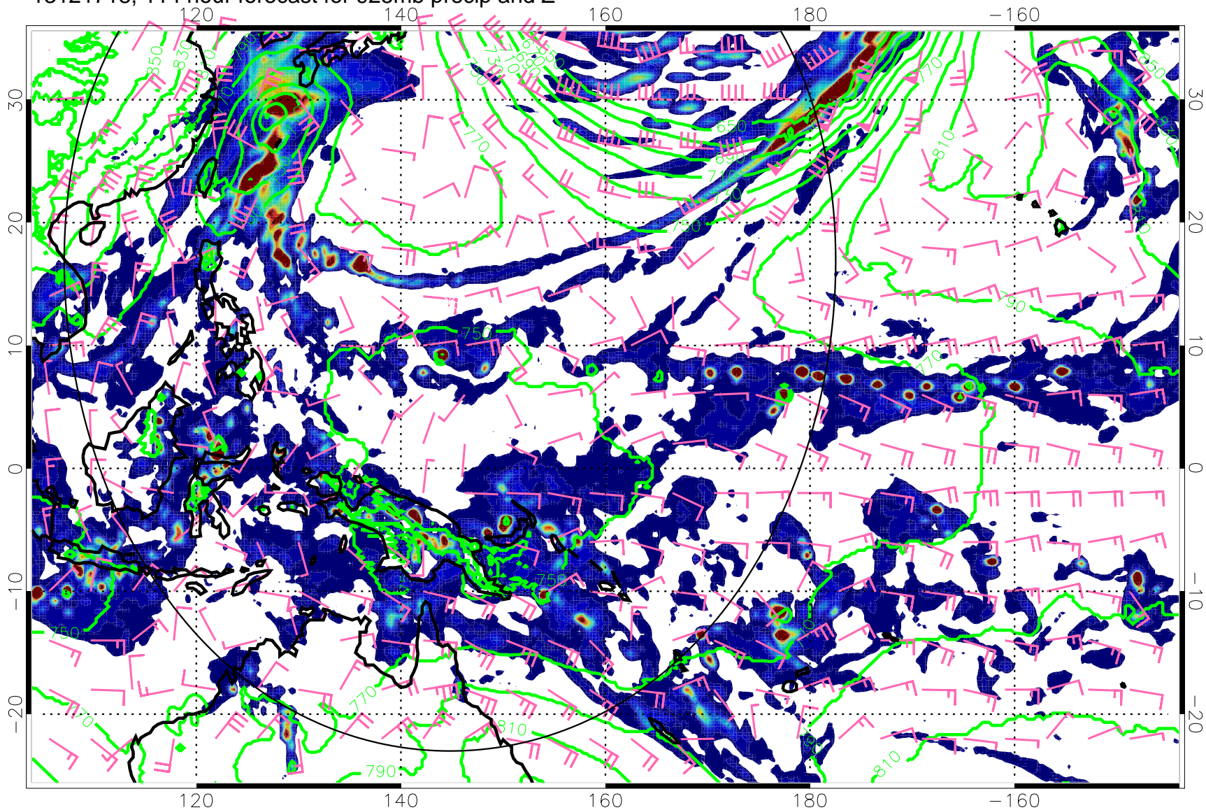
13121718, 114 hour forecast for 925mb precip and Z
