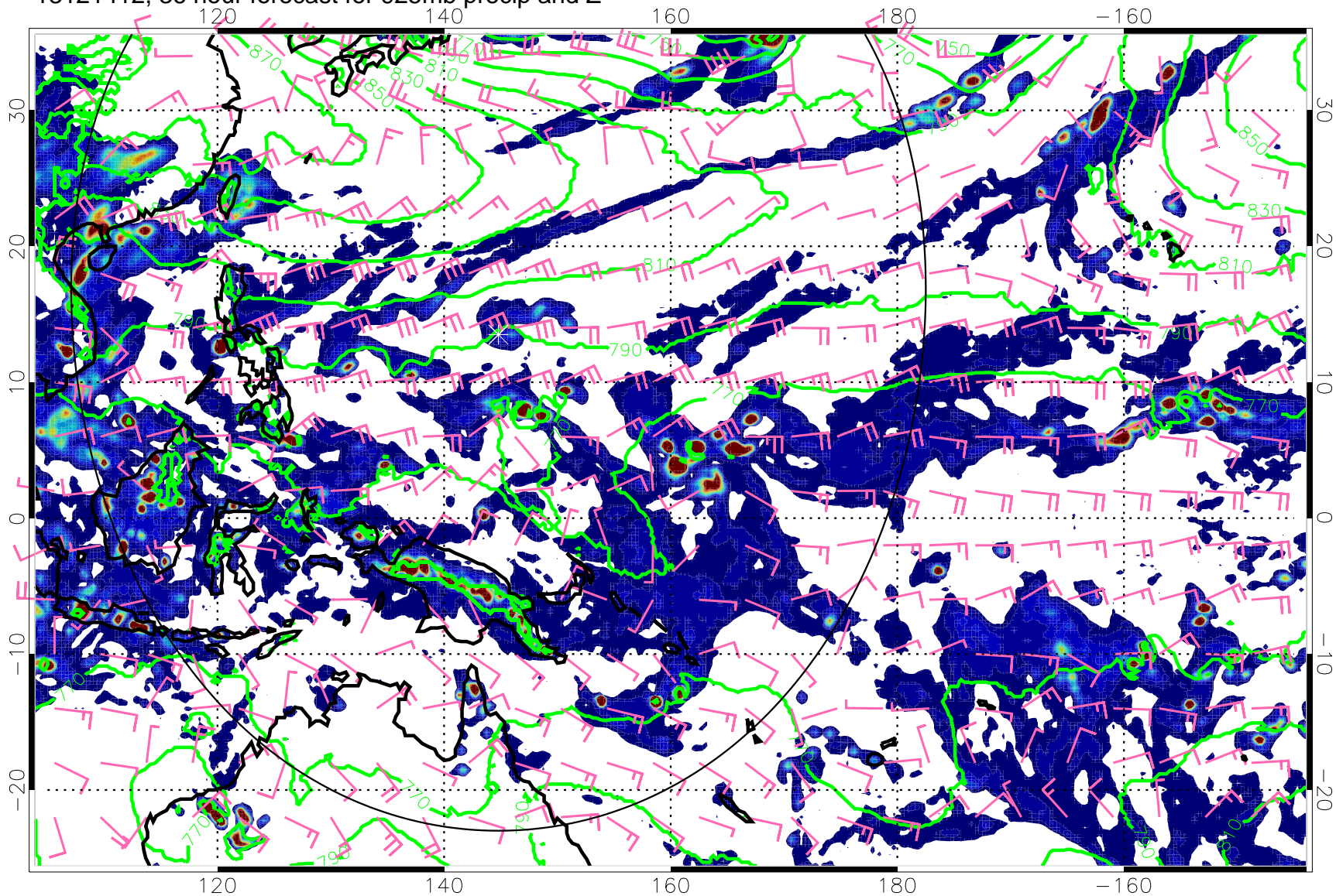
13121412, 36 hour forecast for 925mb precip and Z
