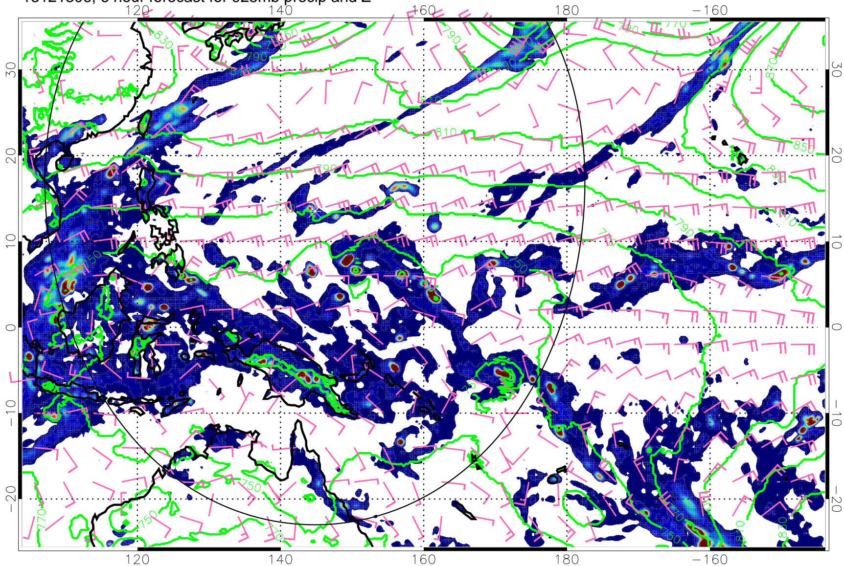
13121306, 6 hour forecast for 925mb precip and Z
