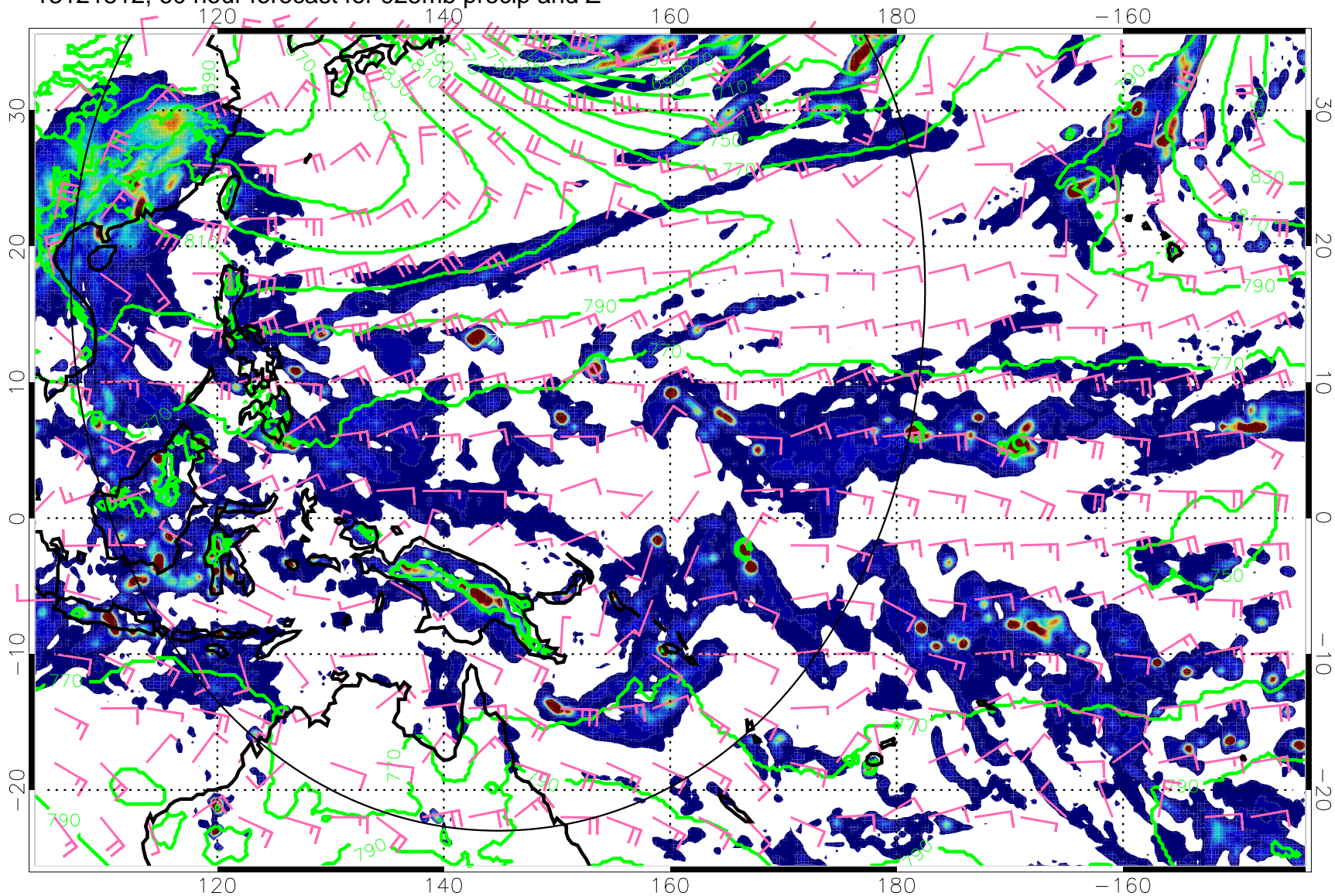
13121512, 60 hour forecast for 925mb precip and Z
