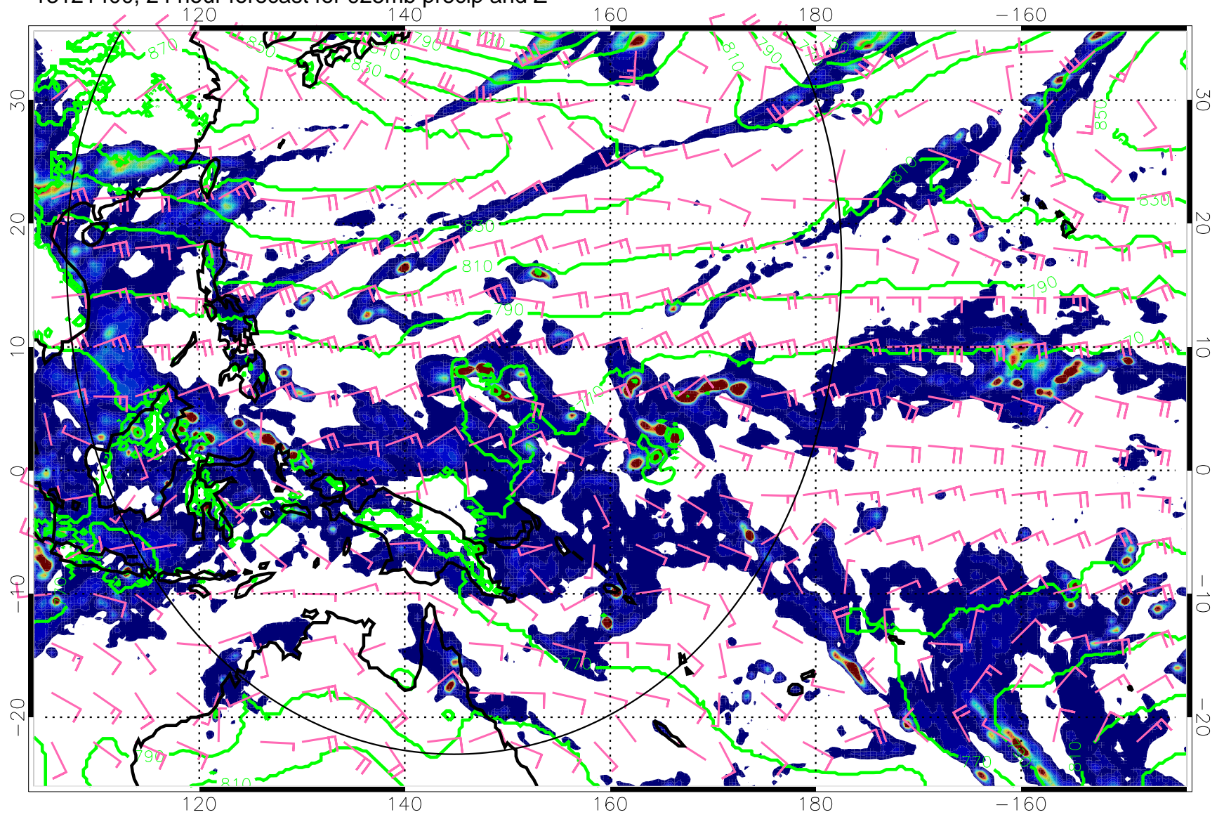
13121400, 24 hour forecast for 925mb precip and Z
