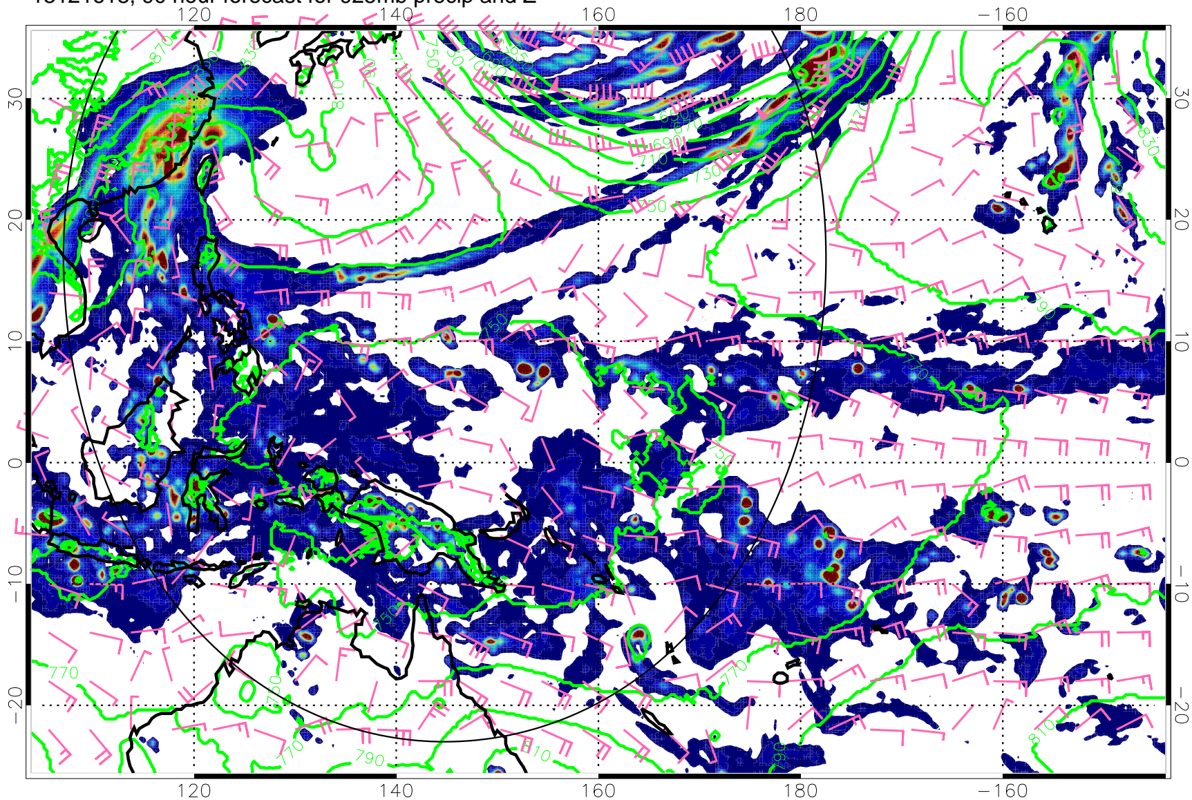
13121618, 90 hour forecast for 925mb precip and Z
