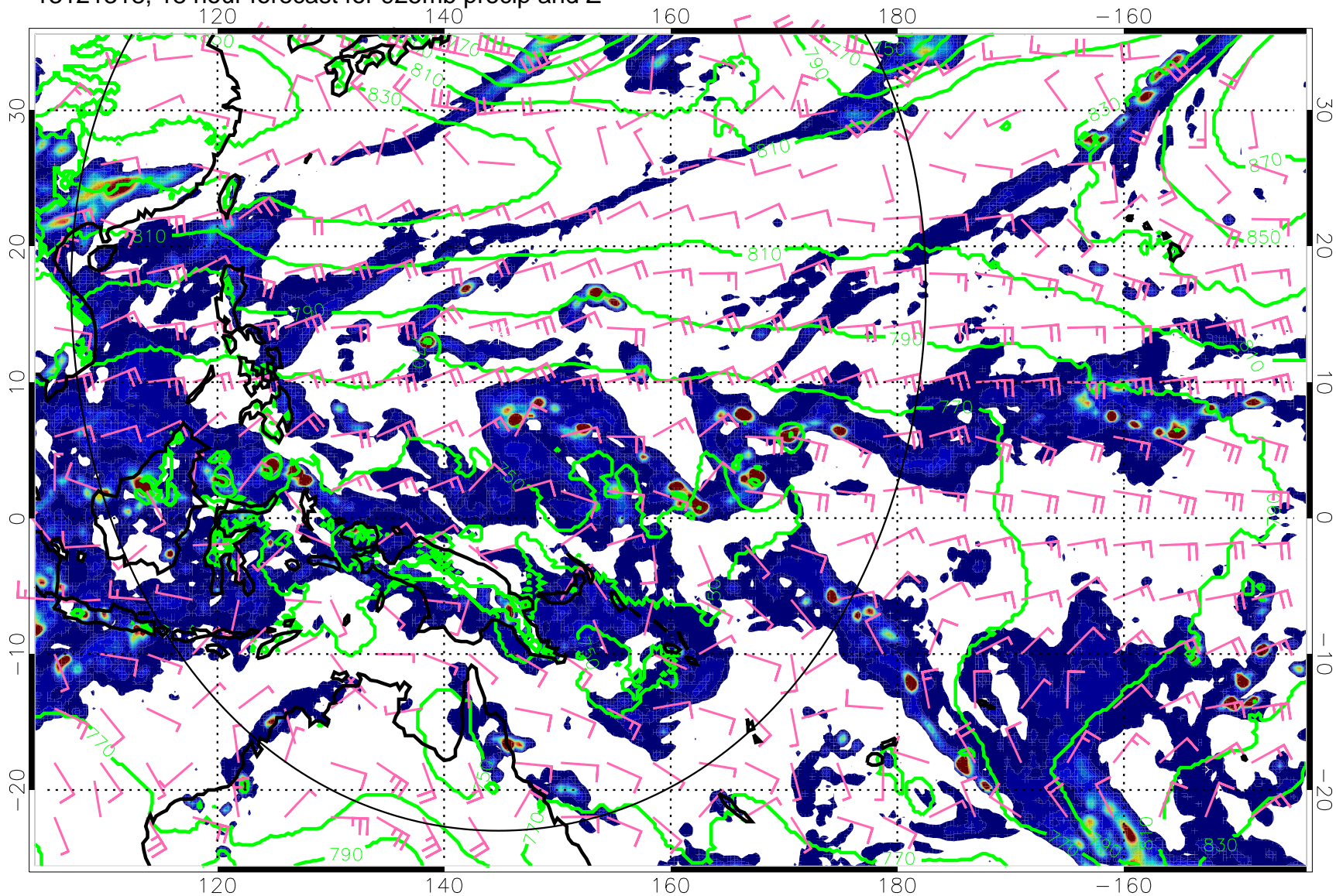
13121318, 18 hour forecast for 925mb precip and Z
