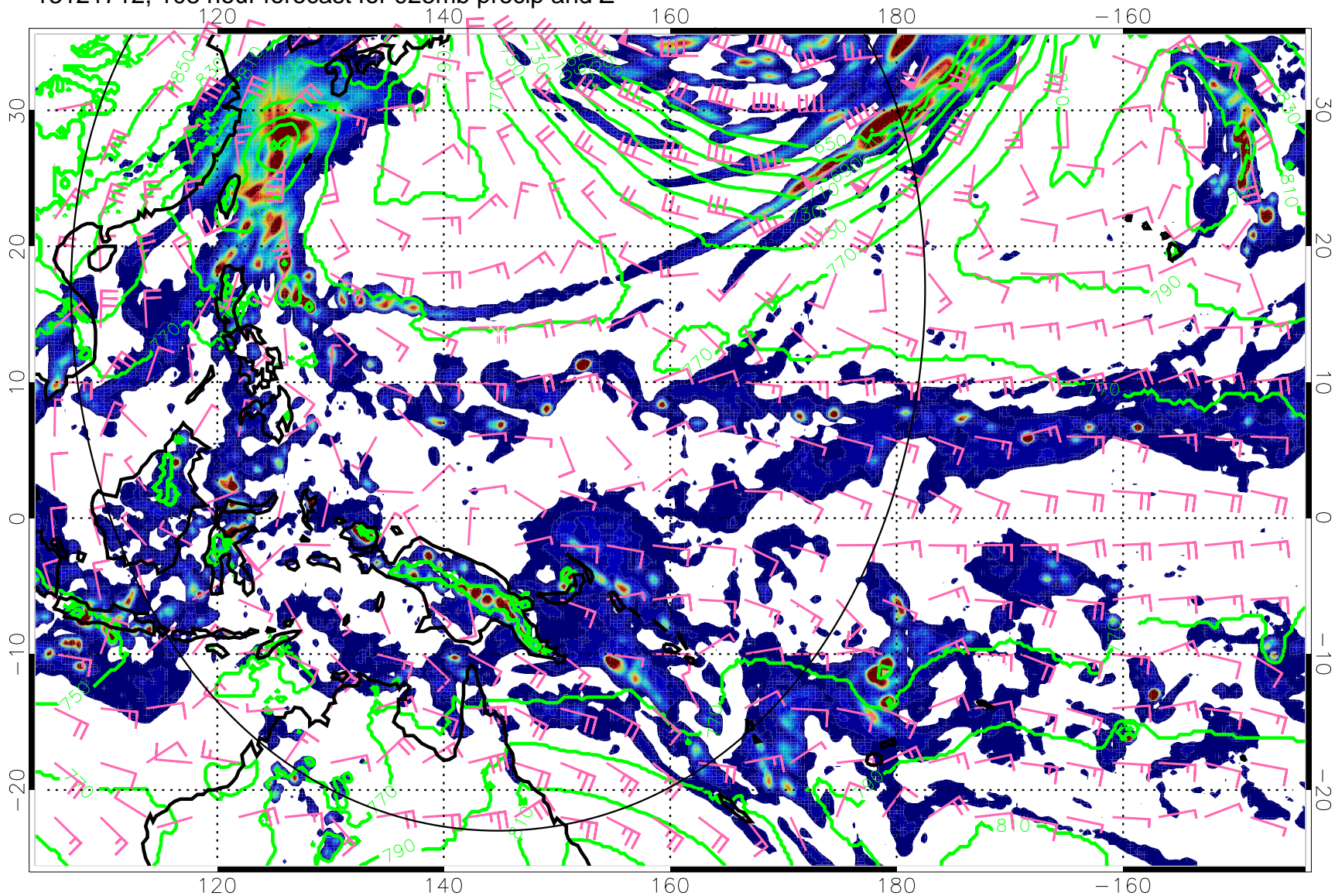
13121712, 108 hour forecast for 925mb precip and Z
