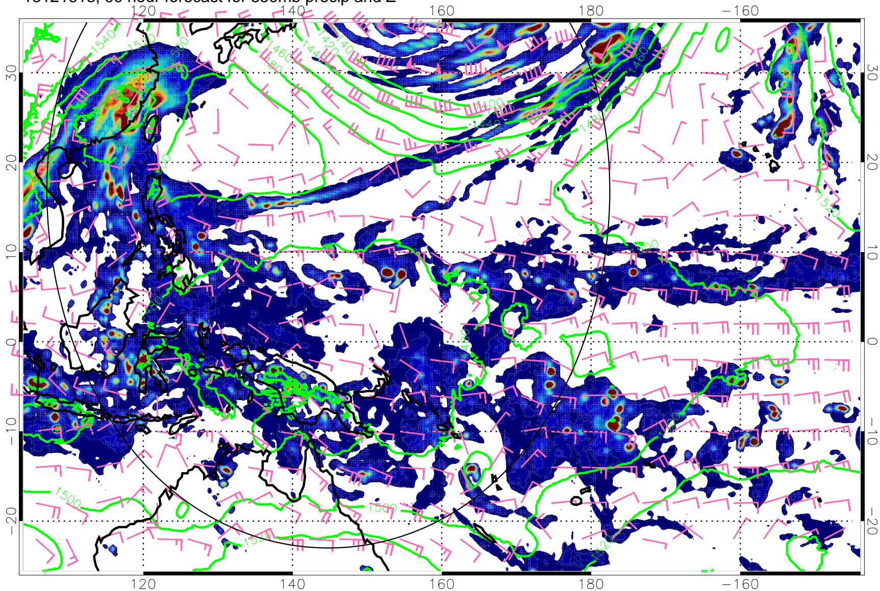
13121618, 90 hour forecast for 850mb precip and Z
