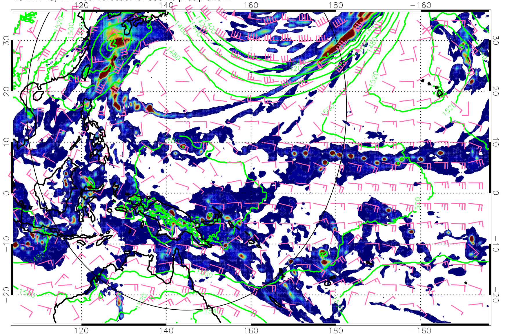
13121718, 114 hour forecast for 850mb precip and Z
