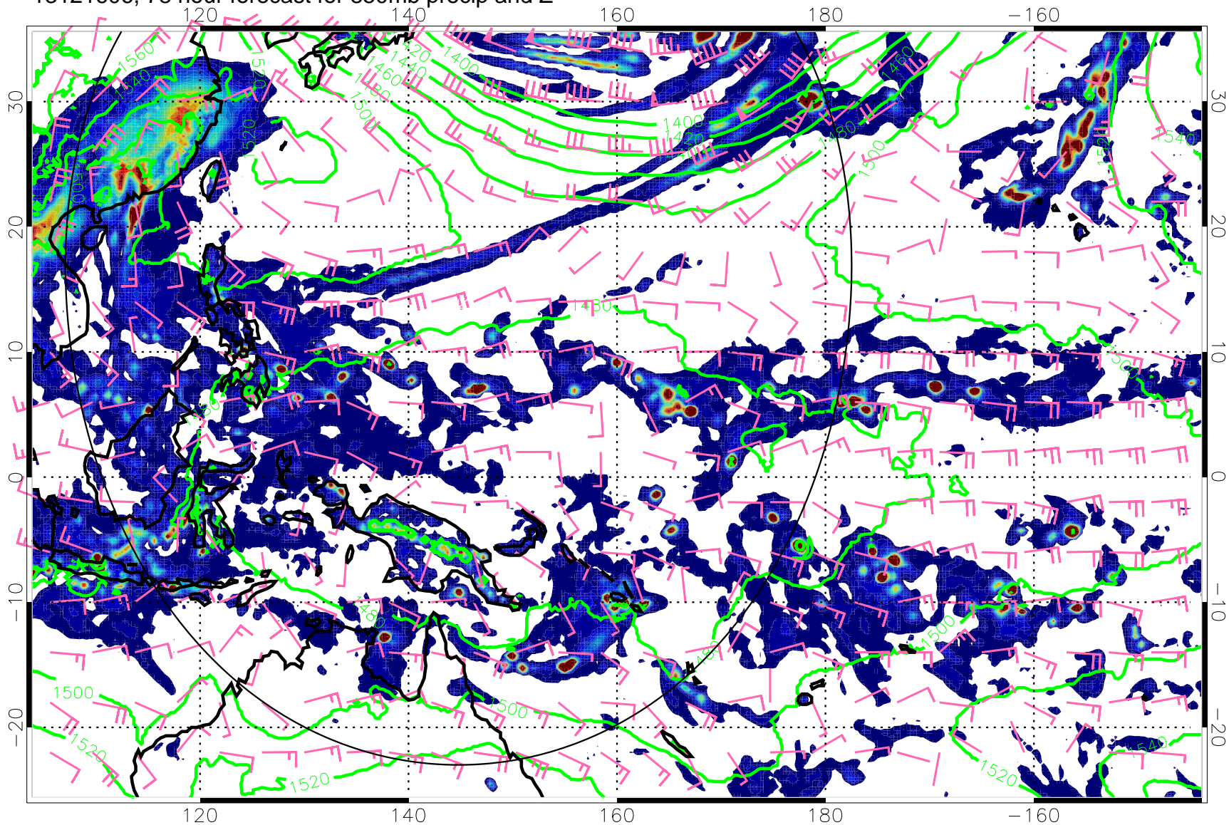
13121606, 78 hour forecast for 850mb precip and Z
