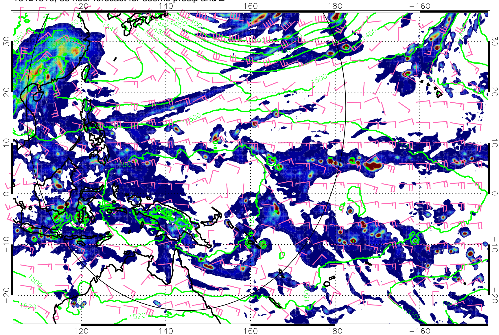
13121518, 66 hour forecast for 850mb precip and Z
