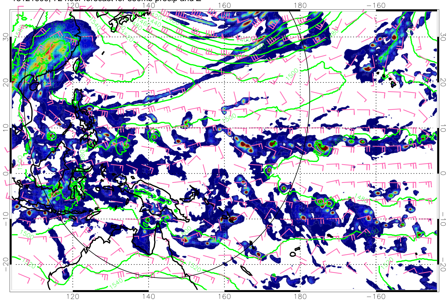
13121600, 72 hour forecast for 850mb precip and Z
