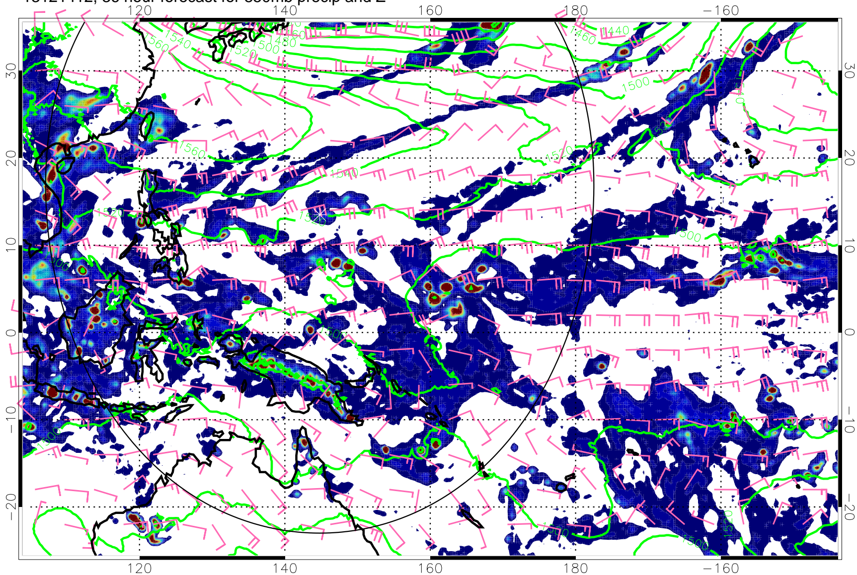
13121412, 36 hour forecast for 850mb precip and Z
