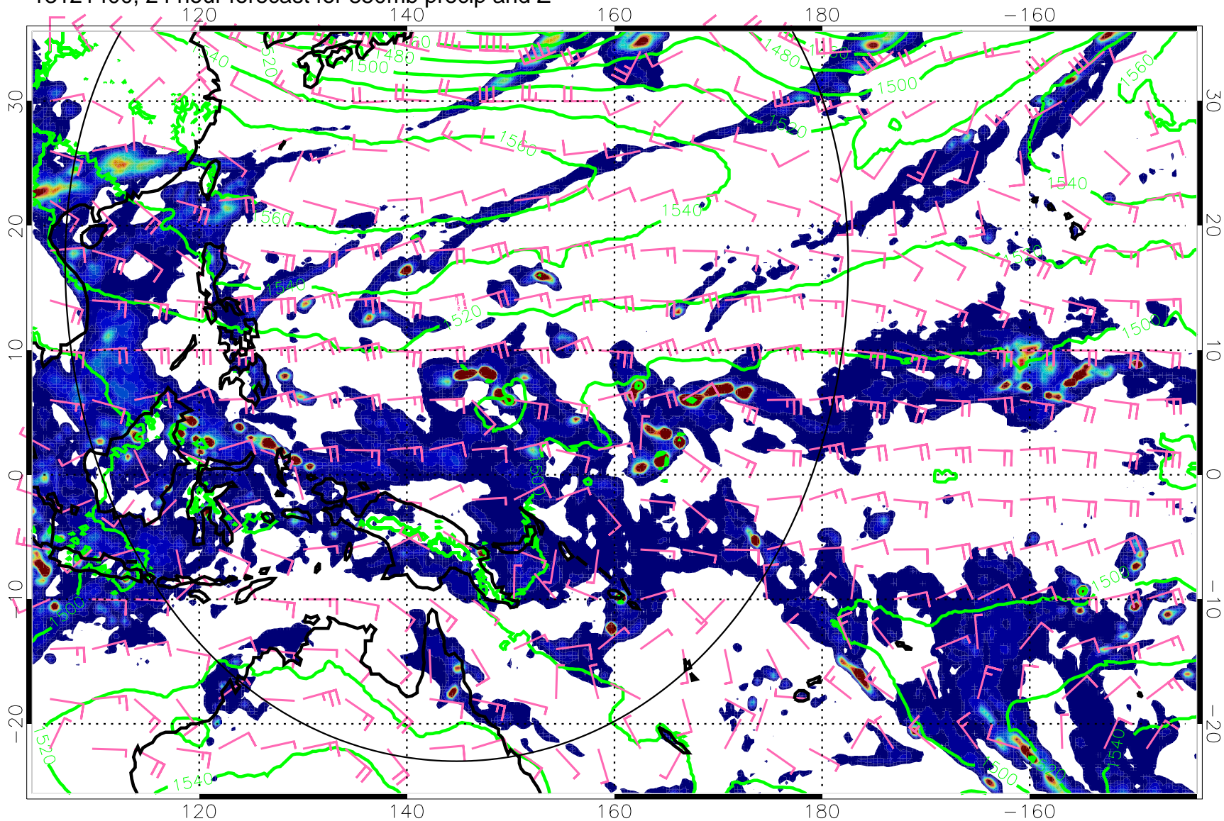
13121400, 24 hour forecast for 850mb precip and Z
