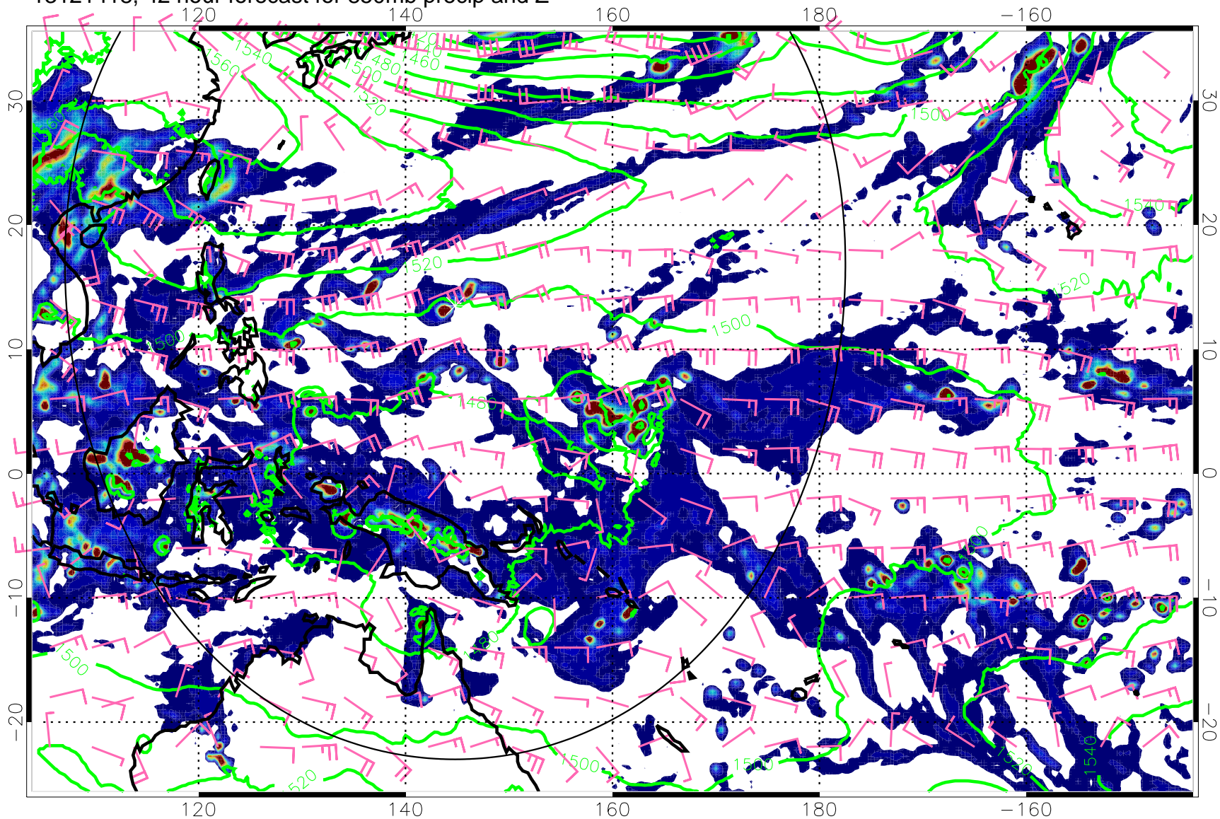
13121418, 42 hour forecast for 850mb precip and Z
