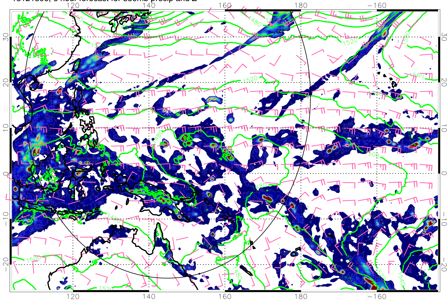
13121306, 6 hour forecast for 850mb precip and Z
