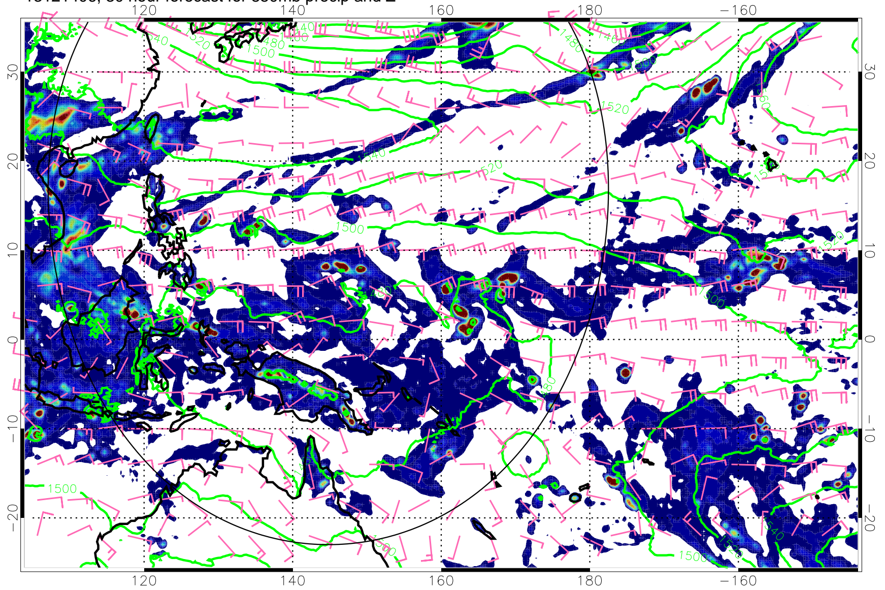
13121406, 30 hour forecast for 850mb precip and Z
