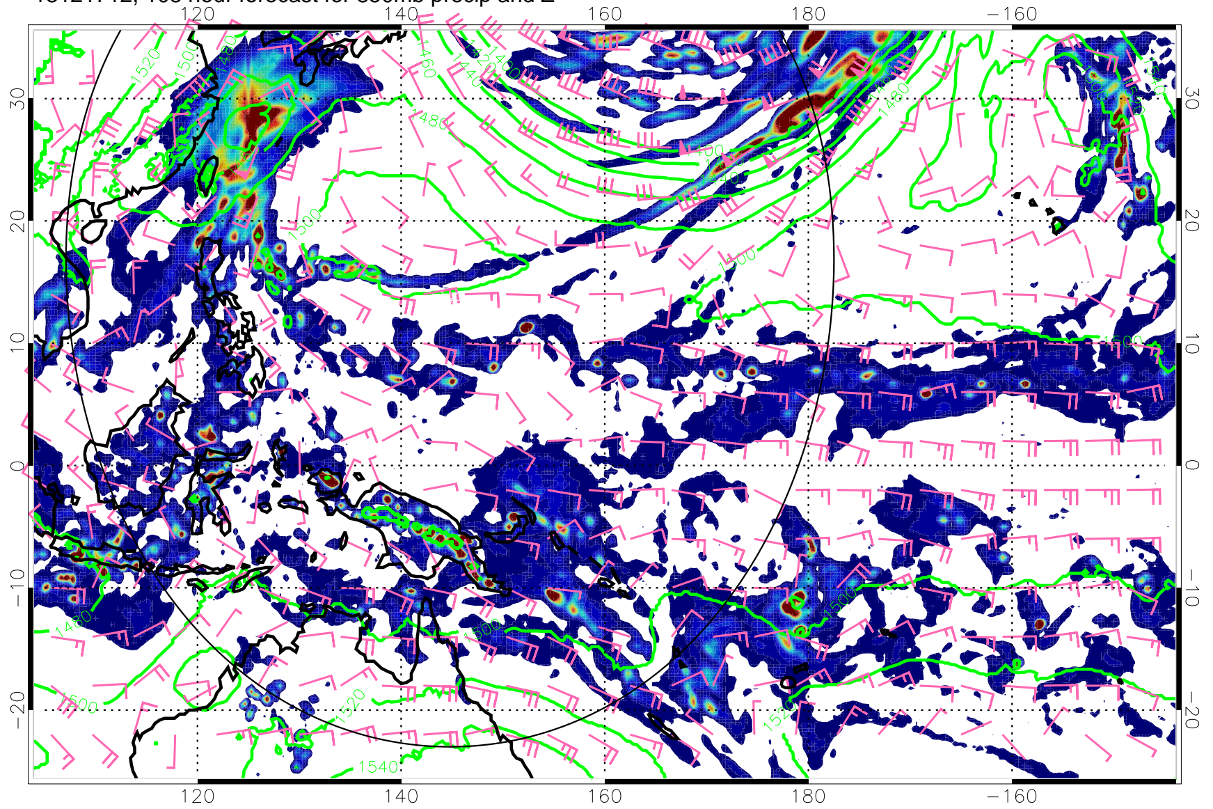
13121712, 108 hour forecast for 850mb precip and Z
