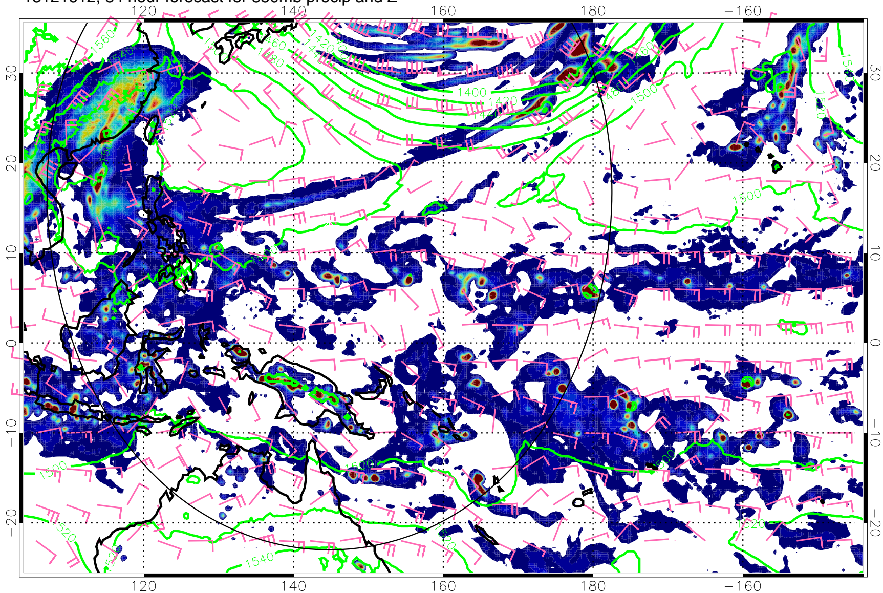
13121612, 84 hour forecast for 850mb precip and Z
