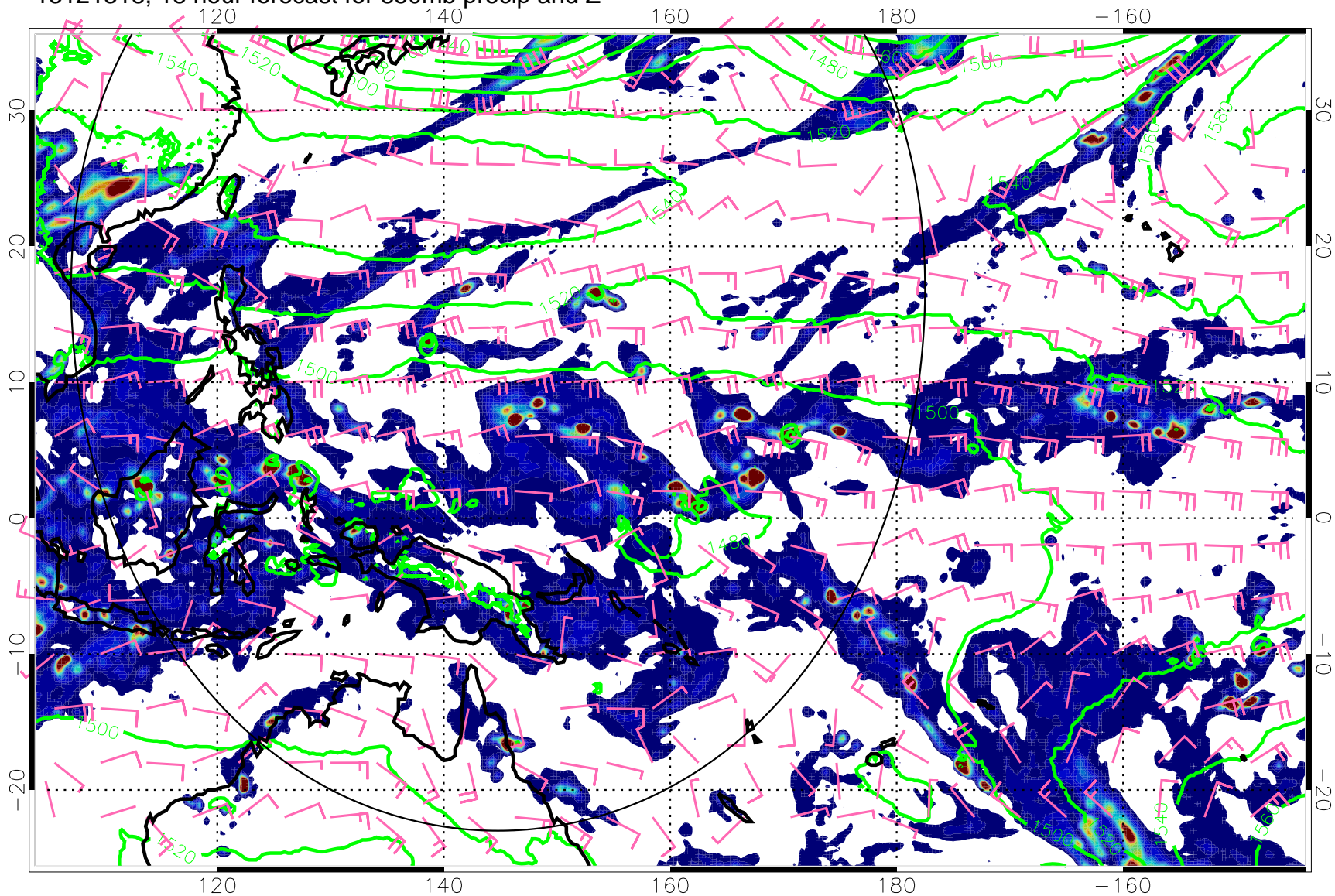
13121318, 18 hour forecast for 850mb precip and Z
