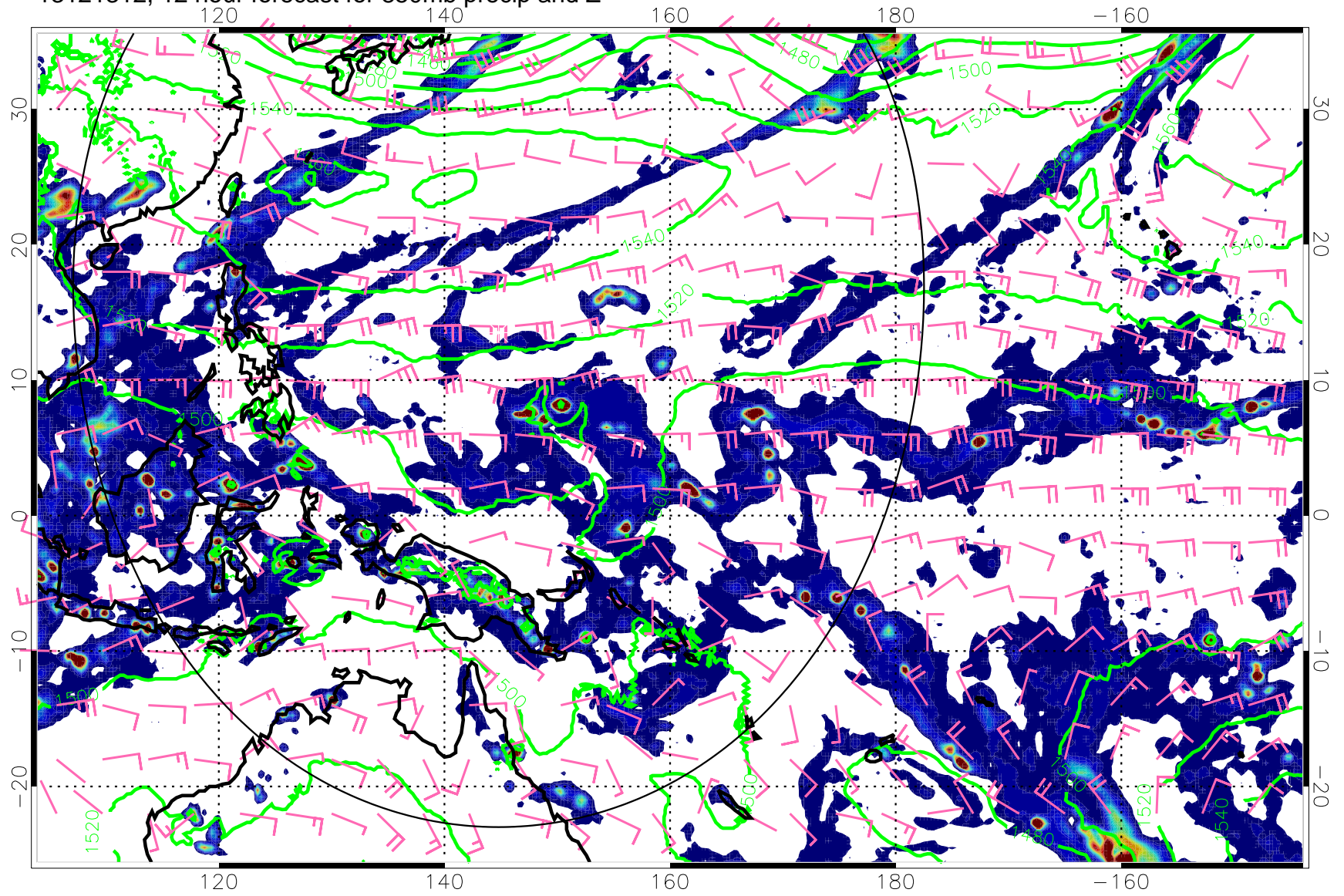
13121312, 12 hour forecast for 850mb precip and Z
