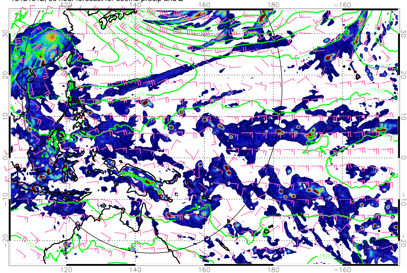
13121512, 60 hour forecast for 850mb precip and Z
