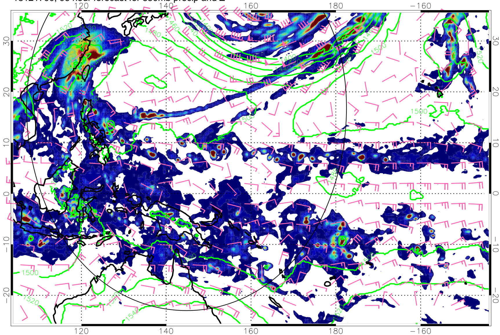
13121700, 96 hour forecast for 850mb precip and Z
