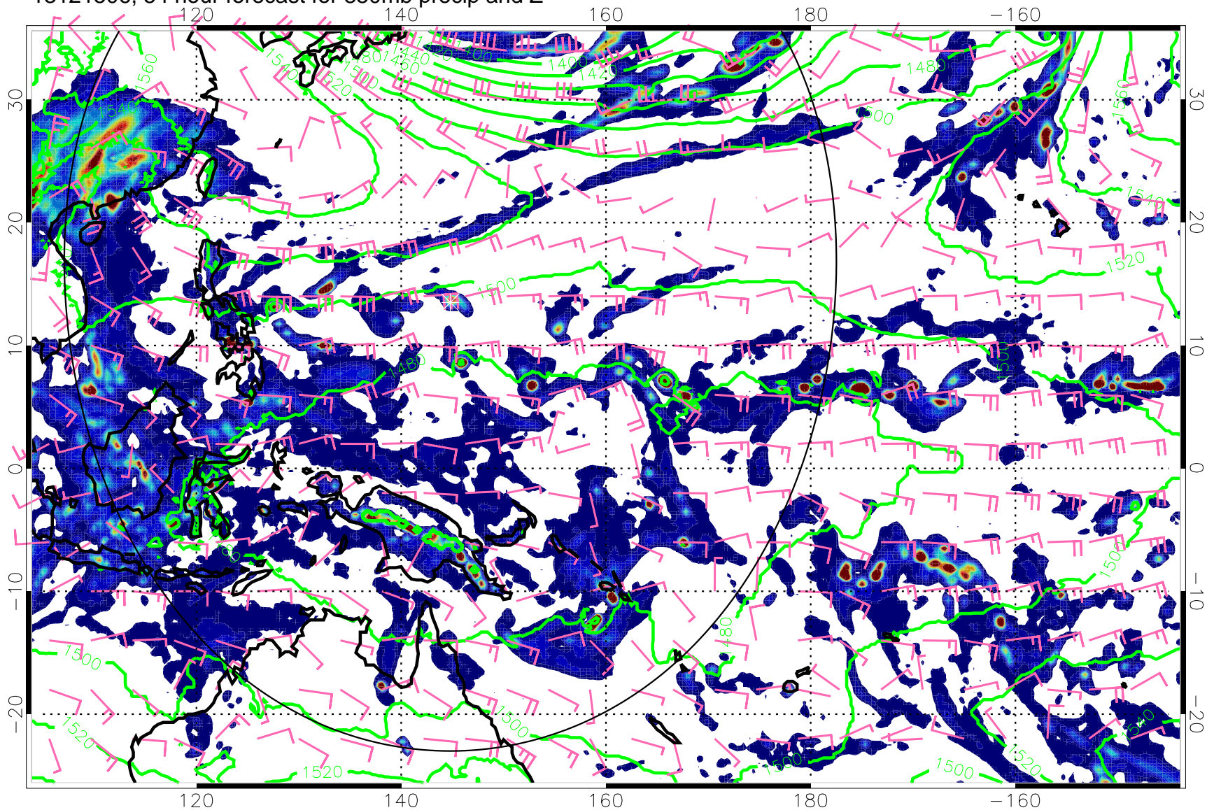
13121506, 54 hour forecast for 850mb precip and Z
