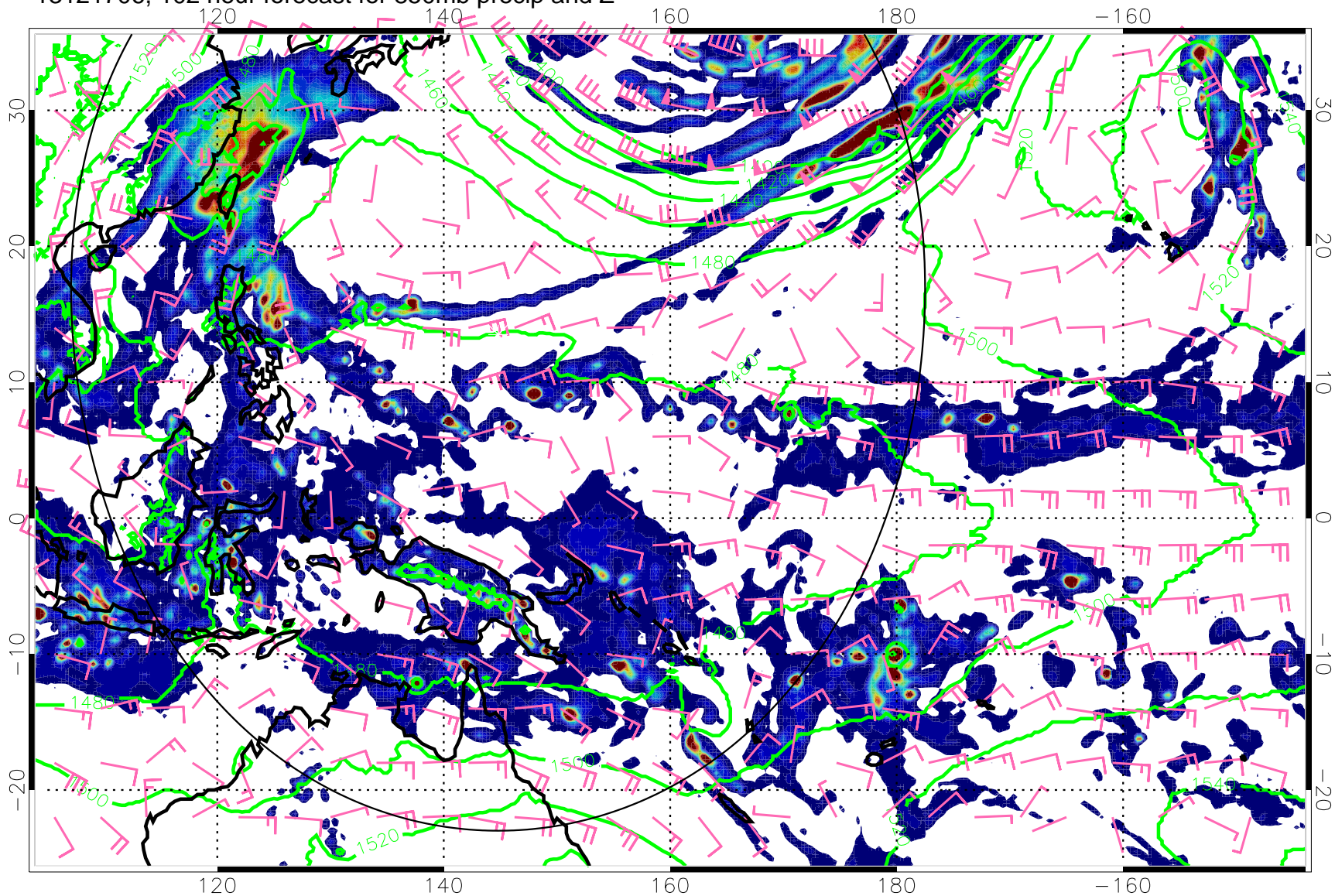
13121706, 102 hour forecast for 850mb precip and Z
