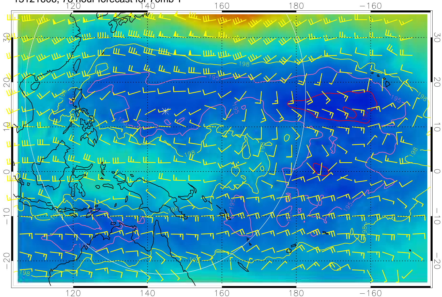
13121606, 78 hour forecast for 70mb T
