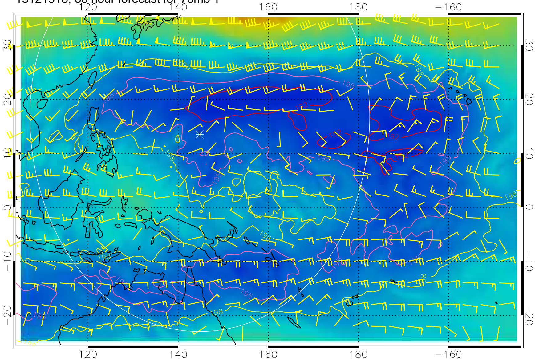
13121518, 66 hour forecast for 70mb T
