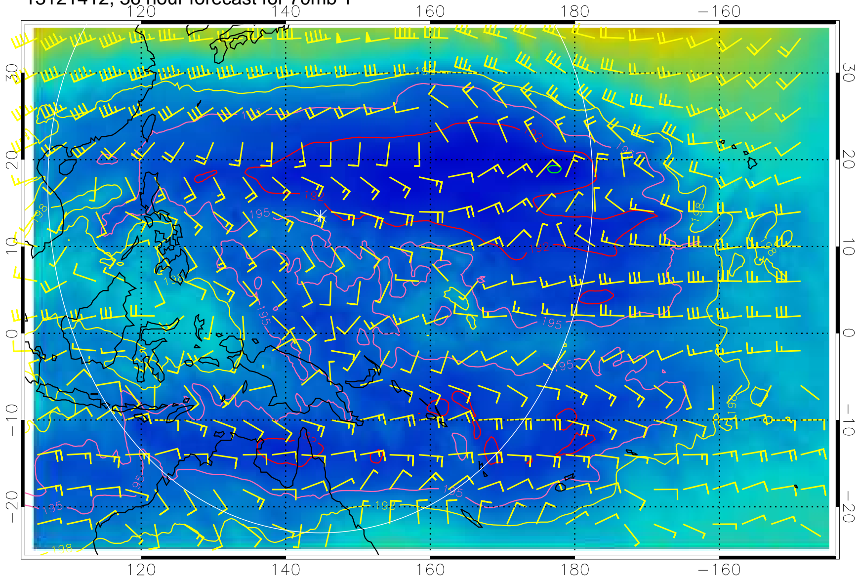
13121412, 36 hour forecast for 70mb T
