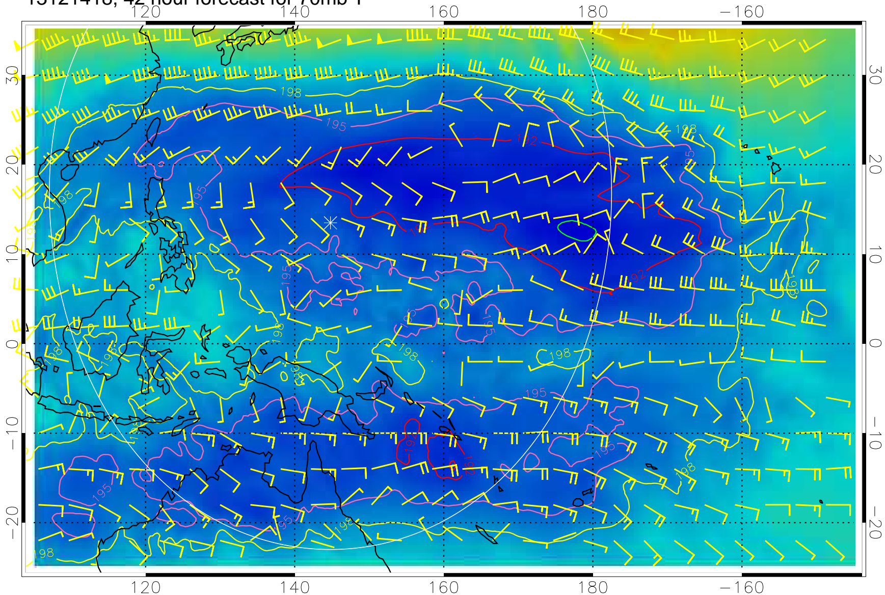
13121418, 42 hour forecast for 70mb T
