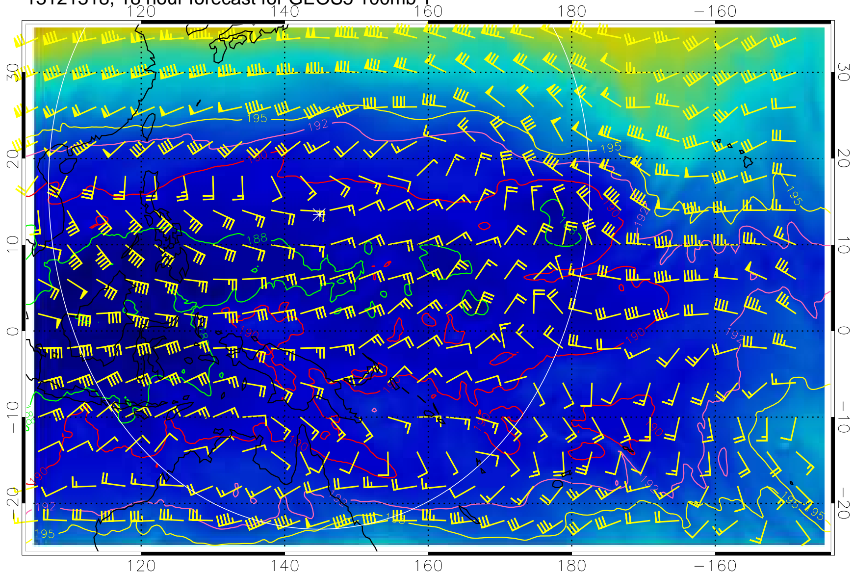
13121318, 18 hour forecast for GEOS5 100mb T
