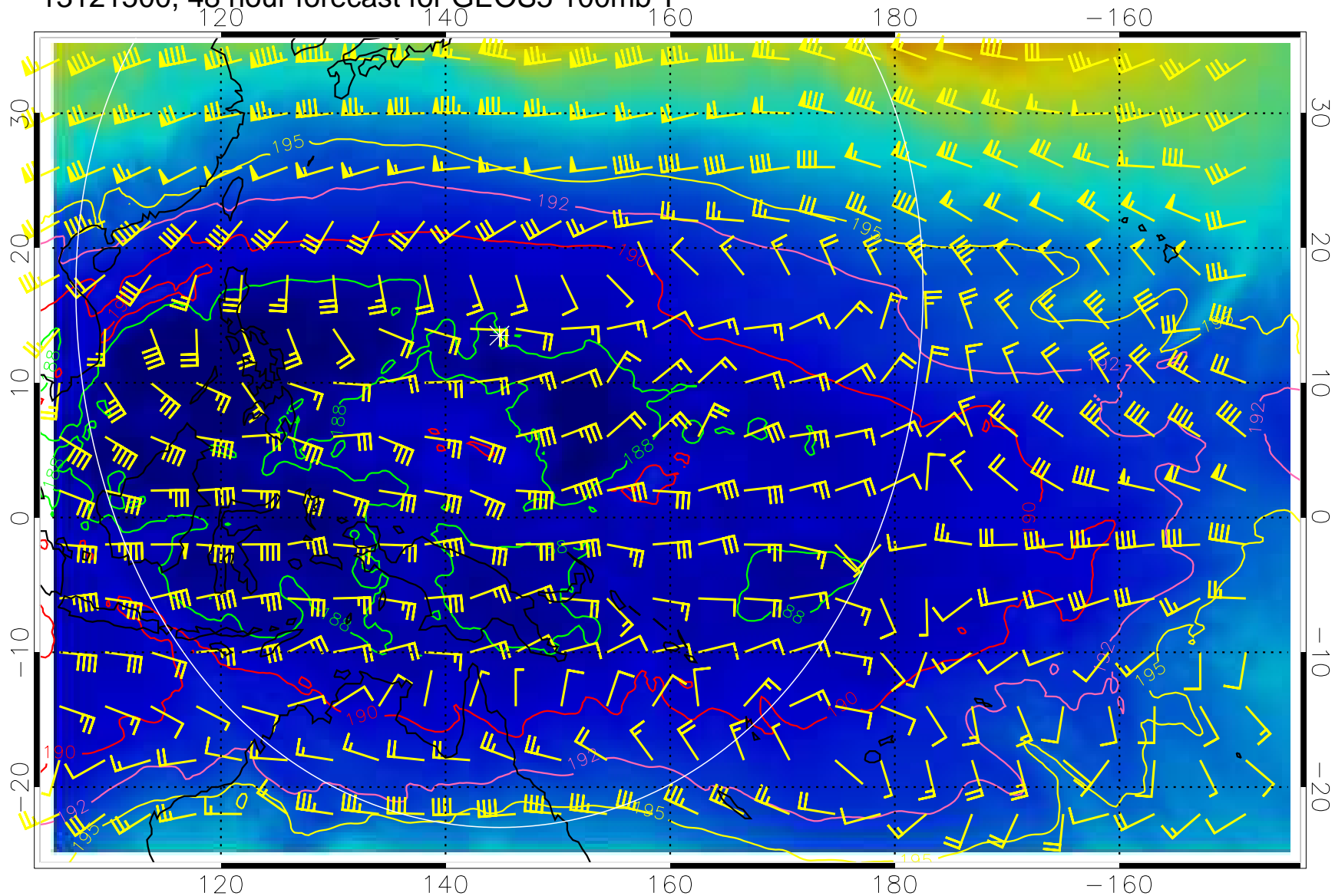
13121500, 48 hour forecast for GEOS5 100mb T
