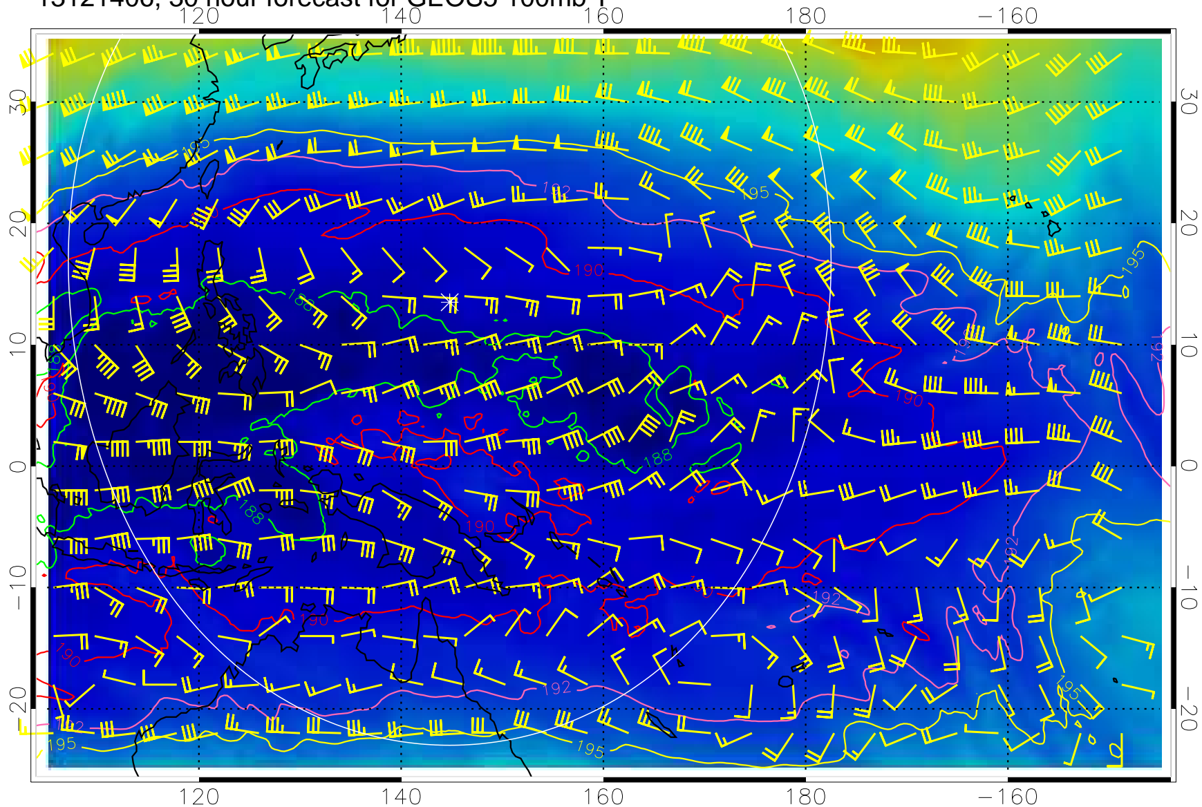
13121406, 30 hour forecast for GEOS5 100mb T
