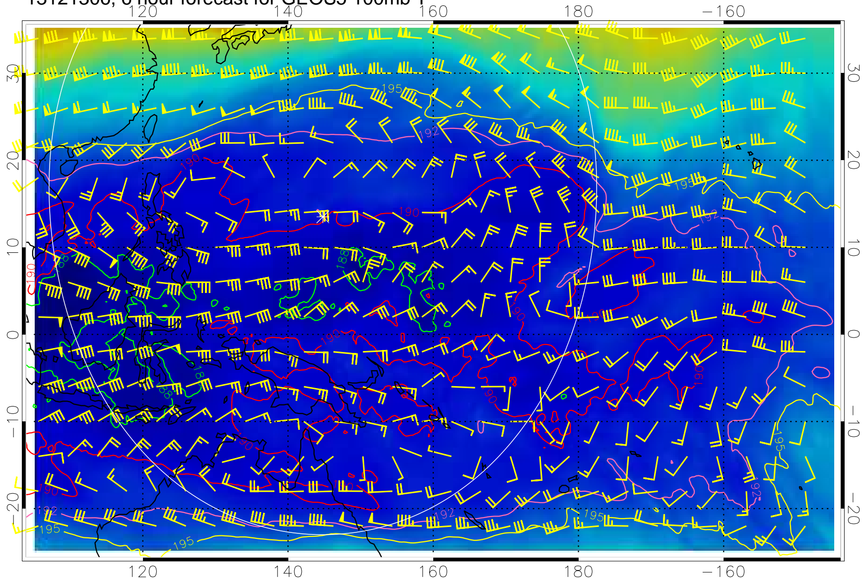
13121306, 6 hour forecast for GEOS5 100mb T
