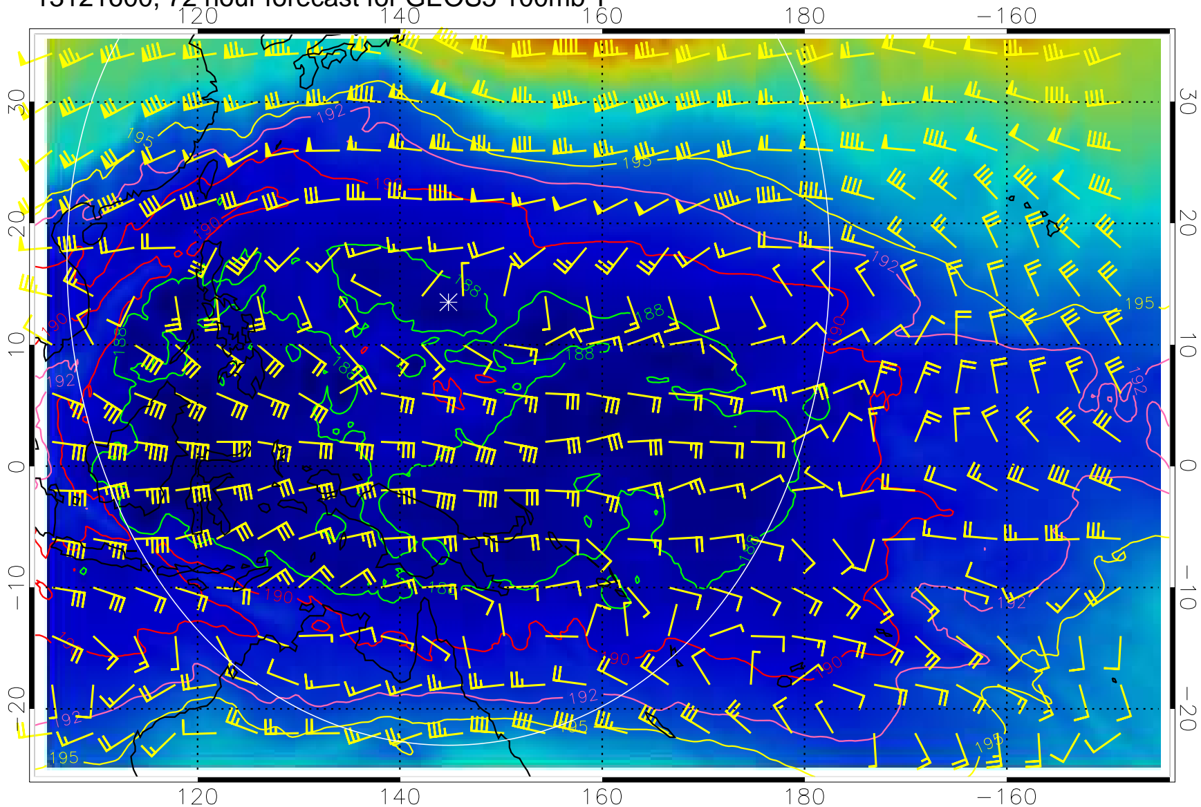
13121600, 72 hour forecast for GEOS5 100mb T
