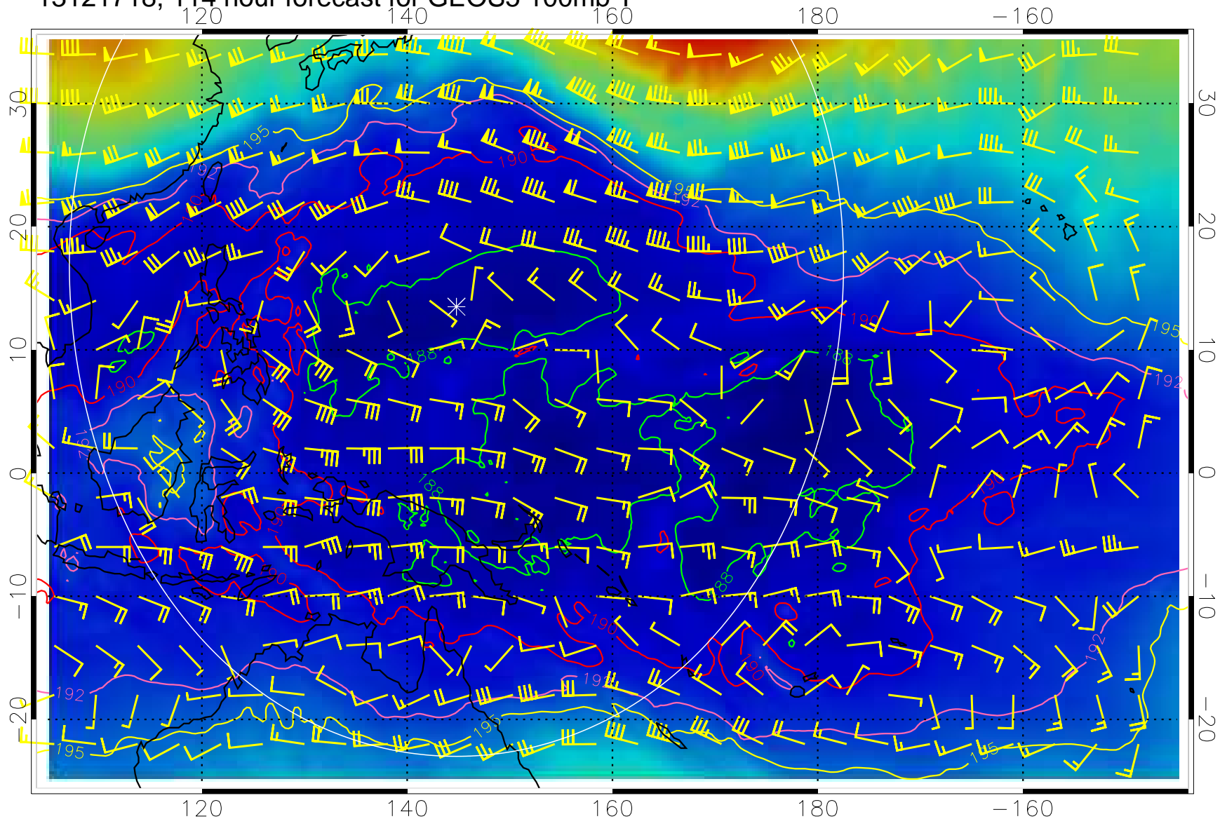
13121718, 114 hour forecast for GEOS5 100mb T
