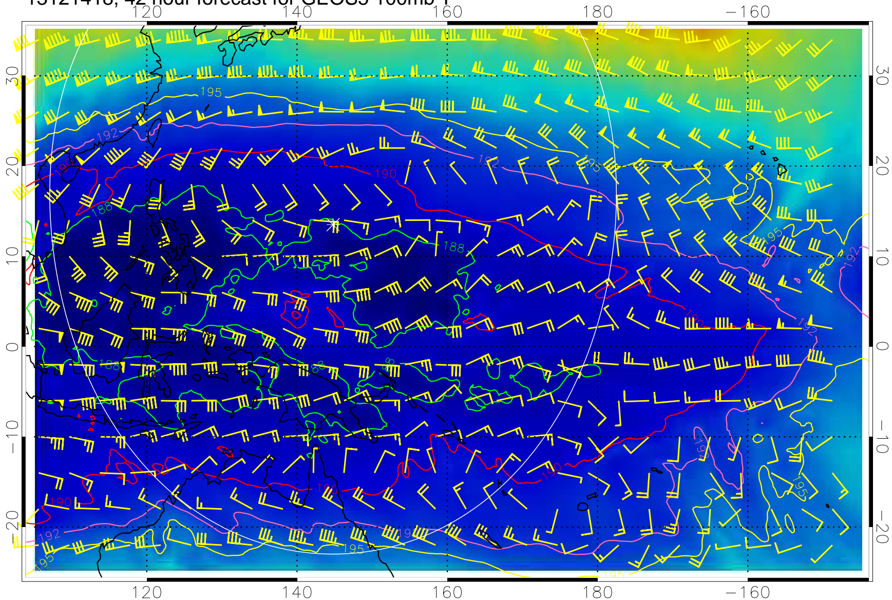
13121418, 42 hour forecast for GEOS5 100mb T
