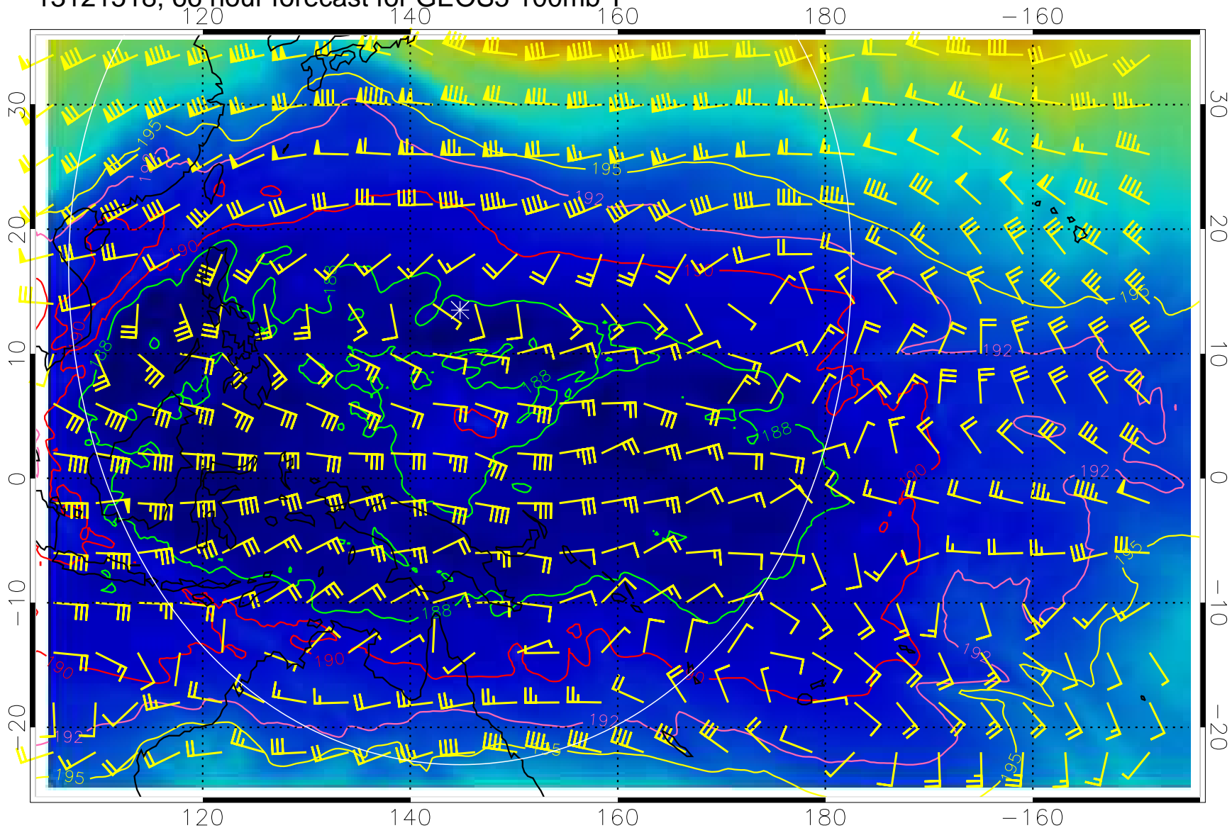
13121518, 66 hour forecast for GEOS5 100mb T
